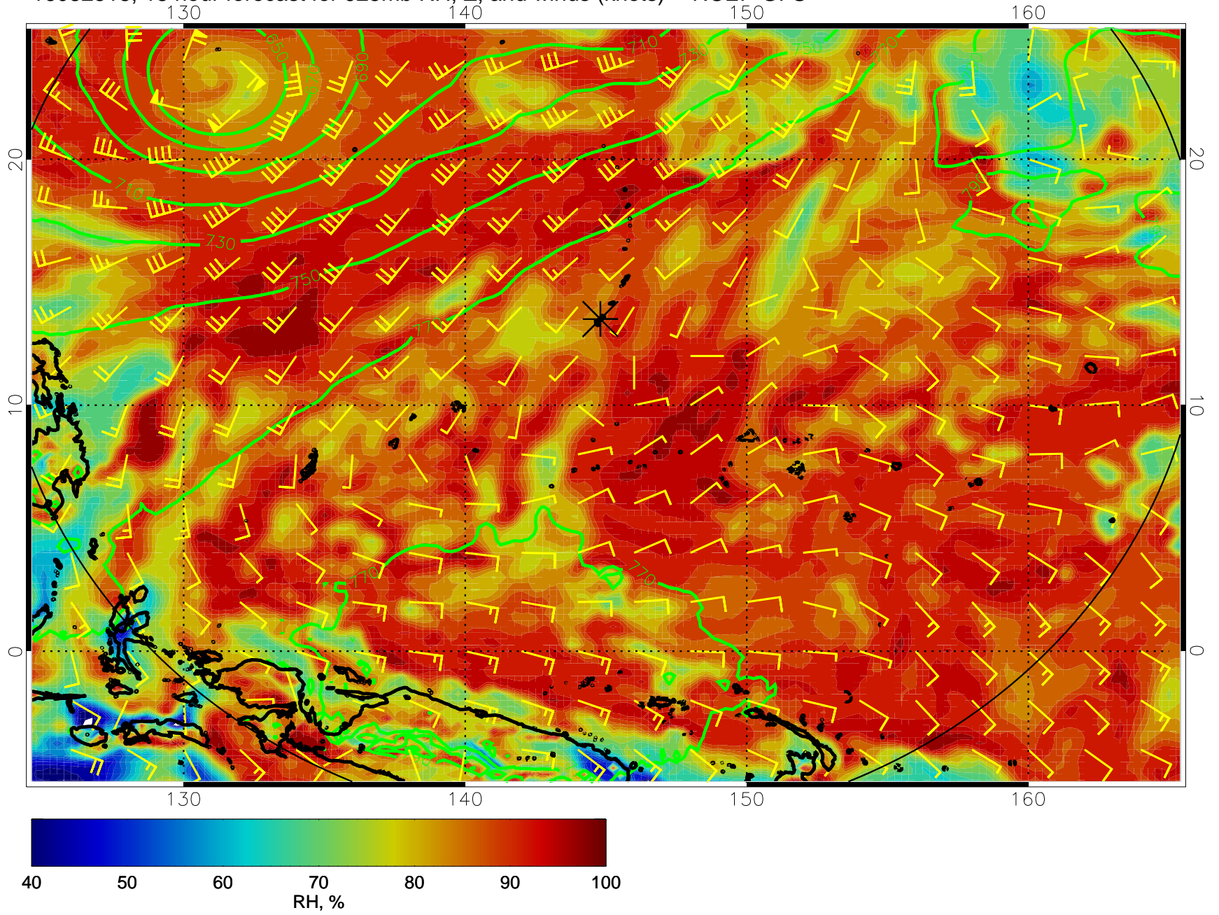
16082518, 18 hour forecast for 925mb RH, Z, and winds (knots) -- NCEP GFS
