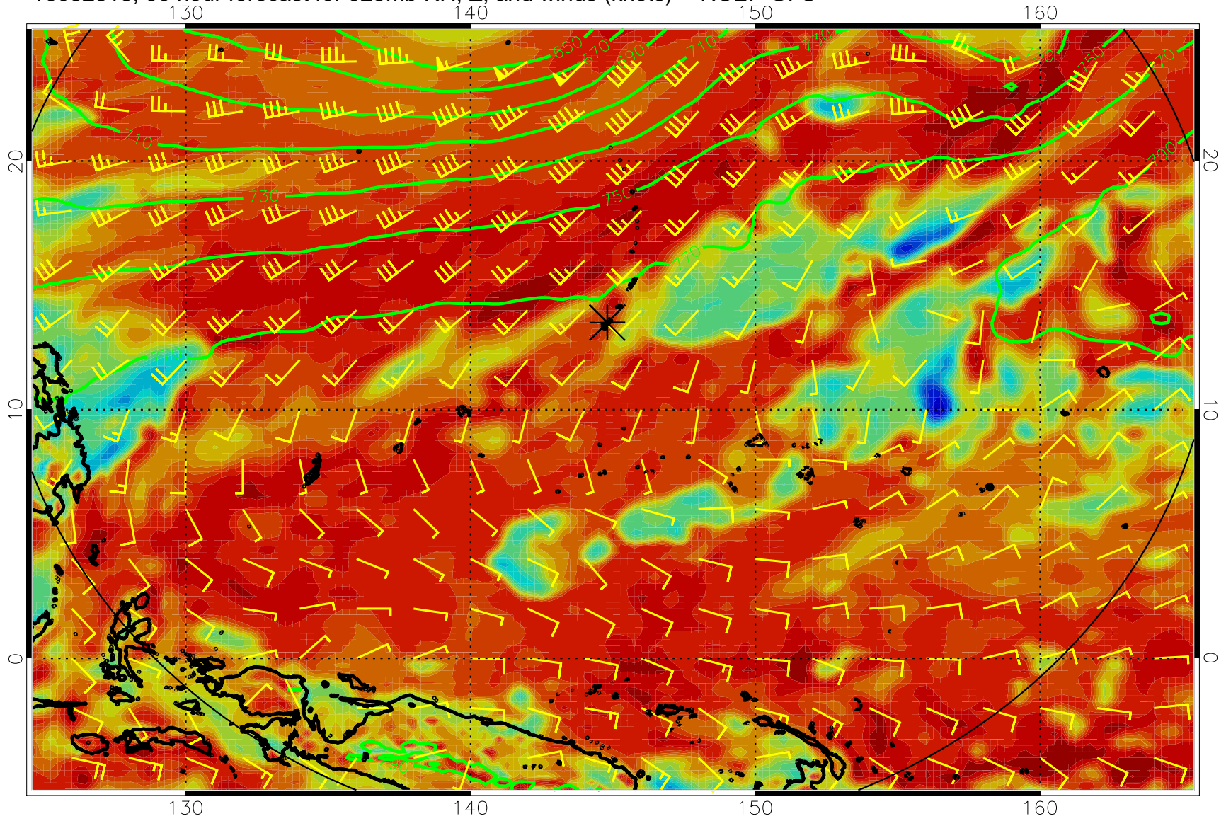
16082818, 90 hour forecast for 925mb RH, Z, and winds (knots) -- NCEP GFS
