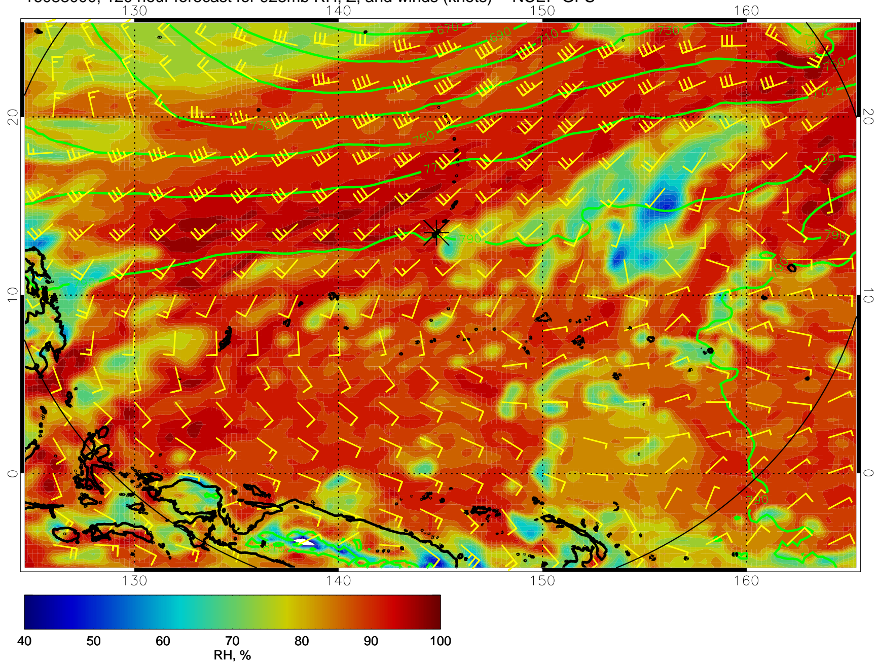
16083000, 120 hour forecast for 925mb RH, Z, and winds (knots) -- NCEP GFS
