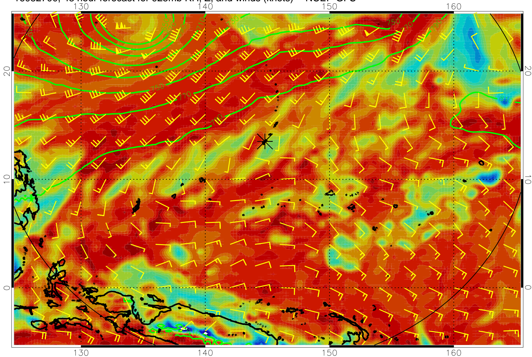
16082700, 48 hour forecast for 925mb RH, Z, and winds (knots) -- NCEP GFS
