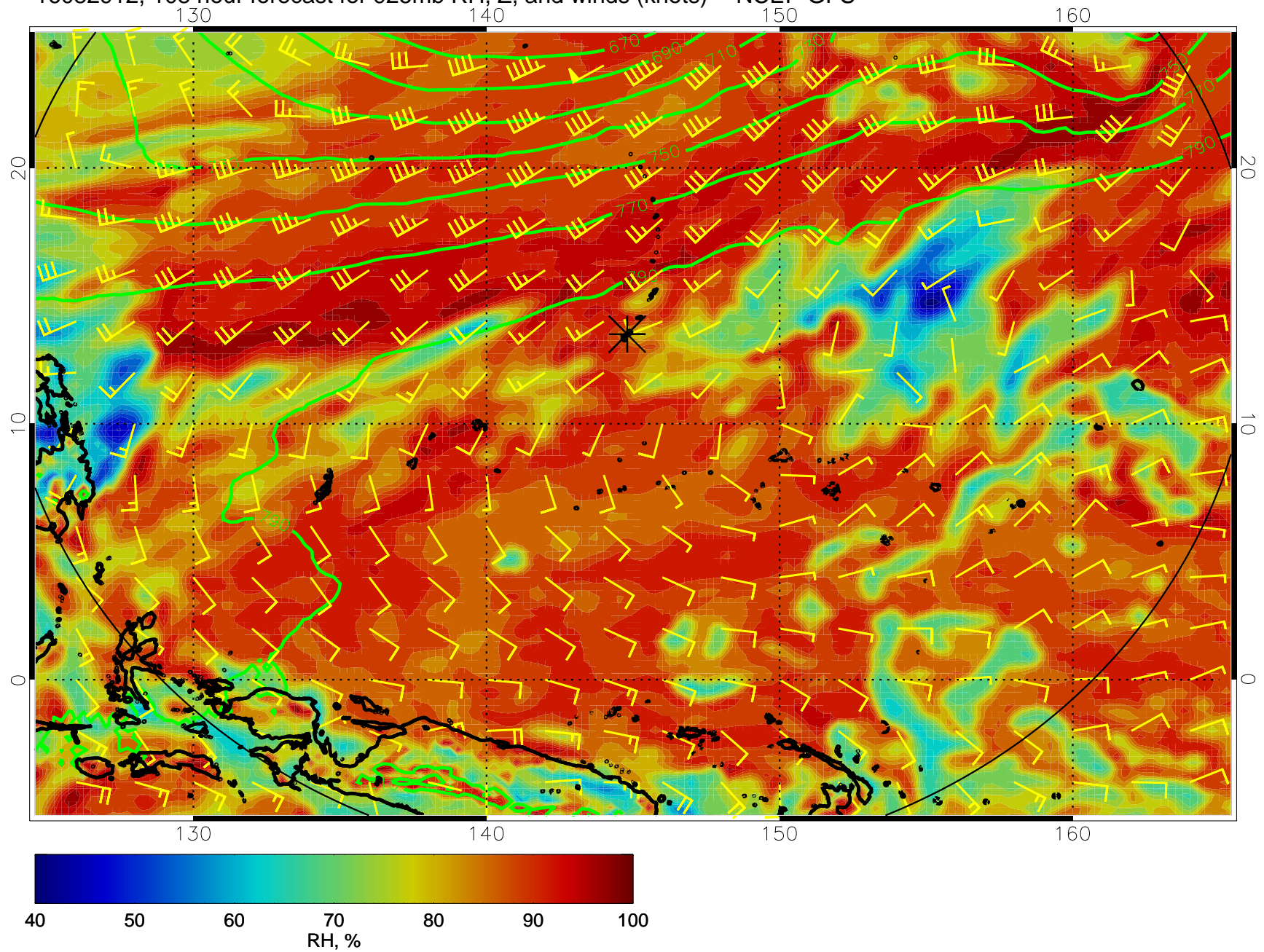
16082912, 108 hour forecast for 925mb RH, Z, and winds (knots) -- NCEP GFS
