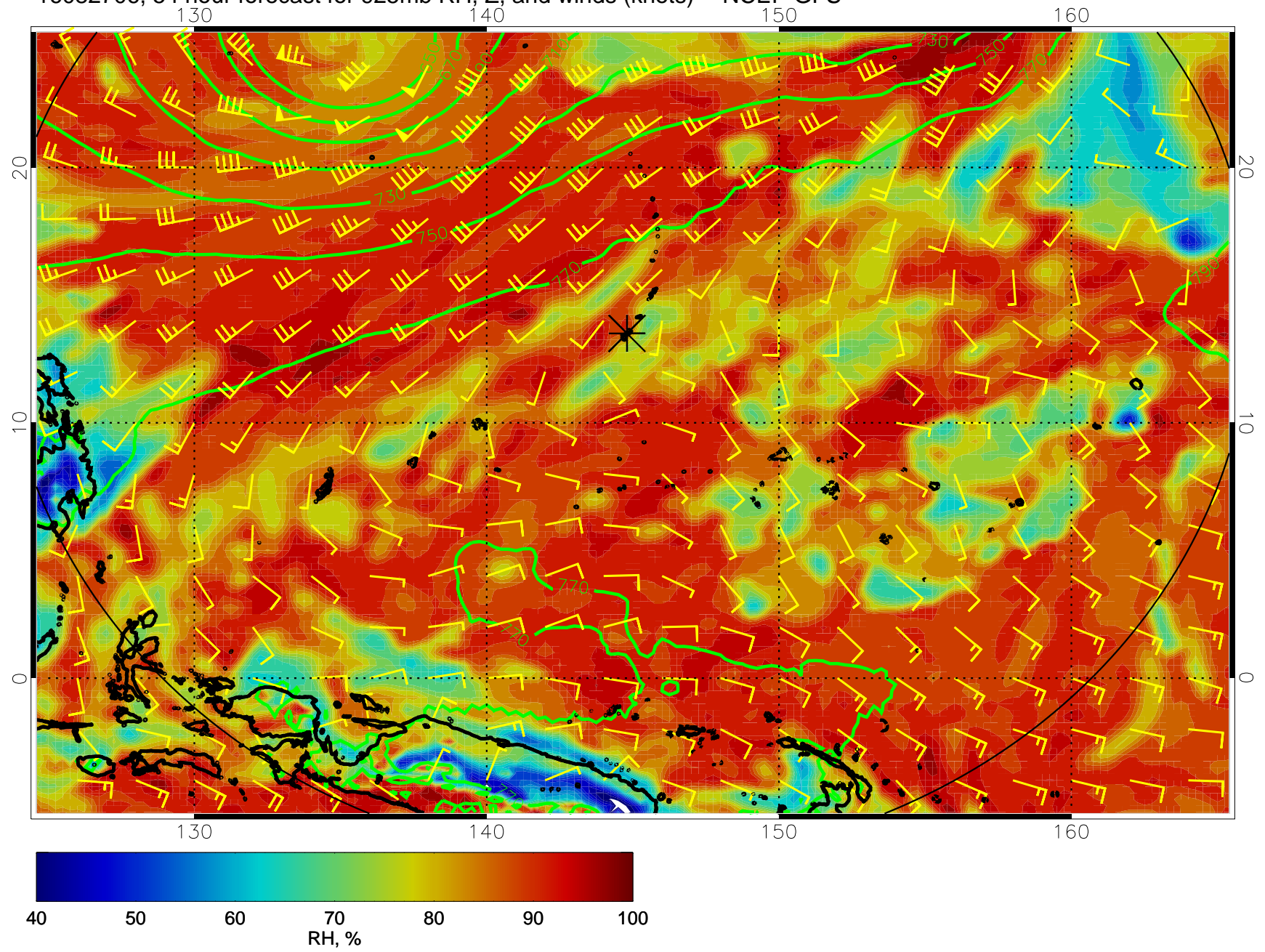
16082706, 54 hour forecast for 925mb RH, Z, and winds (knots) -- NCEP GFS
