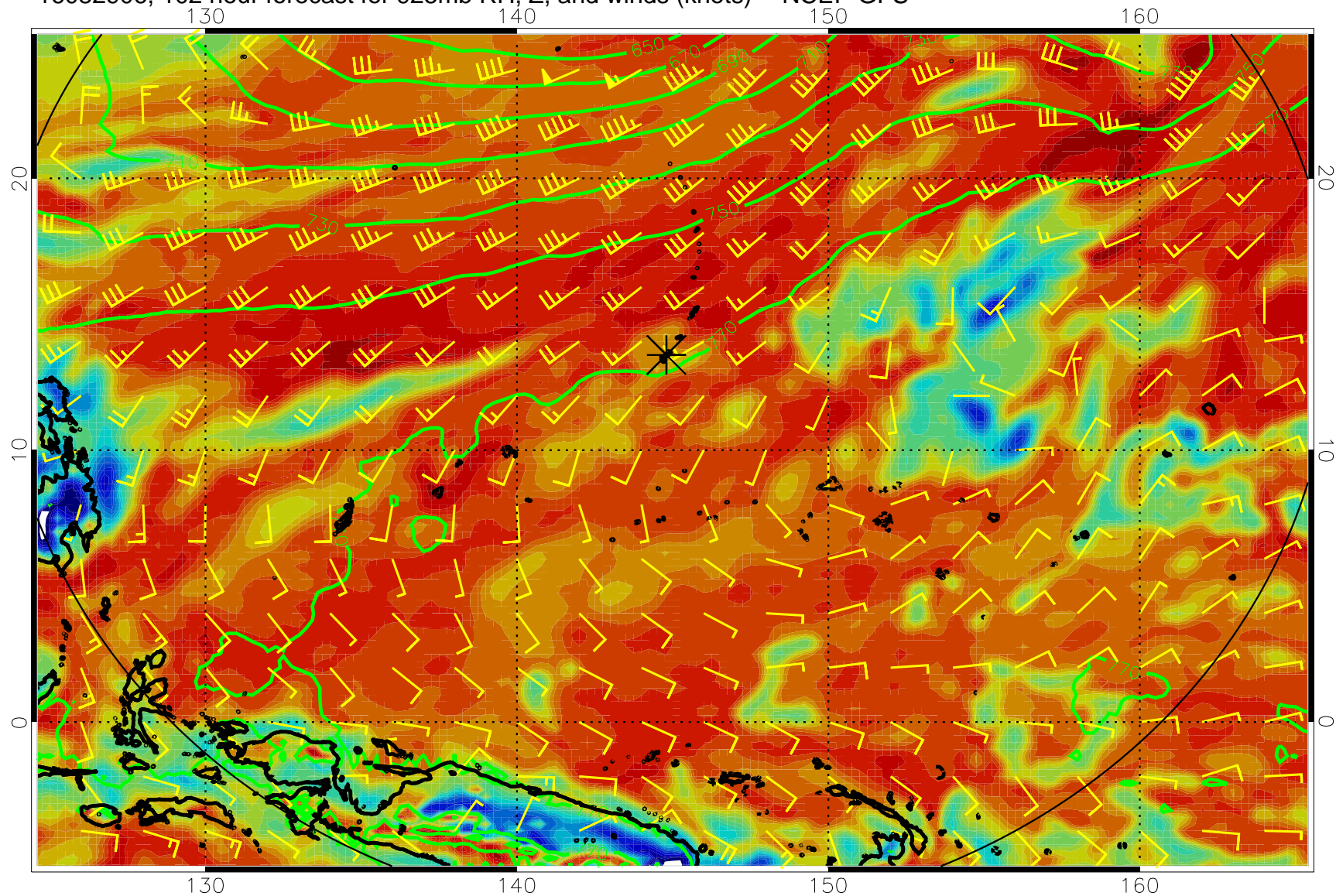
16082906, 102 hour forecast for 925mb RH, Z, and winds (knots) -- NCEP GFS
