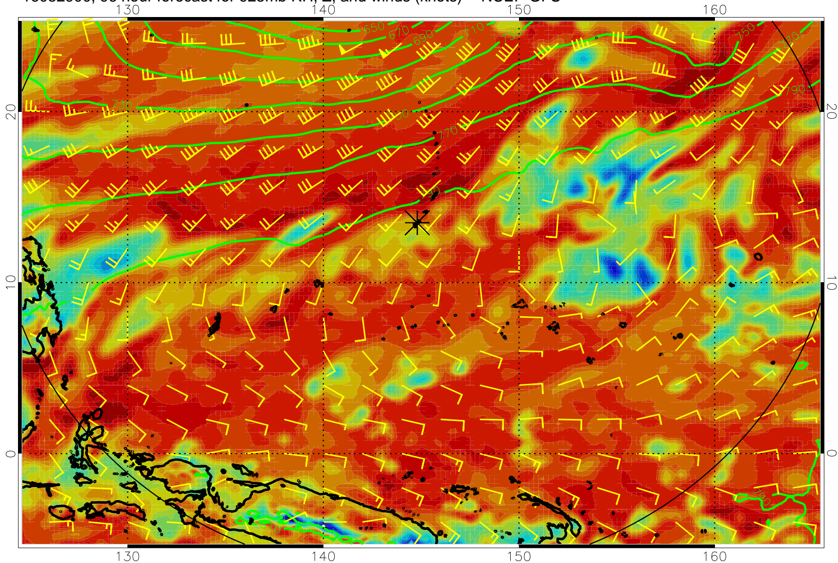
16082900, 96 hour forecast for 925mb RH, Z, and winds (knots) -- NCEP GFS
