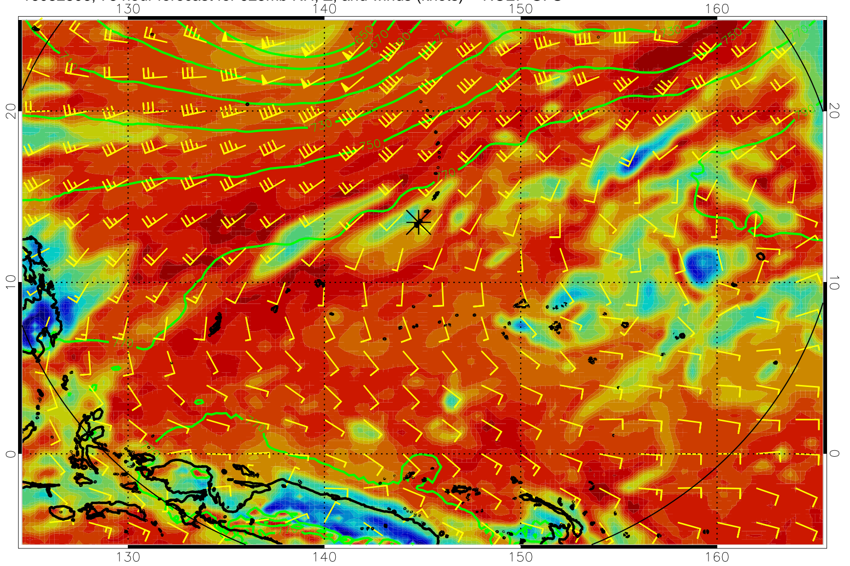
16082806, 78 hour forecast for 925mb RH, Z, and winds (knots) -- NCEP GFS
