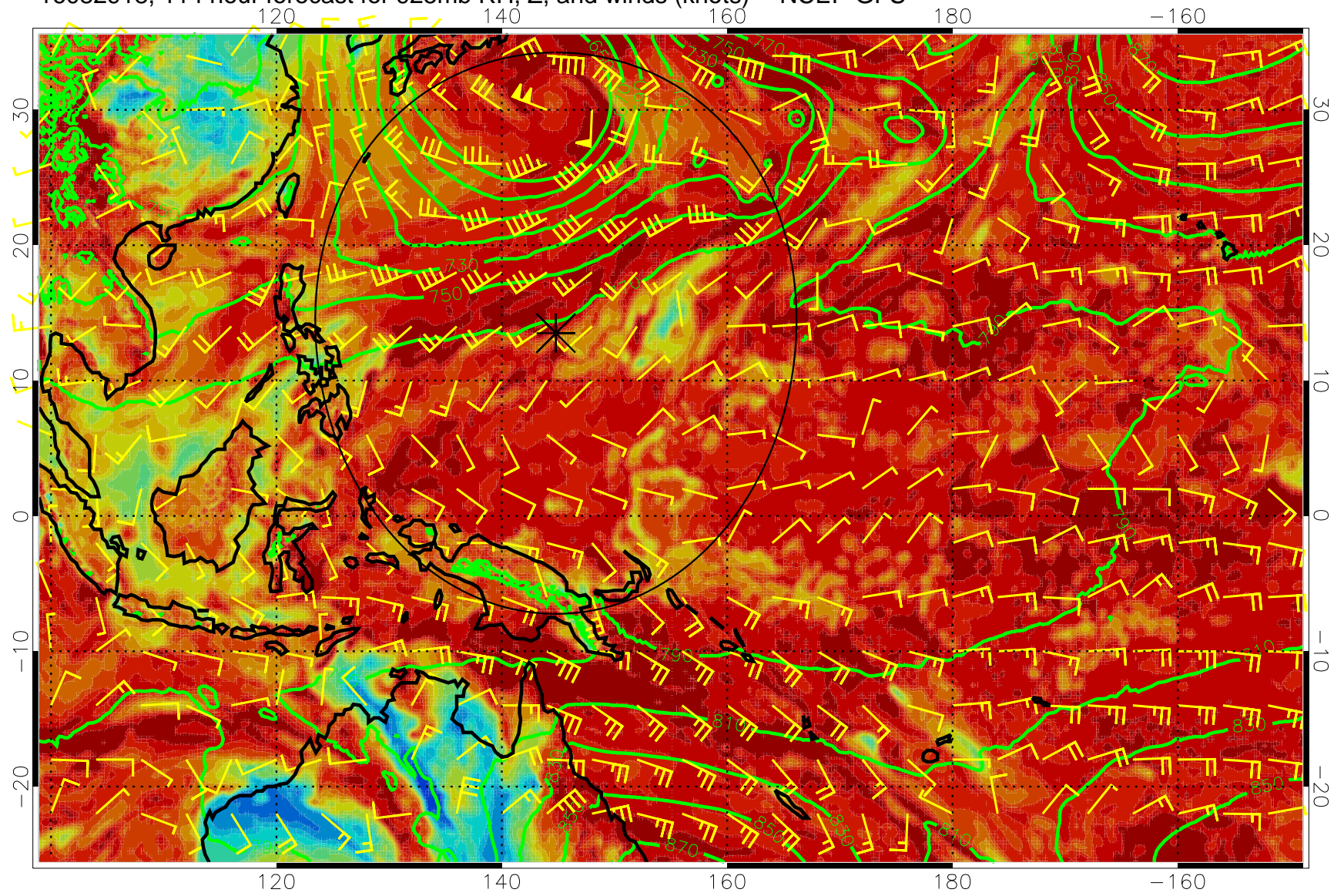
16082918, 114 hour forecast for 925mb RH, Z, and winds (knots) -- NCEP GFS
