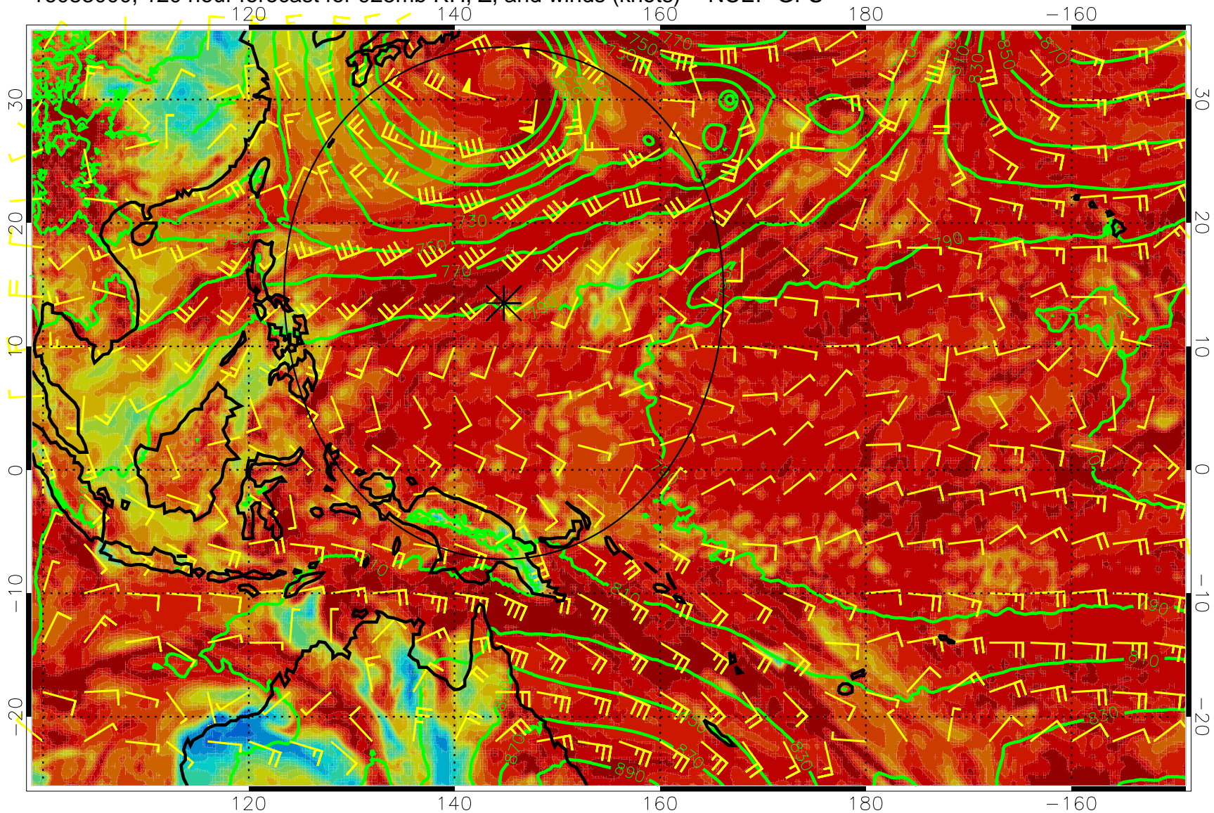
16083000, 120 hour forecast for 925mb RH, Z, and winds (knots) -- NCEP GFS
