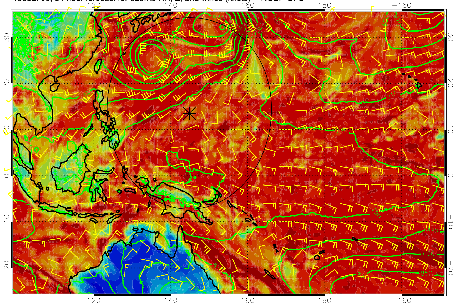
16082706, 54 hour forecast for 925mb RH, Z, and winds (knots) -- NCEP GFS
