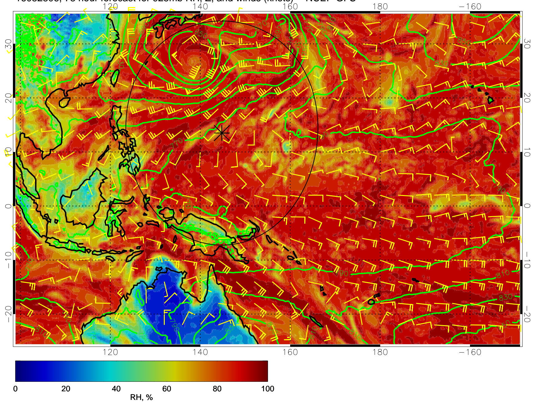
16082806, 78 hour forecast for 925mb RH, Z, and winds (knots) -- NCEP GFS
