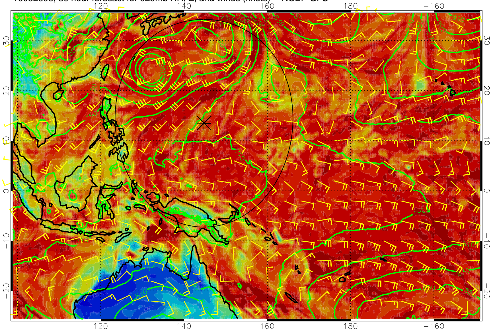
16082606, 30 hour forecast for 925mb RH, Z, and winds (knots) -- NCEP GFS
