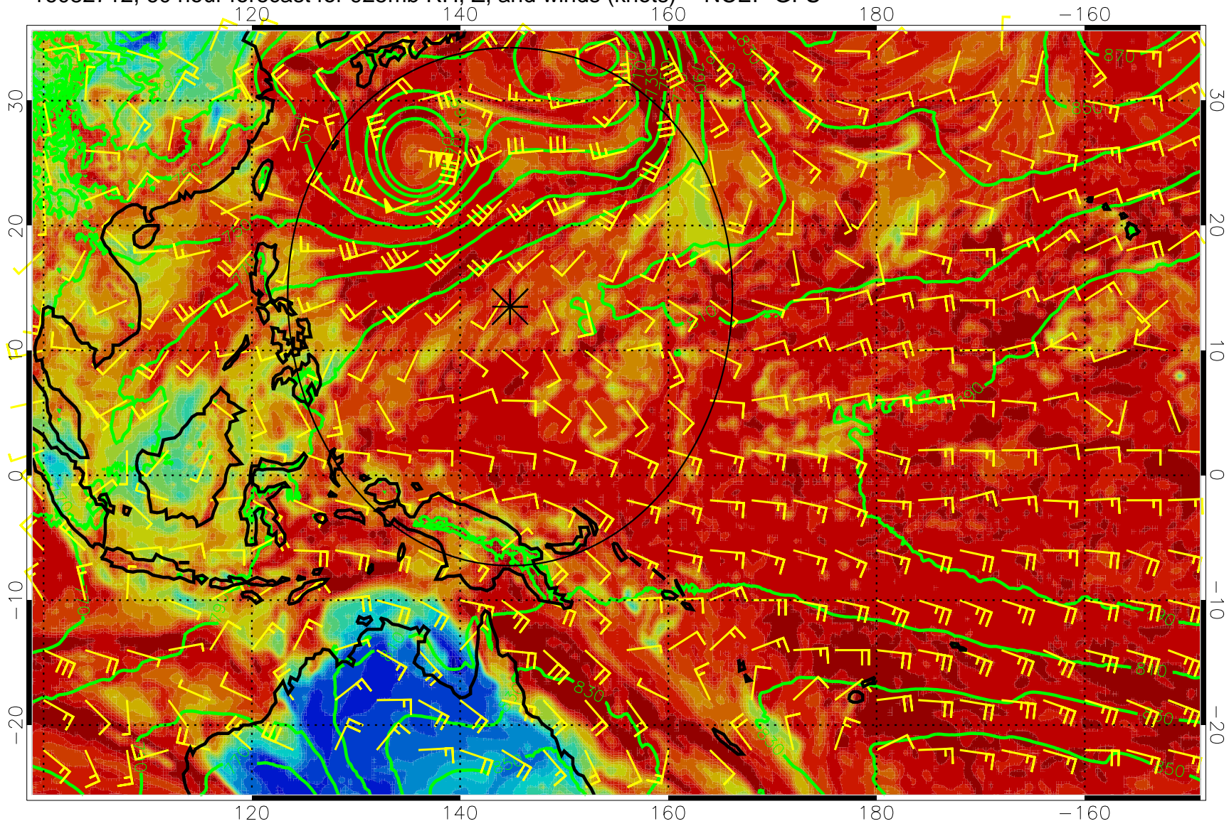
16082712, 60 hour forecast for 925mb RH, Z, and winds (knots) -- NCEP GFS
