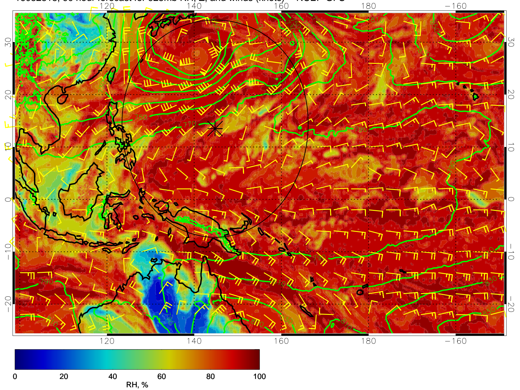
16082818, 90 hour forecast for 925mb RH, Z, and winds (knots) -- NCEP GFS
