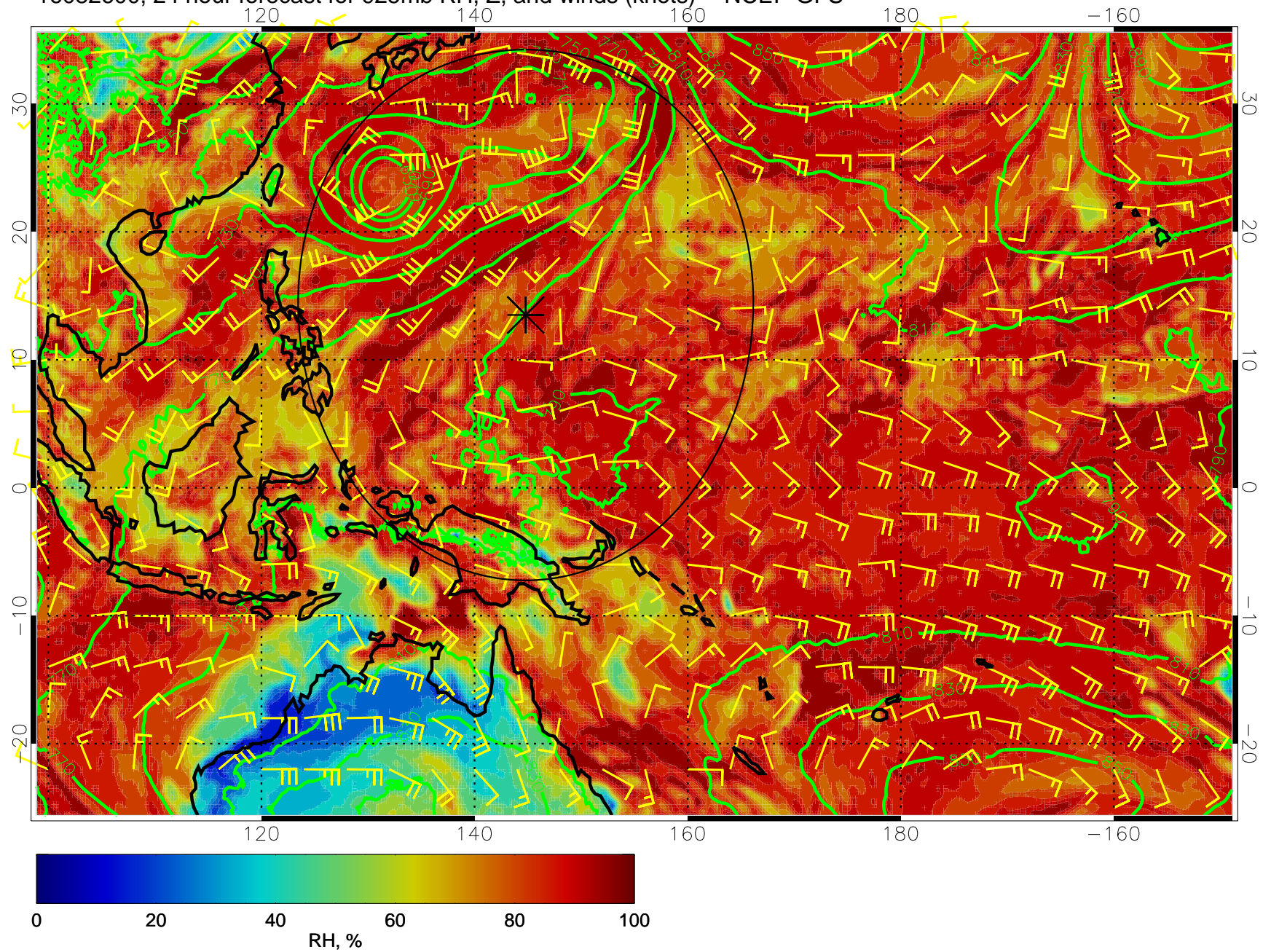
16082600, 24 hour forecast for 925mb RH, Z, and winds (knots) -- NCEP GFS
