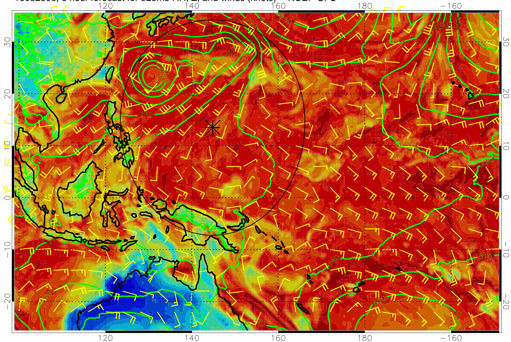
16082506, 6 hour forecast for 925mb RH, Z, and winds (knots) -- NCEP GFS
