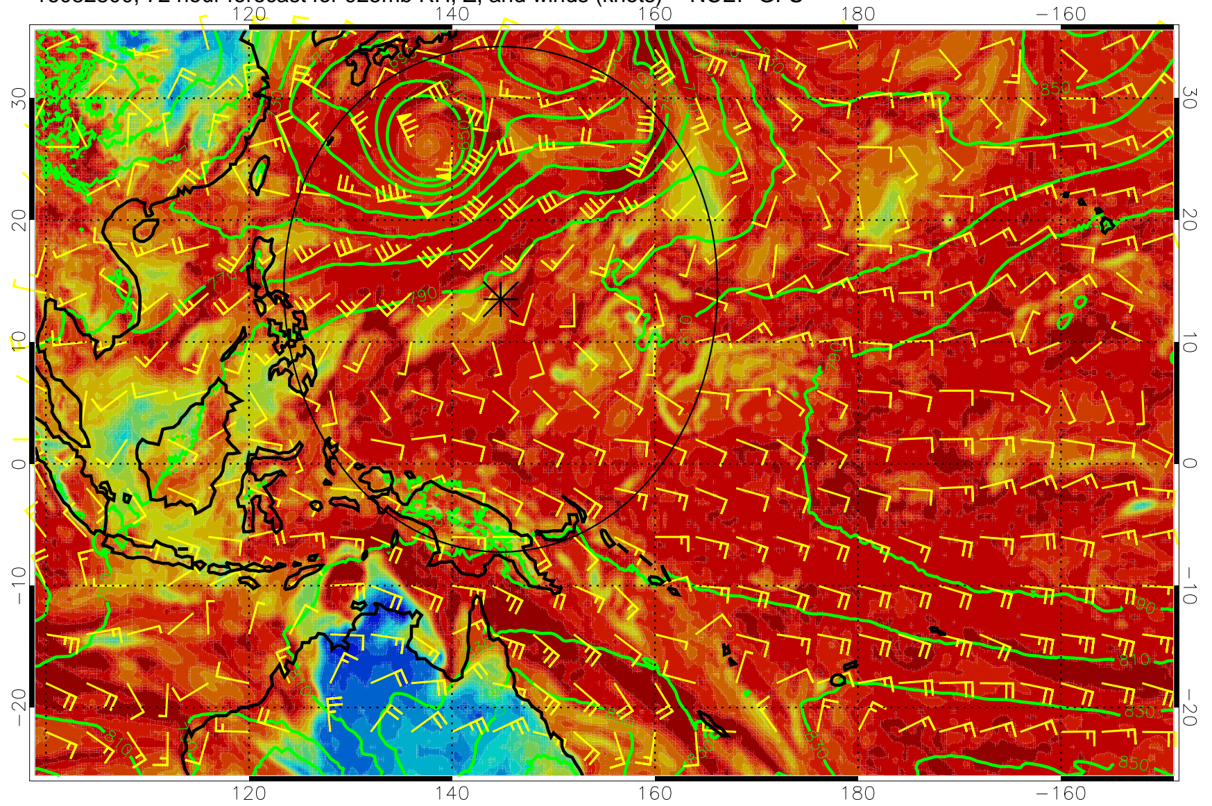
16082800, 72 hour forecast for 925mb RH, Z, and winds (knots) -- NCEP GFS
