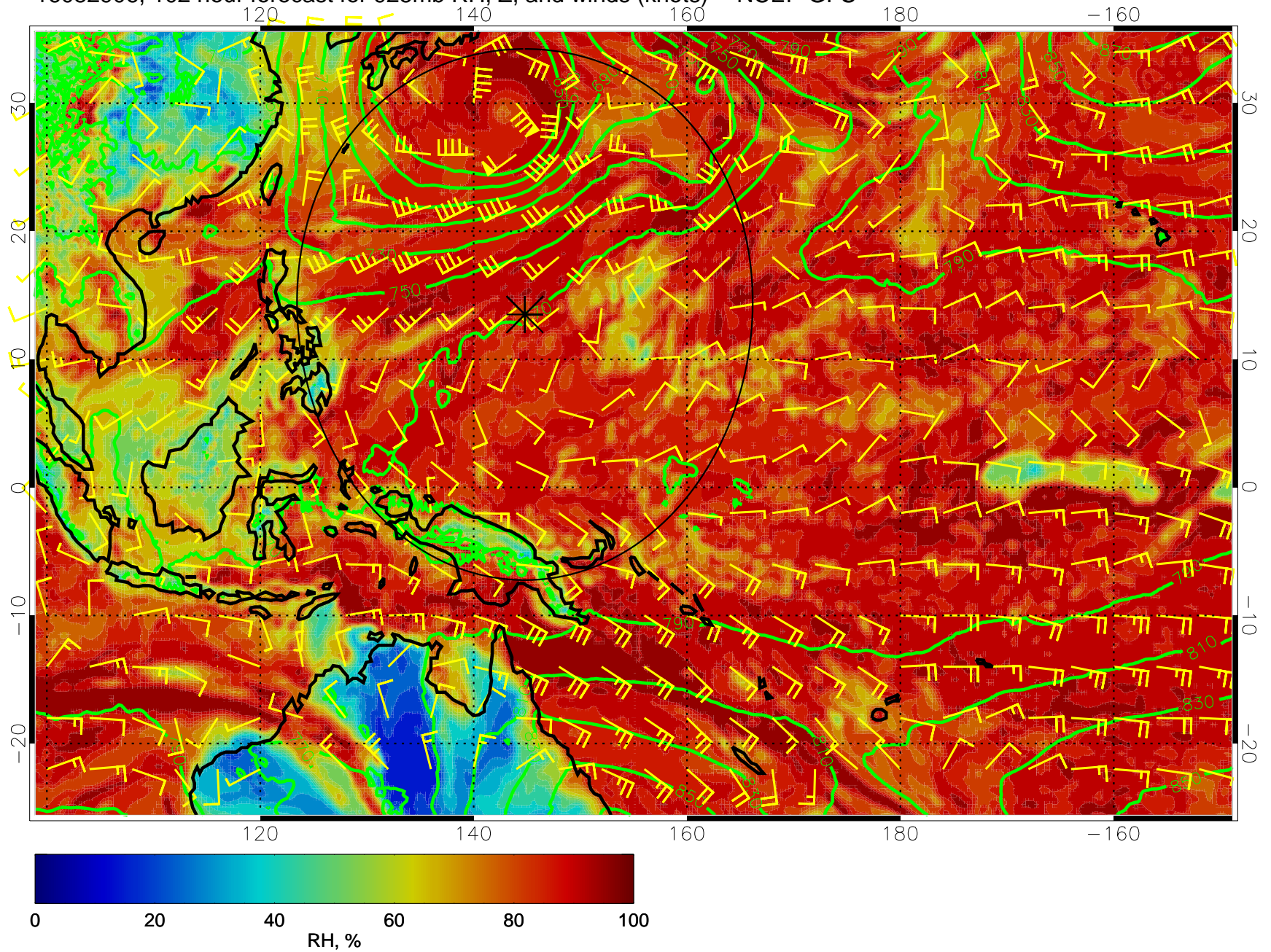
16082906, 102 hour forecast for 925mb RH, Z, and winds (knots) -- NCEP GFS
