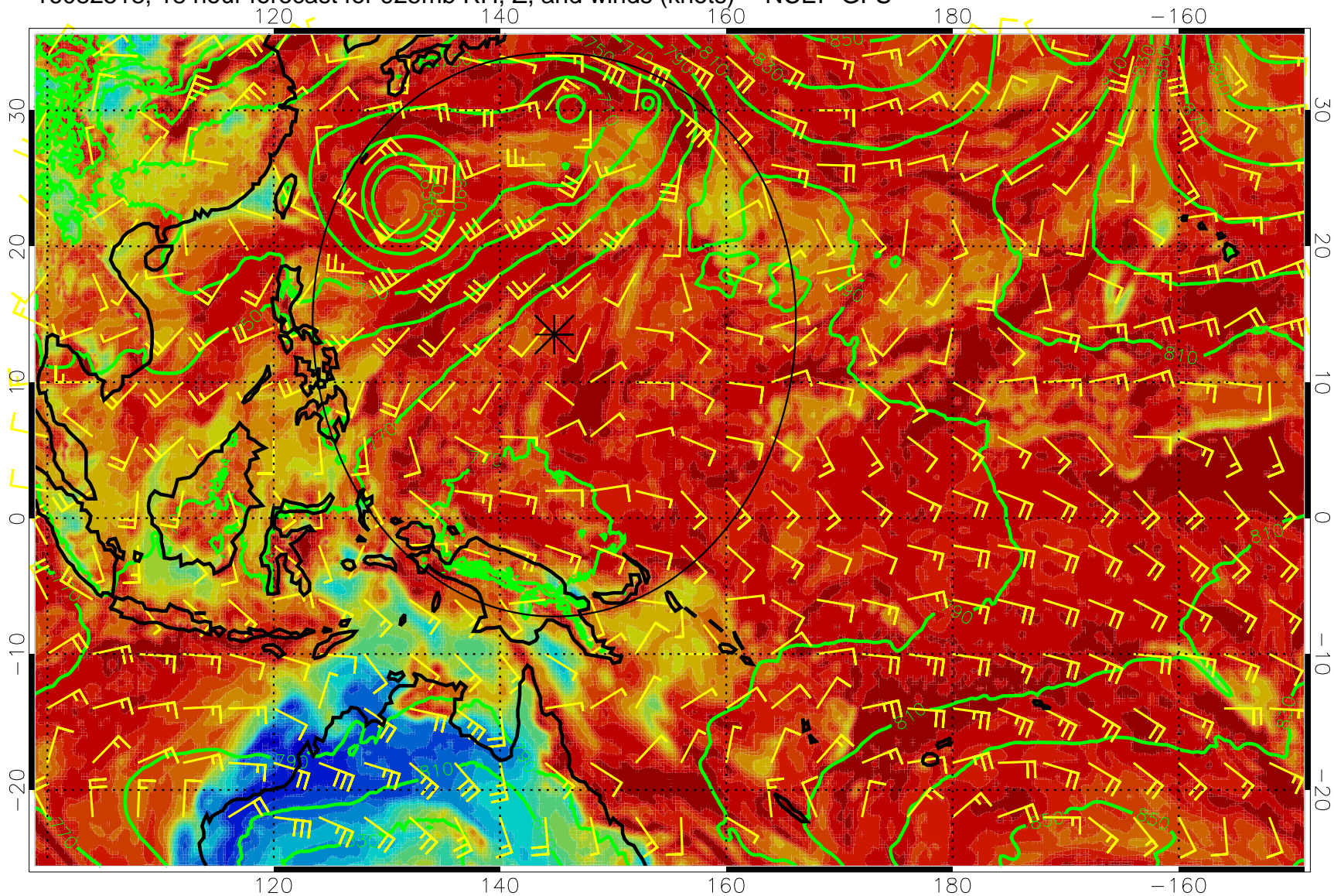
16082518, 18 hour forecast for 925mb RH, Z, and winds (knots) -- NCEP GFS
