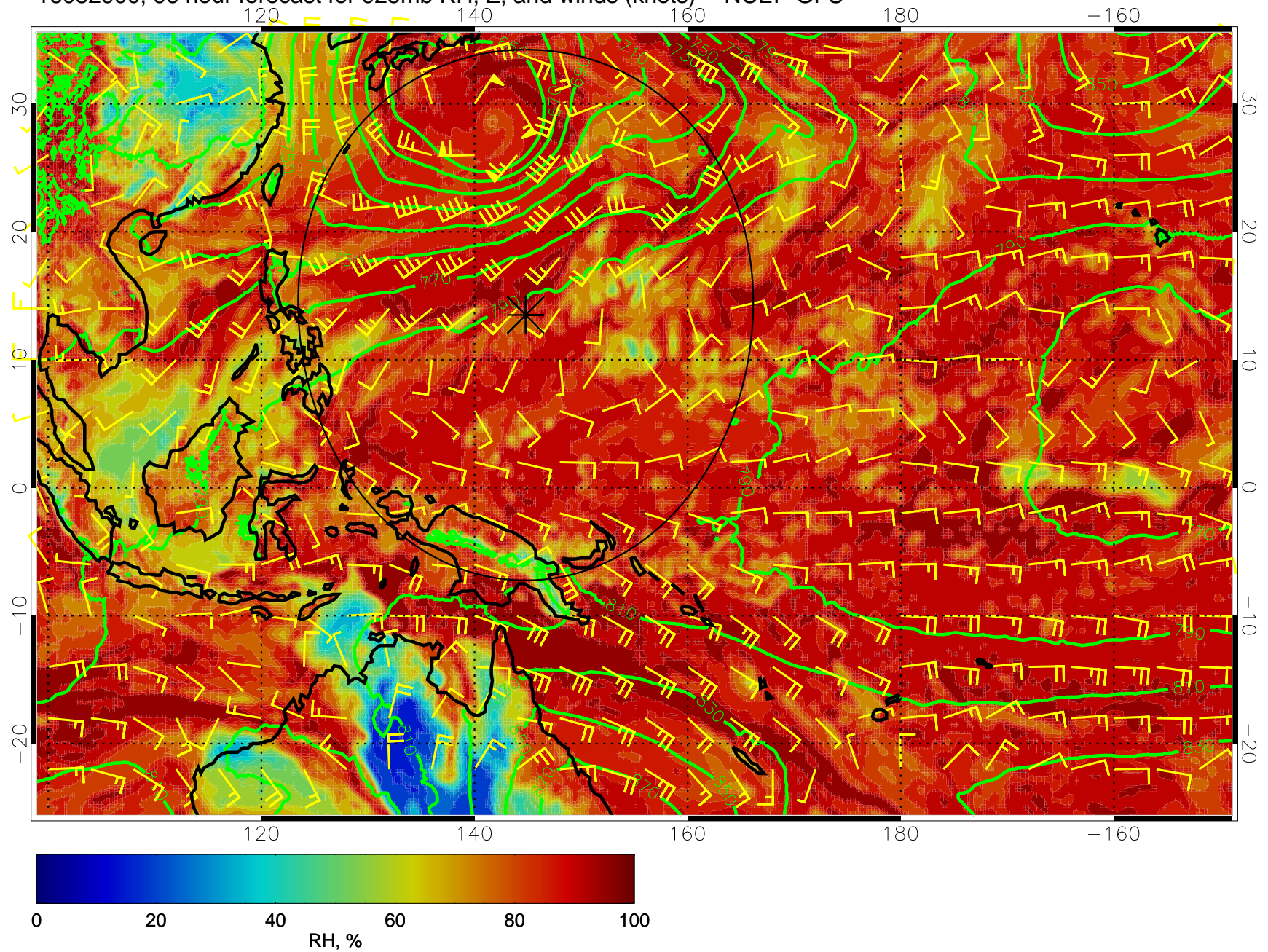
16082900, 96 hour forecast for 925mb RH, Z, and winds (knots) -- NCEP GFS
