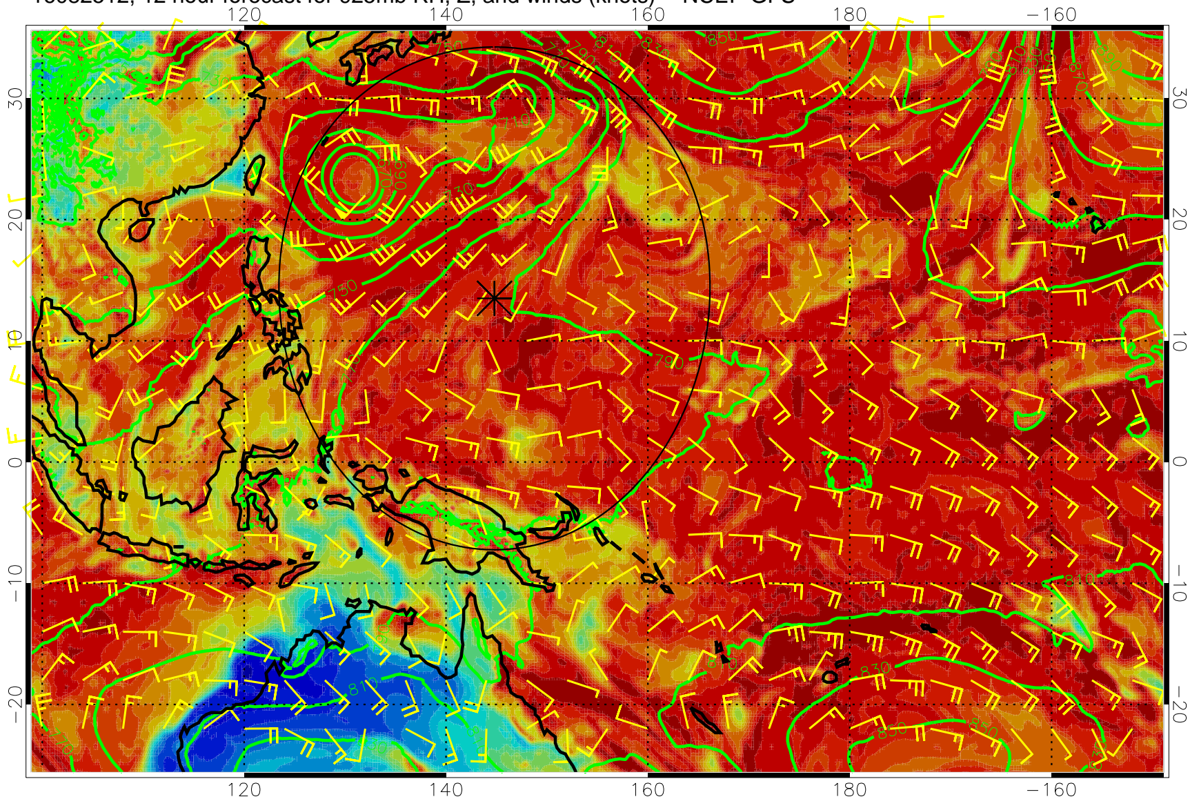
16082512, 12 hour forecast for 925mb RH, Z, and winds (knots) -- NCEP GFS
