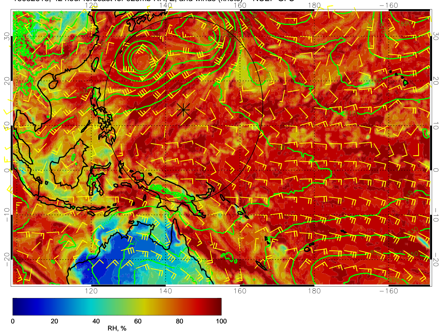
16082618, 42 hour forecast for 925mb RH, Z, and winds (knots) -- NCEP GFS
