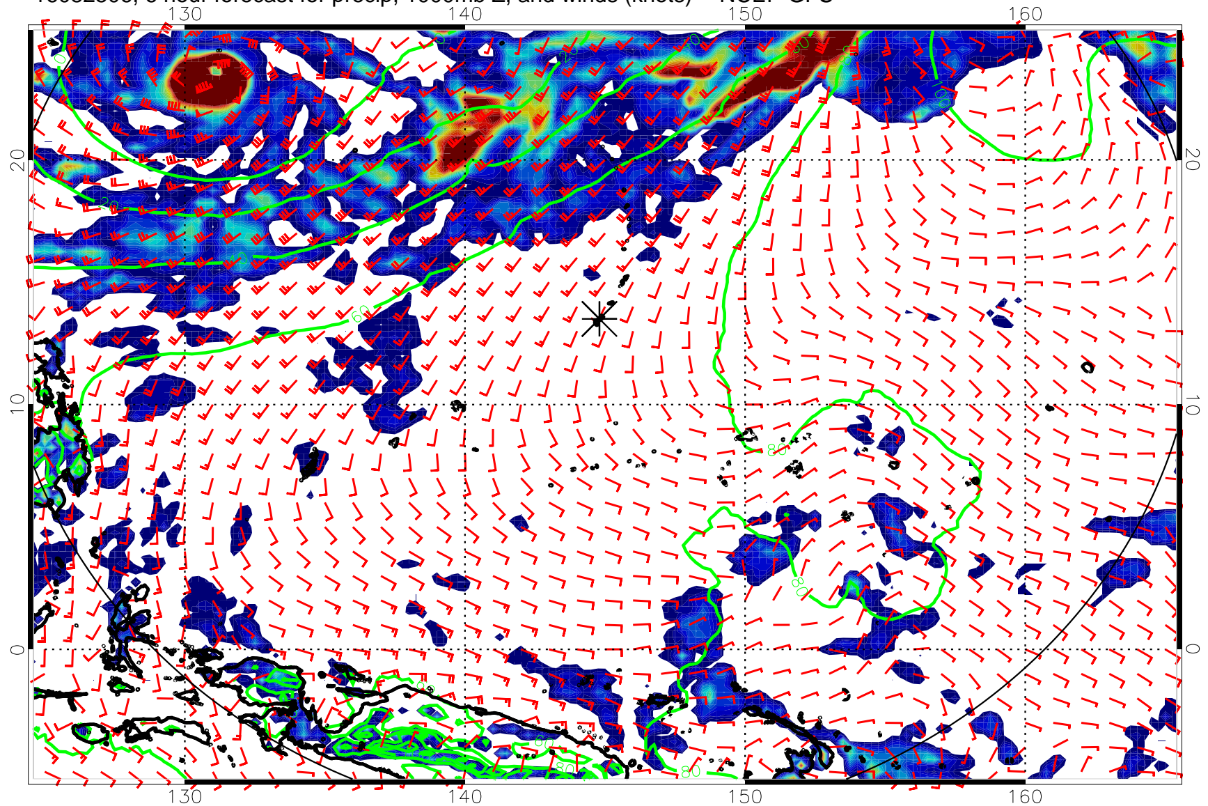
16082506, 6 hour forecast for precip, 1000mb Z, and winds (knots) -- NCEP GFS
