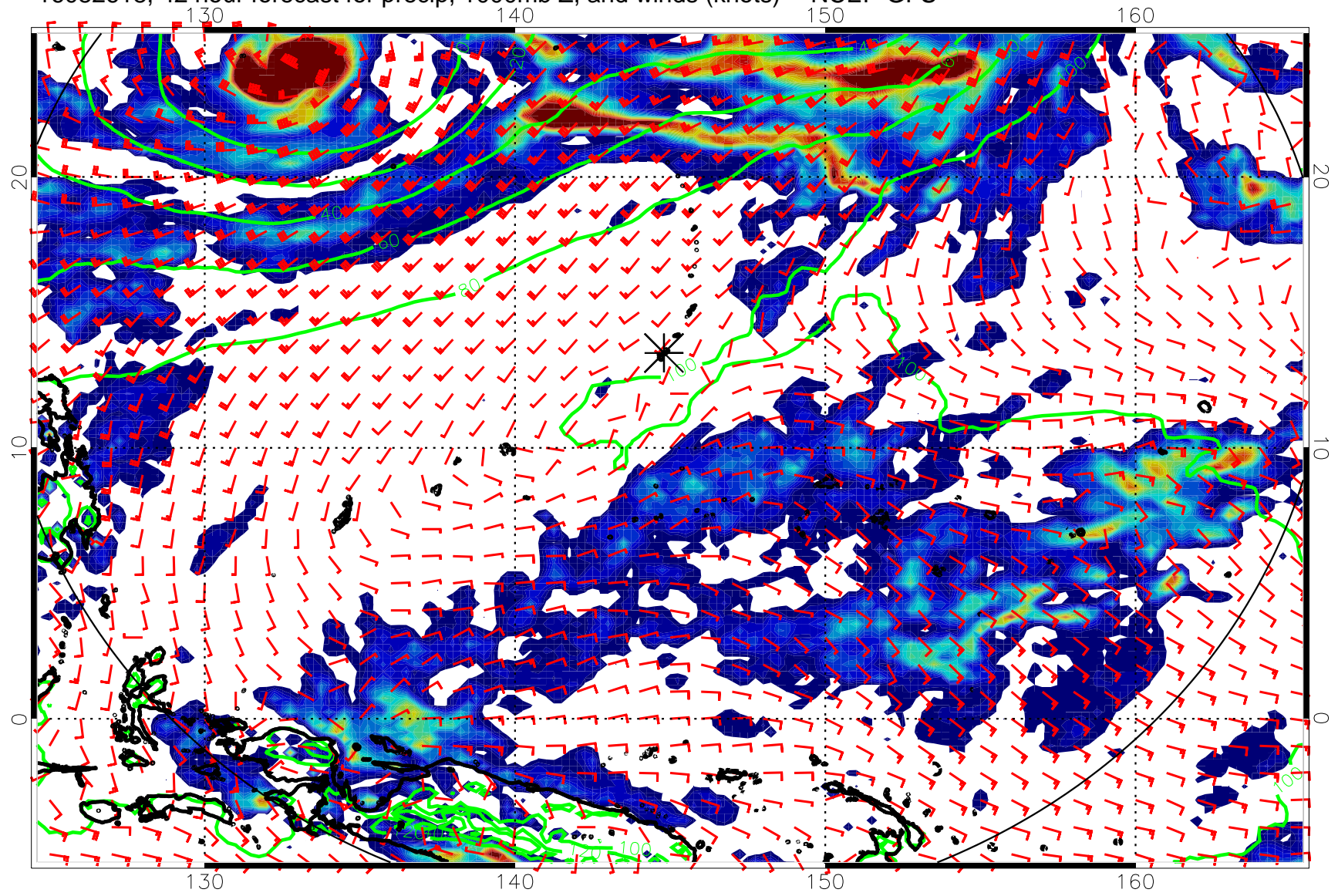
16082618, 42 hour forecast for precip, 1000mb Z, and winds (knots) -- NCEP GFS
