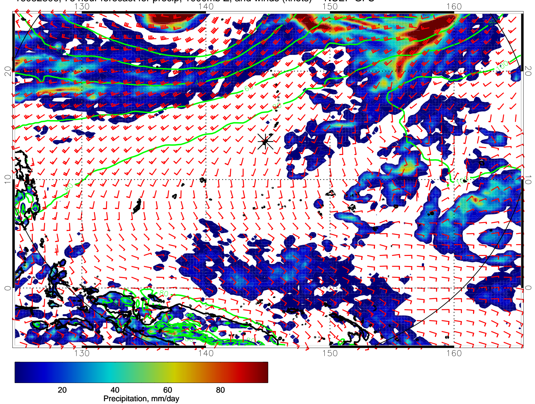
16082806, 78 hour forecast for precip, 1000mb Z, and winds (knots) -- NCEP GFS
