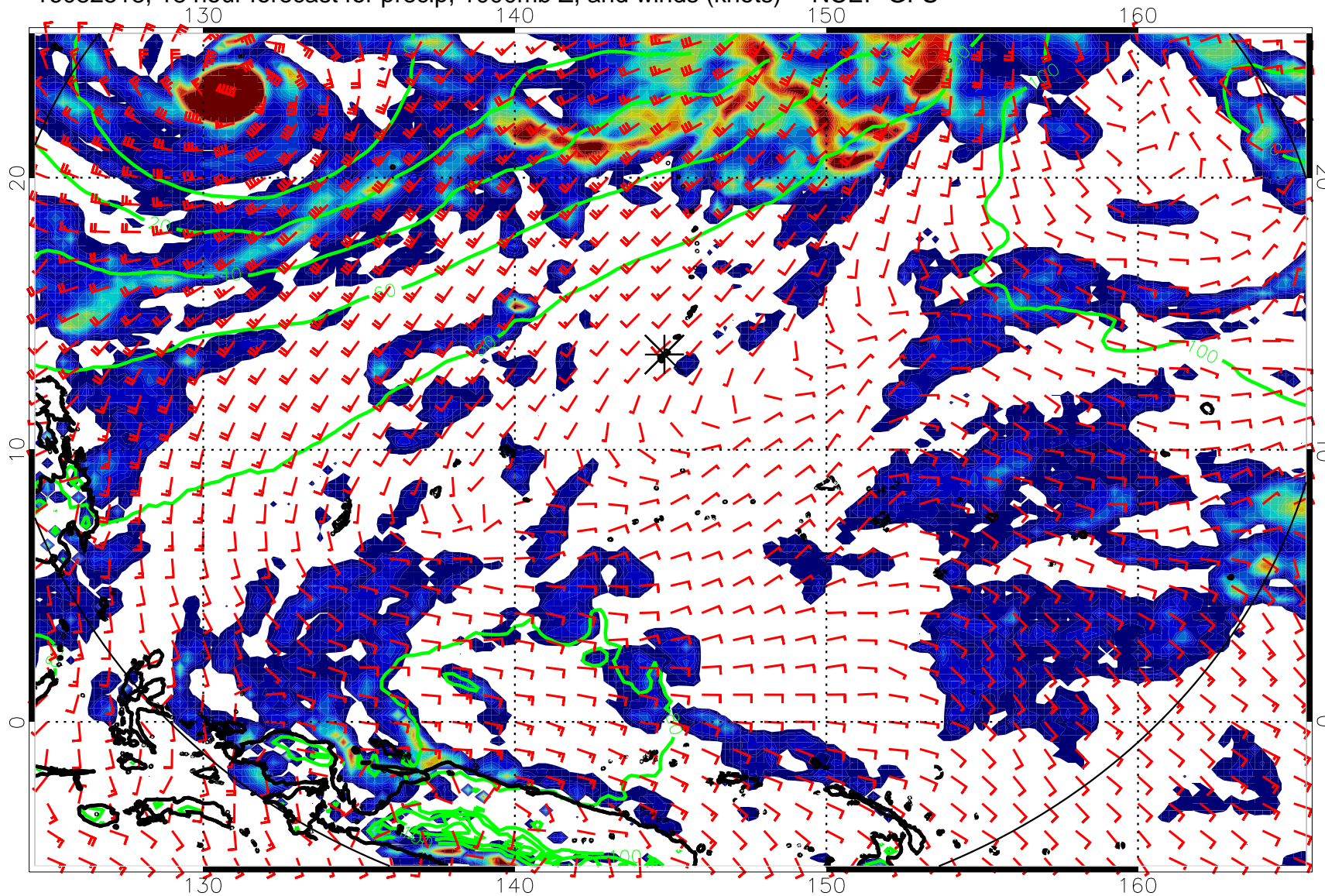
16082518, 18 hour forecast for precip, 1000mb Z, and winds (knots) -- NCEP GFS
