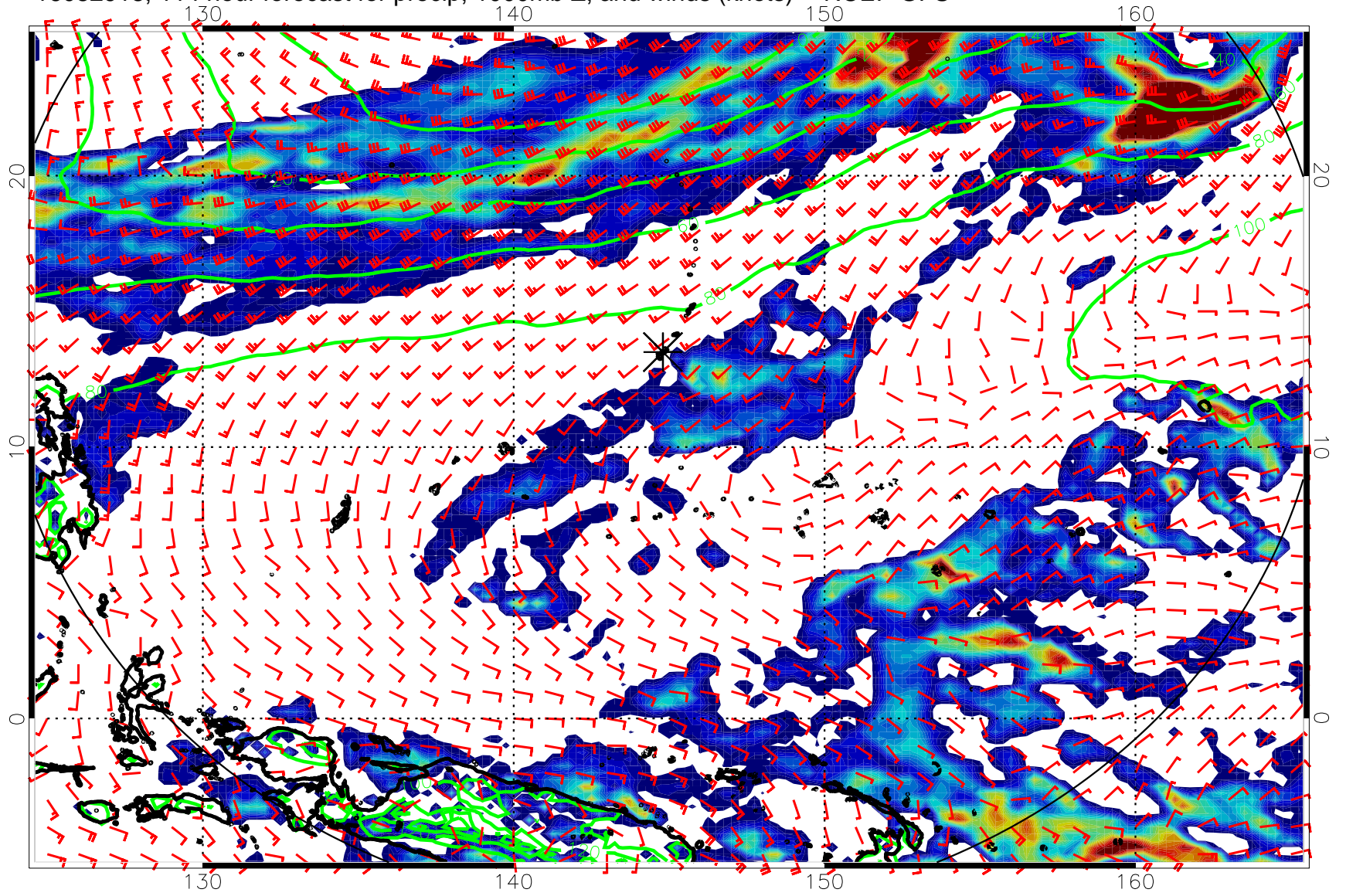
16082918, 114 hour forecast for precip, 1000mb Z, and winds (knots) -- NCEP GFS
