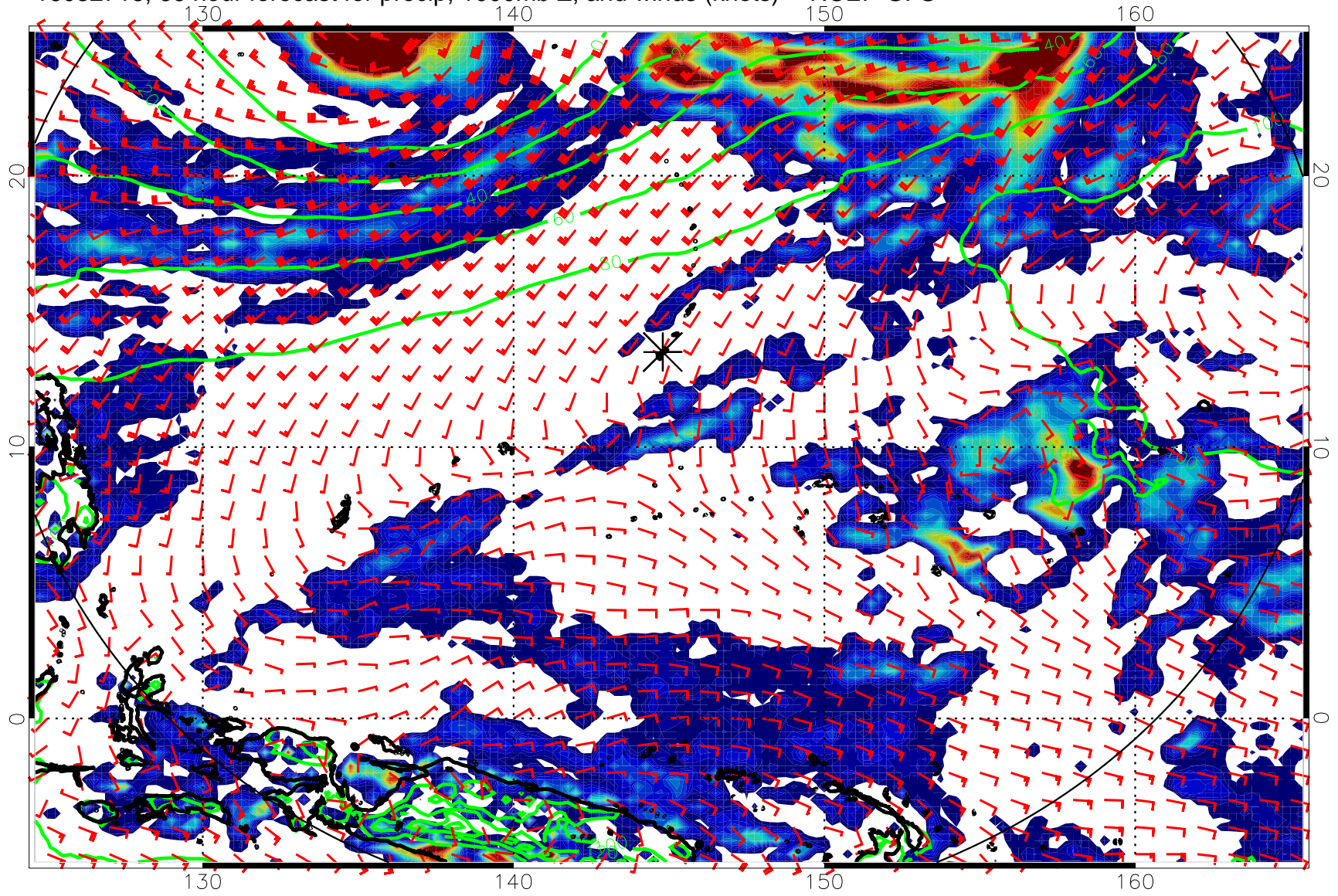
16082718, 66 hour forecast for precip, 1000mb Z, and winds (knots) -- NCEP GFS
