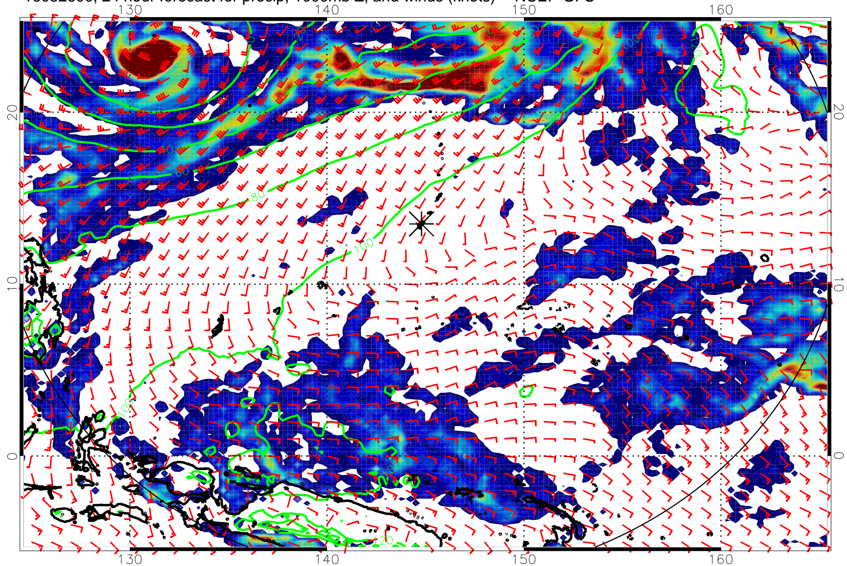
16082600, 24 hour forecast for precip, 1000mb Z, and winds (knots) -- NCEP GFS
