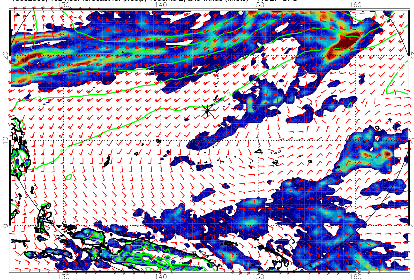
16082906, 102 hour forecast for precip, 1000mb Z, and winds (knots) -- NCEP GFS
