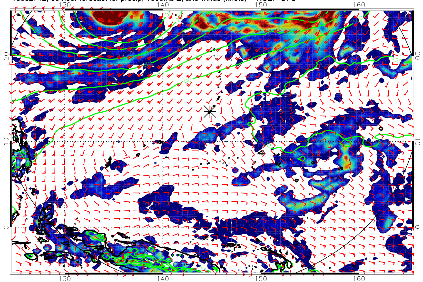
16082712, 60 hour forecast for precip, 1000mb Z, and winds (knots) -- NCEP GFS
