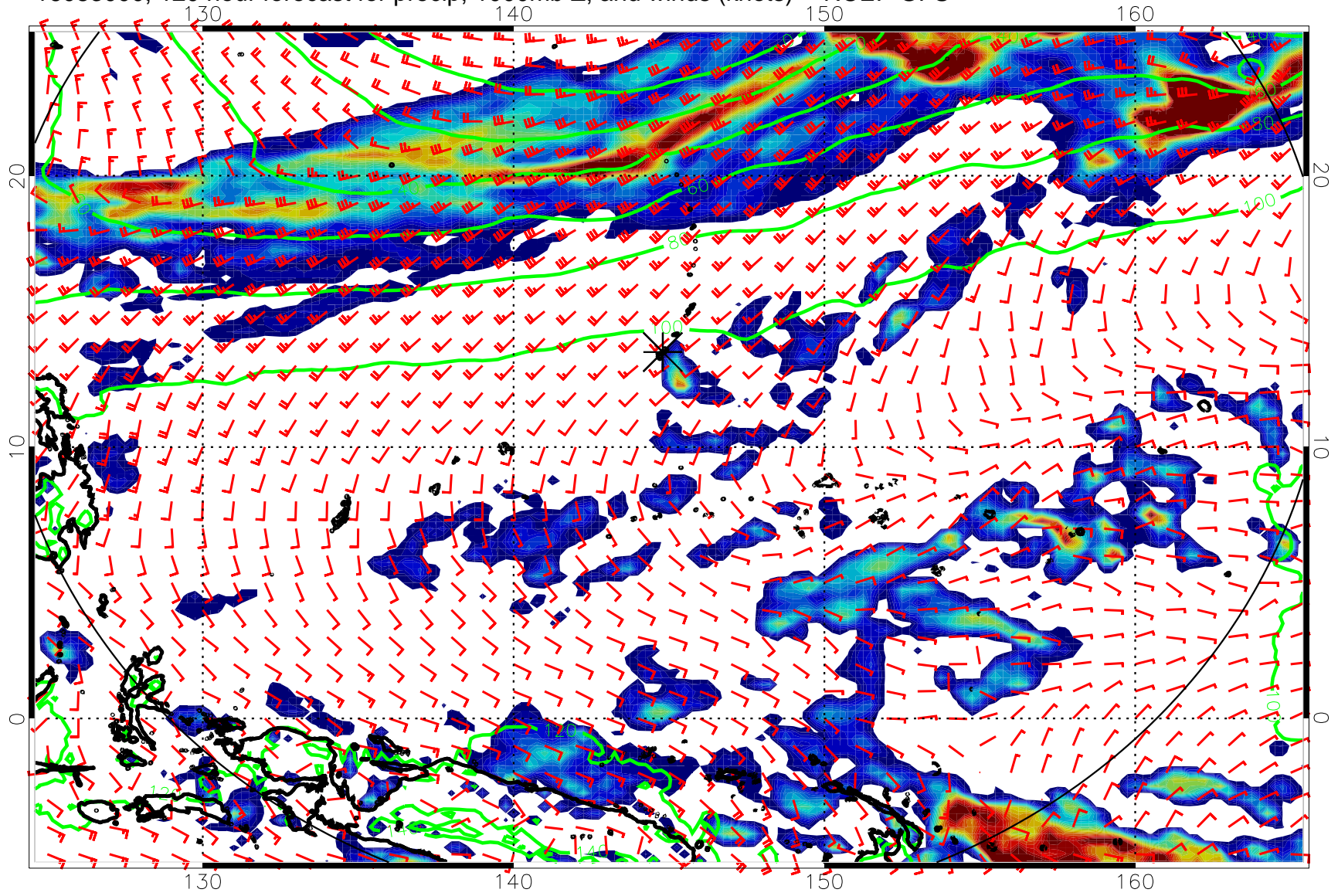
16083000, 120 hour forecast for precip, 1000mb Z, and winds (knots) -- NCEP GFS
