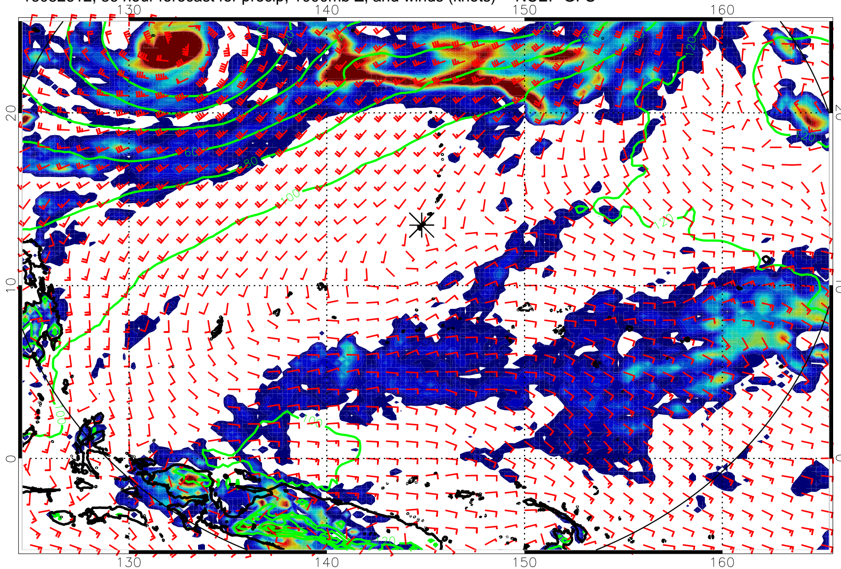
16082612, 36 hour forecast for precip, 1000mb Z, and winds (knots) -- NCEP GFS
