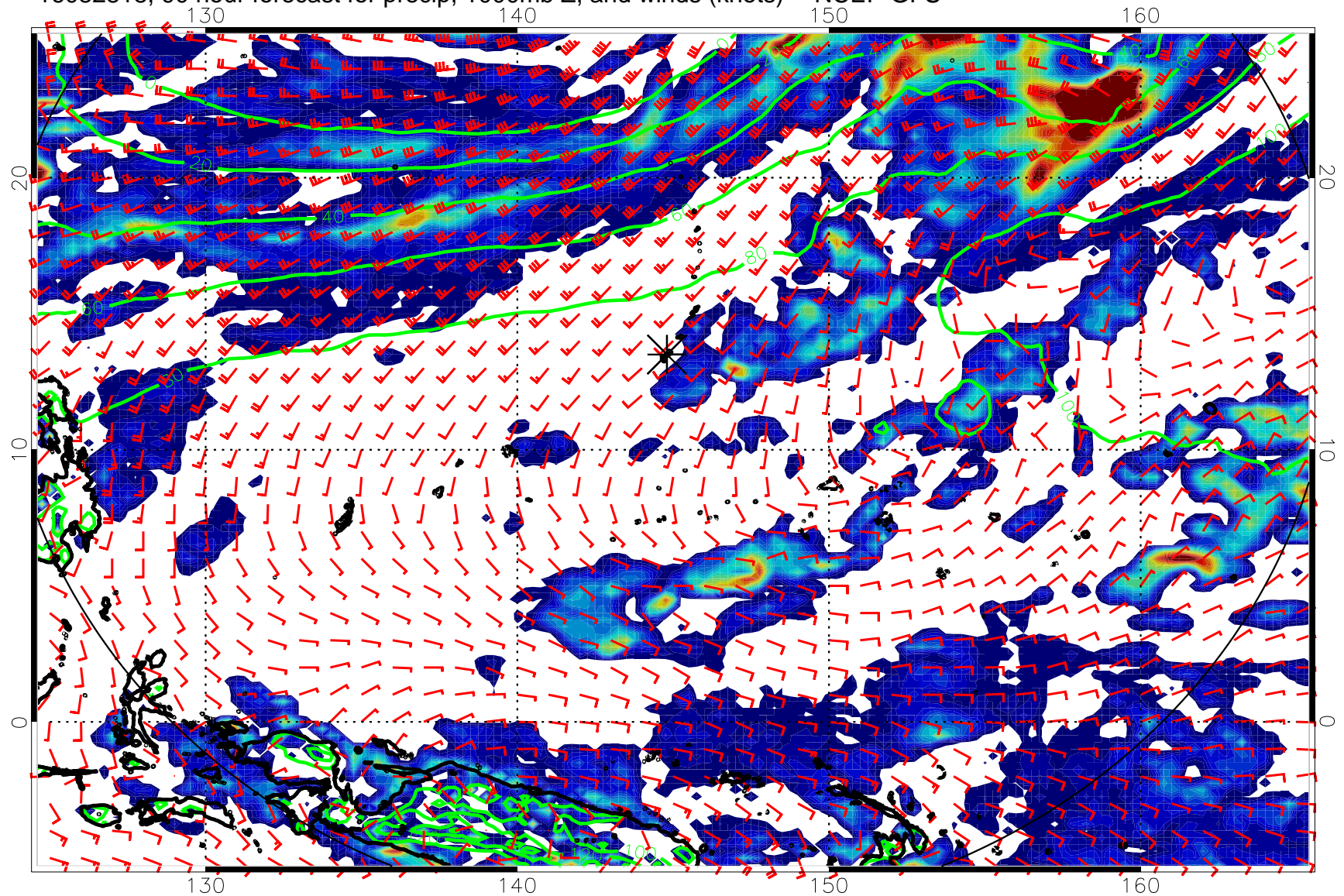
16082818, 90 hour forecast for precip, 1000mb Z, and winds (knots) -- NCEP GFS
