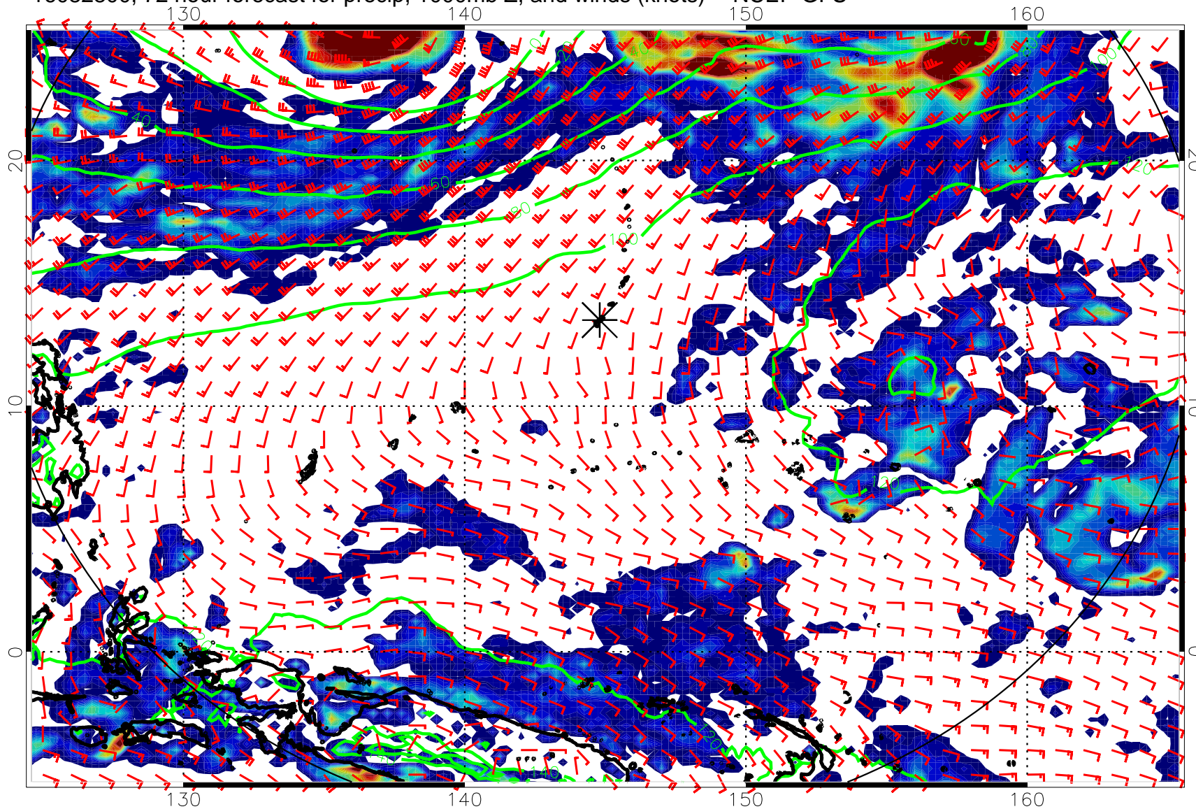
16082800, 72 hour forecast for precip, 1000mb Z, and winds (knots) -- NCEP GFS
