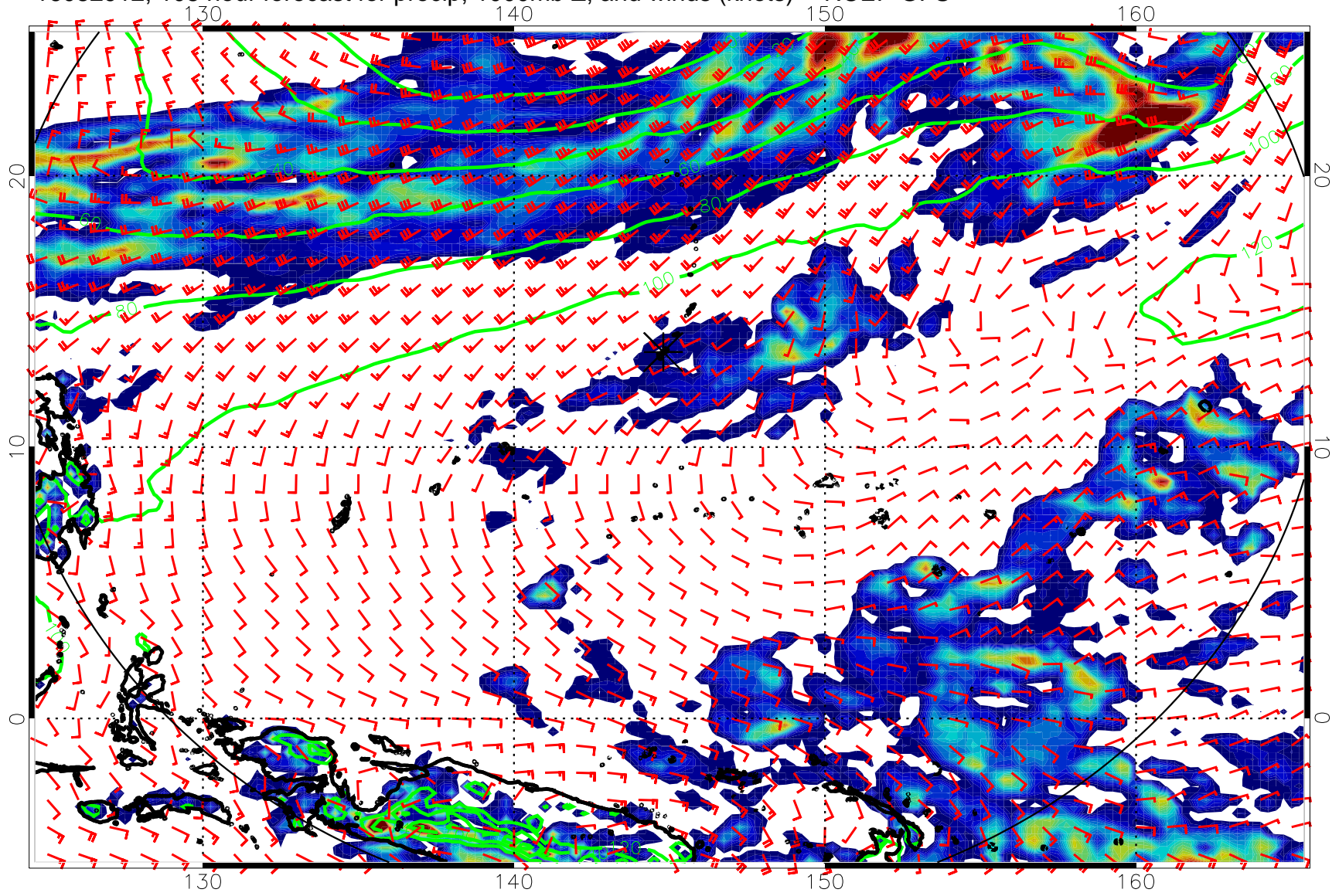
16082912, 108 hour forecast for precip, 1000mb Z, and winds (knots) -- NCEP GFS
