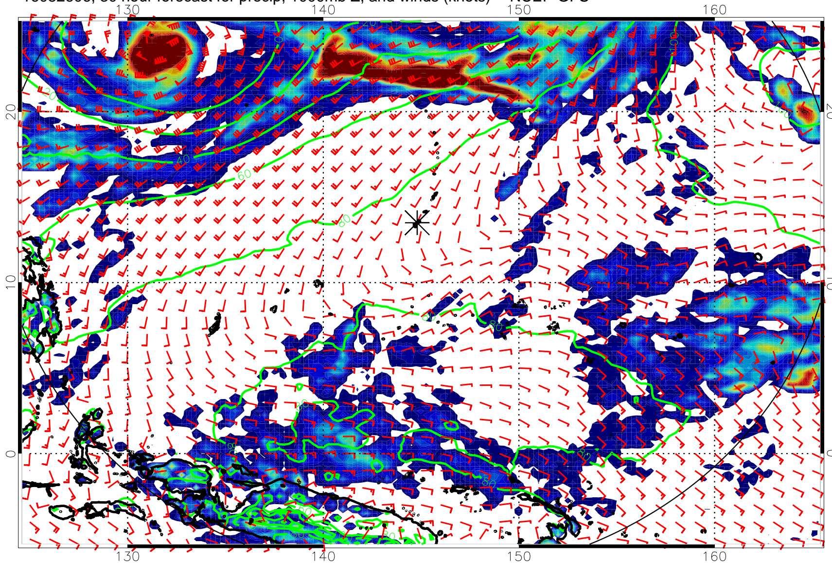
16082606, 30 hour forecast for precip, 1000mb Z, and winds (knots) -- NCEP GFS
