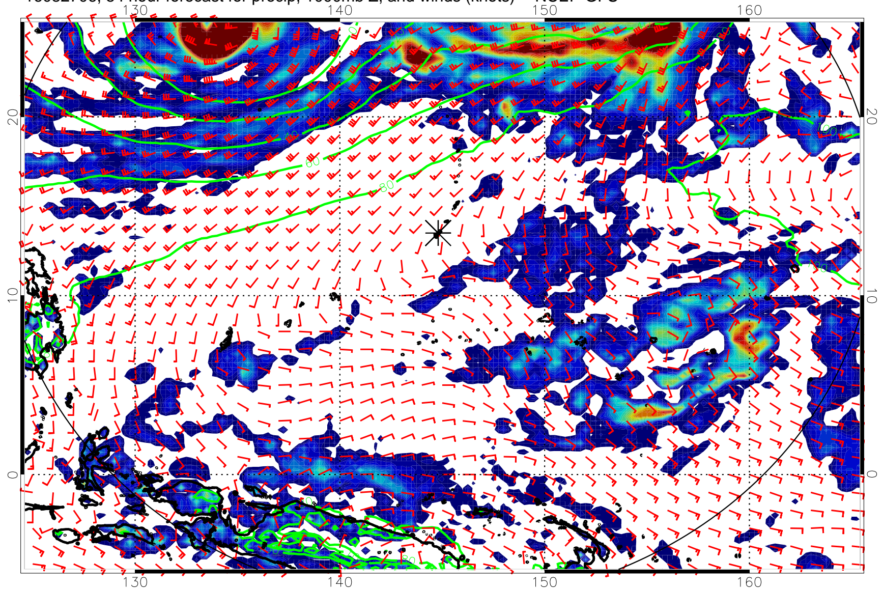
16082706, 54 hour forecast for precip, 1000mb Z, and winds (knots) -- NCEP GFS
