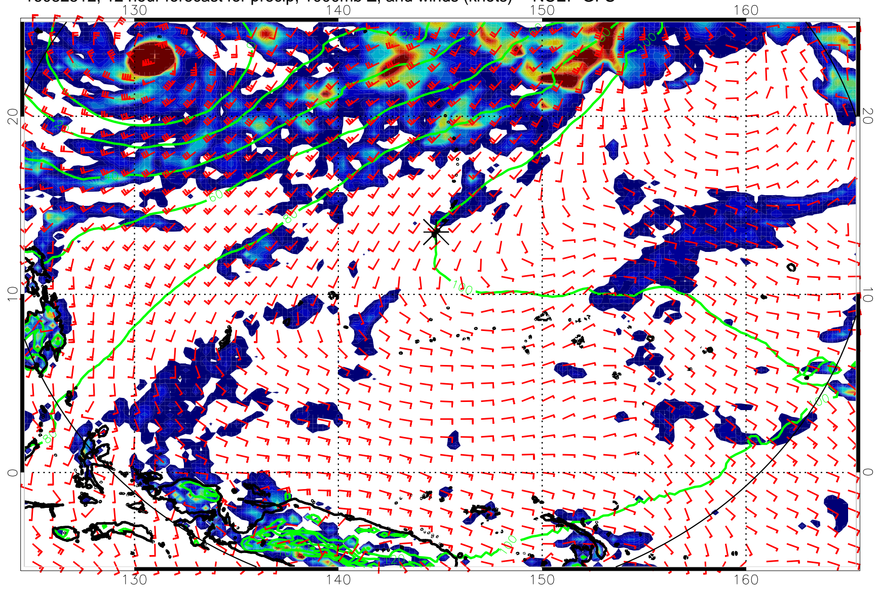
16082512, 12 hour forecast for precip, 1000mb Z, and winds (knots) -- NCEP GFS
