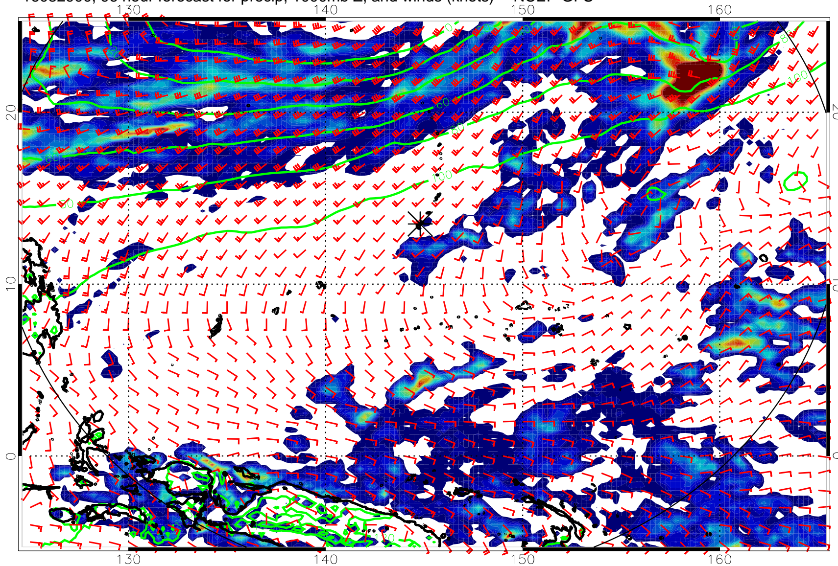
16082900, 96 hour forecast for precip, 1000mb Z, and winds (knots) -- NCEP GFS
