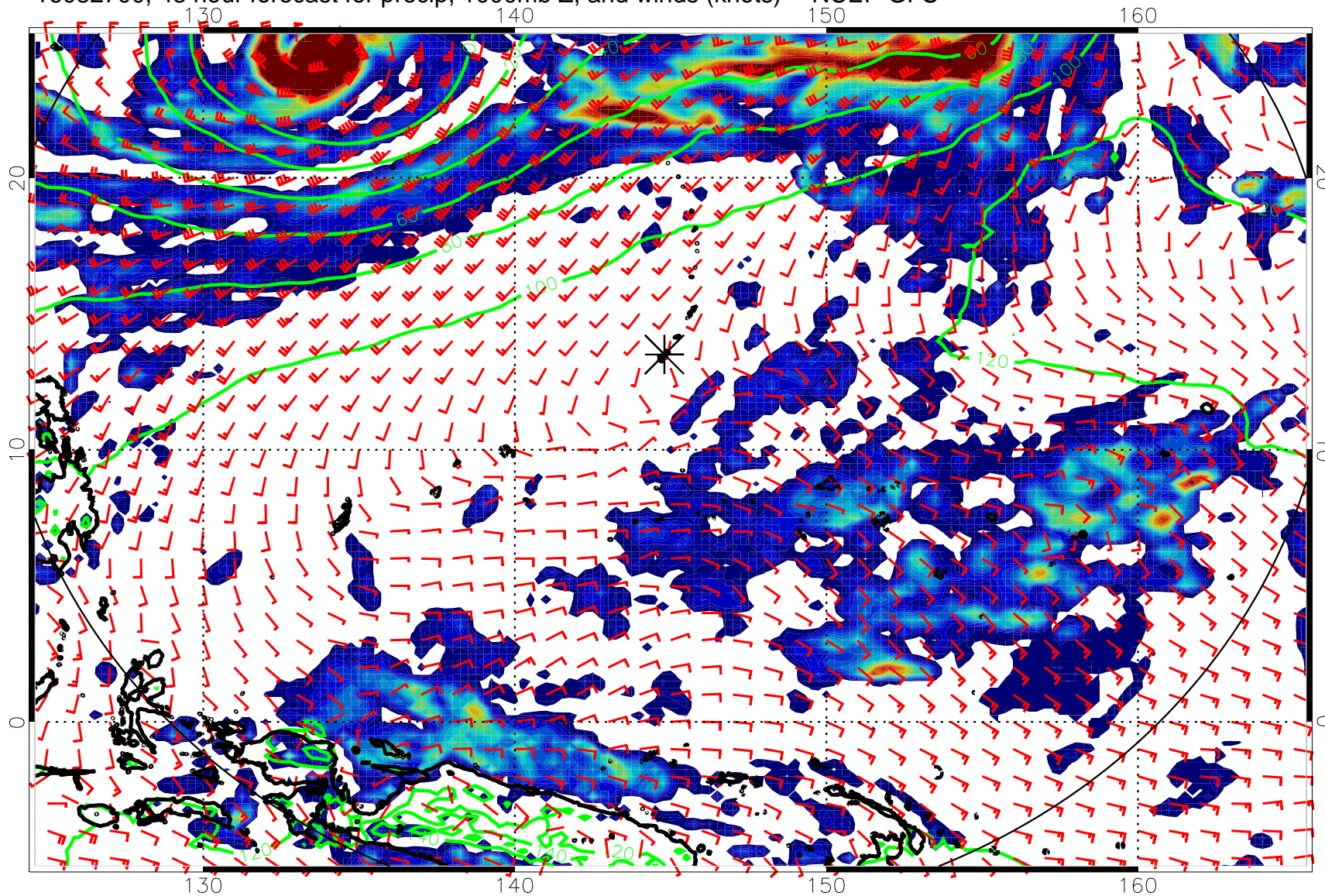
16082700, 48 hour forecast for precip, 1000mb Z, and winds (knots) -- NCEP GFS
