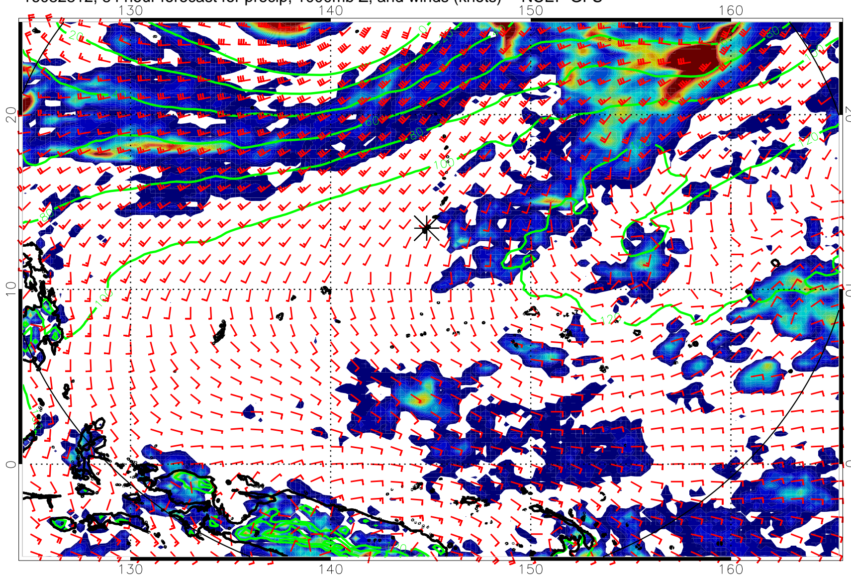
16082812, 84 hour forecast for precip, 1000mb Z, and winds (knots) -- NCEP GFS
