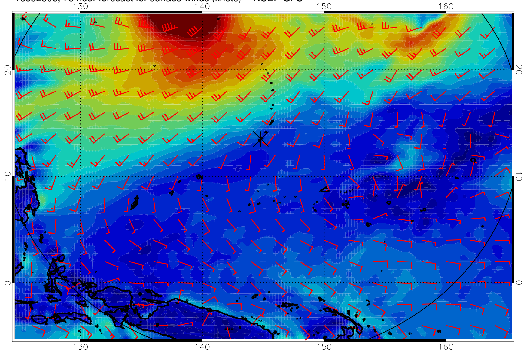
16082806, 78 hour forecast for surface winds (knots) -- NCEP GFS
