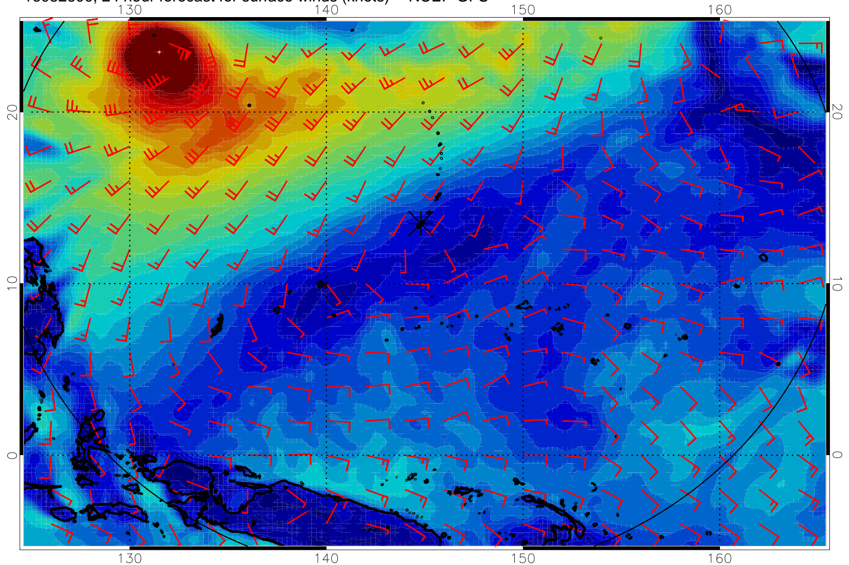
16082600, 24 hour forecast for surface winds (knots) -- NCEP GFS
