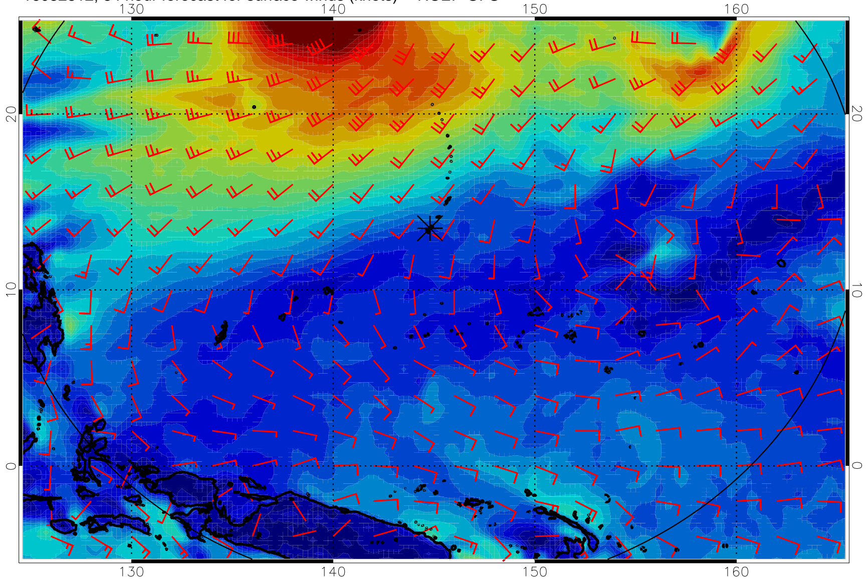
16082812, 84 hour forecast for surface winds (knots) -- NCEP GFS
