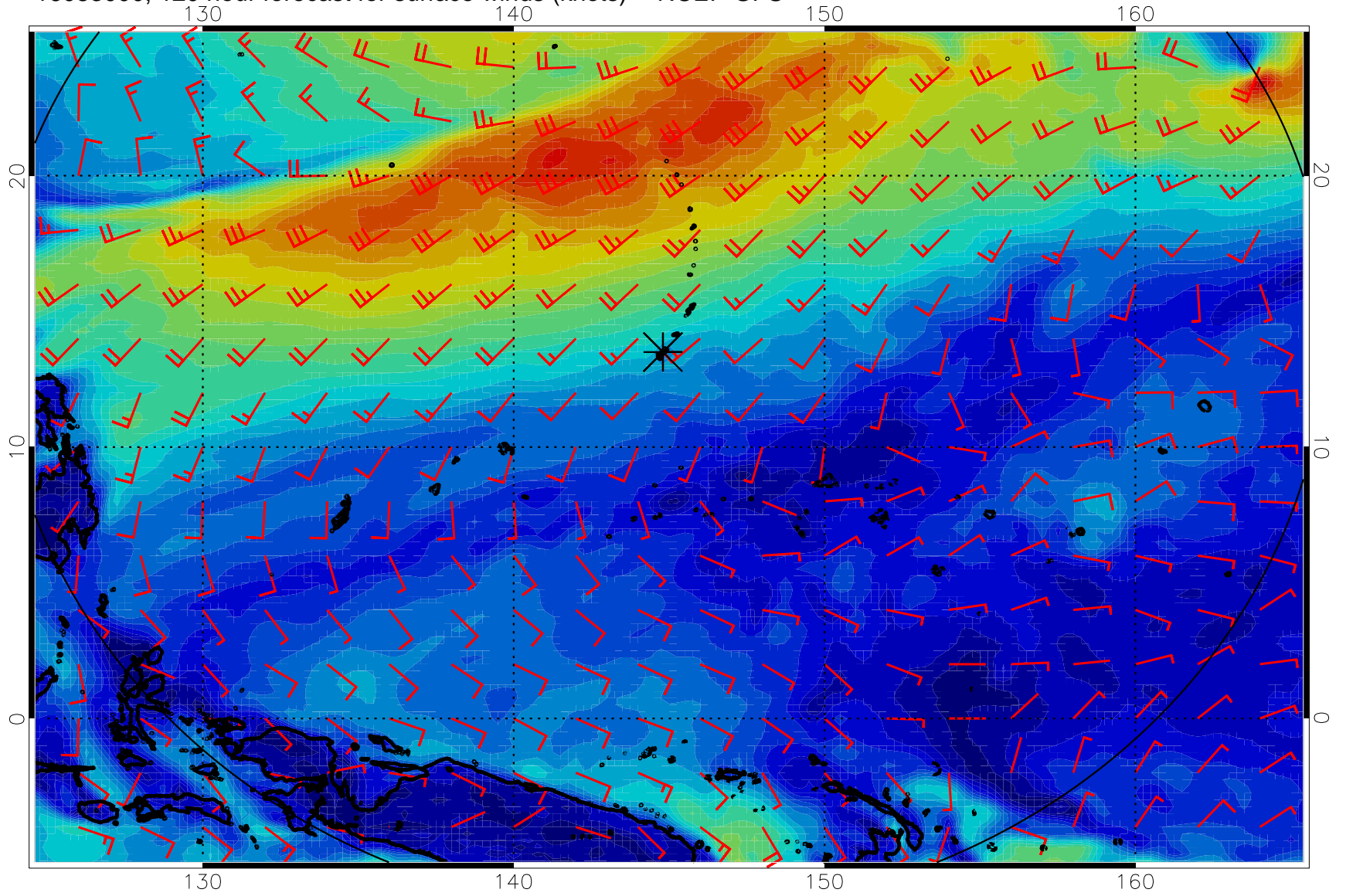
16083000, 120 hour forecast for surface winds (knots) -- NCEP GFS
