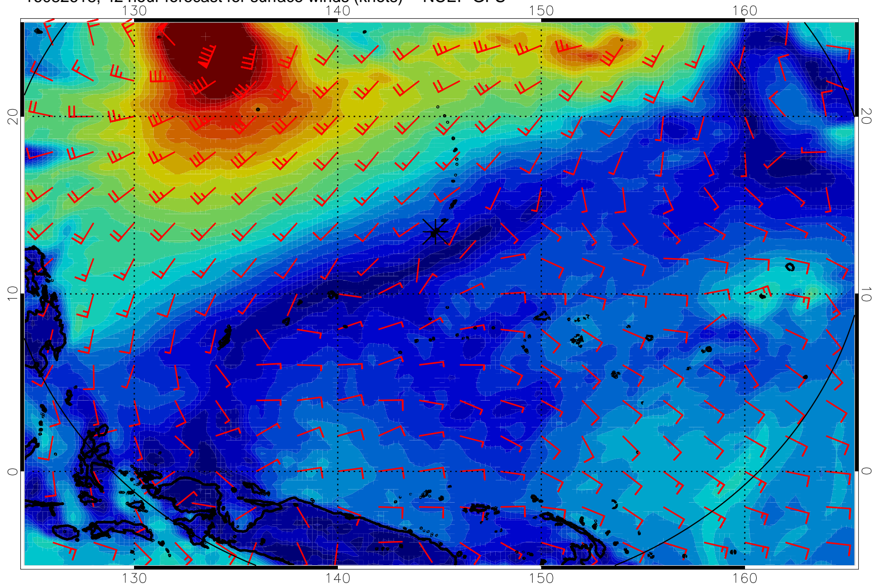
16082618, 42 hour forecast for surface winds (knots) -- NCEP GFS
