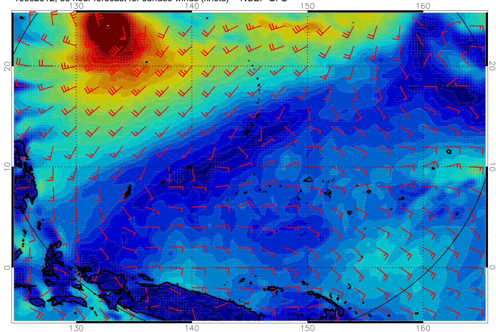
16082612, 36 hour forecast for surface winds (knots) -- NCEP GFS
