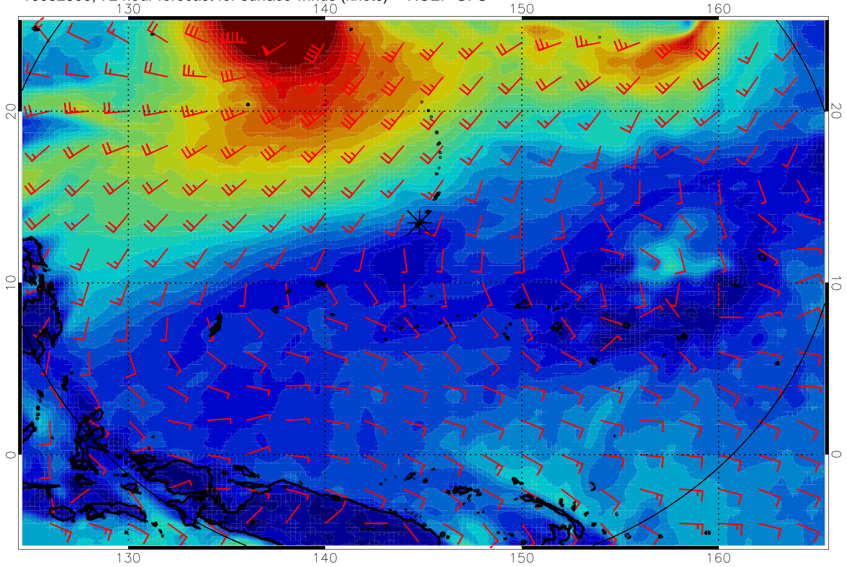
16082800, 72 hour forecast for surface winds (knots) -- NCEP GFS
