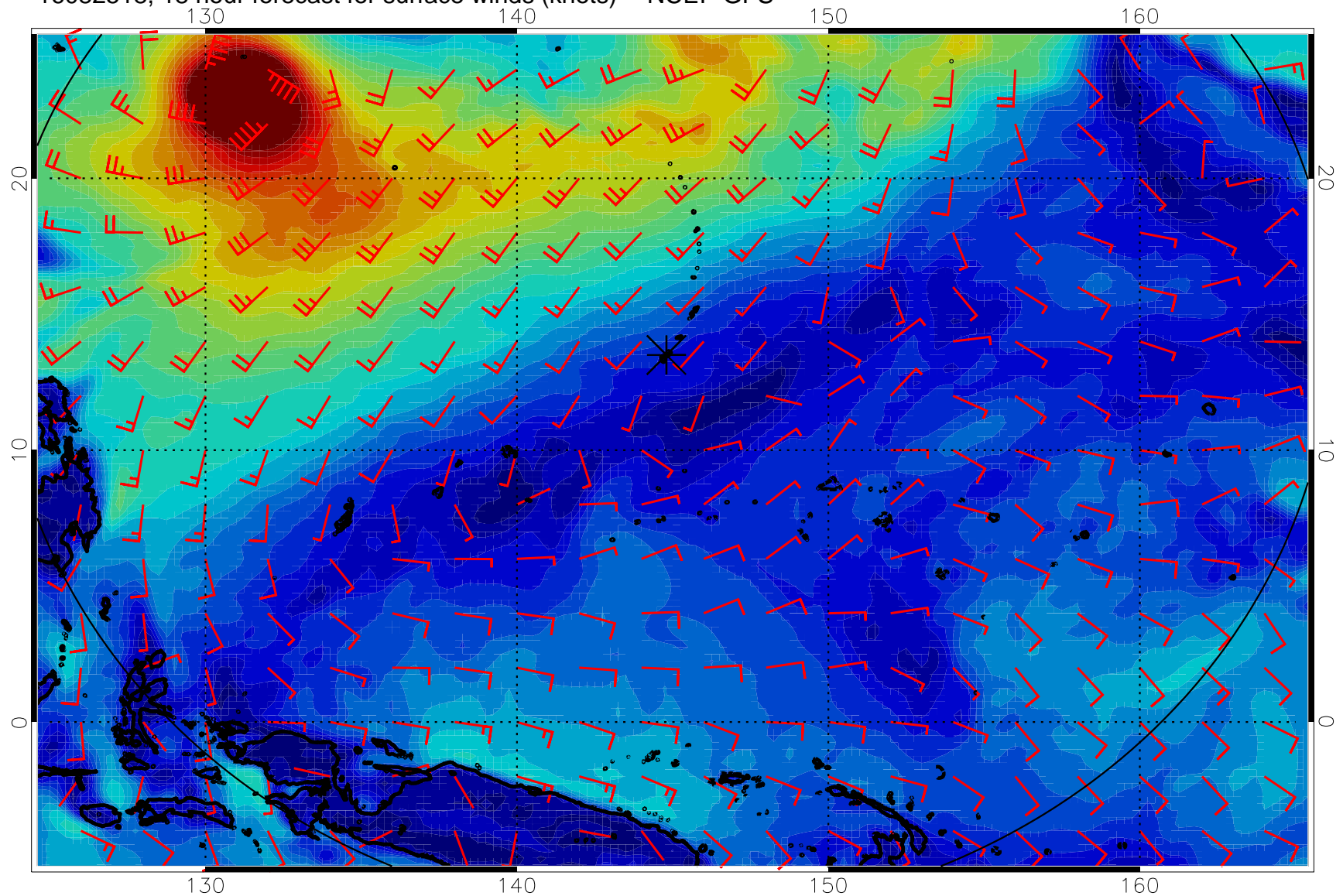
16082518, 18 hour forecast for surface winds (knots) -- NCEP GFS
