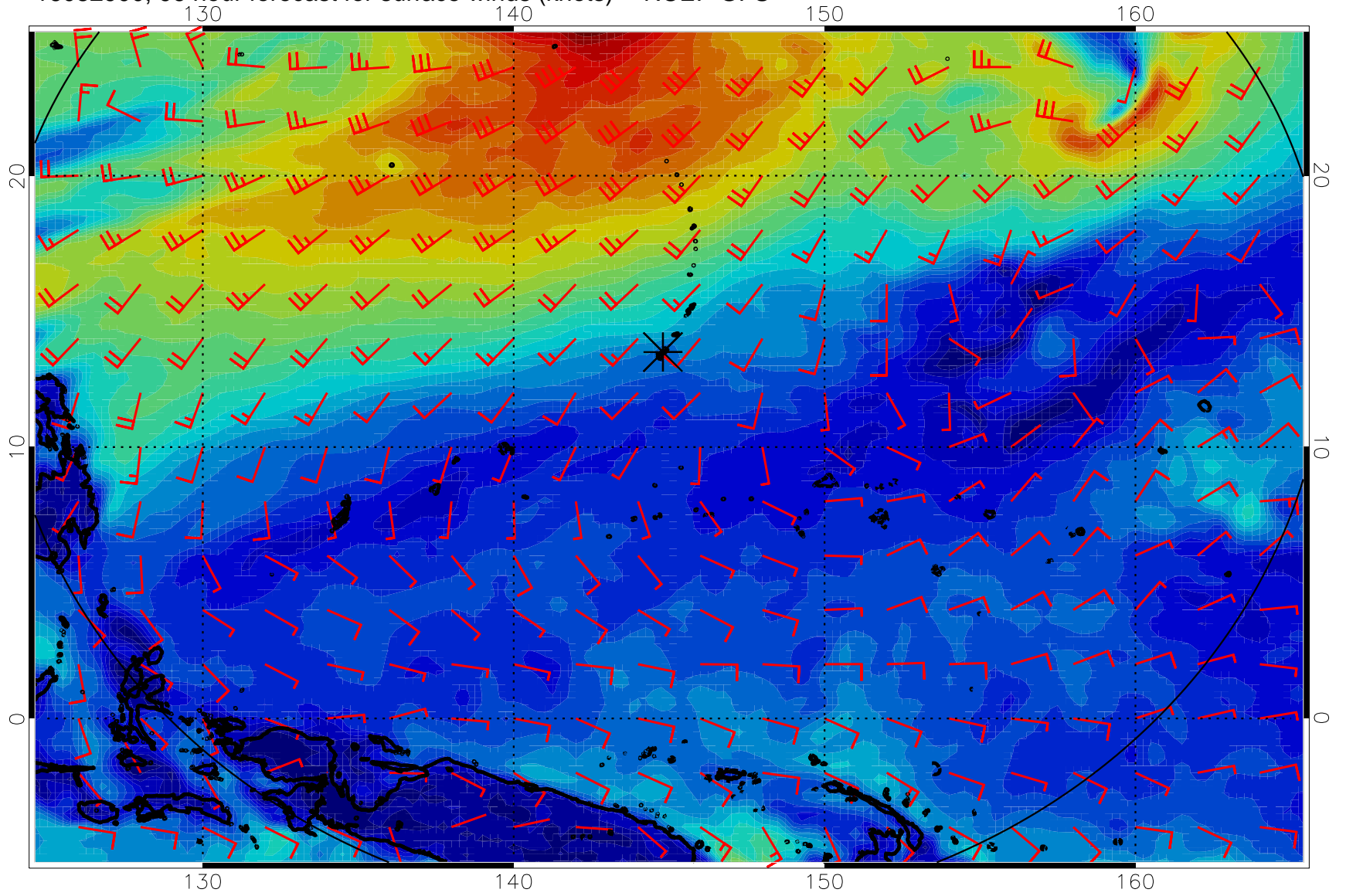
16082900, 96 hour forecast for surface winds (knots) -- NCEP GFS
