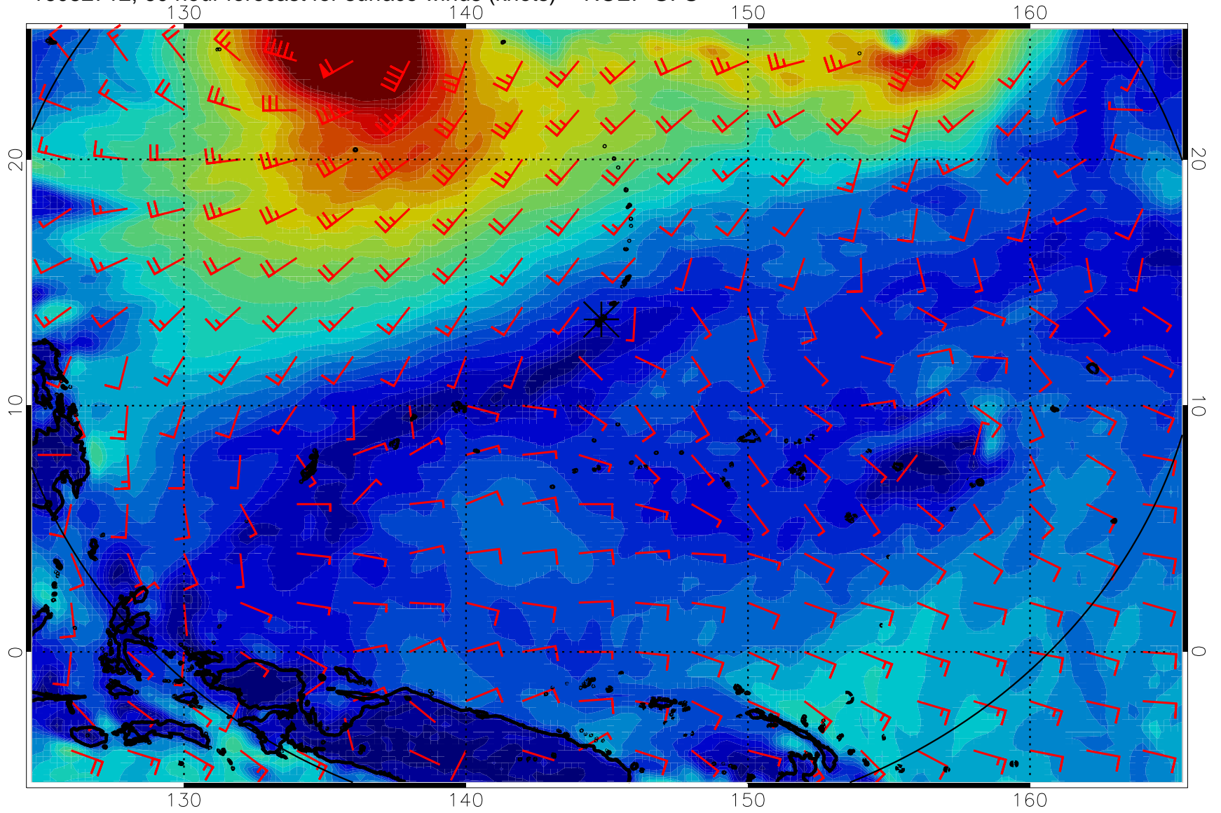
16082712, 60 hour forecast for surface winds (knots) -- NCEP GFS
