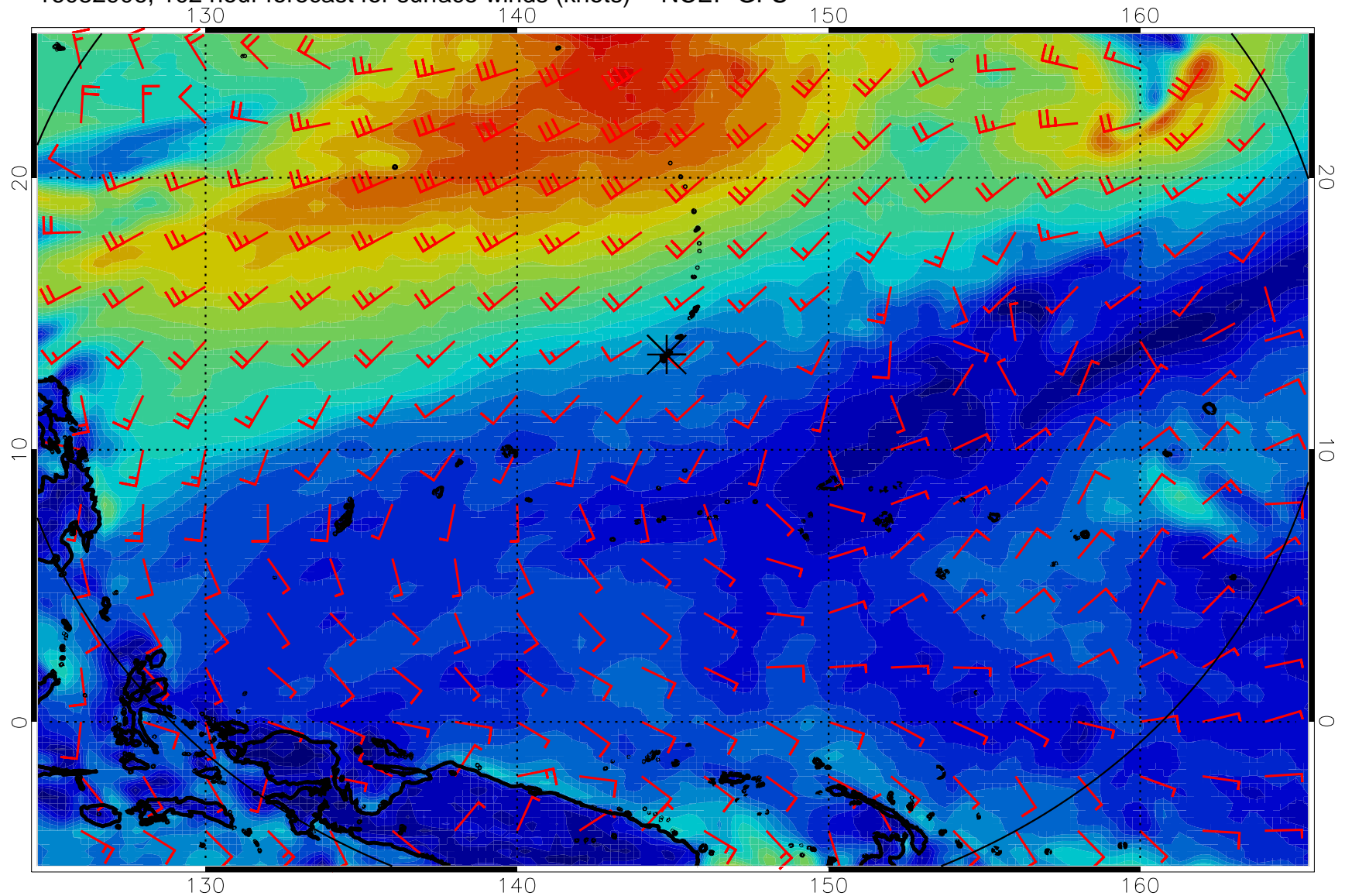
16082906, 102 hour forecast for surface winds (knots) -- NCEP GFS
