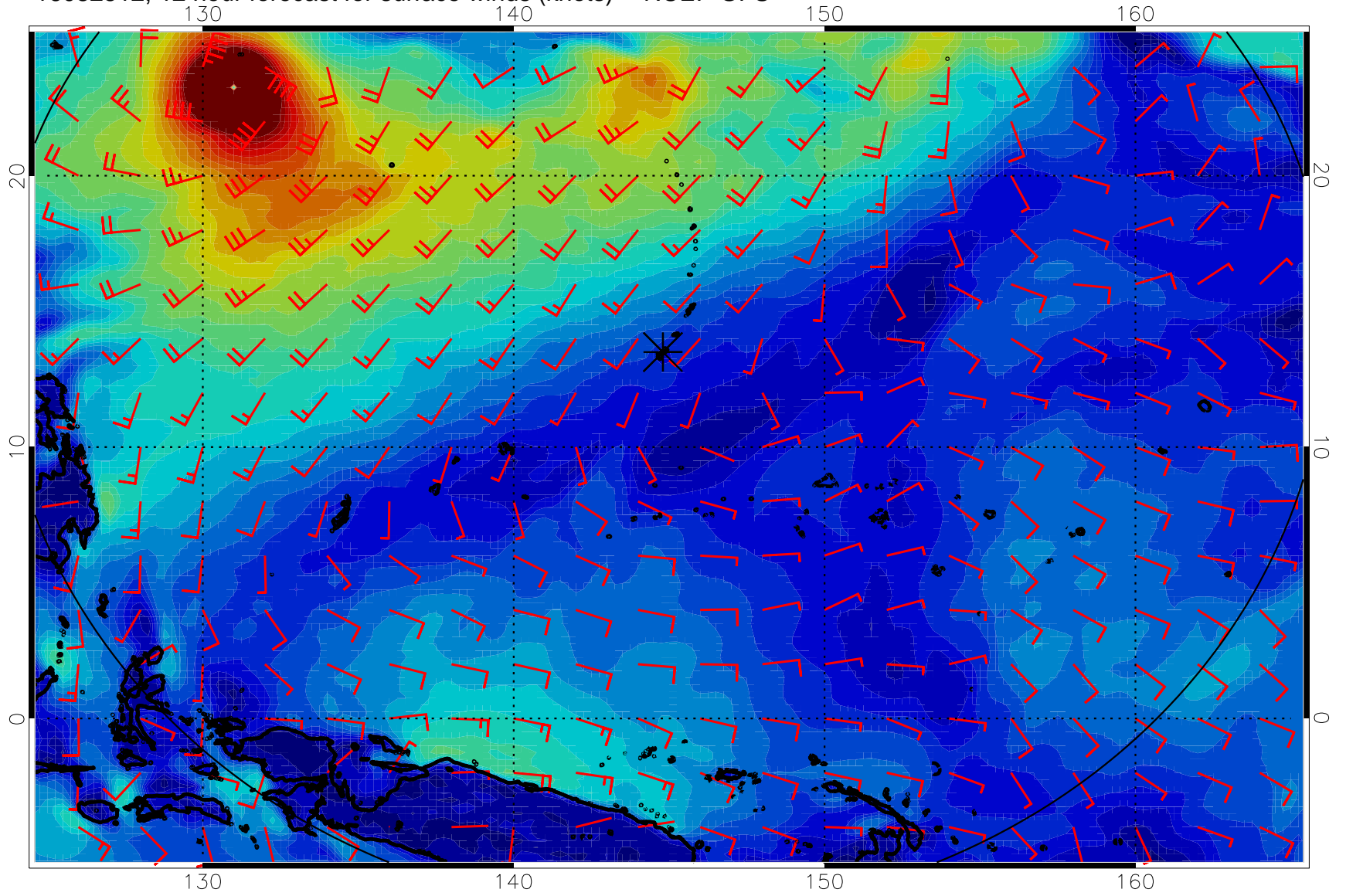
16082512, 12 hour forecast for surface winds (knots) -- NCEP GFS
