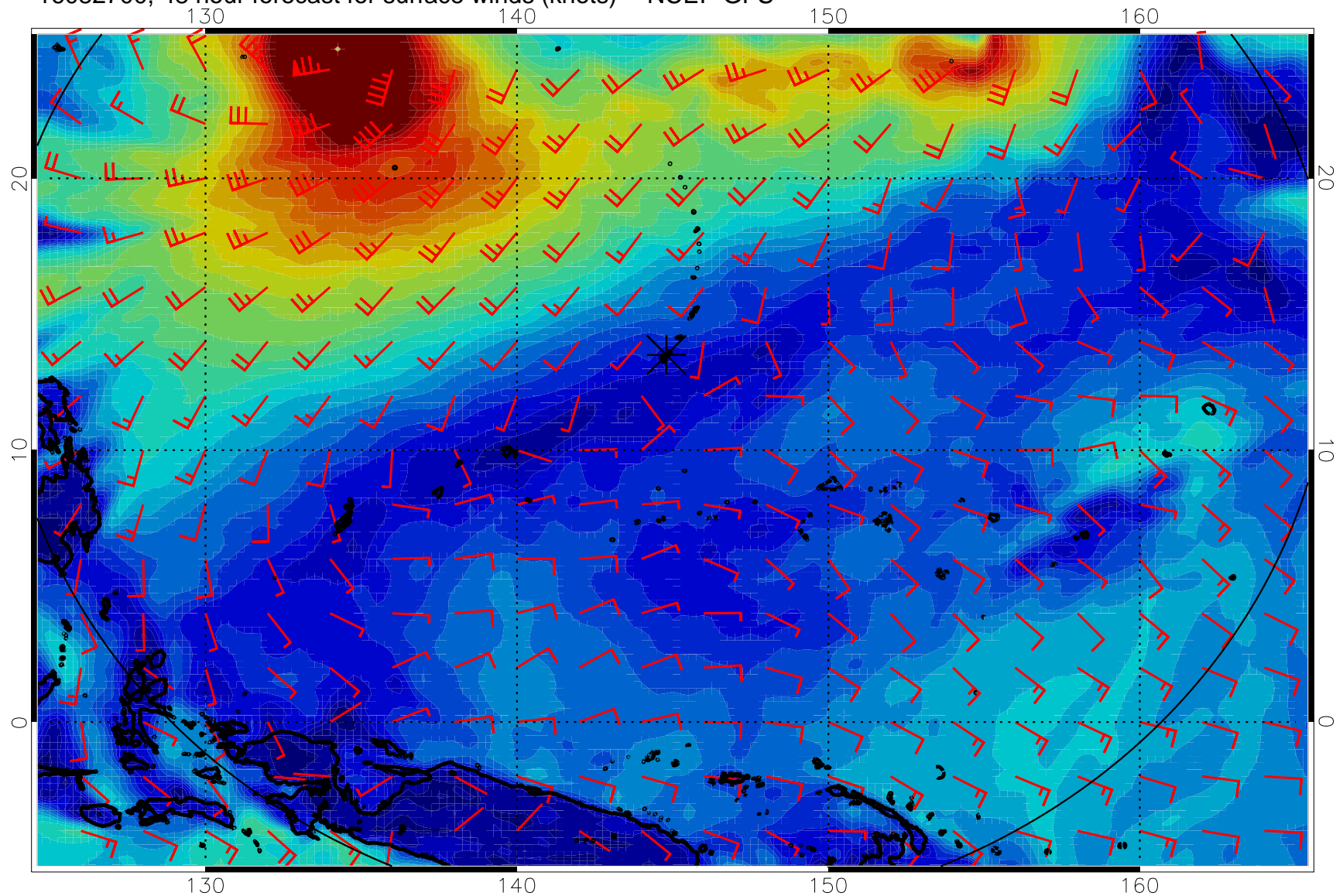
16082700, 48 hour forecast for surface winds (knots) -- NCEP GFS
