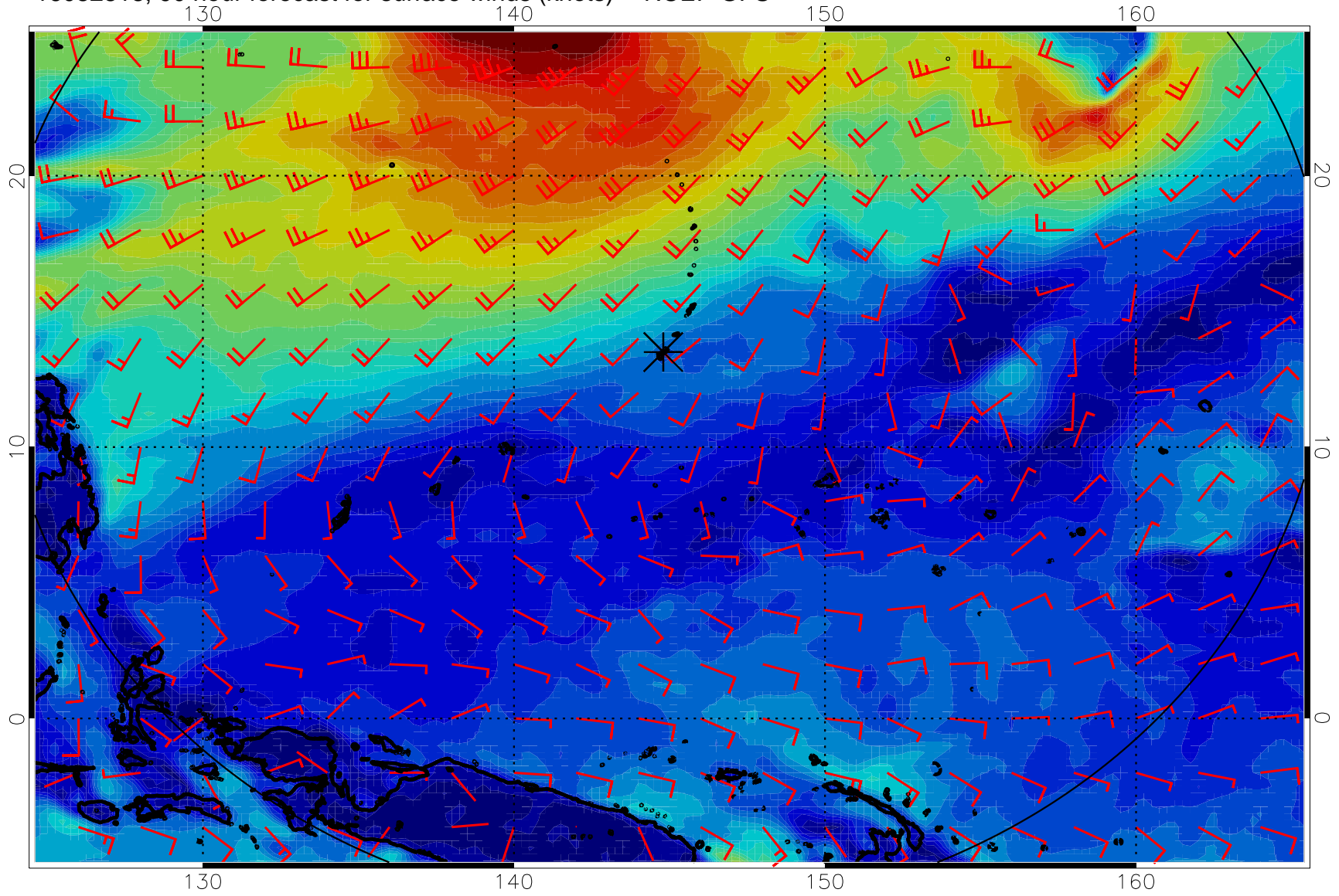
16082818, 90 hour forecast for surface winds (knots) -- NCEP GFS
