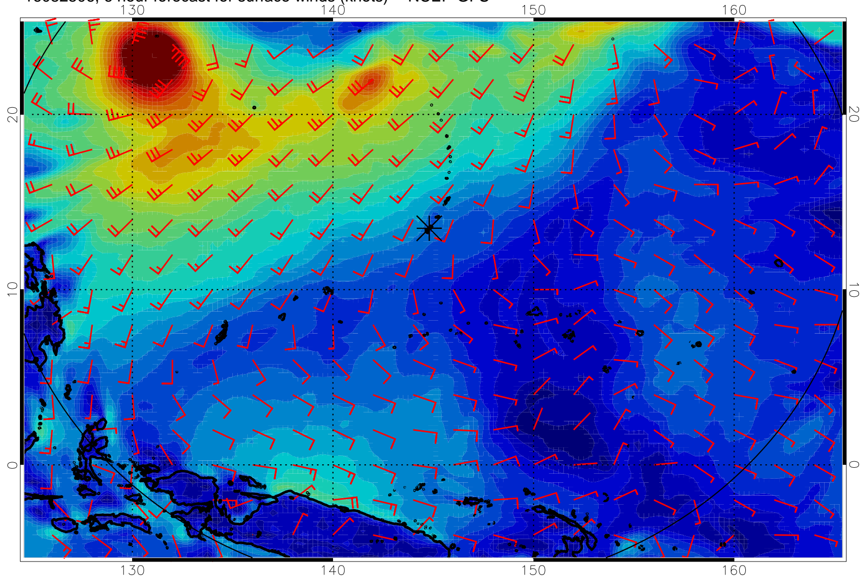
16082506, 6 hour forecast for surface winds (knots) -- NCEP GFS
