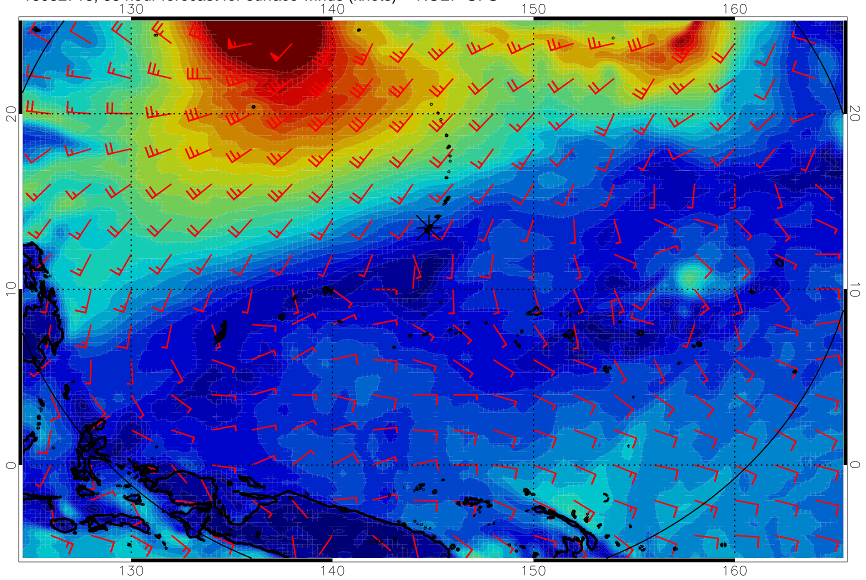
16082718, 66 hour forecast for surface winds (knots) -- NCEP GFS
