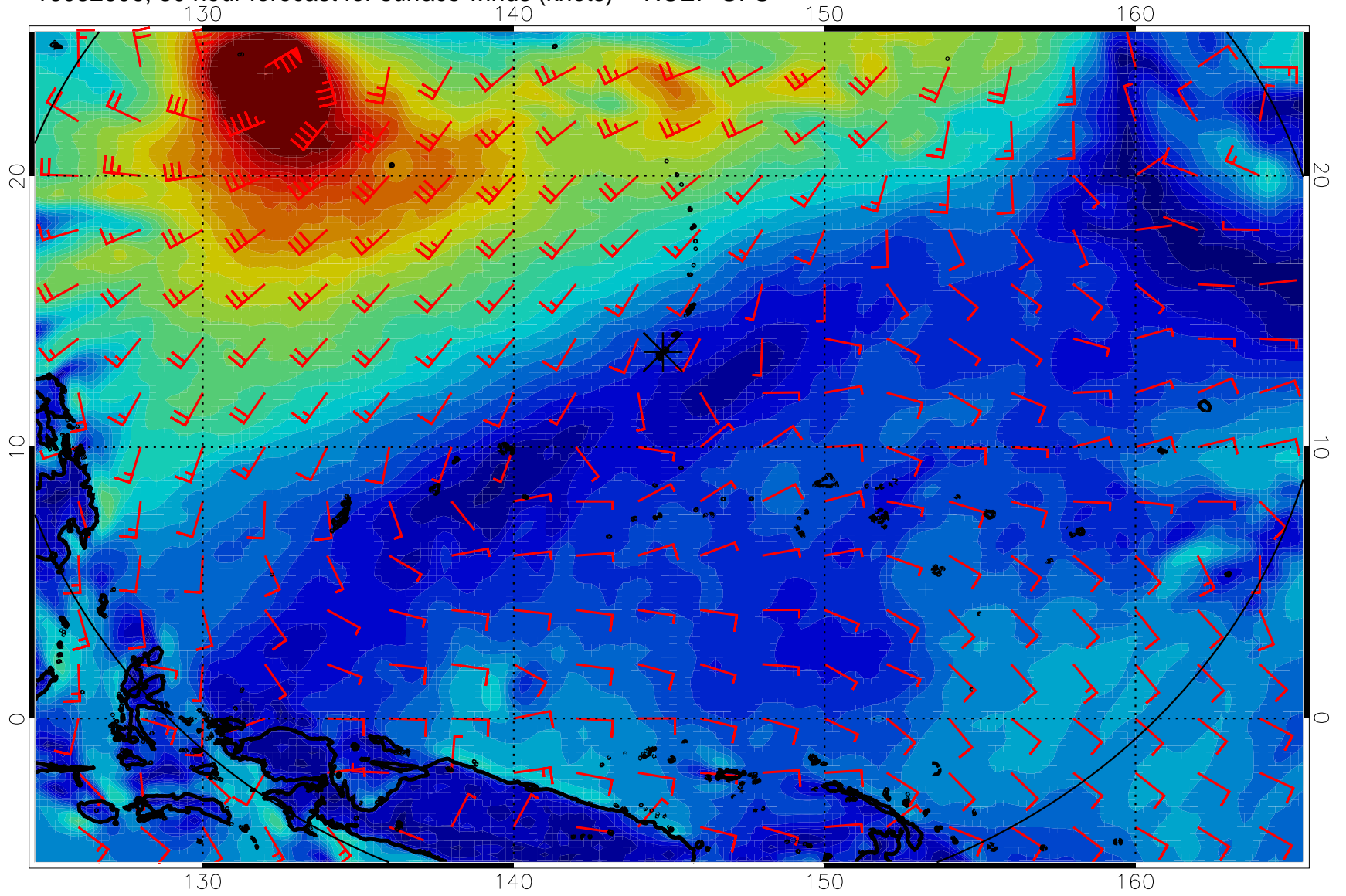
16082606, 30 hour forecast for surface winds (knots) -- NCEP GFS
