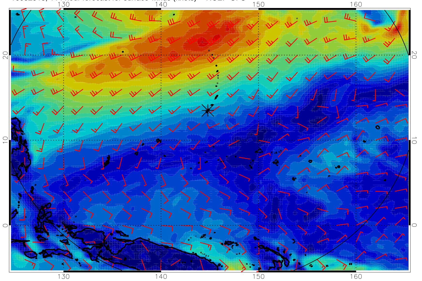
16082918, 114 hour forecast for surface winds (knots) -- NCEP GFS
