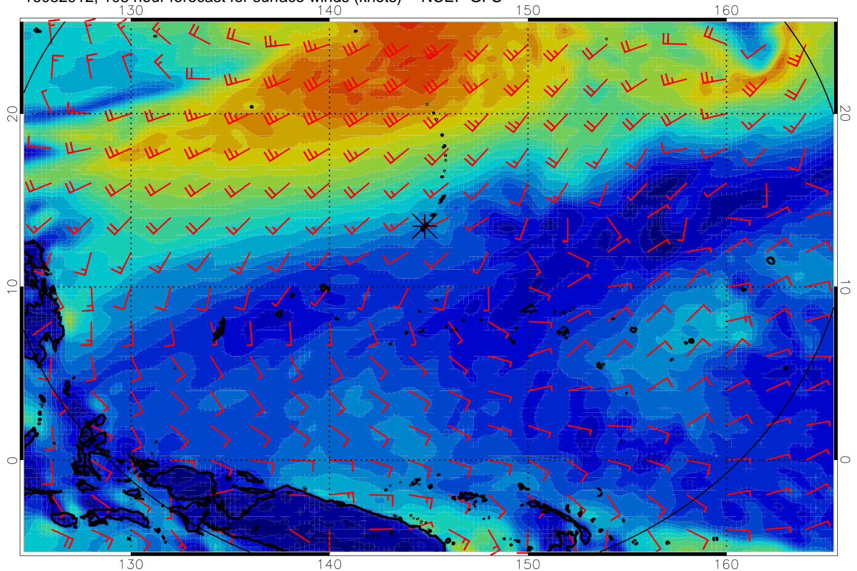
16082912, 108 hour forecast for surface winds (knots) -- NCEP GFS
