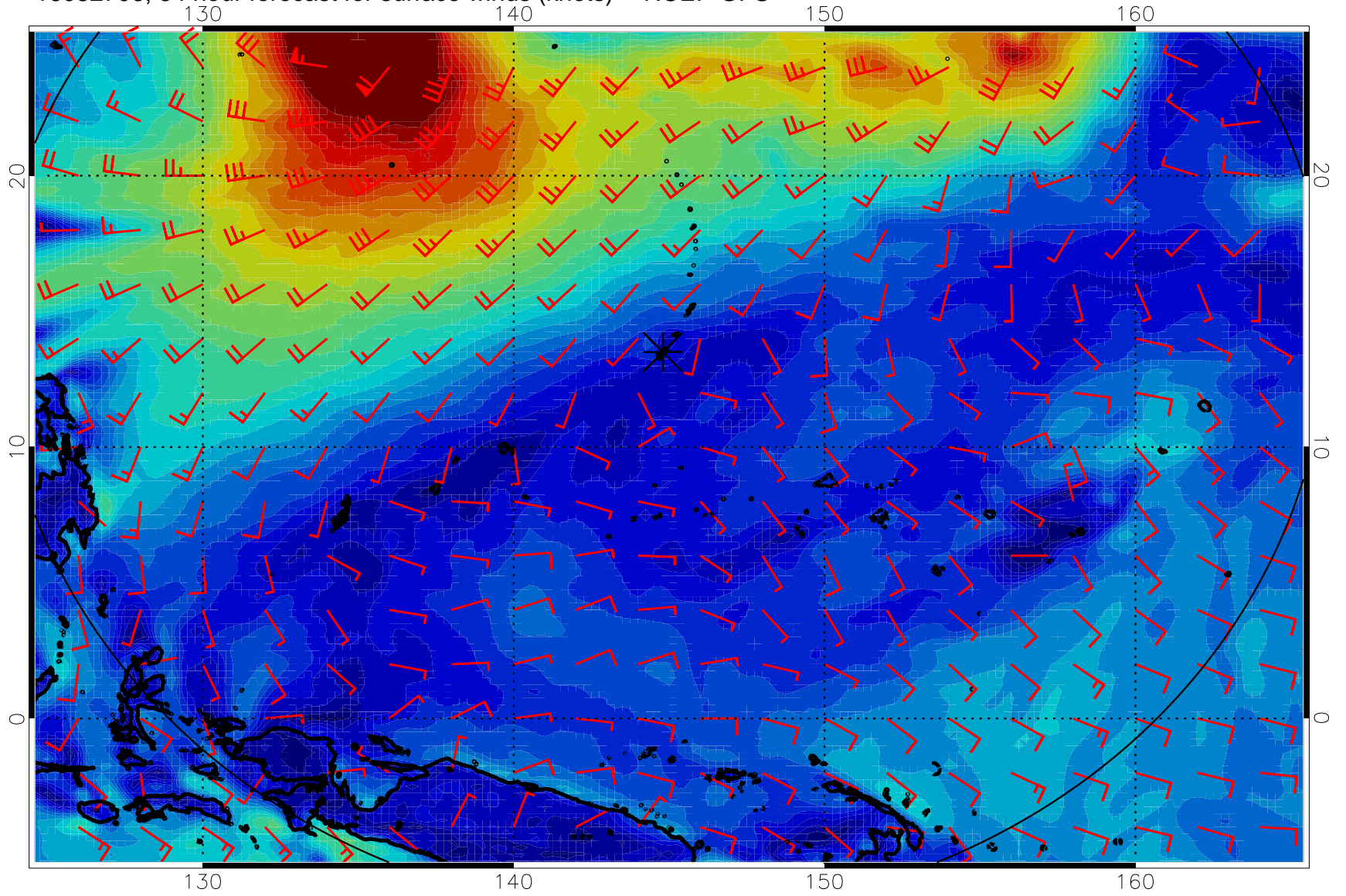
16082706, 54 hour forecast for surface winds (knots) -- NCEP GFS
