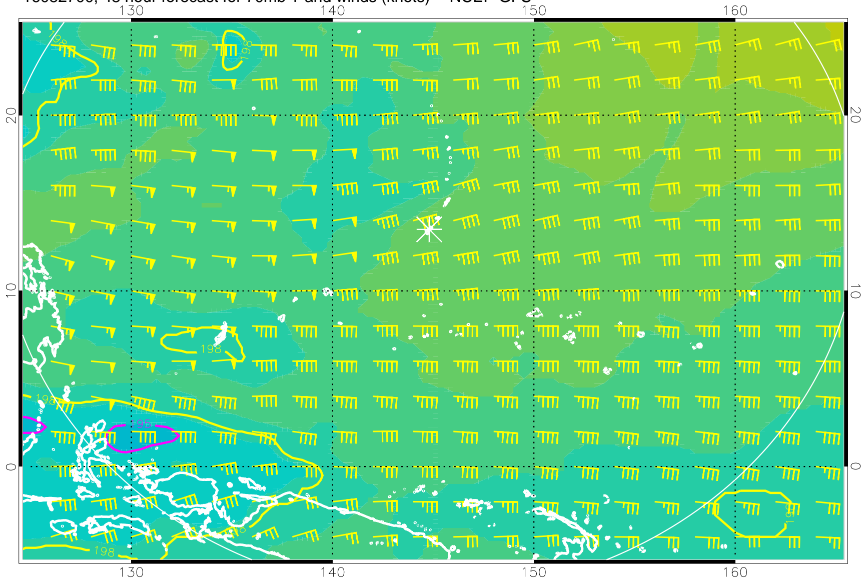
16082700, 48 hour forecast for 70mb T and winds (knots) -- NCEP GFS
