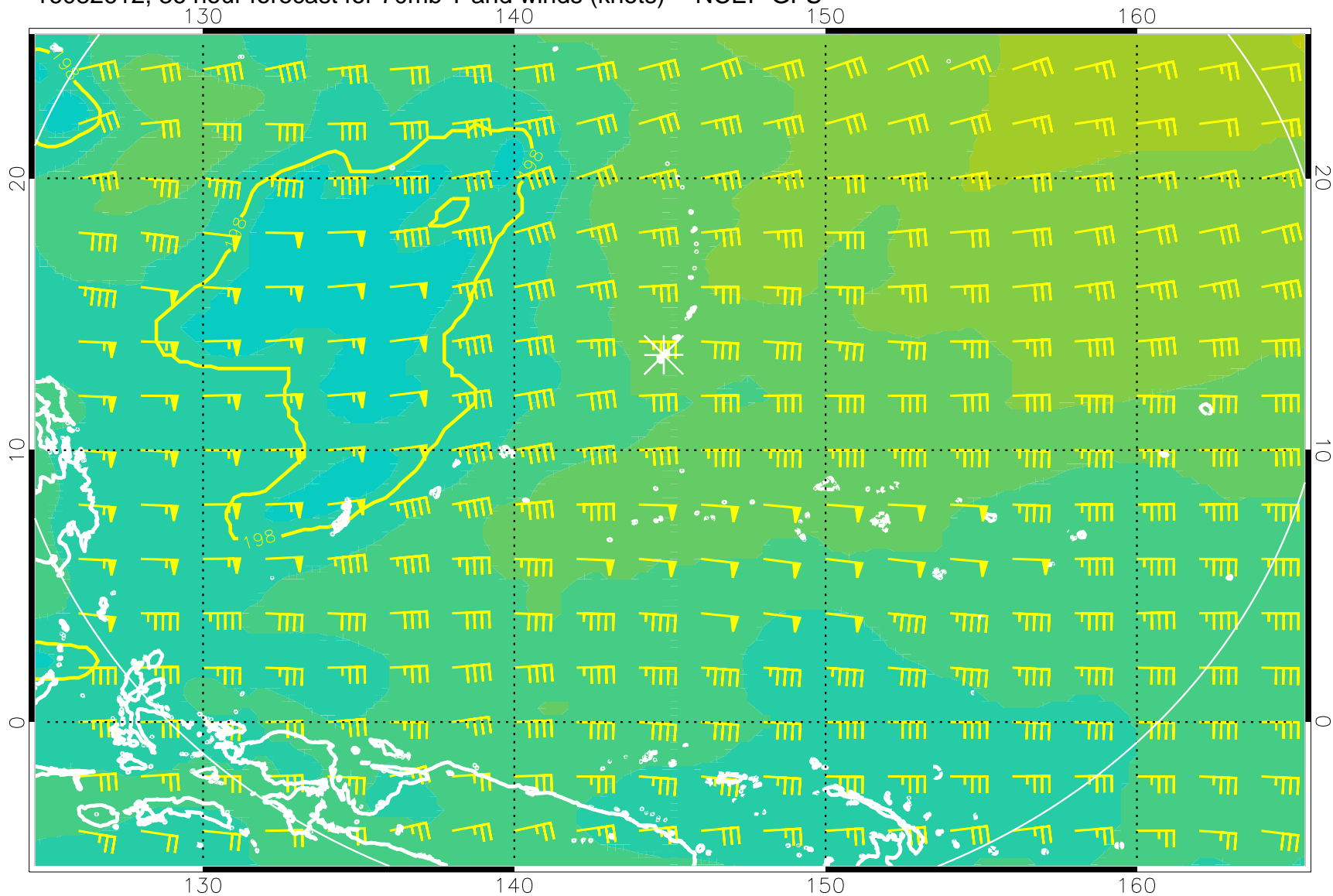
16082612, 36 hour forecast for 70mb T and winds (knots) -- NCEP GFS
