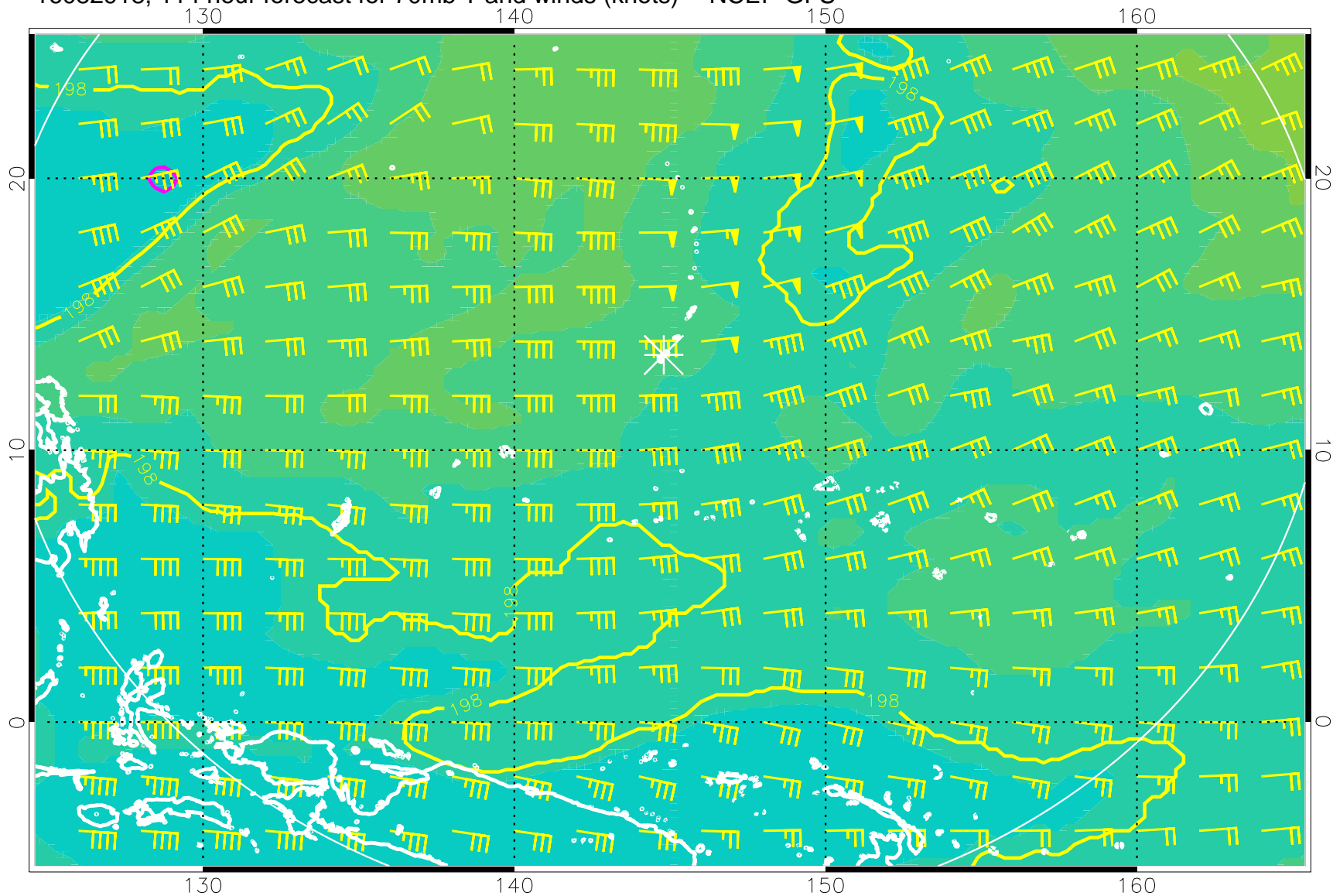
16082918, 114 hour forecast for 70mb T and winds (knots) -- NCEP GFS
