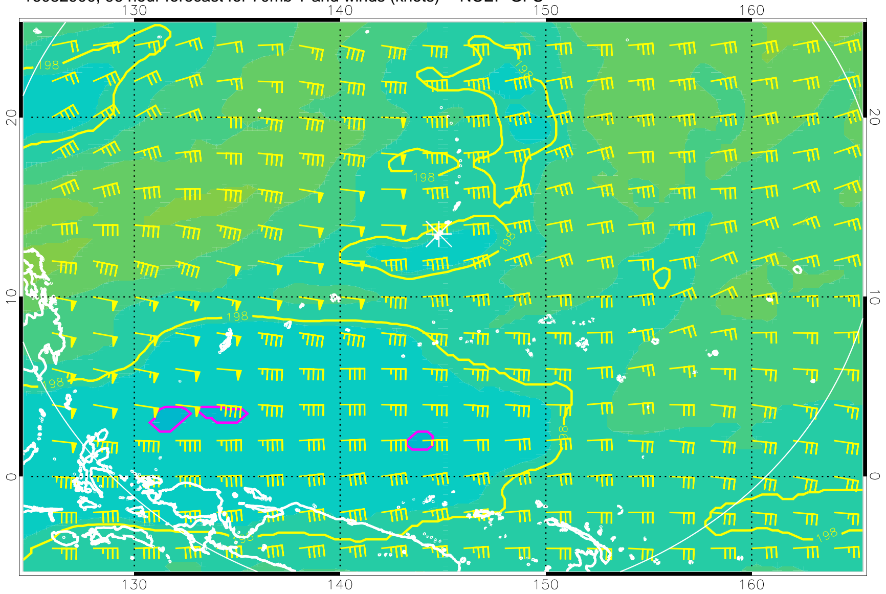
16082900, 96 hour forecast for 70mb T and winds (knots) -- NCEP GFS
