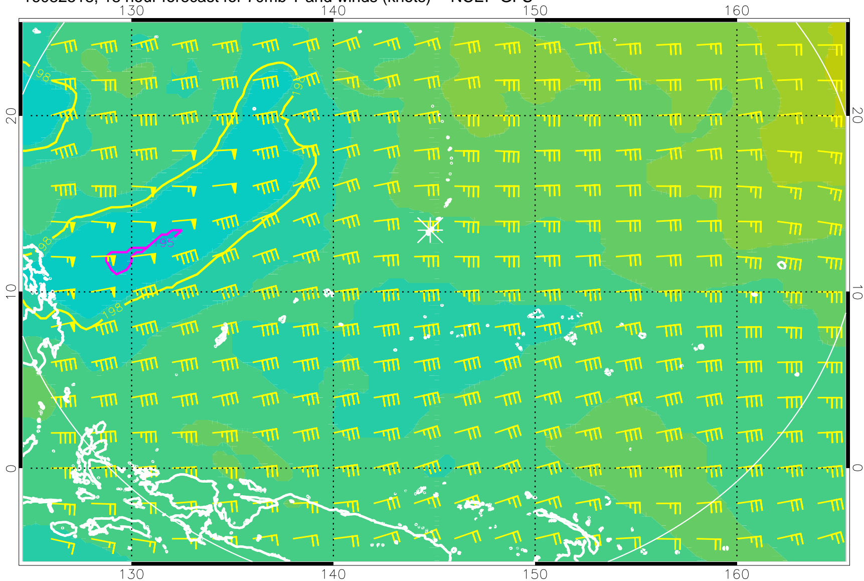
16082518, 18 hour forecast for 70mb T and winds (knots) -- NCEP GFS
