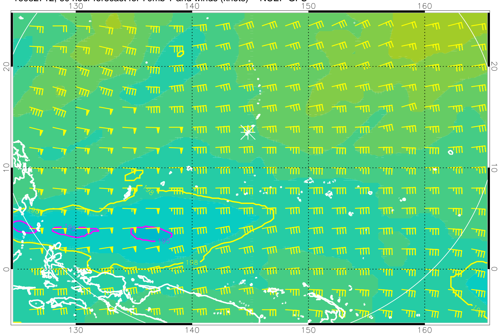
16082712, 60 hour forecast for 70mb T and winds (knots) -- NCEP GFS
