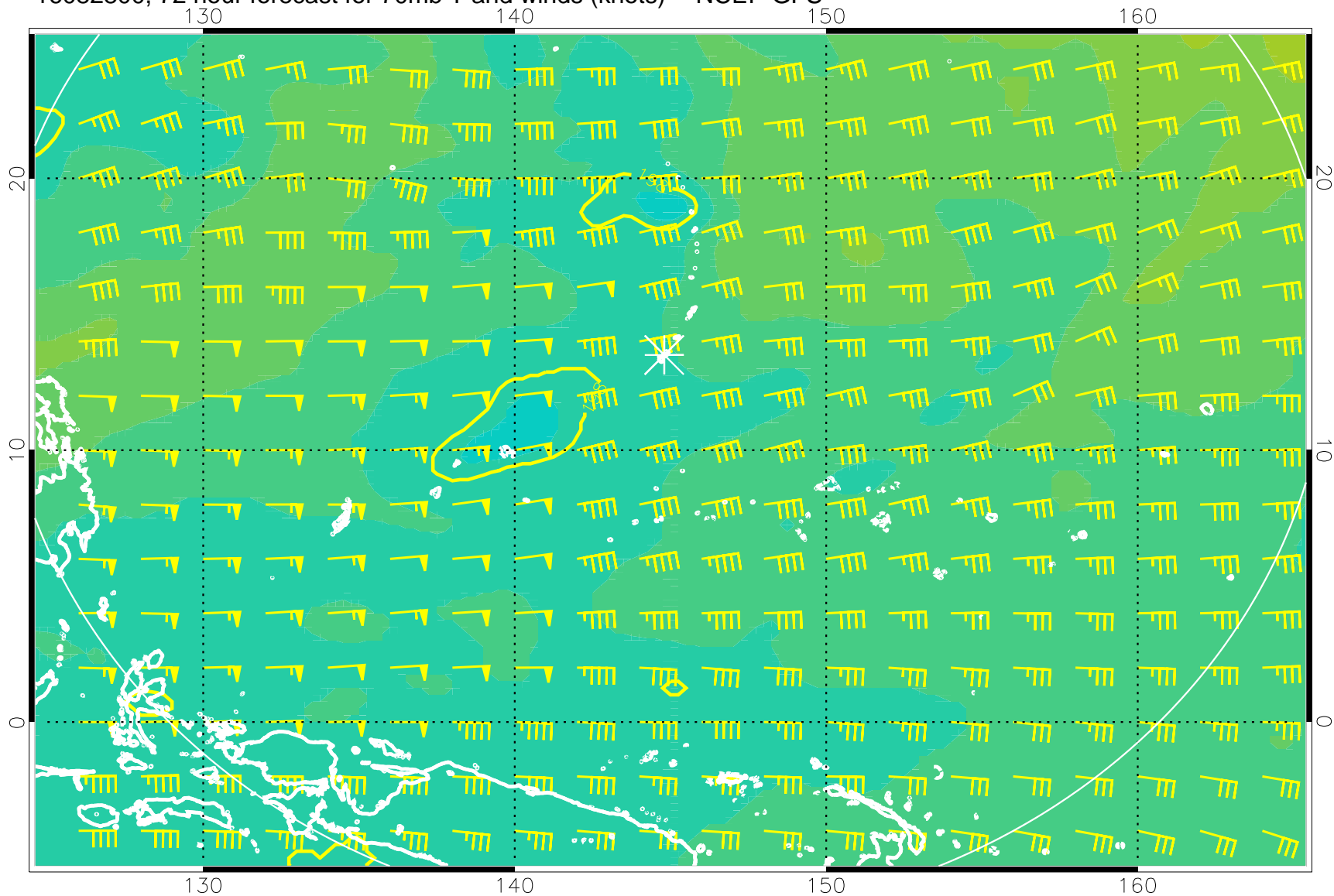
16082800, 72 hour forecast for 70mb T and winds (knots) -- NCEP GFS
