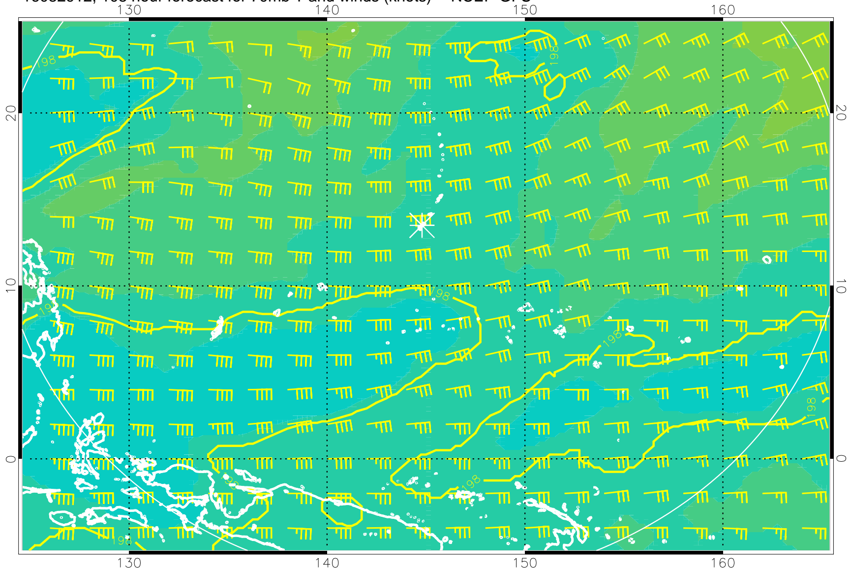
16082912, 108 hour forecast for 70mb T and winds (knots) -- NCEP GFS
