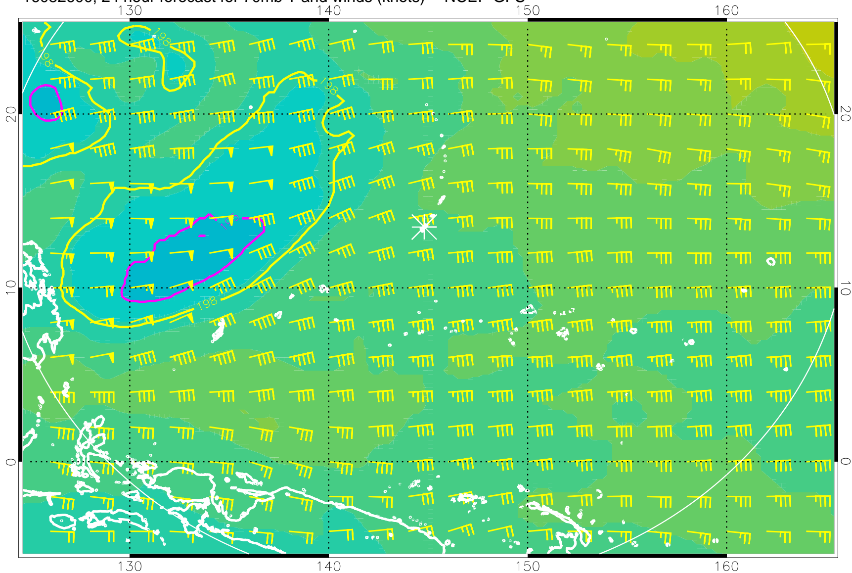
16082600, 24 hour forecast for 70mb T and winds (knots) -- NCEP GFS
