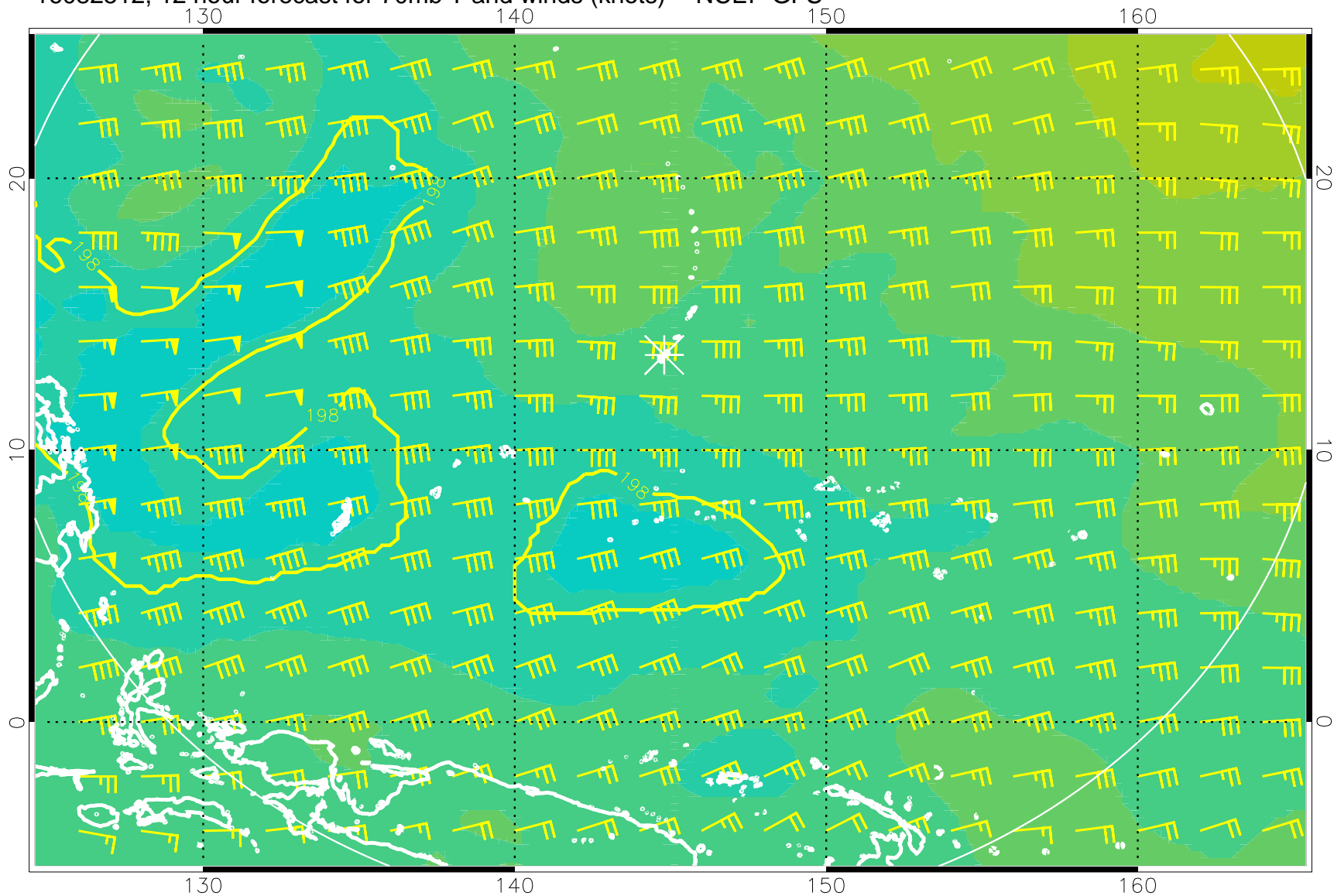
16082512, 12 hour forecast for 70mb T and winds (knots) -- NCEP GFS
