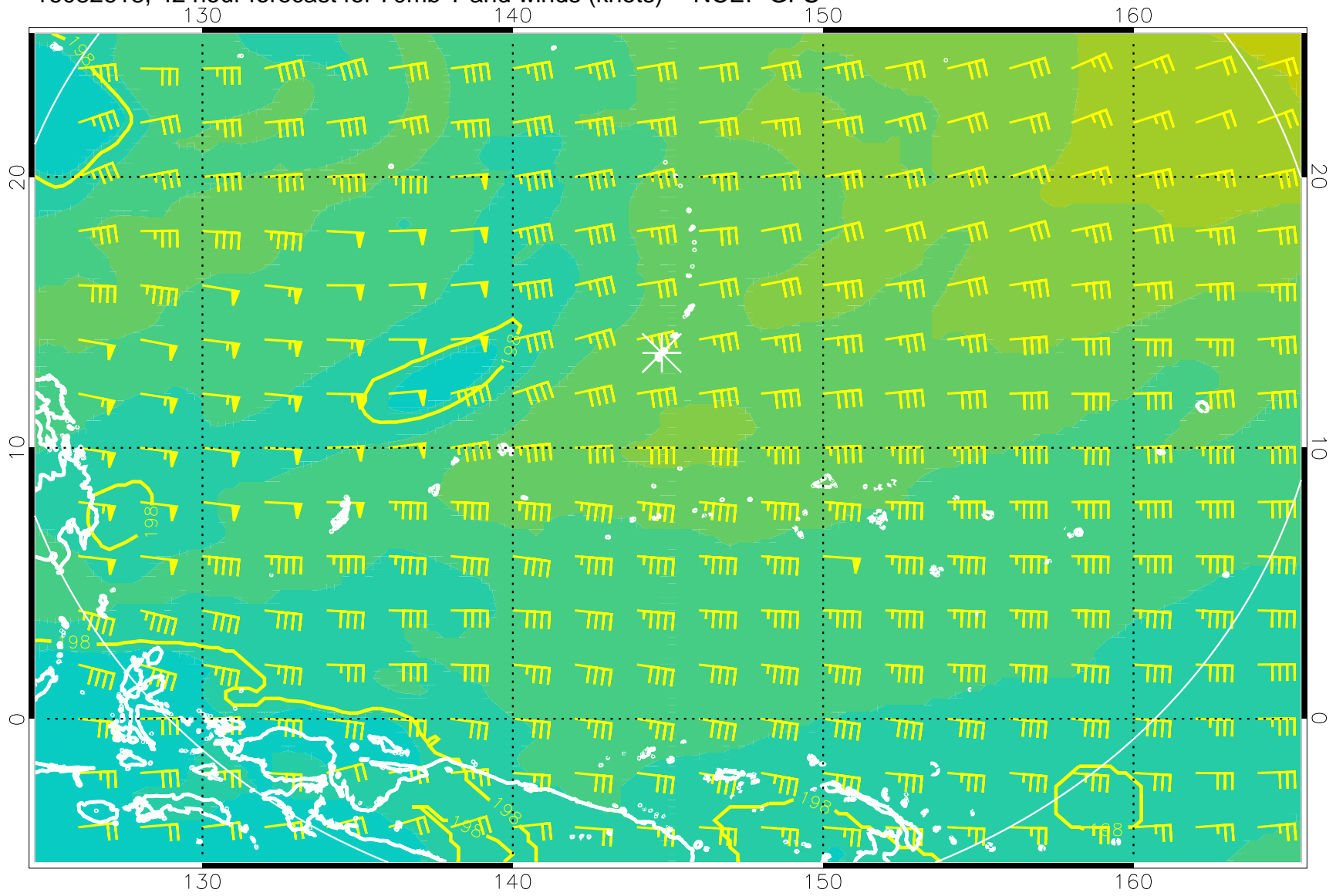
16082618, 42 hour forecast for 70mb T and winds (knots) -- NCEP GFS
