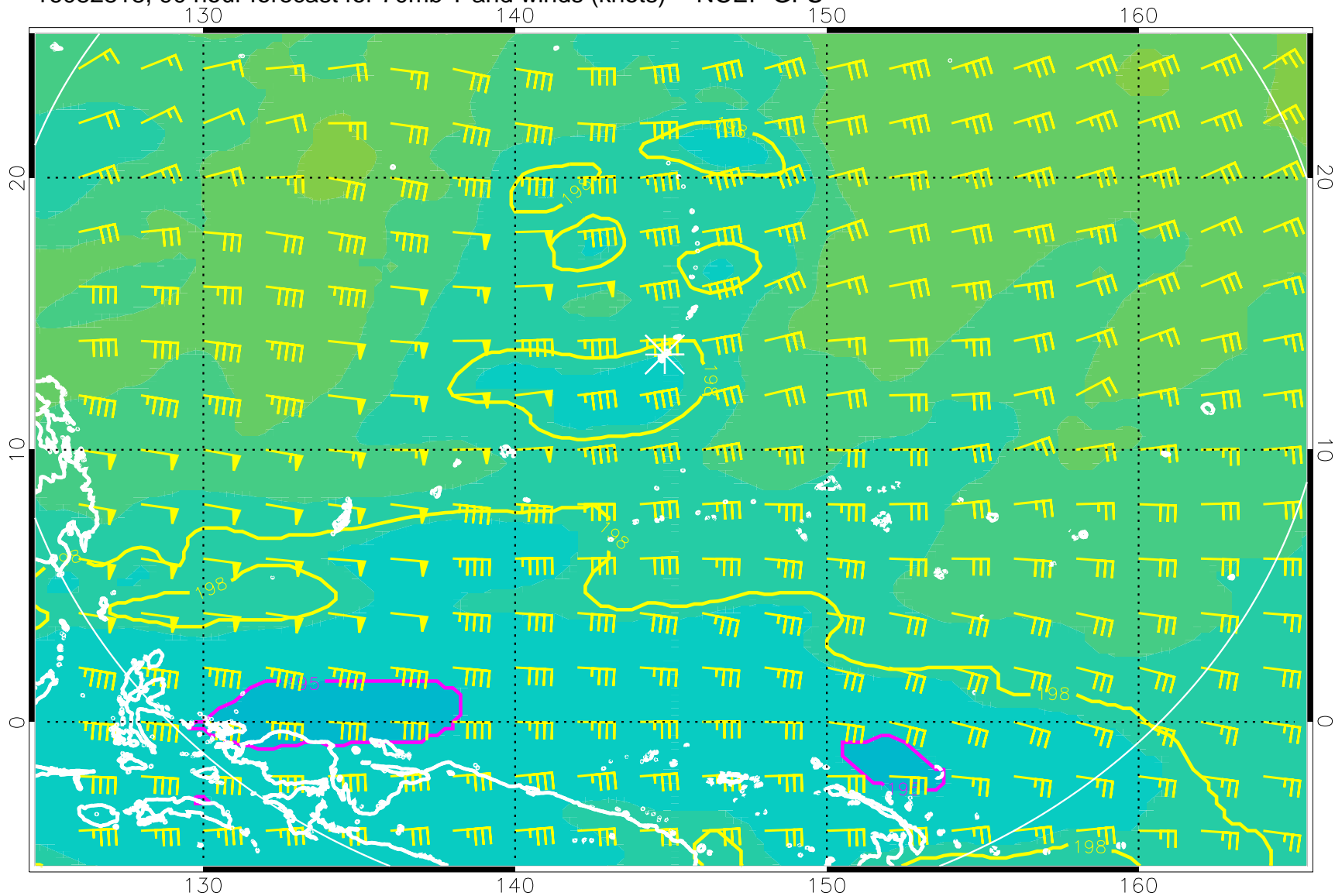
16082818, 90 hour forecast for 70mb T and winds (knots) -- NCEP GFS
