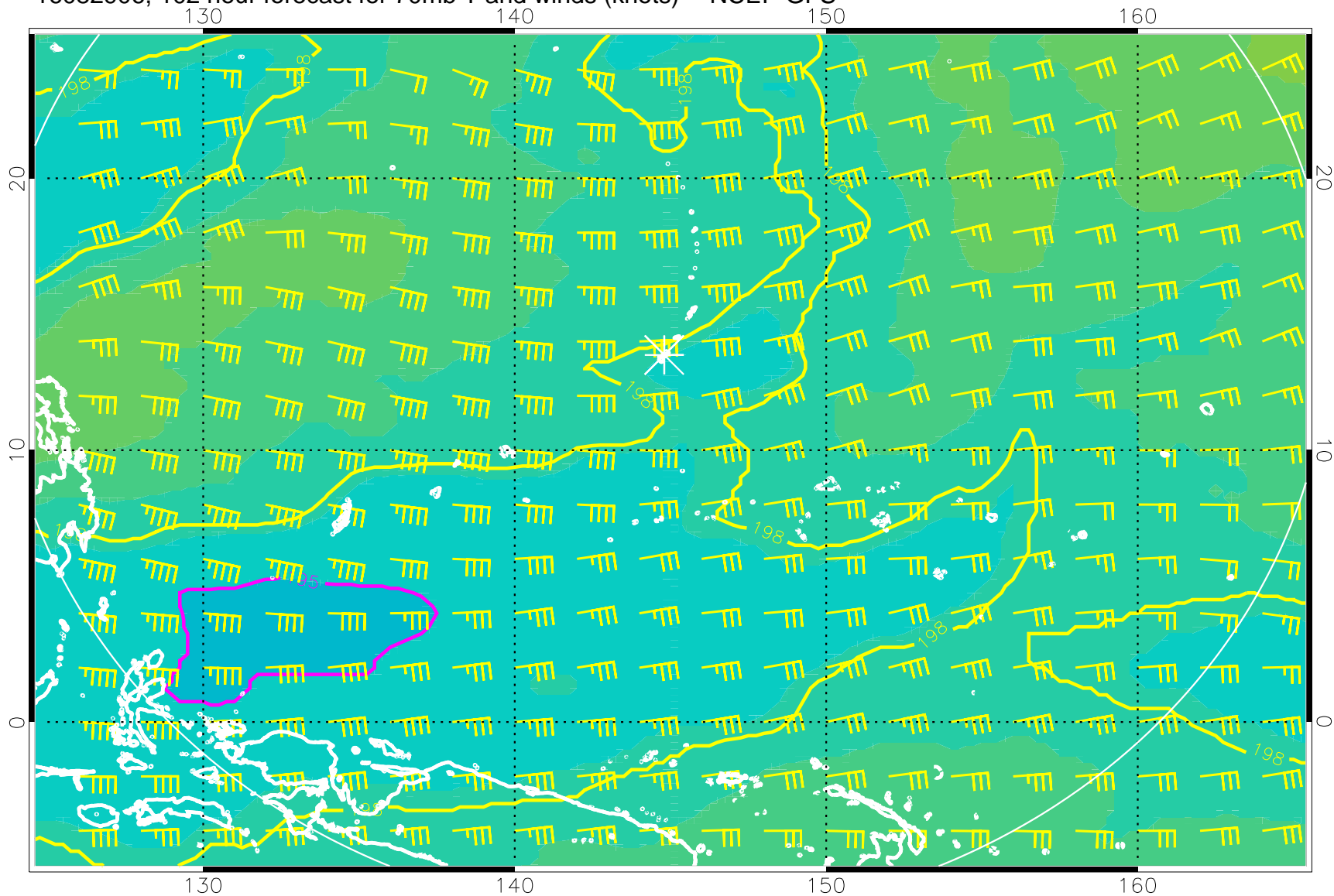
16082906, 102 hour forecast for 70mb T and winds (knots) -- NCEP GFS
