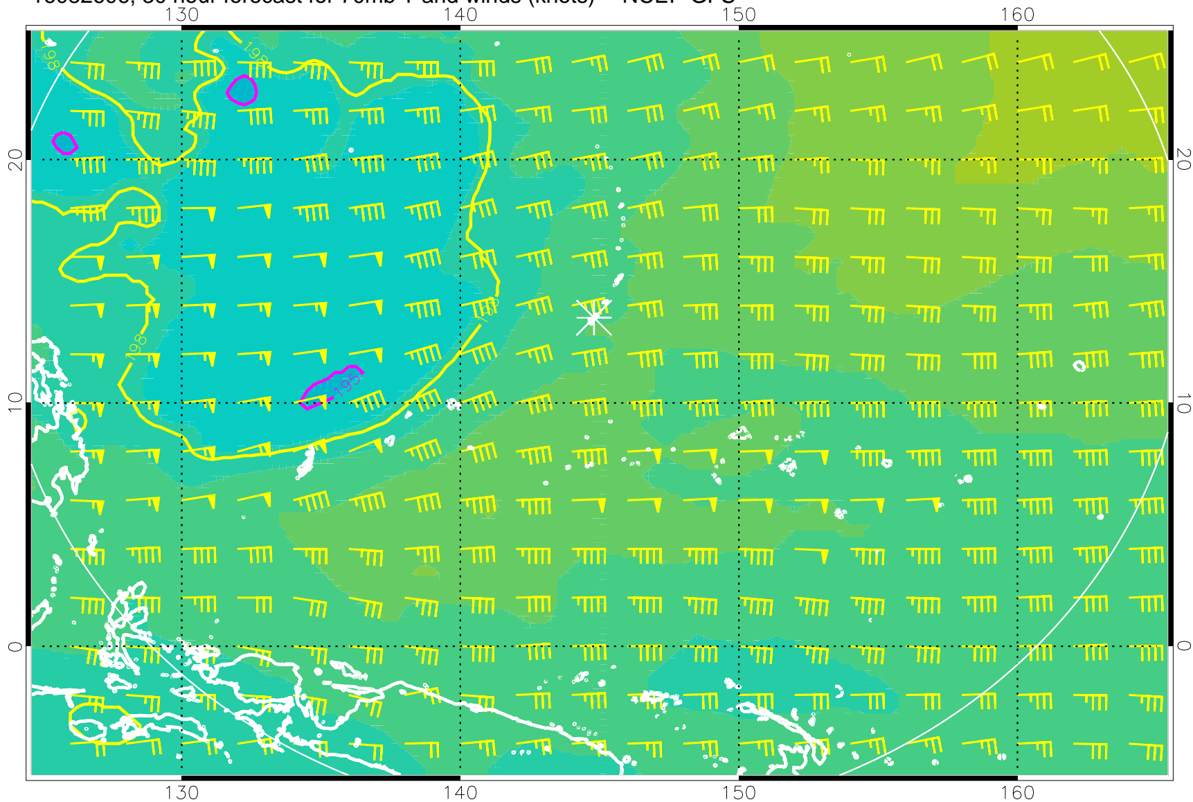
16082606, 30 hour forecast for 70mb T and winds (knots) -- NCEP GFS
