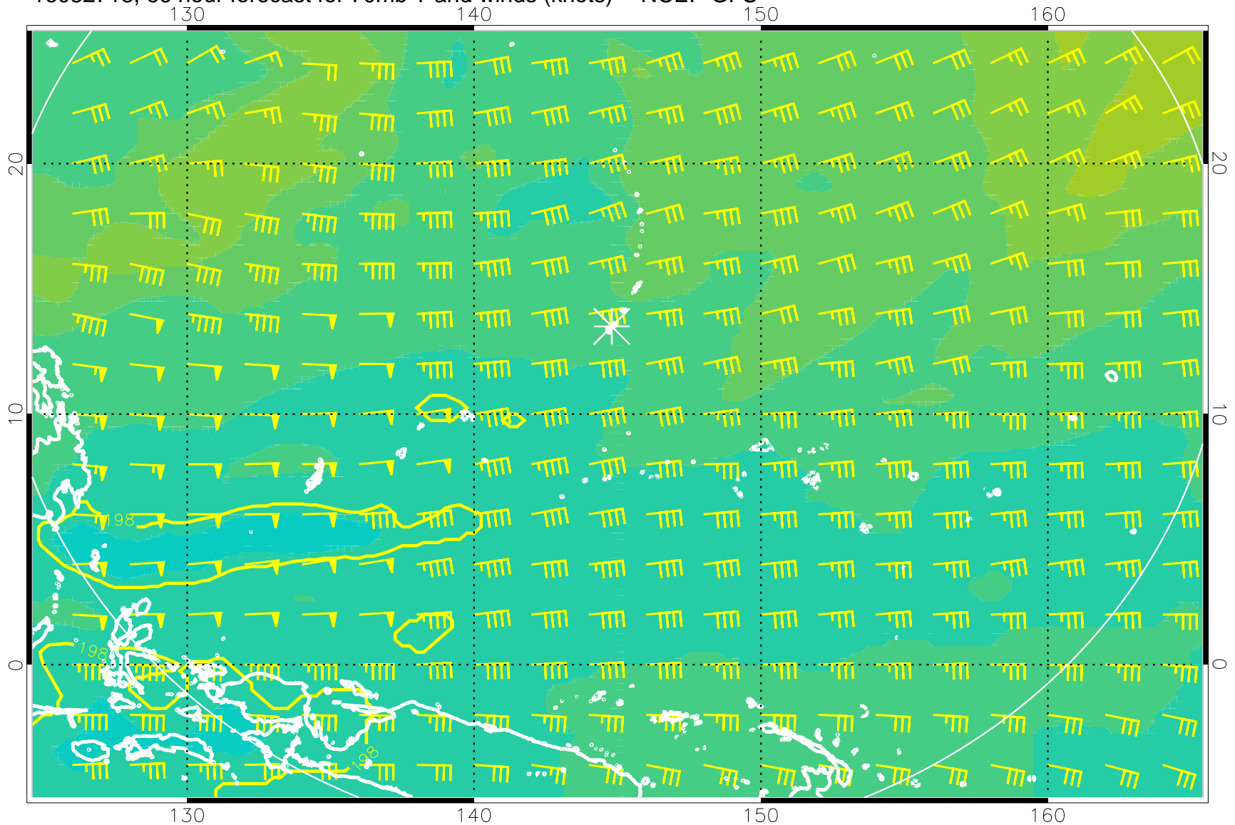
16082718, 66 hour forecast for 70mb T and winds (knots) -- NCEP GFS
