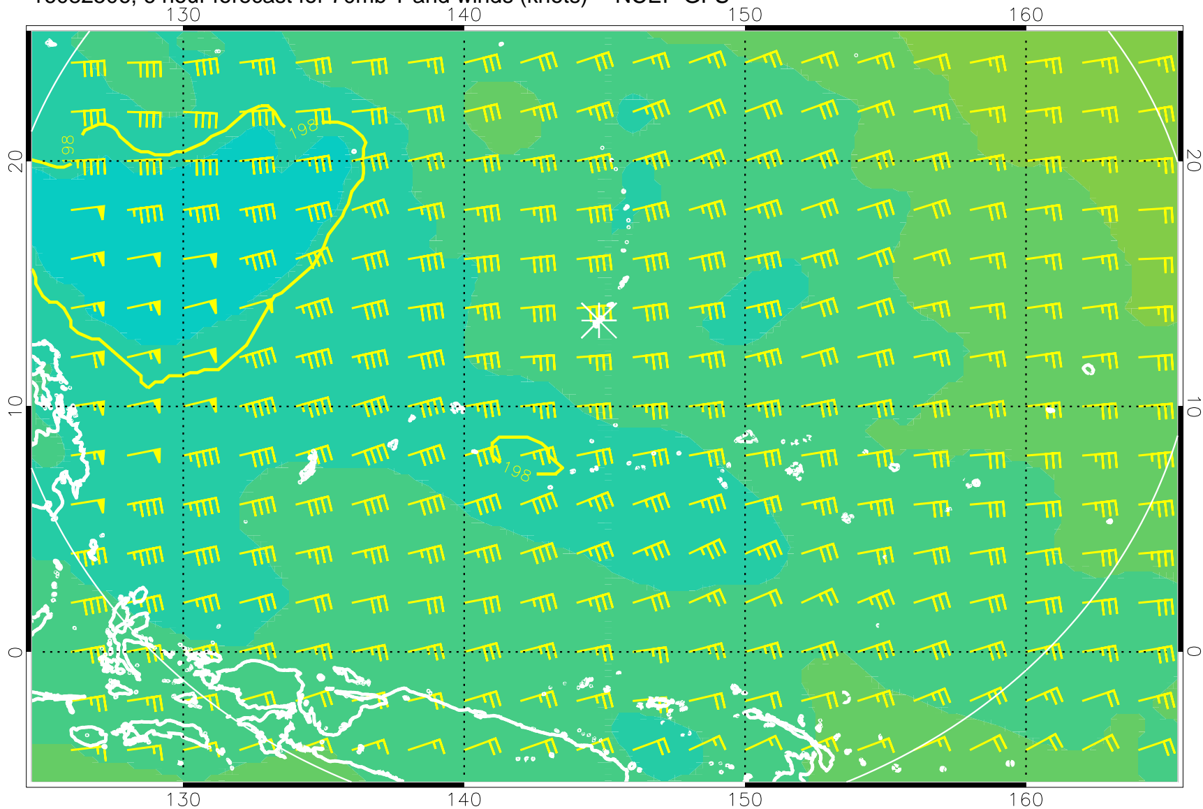
16082506, 6 hour forecast for 70mb T and winds (knots) -- NCEP GFS
