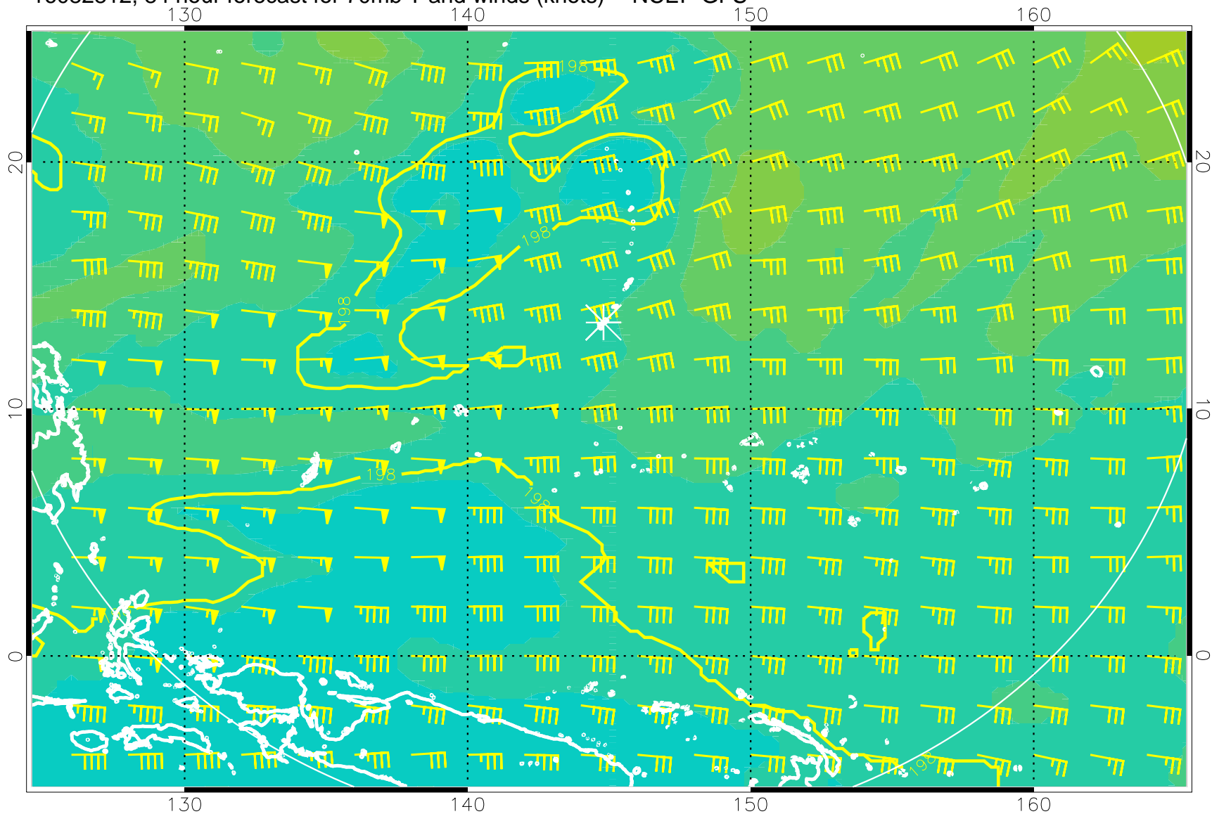
16082812, 84 hour forecast for 70mb T and winds (knots) -- NCEP GFS
