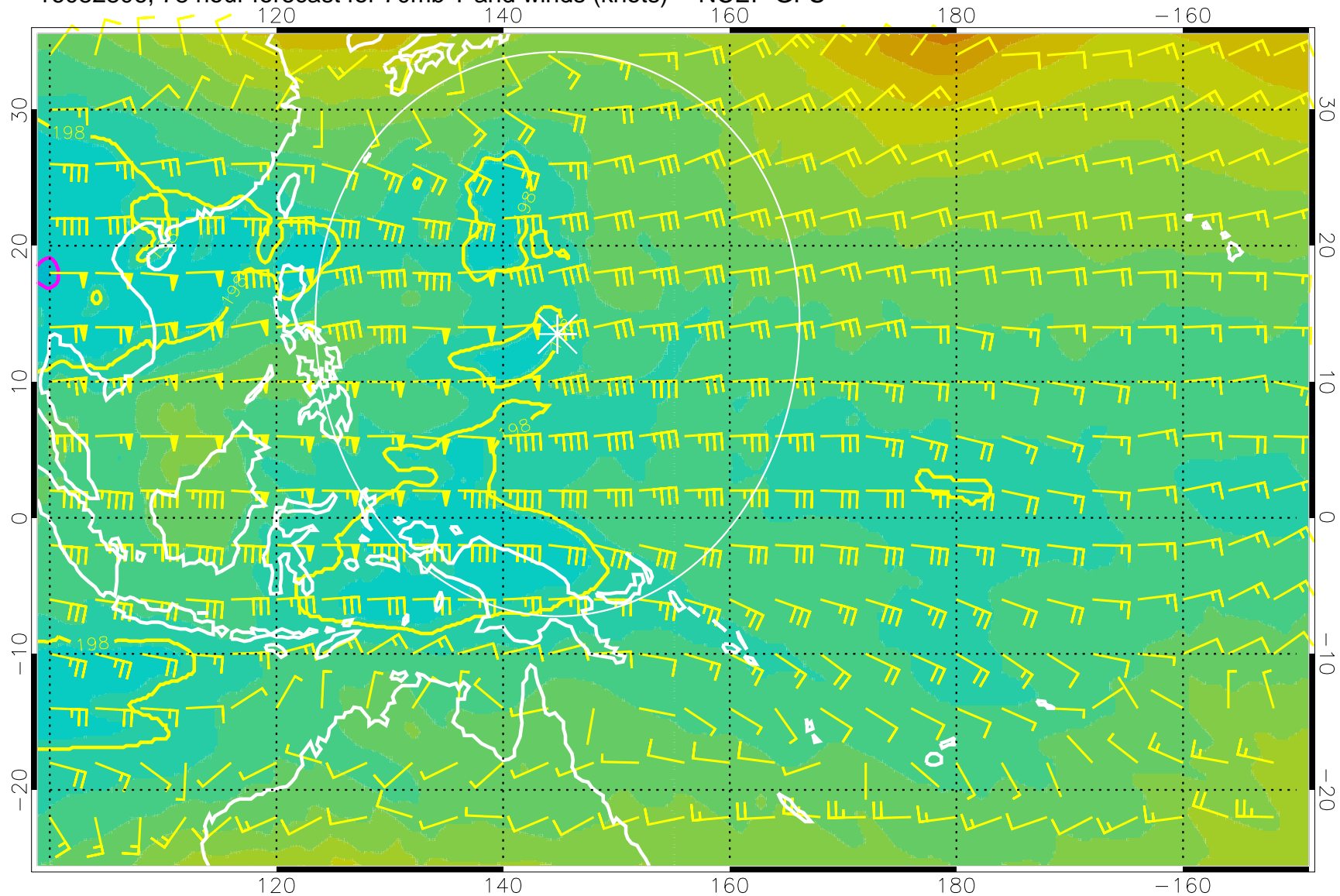
16082806, 78 hour forecast for 70mb T and winds (knots) -- NCEP GFS
