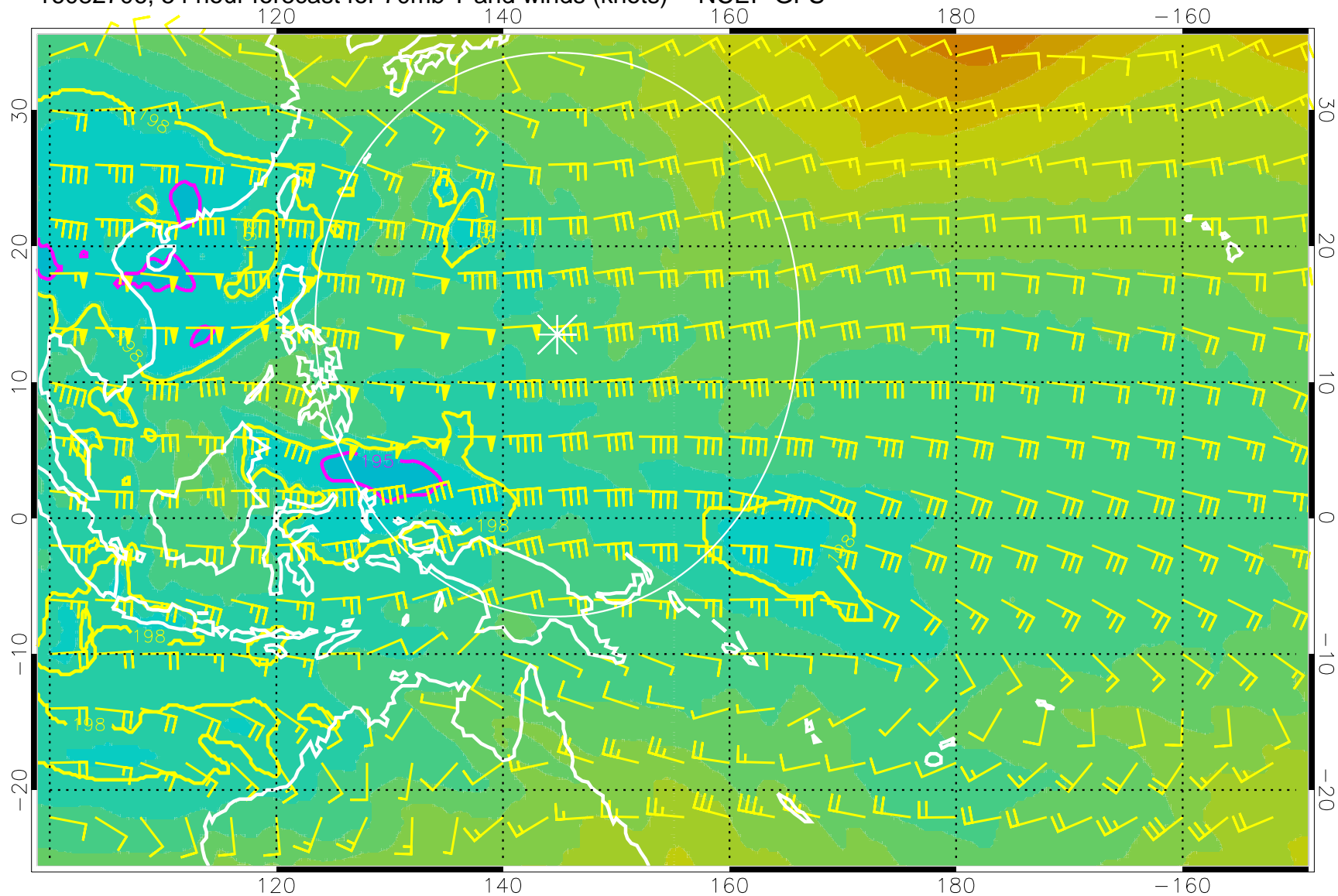
16082706, 54 hour forecast for 70mb T and winds (knots) -- NCEP GFS
