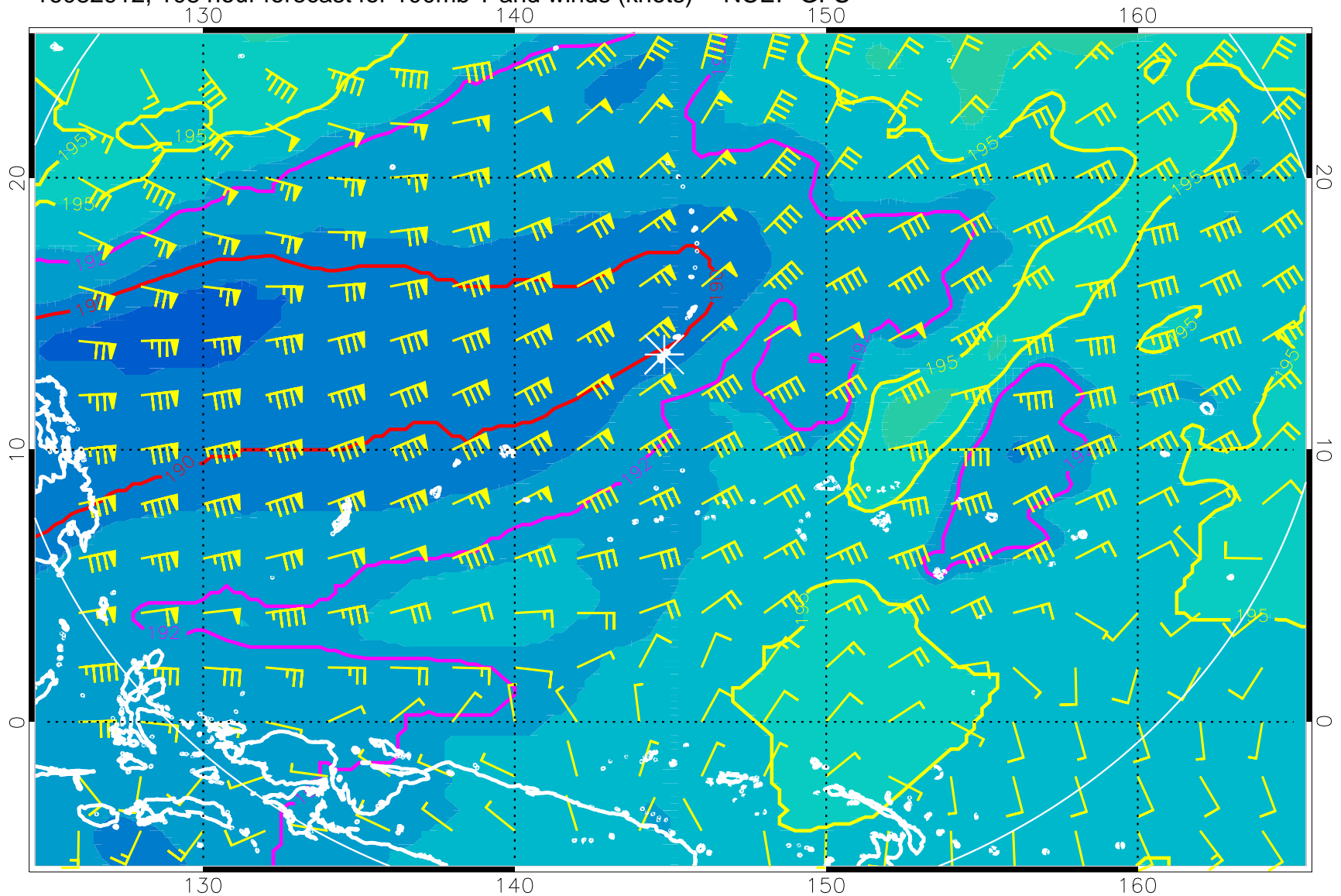
16082912, 108 hour forecast for 100mb T and winds (knots) -- NCEP GFS
