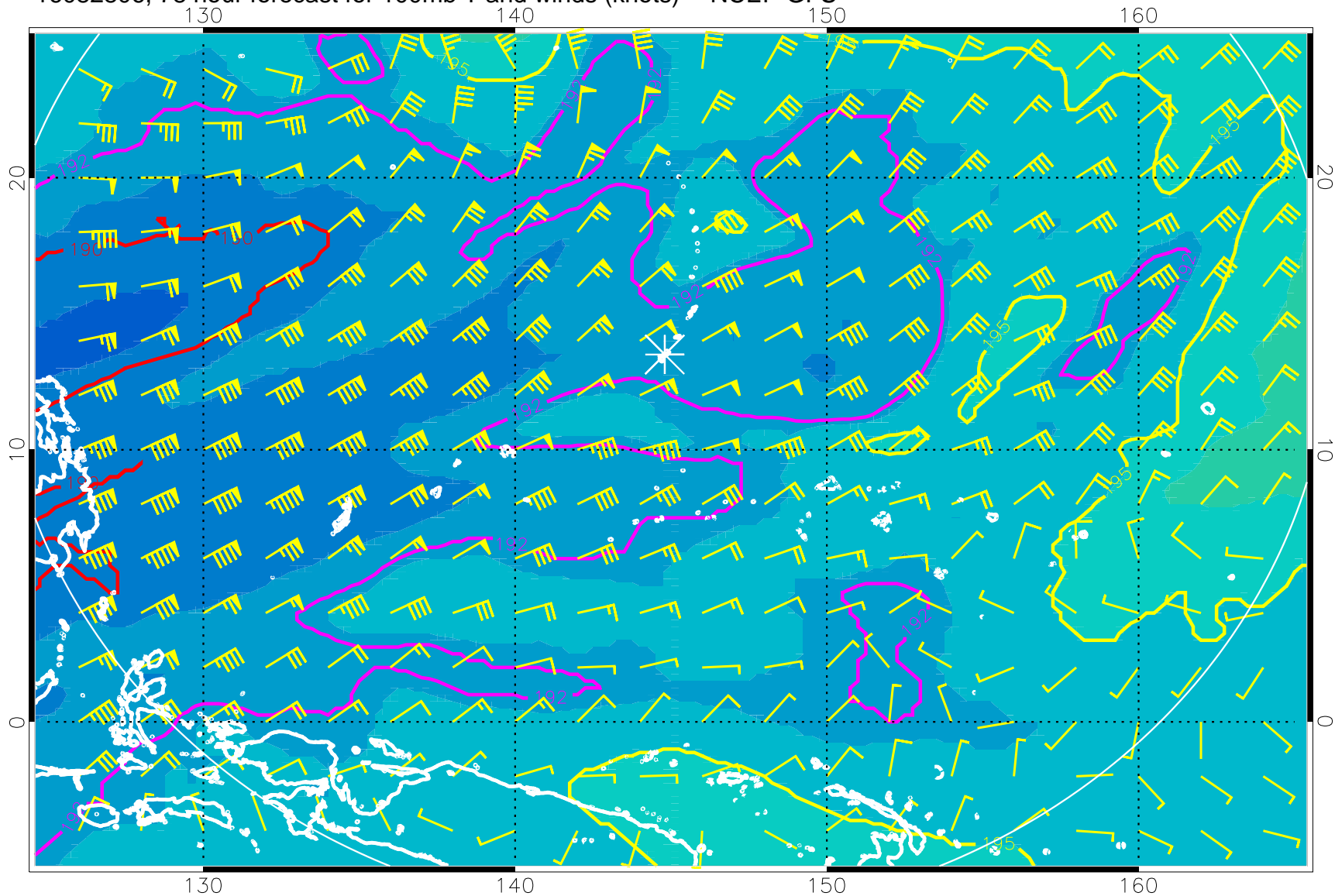
16082806, 78 hour forecast for 100mb T and winds (knots) -- NCEP GFS
