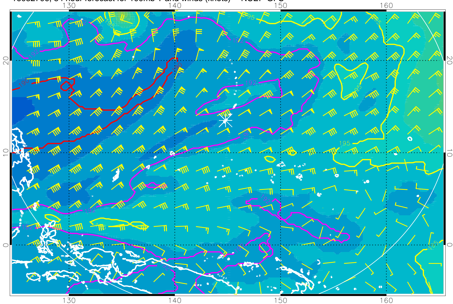
16082706, 54 hour forecast for 100mb T and winds (knots) -- NCEP GFS
