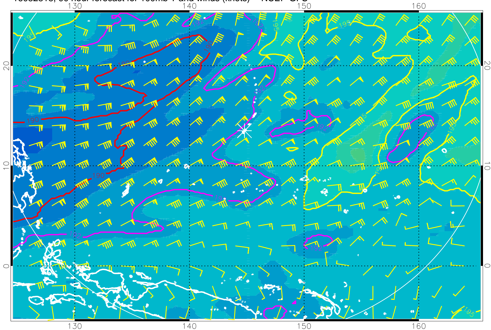
16082818, 90 hour forecast for 100mb T and winds (knots) -- NCEP GFS
