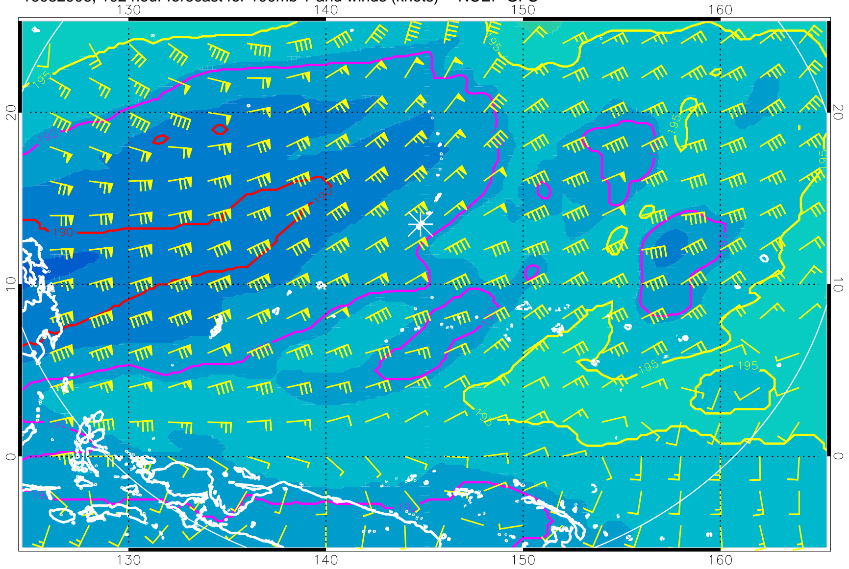
16082906, 102 hour forecast for 100mb T and winds (knots) -- NCEP GFS
