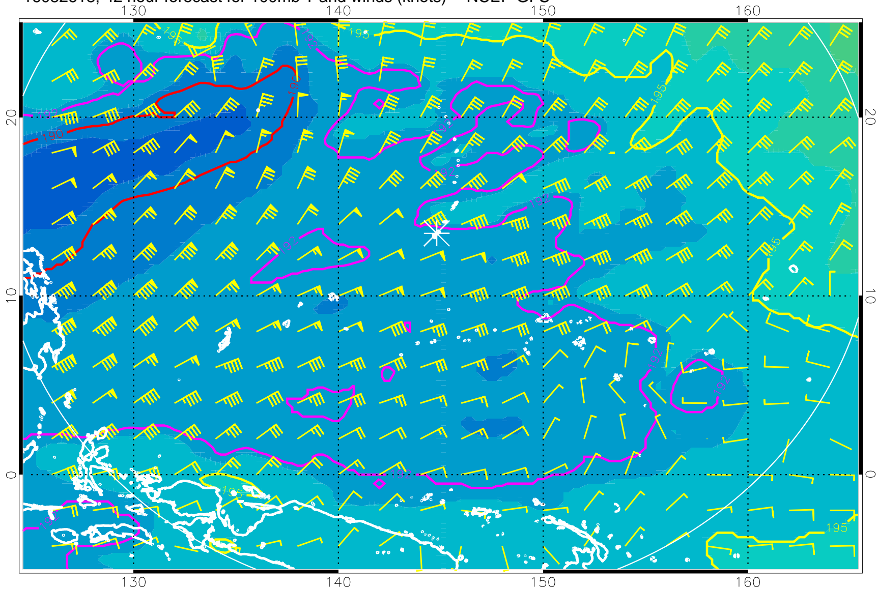
16082618, 42 hour forecast for 100mb T and winds (knots) -- NCEP GFS
