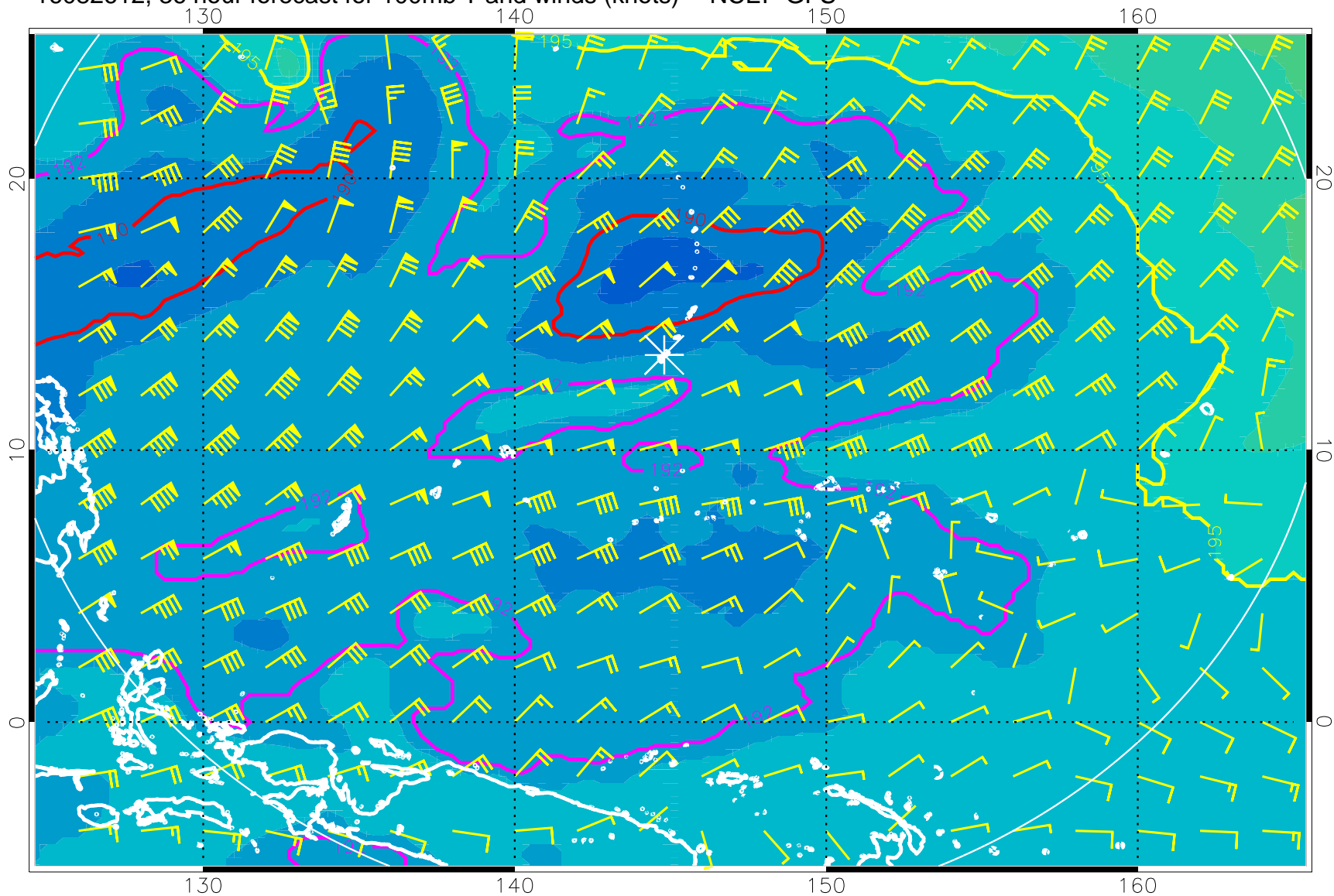
16082612, 36 hour forecast for 100mb T and winds (knots) -- NCEP GFS
