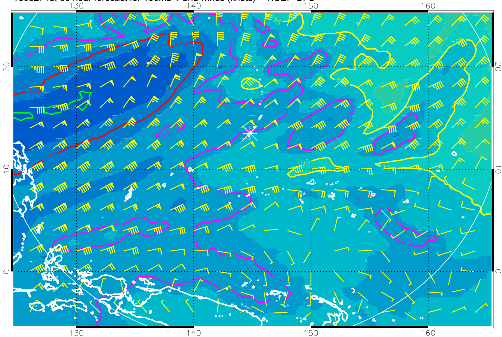
16082718, 66 hour forecast for 100mb T and winds (knots) -- NCEP GFS
