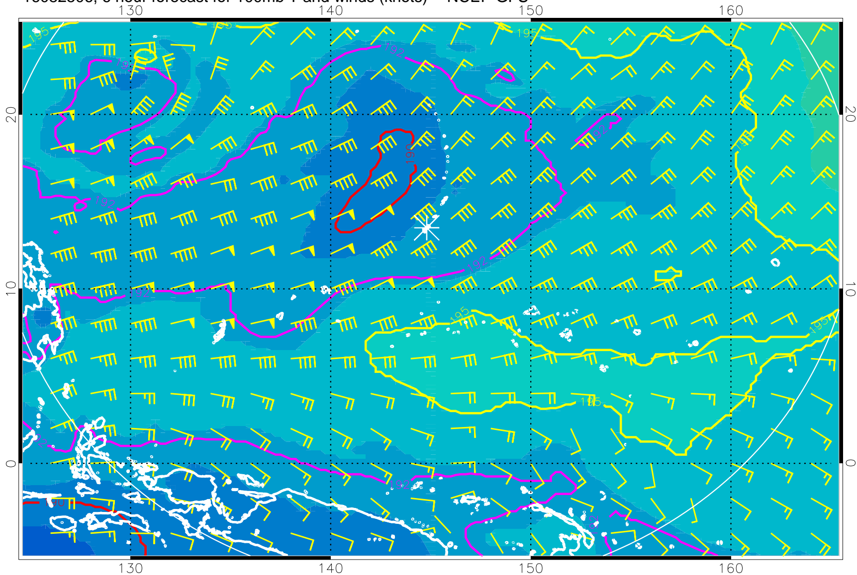
16082506, 6 hour forecast for 100mb T and winds (knots) -- NCEP GFS
