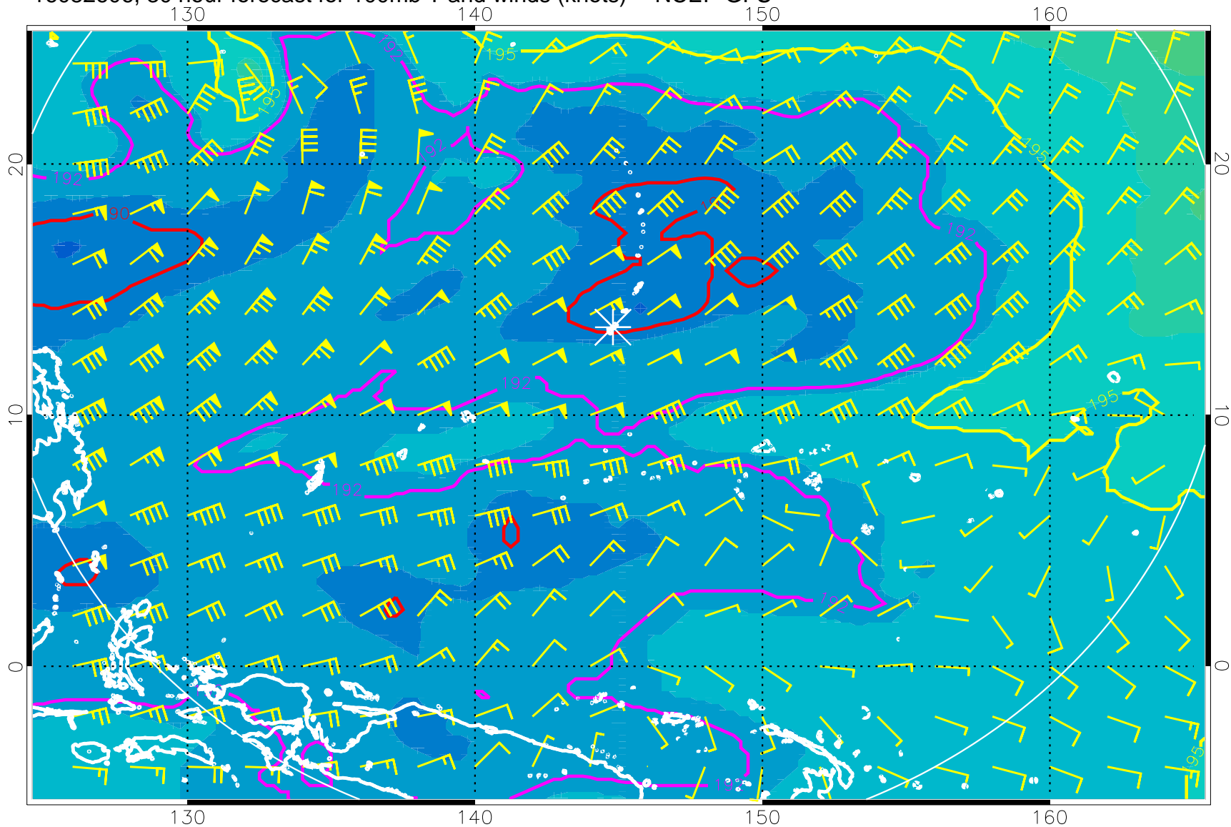
16082606, 30 hour forecast for 100mb T and winds (knots) -- NCEP GFS
