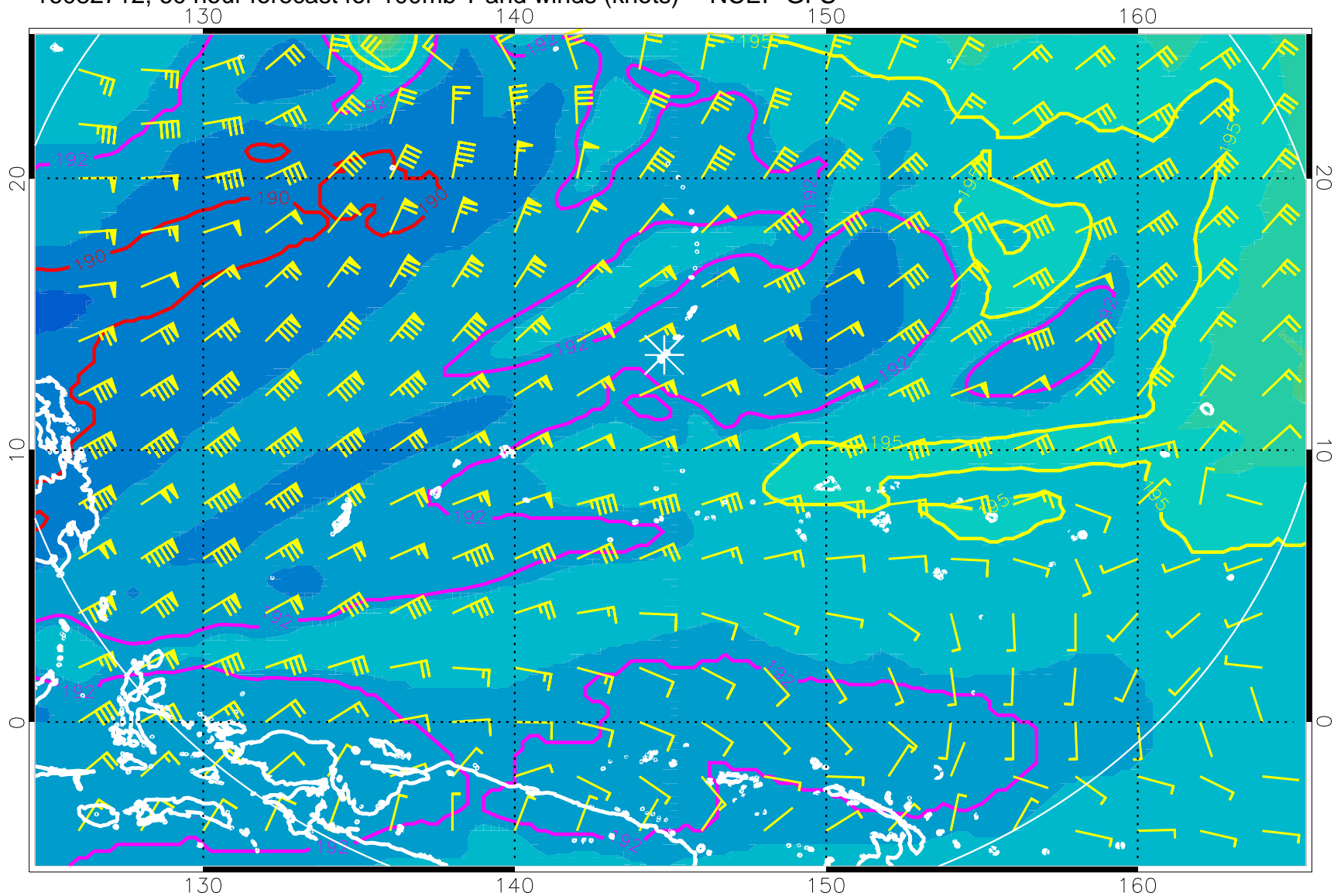
16082712, 60 hour forecast for 100mb T and winds (knots) -- NCEP GFS
