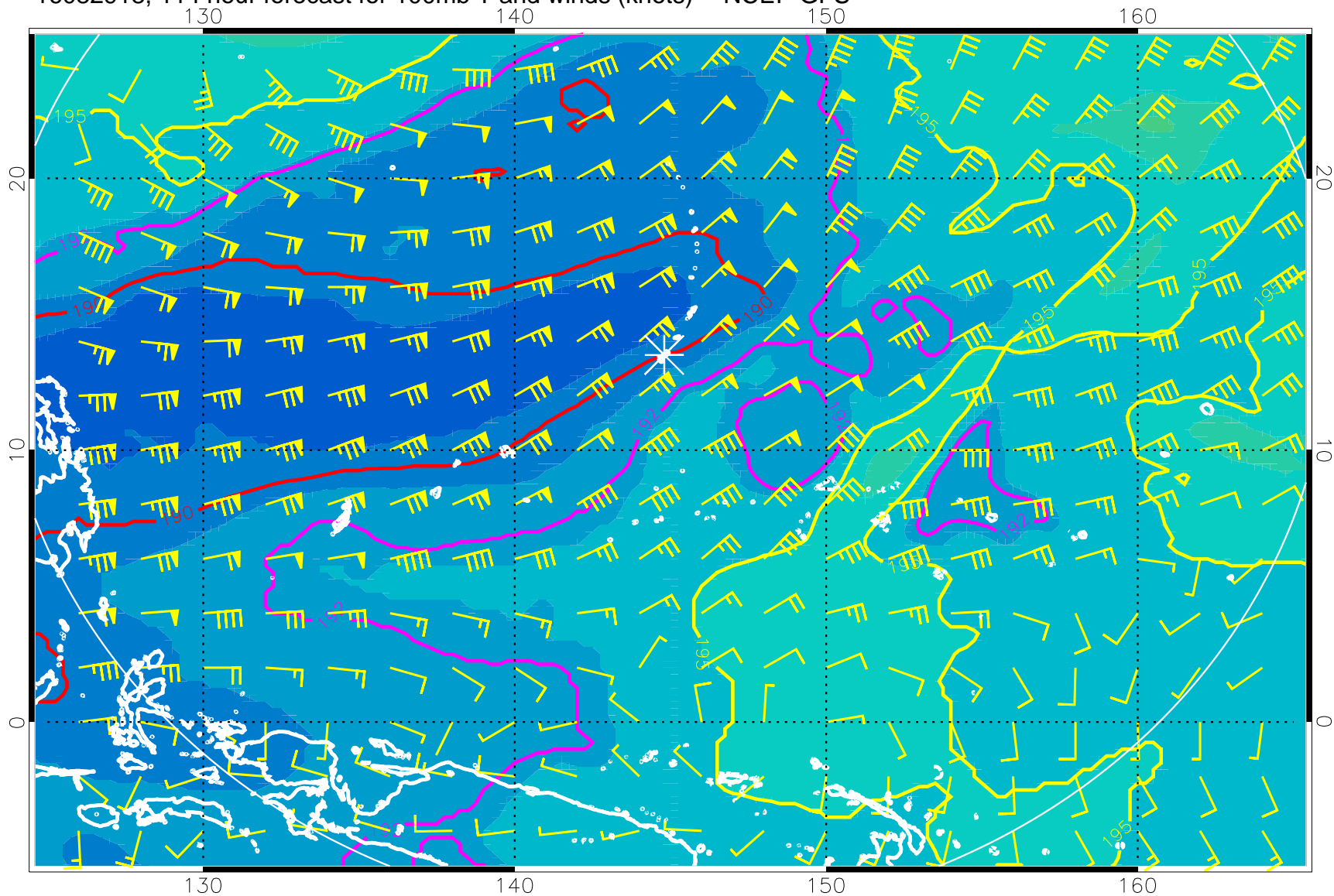
16082918, 114 hour forecast for 100mb T and winds (knots) -- NCEP GFS
