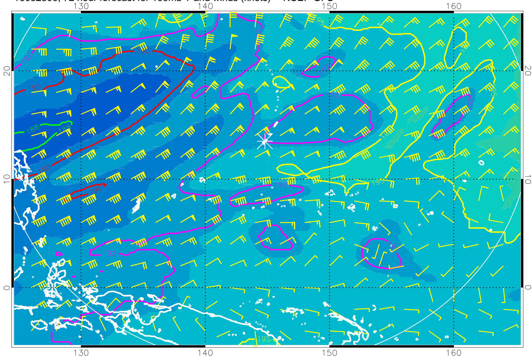
16082800, 72 hour forecast for 100mb T and winds (knots) -- NCEP GFS
