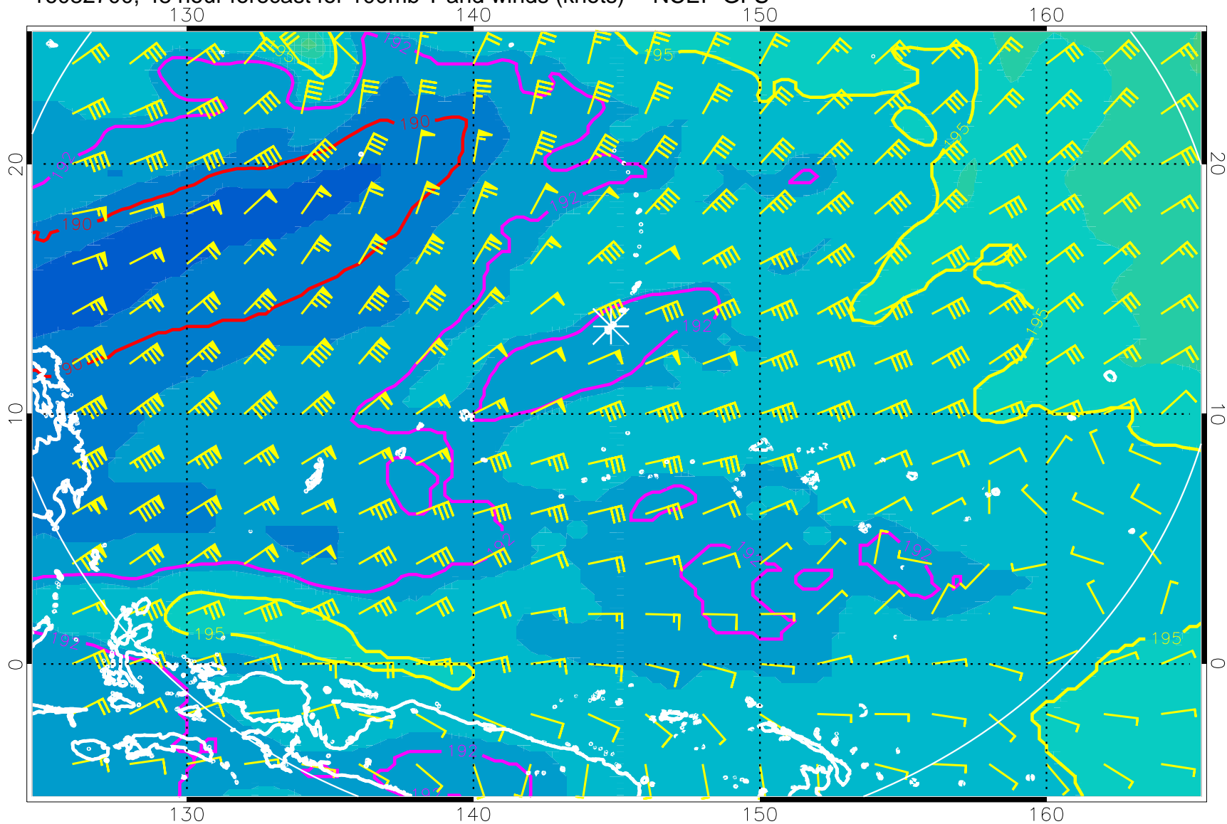
16082700, 48 hour forecast for 100mb T and winds (knots) -- NCEP GFS
