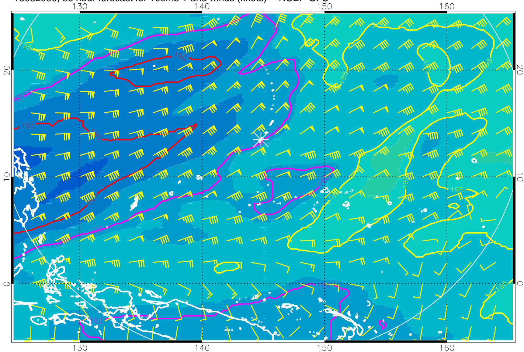
16082900, 96 hour forecast for 100mb T and winds (knots) -- NCEP GFS
