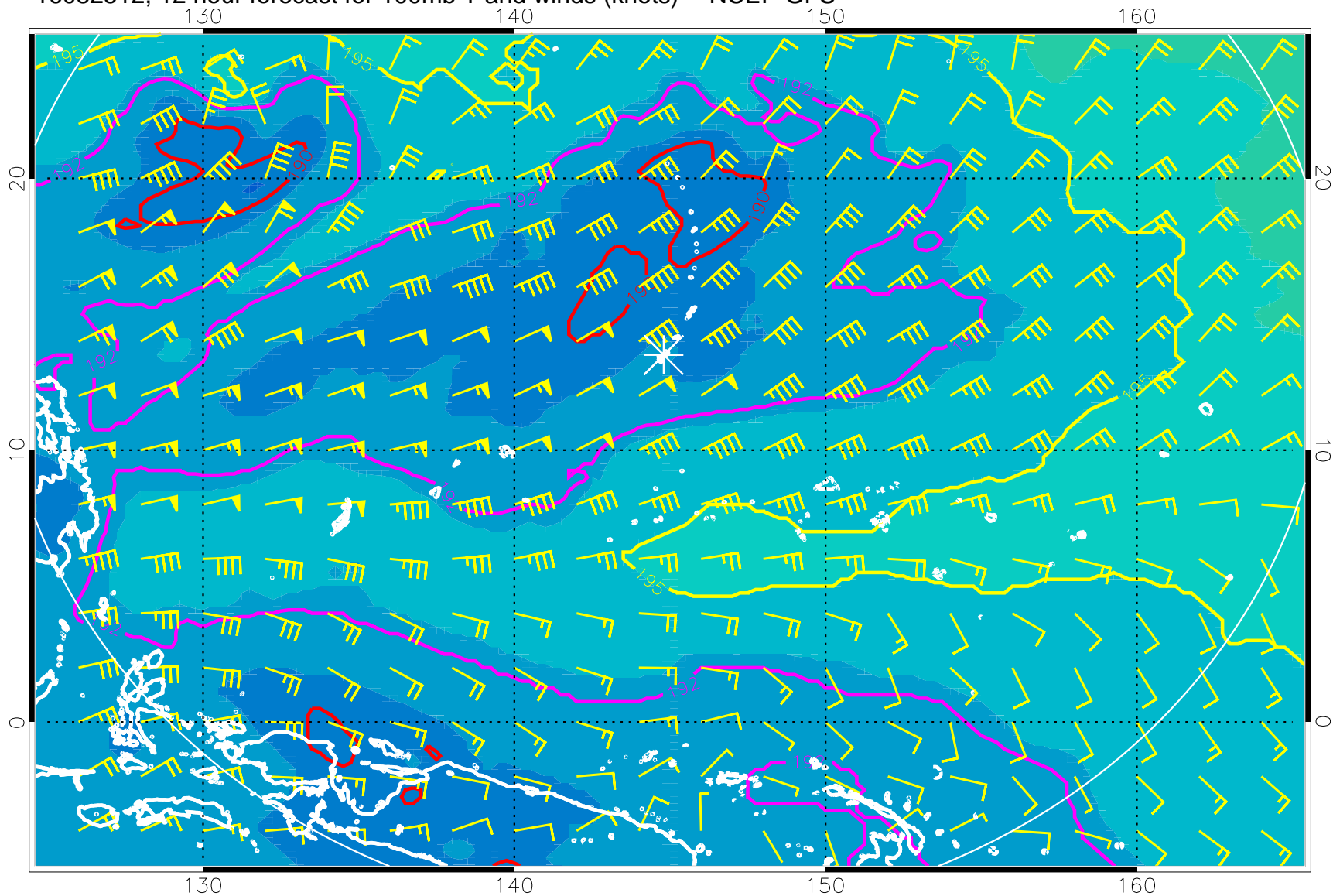
16082512, 12 hour forecast for 100mb T and winds (knots) -- NCEP GFS
