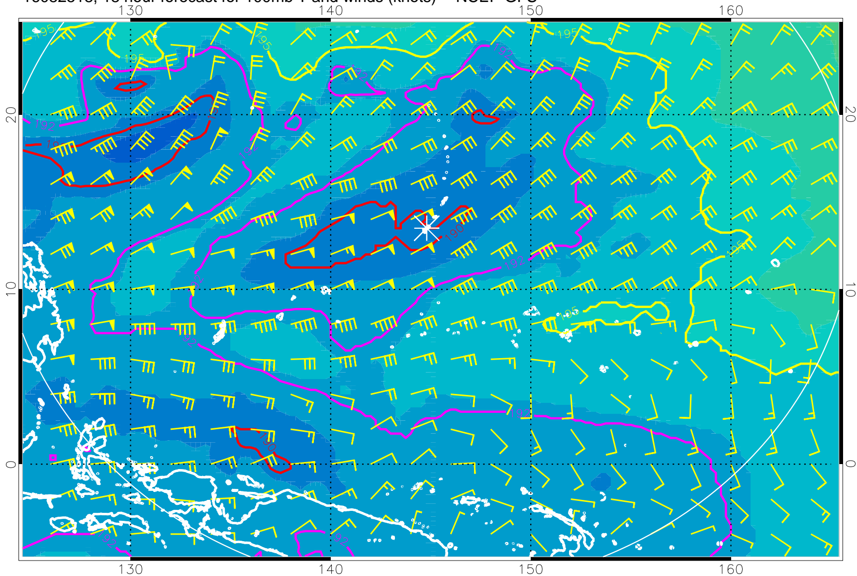
16082518, 18 hour forecast for 100mb T and winds (knots) -- NCEP GFS
