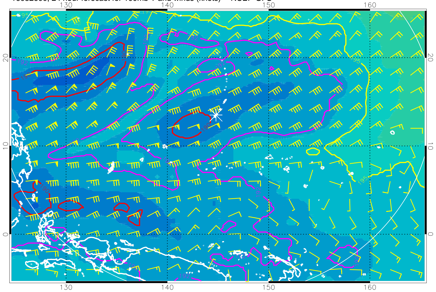
16082600, 24 hour forecast for 100mb T and winds (knots) -- NCEP GFS
