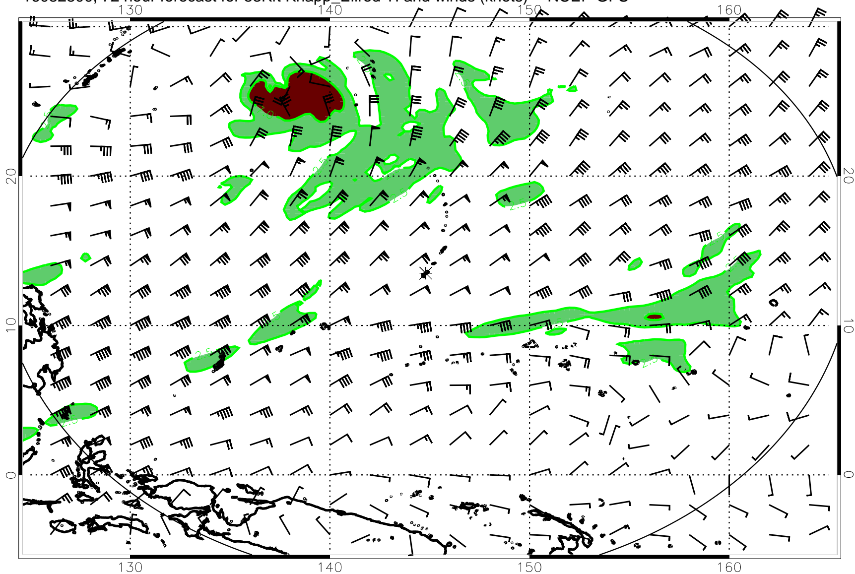
16082800, 72 hour forecast for 53Kft Knapp_Ellrod TI and winds (knots) -- NCEP GFS
