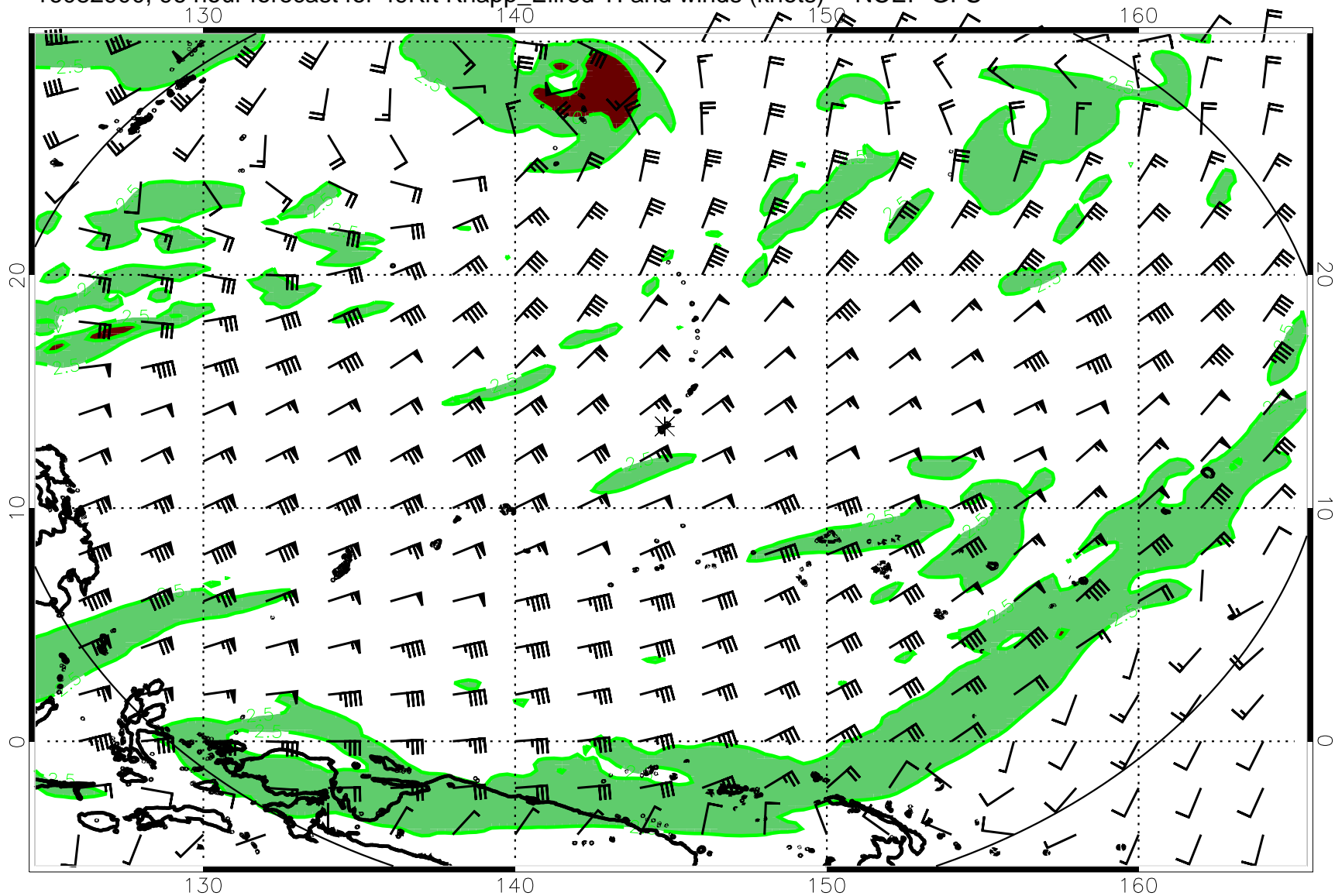
16082900, 96 hour forecast for 49Kft Knapp_Ellrod TI and winds (knots) -- NCEP GFS
