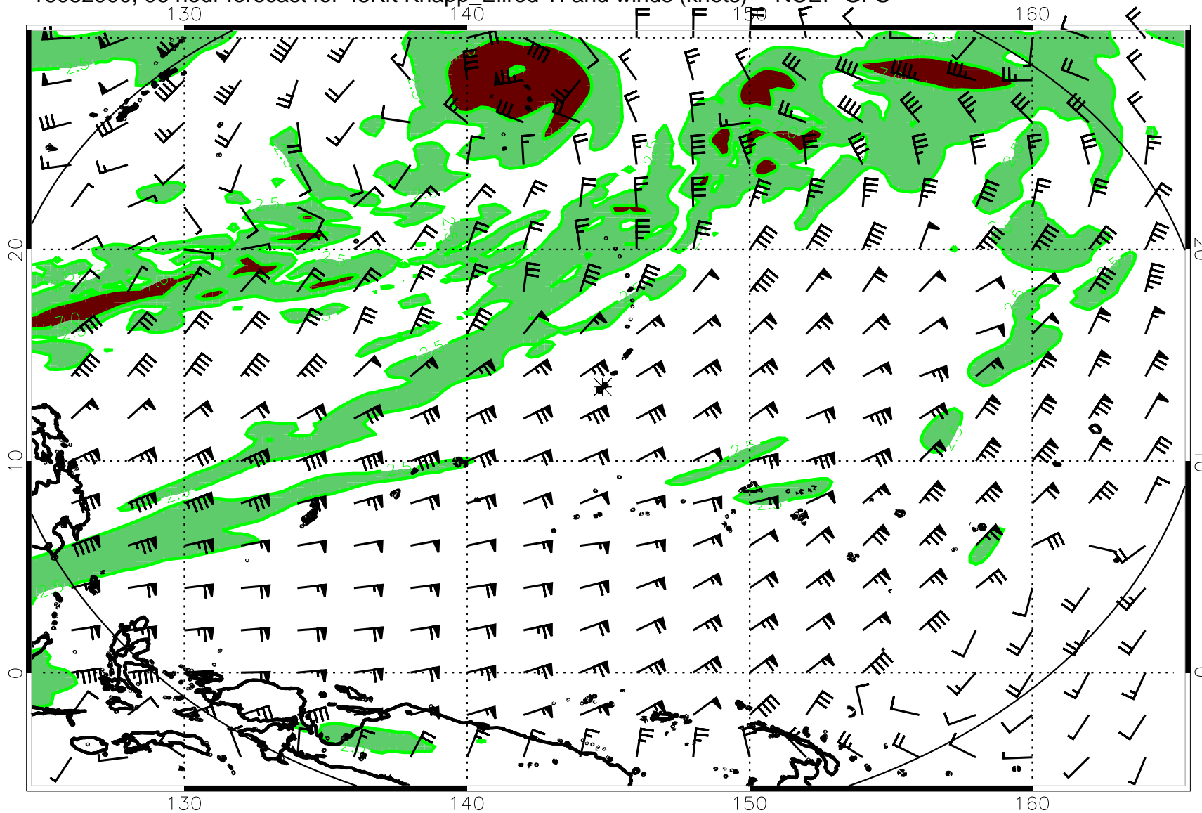
16082900, 96 hour forecast for 45Kft Knapp_Ellrod TI and winds (knots) -- NCEP GFS
