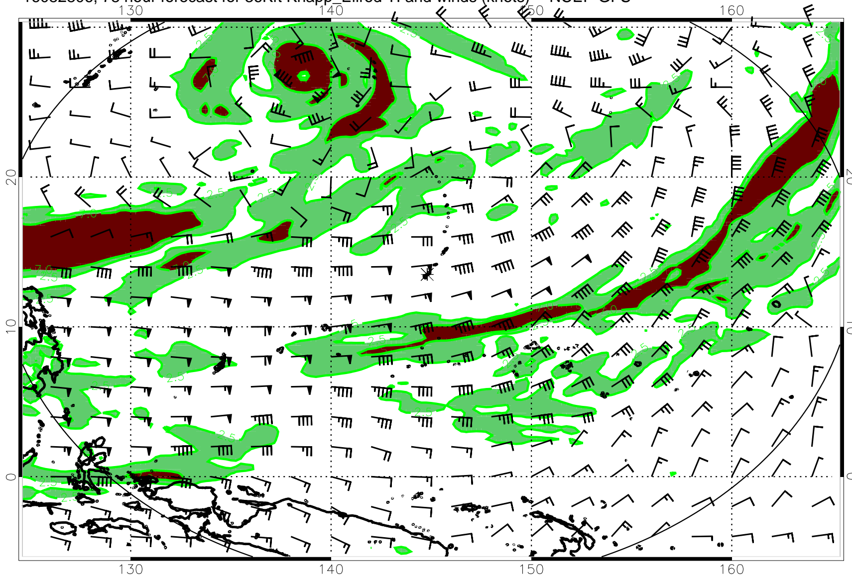
16082806, 78 hour forecast for 36Kft Knapp_Ellrod TI and winds (knots) -- NCEP GFS
