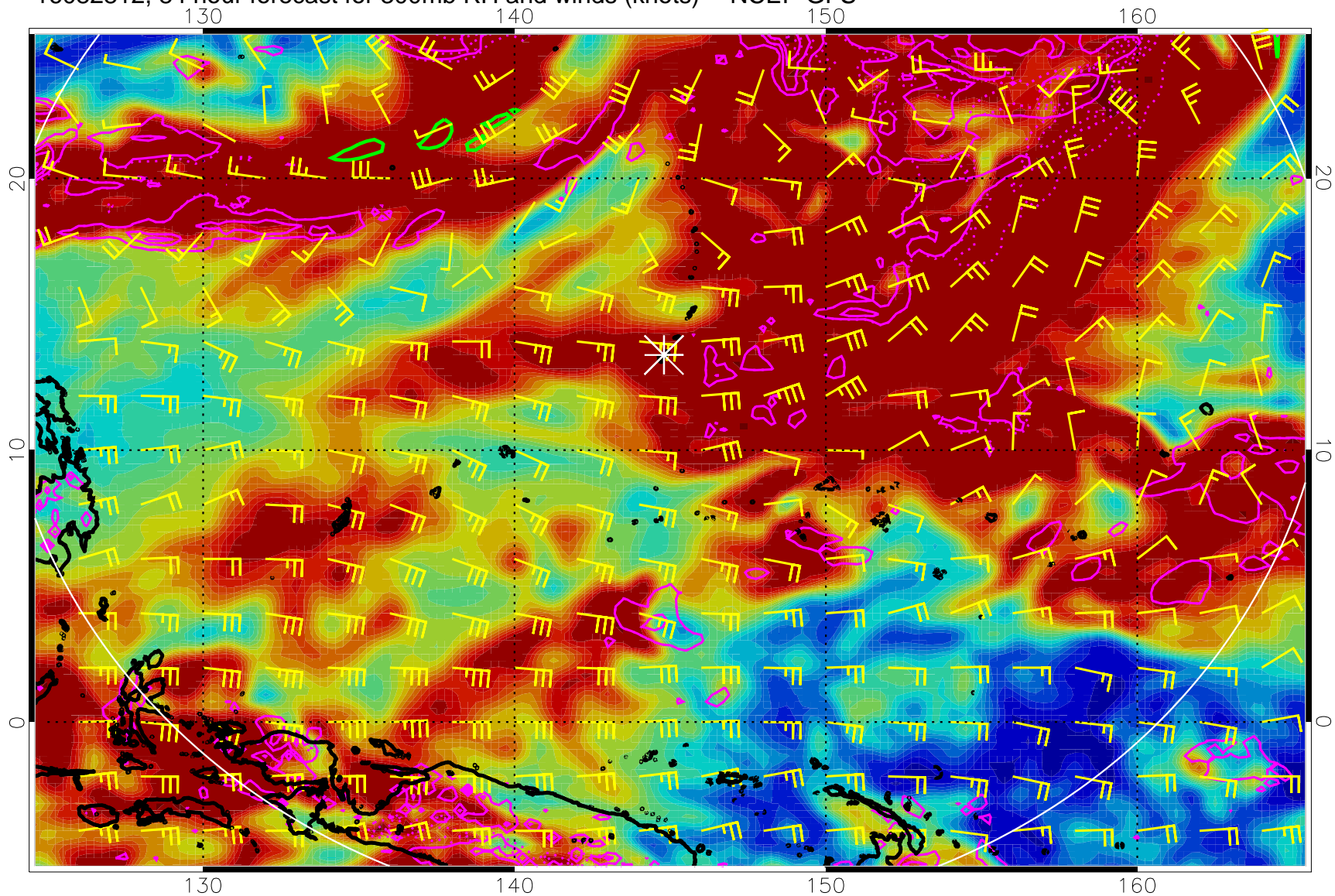
16082812, 84 hour forecast for 300mb RH and winds (knots) -- NCEP GFS
