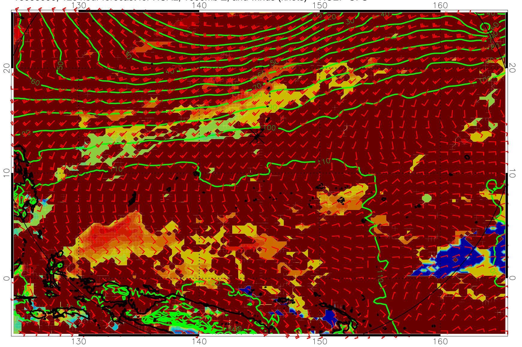
16083000, 120 hour forecast for HCAL, 1000mb Z, and winds (knots) -- NCEP GFS
