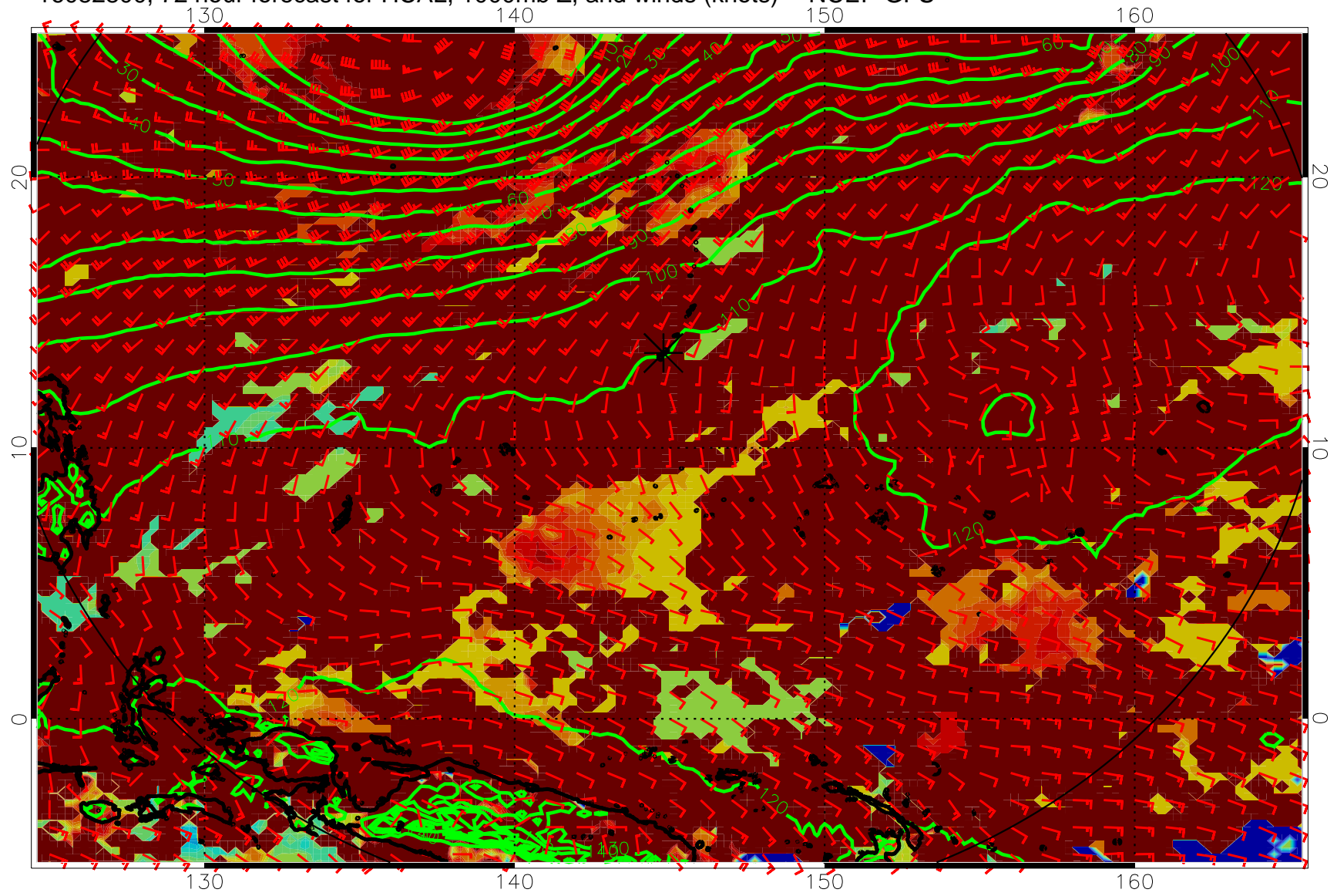
16082800, 72 hour forecast for HCAL, 1000mb Z, and winds (knots) -- NCEP GFS
