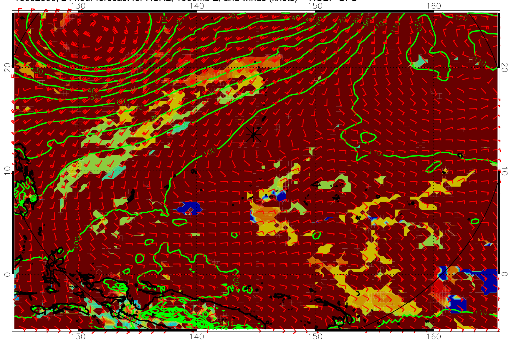
16082600, 24 hour forecast for HCAL, 1000mb Z, and winds (knots) -- NCEP GFS
