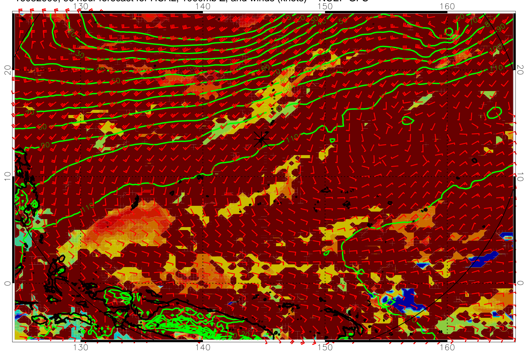
16082900, 96 hour forecast for HCAL, 1000mb Z, and winds (knots) -- NCEP GFS
