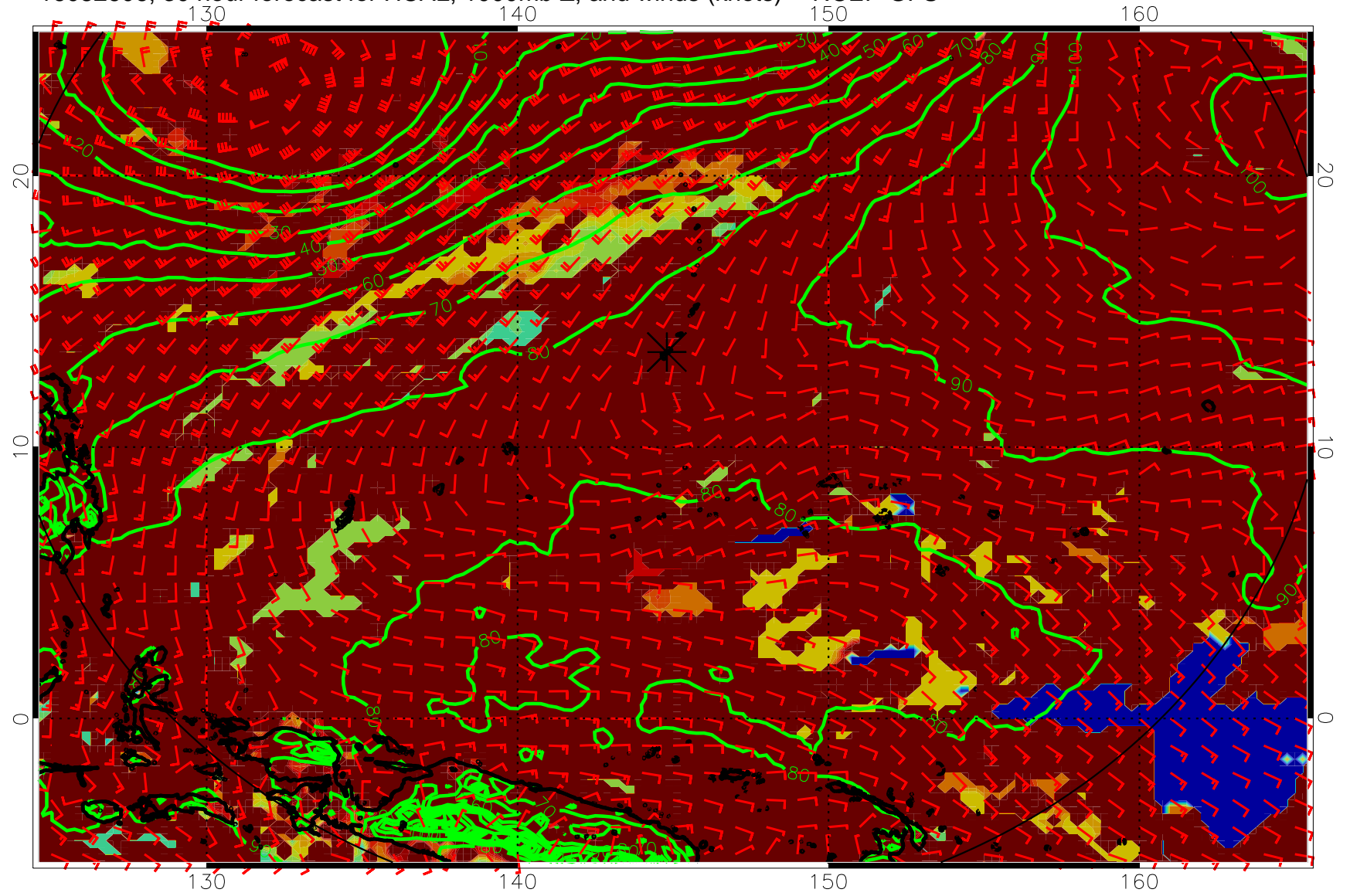
16082606, 30 hour forecast for HCAL, 1000mb Z, and winds (knots) -- NCEP GFS
