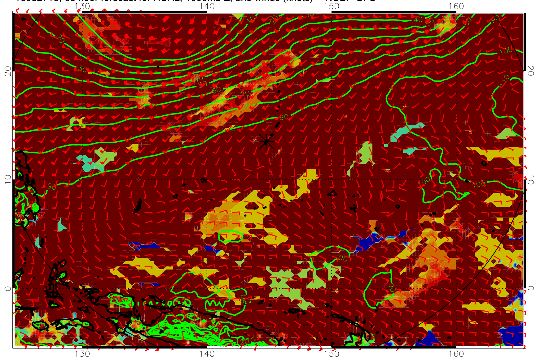
16082718, 66 hour forecast for HCAL, 1000mb Z, and winds (knots) -- NCEP GFS
