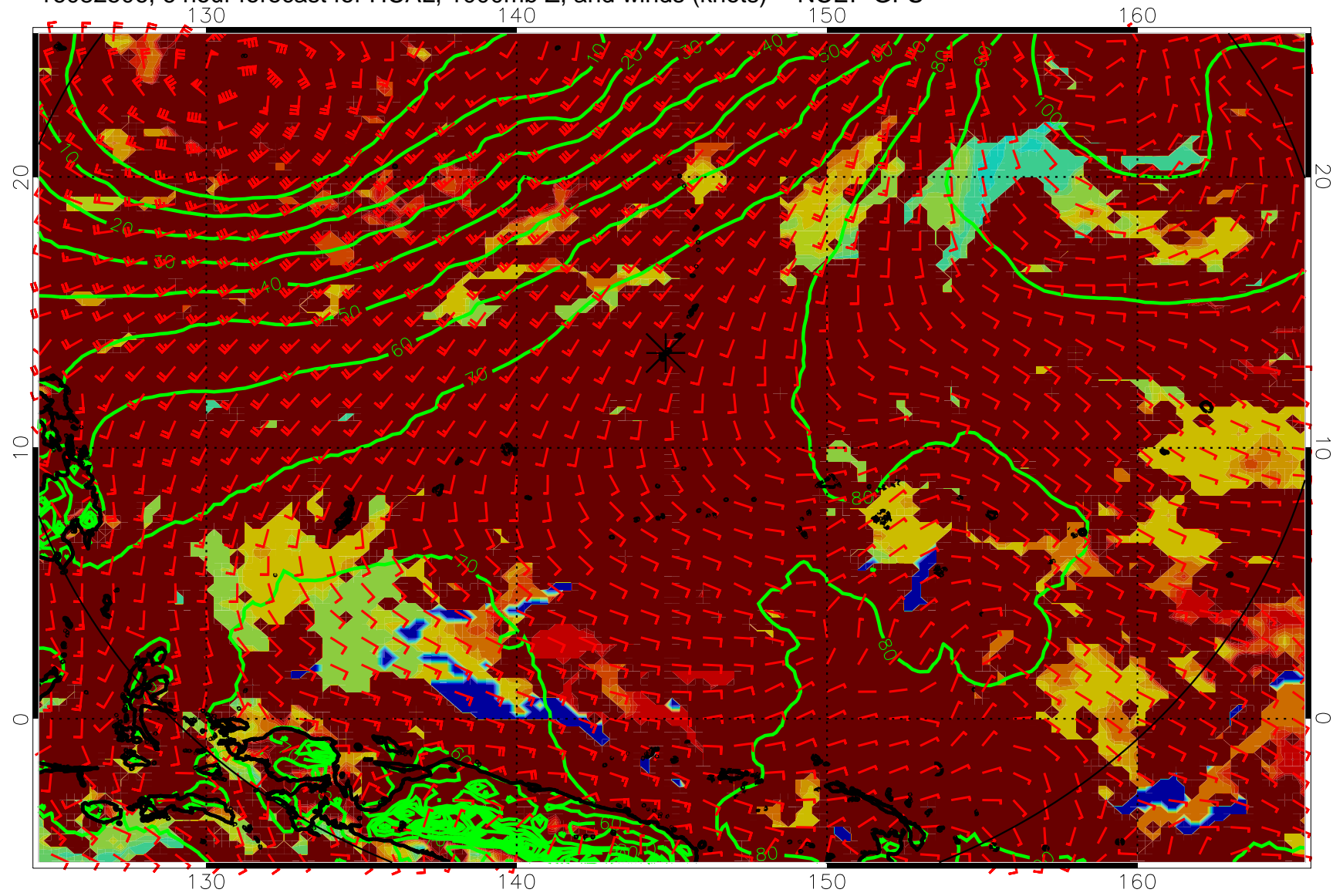
16082506, 6 hour forecast for HCAL, 1000mb Z, and winds (knots) -- NCEP GFS
