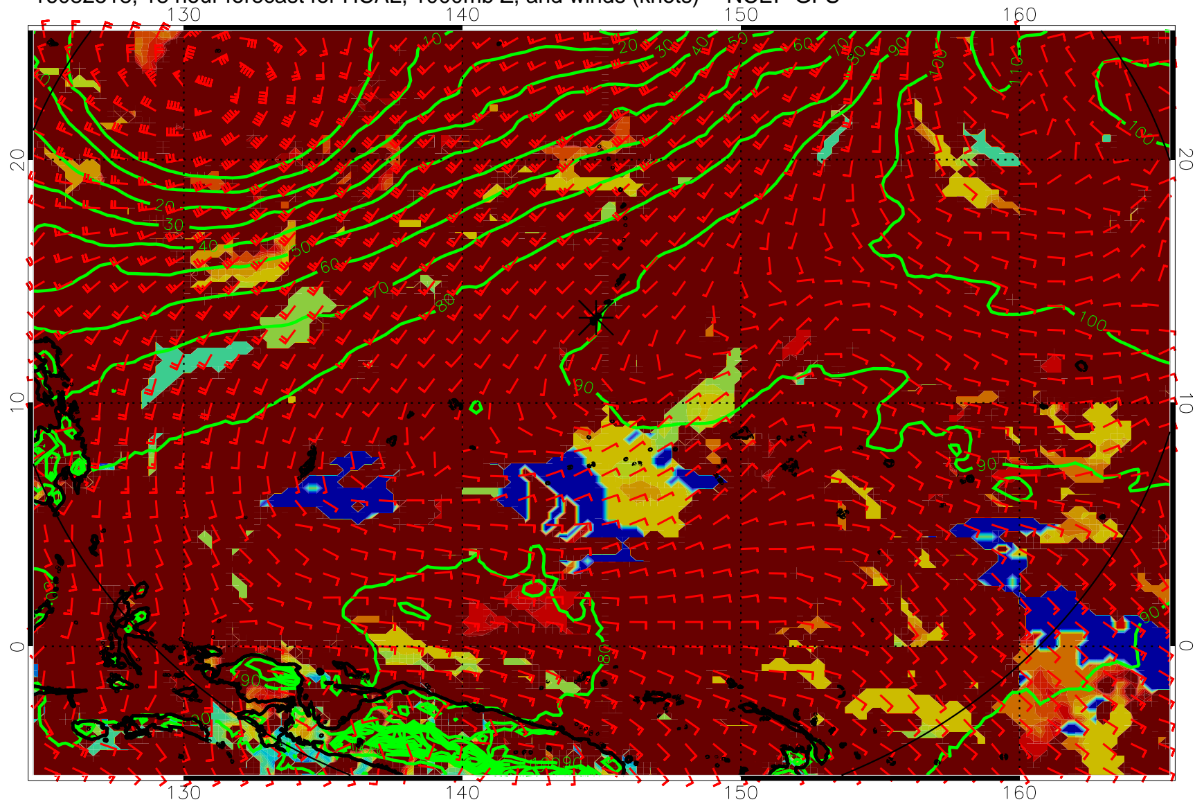
16082518, 18 hour forecast for HCAL, 1000mb Z, and winds (knots) -- NCEP GFS
