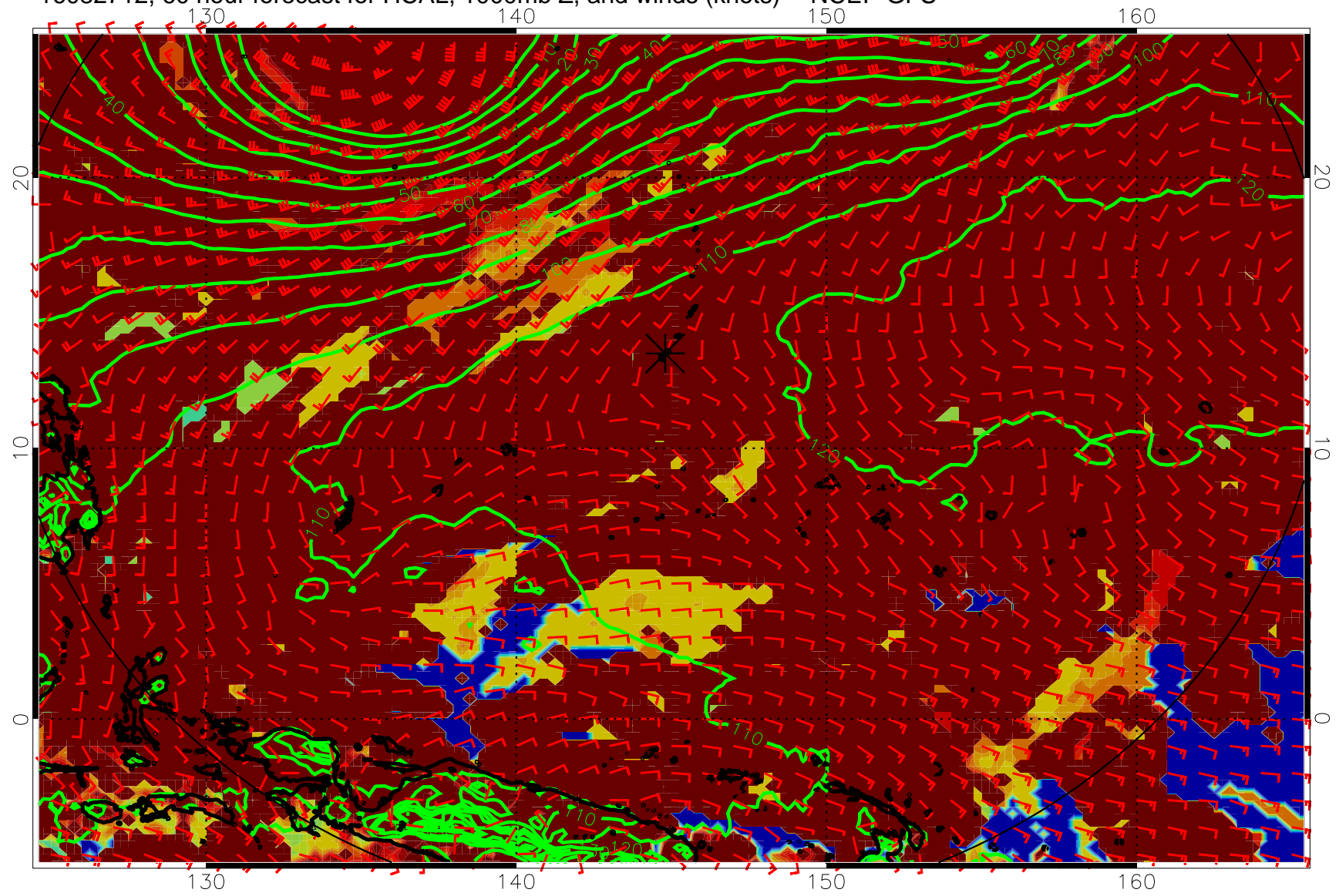
16082712, 60 hour forecast for HCAL, 1000mb Z, and winds (knots) -- NCEP GFS
