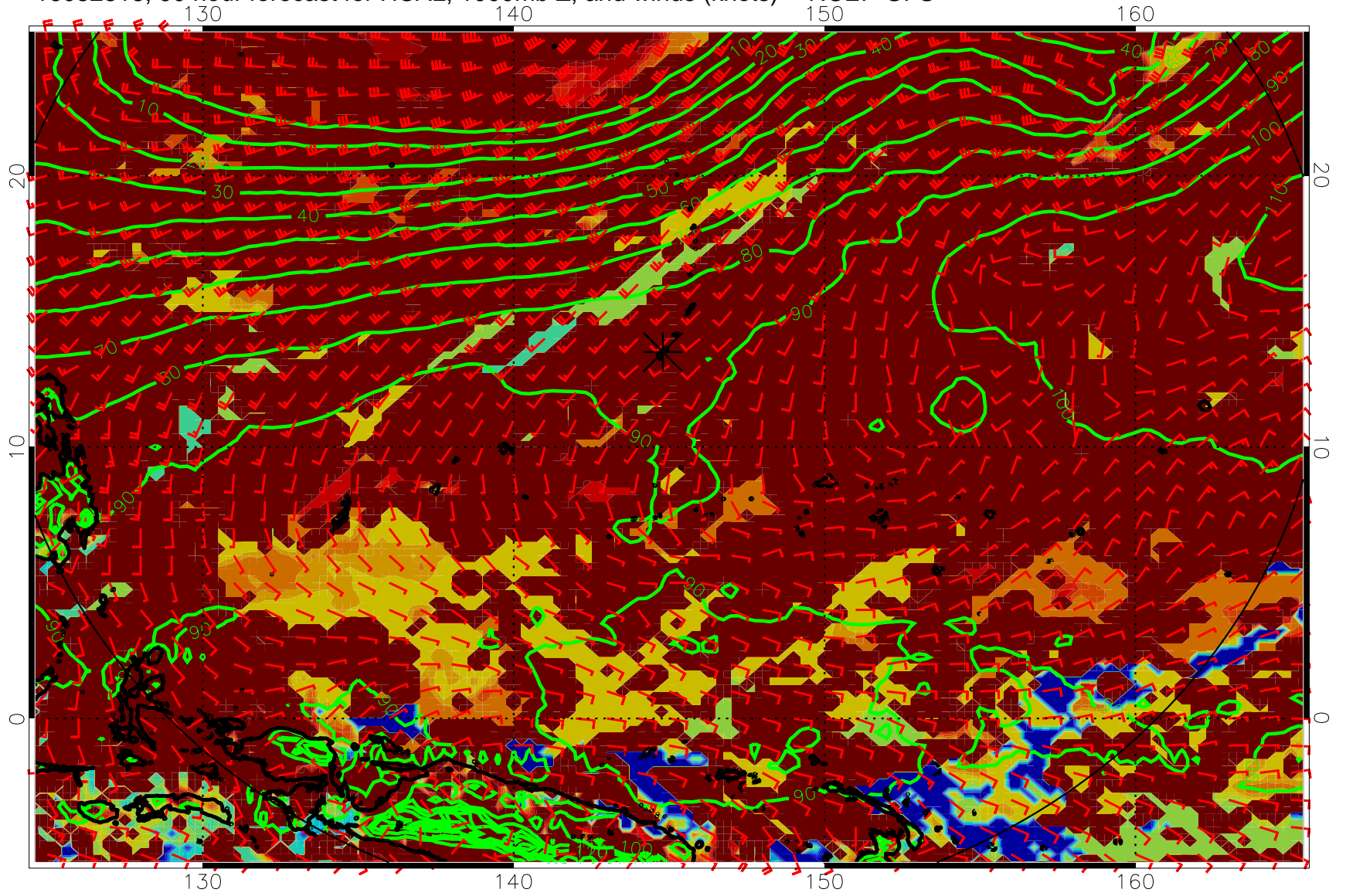
16082818, 90 hour forecast for HCAL, 1000mb Z, and winds (knots) -- NCEP GFS
