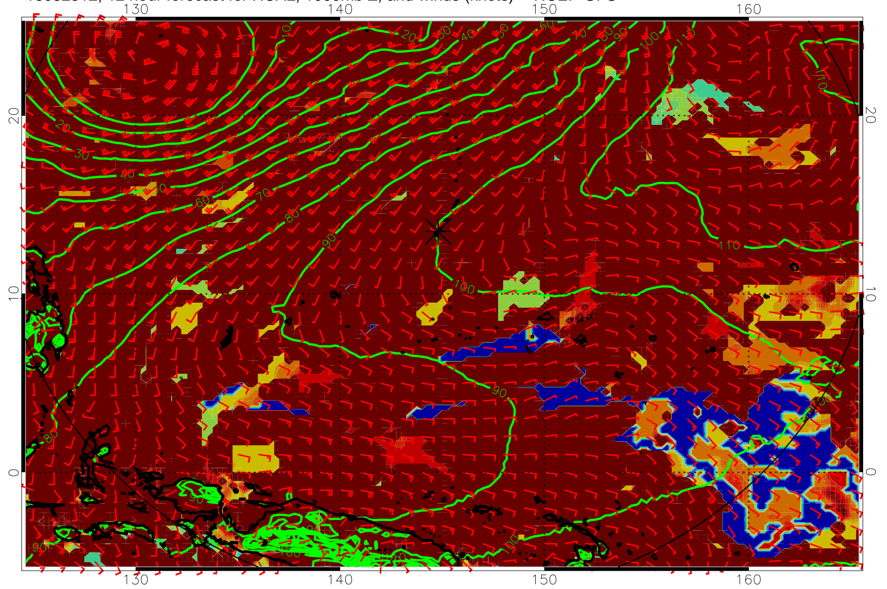
16082512, 12 hour forecast for HCAL, 1000mb Z, and winds (knots) -- NCEP GFS
