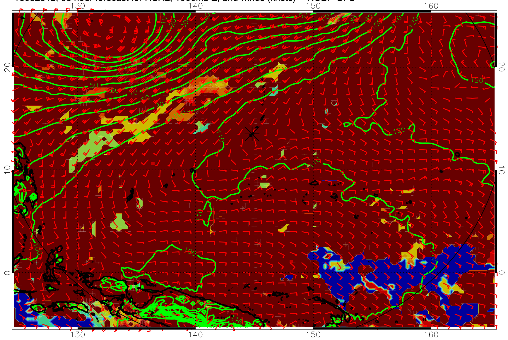
16082612, 36 hour forecast for HCAL, 1000mb Z, and winds (knots) -- NCEP GFS
