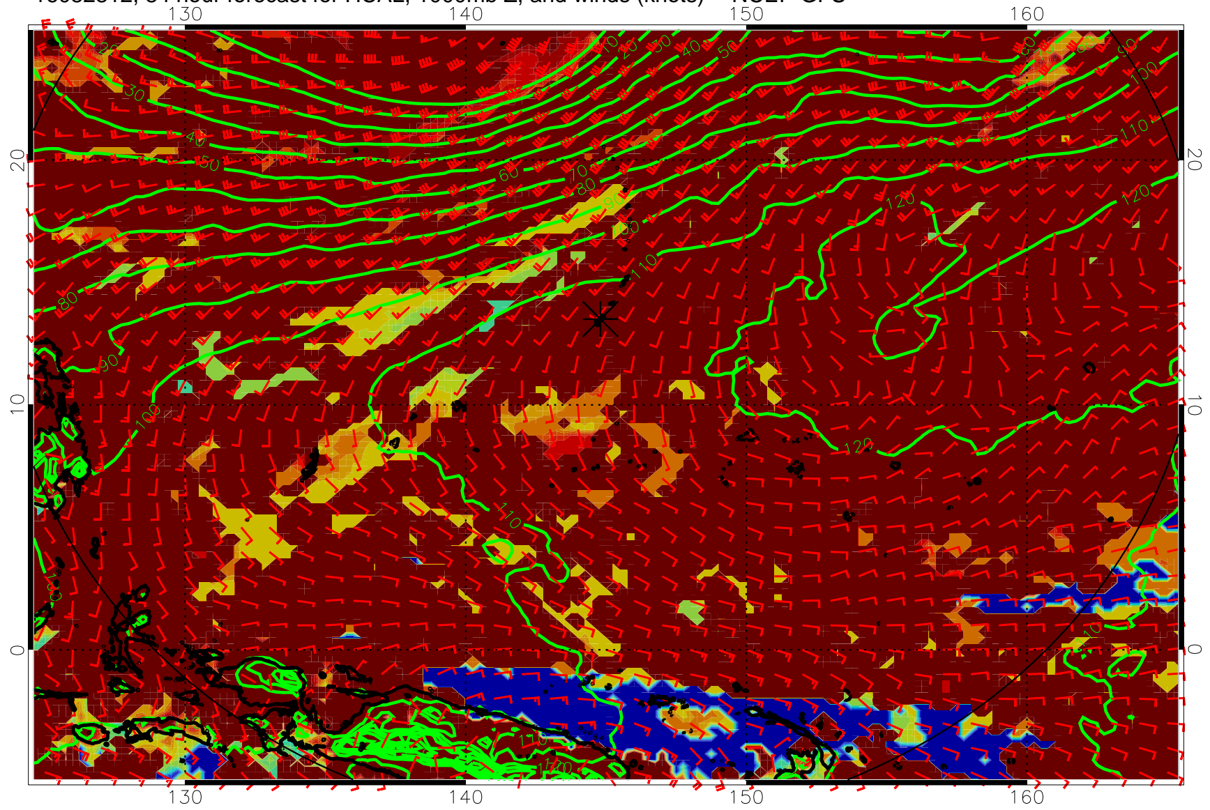
16082812, 84 hour forecast for HCAL, 1000mb Z, and winds (knots) -- NCEP GFS
