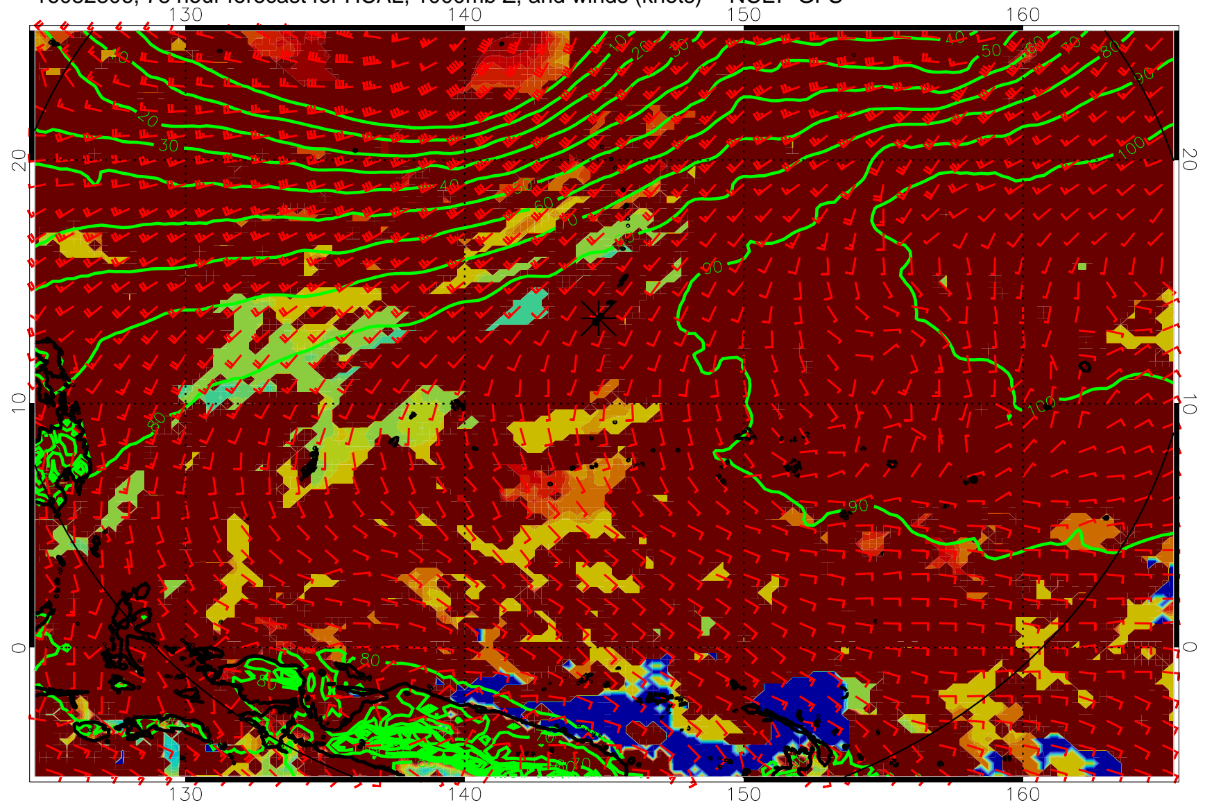
16082806, 78 hour forecast for HCAL, 1000mb Z, and winds (knots) -- NCEP GFS
