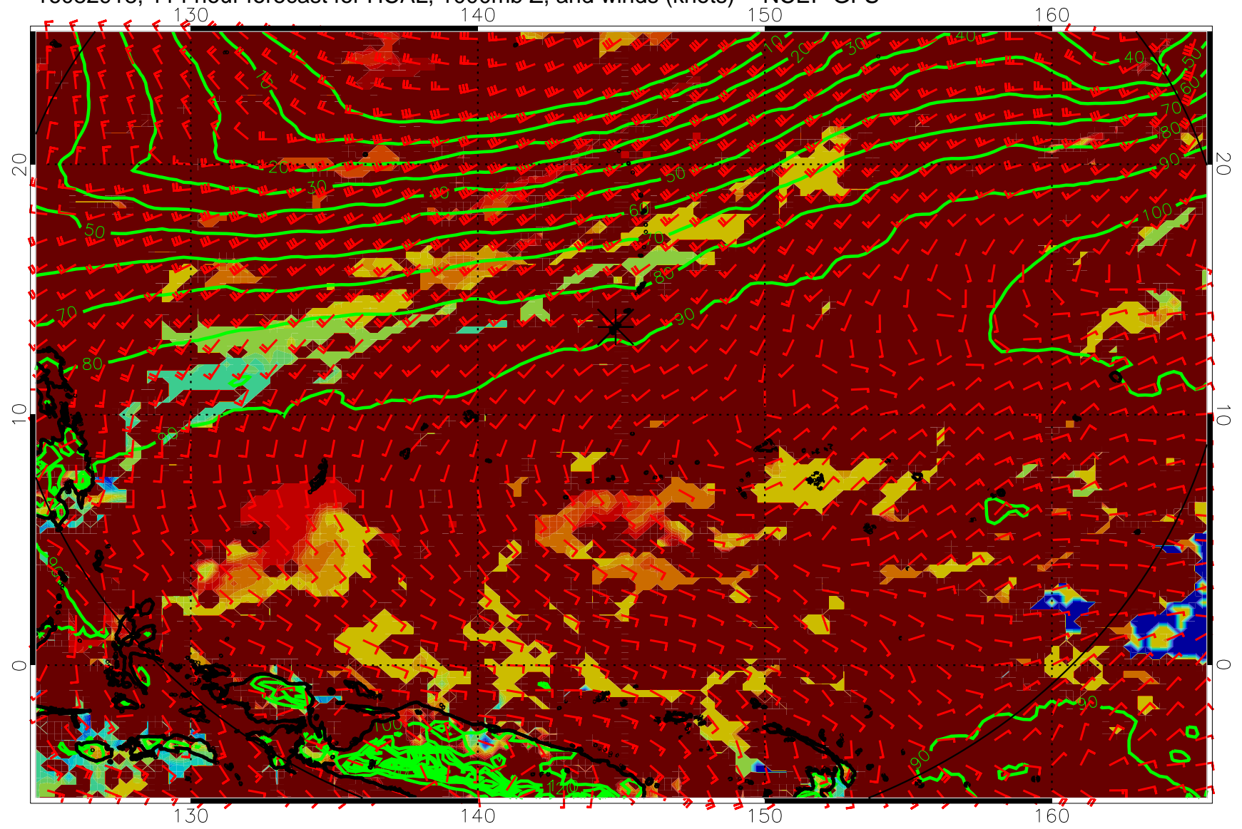
16082918, 114 hour forecast for HCAL, 1000mb Z, and winds (knots) -- NCEP GFS
