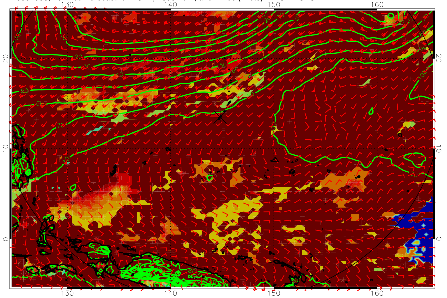
16082906, 102 hour forecast for HCAL, 1000mb Z, and winds (knots) -- NCEP GFS
