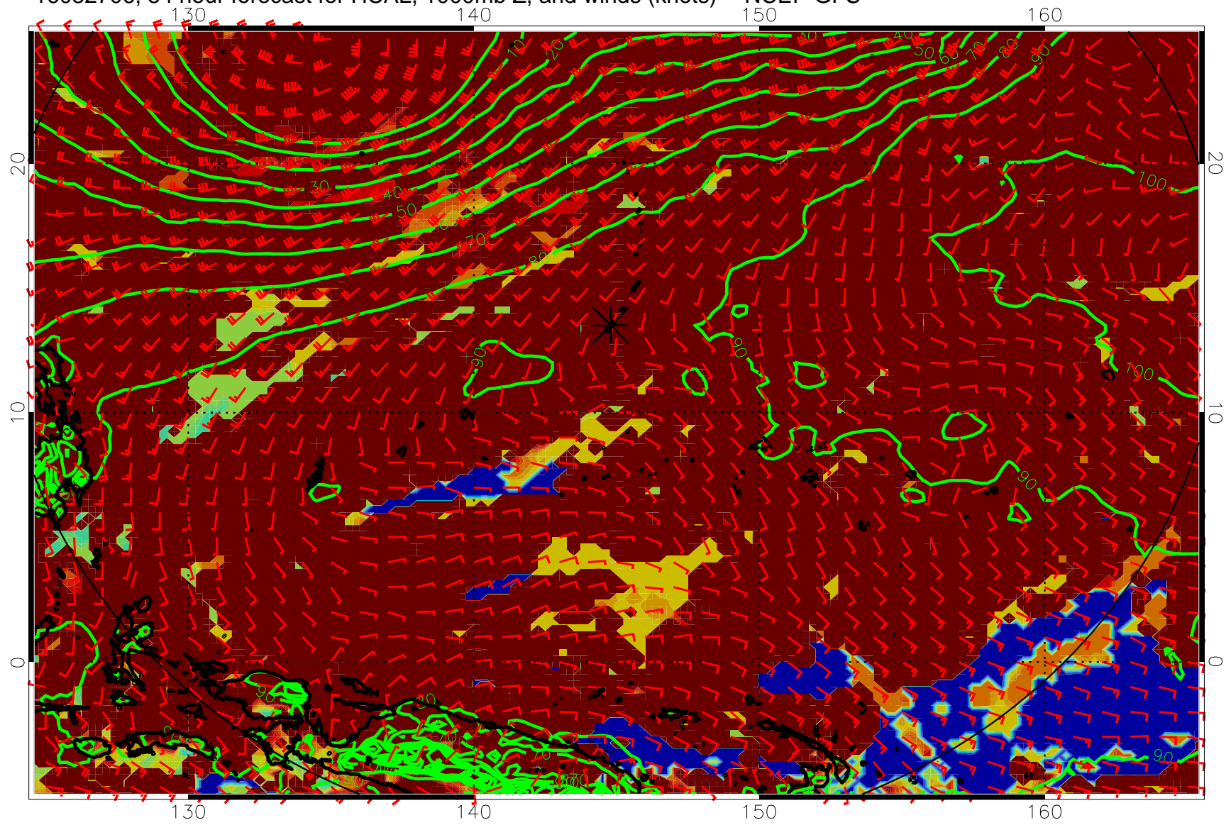
16082706, 54 hour forecast for HCAL, 1000mb Z, and winds (knots) -- NCEP GFS
