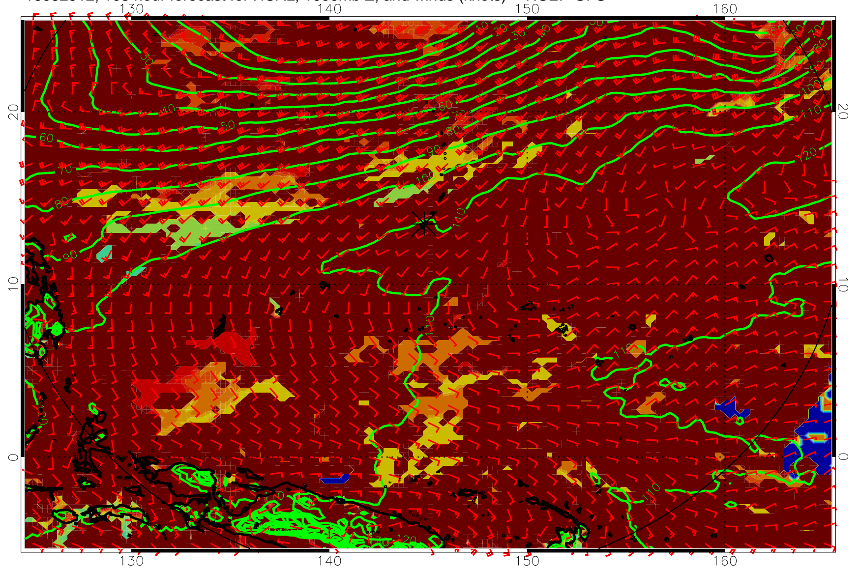
16082912, 108 hour forecast for HCAL, 1000mb Z, and winds (knots) -- NCEP GFS
