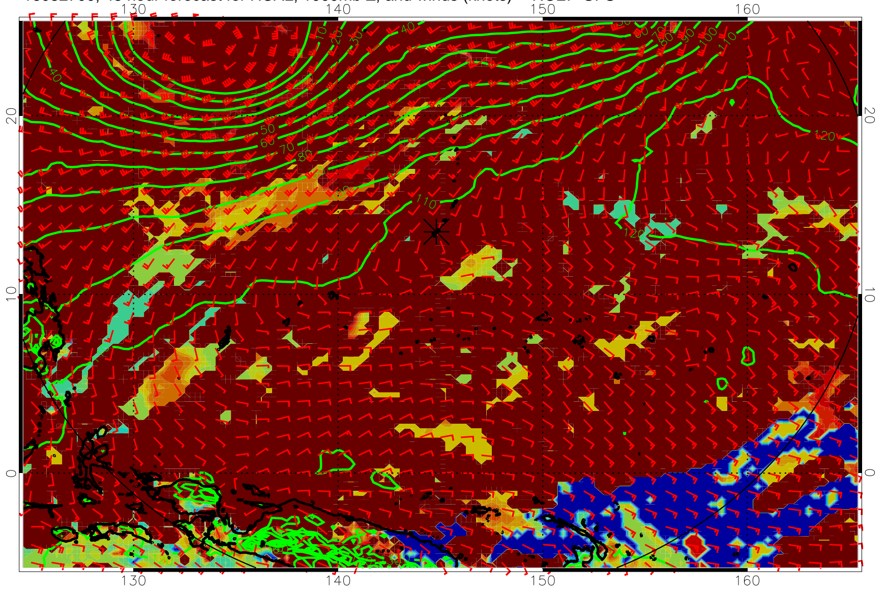
16082700, 48 hour forecast for HCAL, 1000mb Z, and winds (knots) -- NCEP GFS
