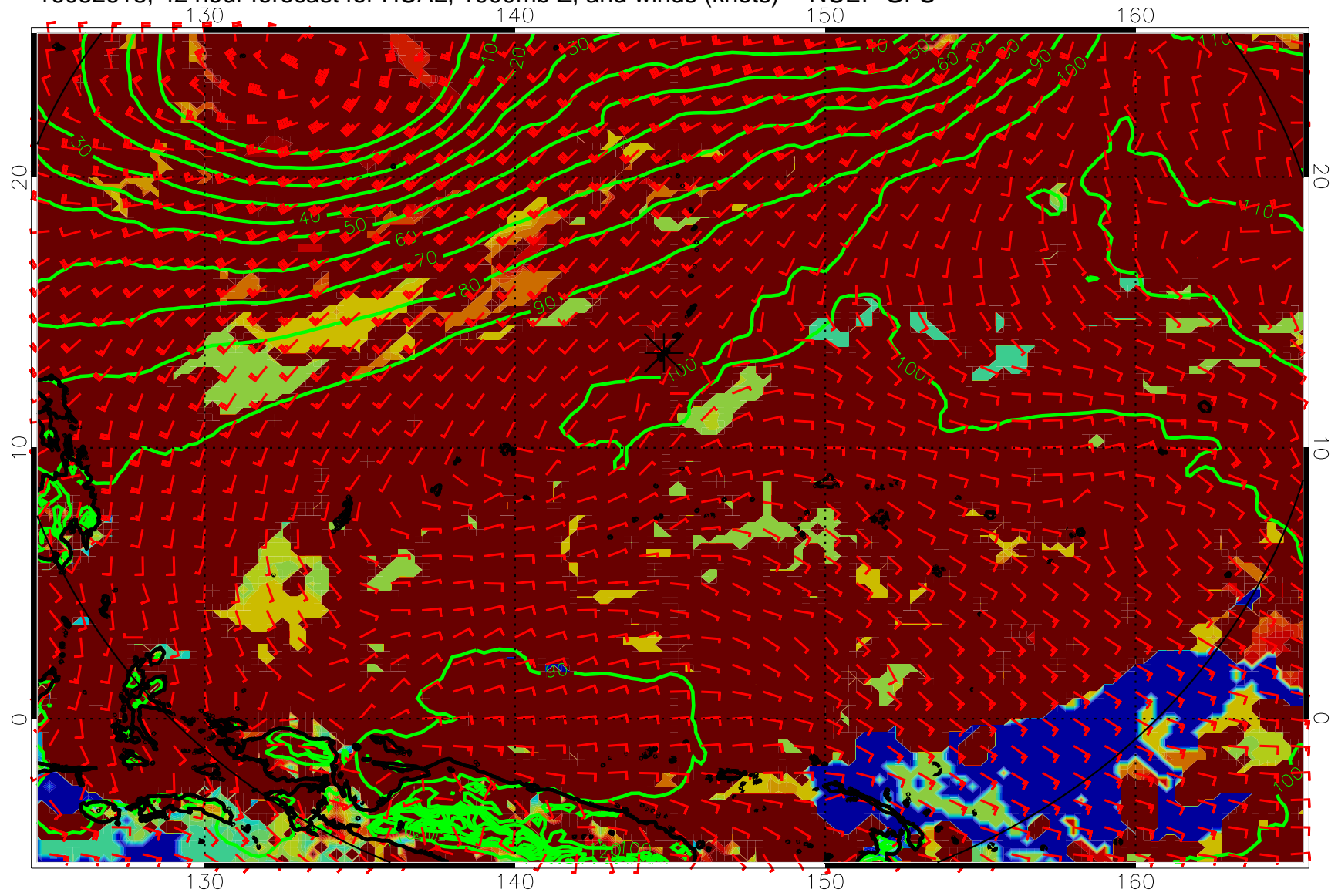
16082618, 42 hour forecast for HCAL, 1000mb Z, and winds (knots) -- NCEP GFS
