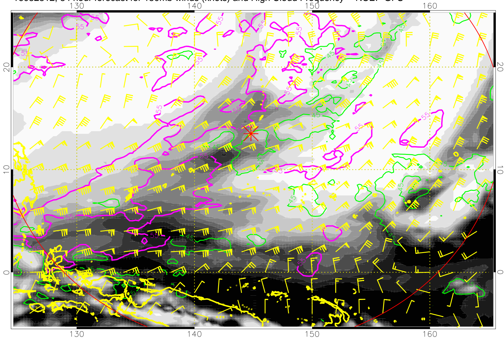
16082812, 84 hour forecast for 150mb winds (knots) and High Cloud Frequency -- NCEP GFS
