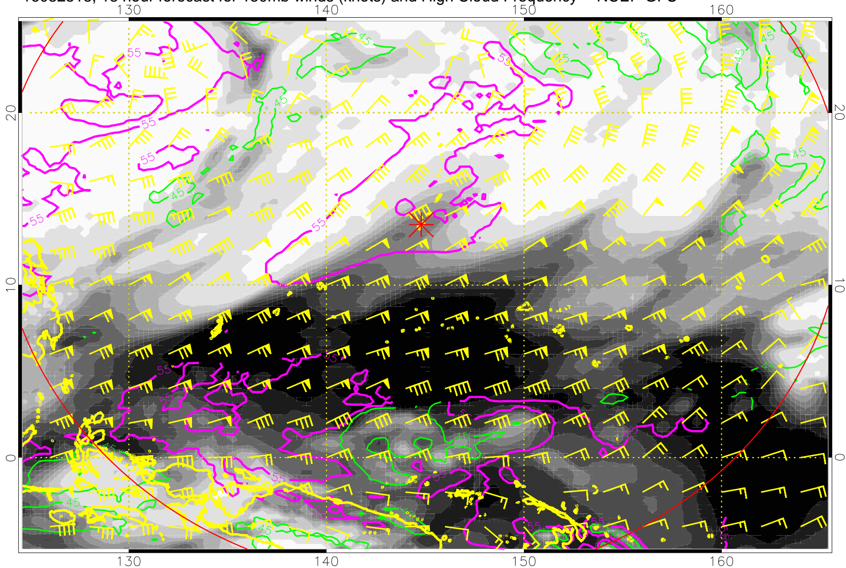
16082518, 18 hour forecast for 150mb winds (knots) and High Cloud Frequency -- NCEP GFS
