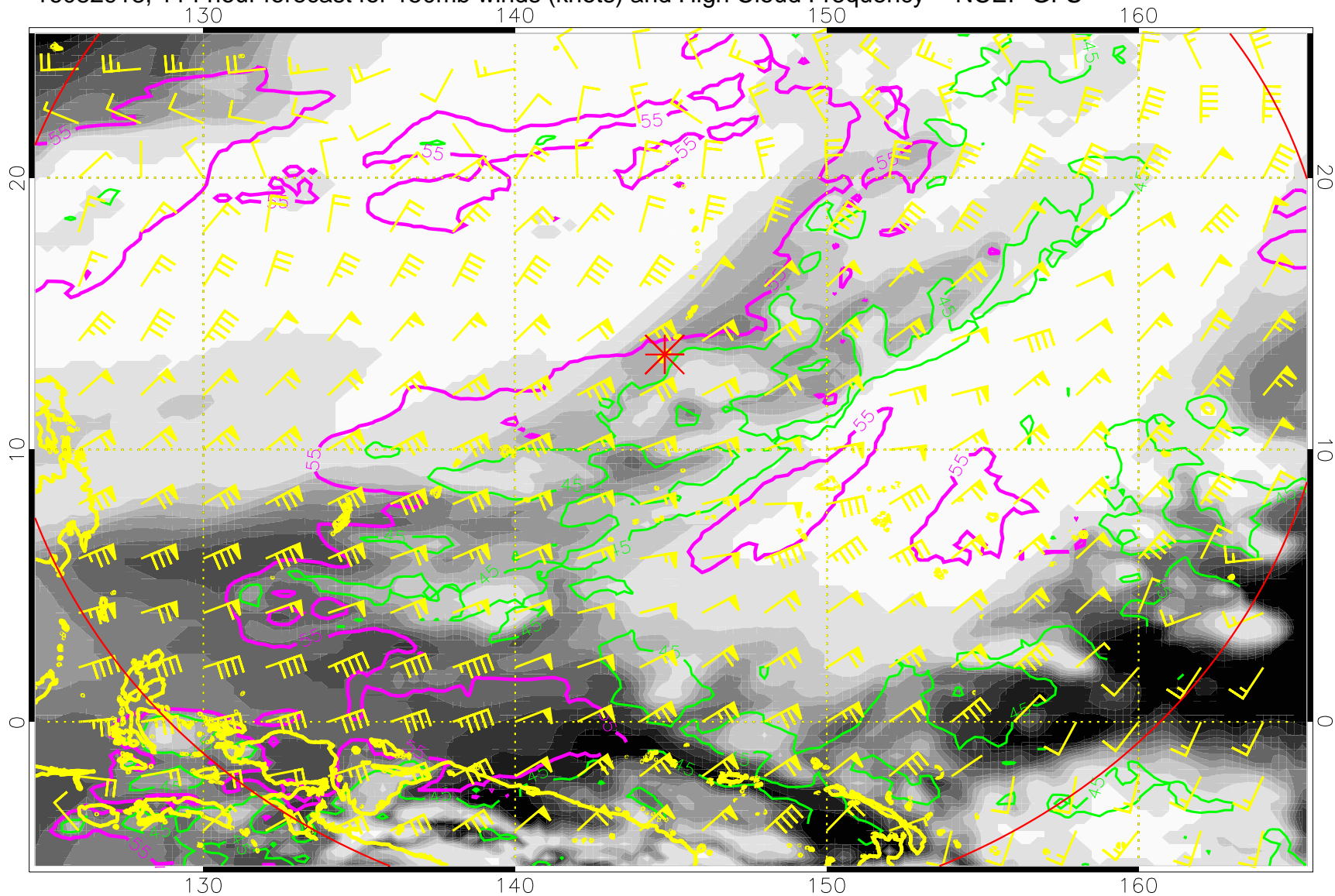
16082918, 114 hour forecast for 150mb winds (knots) and High Cloud Frequency -- NCEP GFS
