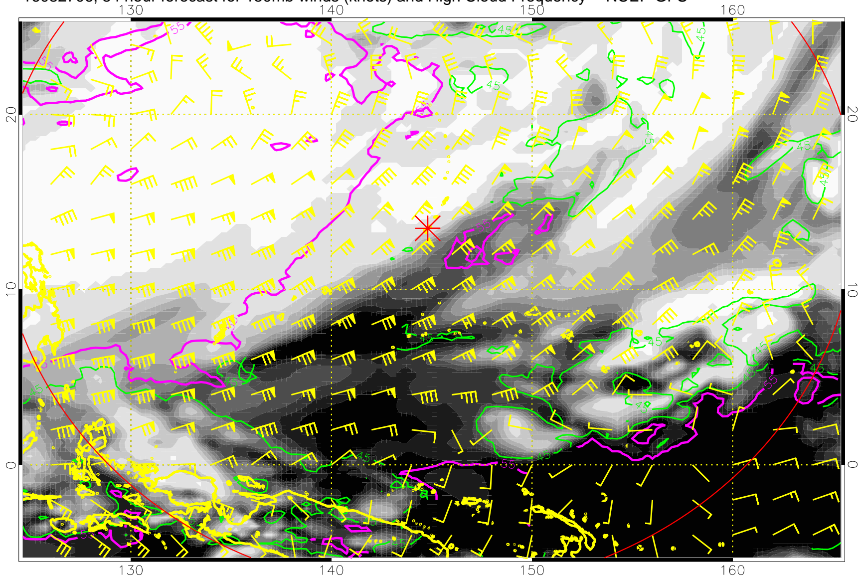
16082706, 54 hour forecast for 150mb winds (knots) and High Cloud Frequency -- NCEP GFS
