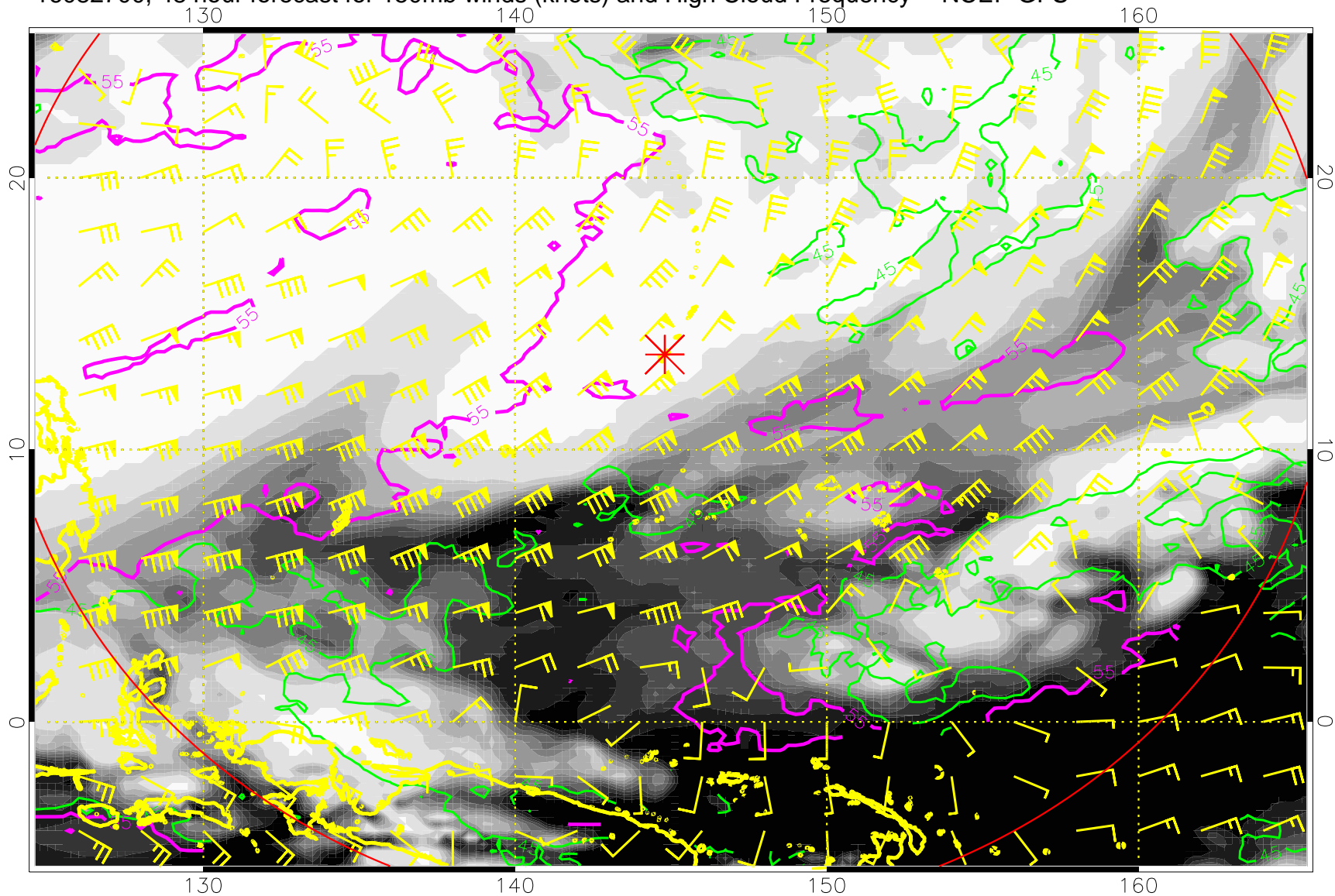
16082700, 48 hour forecast for 150mb winds (knots) and High Cloud Frequency -- NCEP GFS
