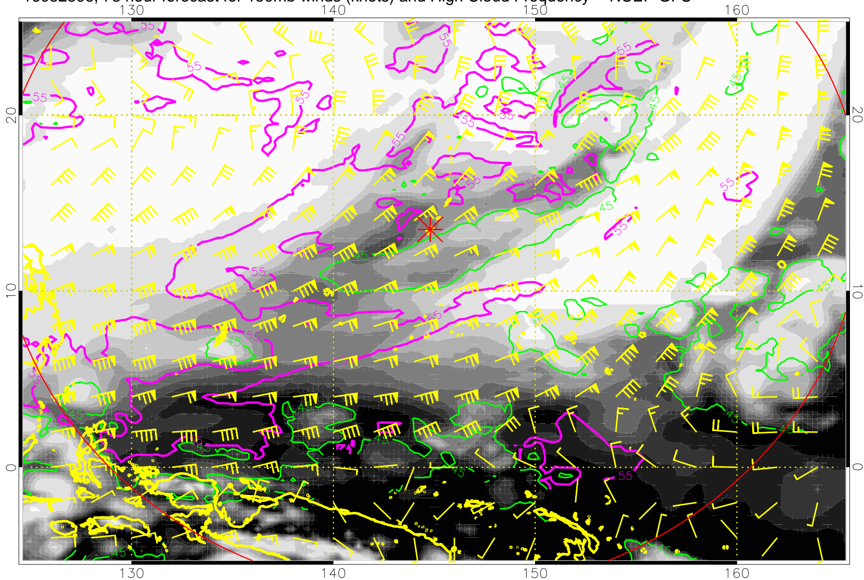
16082806, 78 hour forecast for 150mb winds (knots) and High Cloud Frequency -- NCEP GFS
