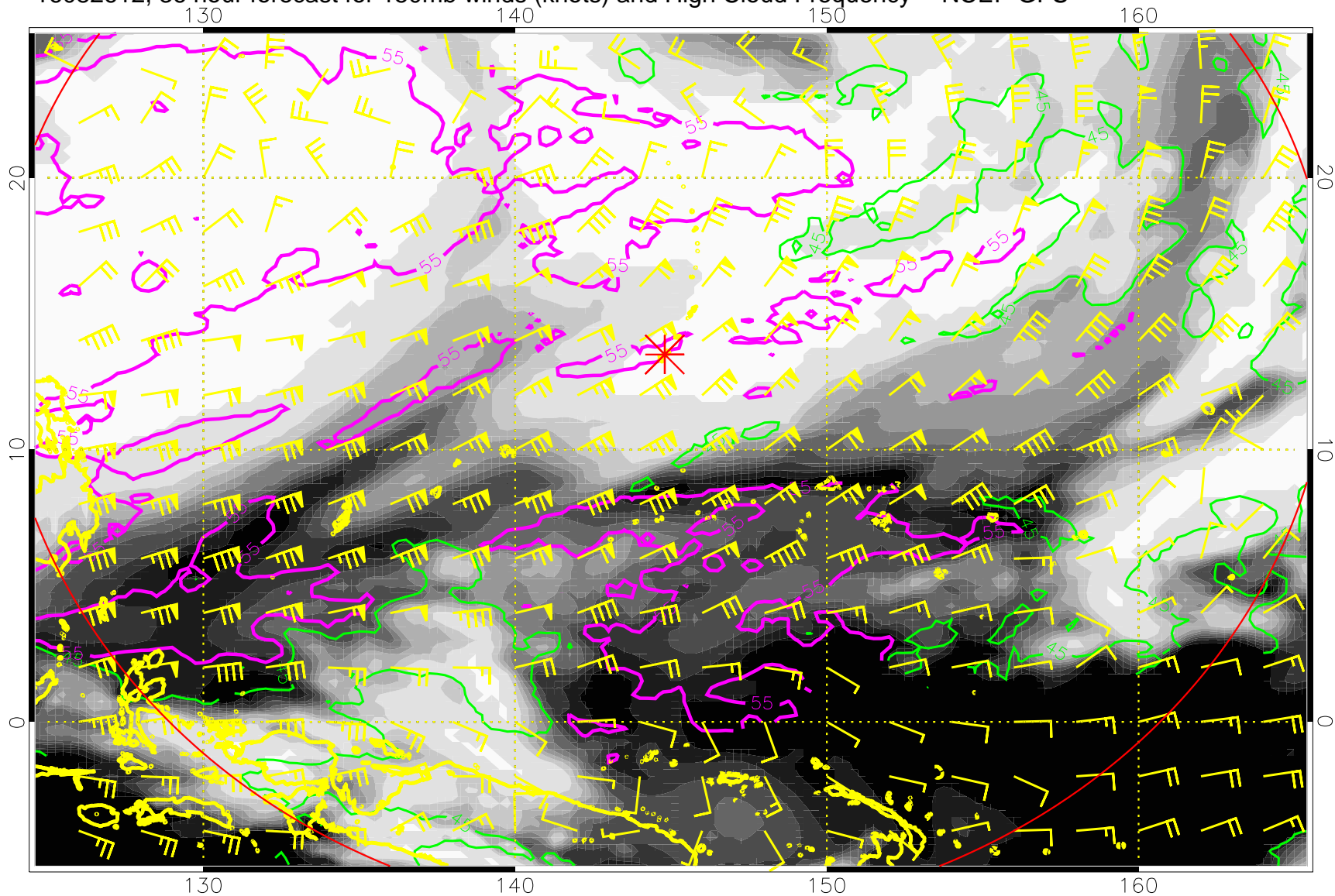
16082612, 36 hour forecast for 150mb winds (knots) and High Cloud Frequency -- NCEP GFS
