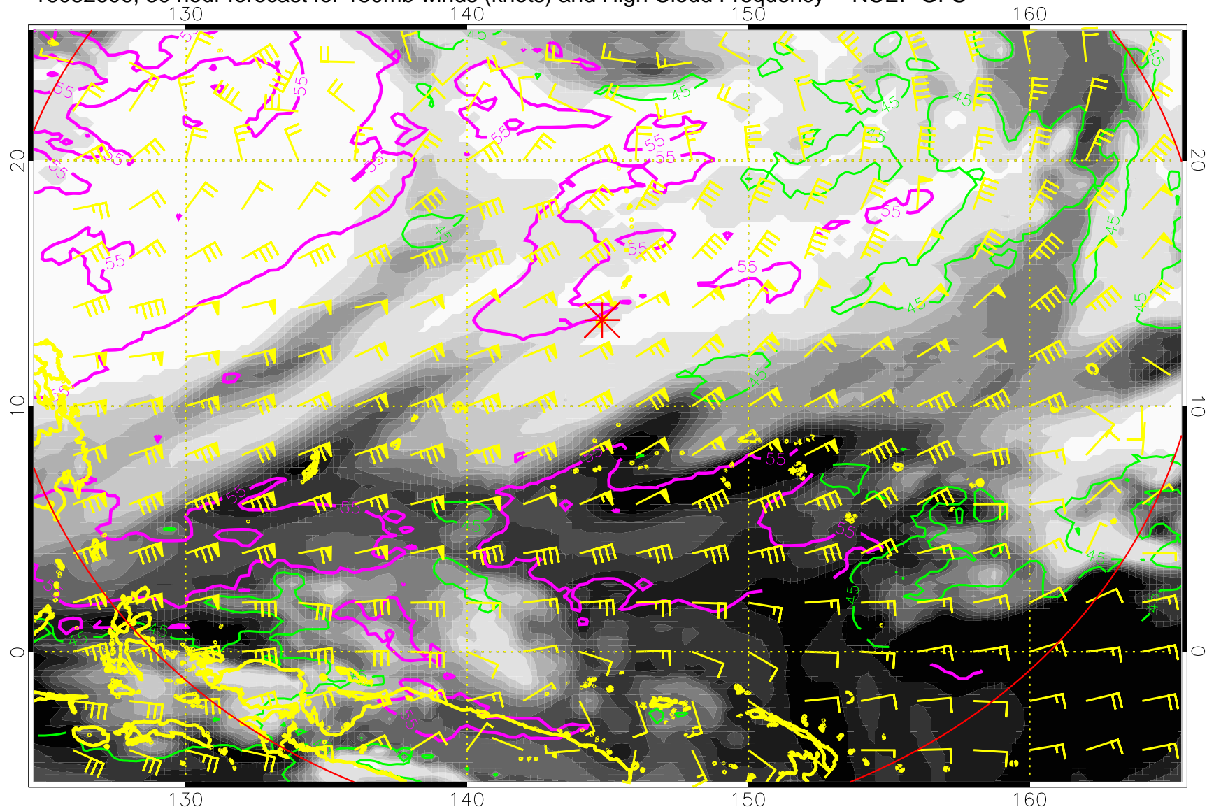
16082606, 30 hour forecast for 150mb winds (knots) and High Cloud Frequency -- NCEP GFS
