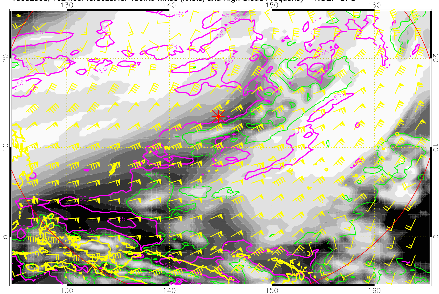
16082906, 102 hour forecast for 150mb winds (knots) and High Cloud Frequency -- NCEP GFS
