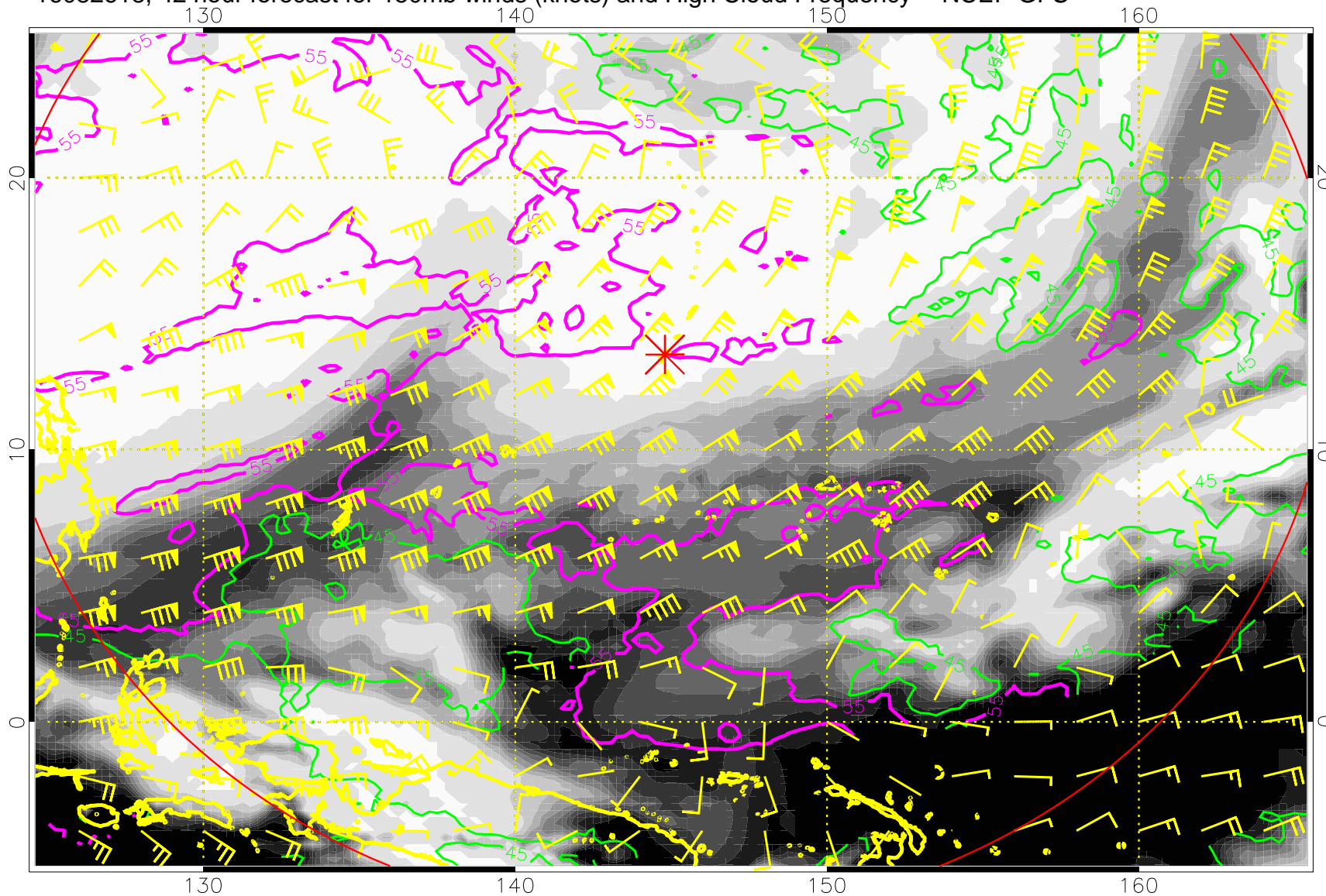
16082618, 42 hour forecast for 150mb winds (knots) and High Cloud Frequency -- NCEP GFS
