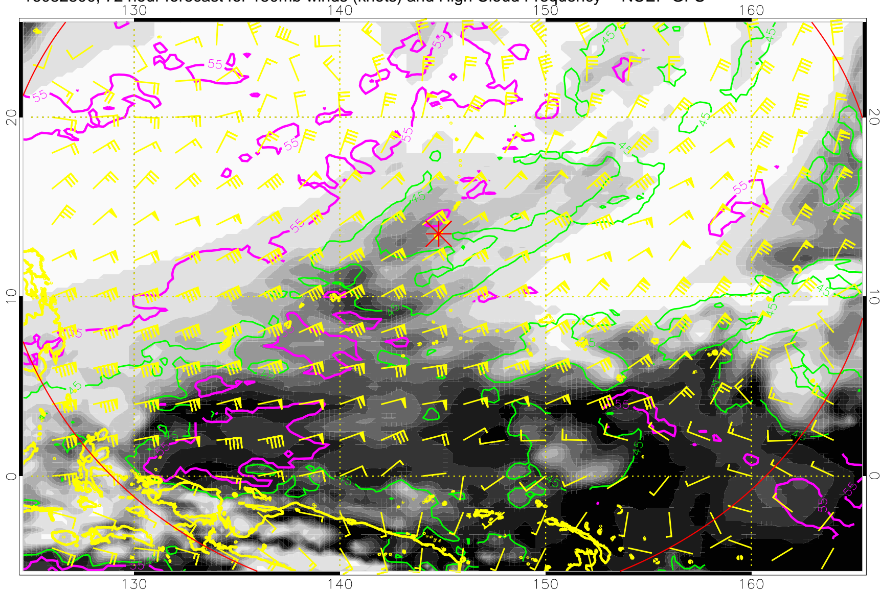
16082800, 72 hour forecast for 150mb winds (knots) and High Cloud Frequency -- NCEP GFS
