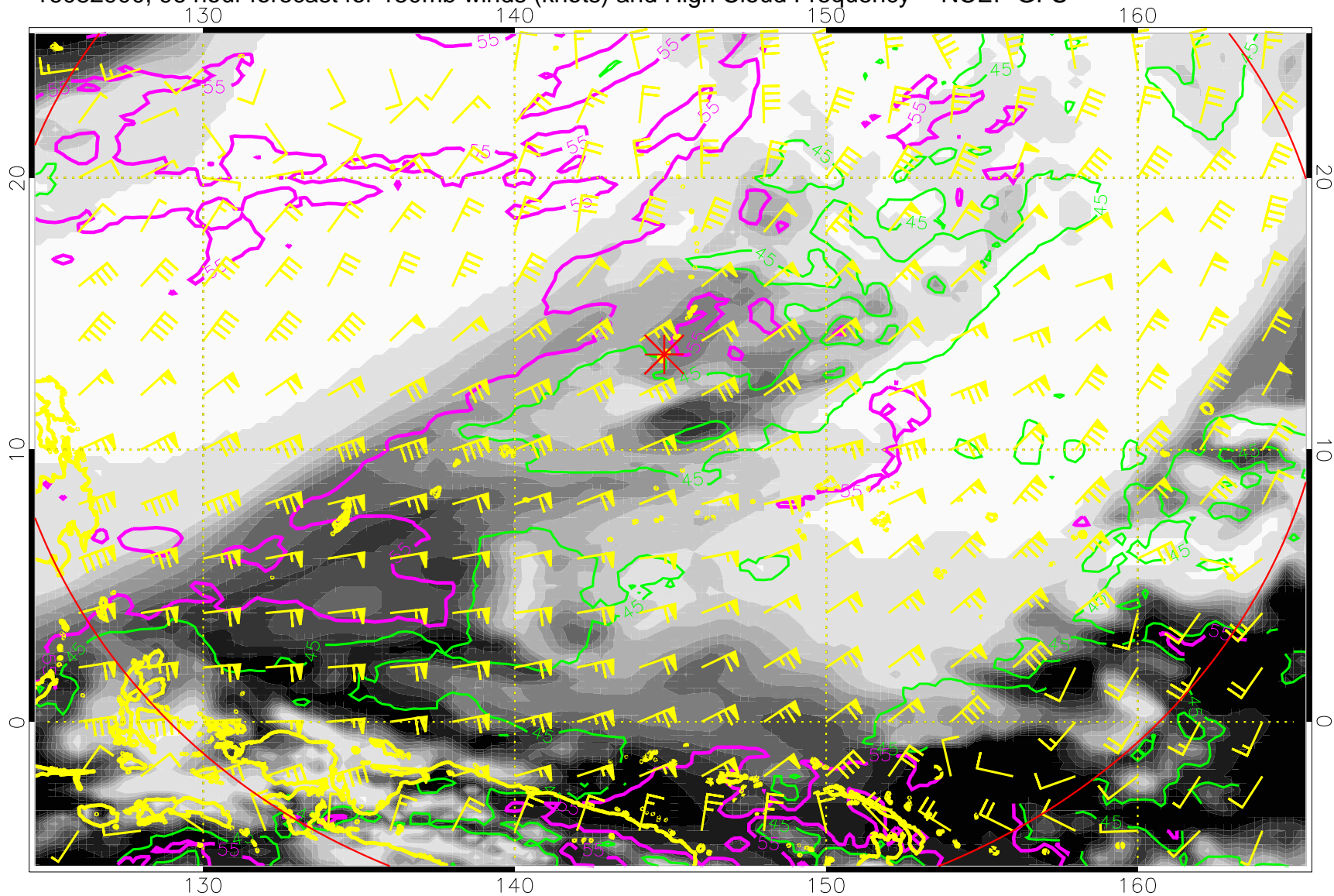
16082900, 96 hour forecast for 150mb winds (knots) and High Cloud Frequency -- NCEP GFS
