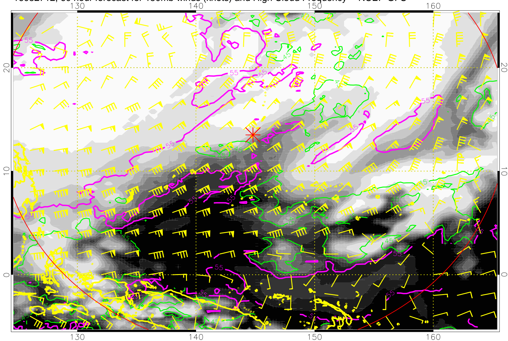
16082712, 60 hour forecast for 150mb winds (knots) and High Cloud Frequency -- NCEP GFS
