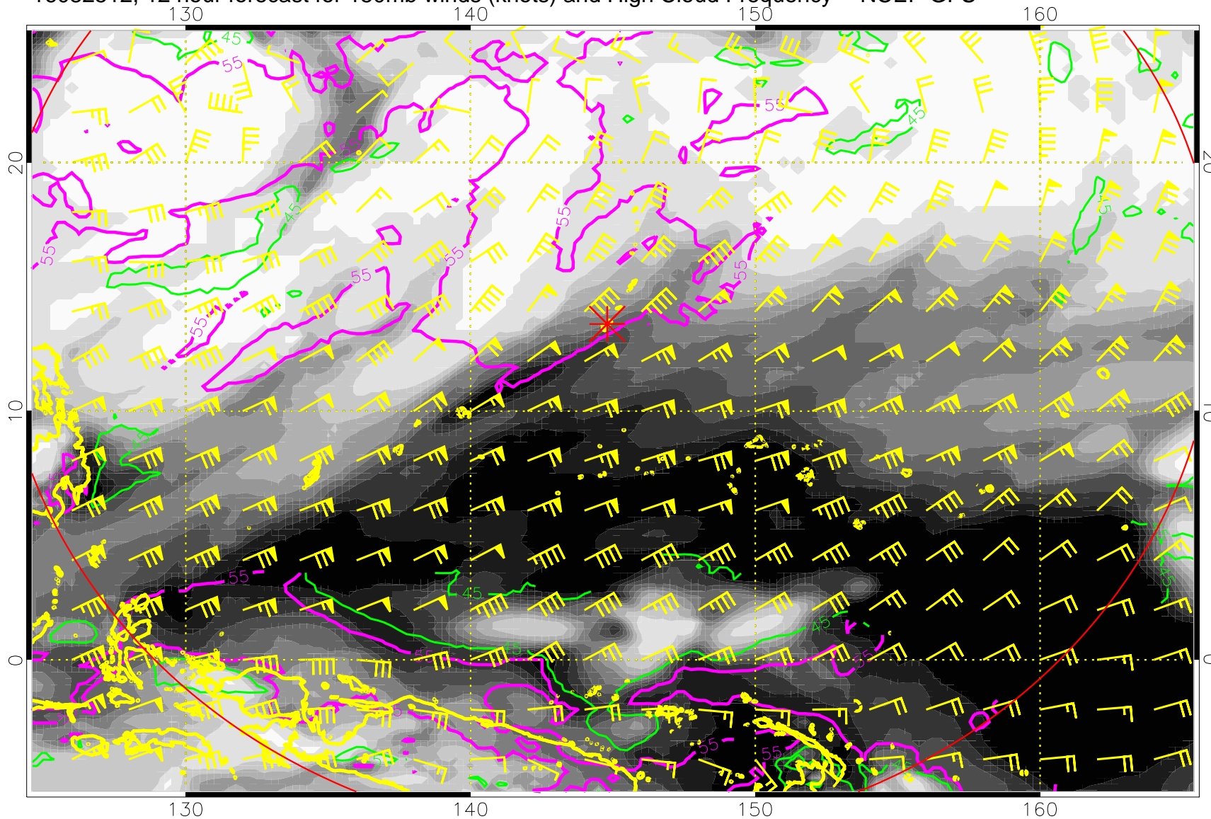
16082512, 12 hour forecast for 150mb winds (knots) and High Cloud Frequency -- NCEP GFS
