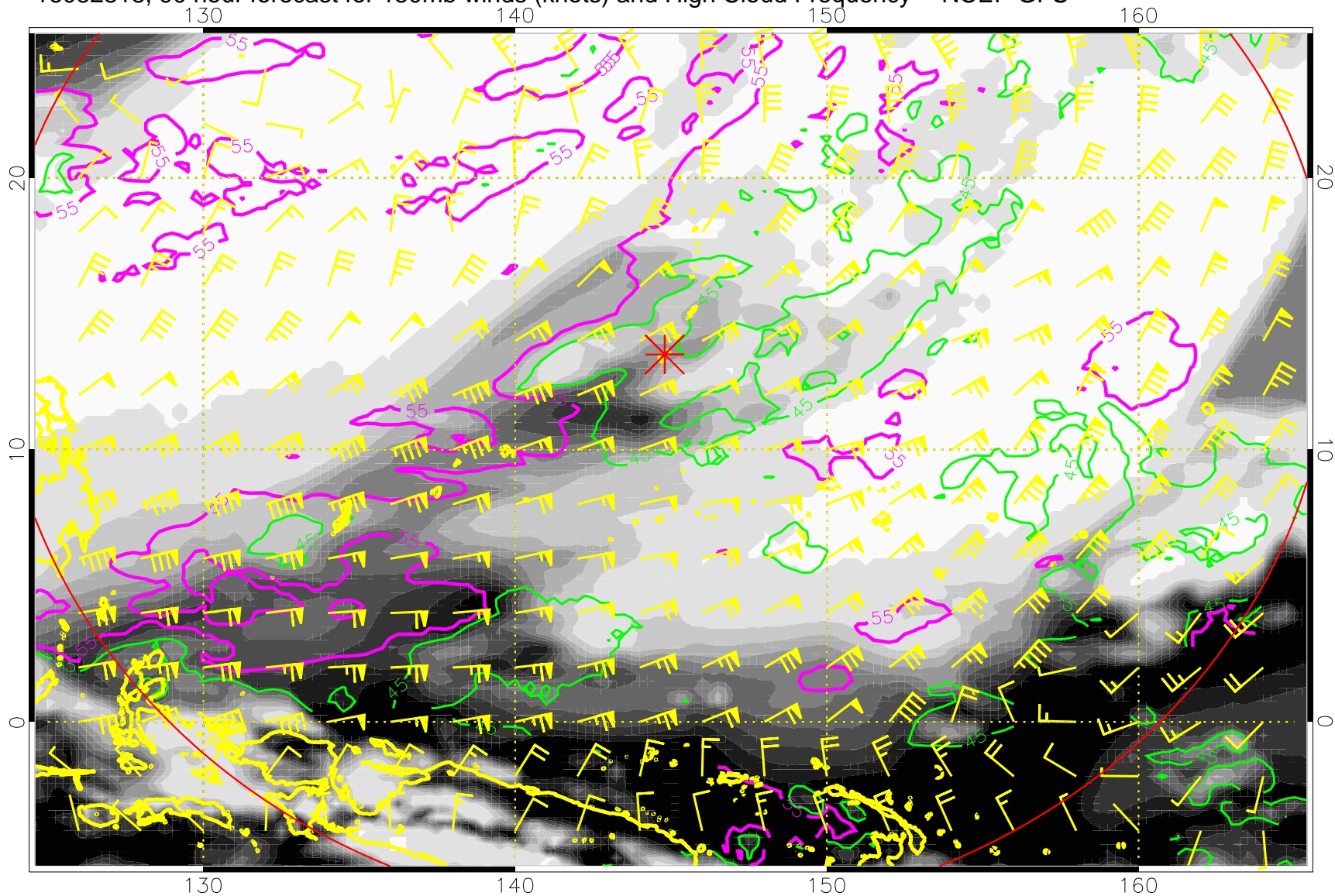
16082818, 90 hour forecast for 150mb winds (knots) and High Cloud Frequency -- NCEP GFS
