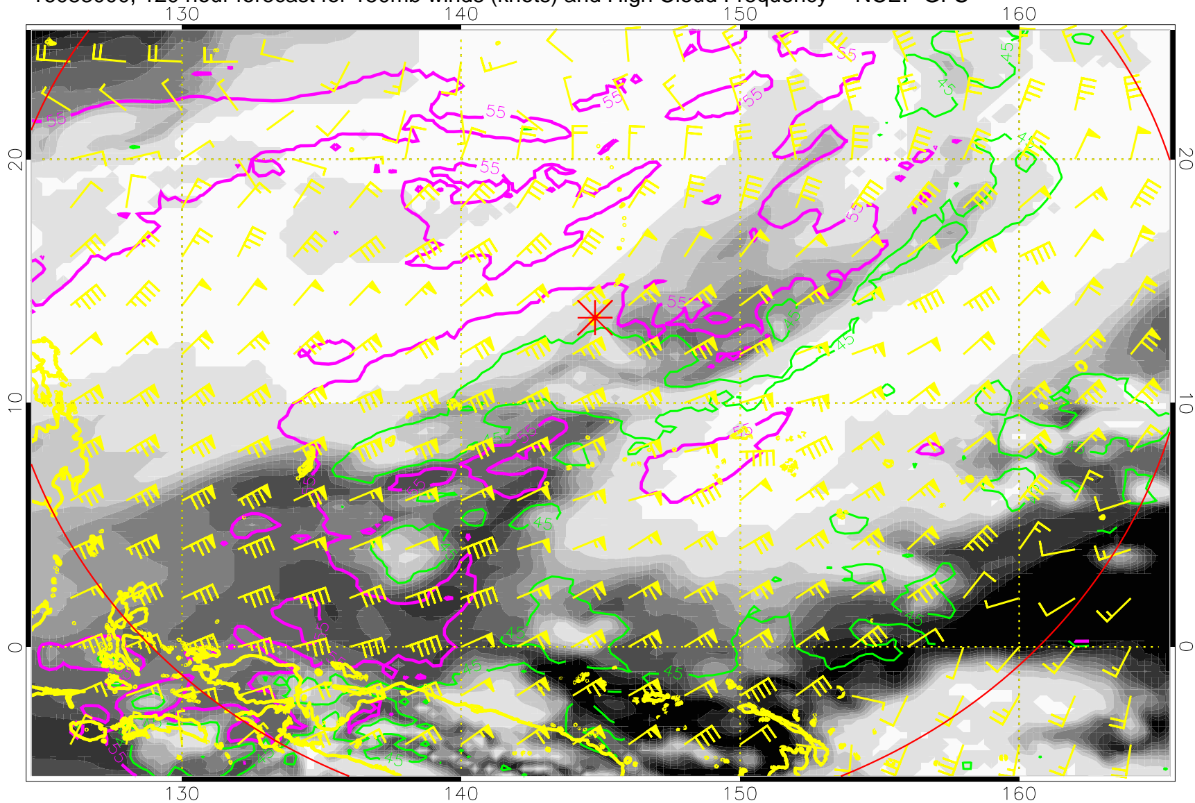
16083000, 120 hour forecast for 150mb winds (knots) and High Cloud Frequency -- NCEP GFS
