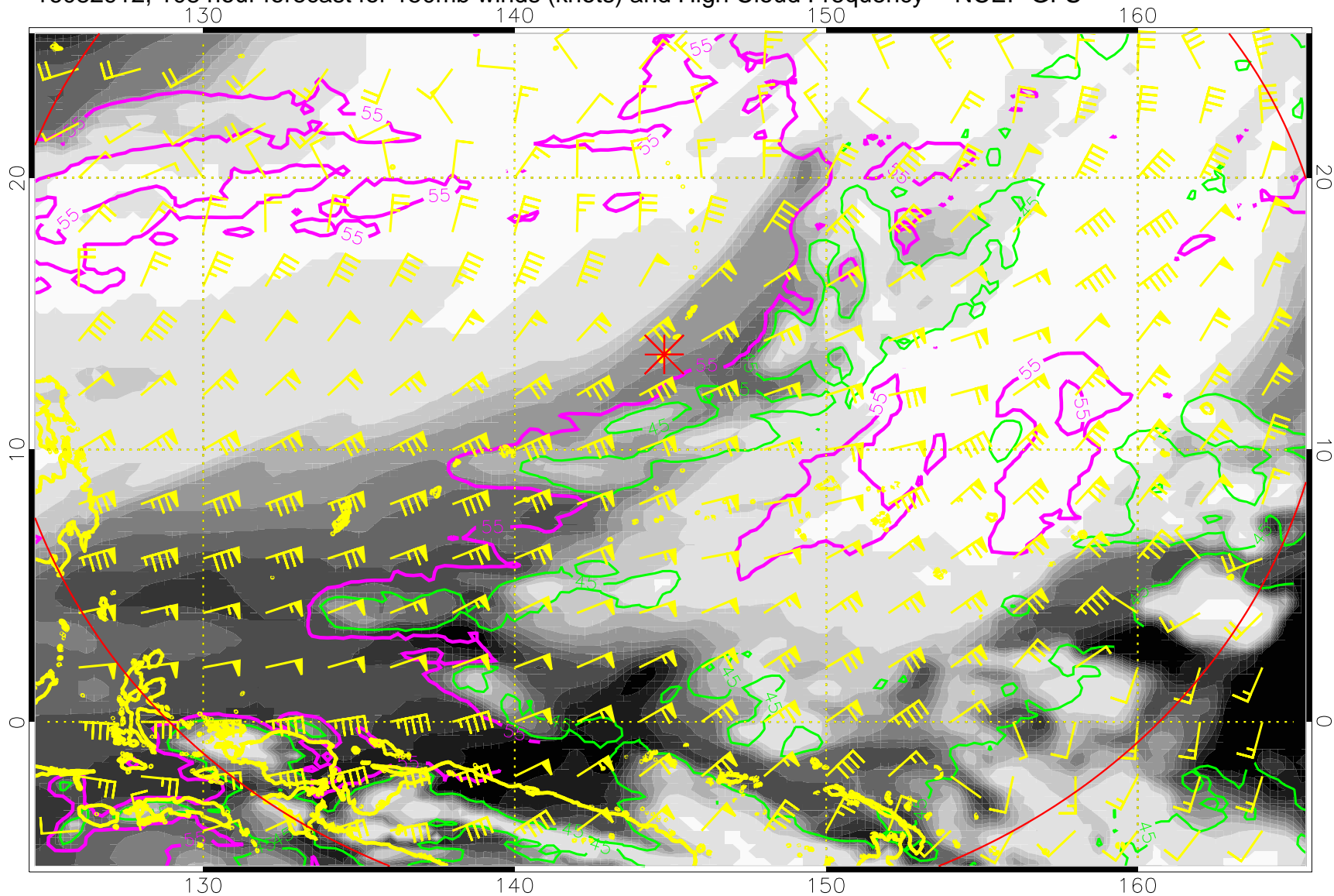
16082912, 108 hour forecast for 150mb winds (knots) and High Cloud Frequency -- NCEP GFS
