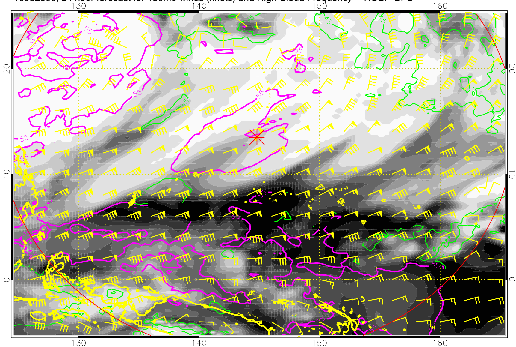
16082600, 24 hour forecast for 150mb winds (knots) and High Cloud Frequency -- NCEP GFS
