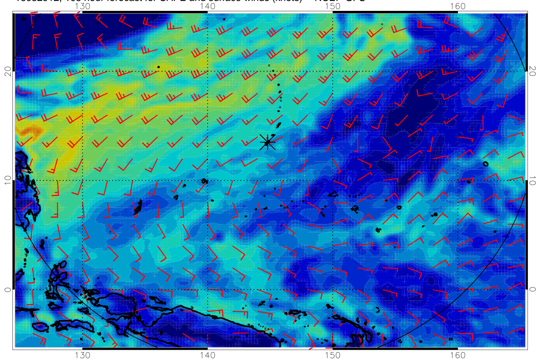
16082912, 108 hour forecast for CAPE and surface winds (knots) -- NCEP GFS
