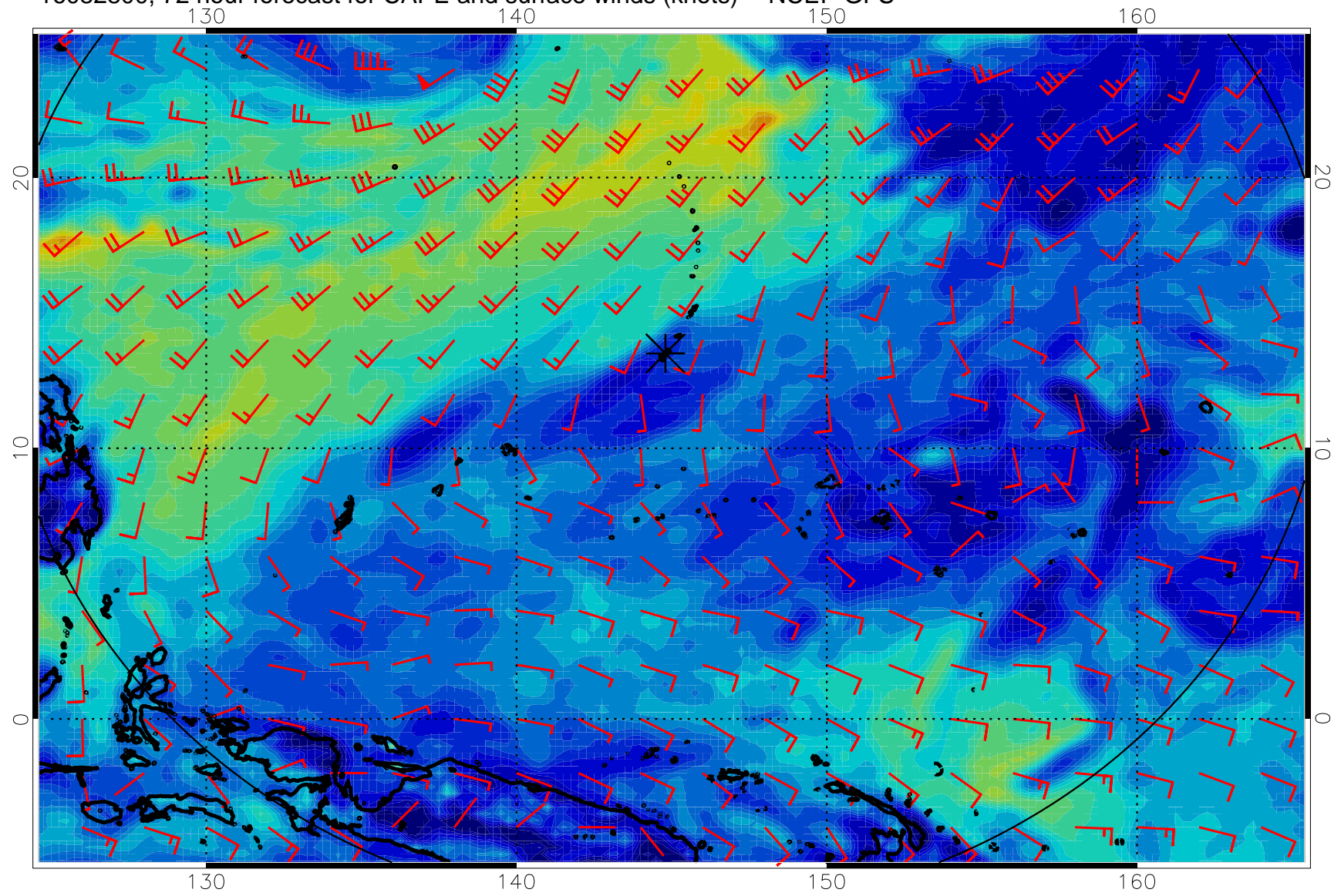
16082800, 72 hour forecast for CAPE and surface winds (knots) -- NCEP GFS
