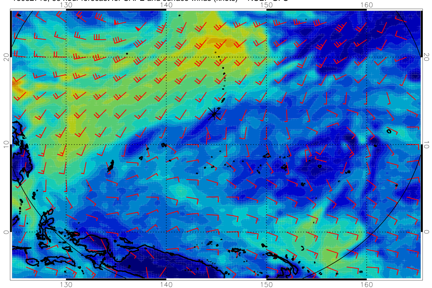
16082718, 66 hour forecast for CAPE and surface winds (knots) -- NCEP GFS
