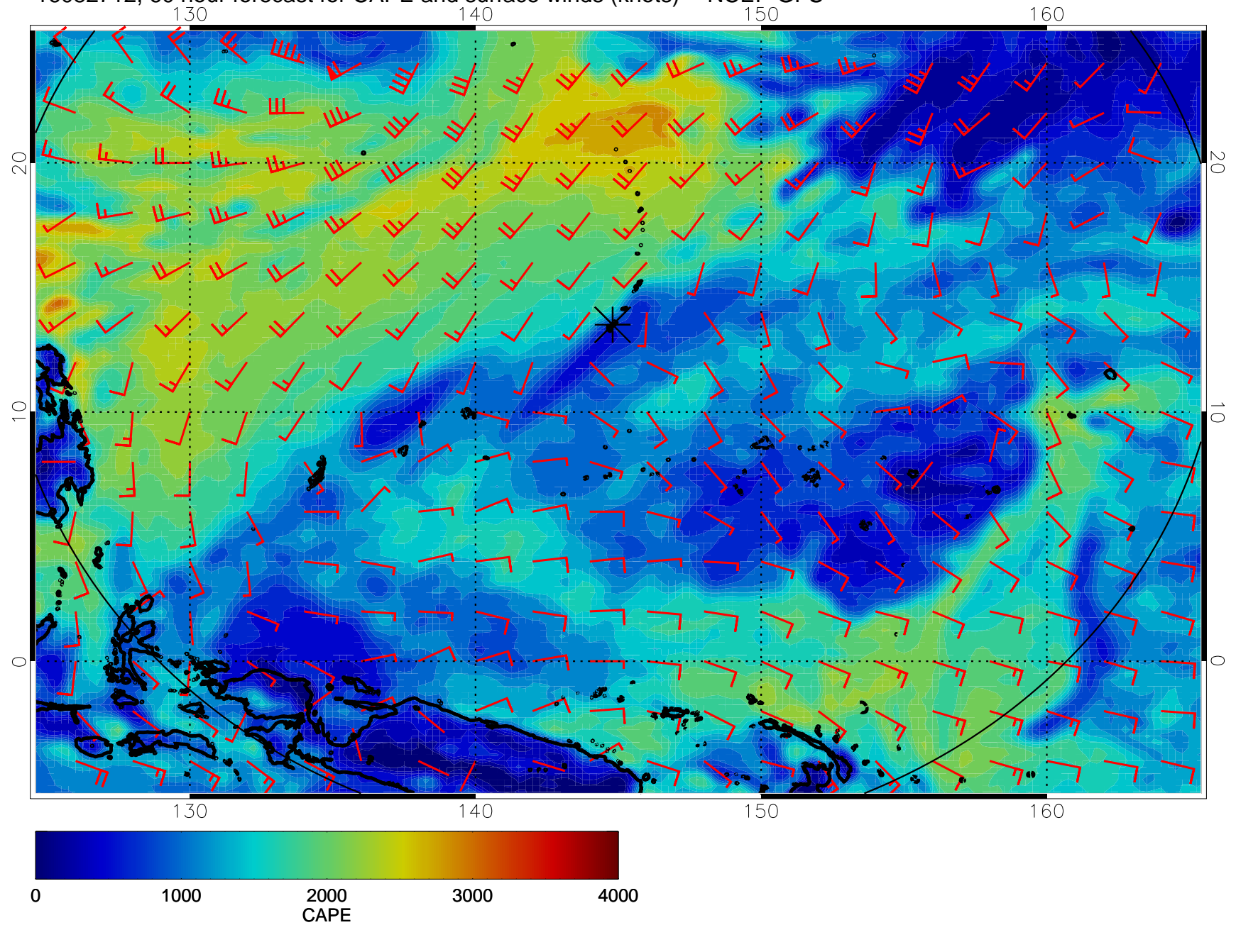
16082712, 60 hour forecast for CAPE and surface winds (knots) -- NCEP GFS
