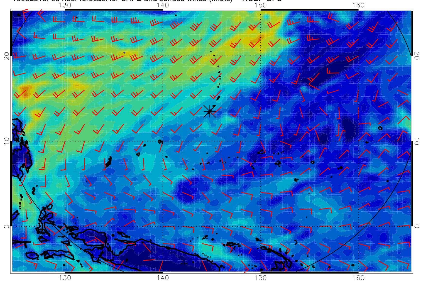
16082818, 90 hour forecast for CAPE and surface winds (knots) -- NCEP GFS
