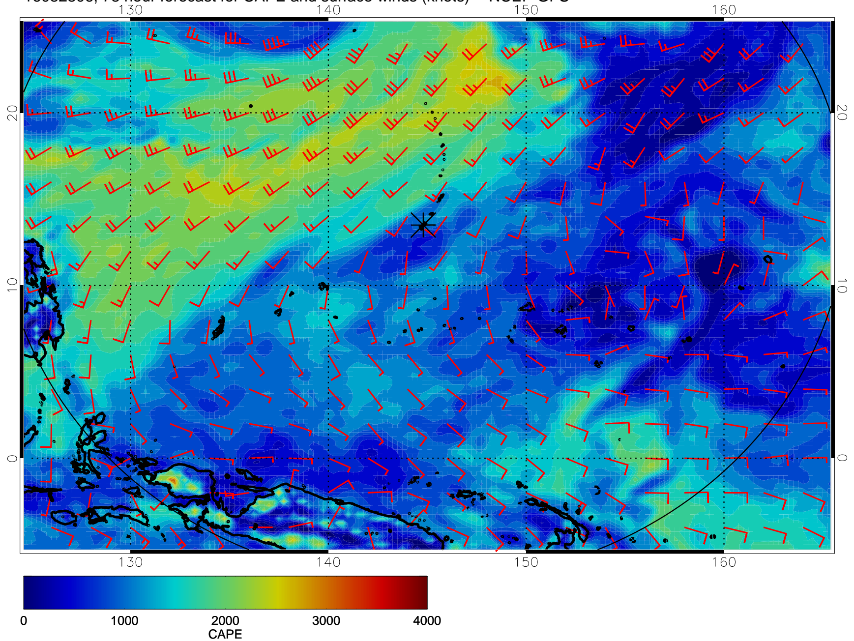
16082806, 78 hour forecast for CAPE and surface winds (knots) -- NCEP GFS
