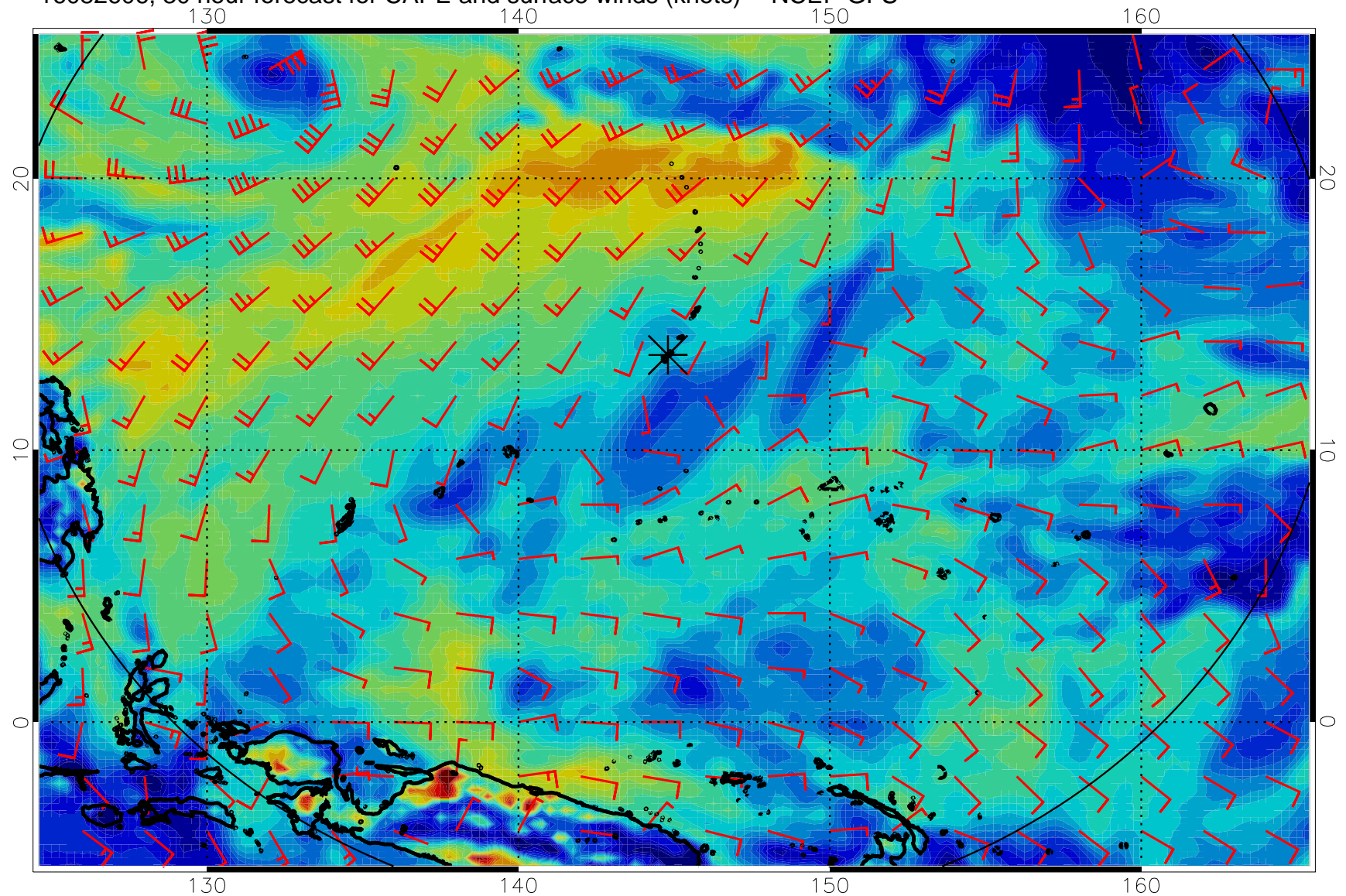
16082606, 30 hour forecast for CAPE and surface winds (knots) -- NCEP GFS
