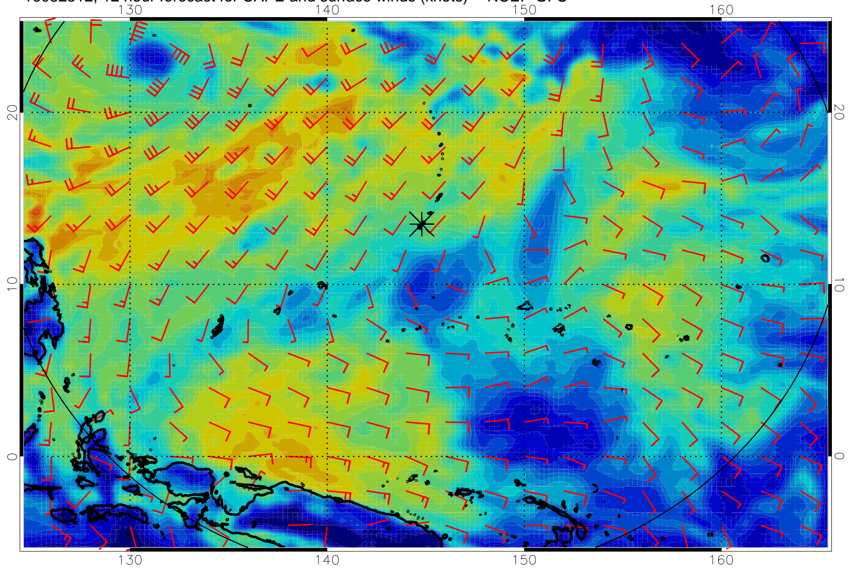
16082512, 12 hour forecast for CAPE and surface winds (knots) -- NCEP GFS
