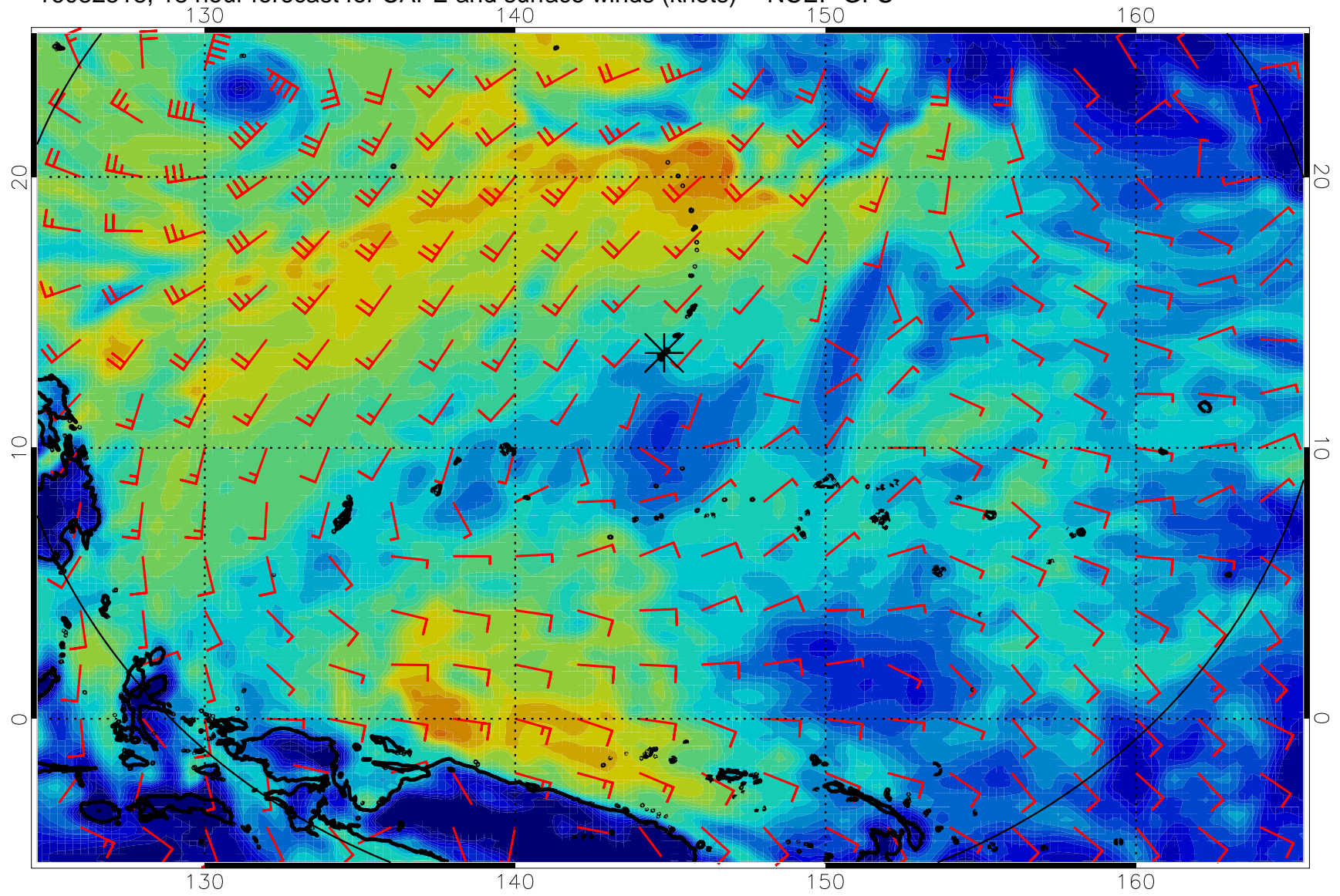
16082518, 18 hour forecast for CAPE and surface winds (knots) -- NCEP GFS
