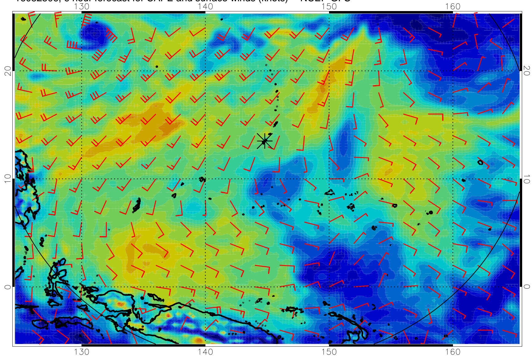
16082506, 6 hour forecast for CAPE and surface winds (knots) -- NCEP GFS
