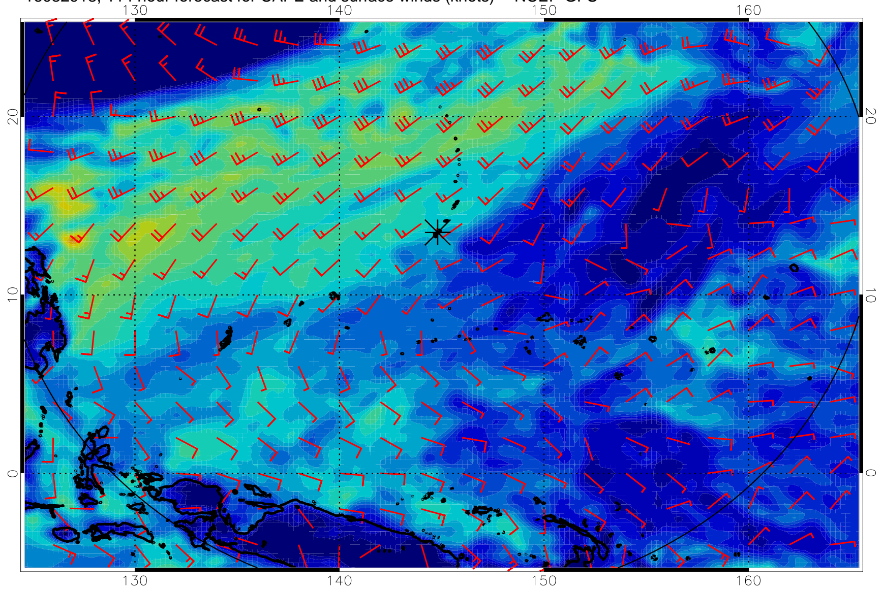
16082918, 114 hour forecast for CAPE and surface winds (knots) -- NCEP GFS
