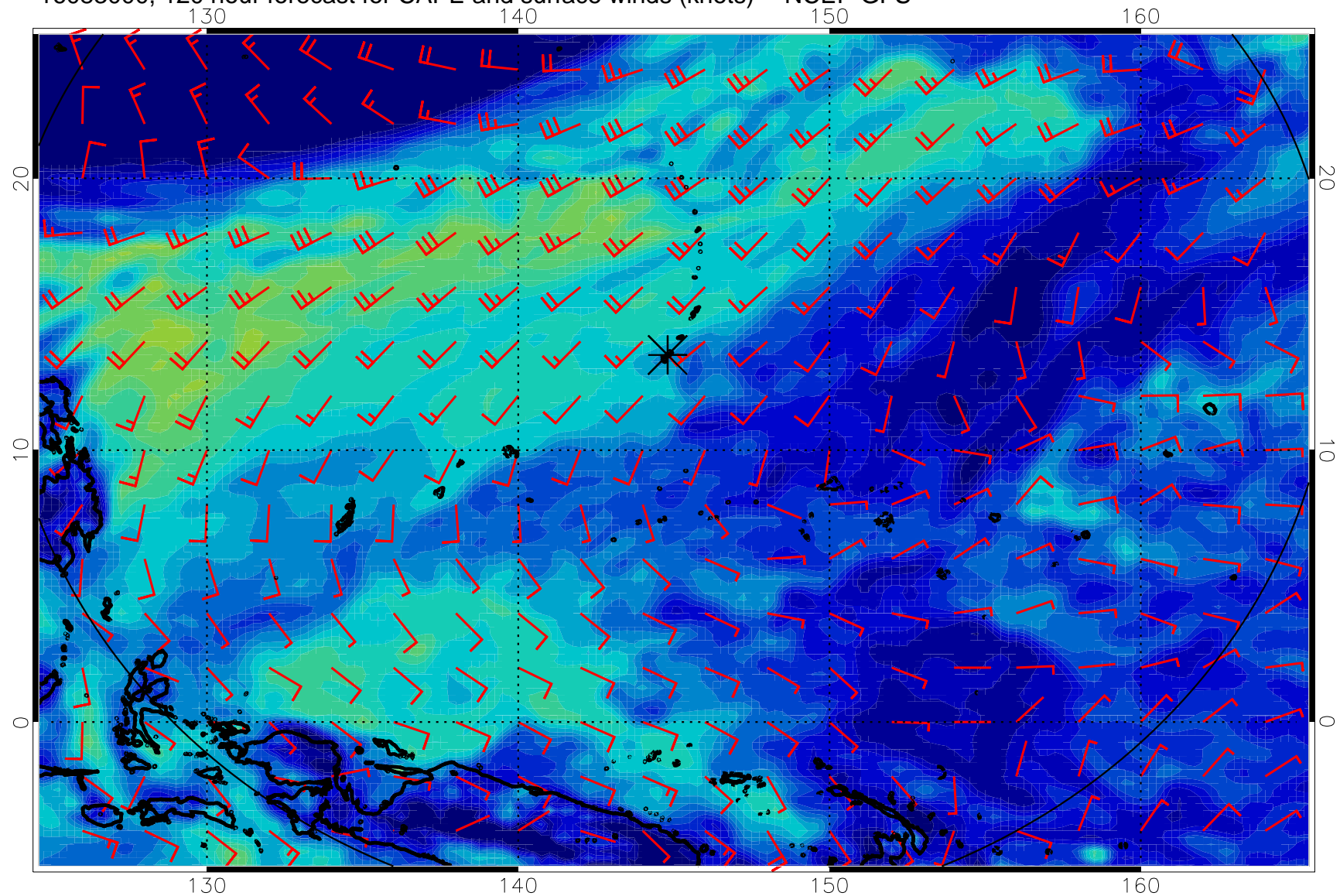
16083000, 120 hour forecast for CAPE and surface winds (knots) -- NCEP GFS
