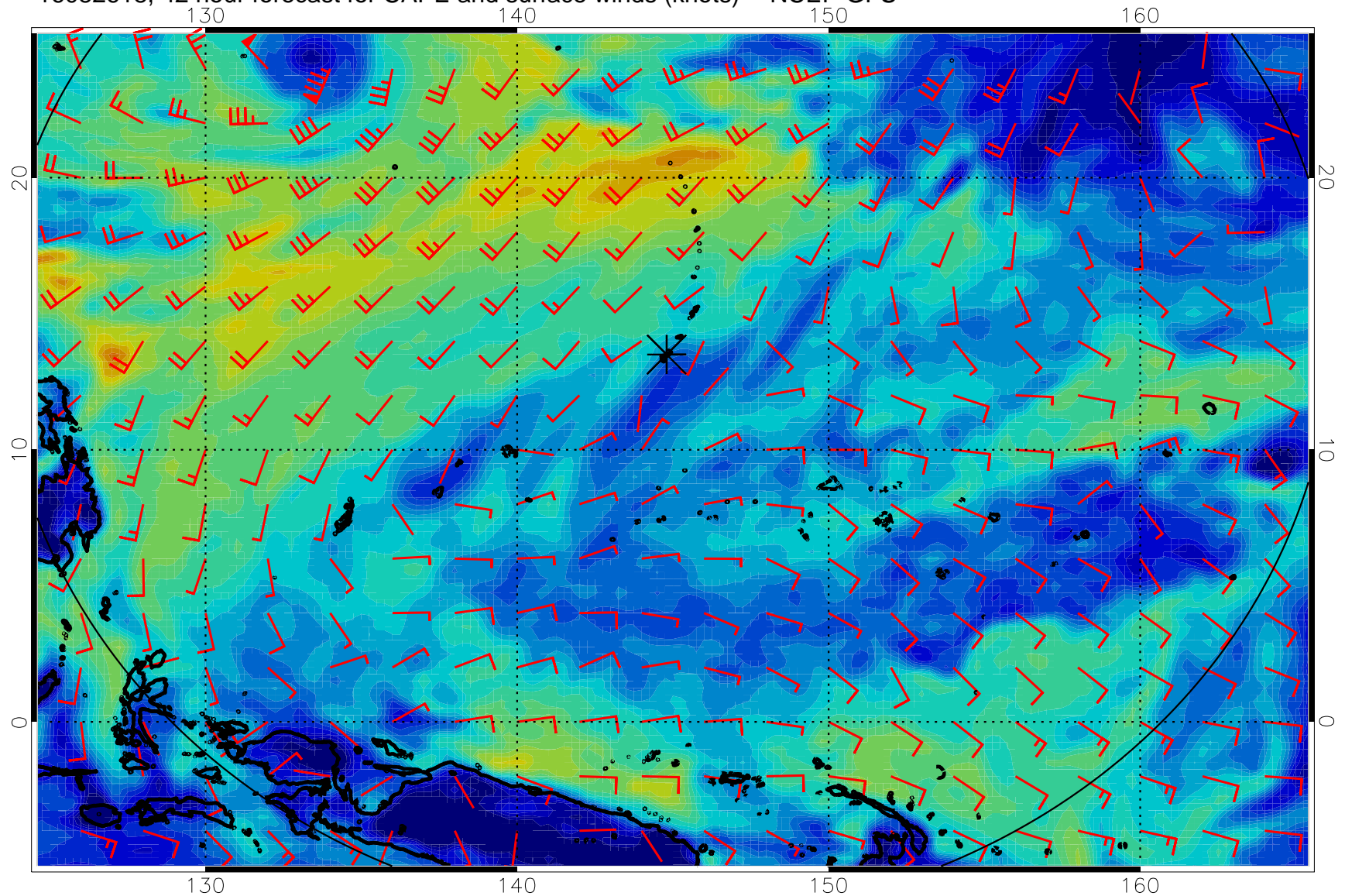
16082618, 42 hour forecast for CAPE and surface winds (knots) -- NCEP GFS
