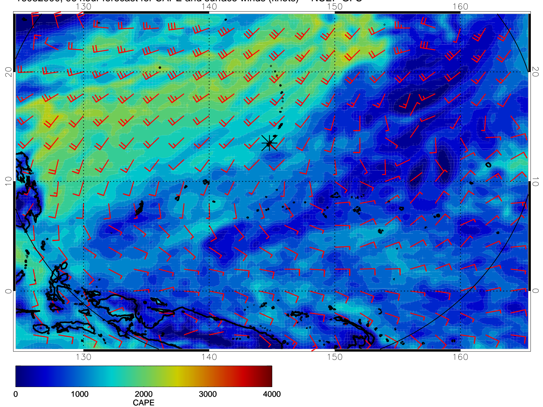
16082900, 96 hour forecast for CAPE and surface winds (knots) -- NCEP GFS
