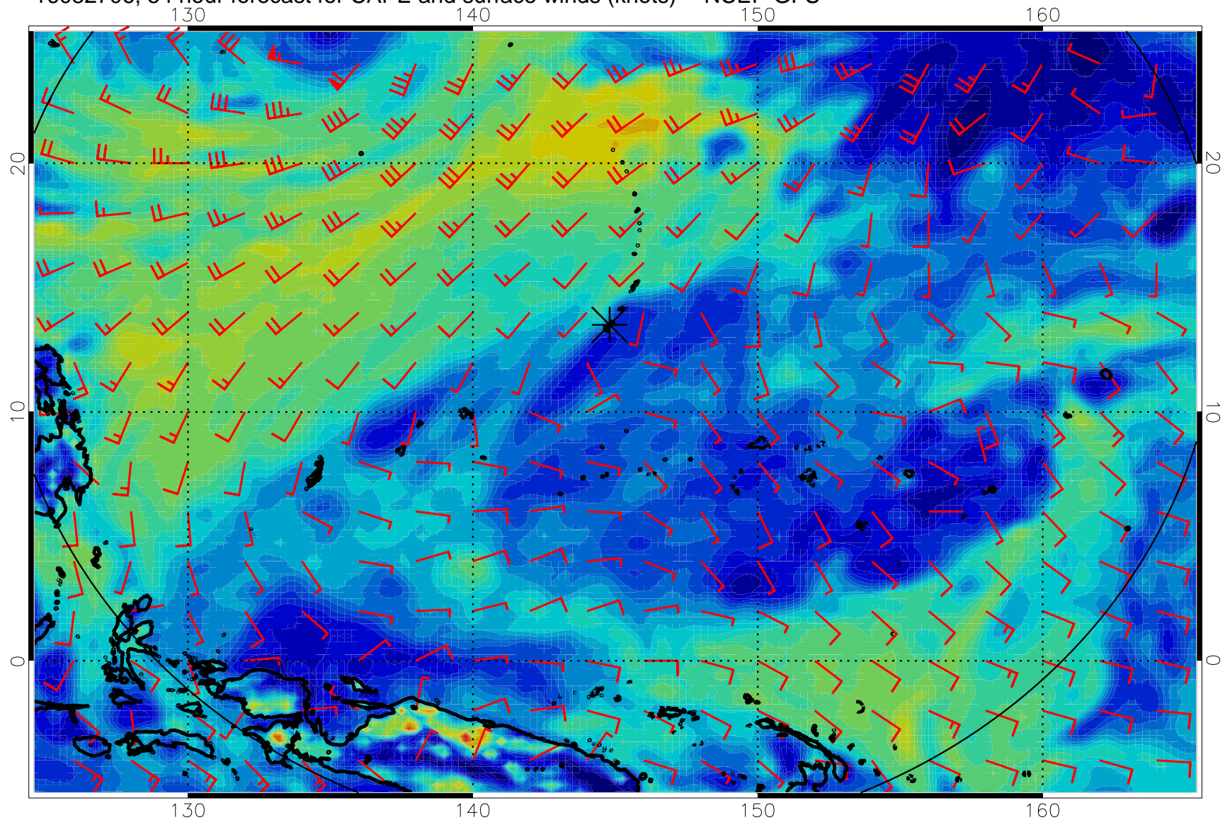
16082706, 54 hour forecast for CAPE and surface winds (knots) -- NCEP GFS
