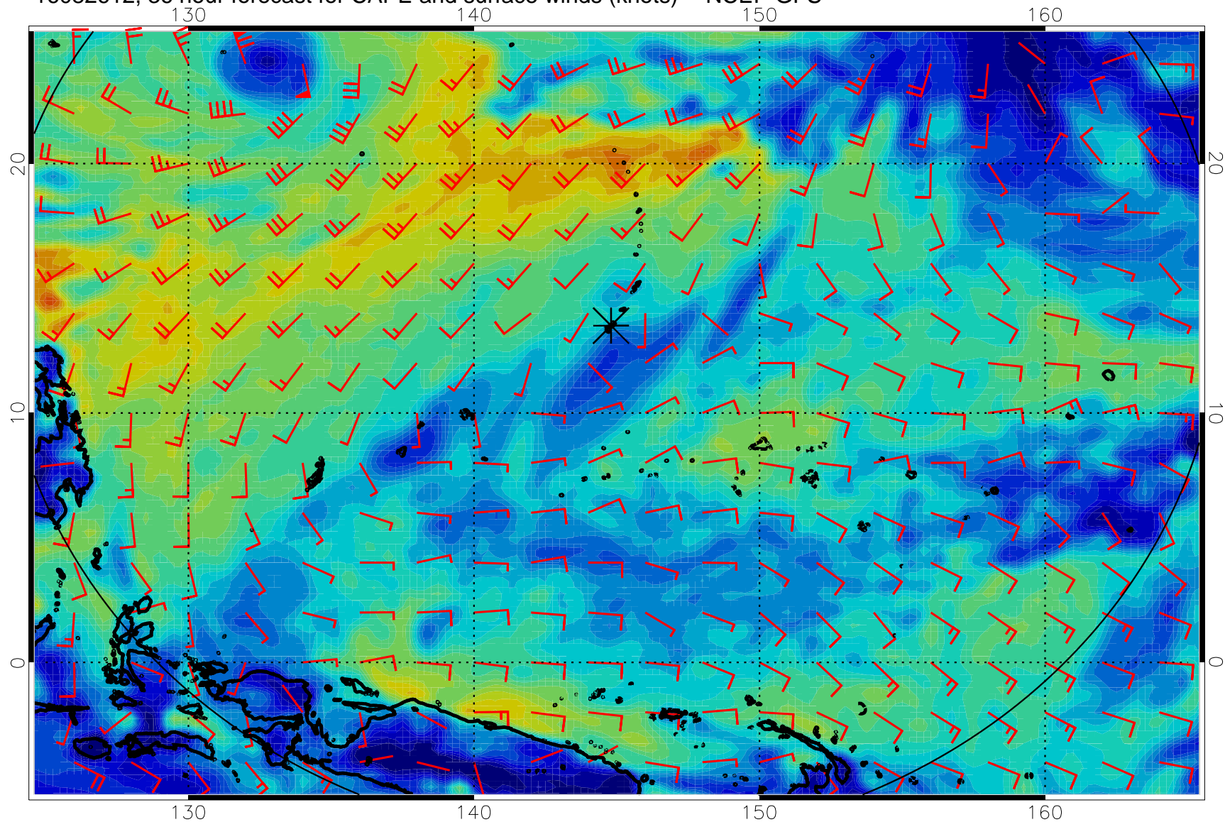
16082612, 36 hour forecast for CAPE and surface winds (knots) -- NCEP GFS
