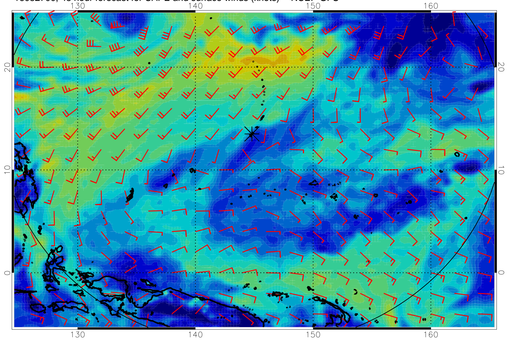
16082700, 48 hour forecast for CAPE and surface winds (knots) -- NCEP GFS
