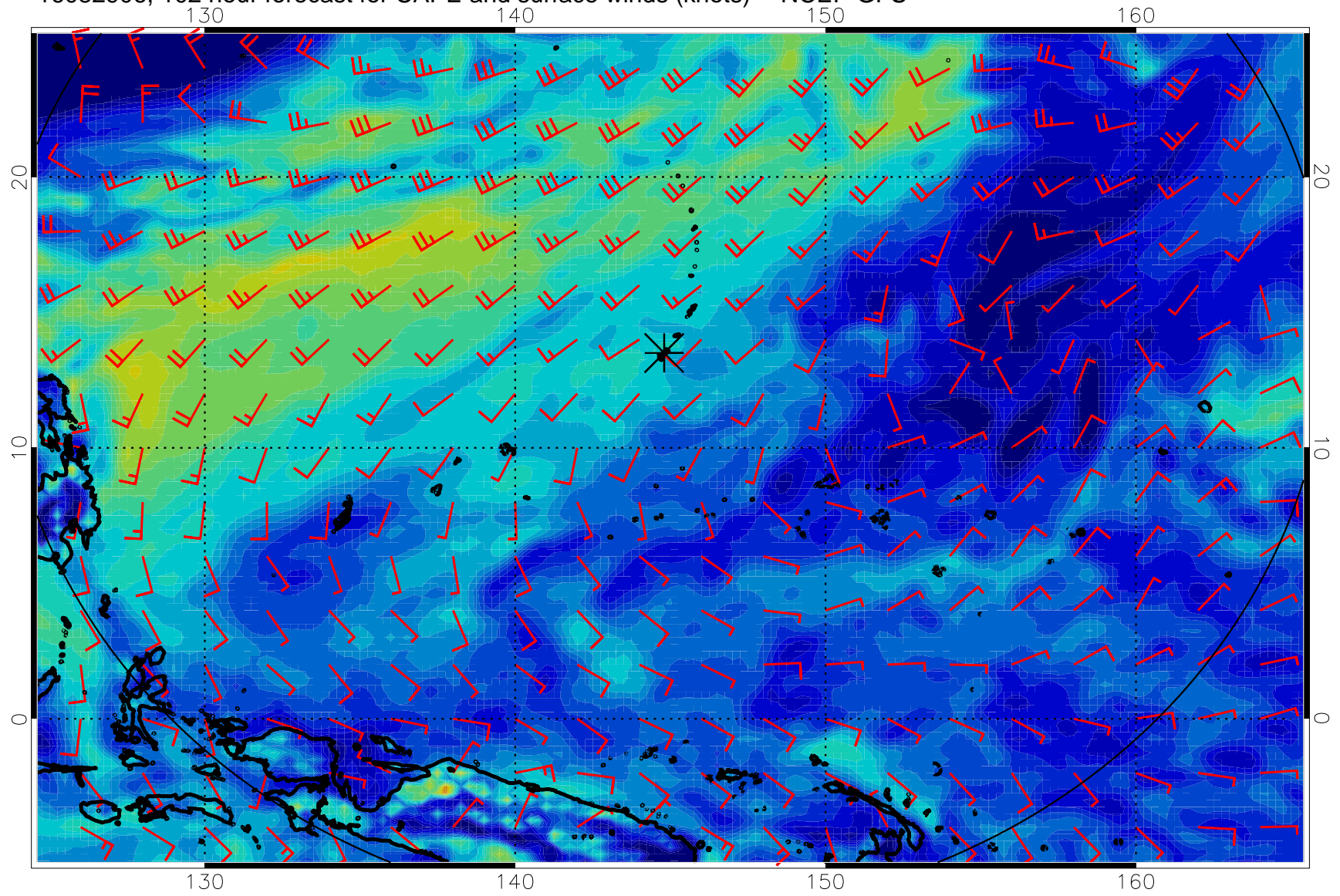
16082906, 102 hour forecast for CAPE and surface winds (knots) -- NCEP GFS
