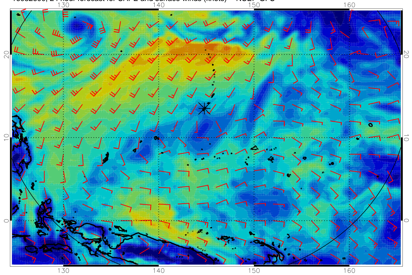
16082600, 24 hour forecast for CAPE and surface winds (knots) -- NCEP GFS
