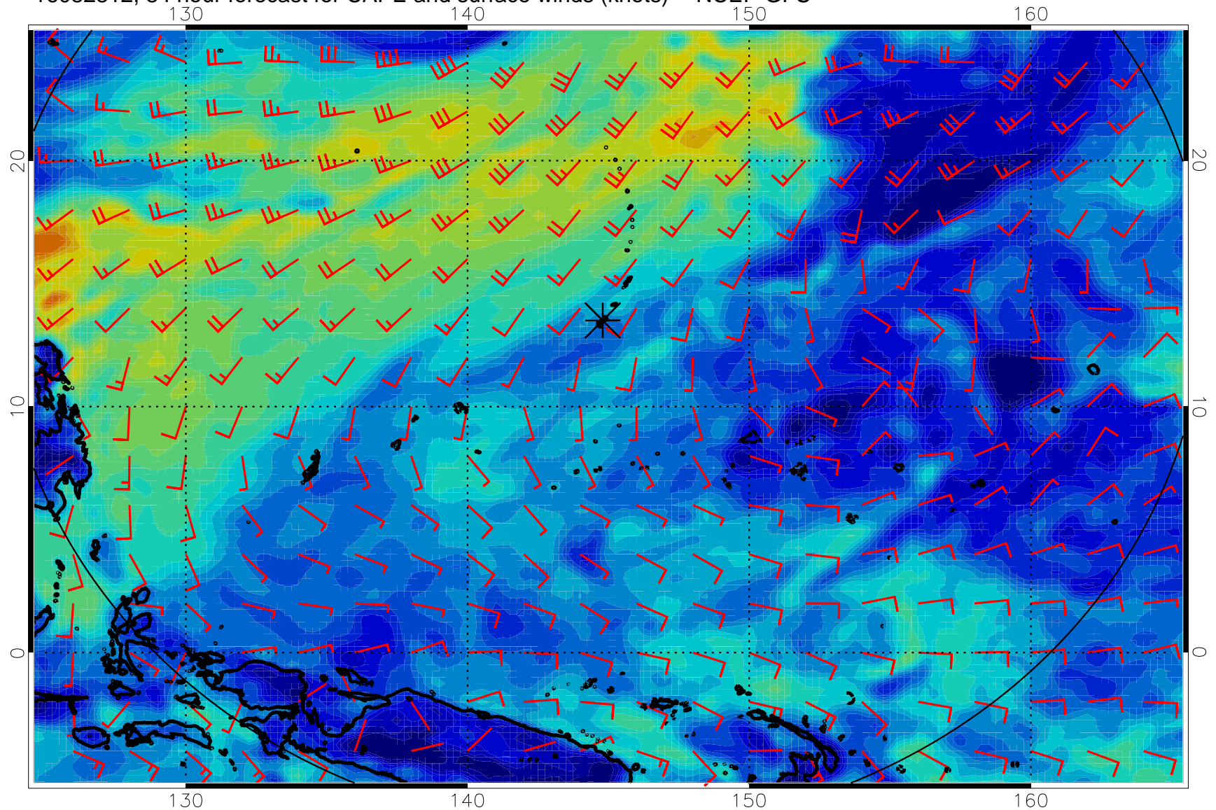
16082812, 84 hour forecast for CAPE and surface winds (knots) -- NCEP GFS
