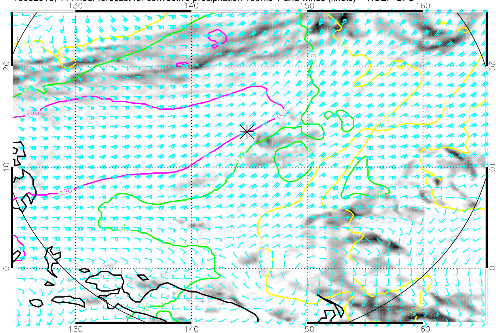
16082918, 114 hour forecast for convective precipitation 100mb T and winds (knots) -- NCEP GFS
