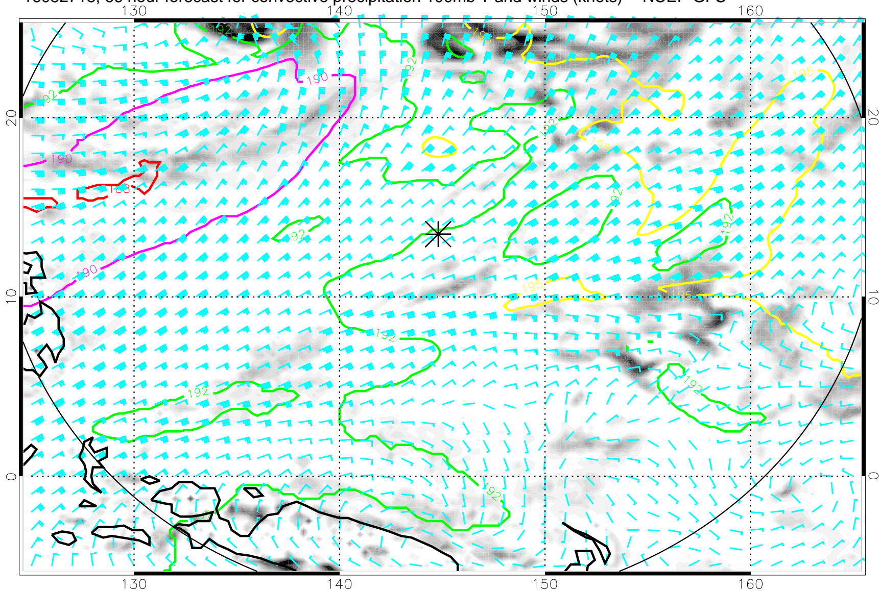
16082718, 66 hour forecast for convective precipitation 100mb T and winds (knots) -- NCEP GFS
