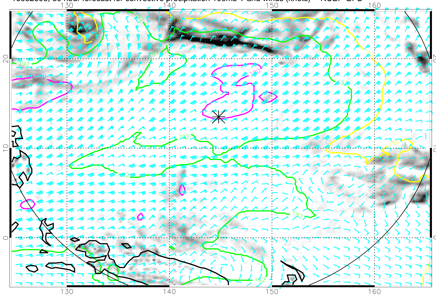
16082606, 30 hour forecast for convective precipitation 100mb T and winds (knots) -- NCEP GFS
