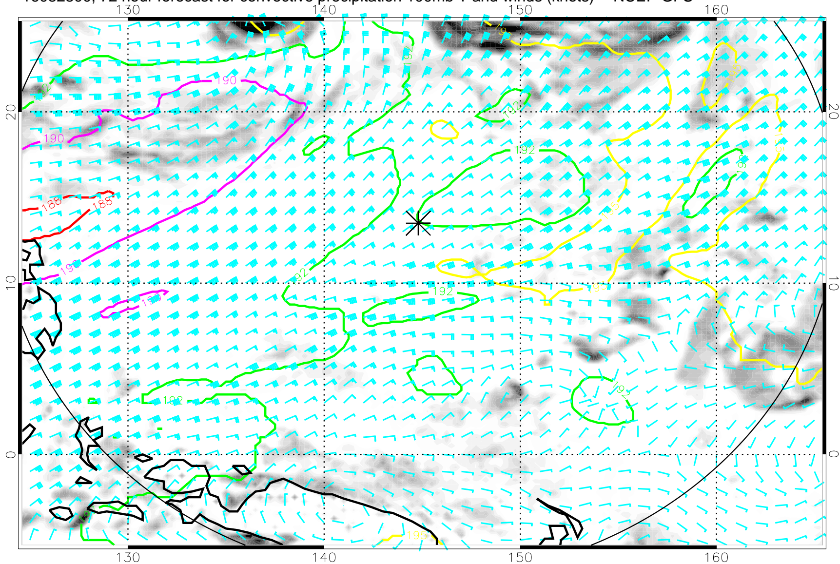
16082800, 72 hour forecast for convective precipitation 100mb T and winds (knots) -- NCEP GFS
