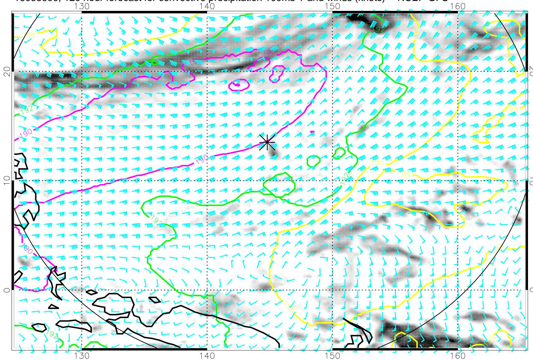
16083000, 120 hour forecast for convective precipitation 100mb T and winds (knots) -- NCEP GFS
