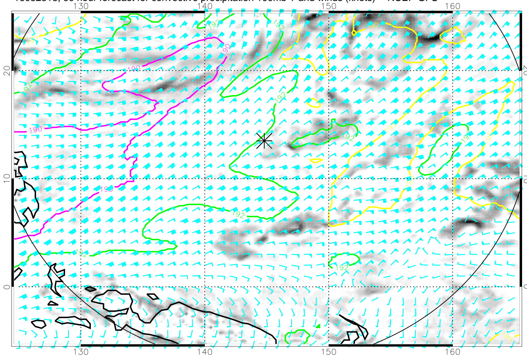
16082818, 90 hour forecast for convective precipitation 100mb T and winds (knots) -- NCEP GFS
