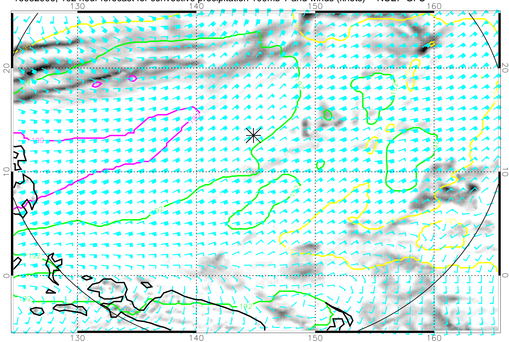
16082906, 102 hour forecast for convective precipitation 100mb T and winds (knots) -- NCEP GFS
