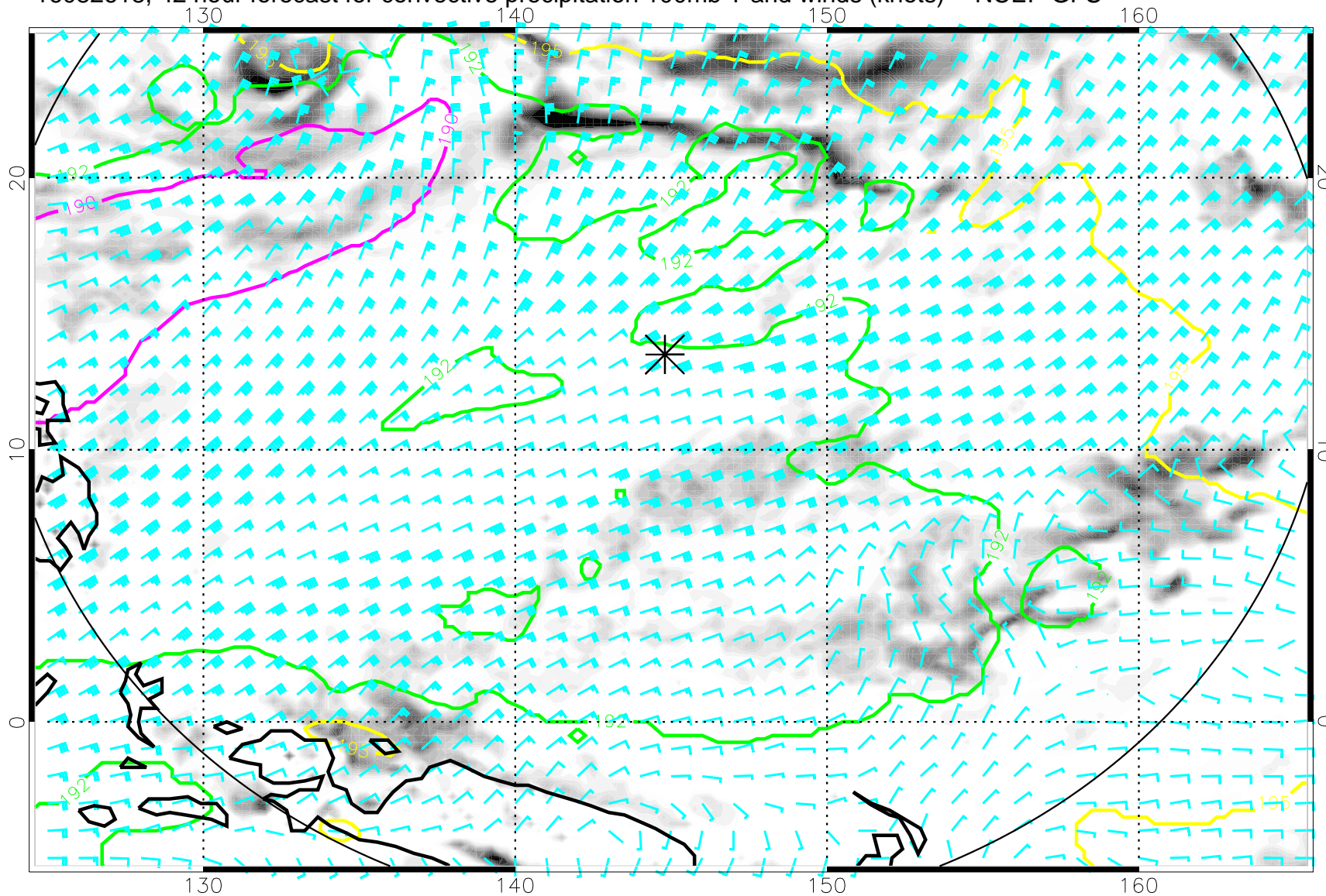
16082618, 42 hour forecast for convective precipitation 100mb T and winds (knots) -- NCEP GFS
