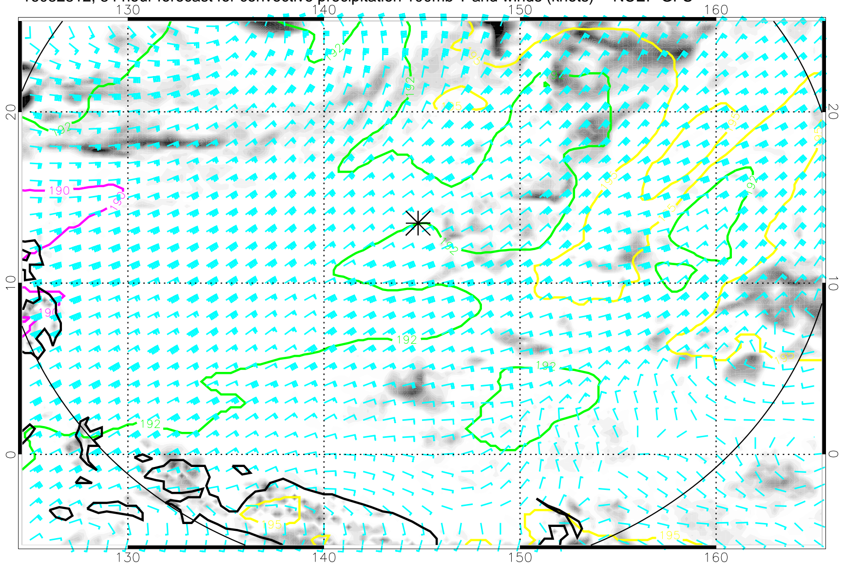
16082812, 84 hour forecast for convective precipitation 100mb T and winds (knots) -- NCEP GFS
