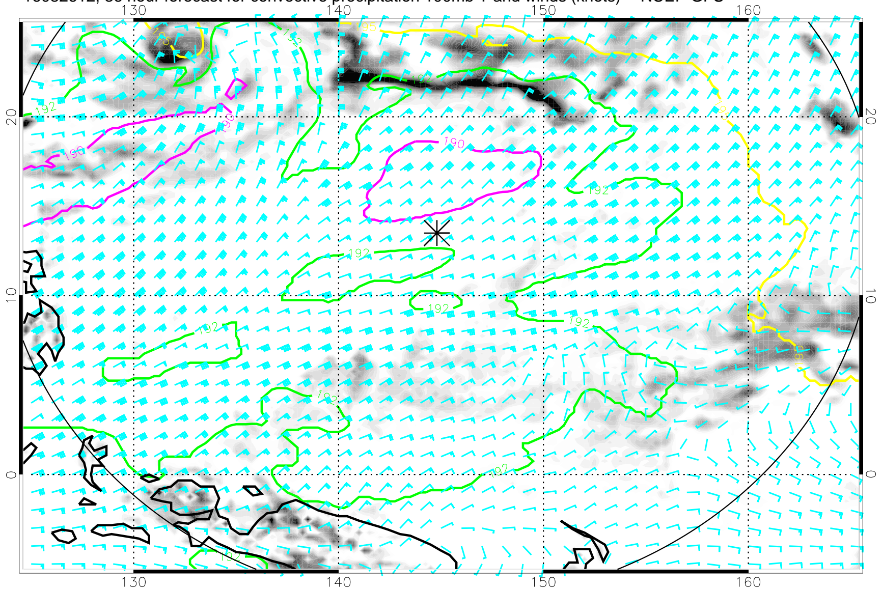
16082612, 36 hour forecast for convective precipitation 100mb T and winds (knots) -- NCEP GFS
