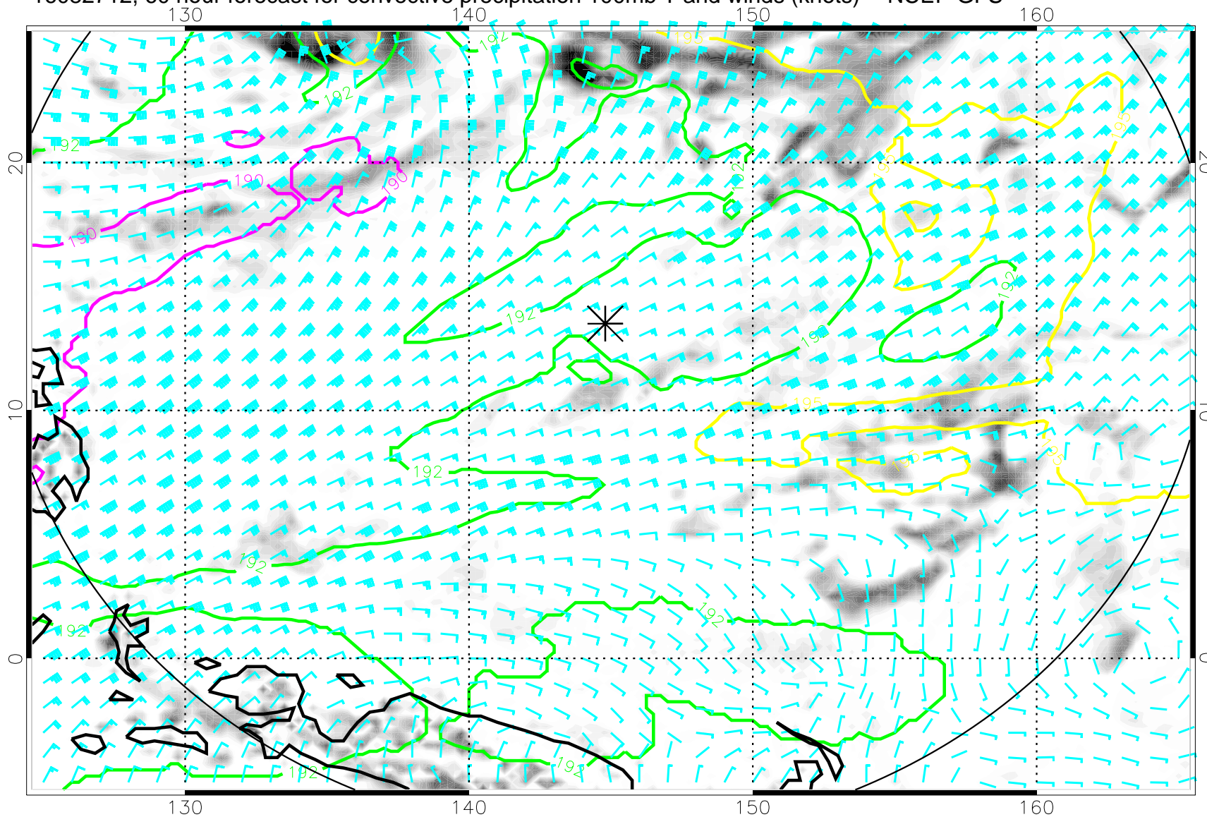
16082712, 60 hour forecast for convective precipitation 100mb T and winds (knots) -- NCEP GFS
