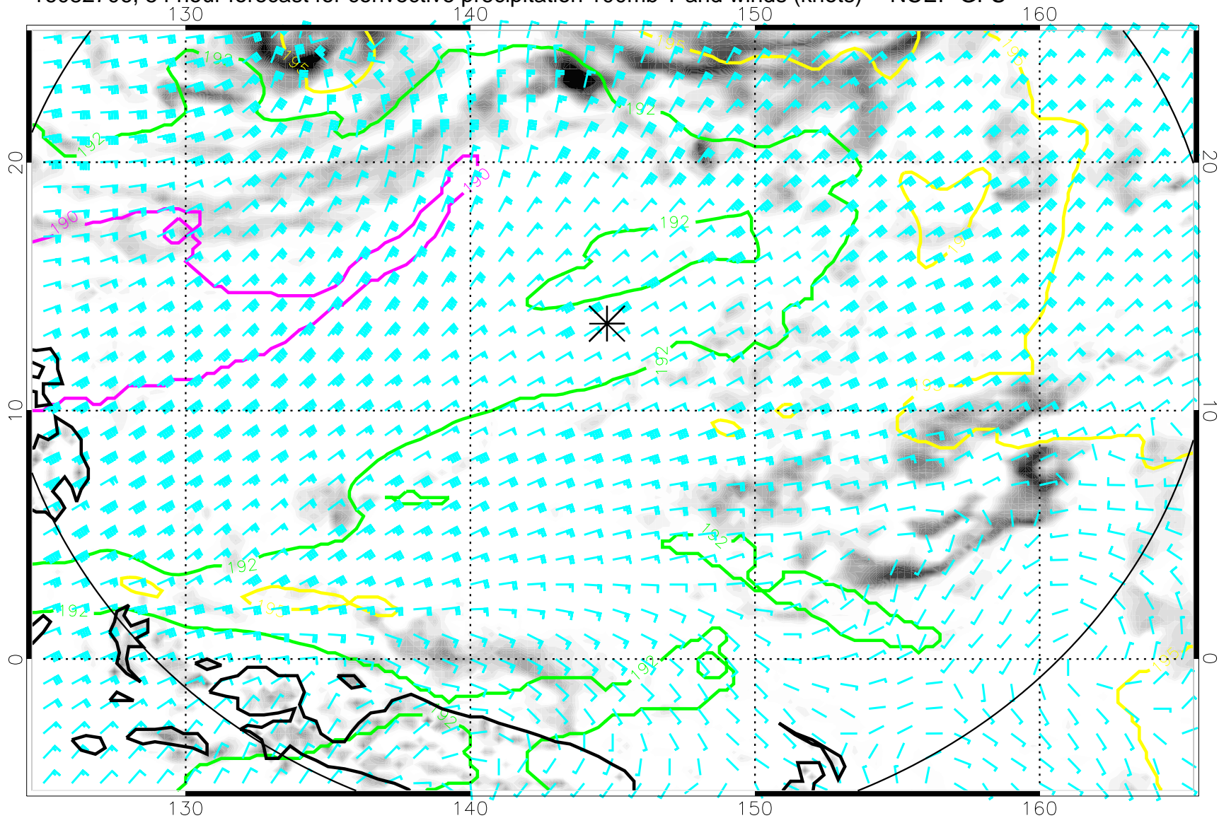
16082706, 54 hour forecast for convective precipitation 100mb T and winds (knots) -- NCEP GFS
