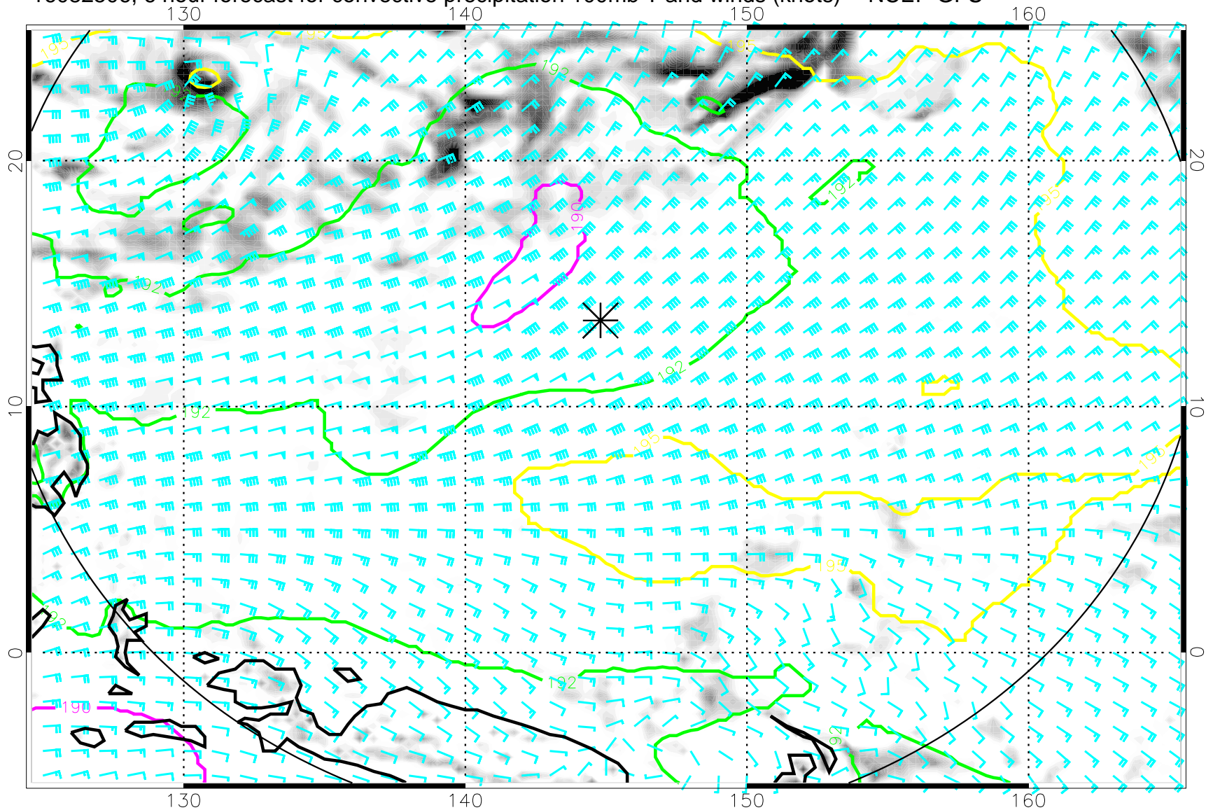
16082506, 6 hour forecast for convective precipitation 100mb T and winds (knots) -- NCEP GFS
