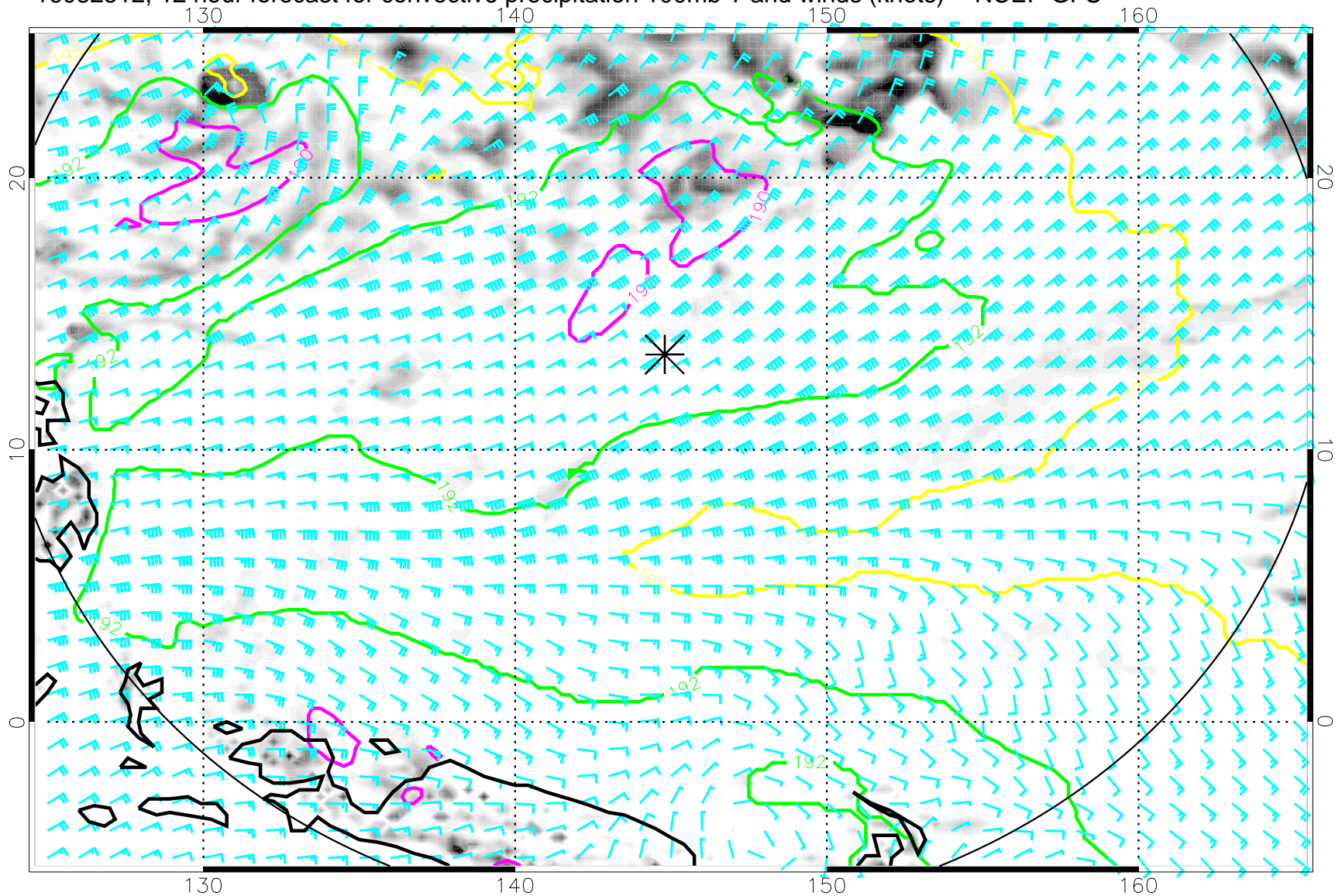
16082512, 12 hour forecast for convective precipitation 100mb T and winds (knots) -- NCEP GFS
