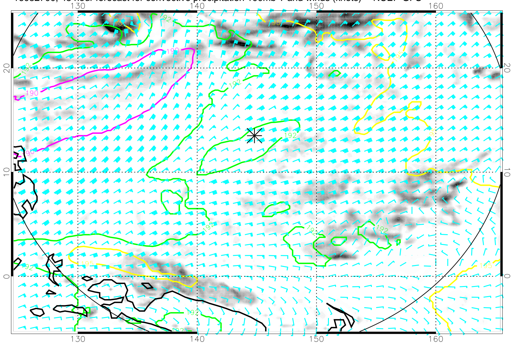
16082700, 48 hour forecast for convective precipitation 100mb T and winds (knots) -- NCEP GFS
