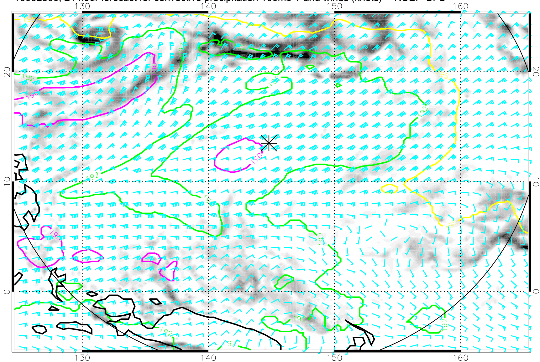
16082600, 24 hour forecast for convective precipitation 100mb T and winds (knots) -- NCEP GFS
