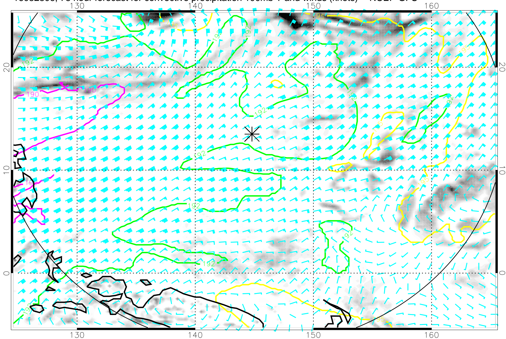
16082806, 78 hour forecast for convective precipitation 100mb T and winds (knots) -- NCEP GFS
