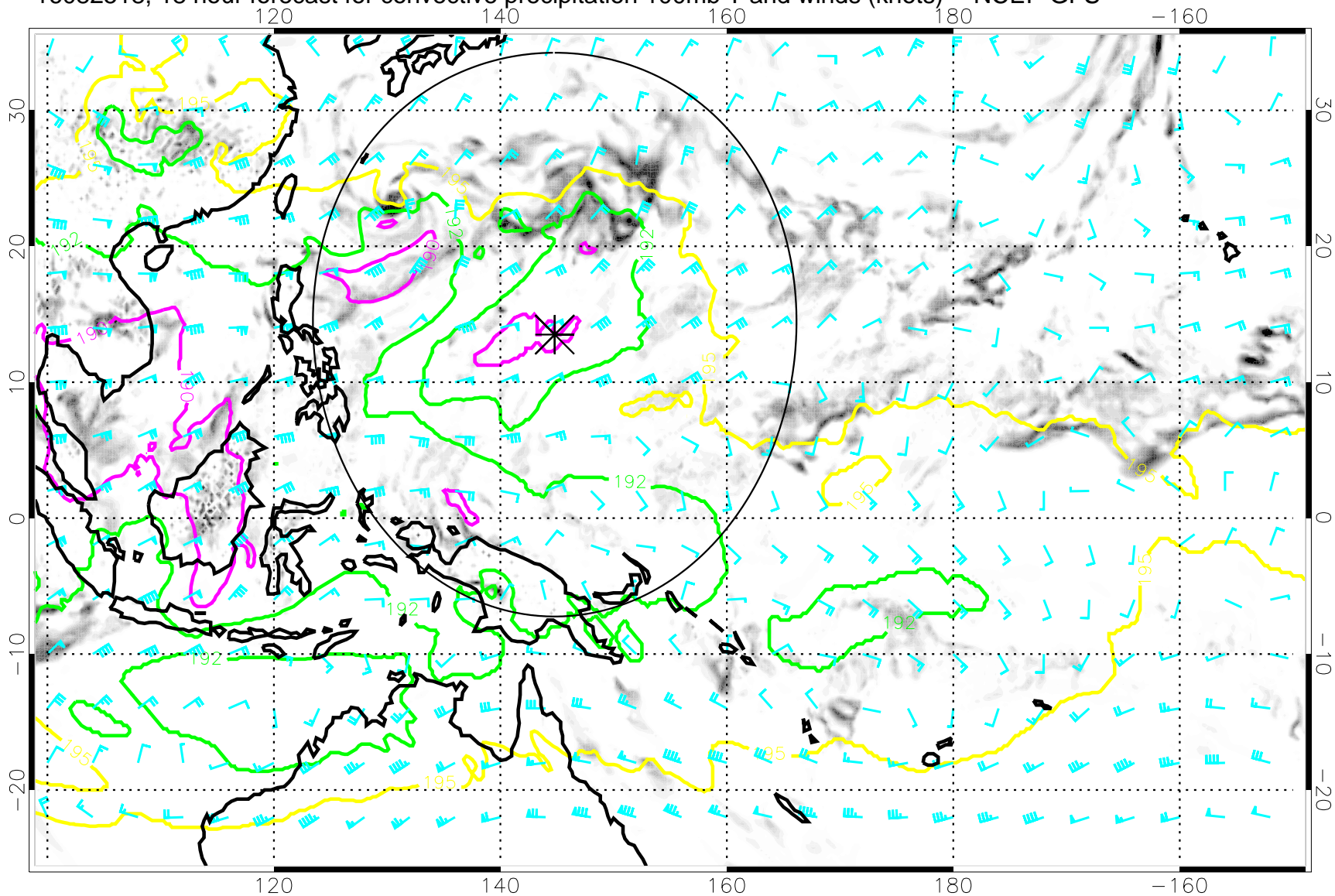
16082518, 18 hour forecast for convective precipitation 100mb T and winds (knots) -- NCEP GFS
