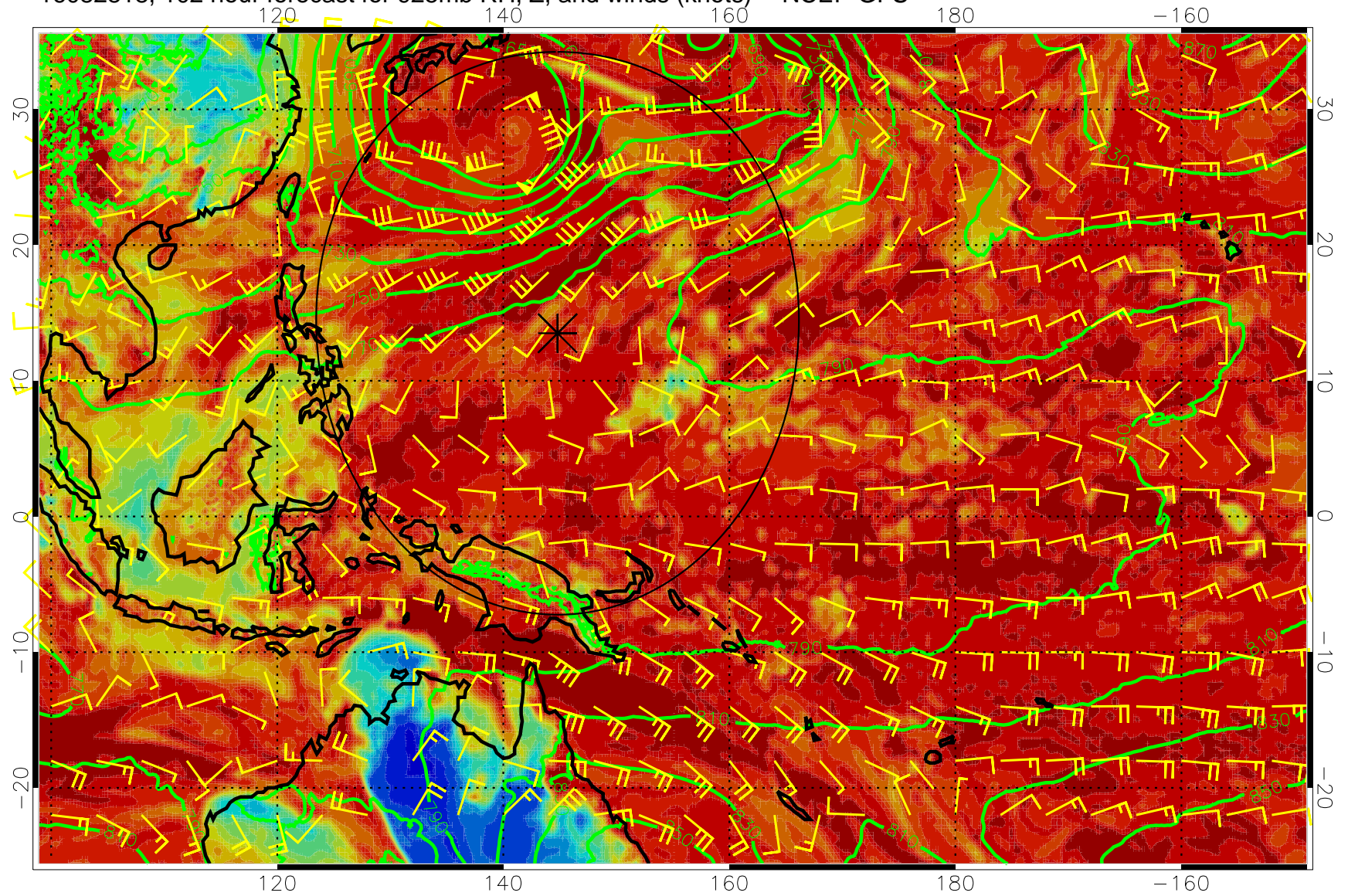
16082818, 102 hour forecast for 925mb RH, Z, and winds (knots) -- NCEP GFS
