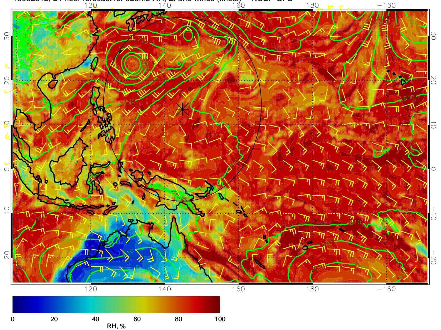
16082512, 24 hour forecast for 925mb RH, Z, and winds (knots) -- NCEP GFS
