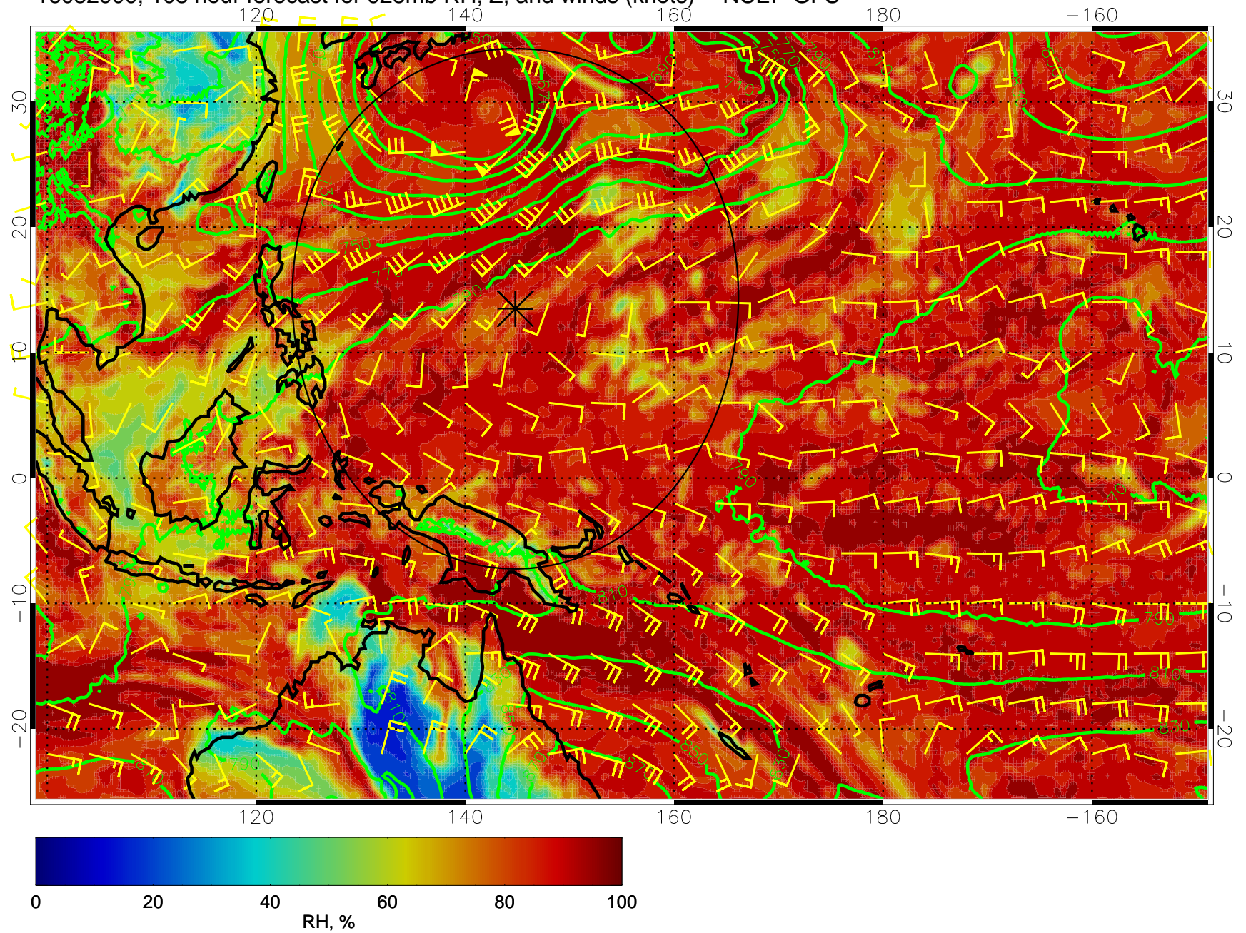
16082900, 108 hour forecast for 925mb RH, Z, and winds (knots) -- NCEP GFS
