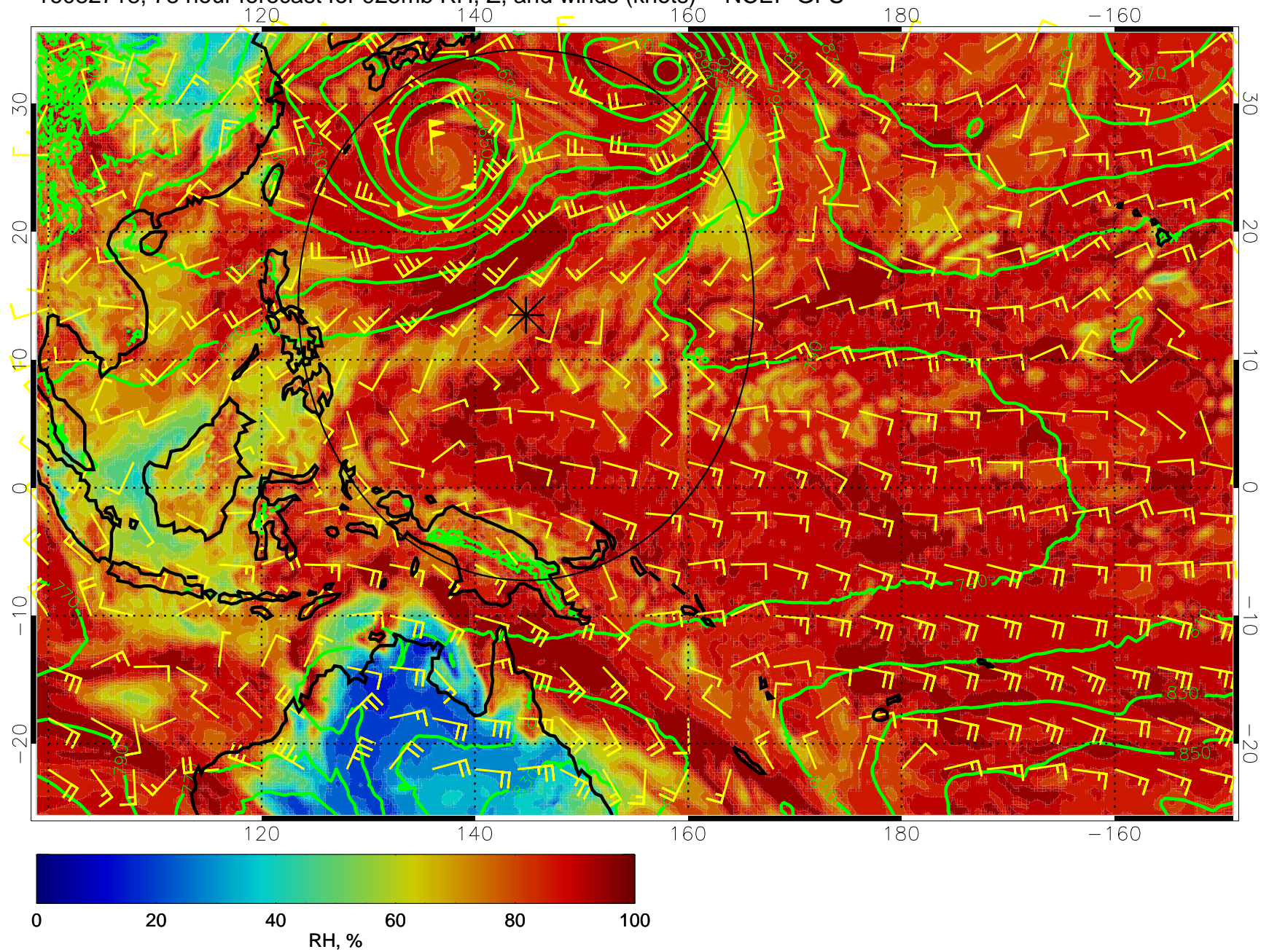
16082718, 78 hour forecast for 925mb RH, Z, and winds (knots) -- NCEP GFS
