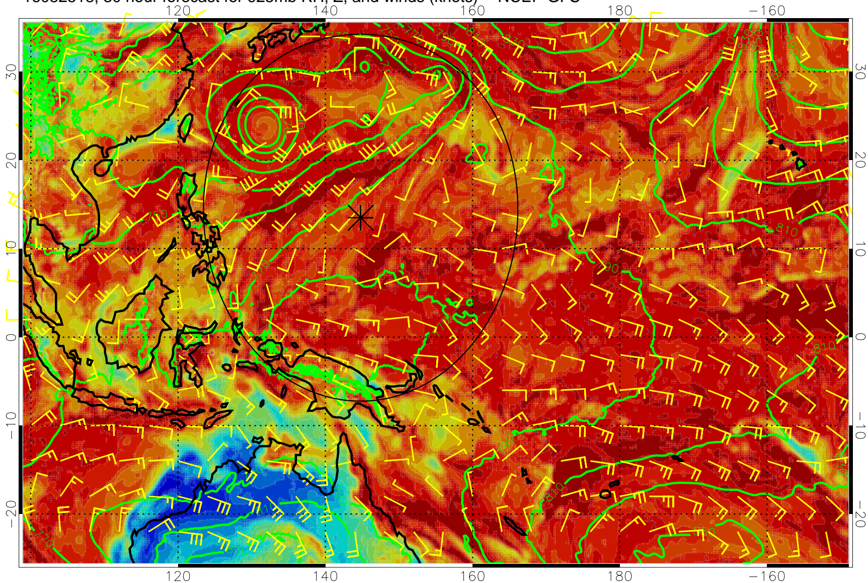
16082518, 30 hour forecast for 925mb RH, Z, and winds (knots) -- NCEP GFS
