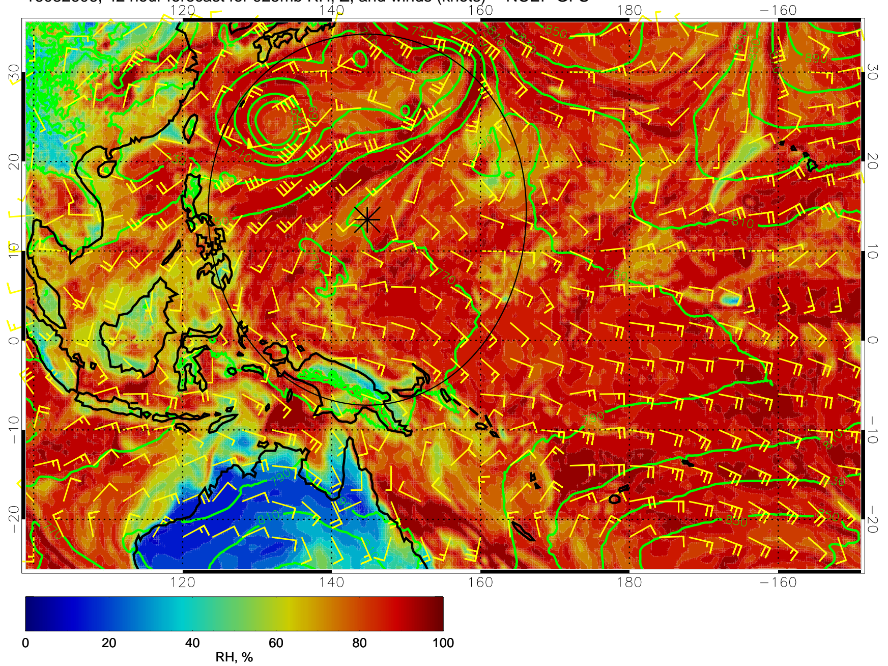
16082606, 42 hour forecast for 925mb RH, Z, and winds (knots) -- NCEP GFS
