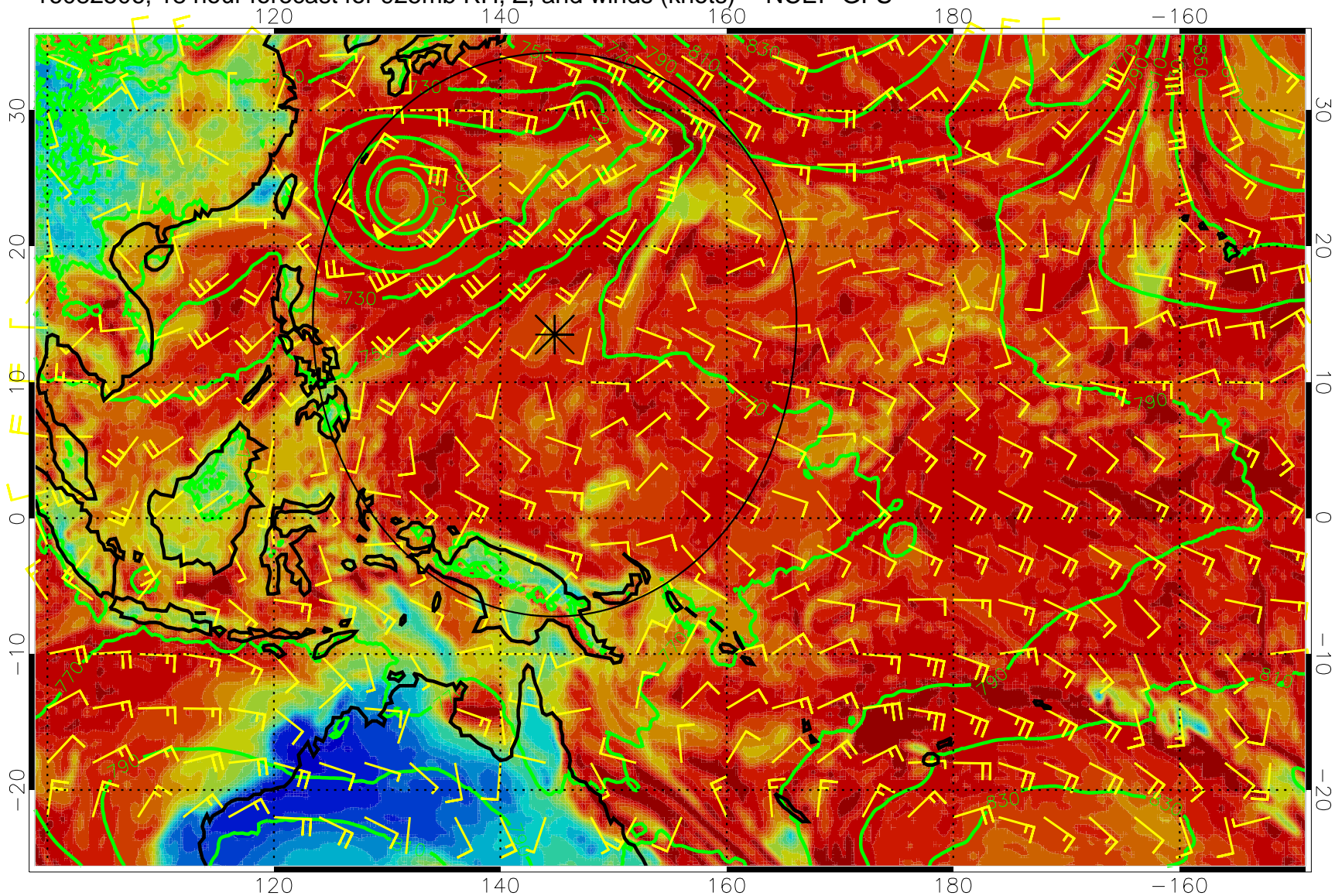
16082506, 18 hour forecast for 925mb RH, Z, and winds (knots) -- NCEP GFS
