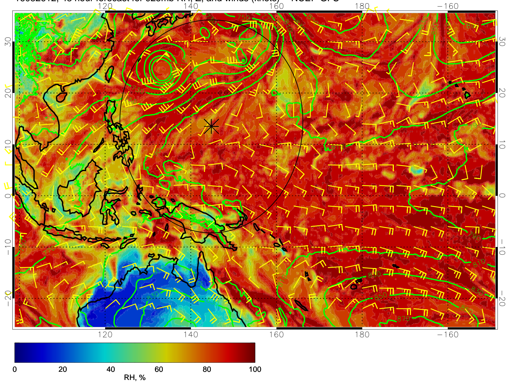
16082612, 48 hour forecast for 925mb RH, Z, and winds (knots) -- NCEP GFS
