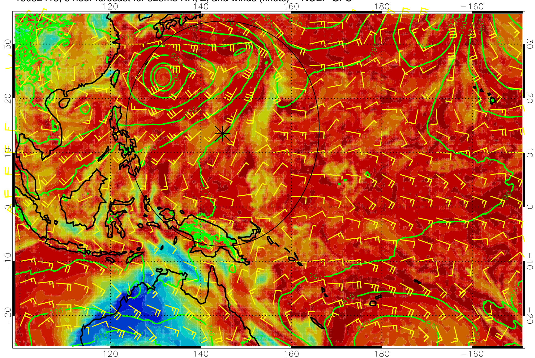
16082418, 6 hour forecast for 925mb RH, Z, and winds (knots) -- NCEP GFS
