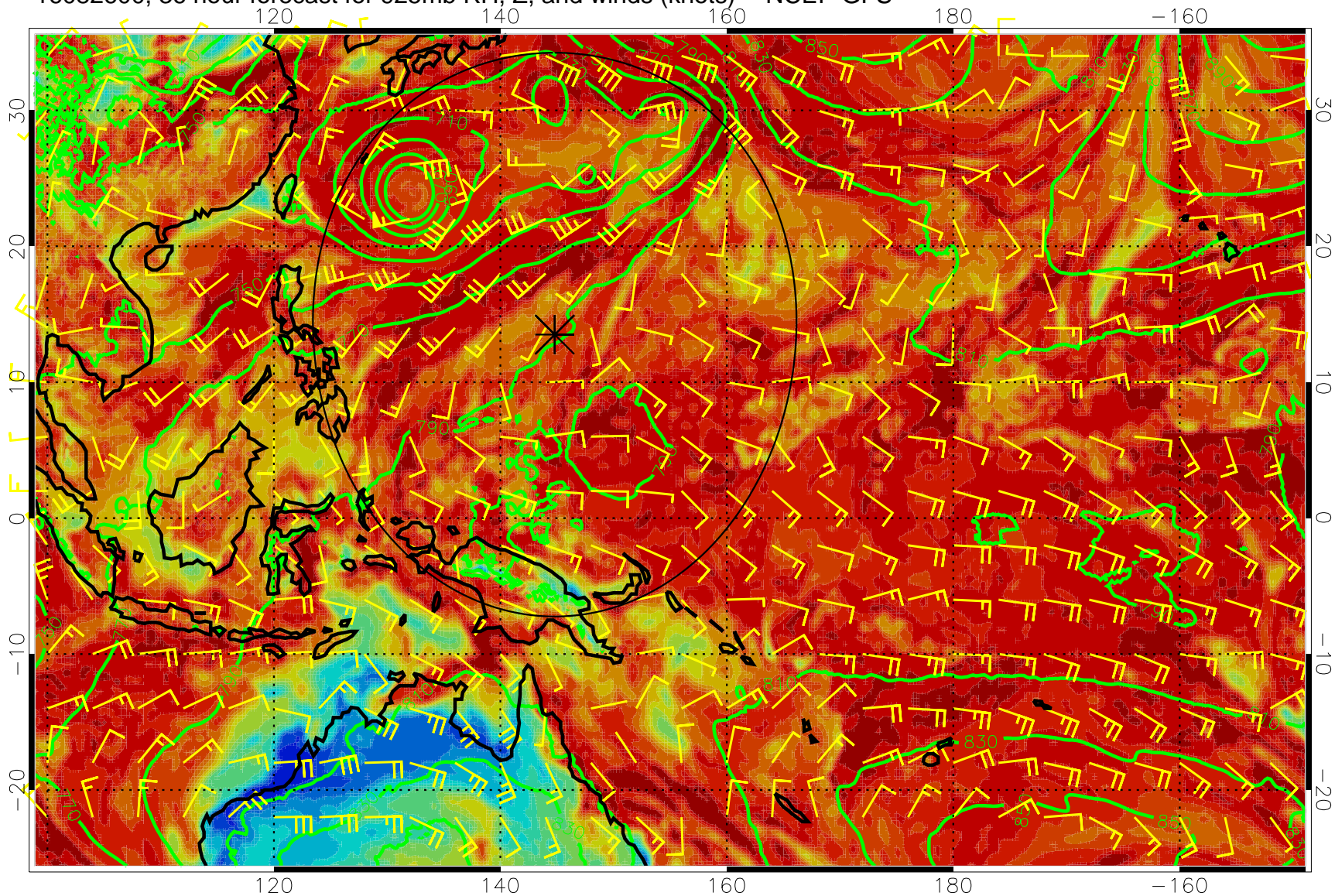
16082600, 36 hour forecast for 925mb RH, Z, and winds (knots) -- NCEP GFS
