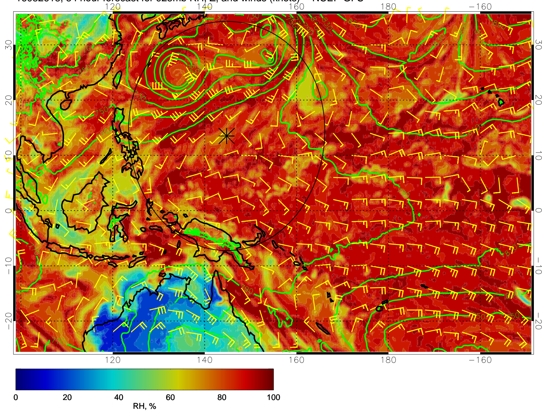
16082618, 54 hour forecast for 925mb RH, Z, and winds (knots) -- NCEP GFS
