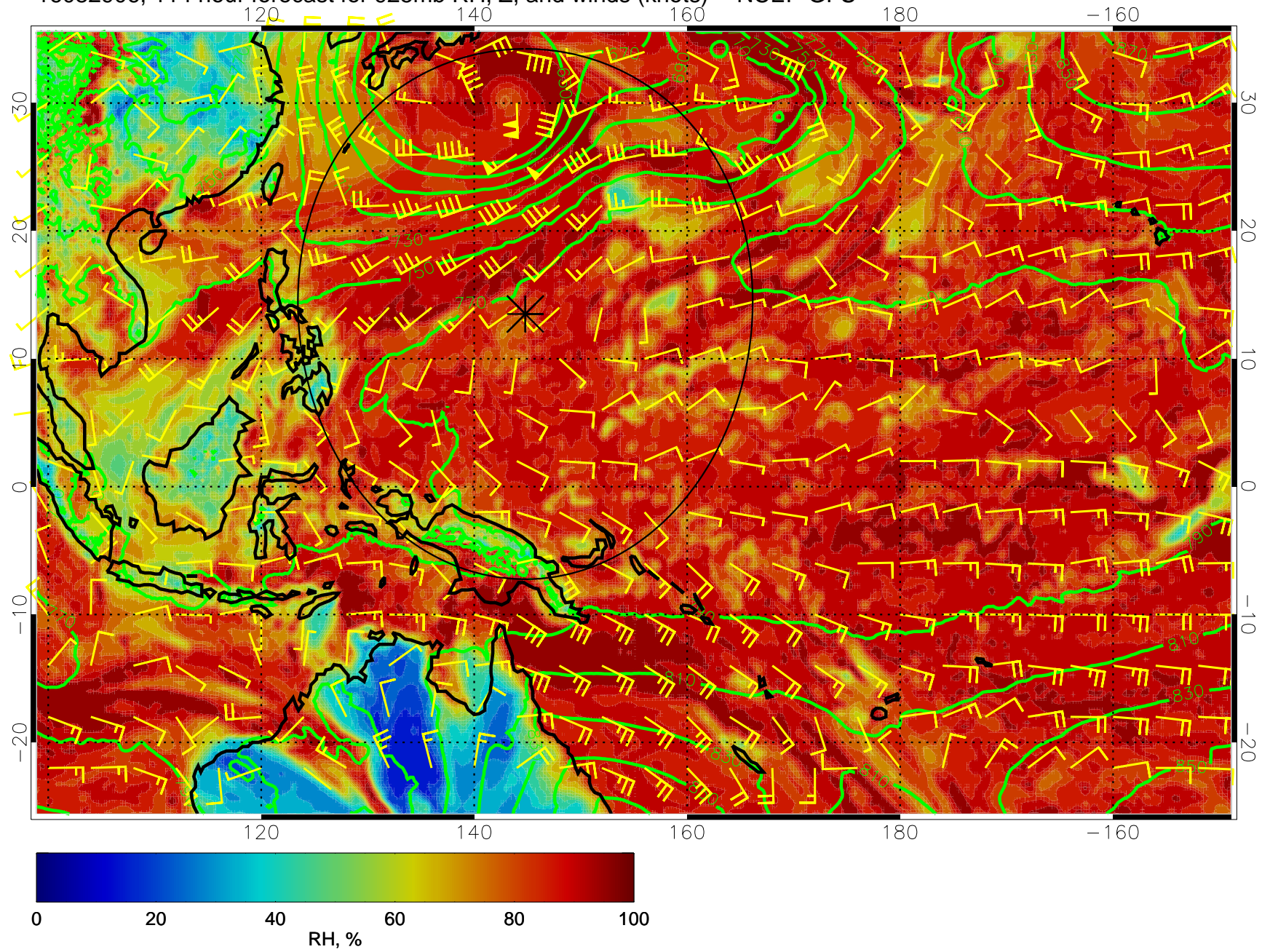
16082906, 114 hour forecast for 925mb RH, Z, and winds (knots) -- NCEP GFS
