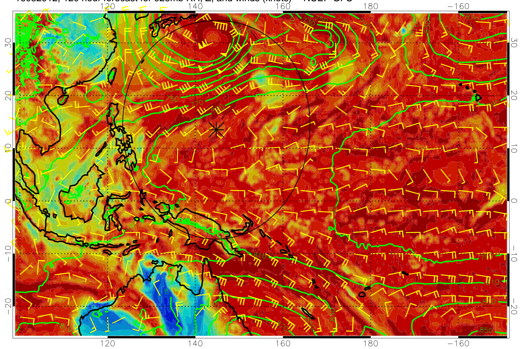
16082912, 120 hour forecast for 925mb RH, Z, and winds (knots) -- NCEP GFS
