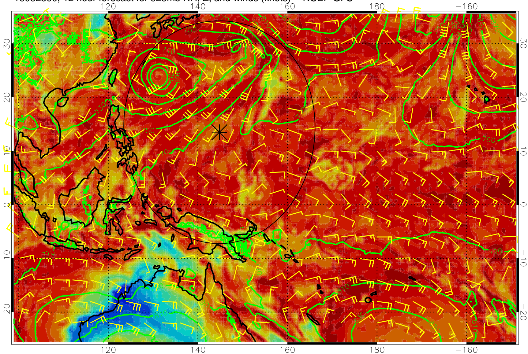
16082500, 12 hour forecast for 925mb RH, Z, and winds (knots) -- NCEP GFS
