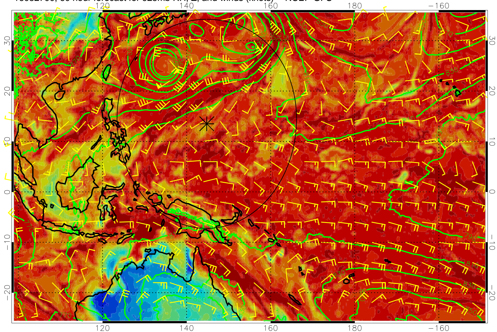
16082700, 60 hour forecast for 925mb RH, Z, and winds (knots) -- NCEP GFS
