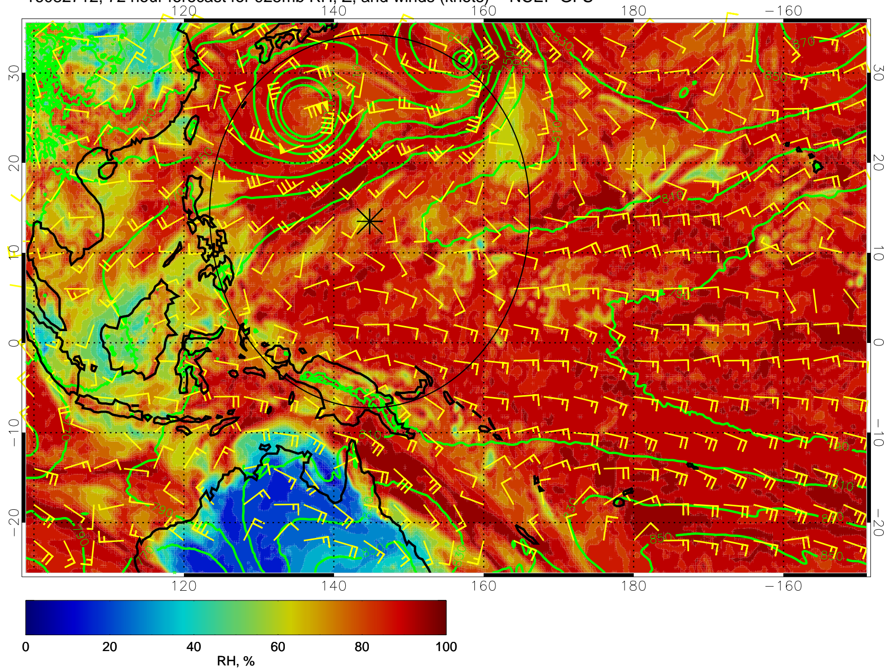
16082712, 72 hour forecast for 925mb RH, Z, and winds (knots) -- NCEP GFS
