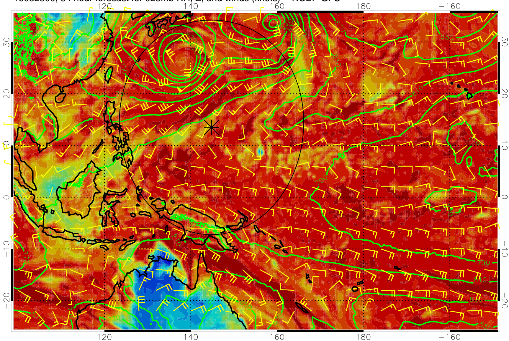
16082800, 84 hour forecast for 925mb RH, Z, and winds (knots) -- NCEP GFS
