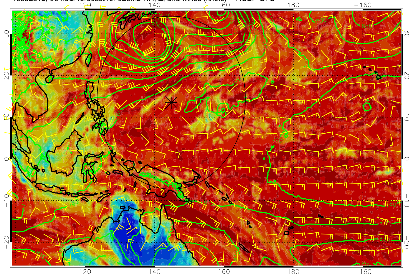
16082812, 96 hour forecast for 925mb RH, Z, and winds (knots) -- NCEP GFS
