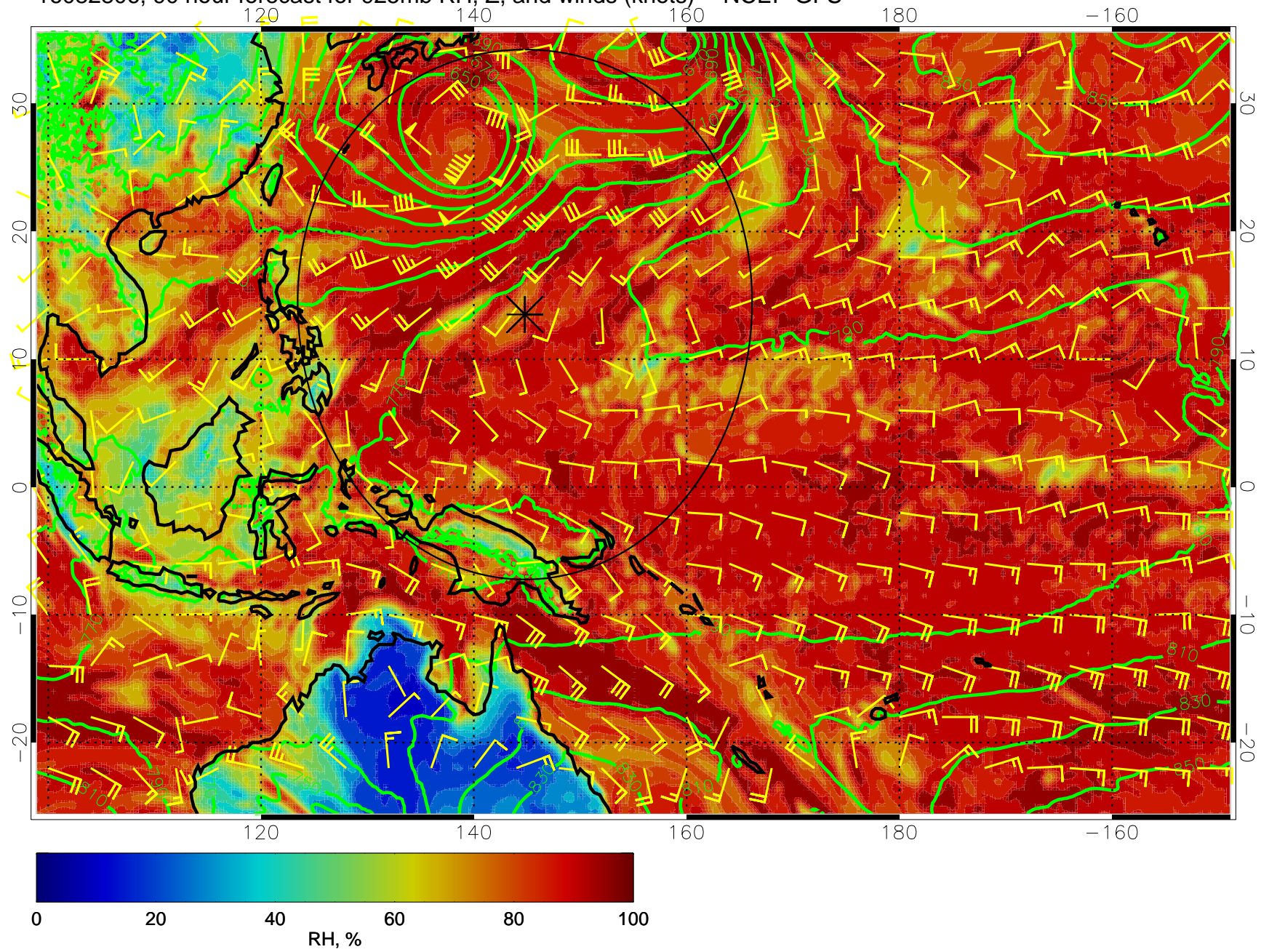
16082806, 90 hour forecast for 925mb RH, Z, and winds (knots) -- NCEP GFS
