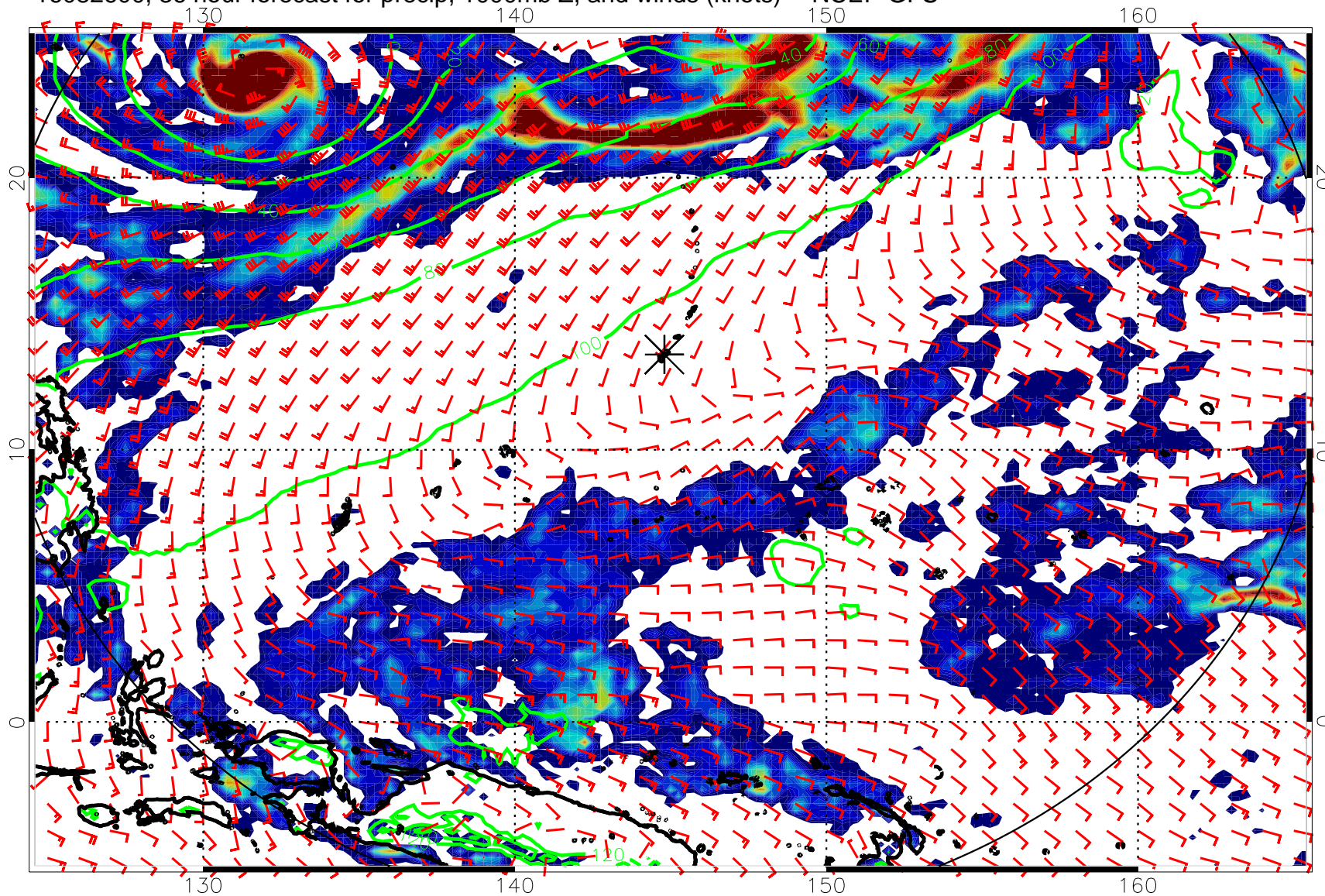
16082600, 36 hour forecast for precip, 1000mb Z, and winds (knots) -- NCEP GFS
