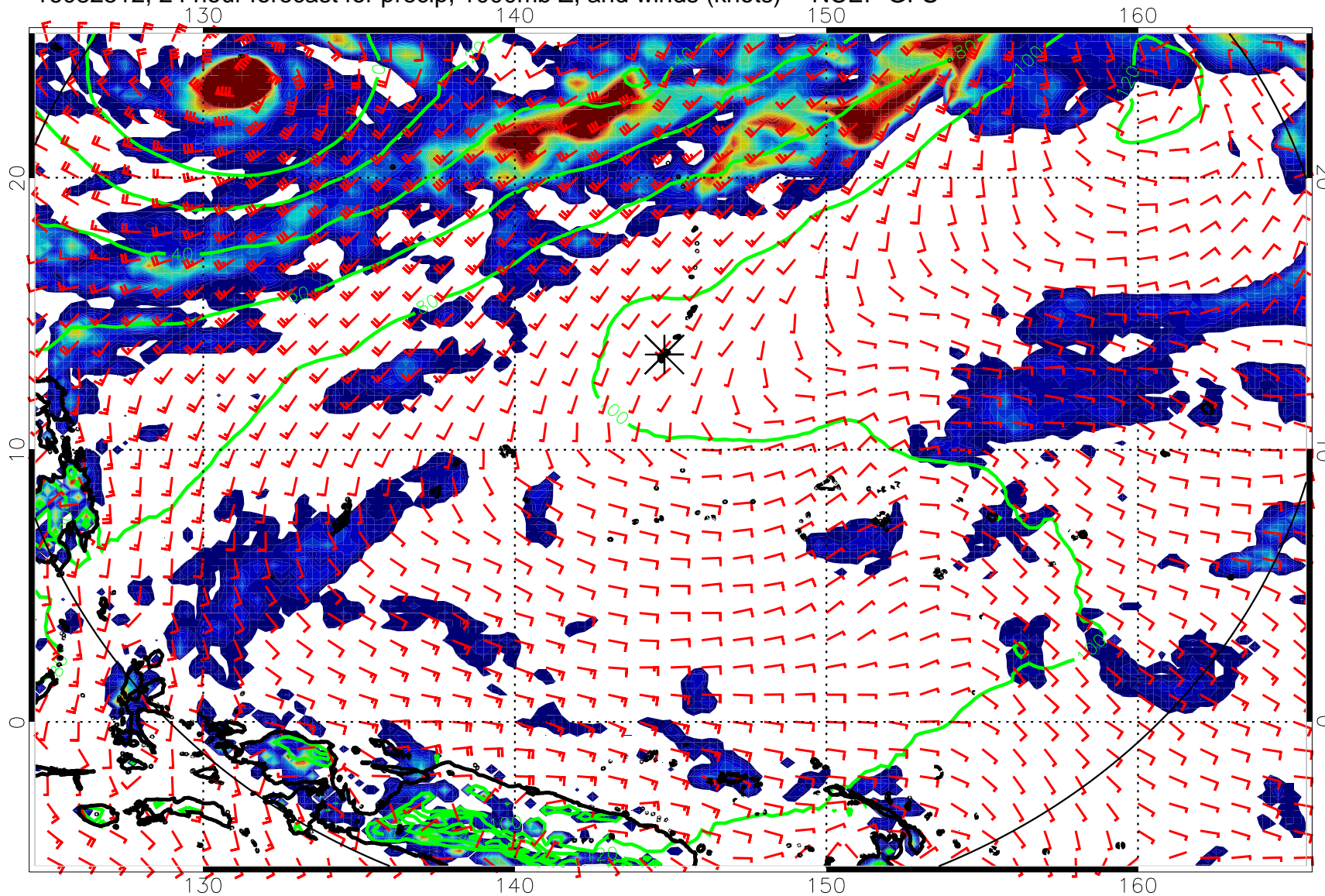
16082512, 24 hour forecast for precip, 1000mb Z, and winds (knots) -- NCEP GFS
