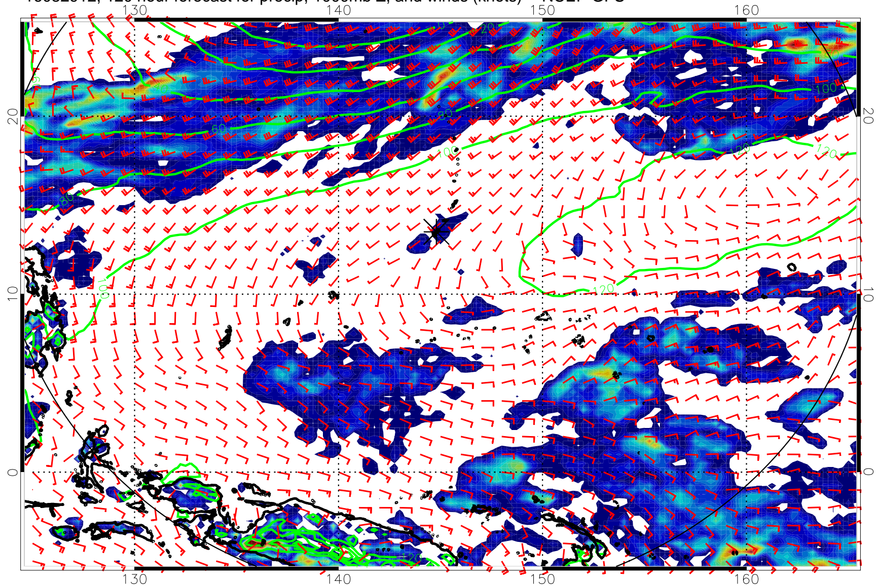
16082912, 120 hour forecast for precip, 1000mb Z, and winds (knots) -- NCEP GFS
