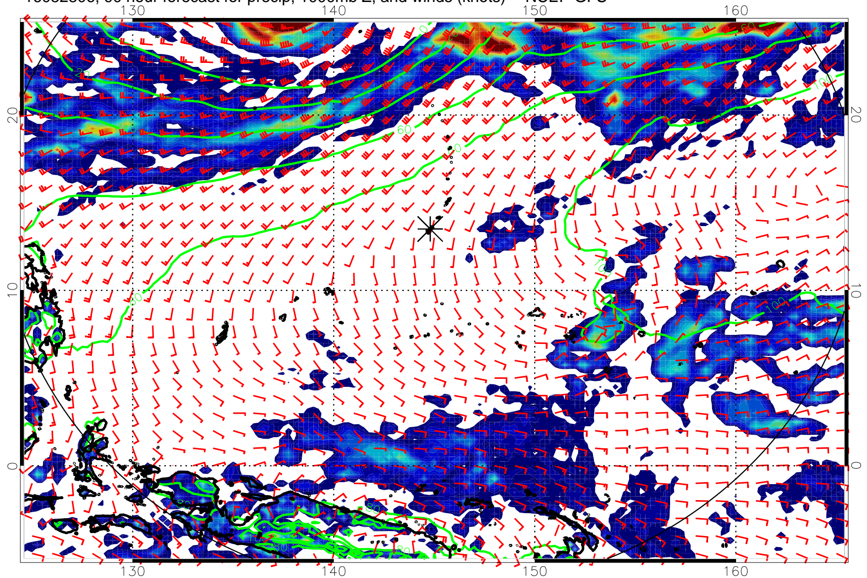
16082806, 90 hour forecast for precip, 1000mb Z, and winds (knots) -- NCEP GFS
