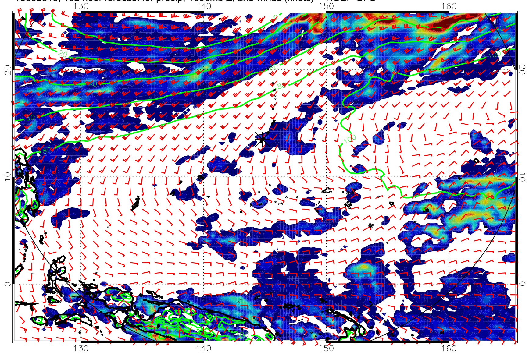
16082818, 102 hour forecast for precip, 1000mb Z, and winds (knots) -- NCEP GFS
