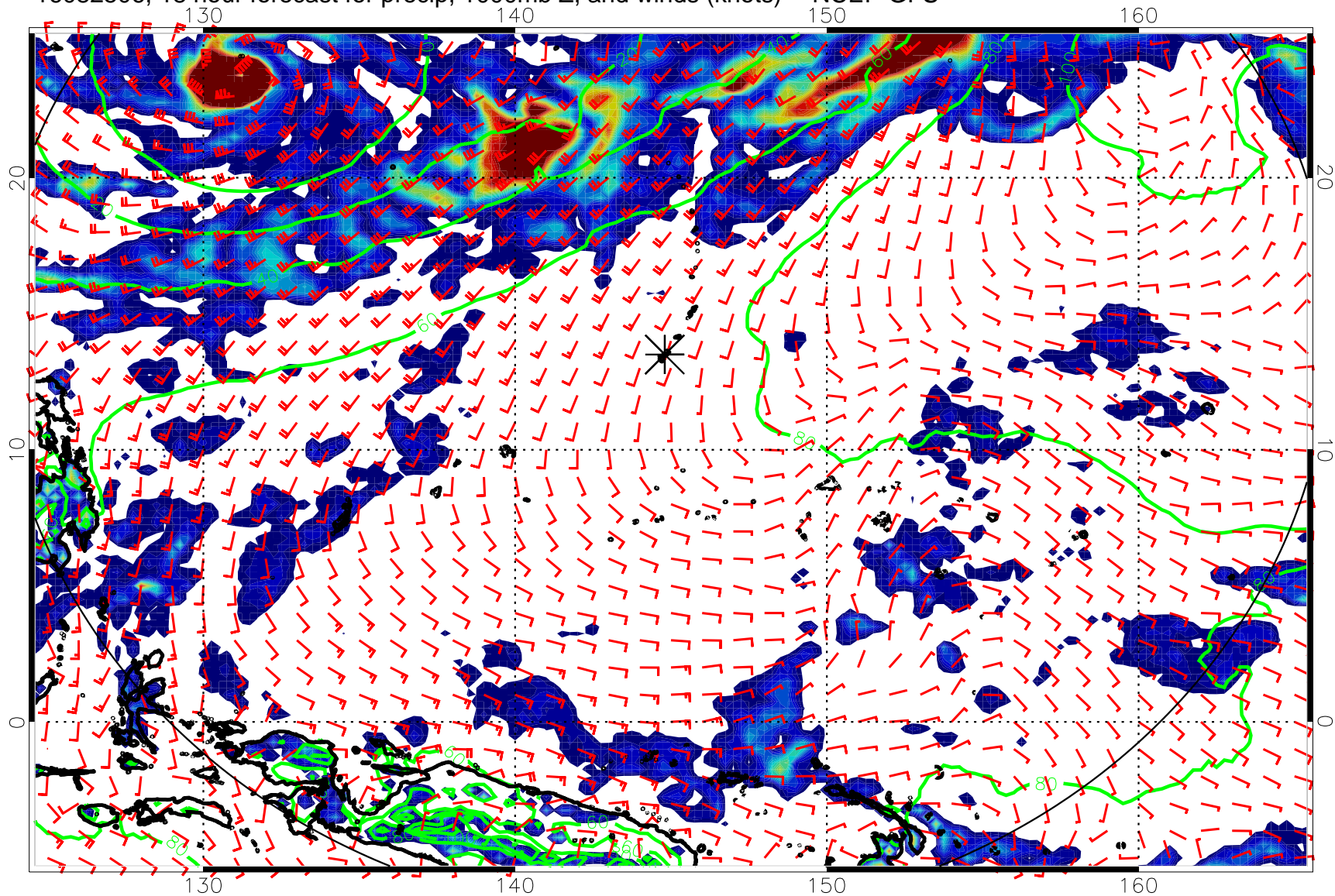
16082506, 18 hour forecast for precip, 1000mb Z, and winds (knots) -- NCEP GFS
