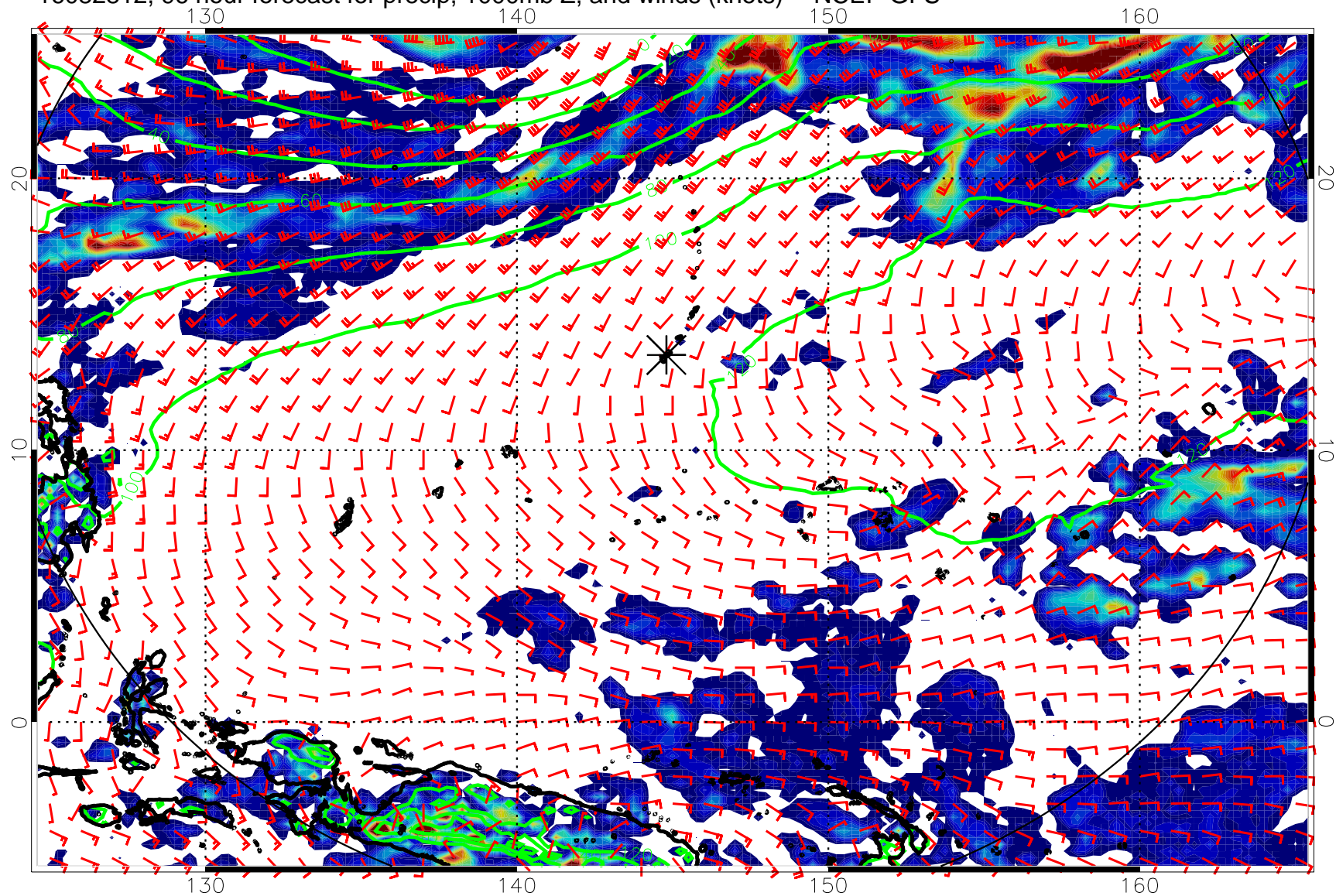
16082812, 96 hour forecast for precip, 1000mb Z, and winds (knots) -- NCEP GFS
