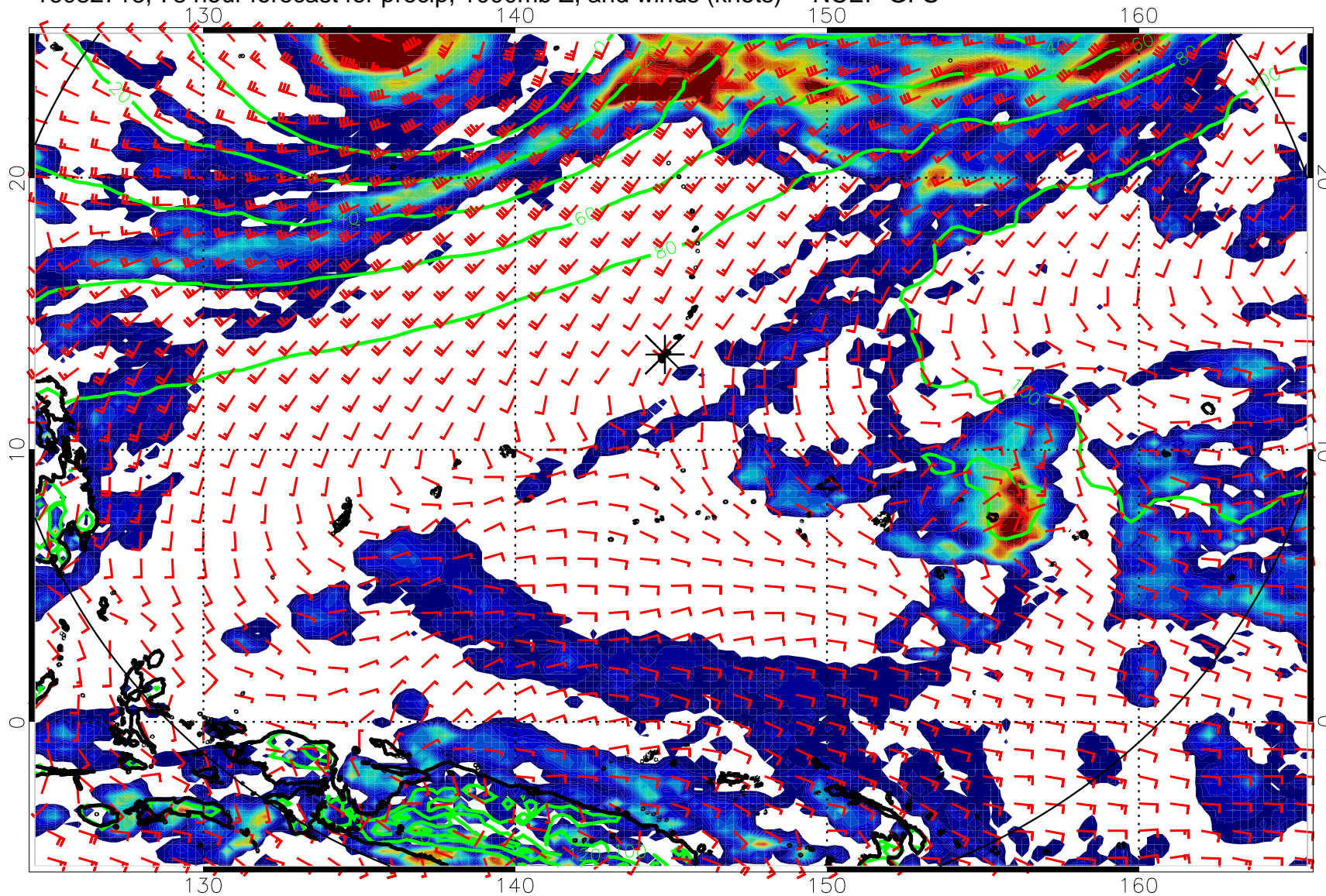
16082718, 78 hour forecast for precip, 1000mb Z, and winds (knots) -- NCEP GFS
