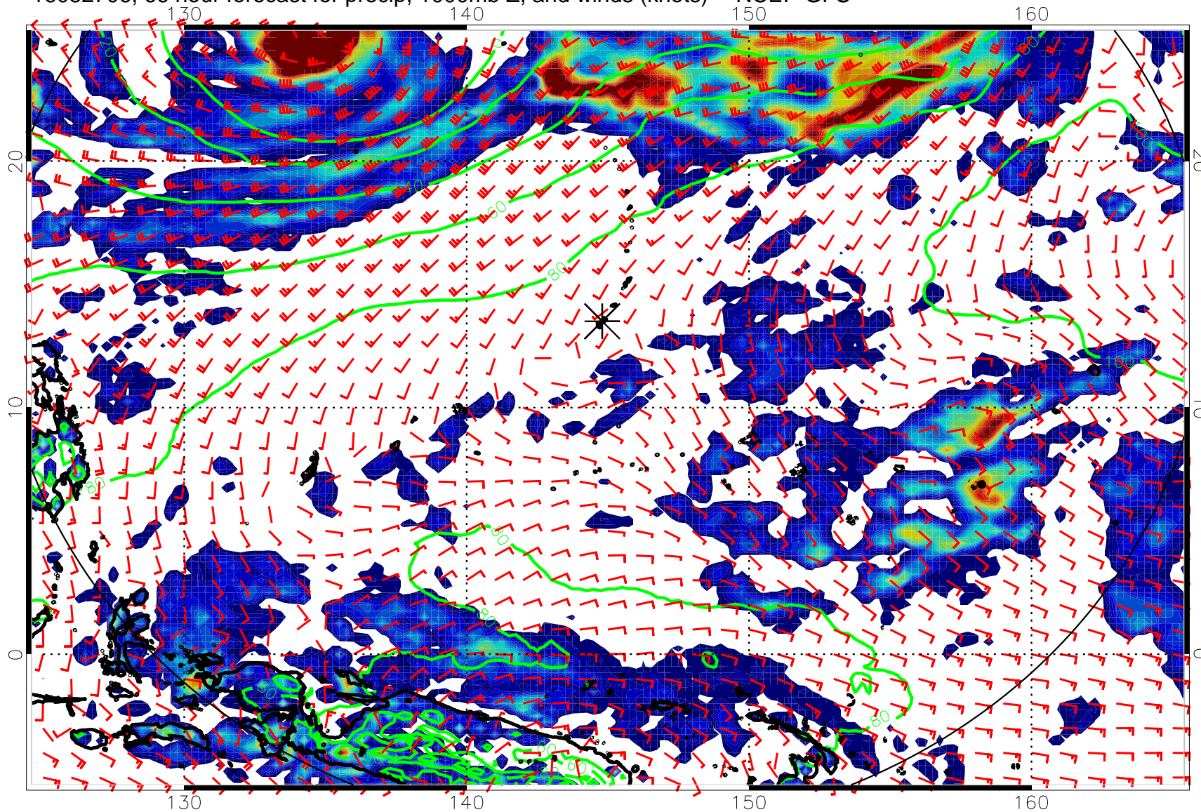
16082706, 66 hour forecast for precip, 1000mb Z, and winds (knots) -- NCEP GFS
