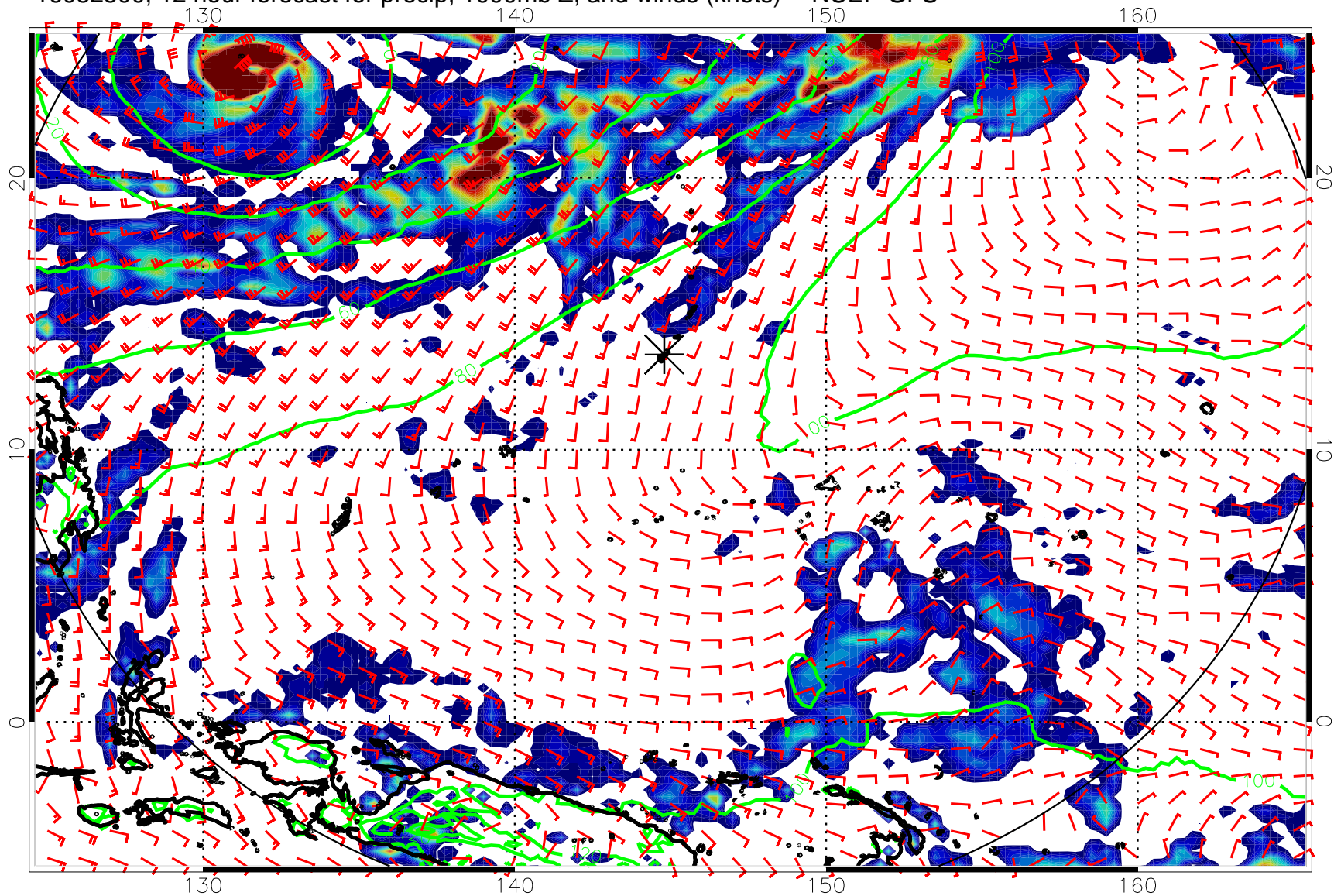
16082500, 12 hour forecast for precip, 1000mb Z, and winds (knots) -- NCEP GFS
