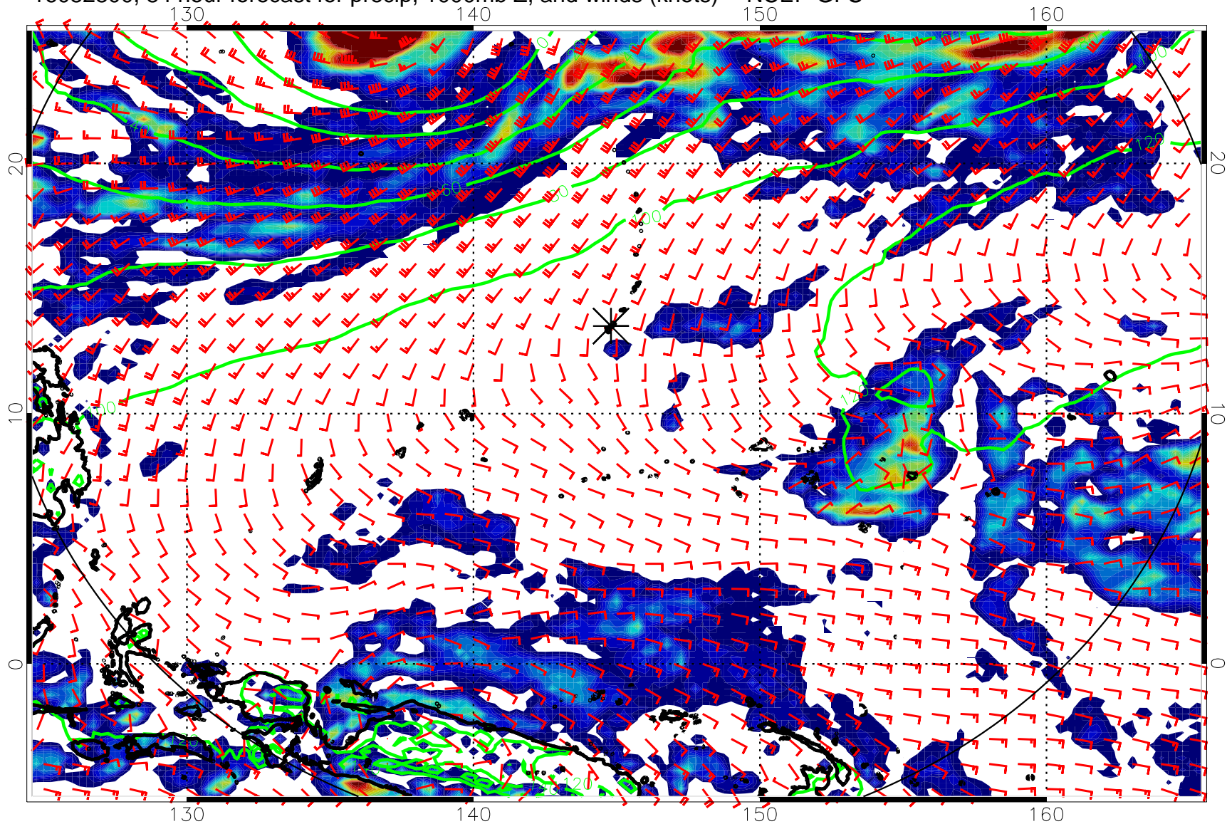
16082800, 84 hour forecast for precip, 1000mb Z, and winds (knots) -- NCEP GFS
