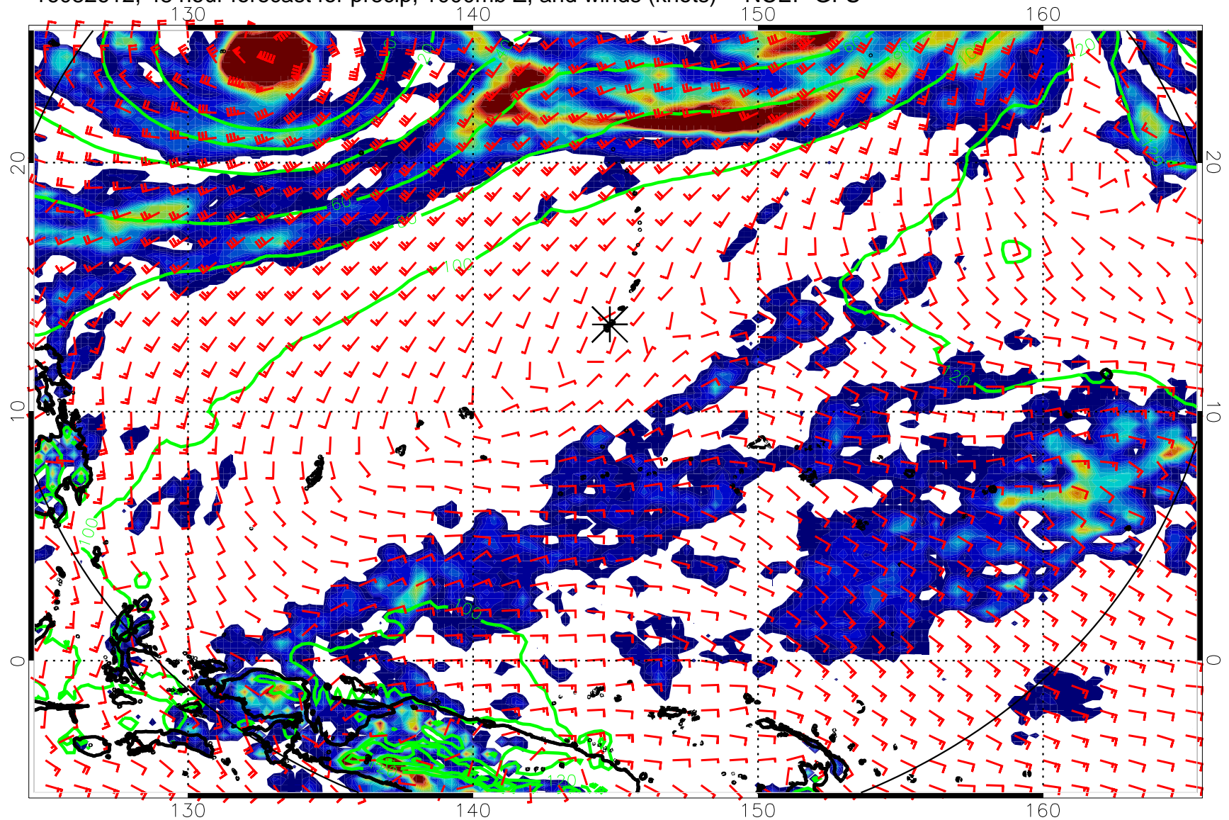
16082612, 48 hour forecast for precip, 1000mb Z, and winds (knots) -- NCEP GFS
