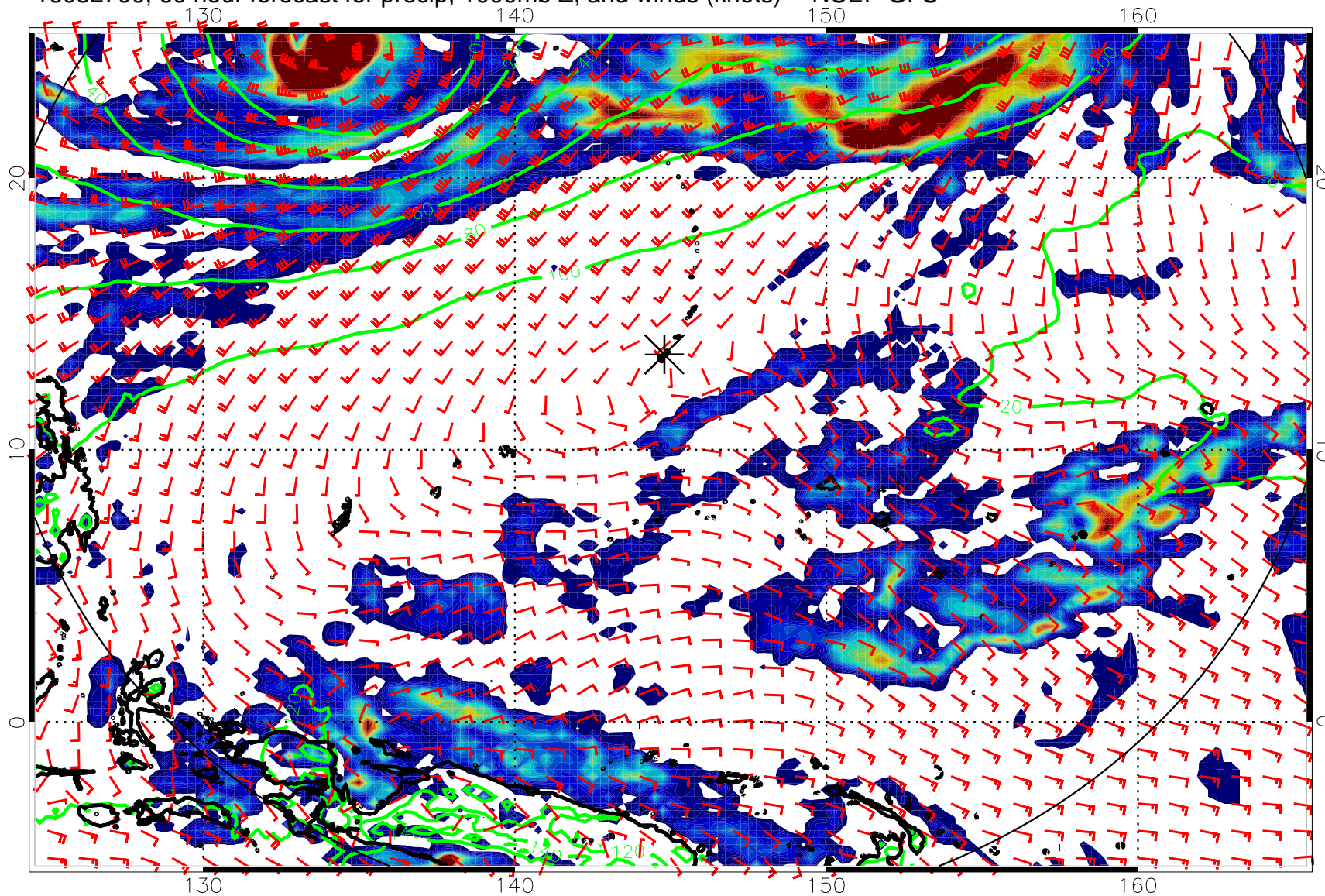
16082700, 60 hour forecast for precip, 1000mb Z, and winds (knots) -- NCEP GFS
