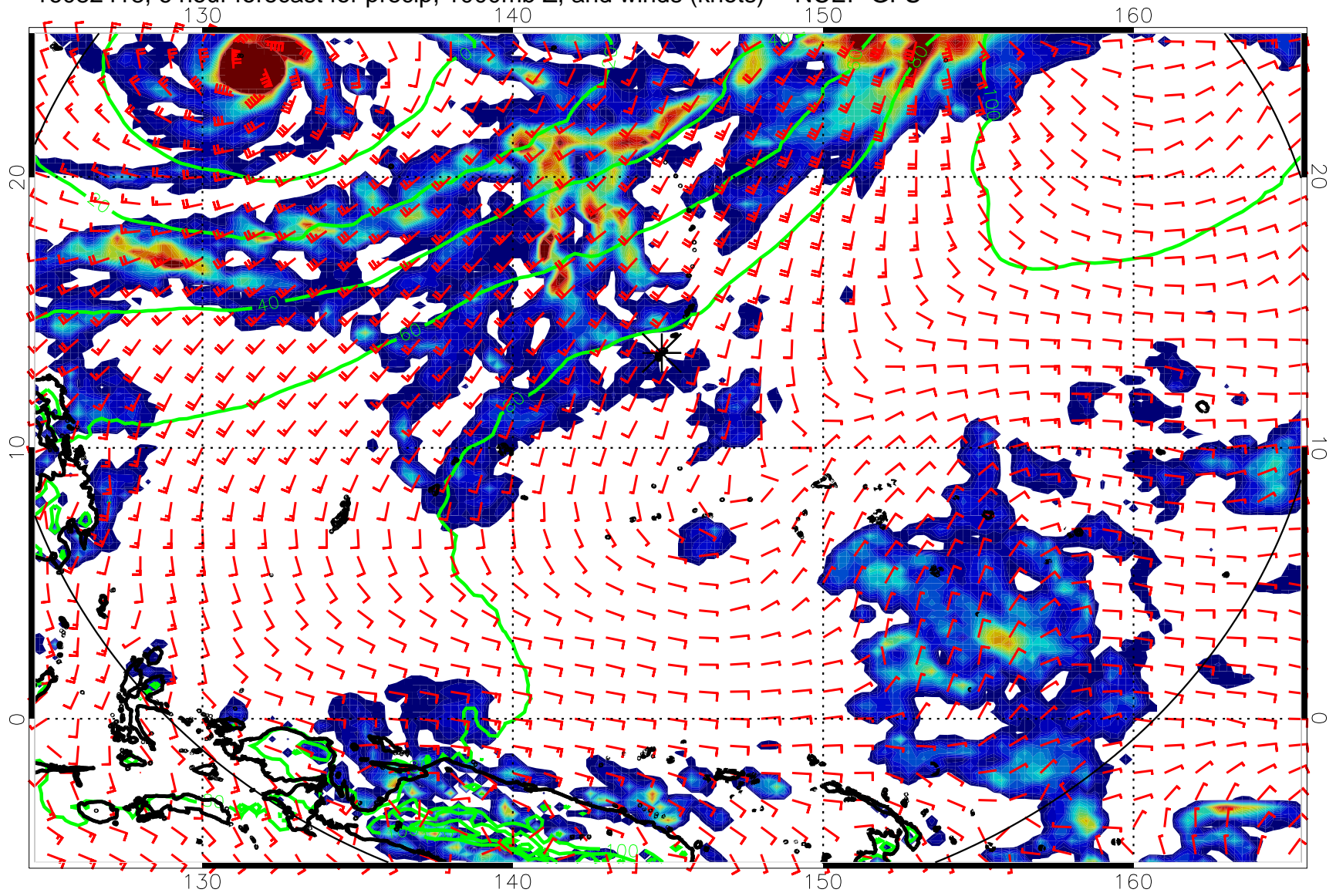
16082418, 6 hour forecast for precip, 1000mb Z, and winds (knots) -- NCEP GFS
