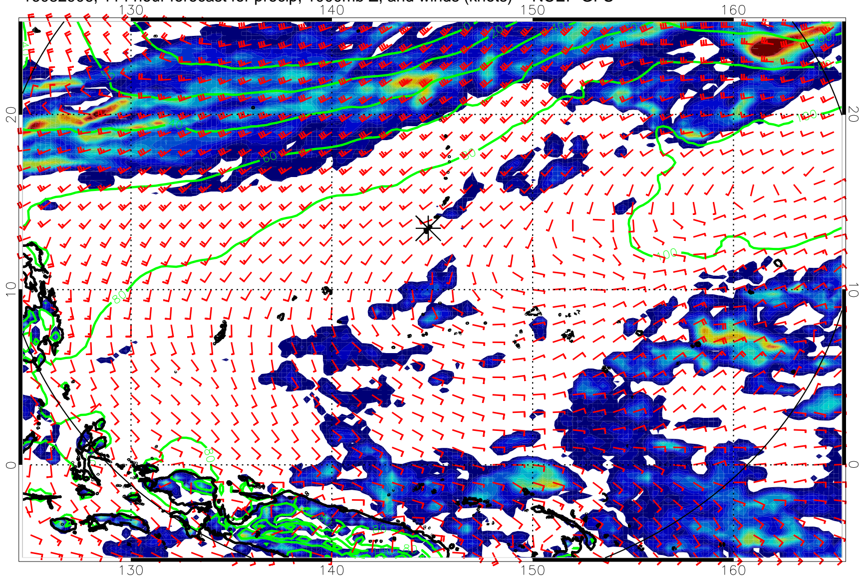
16082906, 114 hour forecast for precip, 1000mb Z, and winds (knots) -- NCEP GFS
