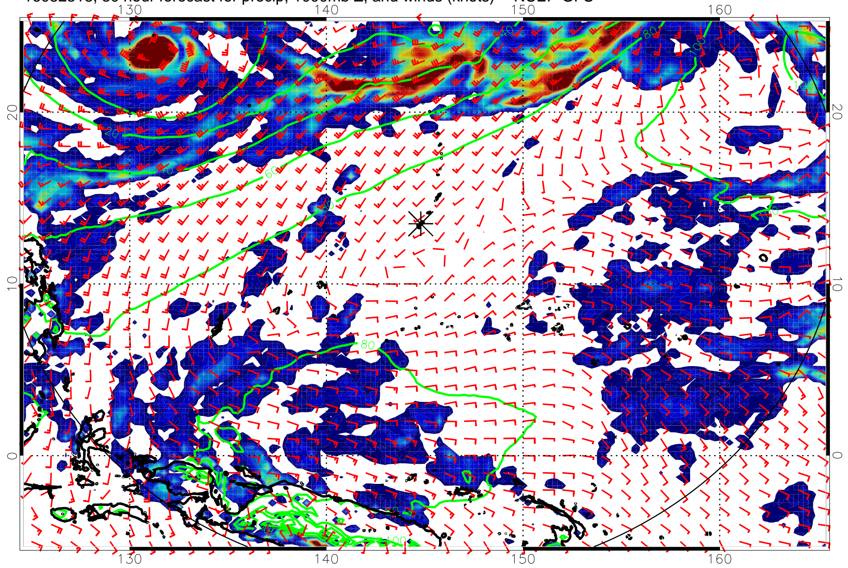
16082518, 30 hour forecast for precip, 1000mb Z, and winds (knots) -- NCEP GFS
