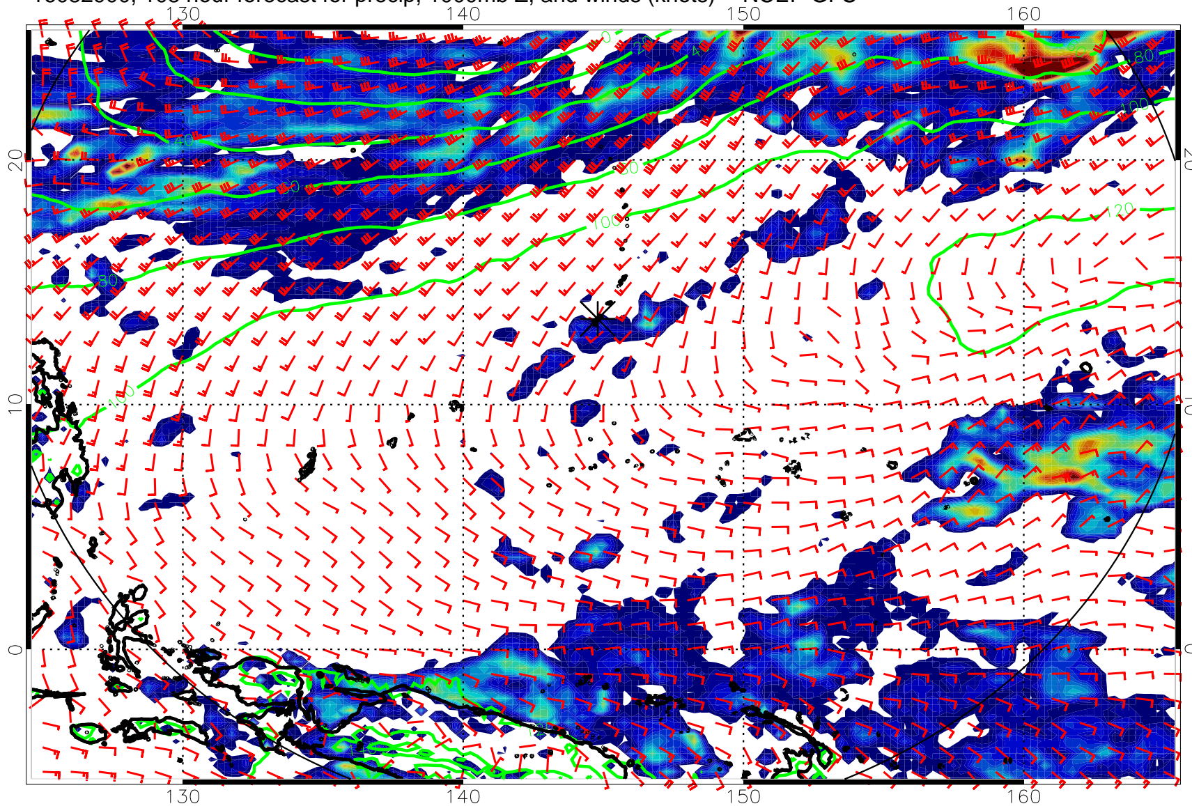
16082900, 108 hour forecast for precip, 1000mb Z, and winds (knots) -- NCEP GFS
