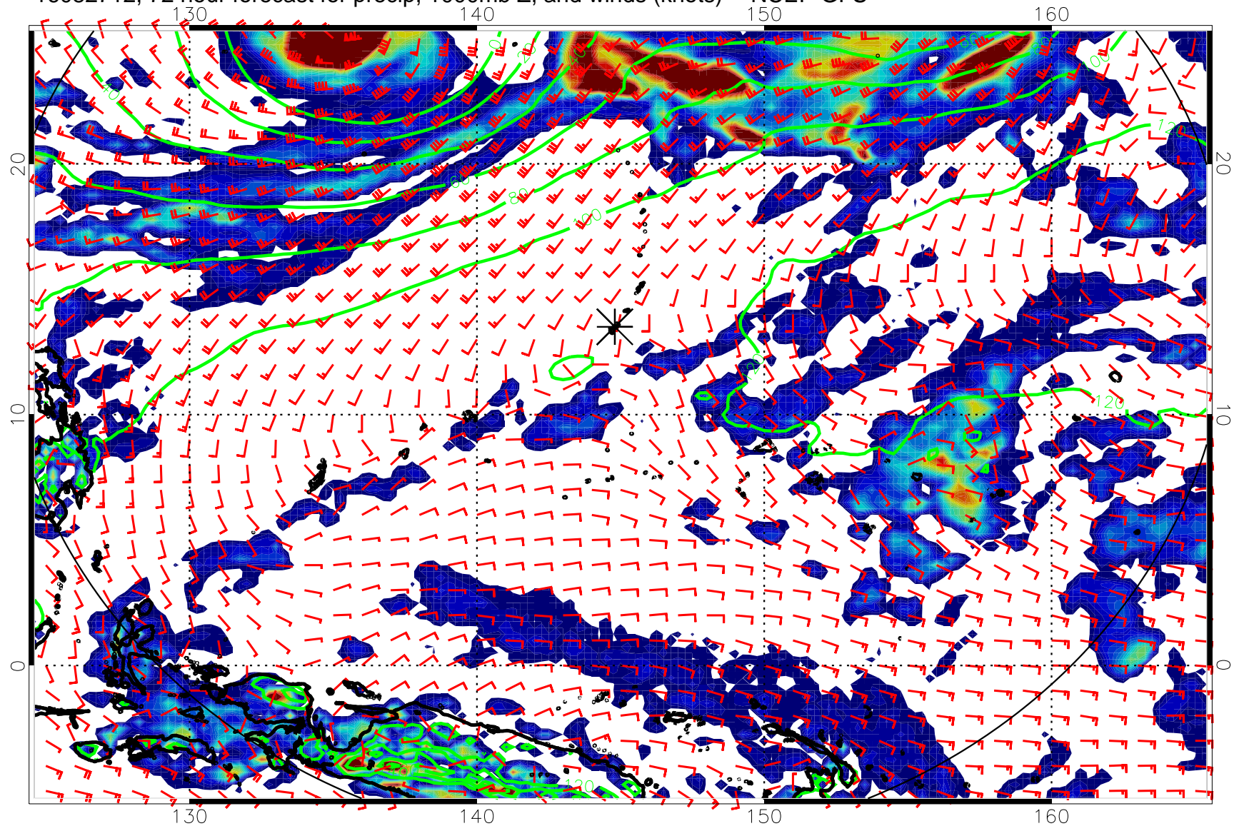
16082712, 72 hour forecast for precip, 1000mb Z, and winds (knots) -- NCEP GFS
