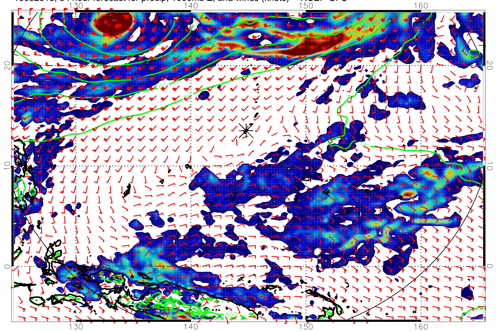
16082618, 54 hour forecast for precip, 1000mb Z, and winds (knots) -- NCEP GFS
