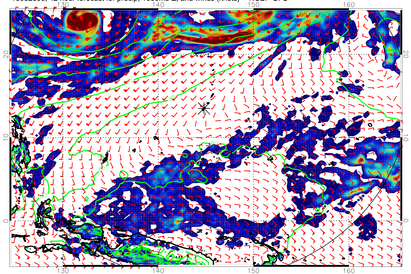
16082606, 42 hour forecast for precip, 1000mb Z, and winds (knots) -- NCEP GFS
