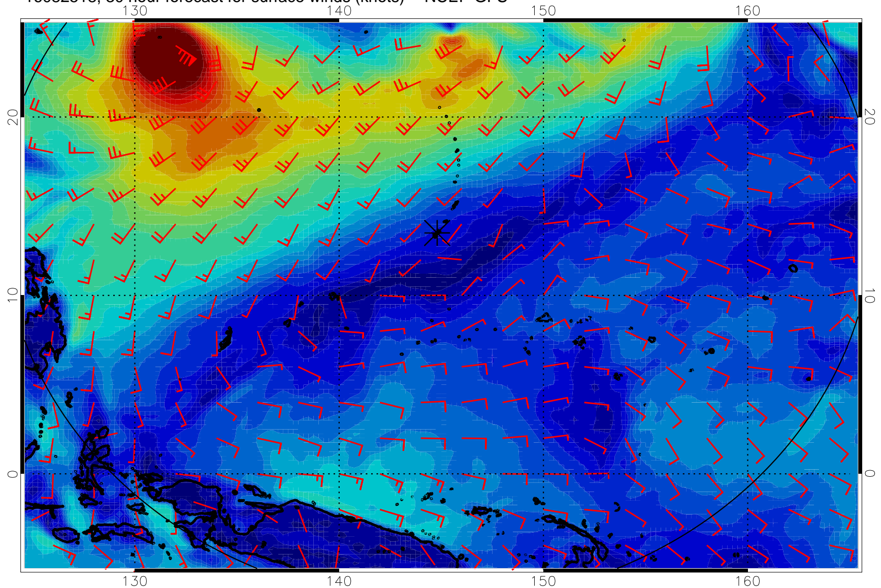
16082518, 30 hour forecast for surface winds (knots) -- NCEP GFS
