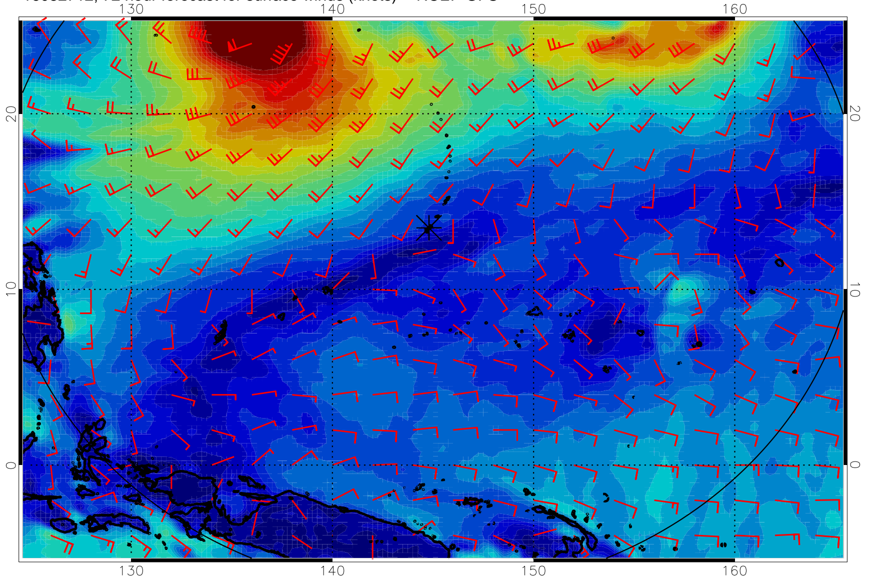
16082712, 72 hour forecast for surface winds (knots) -- NCEP GFS
