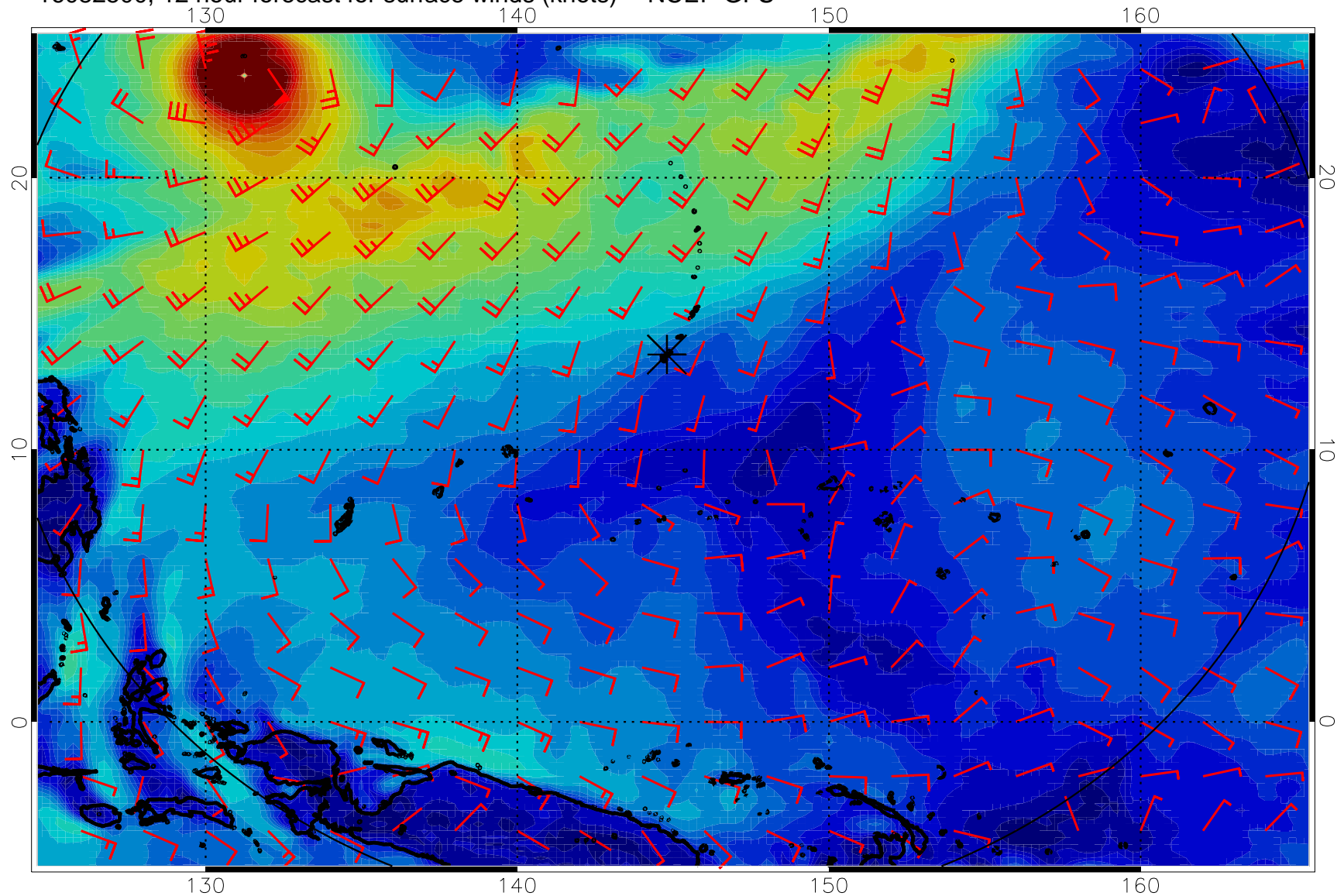
16082500, 12 hour forecast for surface winds (knots) -- NCEP GFS
