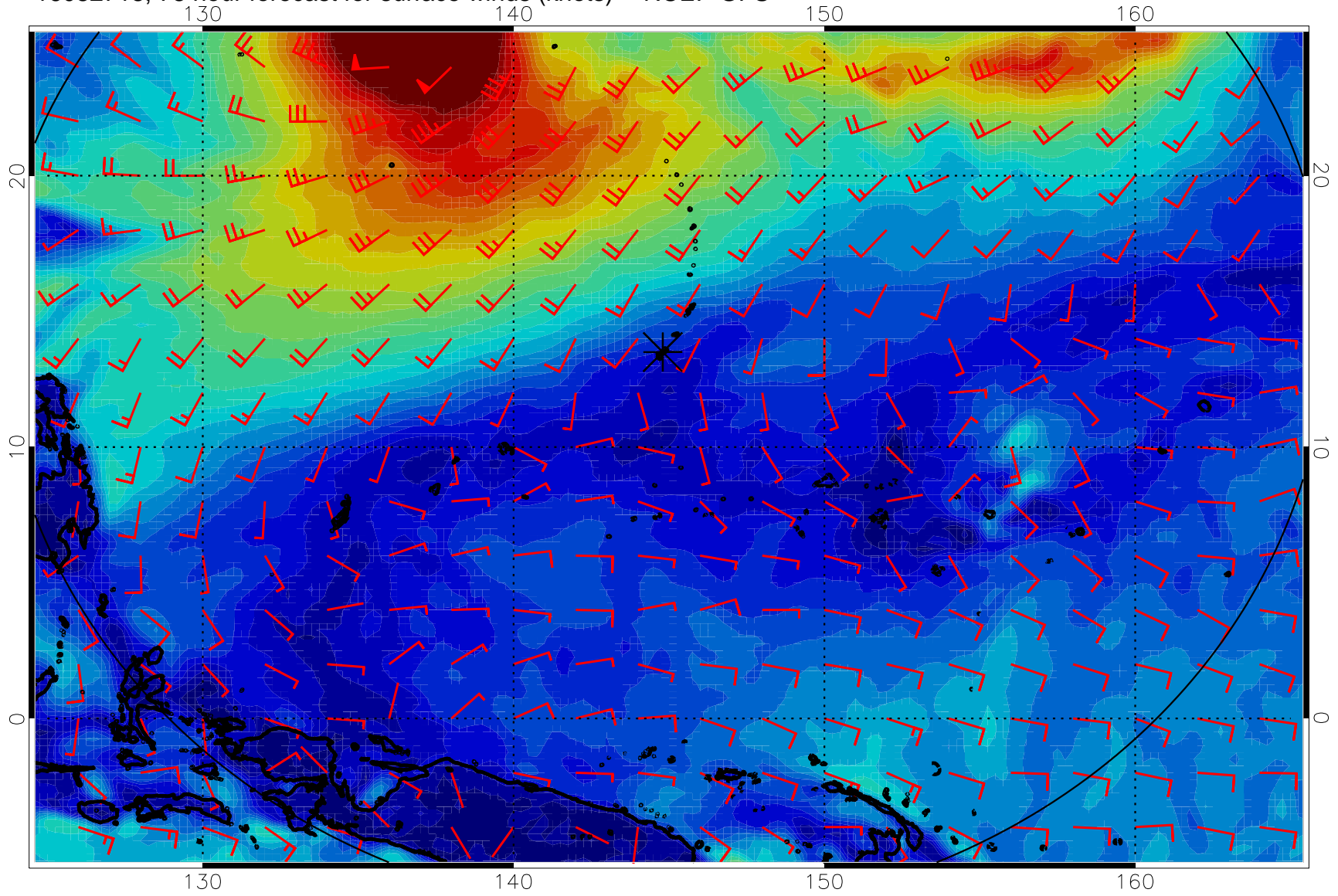
16082718, 78 hour forecast for surface winds (knots) -- NCEP GFS
