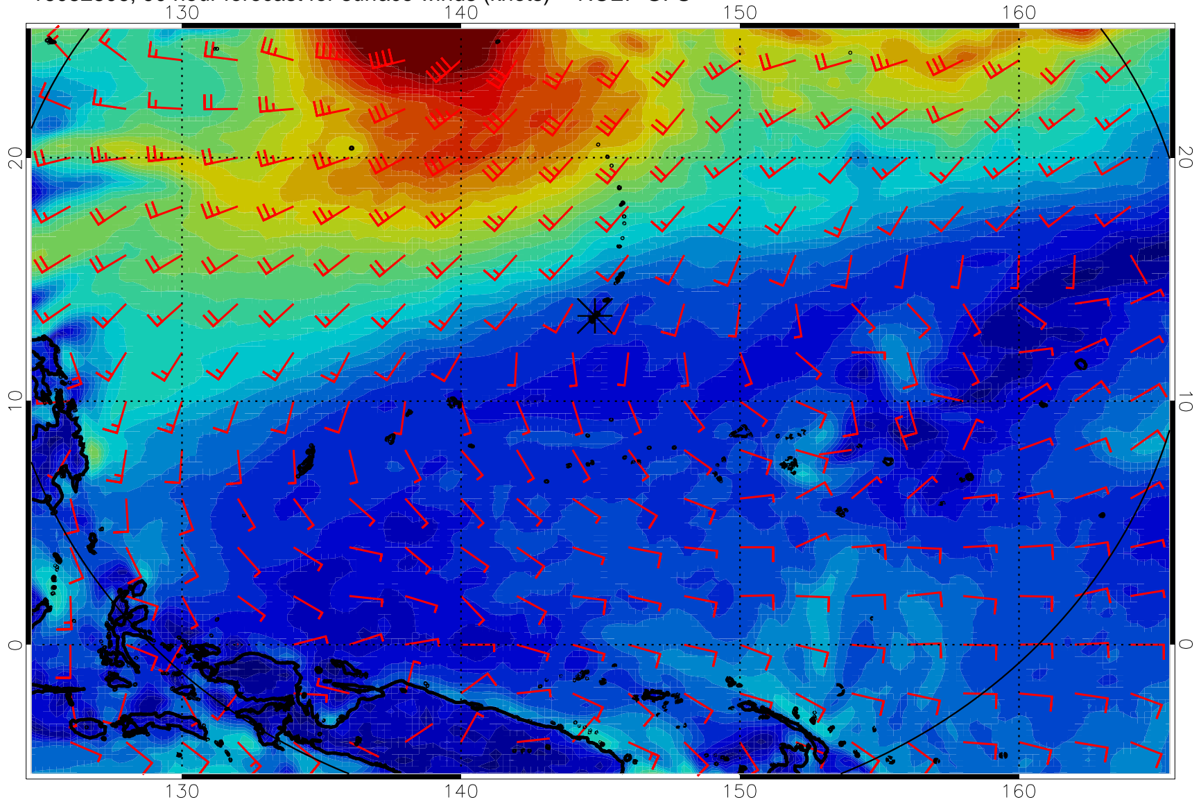
16082806, 90 hour forecast for surface winds (knots) -- NCEP GFS
