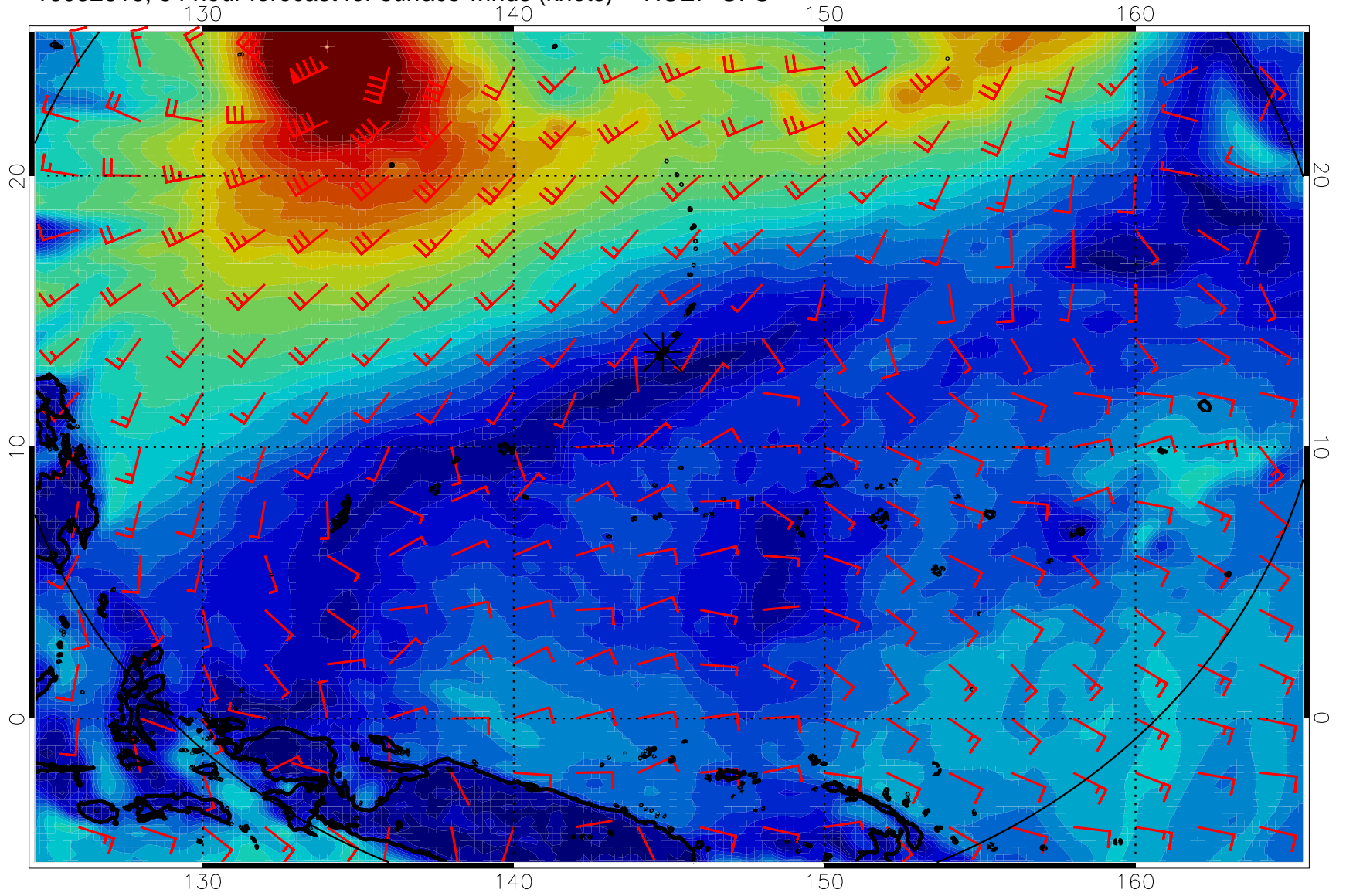
16082618, 54 hour forecast for surface winds (knots) -- NCEP GFS
