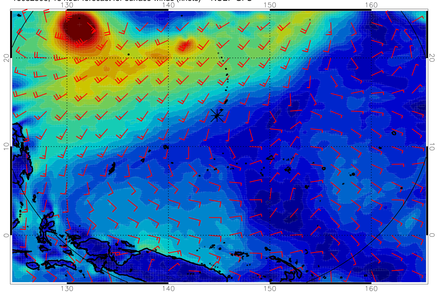
16082506, 18 hour forecast for surface winds (knots) -- NCEP GFS
