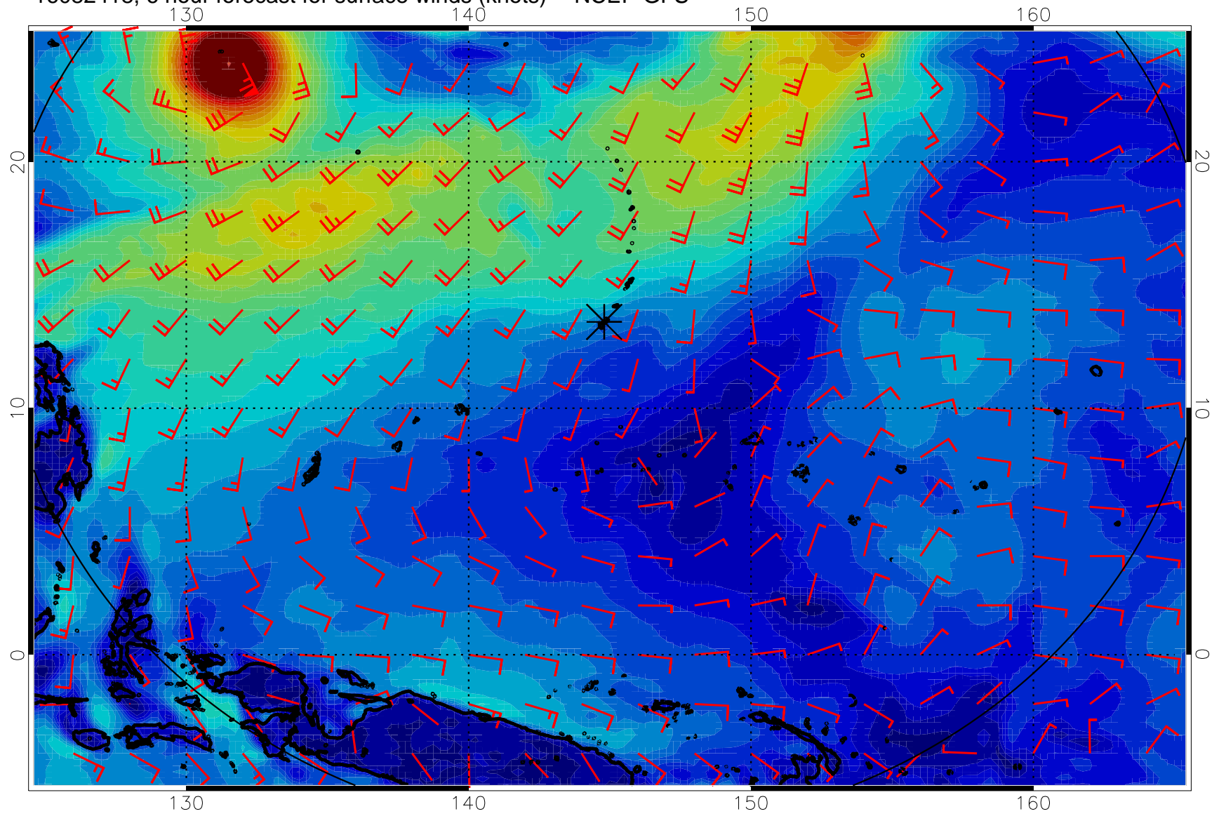
16082418, 6 hour forecast for surface winds (knots) -- NCEP GFS
