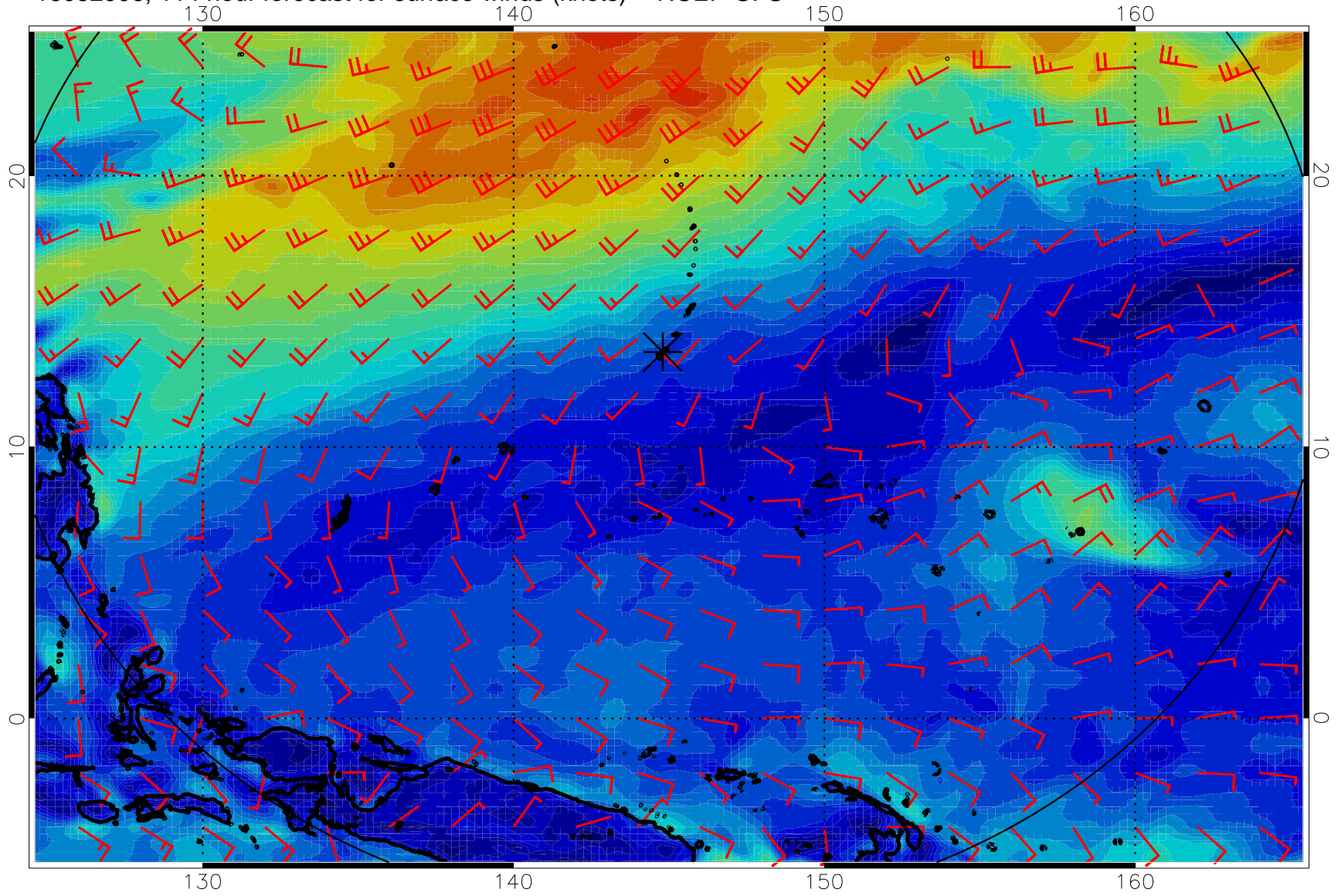
16082906, 114 hour forecast for surface winds (knots) -- NCEP GFS
