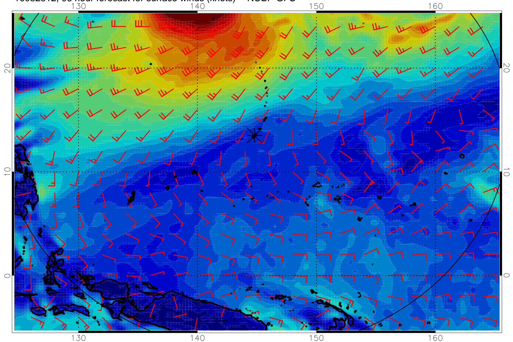
16082812, 96 hour forecast for surface winds (knots) -- NCEP GFS
