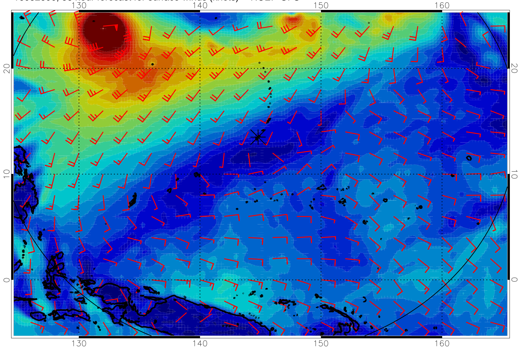
16082600, 36 hour forecast for surface winds (knots) -- NCEP GFS
