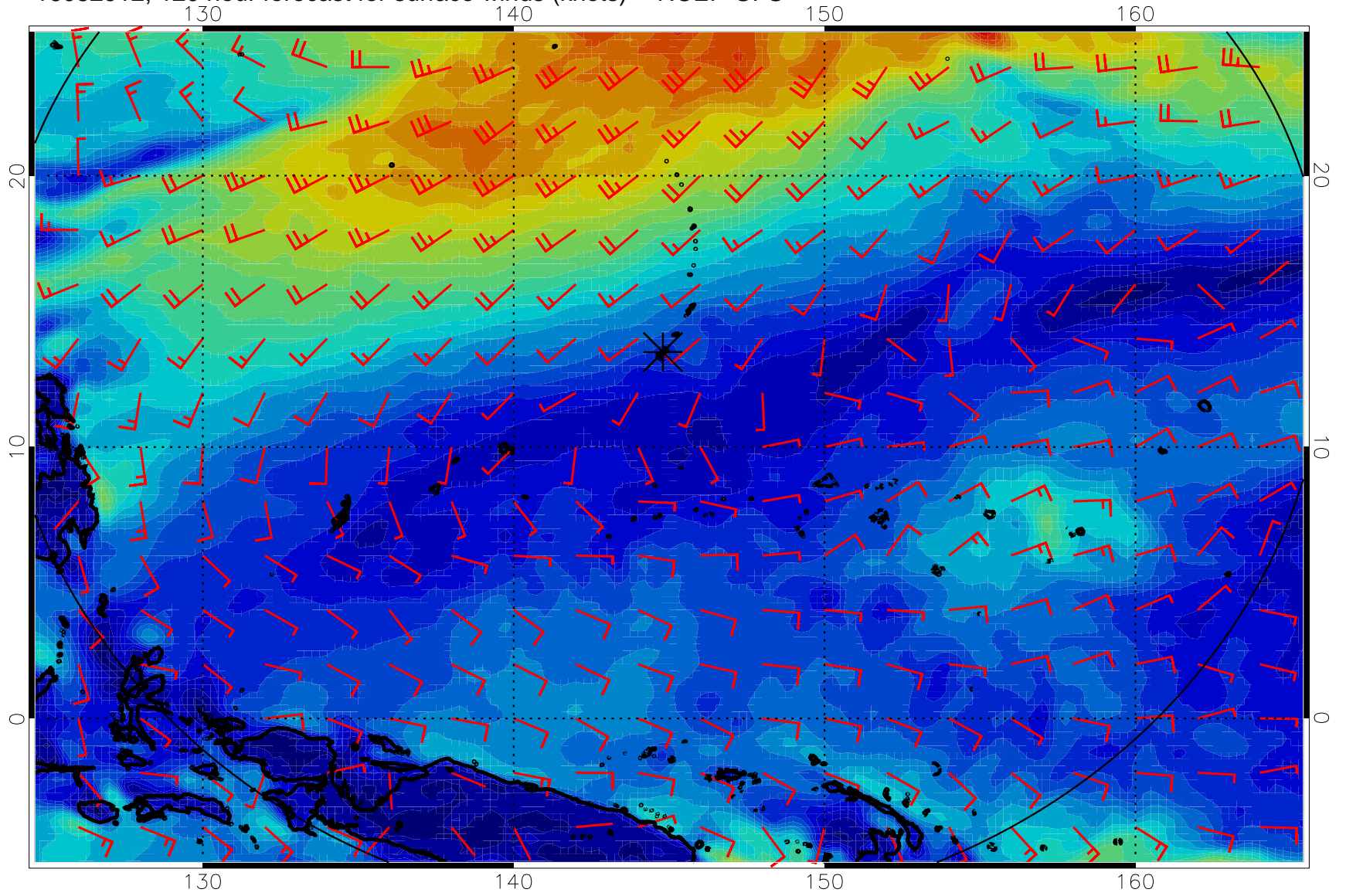
16082912, 120 hour forecast for surface winds (knots) -- NCEP GFS
