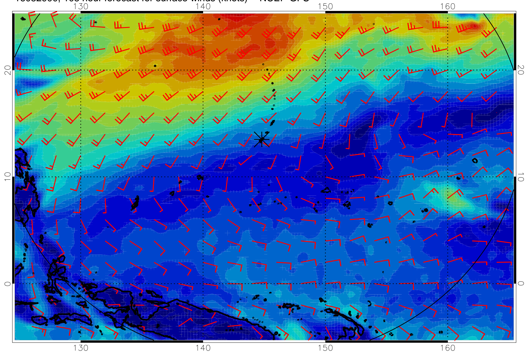
16082900, 108 hour forecast for surface winds (knots) -- NCEP GFS
