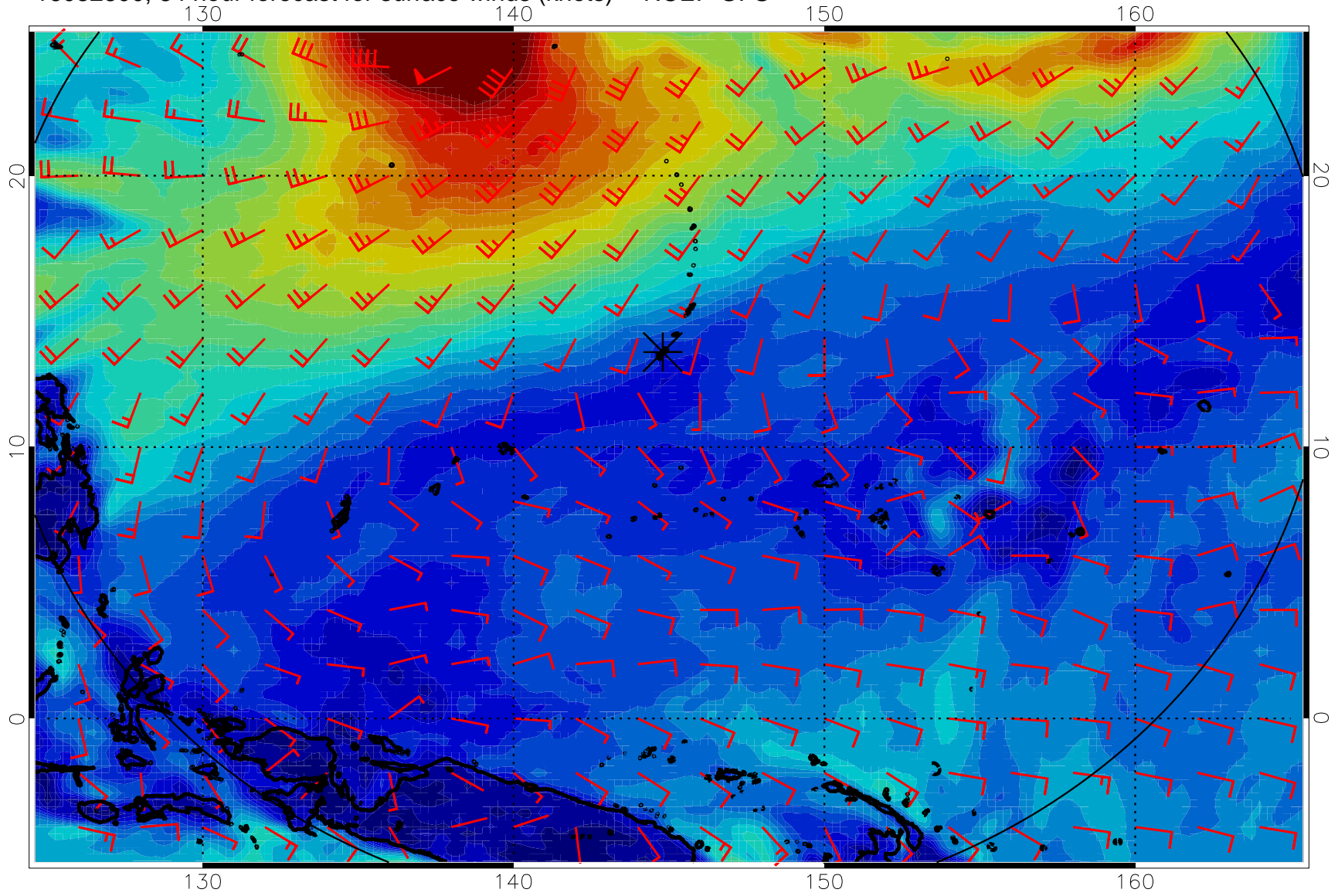
16082800, 84 hour forecast for surface winds (knots) -- NCEP GFS
