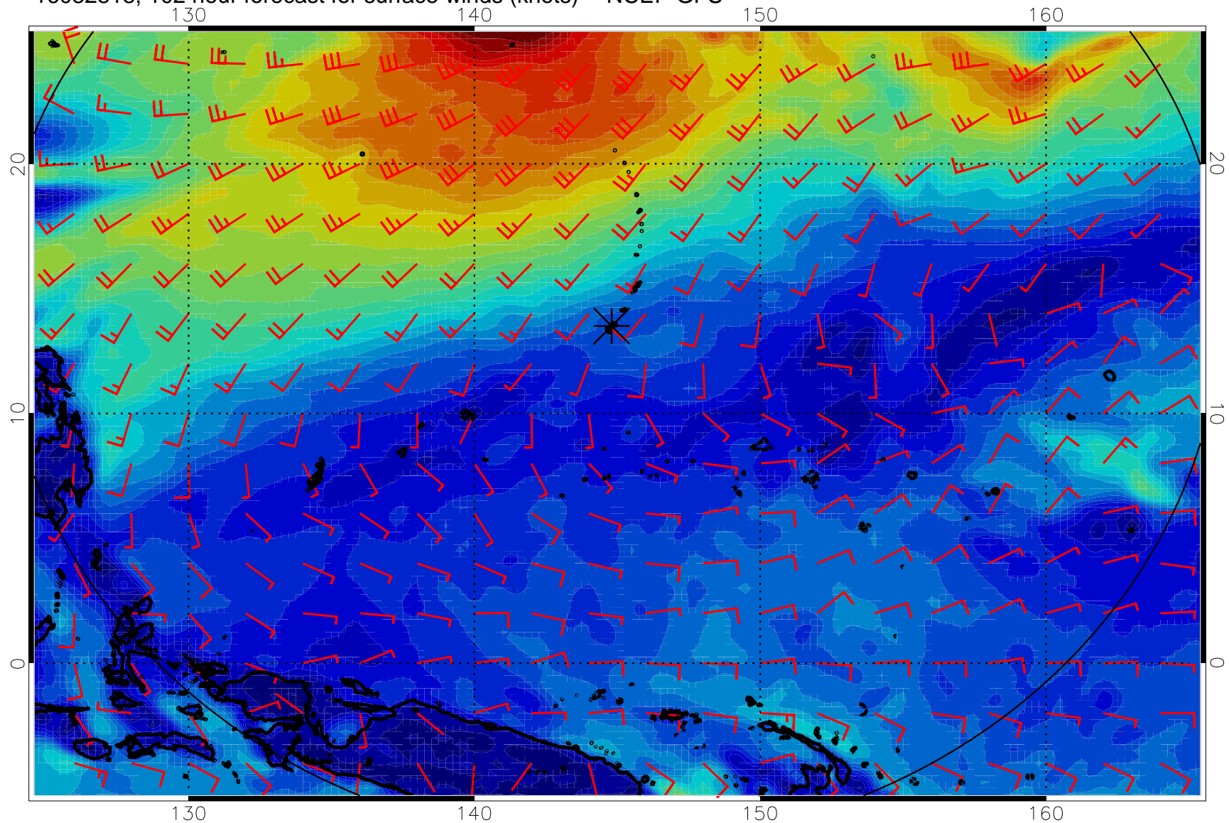
16082818, 102 hour forecast for surface winds (knots) -- NCEP GFS
