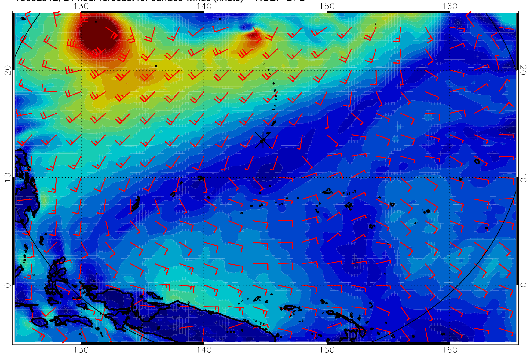
16082512, 24 hour forecast for surface winds (knots) -- NCEP GFS
