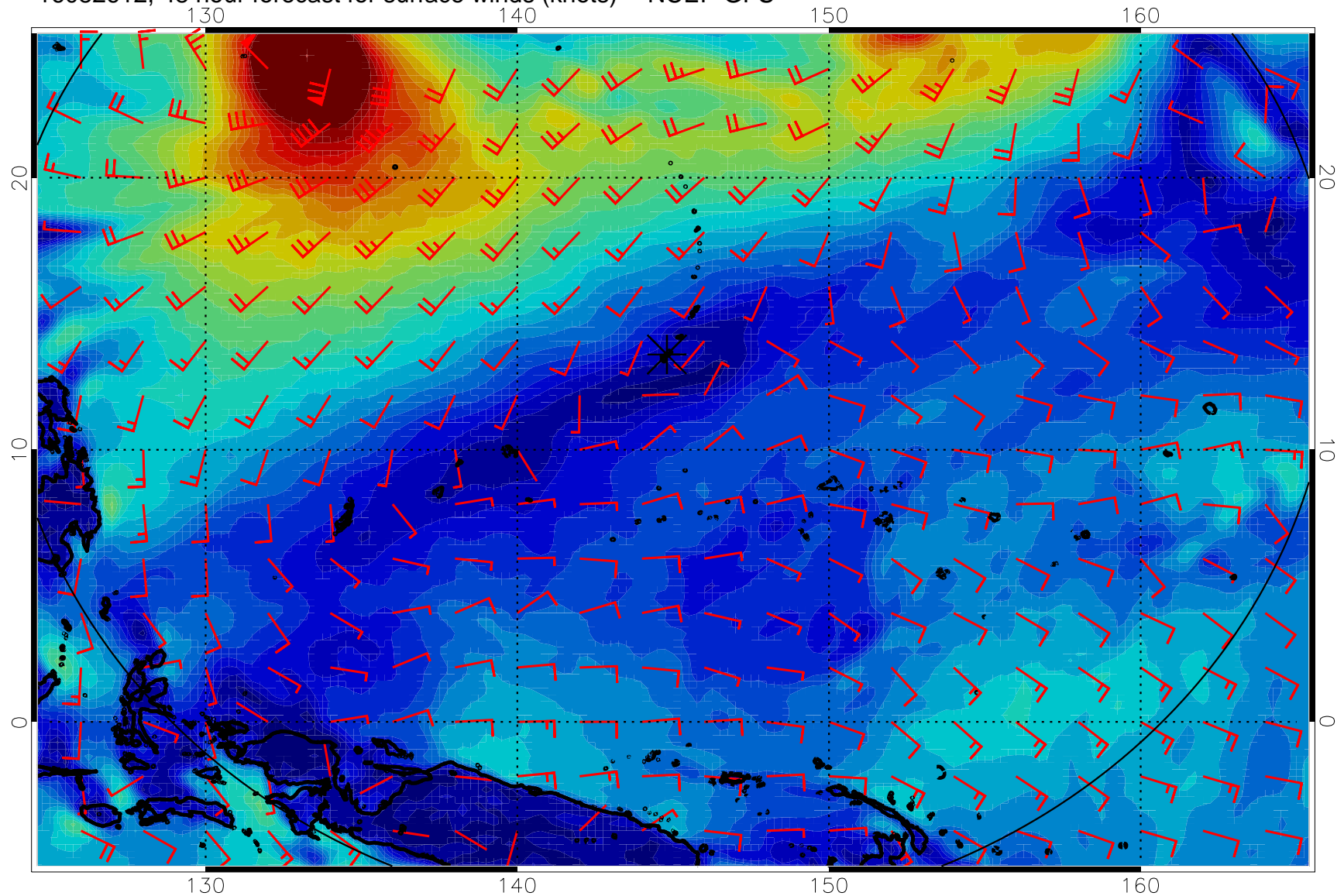
16082612, 48 hour forecast for surface winds (knots) -- NCEP GFS
