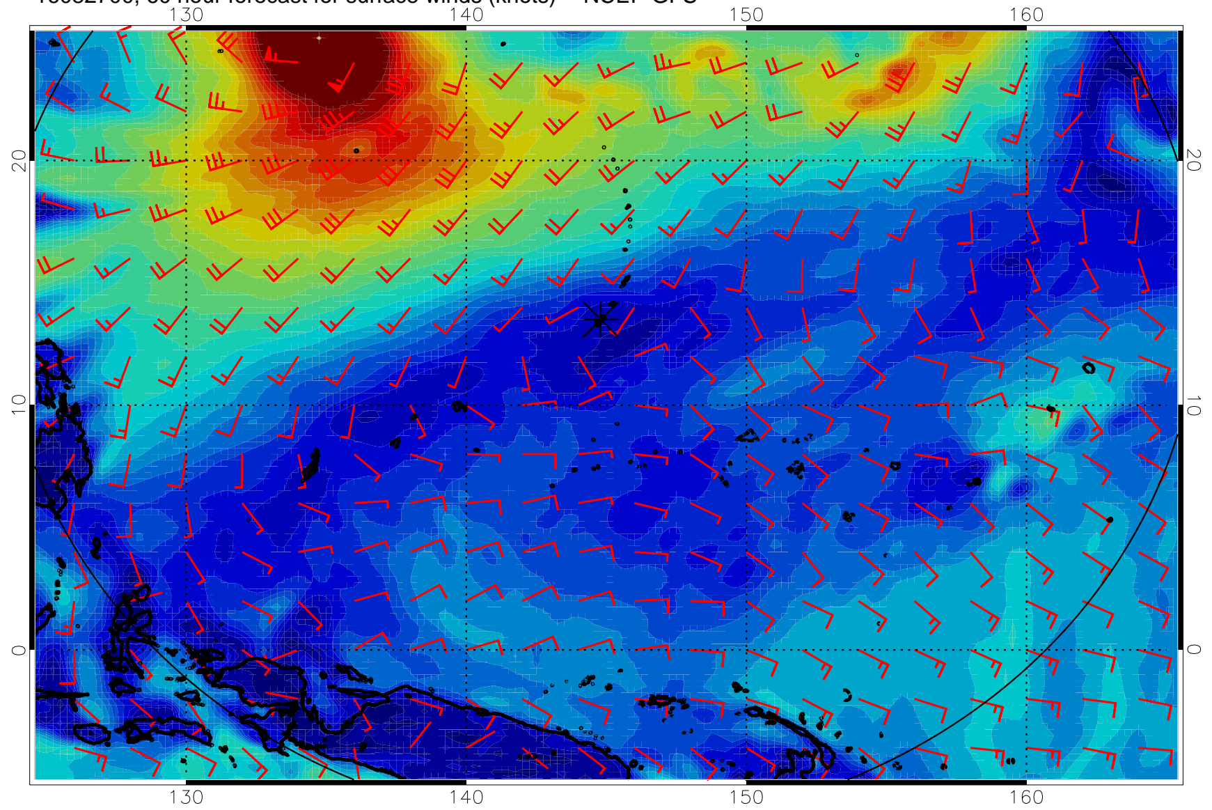
16082700, 60 hour forecast for surface winds (knots) -- NCEP GFS
