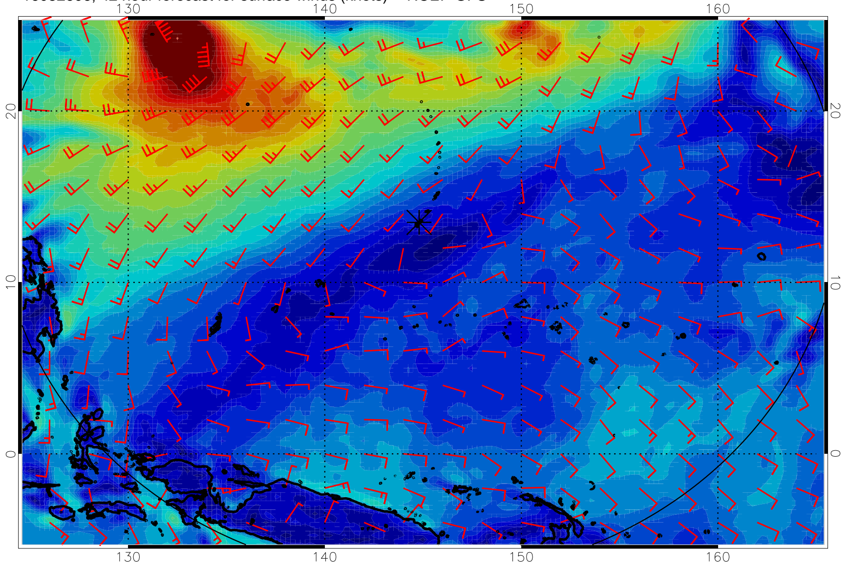
16082606, 42 hour forecast for surface winds (knots) -- NCEP GFS
