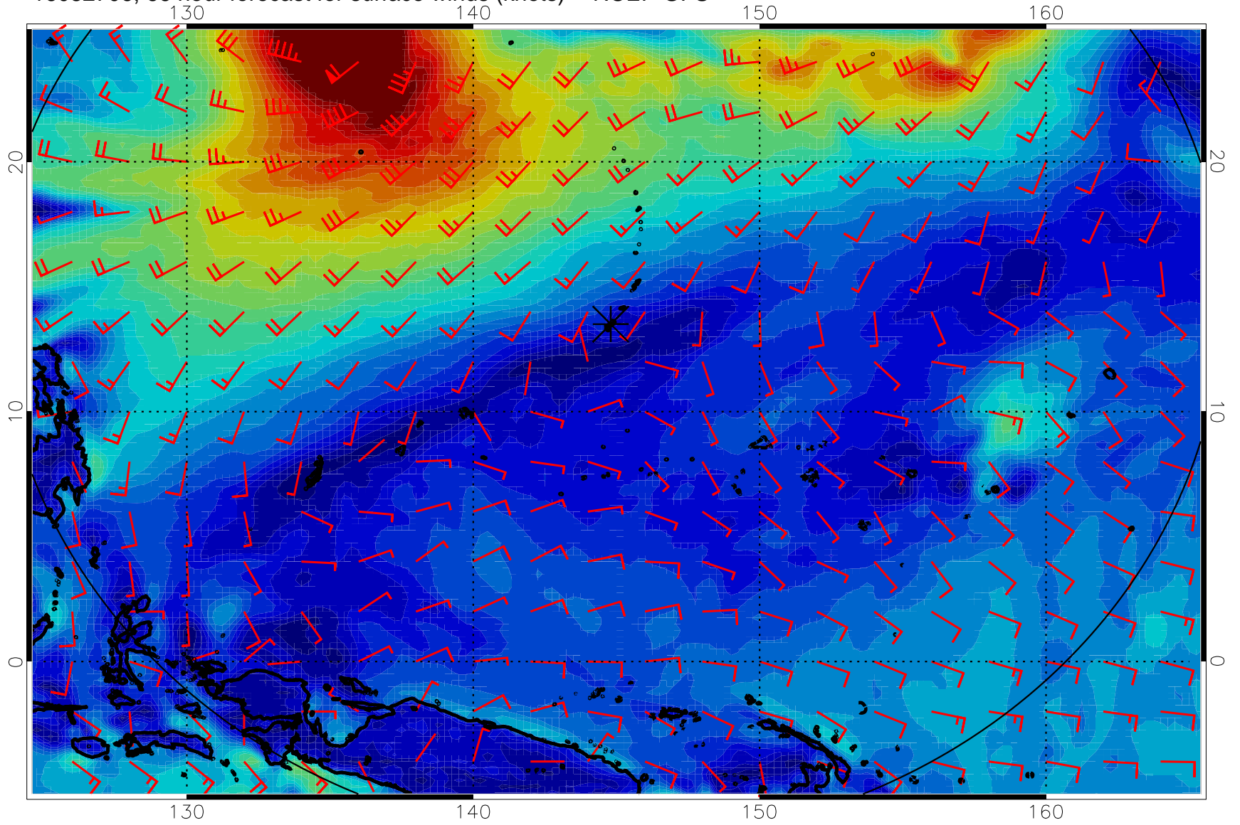
16082706, 66 hour forecast for surface winds (knots) -- NCEP GFS
