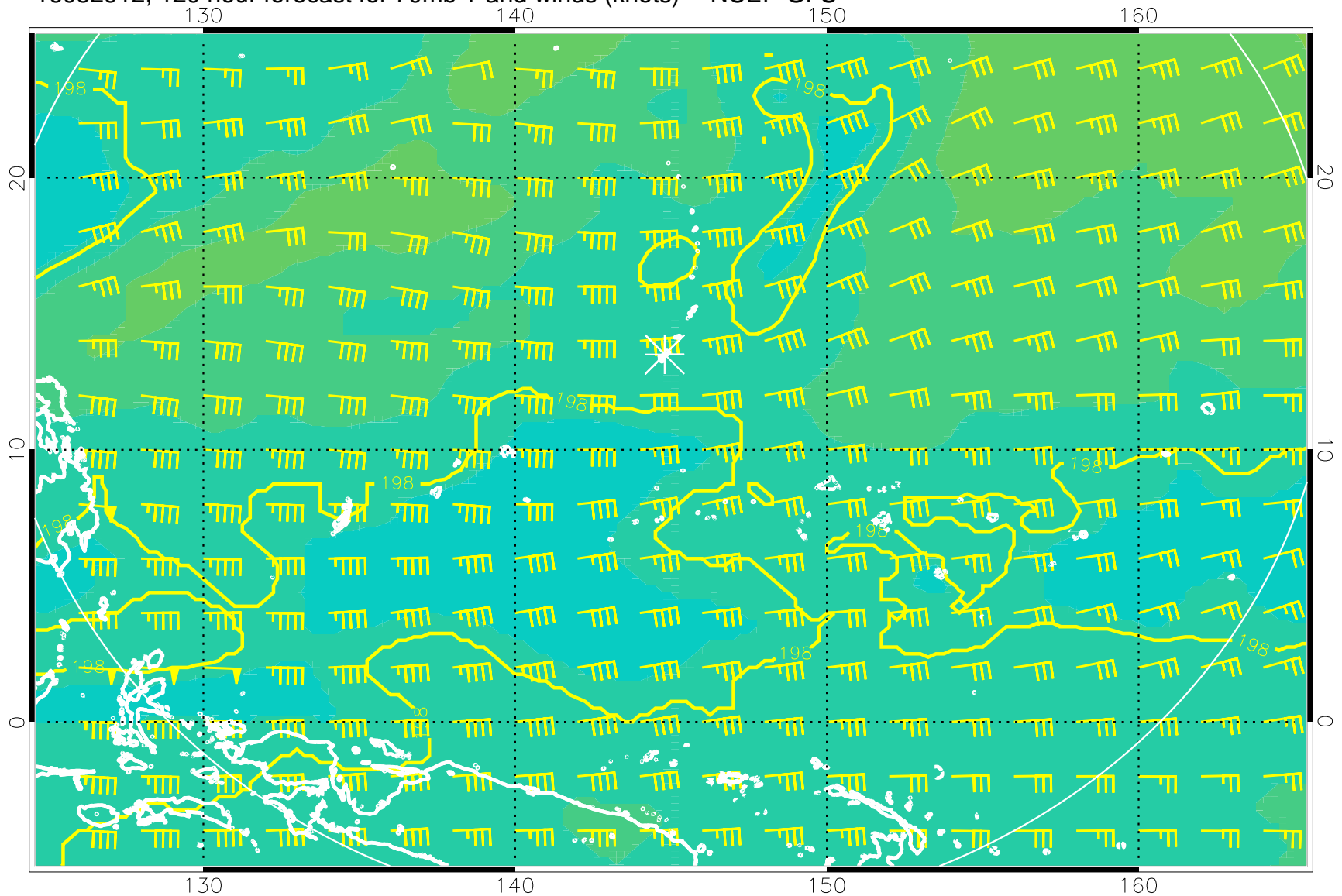
16082912, 120 hour forecast for 70mb T and winds (knots) -- NCEP GFS
