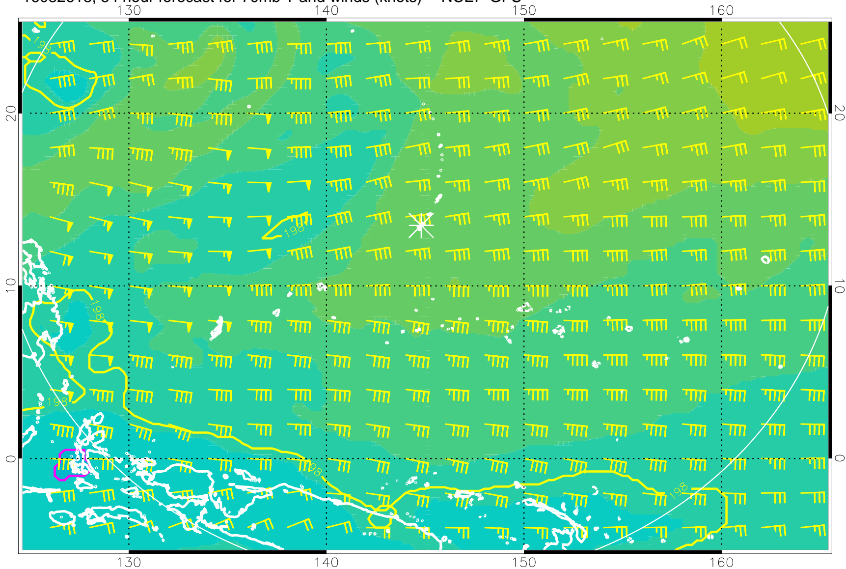
16082618, 54 hour forecast for 70mb T and winds (knots) -- NCEP GFS
