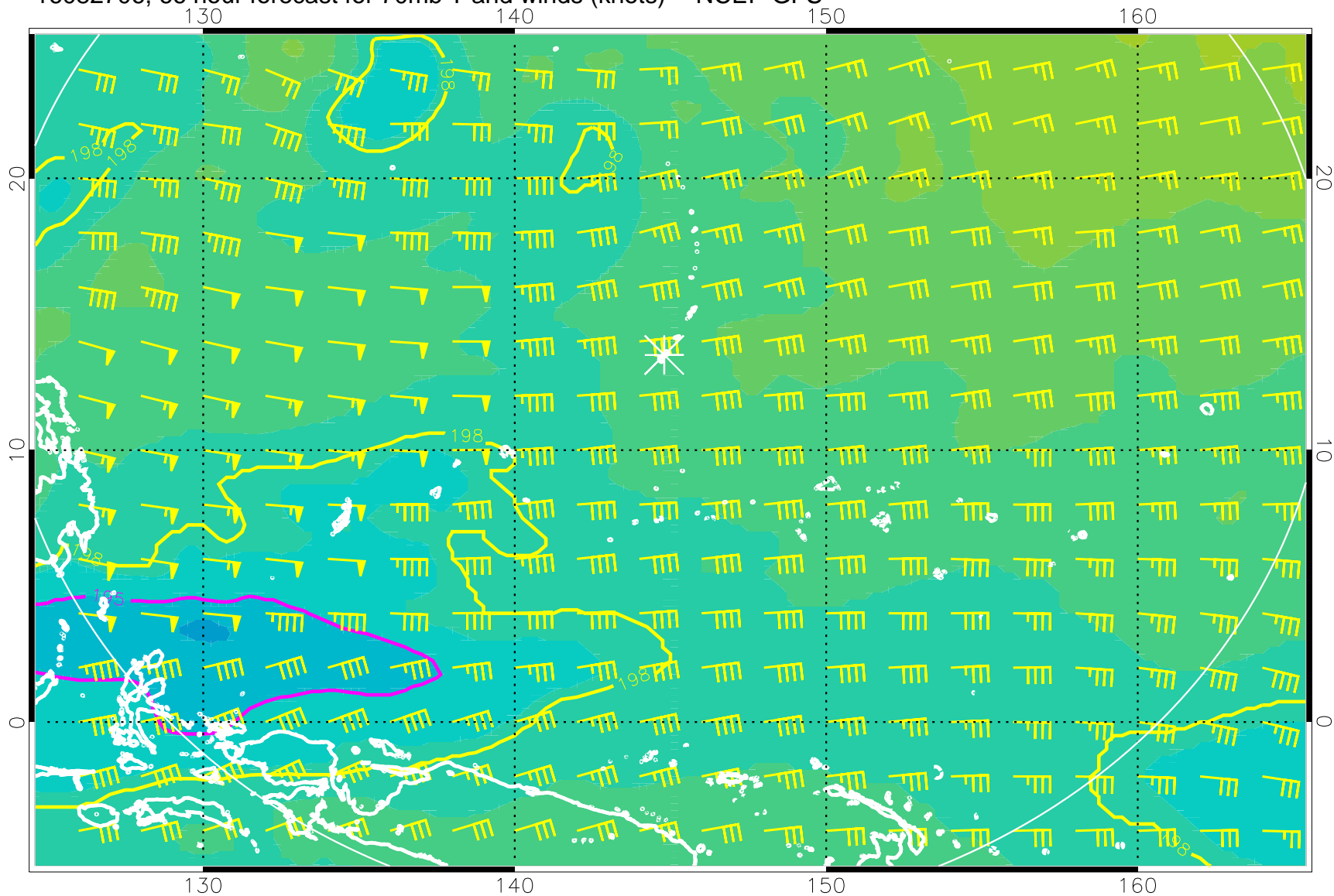
16082706, 66 hour forecast for 70mb T and winds (knots) -- NCEP GFS
