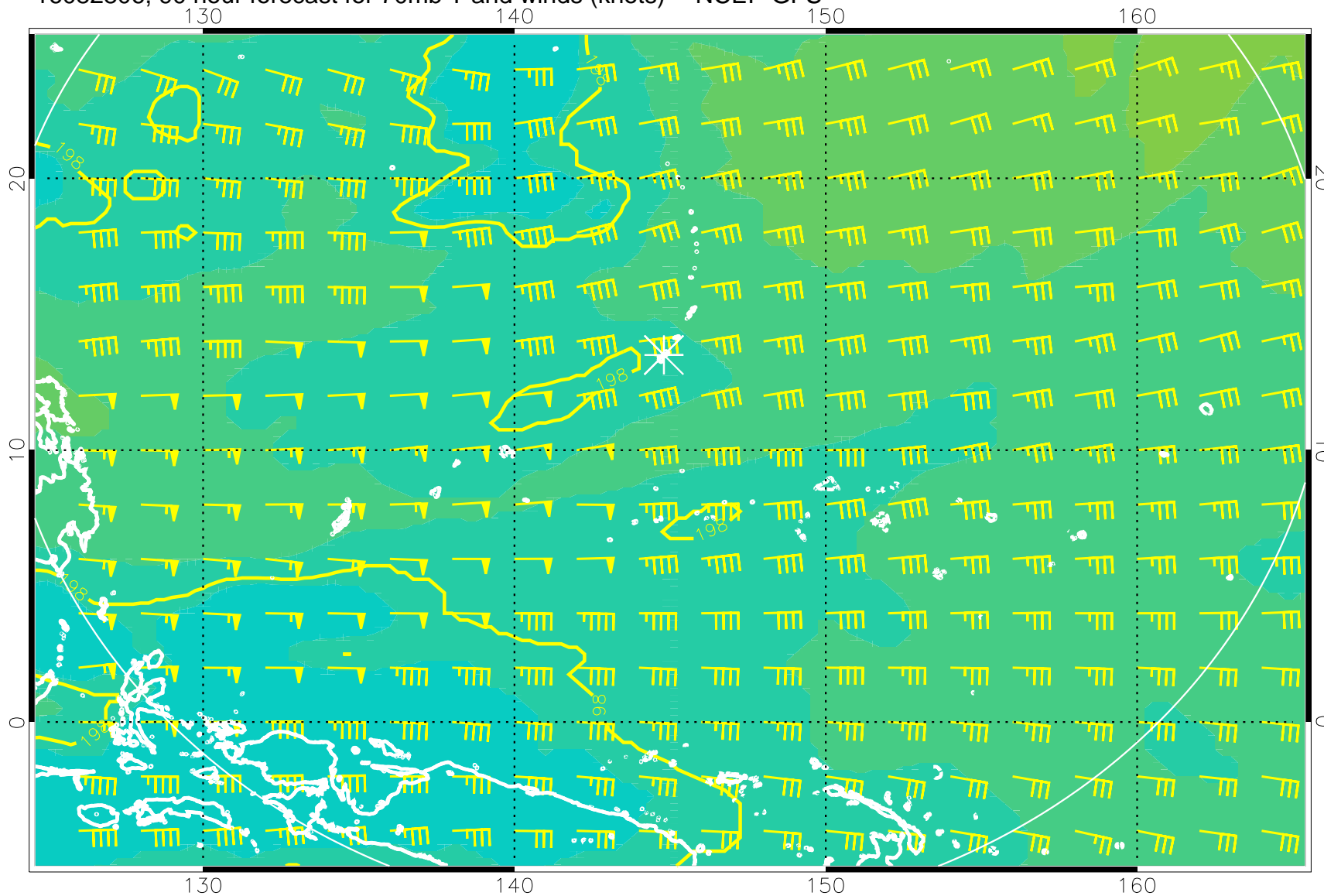
16082806, 90 hour forecast for 70mb T and winds (knots) -- NCEP GFS
