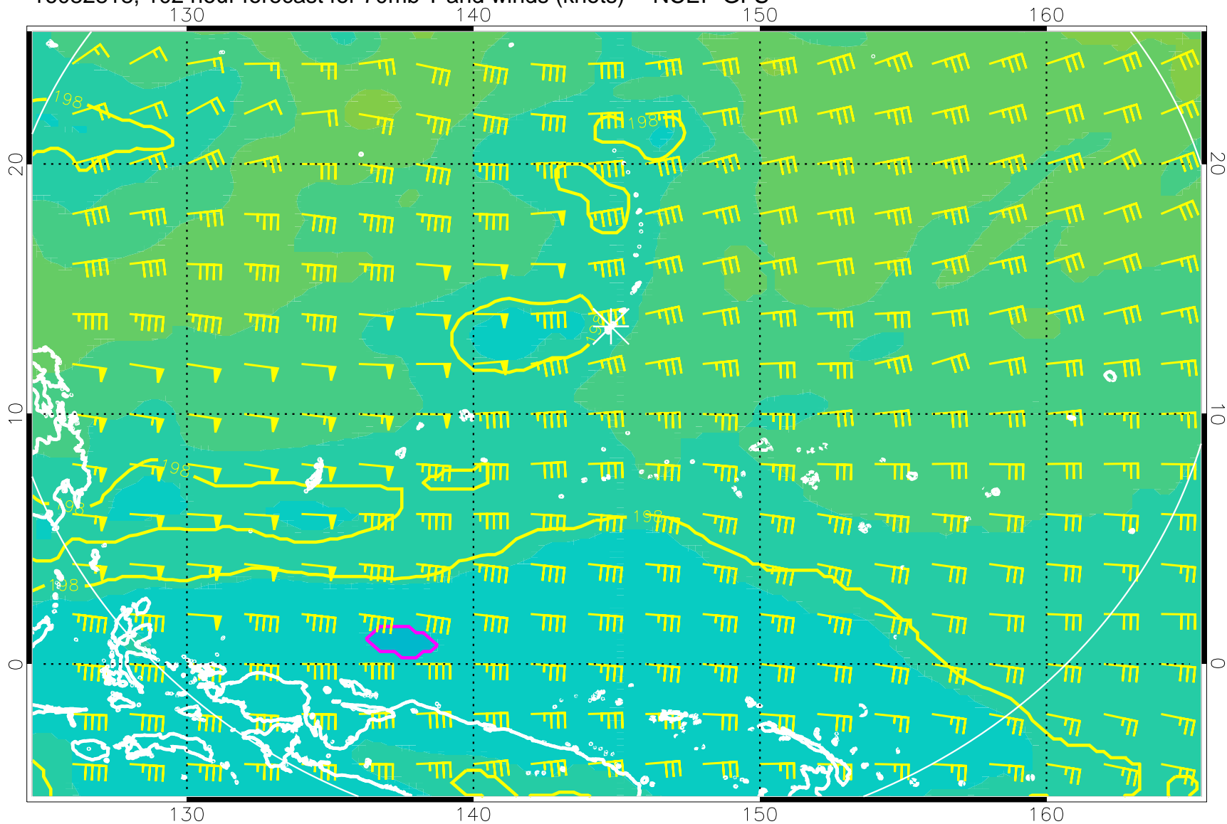
16082818, 102 hour forecast for 70mb T and winds (knots) -- NCEP GFS
