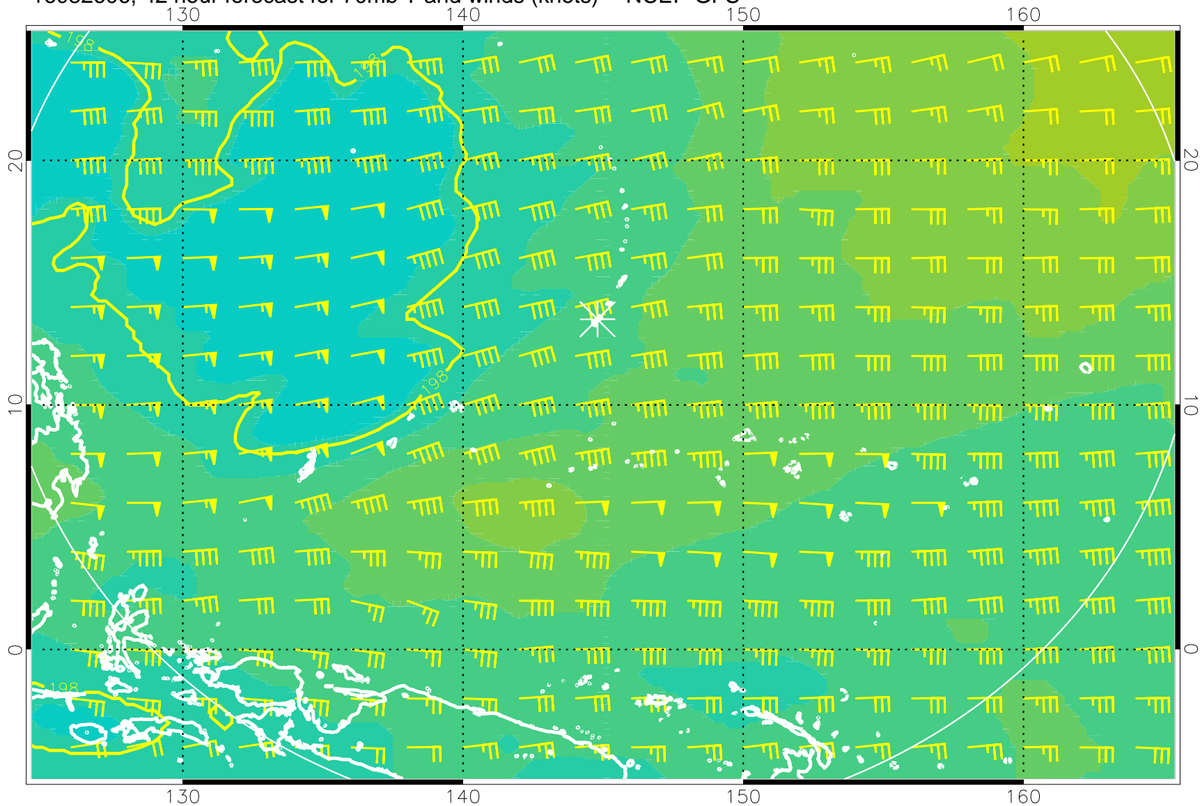
16082606, 42 hour forecast for 70mb T and winds (knots) -- NCEP GFS
