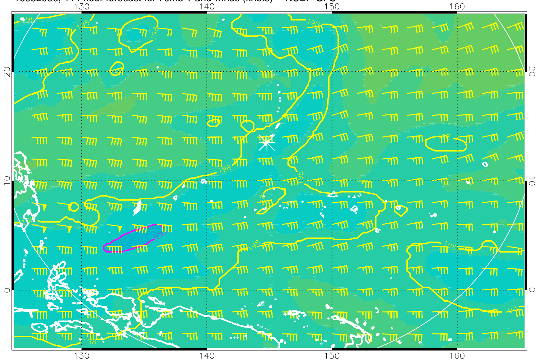
16082906, 114 hour forecast for 70mb T and winds (knots) -- NCEP GFS
