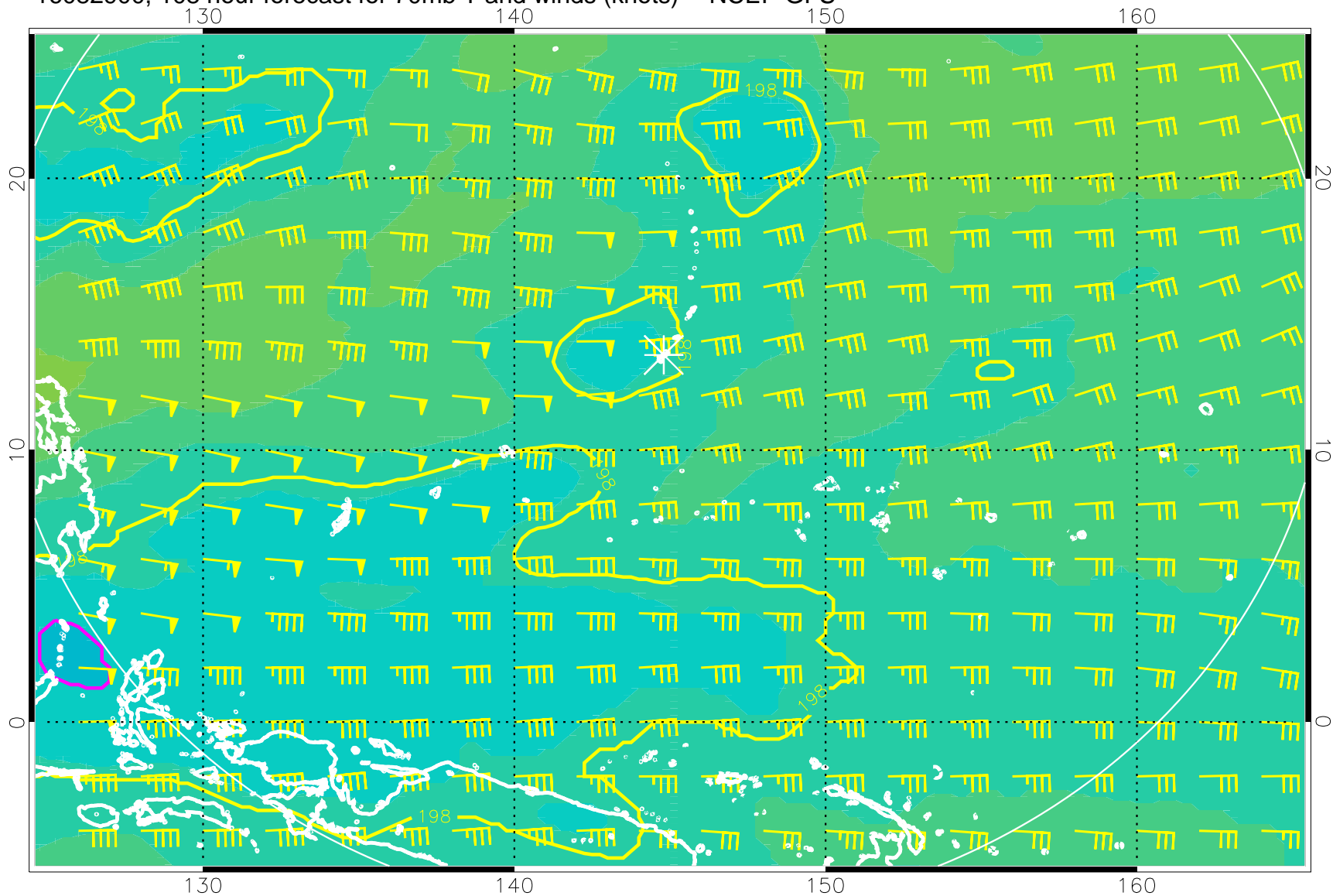
16082900, 108 hour forecast for 70mb T and winds (knots) -- NCEP GFS
