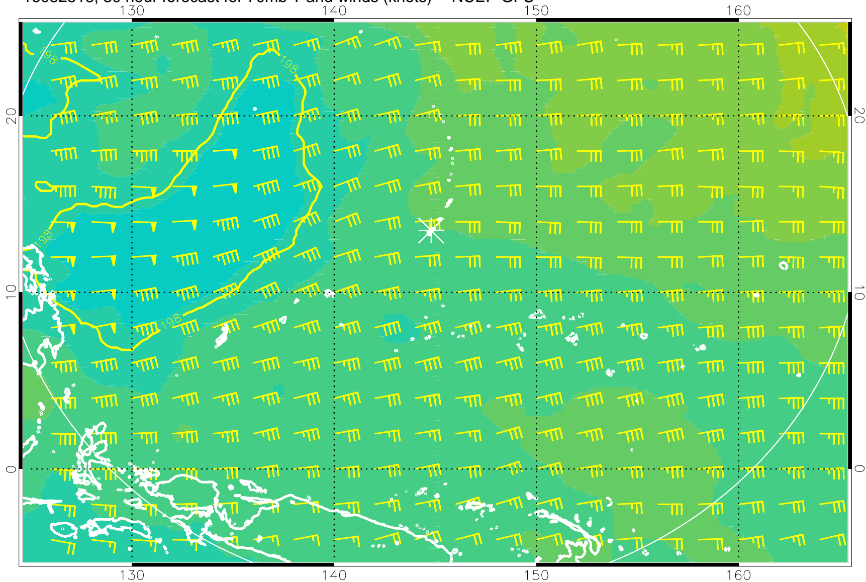
16082518, 30 hour forecast for 70mb T and winds (knots) -- NCEP GFS
