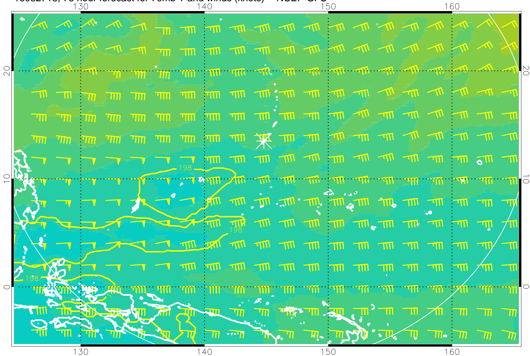
16082718, 78 hour forecast for 70mb T and winds (knots) -- NCEP GFS
