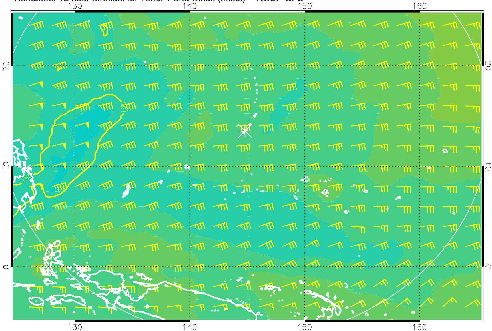
16082500, 12 hour forecast for 70mb T and winds (knots) -- NCEP GFS
