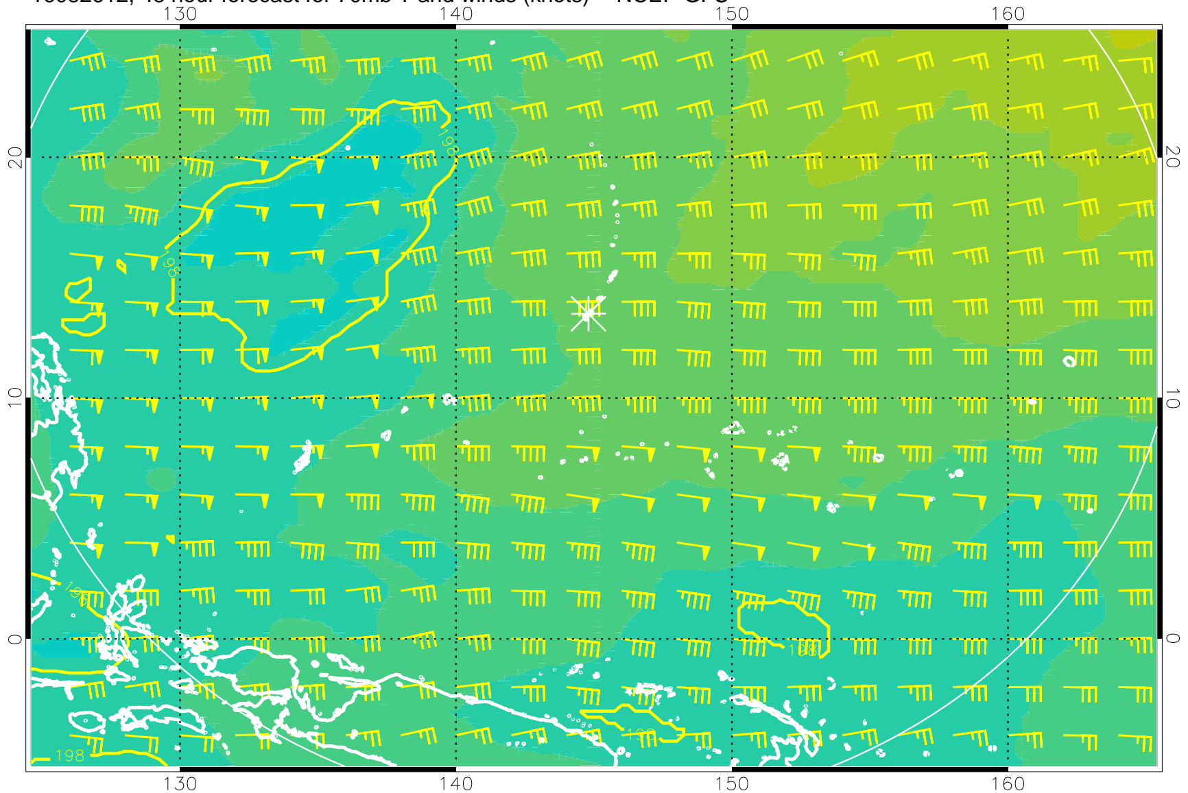
16082612, 48 hour forecast for 70mb T and winds (knots) -- NCEP GFS
