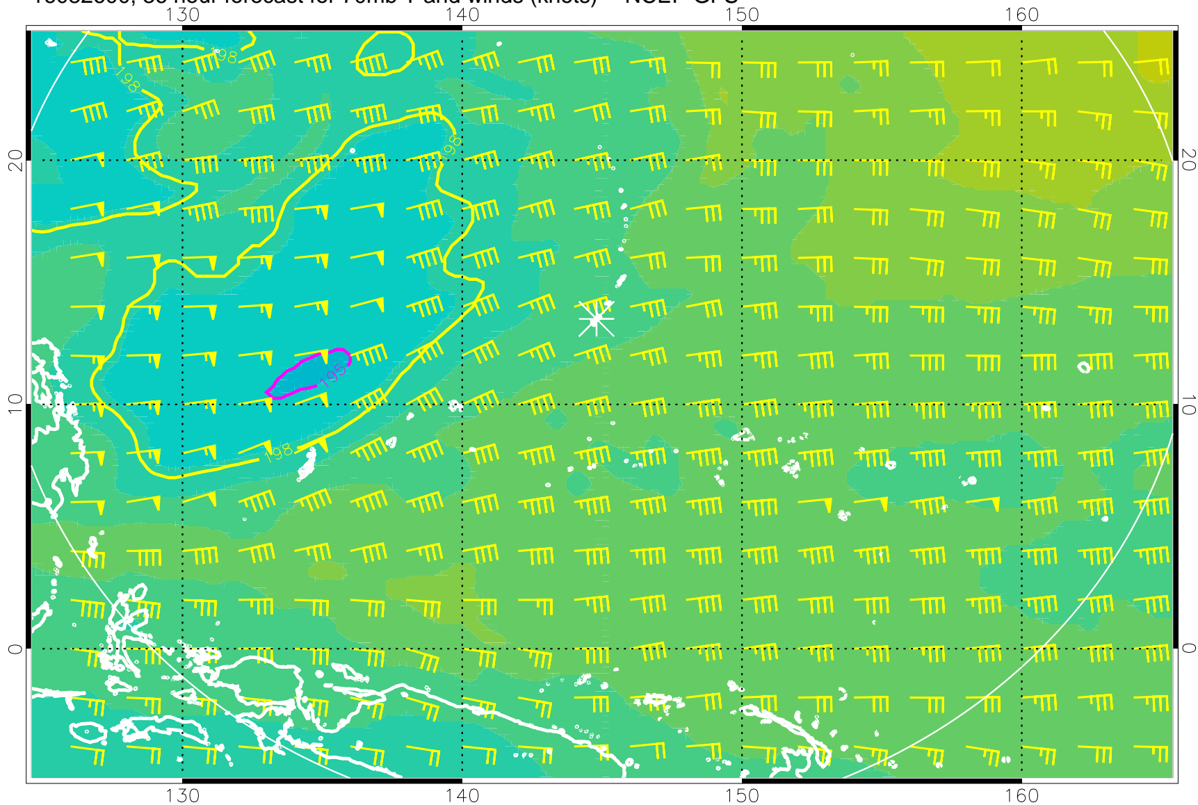
16082600, 36 hour forecast for 70mb T and winds (knots) -- NCEP GFS
