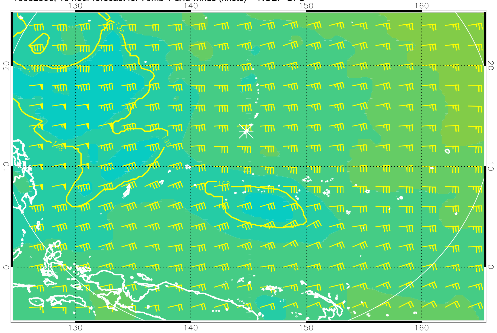
16082506, 18 hour forecast for 70mb T and winds (knots) -- NCEP GFS
