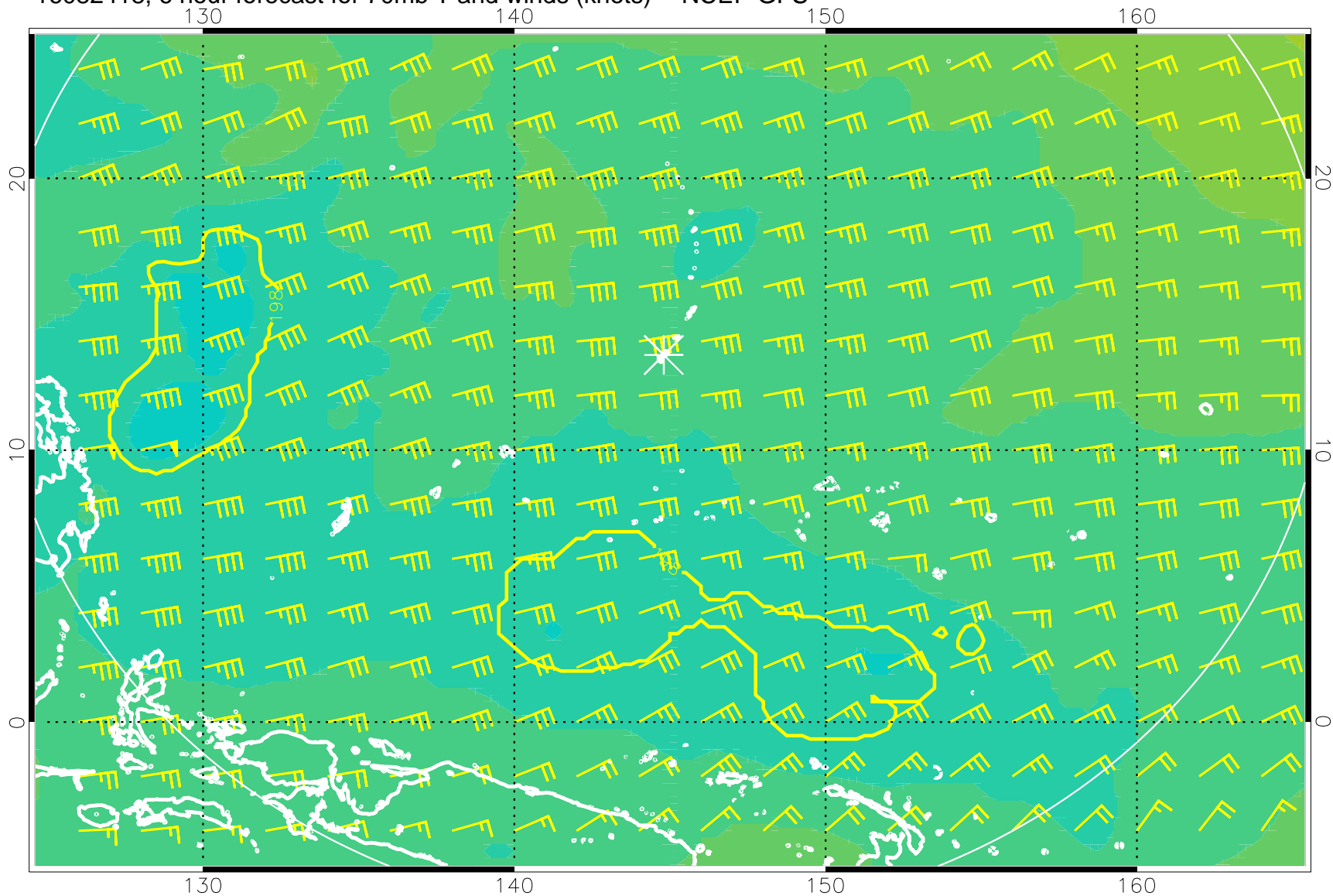
16082418, 6 hour forecast for 70mb T and winds (knots) -- NCEP GFS
