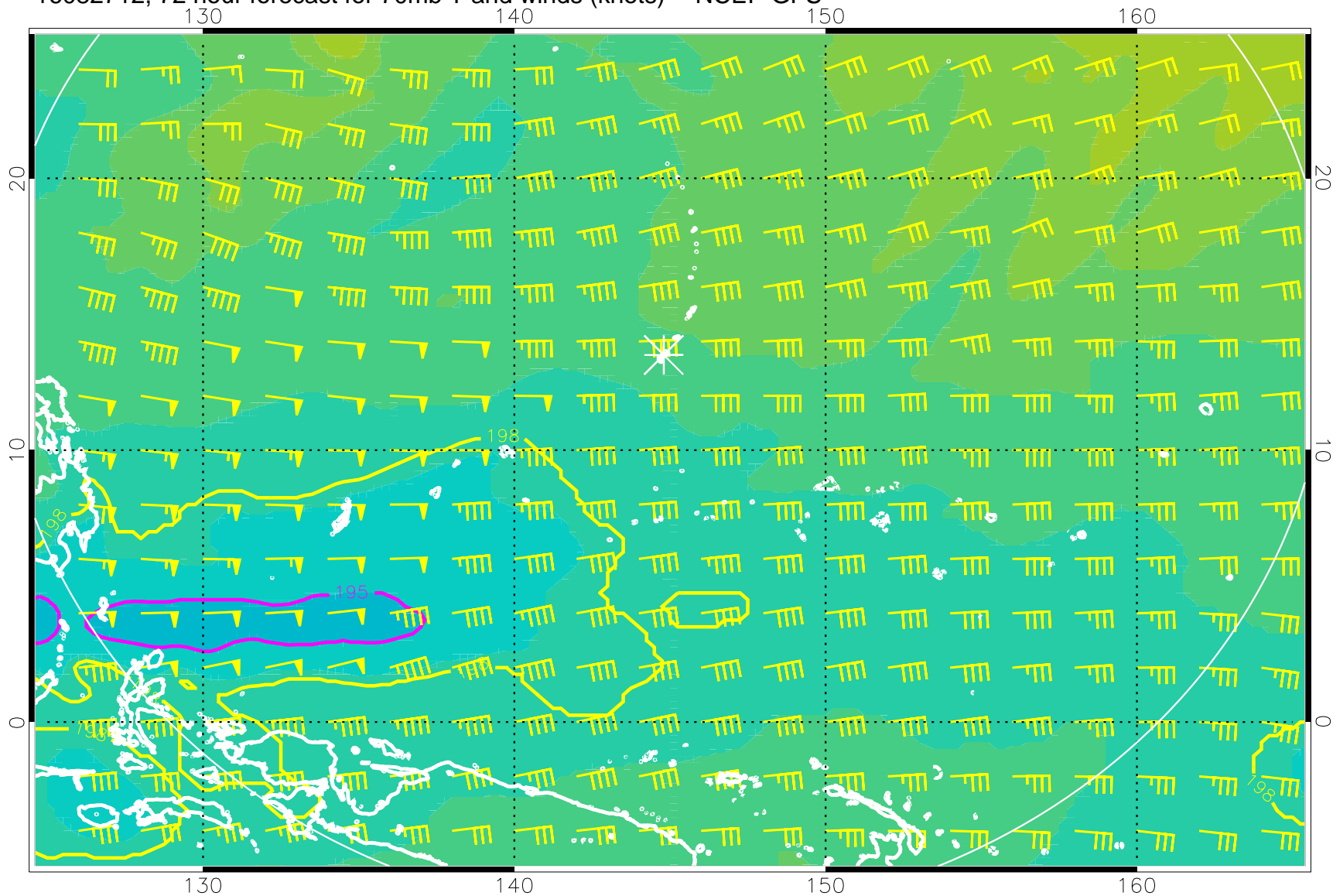
16082712, 72 hour forecast for 70mb T and winds (knots) -- NCEP GFS
