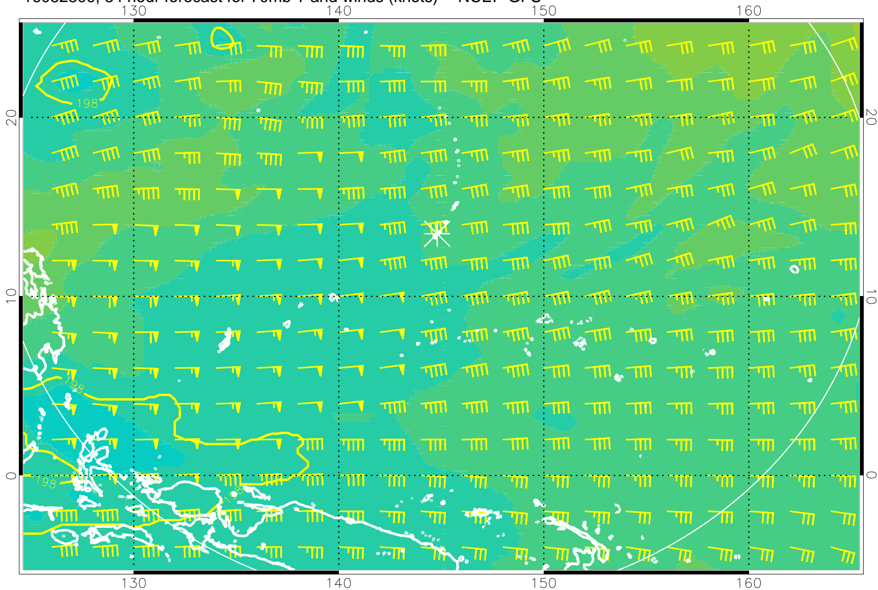
16082800, 84 hour forecast for 70mb T and winds (knots) -- NCEP GFS
