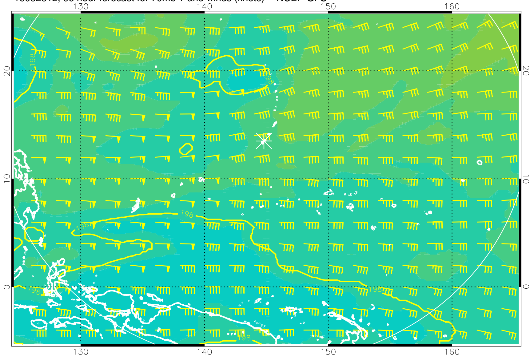
16082812, 96 hour forecast for 70mb T and winds (knots) -- NCEP GFS
