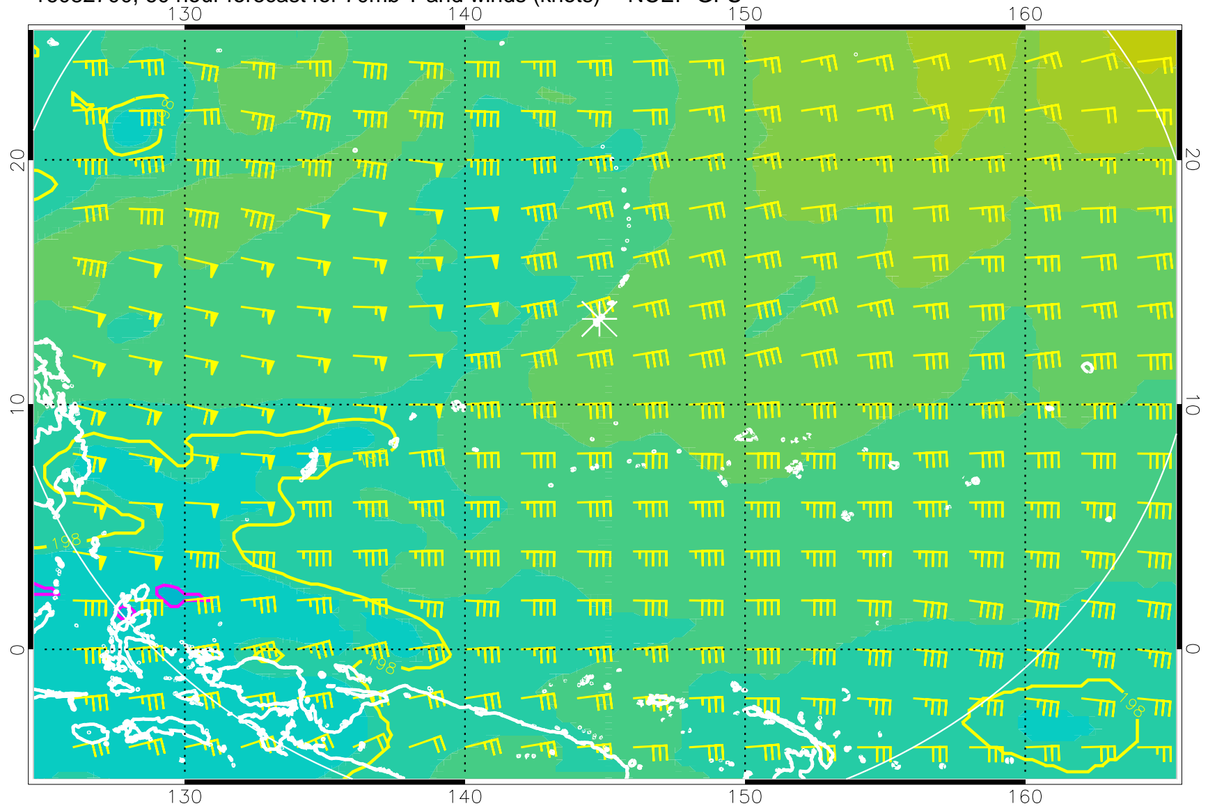
16082700, 60 hour forecast for 70mb T and winds (knots) -- NCEP GFS
