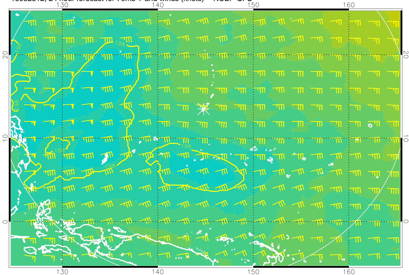
16082512, 24 hour forecast for 70mb T and winds (knots) -- NCEP GFS
