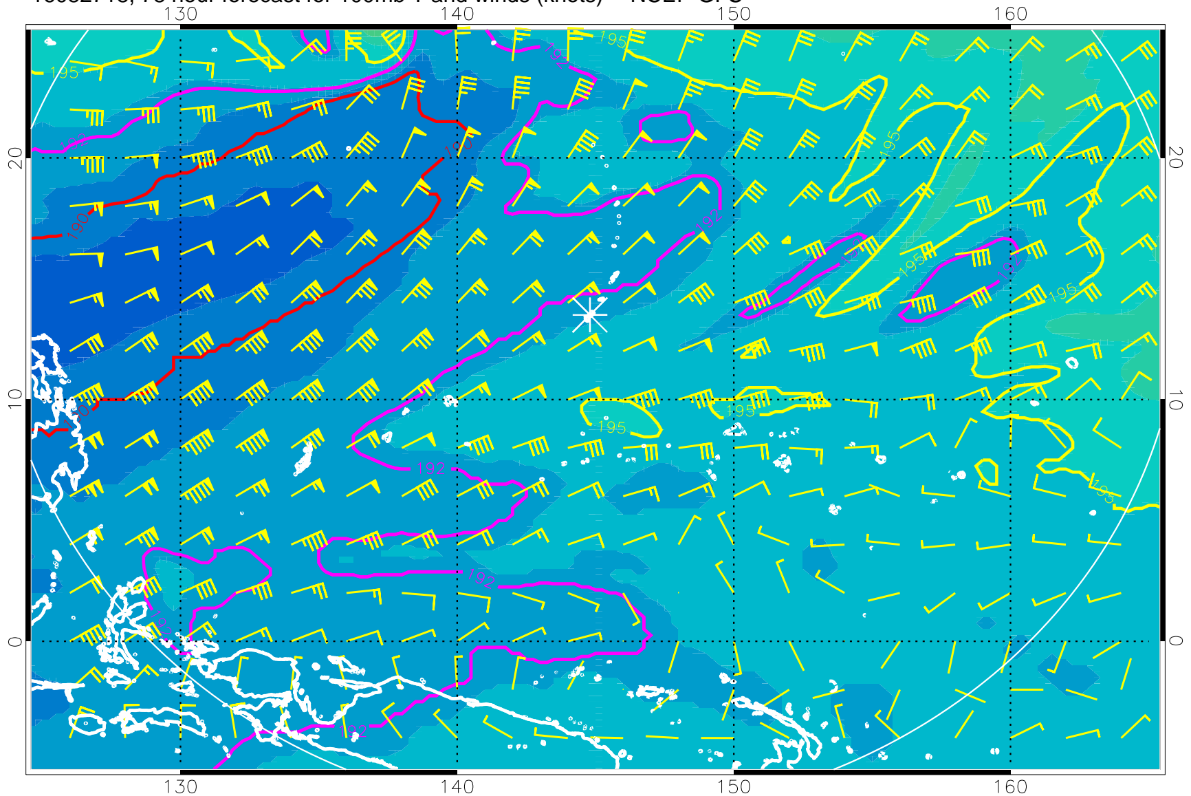
16082718, 78 hour forecast for 100mb T and winds (knots) -- NCEP GFS
