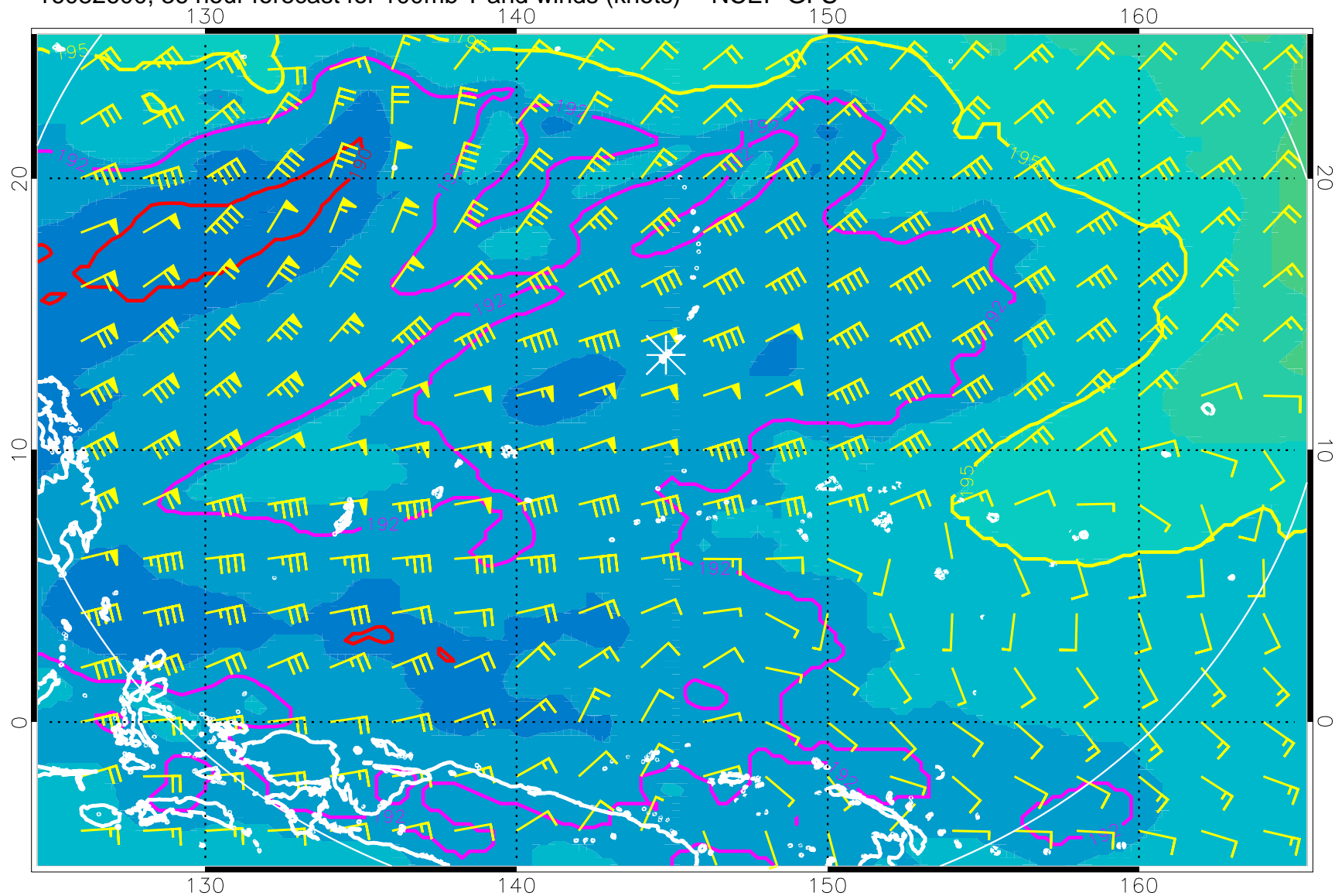
16082600, 36 hour forecast for 100mb T and winds (knots) -- NCEP GFS
