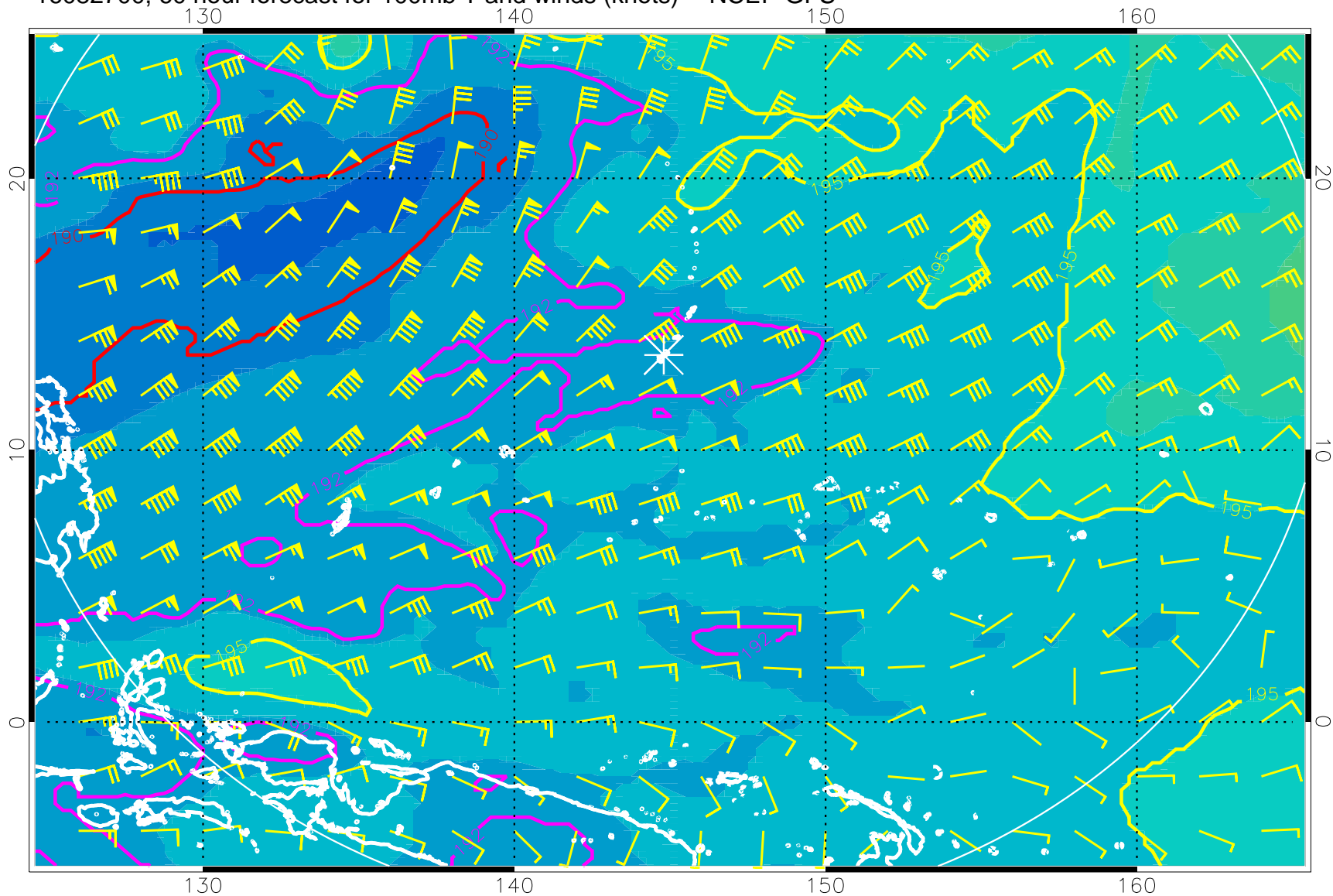
16082700, 60 hour forecast for 100mb T and winds (knots) -- NCEP GFS
