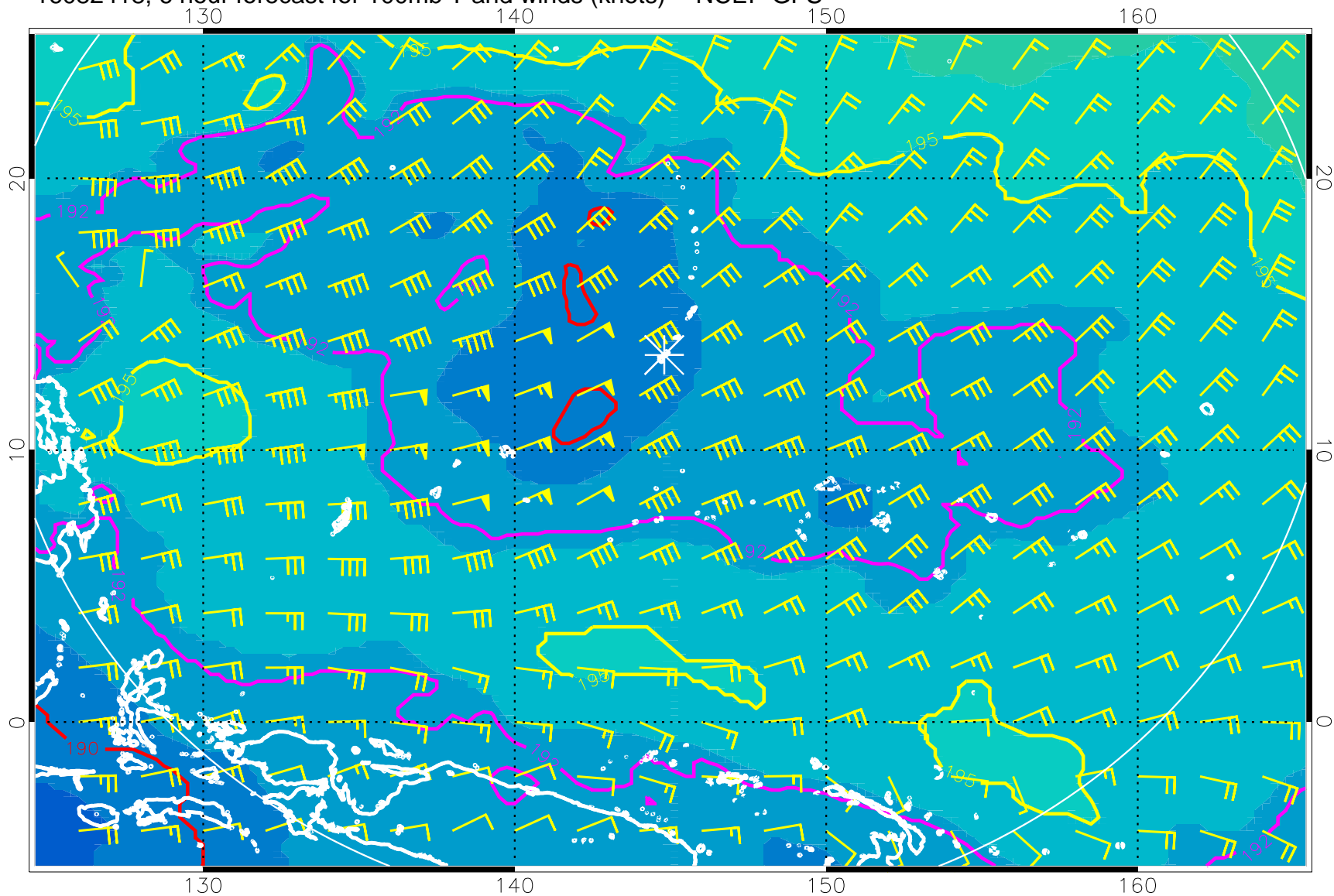
16082418, 6 hour forecast for 100mb T and winds (knots) -- NCEP GFS
