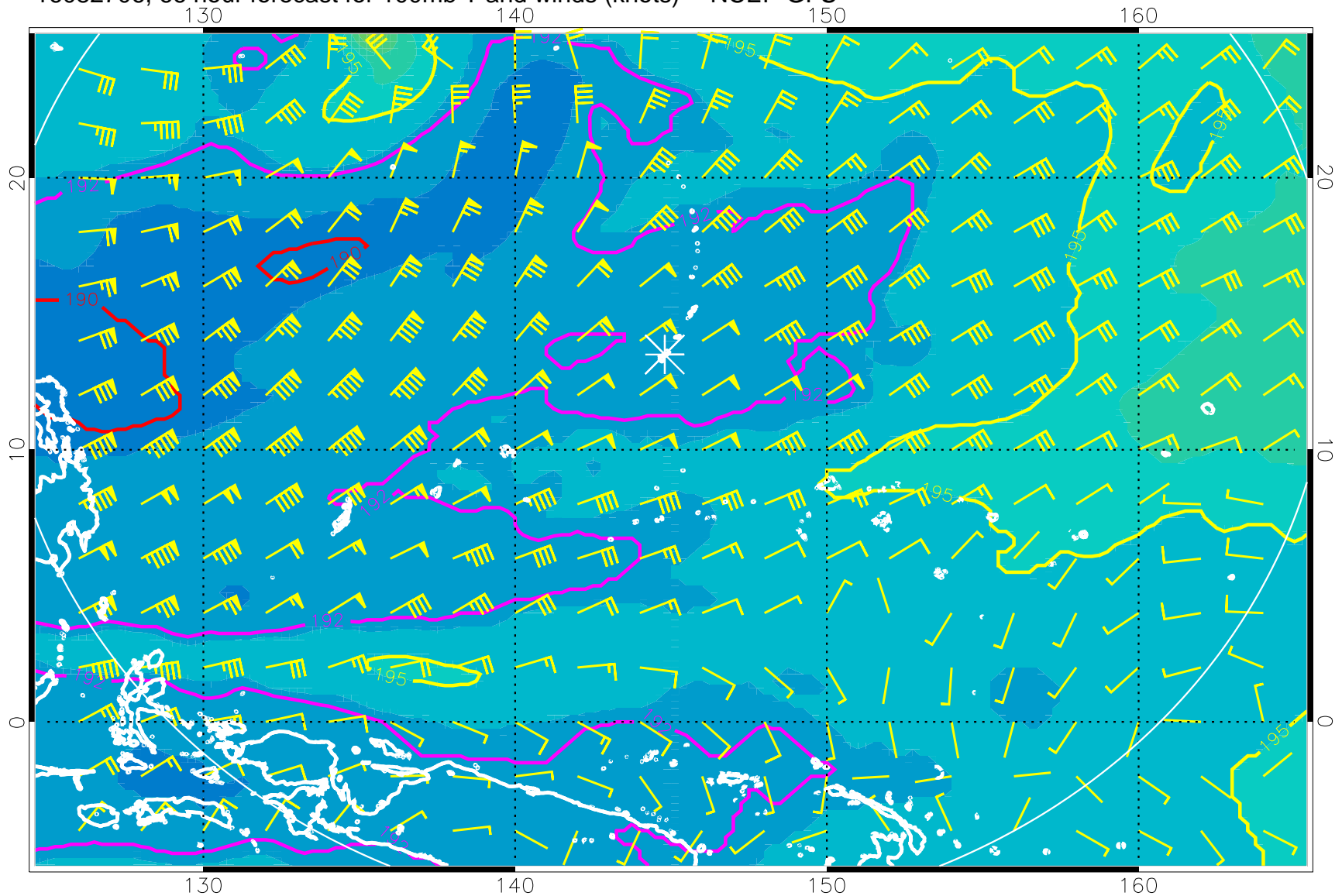
16082706, 66 hour forecast for 100mb T and winds (knots) -- NCEP GFS
