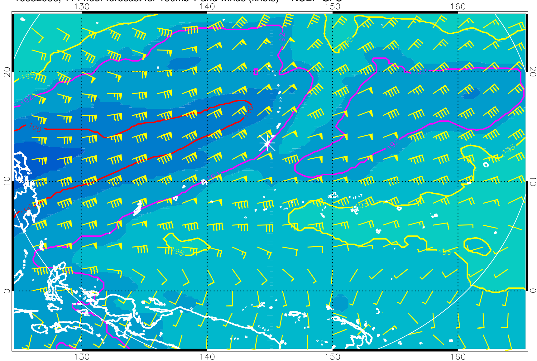
16082906, 114 hour forecast for 100mb T and winds (knots) -- NCEP GFS
