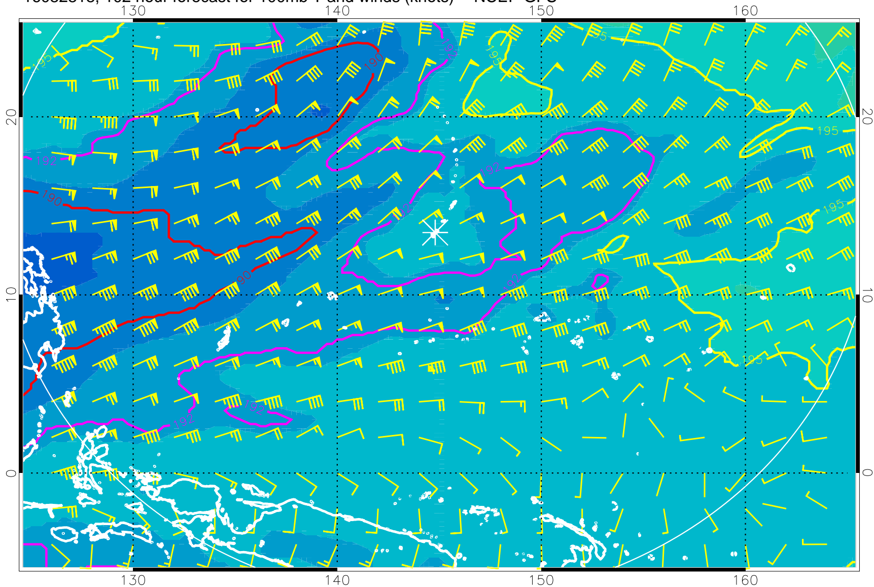
16082818, 102 hour forecast for 100mb T and winds (knots) -- NCEP GFS
