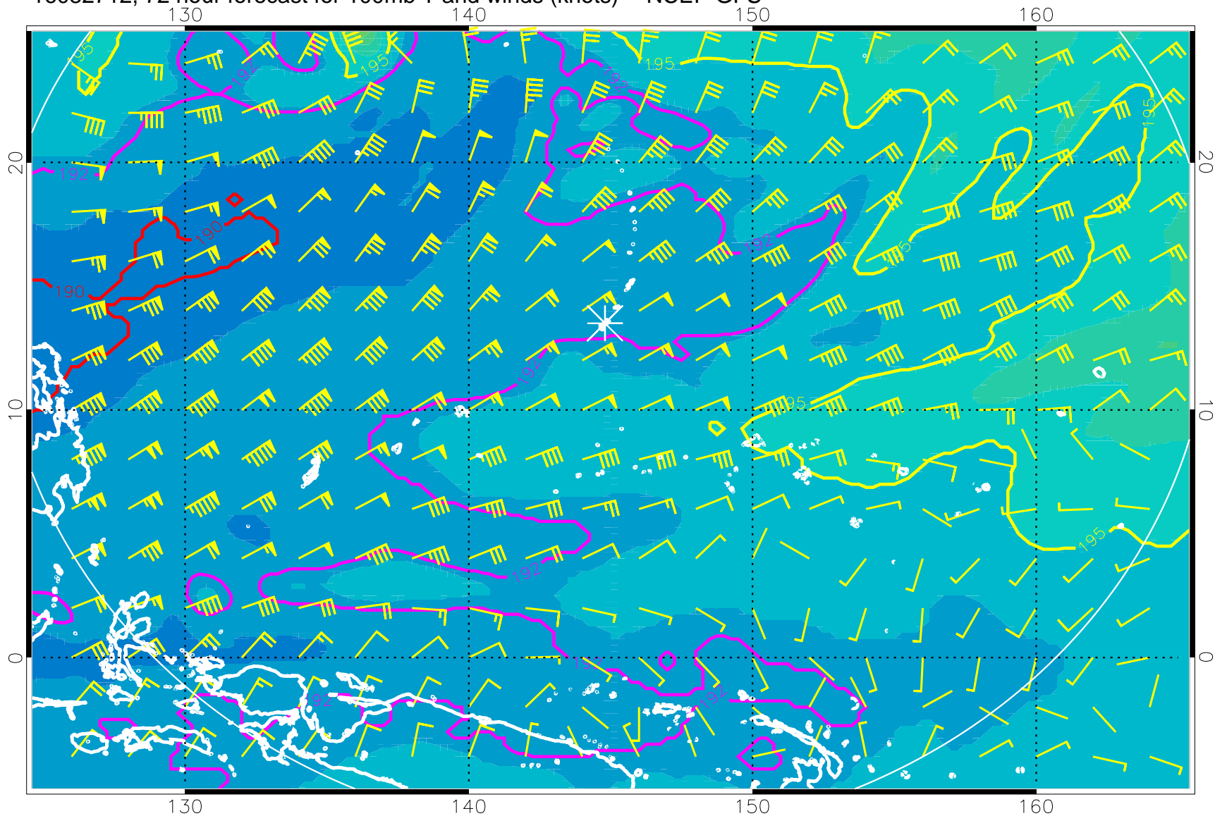
16082712, 72 hour forecast for 100mb T and winds (knots) -- NCEP GFS
