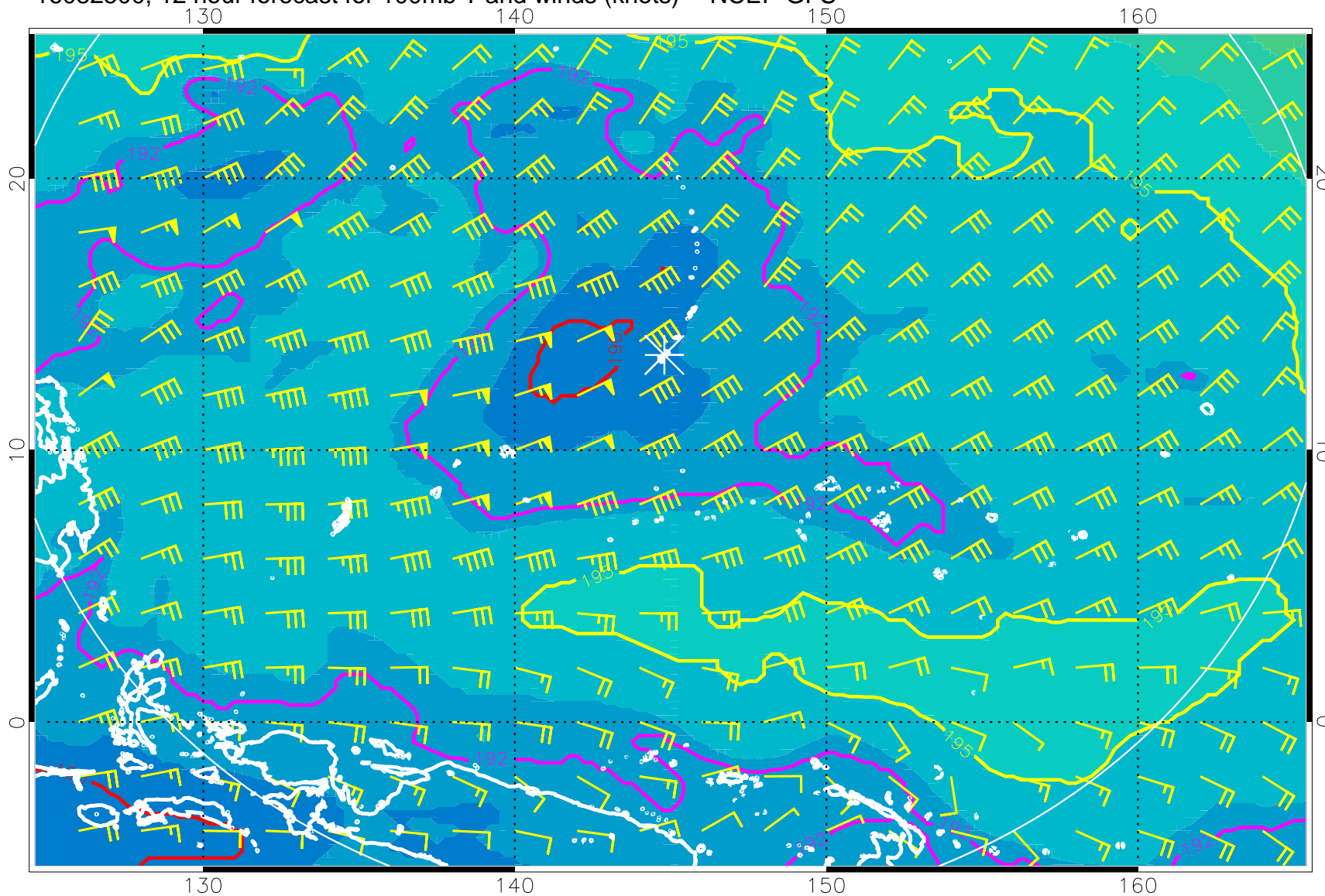
16082500, 12 hour forecast for 100mb T and winds (knots) -- NCEP GFS
