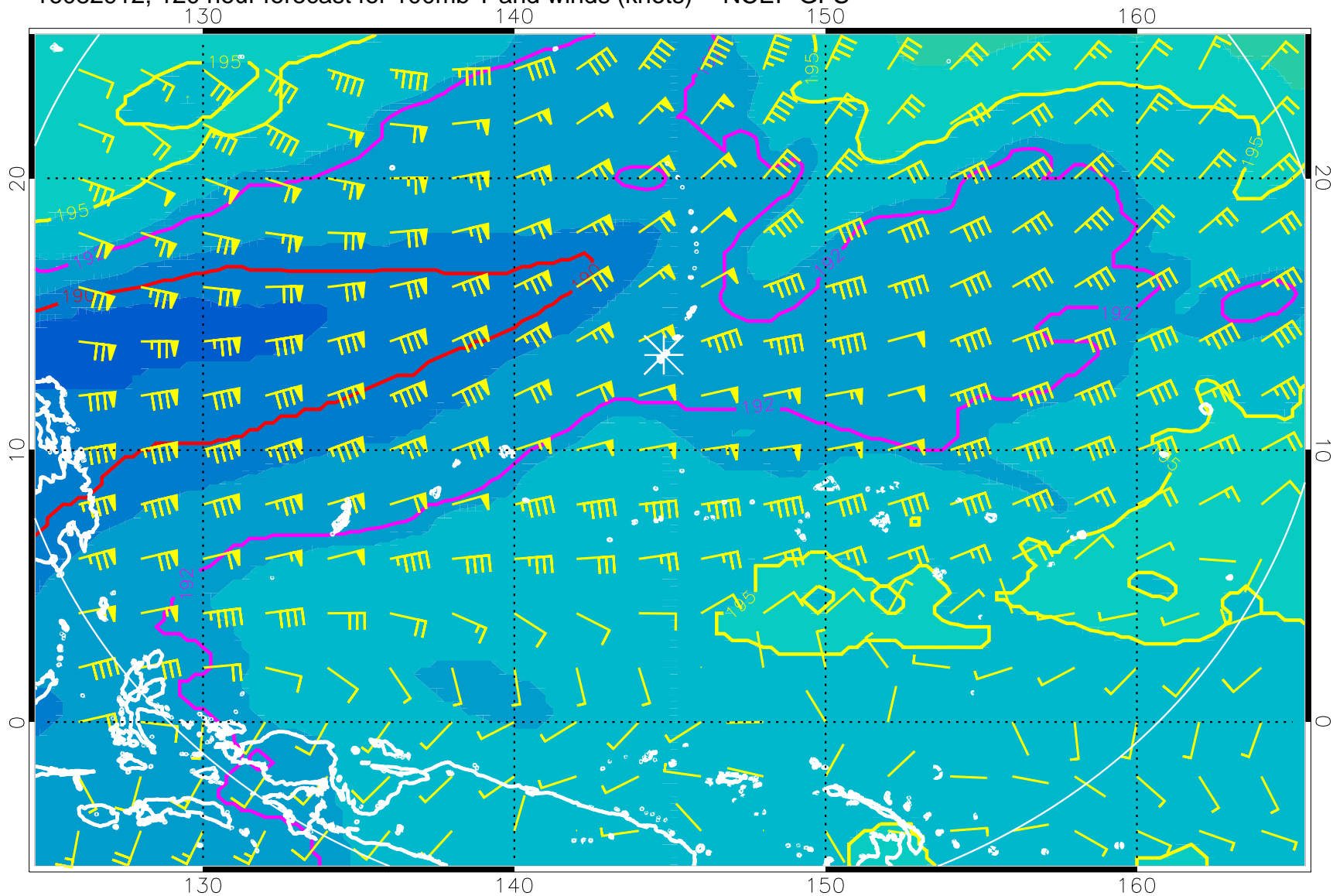
16082912, 120 hour forecast for 100mb T and winds (knots) -- NCEP GFS
