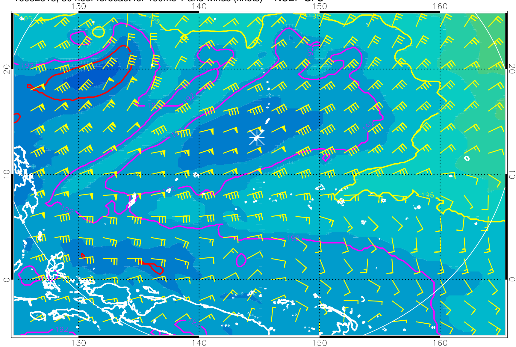
16082518, 30 hour forecast for 100mb T and winds (knots) -- NCEP GFS
