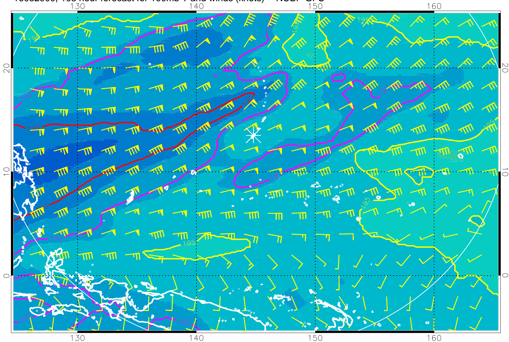
16082900, 108 hour forecast for 100mb T and winds (knots) -- NCEP GFS
