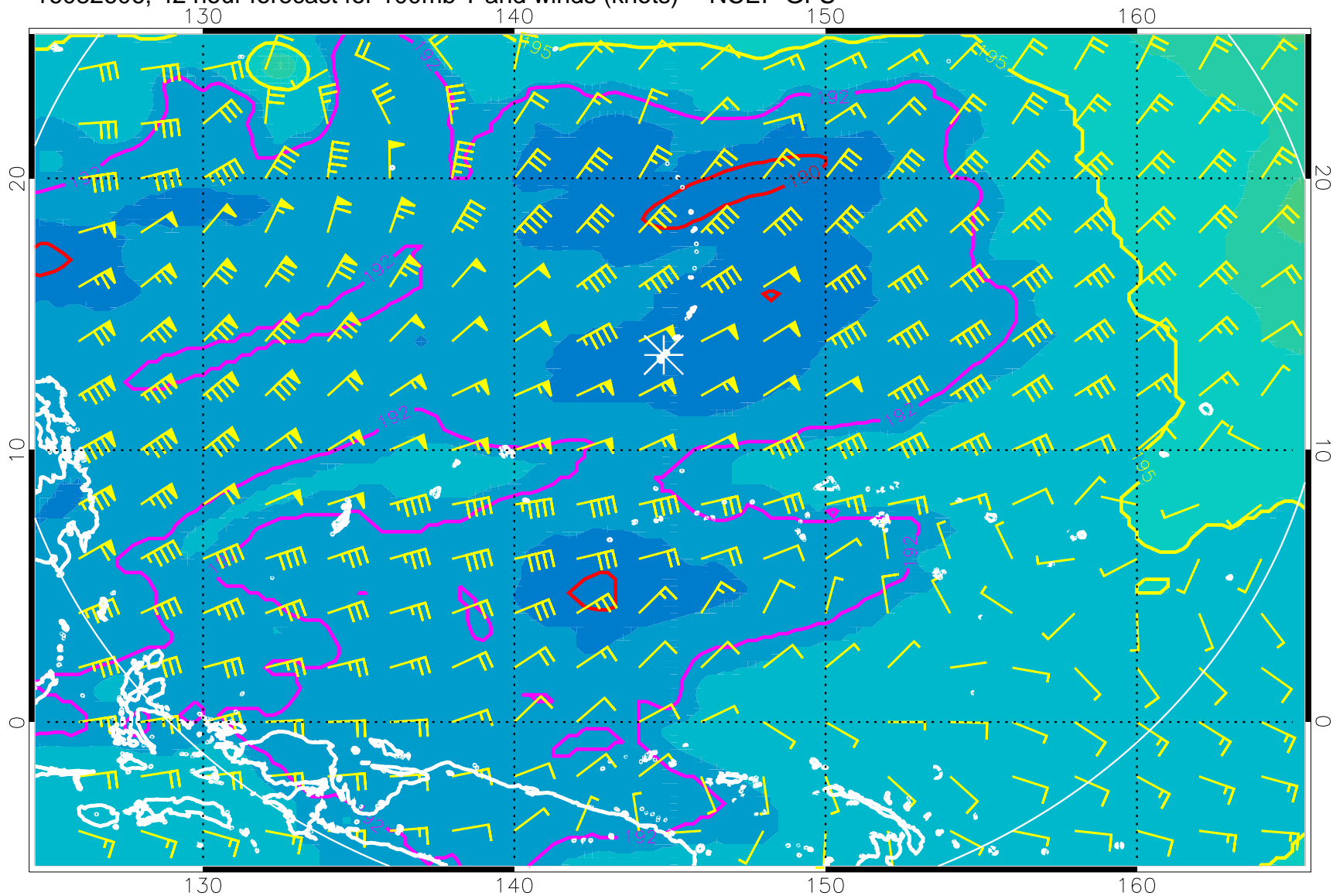
16082606, 42 hour forecast for 100mb T and winds (knots) -- NCEP GFS
