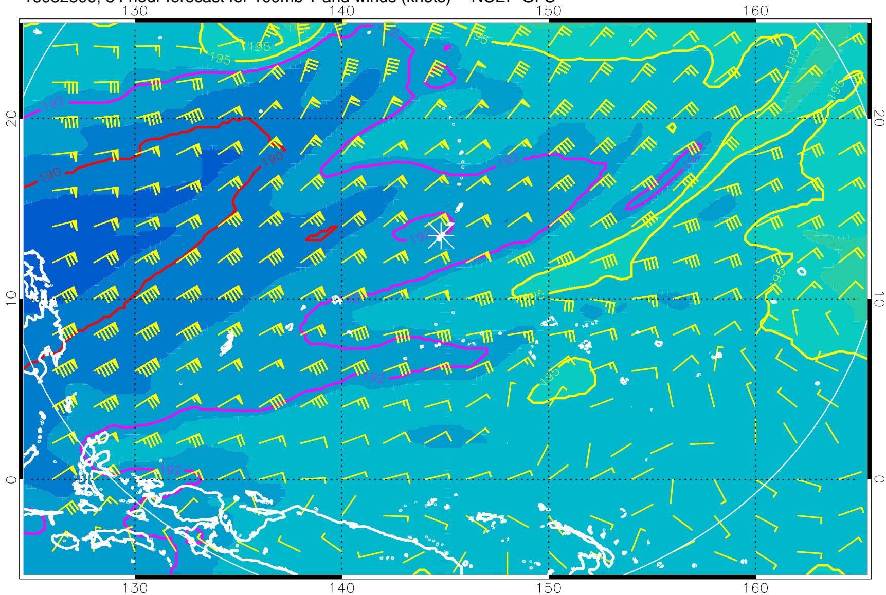
16082800, 84 hour forecast for 100mb T and winds (knots) -- NCEP GFS
