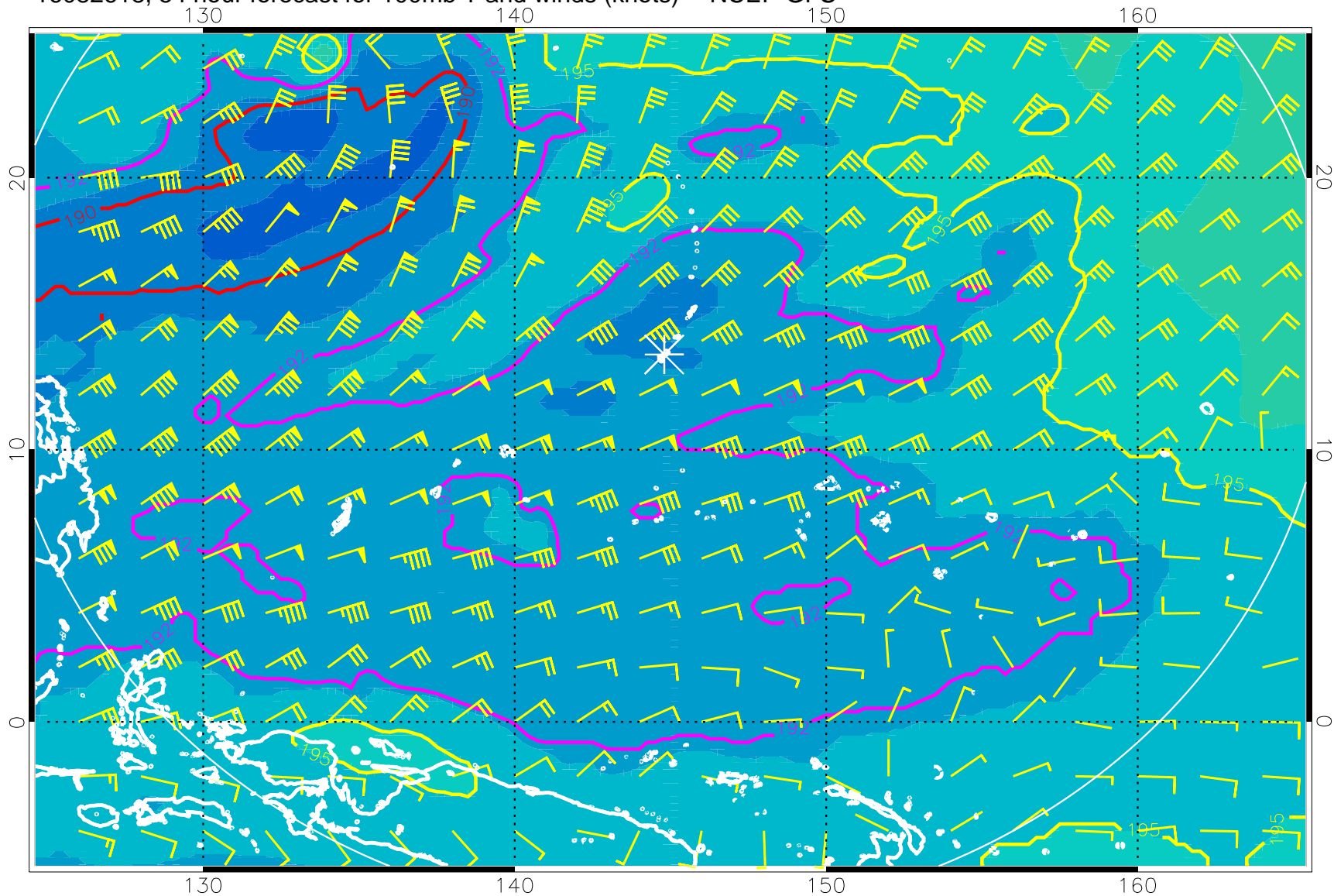
16082618, 54 hour forecast for 100mb T and winds (knots) -- NCEP GFS
