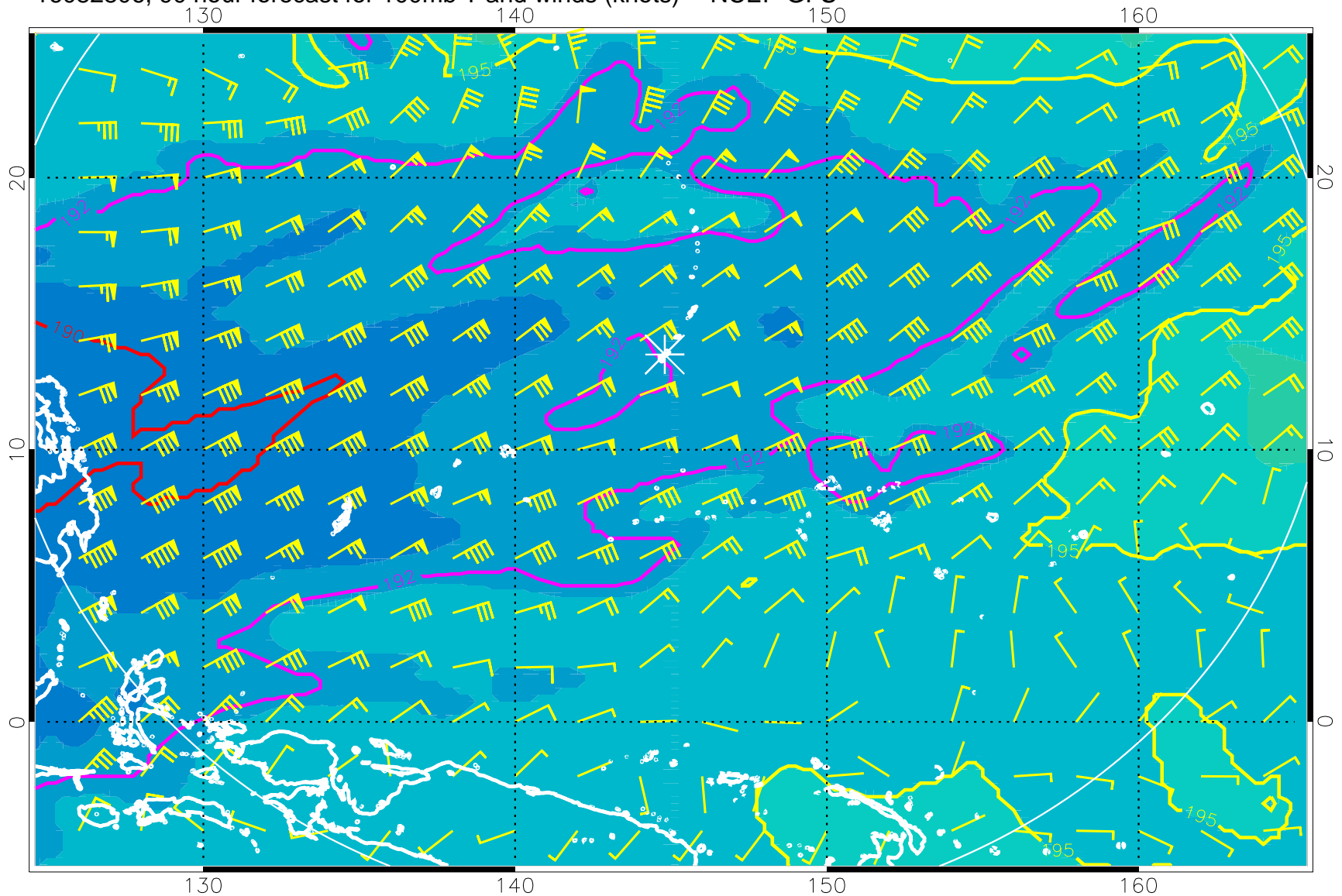
16082806, 90 hour forecast for 100mb T and winds (knots) -- NCEP GFS
