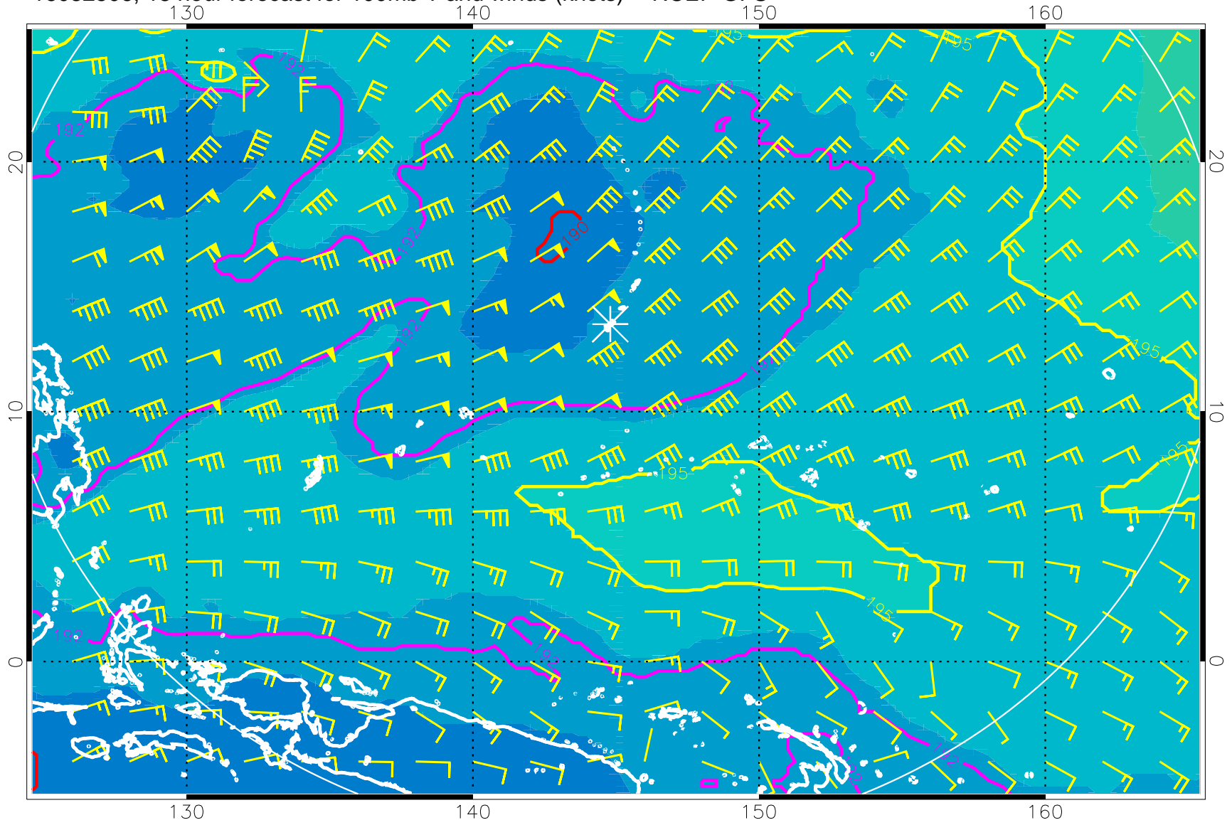
16082506, 18 hour forecast for 100mb T and winds (knots) -- NCEP GFS
