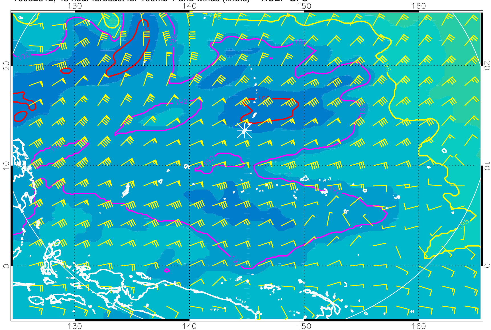
16082612, 48 hour forecast for 100mb T and winds (knots) -- NCEP GFS
