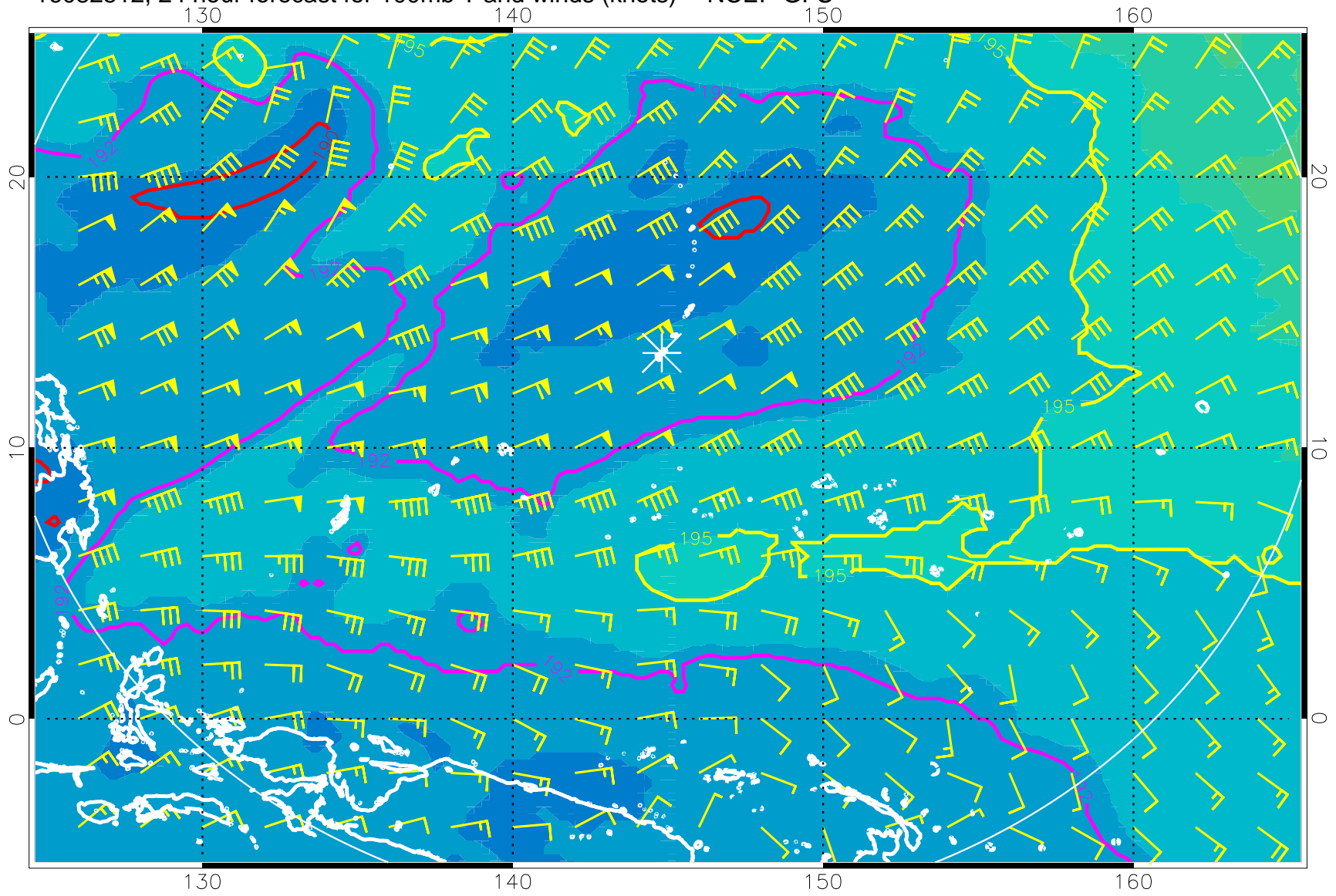
16082512, 24 hour forecast for 100mb T and winds (knots) -- NCEP GFS
