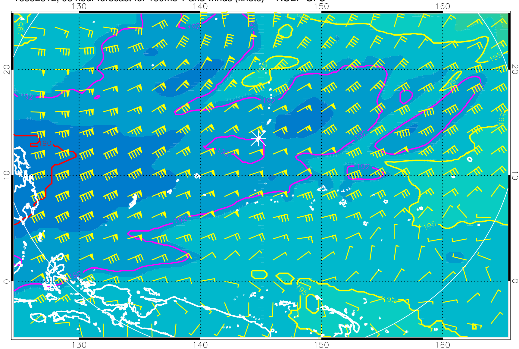
16082812, 96 hour forecast for 100mb T and winds (knots) -- NCEP GFS
