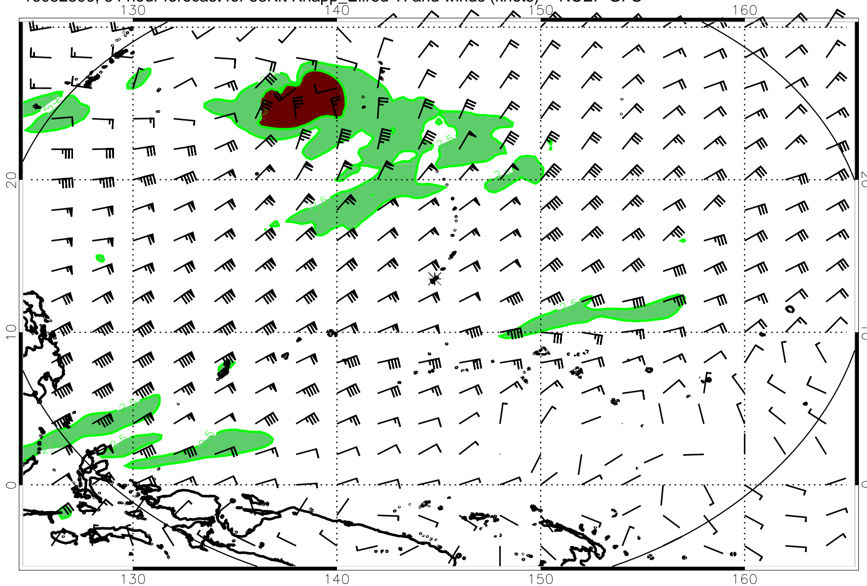
16082800, 84 hour forecast for 53Kft Knapp_Ellrod TI and winds (knots) -- NCEP GFS
