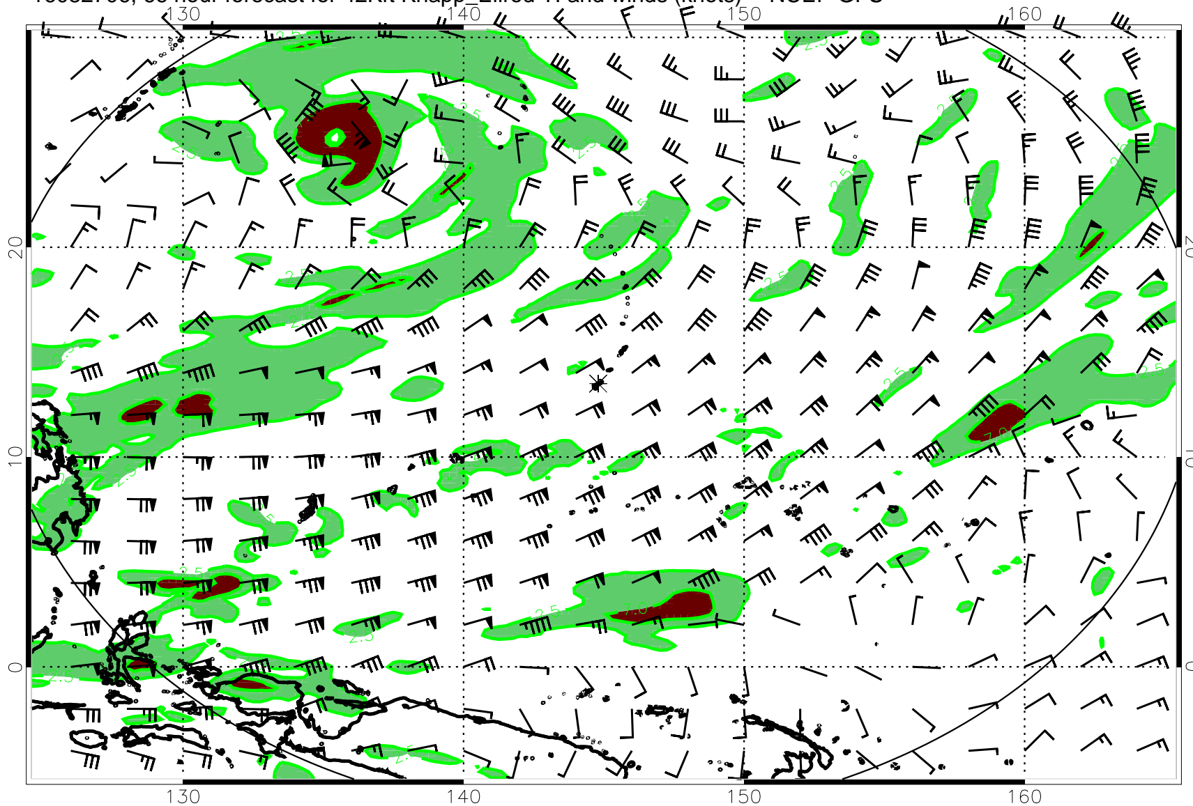
16082706, 66 hour forecast for 42Kft Knapp_Ellrod TI and winds (knots) -- NCEP GFS
