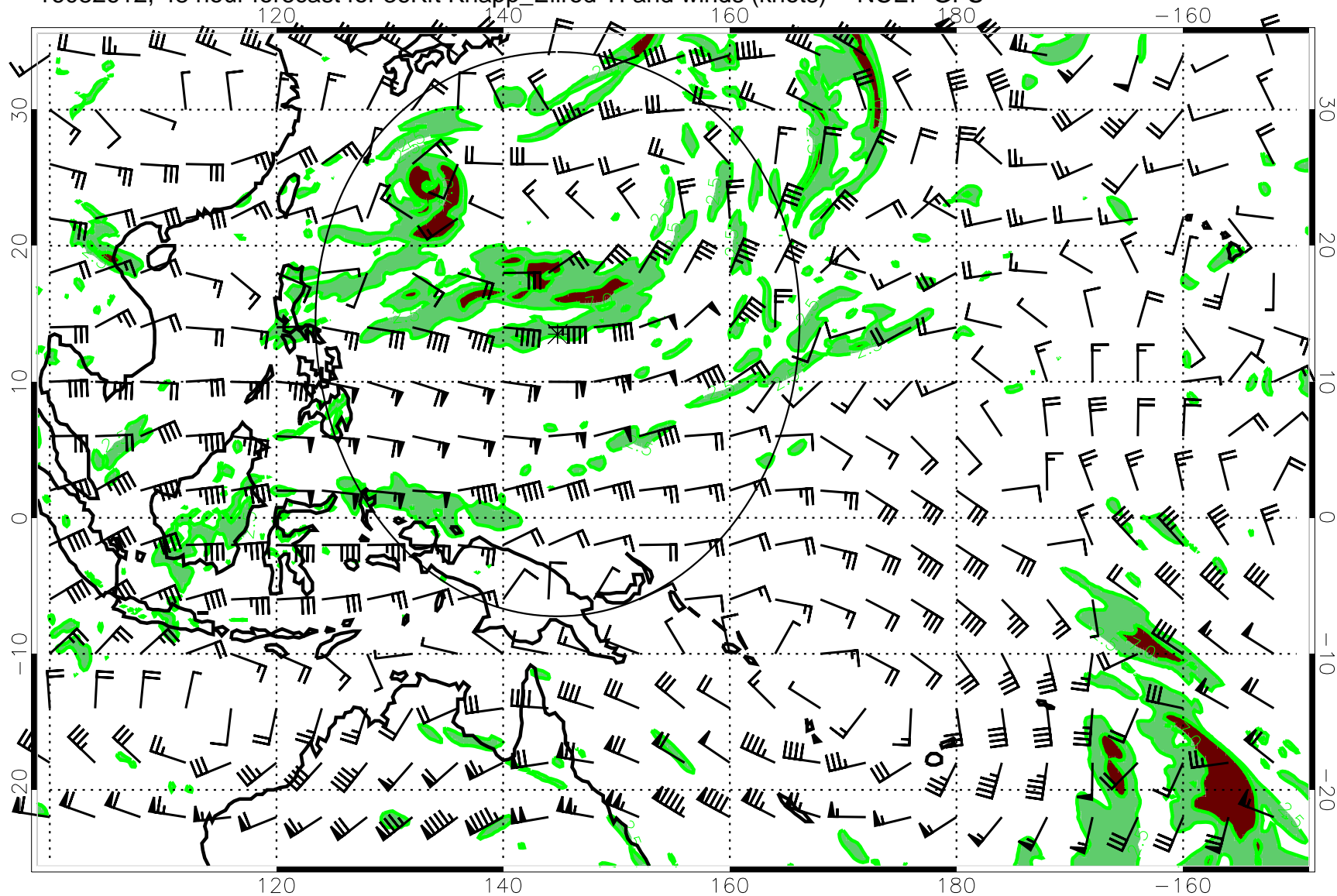
16082612, 48 hour forecast for 36Kft Knapp_Ellrod TI and winds (knots) -- NCEP GFS
