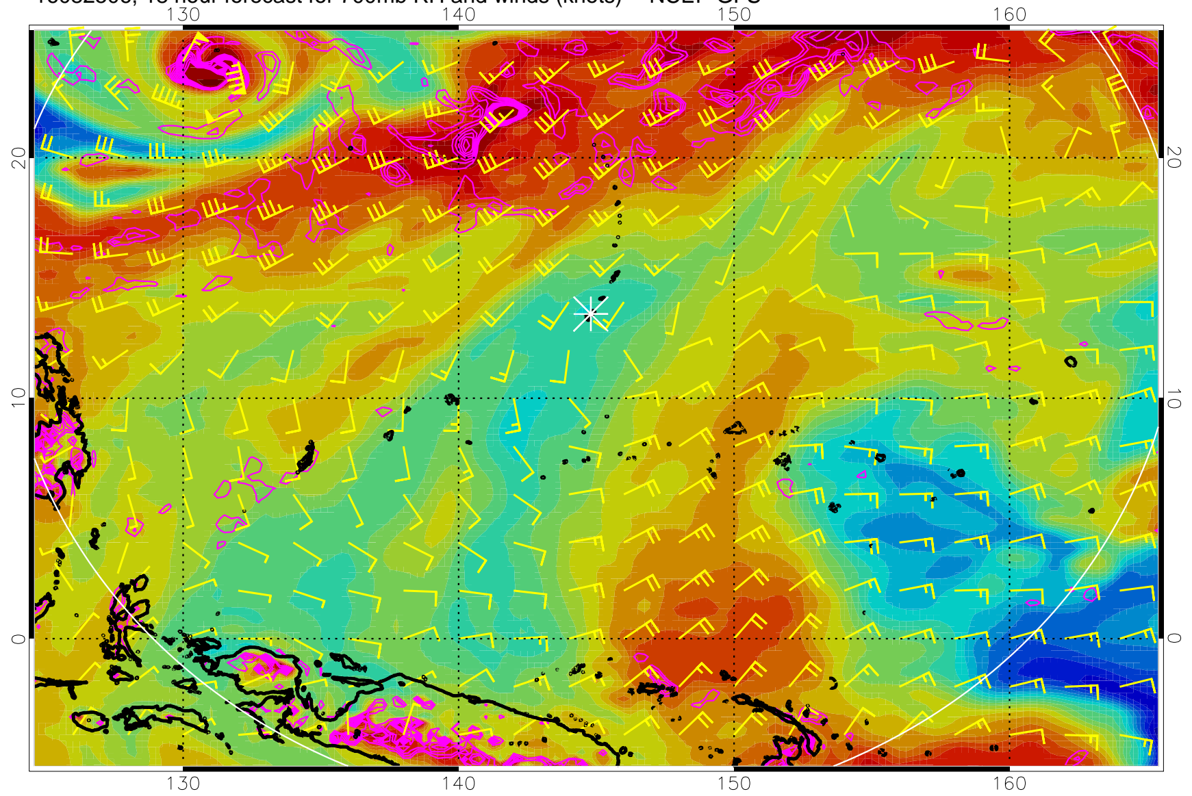
16082506, 18 hour forecast for 700mb RH and winds (knots) -- NCEP GFS
