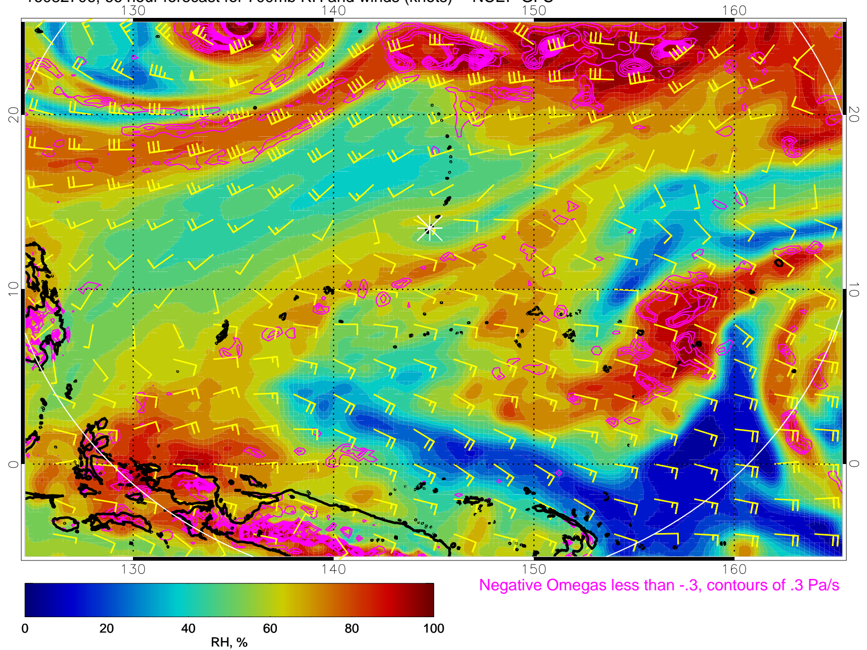
16082706, 66 hour forecast for 700mb RH and winds (knots) -- NCEP GFS
