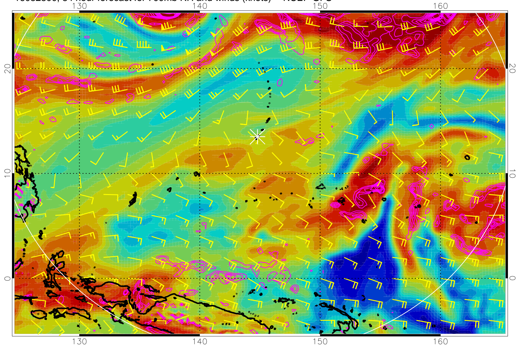
16082800, 84 hour forecast for 700mb RH and winds (knots) -- NCEP GFS
