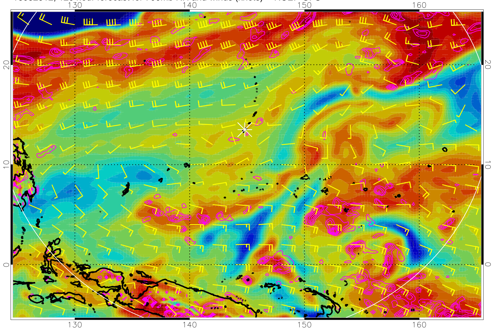
16082912, 120 hour forecast for 700mb RH and winds (knots) -- NCEP GFS
