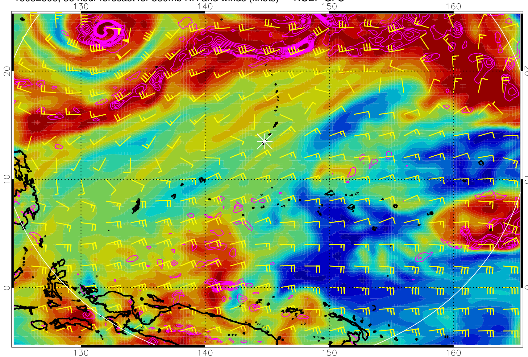
16082600, 36 hour forecast for 500mb RH and winds (knots) -- NCEP GFS
