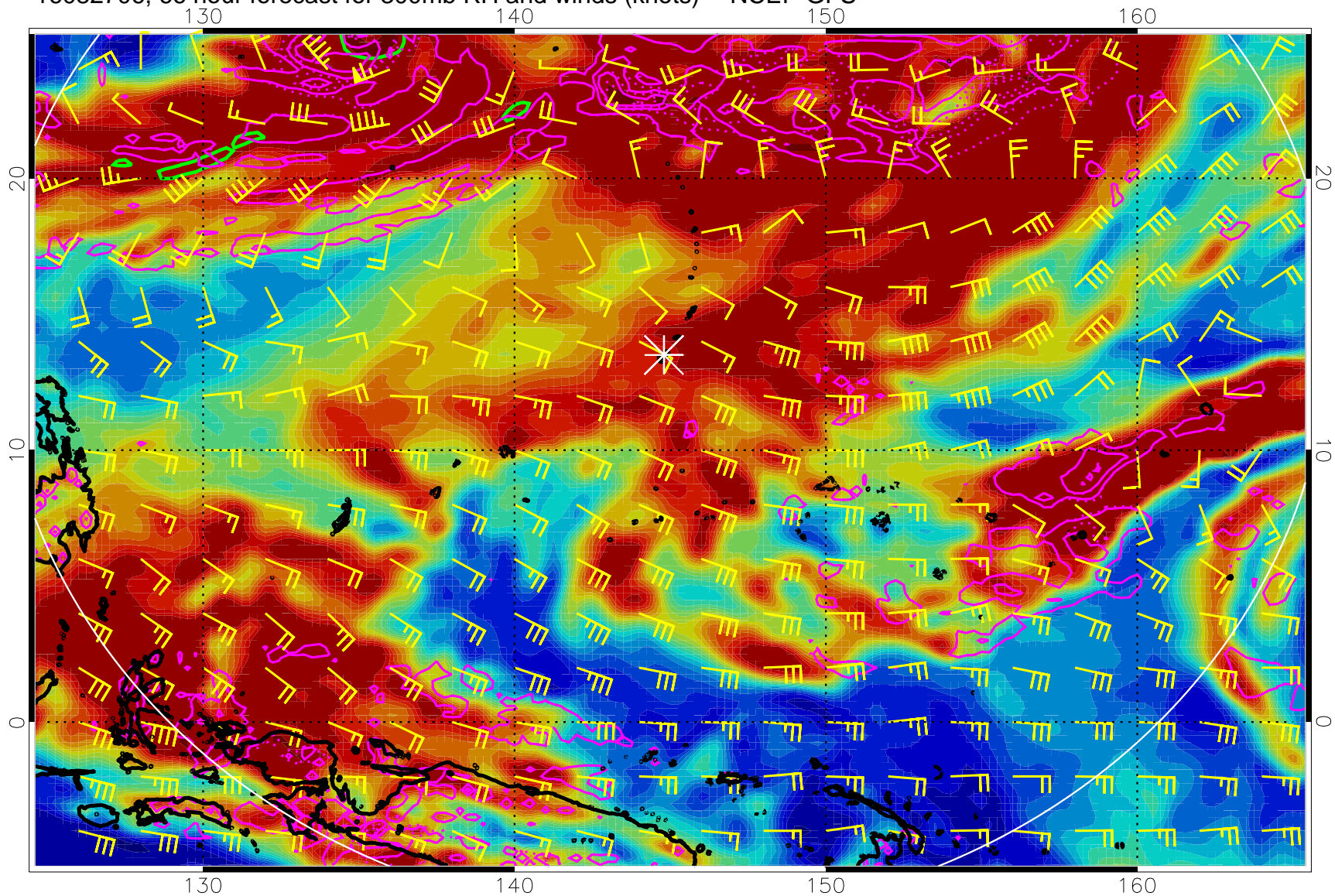
16082706, 66 hour forecast for 300mb RH and winds (knots) -- NCEP GFS
