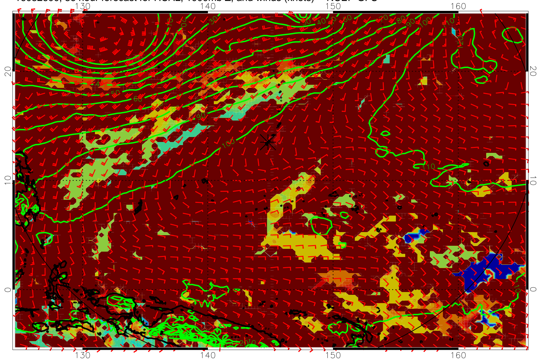
16082600, 36 hour forecast for HCAL, 1000mb Z, and winds (knots) -- NCEP GFS
