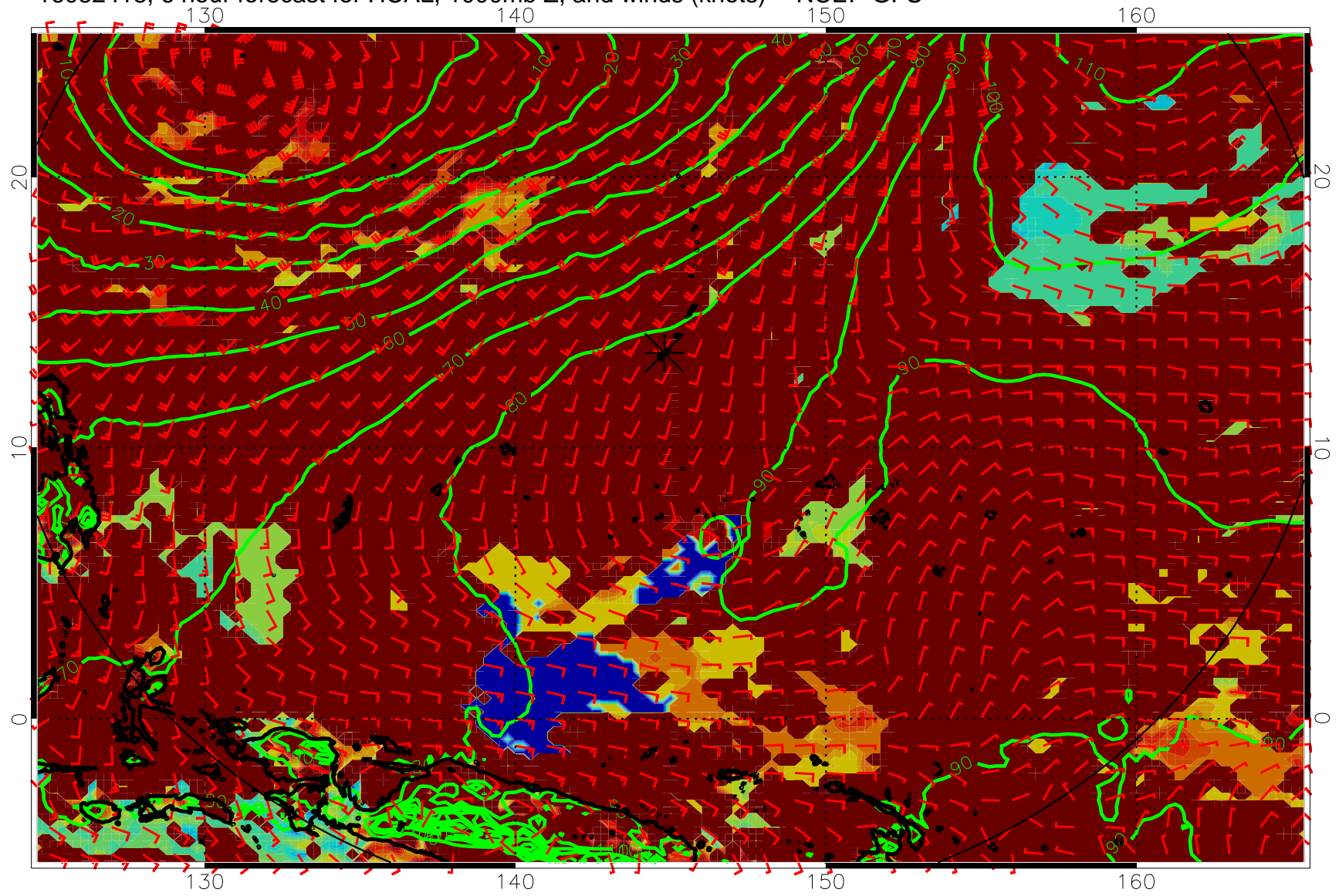
16082418, 6 hour forecast for HCAL, 1000mb Z, and winds (knots) -- NCEP GFS
