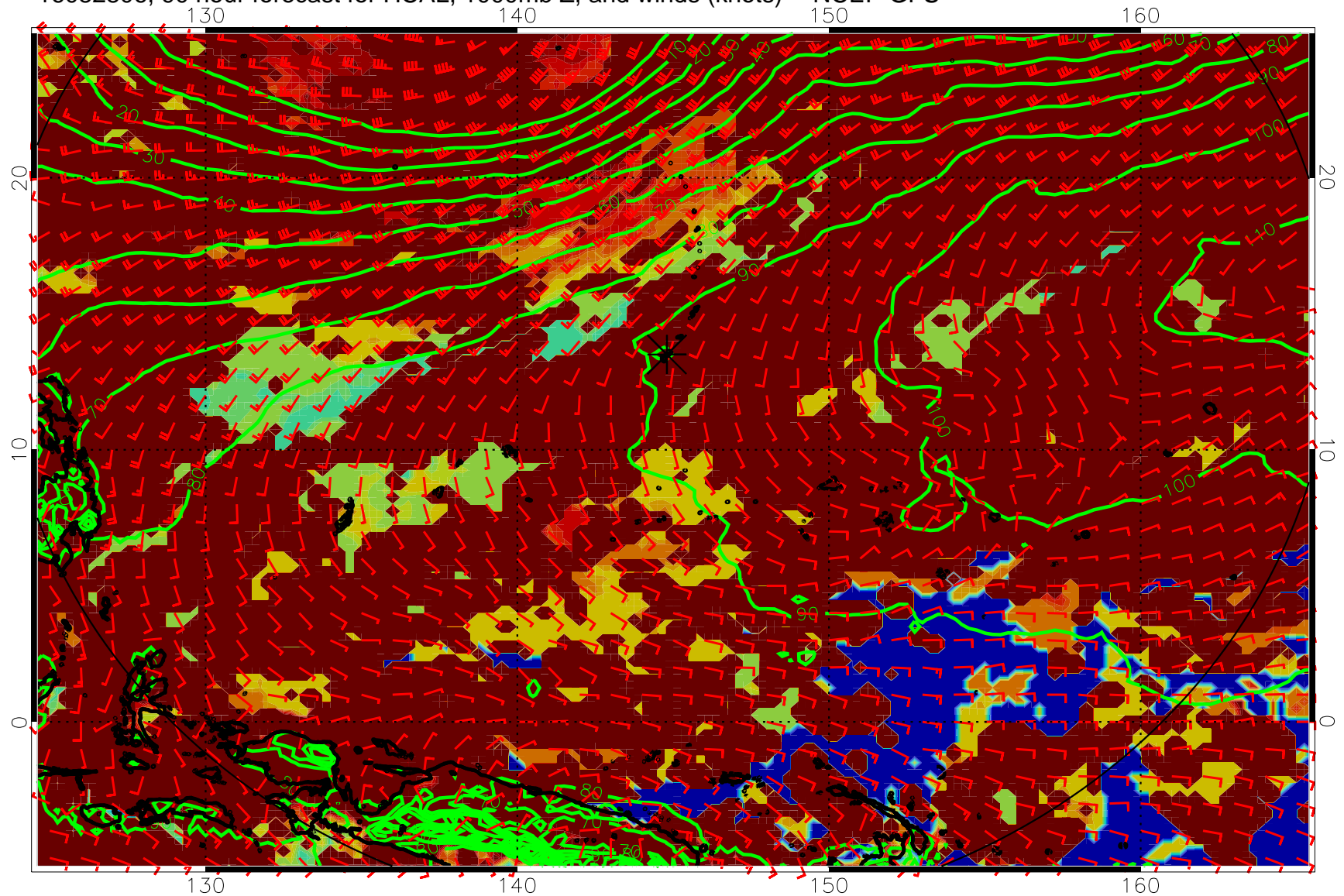
16082806, 90 hour forecast for HCAL, 1000mb Z, and winds (knots) -- NCEP GFS
