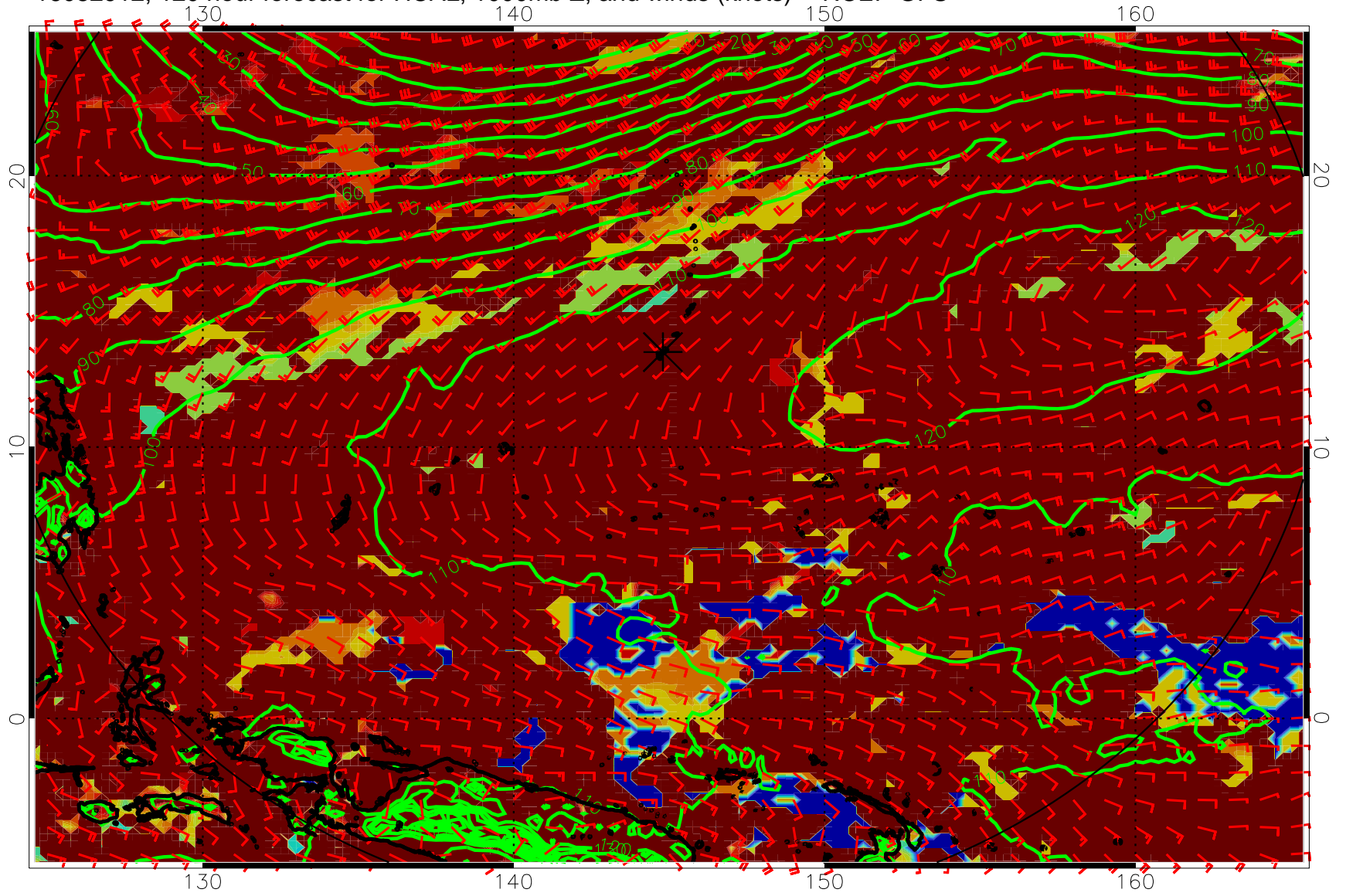
16082912, 120 hour forecast for HCAL, 1000mb Z, and winds (knots) -- NCEP GFS
