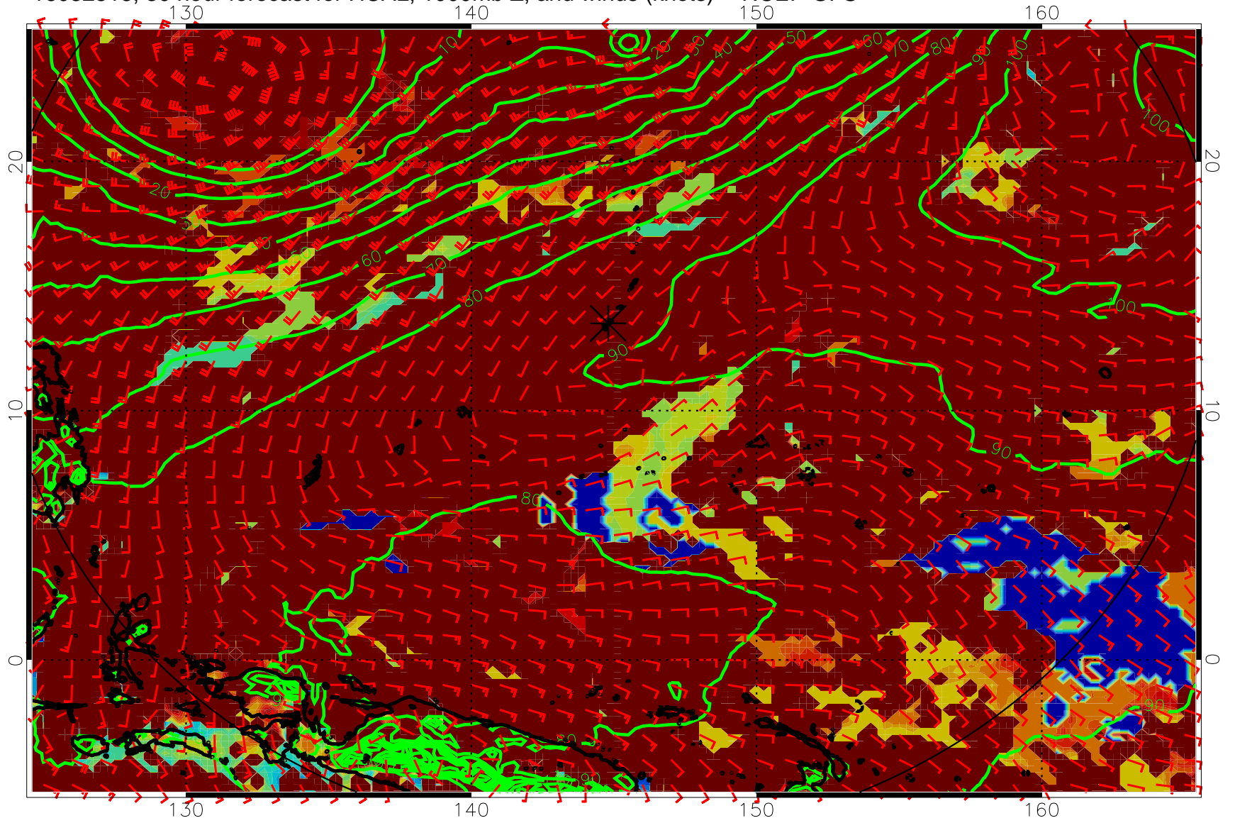
16082518, 30 hour forecast for HCAL, 1000mb Z, and winds (knots) -- NCEP GFS
