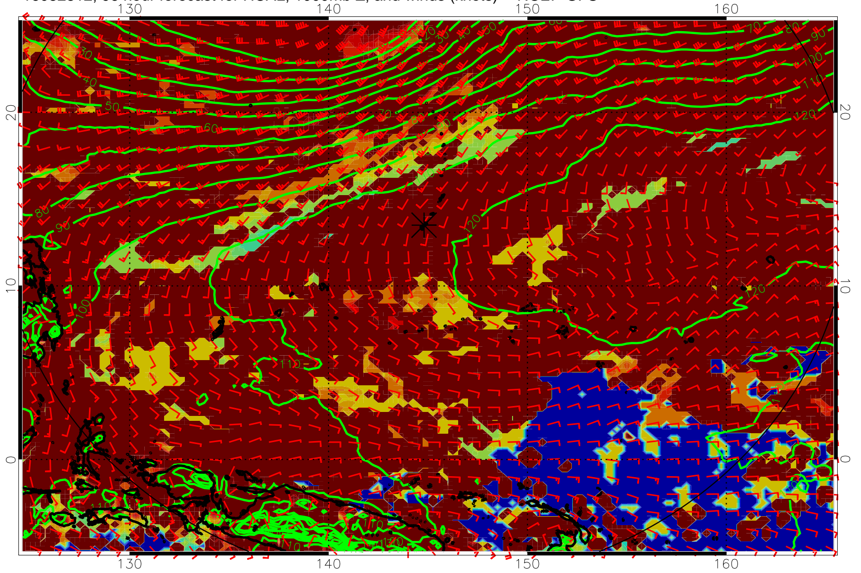
16082812, 96 hour forecast for HCAL, 1000mb Z, and winds (knots) -- NCEP GFS
