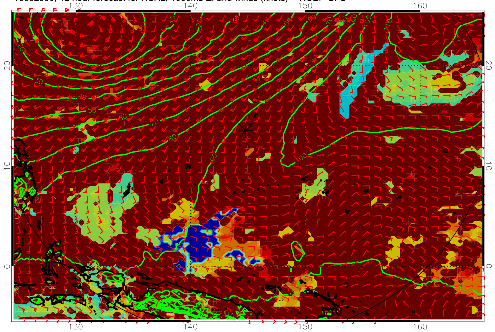
16082500, 12 hour forecast for HCAL, 1000mb Z, and winds (knots) -- NCEP GFS
