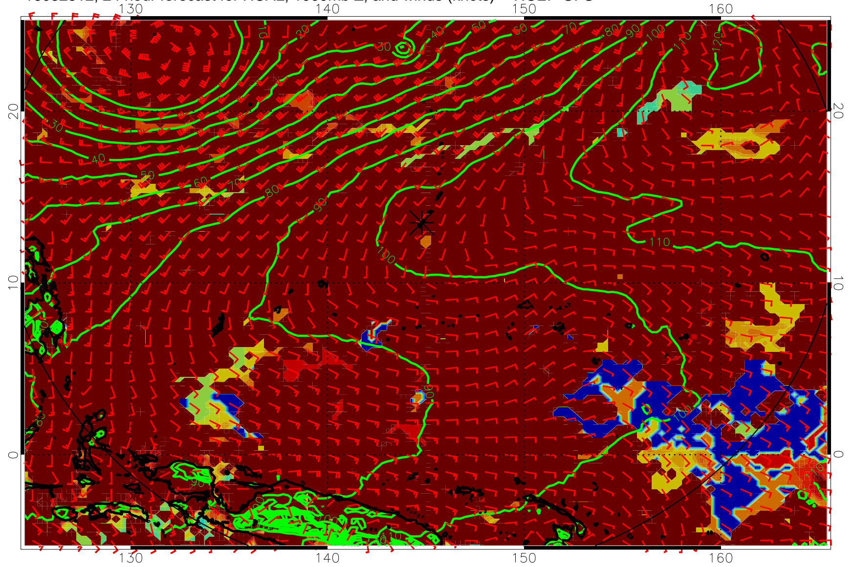
16082512, 24 hour forecast for HCAL, 1000mb Z, and winds (knots) -- NCEP GFS
