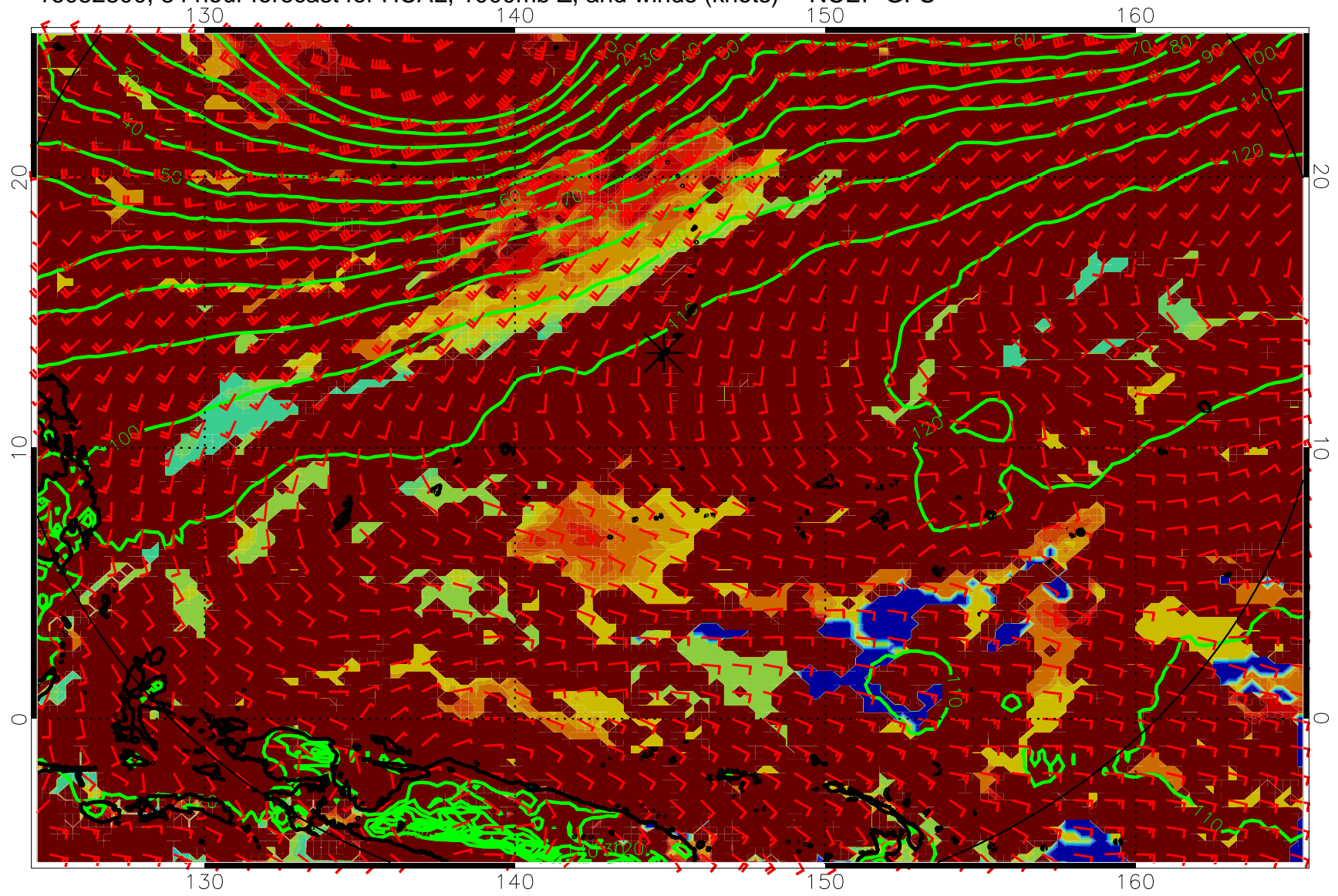
16082800, 84 hour forecast for HCAL, 1000mb Z, and winds (knots) -- NCEP GFS
