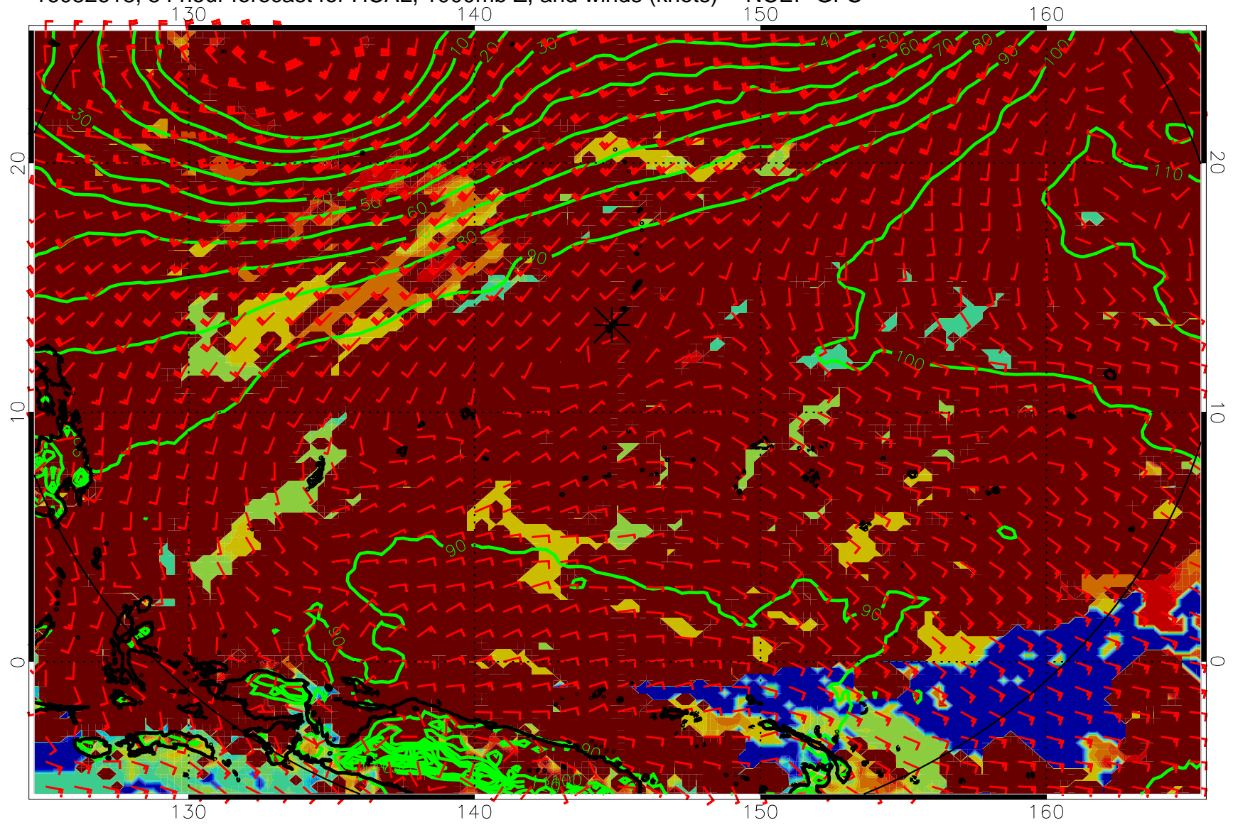
16082618, 54 hour forecast for HCAL, 1000mb Z, and winds (knots) -- NCEP GFS
