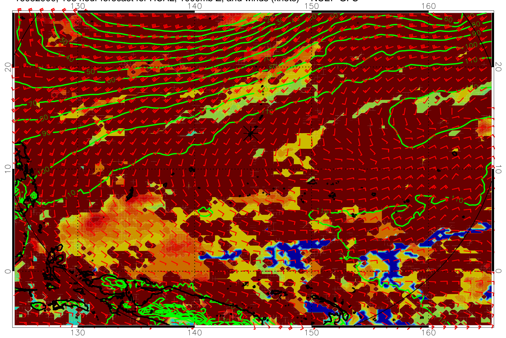
16082900, 108 hour forecast for HCAL, 1000mb Z, and winds (knots) -- NCEP GFS
