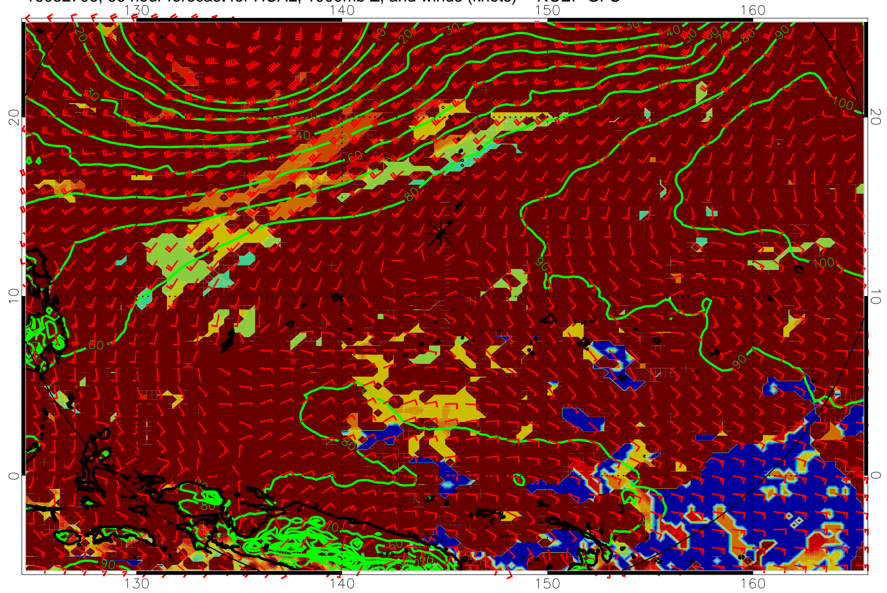
16082706, 66 hour forecast for HCAL, 1000mb Z, and winds (knots) -- NCEP GFS
