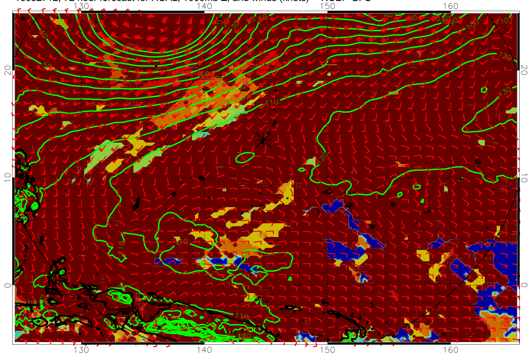
16082712, 72 hour forecast for HCAL, 1000mb Z, and winds (knots) -- NCEP GFS
