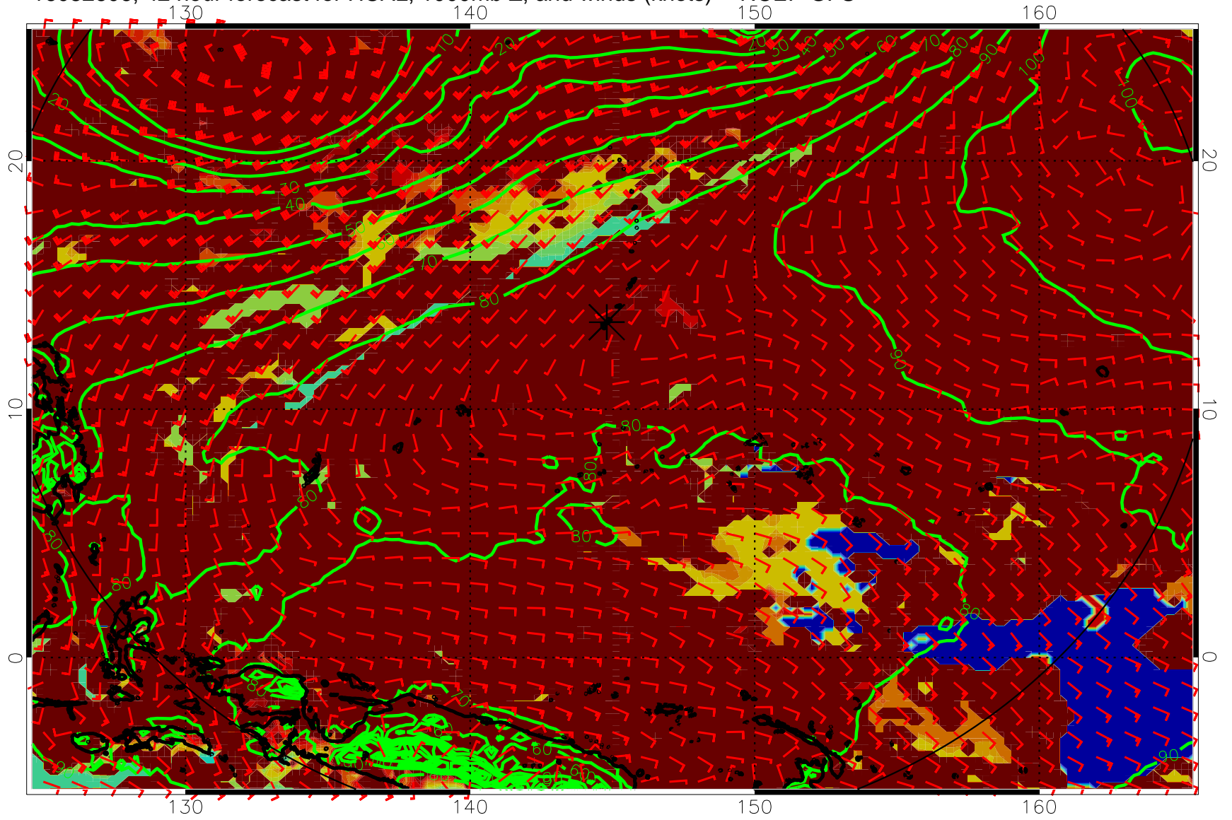
16082606, 42 hour forecast for HCAL, 1000mb Z, and winds (knots) -- NCEP GFS
