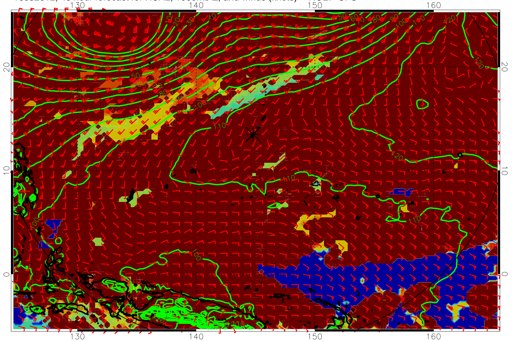
16082612, 48 hour forecast for HCAL, 1000mb Z, and winds (knots) -- NCEP GFS
