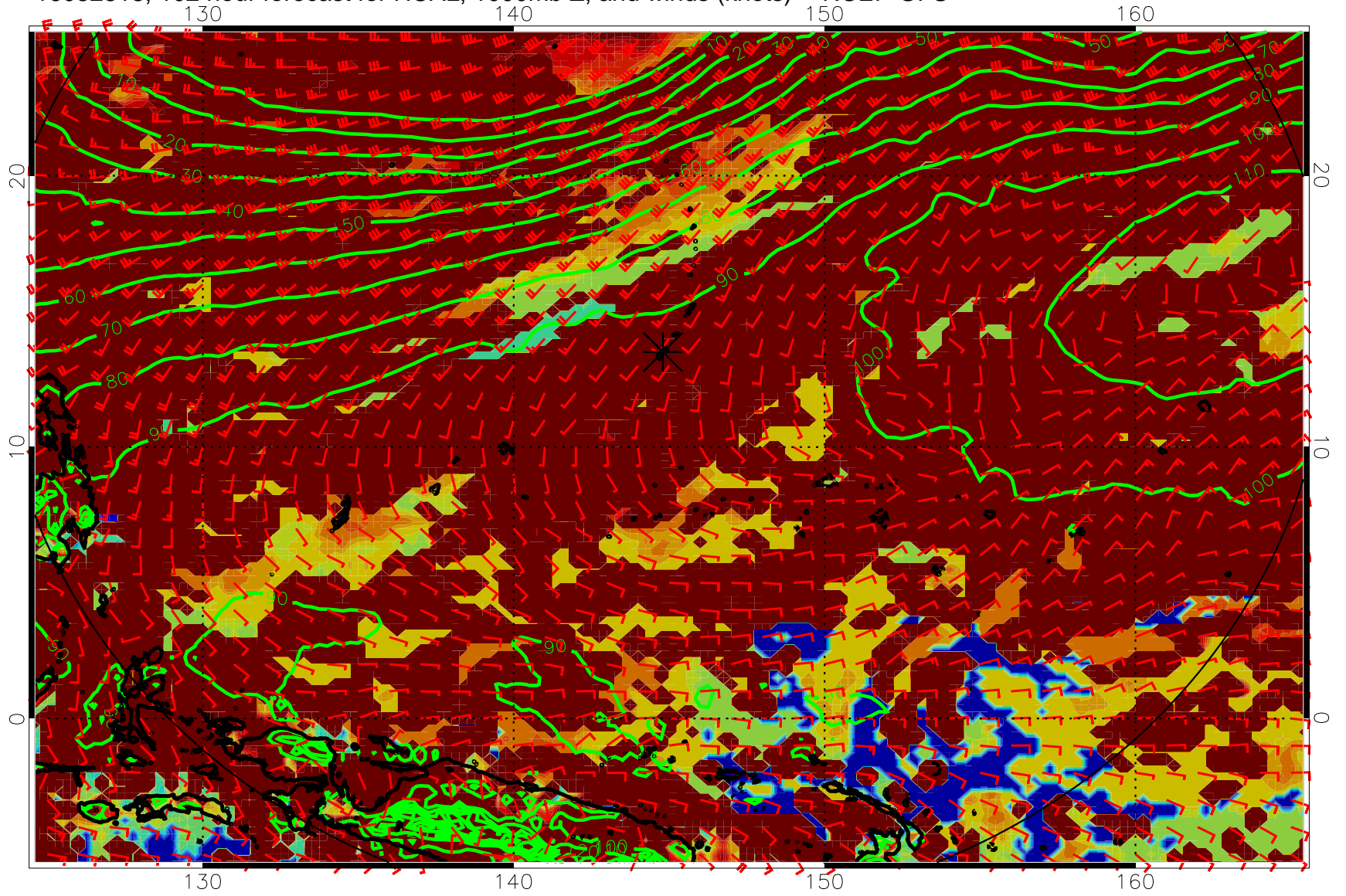
16082818, 102 hour forecast for HCAL, 1000mb Z, and winds (knots) -- NCEP GFS
