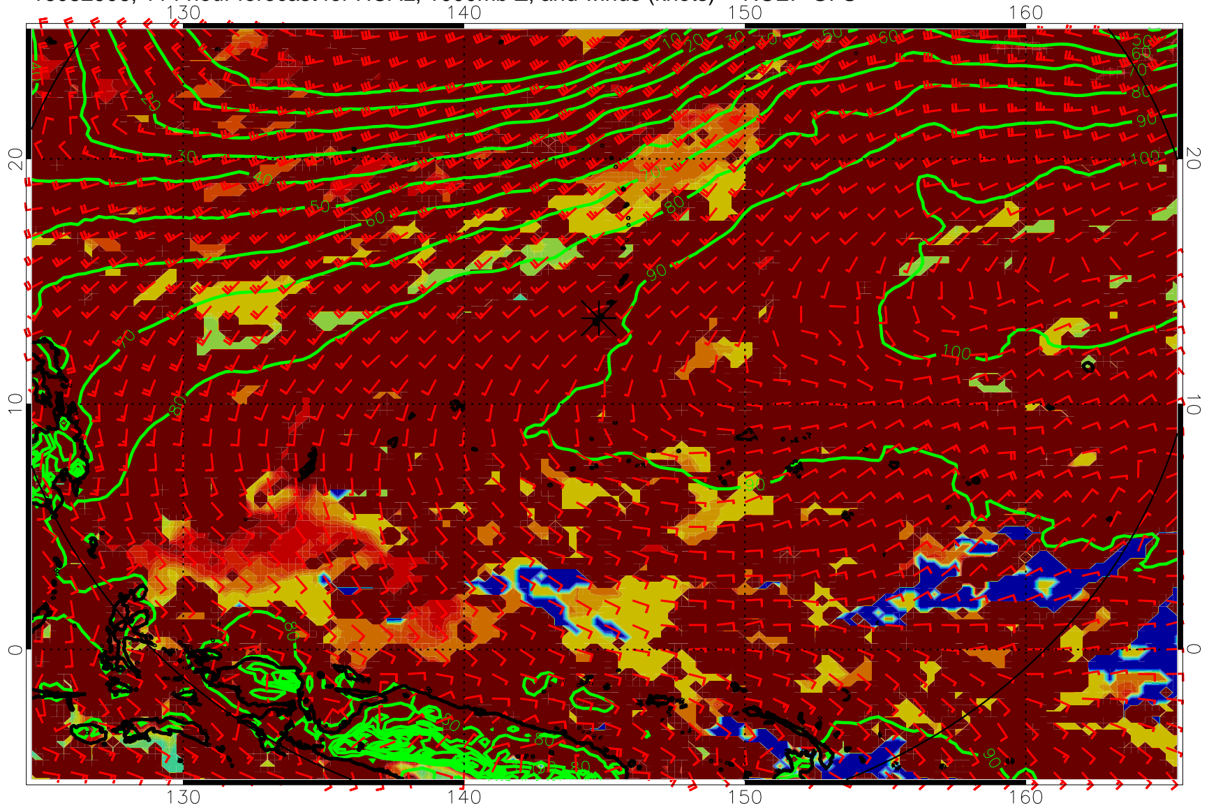
16082906, 114 hour forecast for HCAL, 1000mb Z, and winds (knots) -- NCEP GFS
