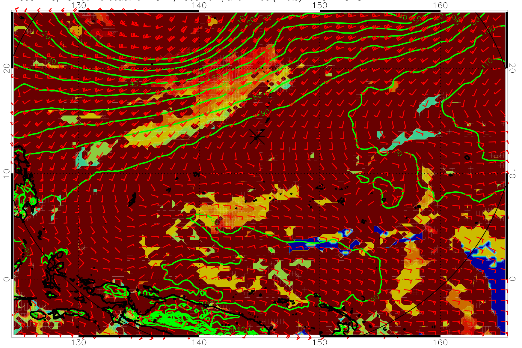
16082718, 78 hour forecast for HCAL, 1000mb Z, and winds (knots) -- NCEP GFS
