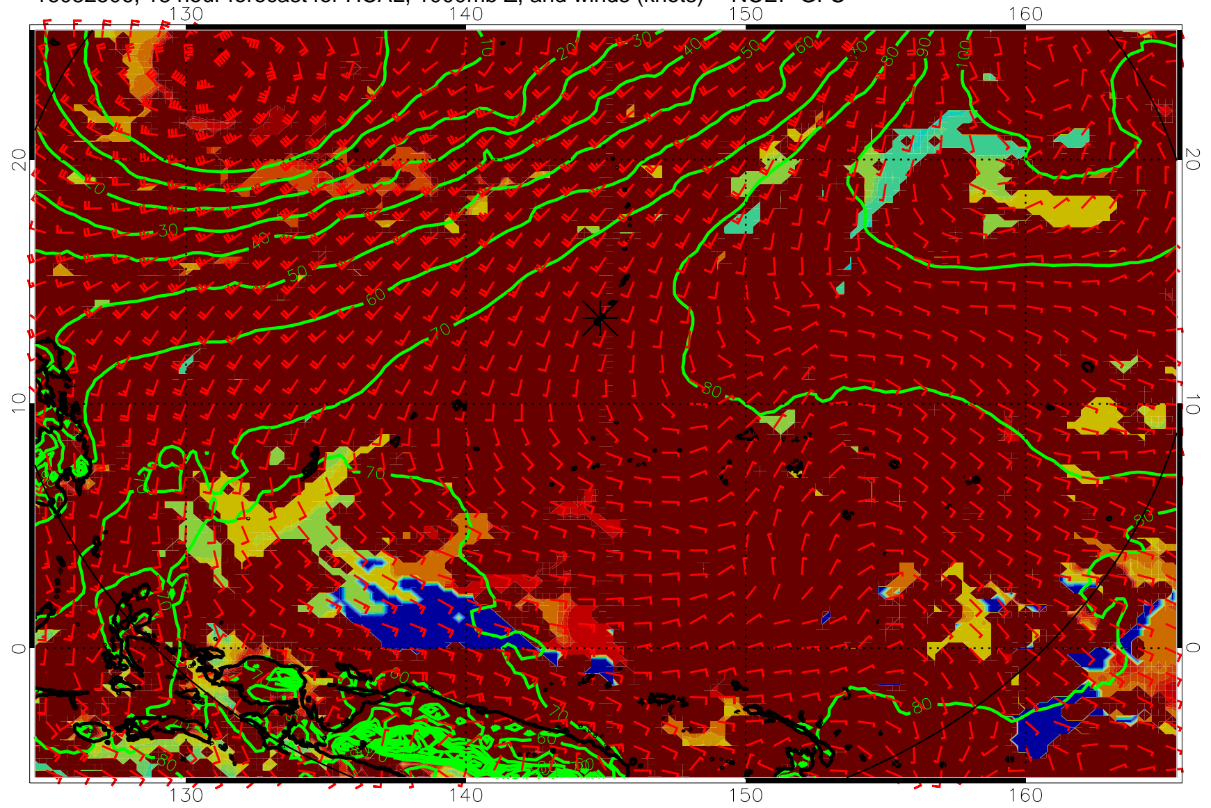
16082506, 18 hour forecast for HCAL, 1000mb Z, and winds (knots) -- NCEP GFS
