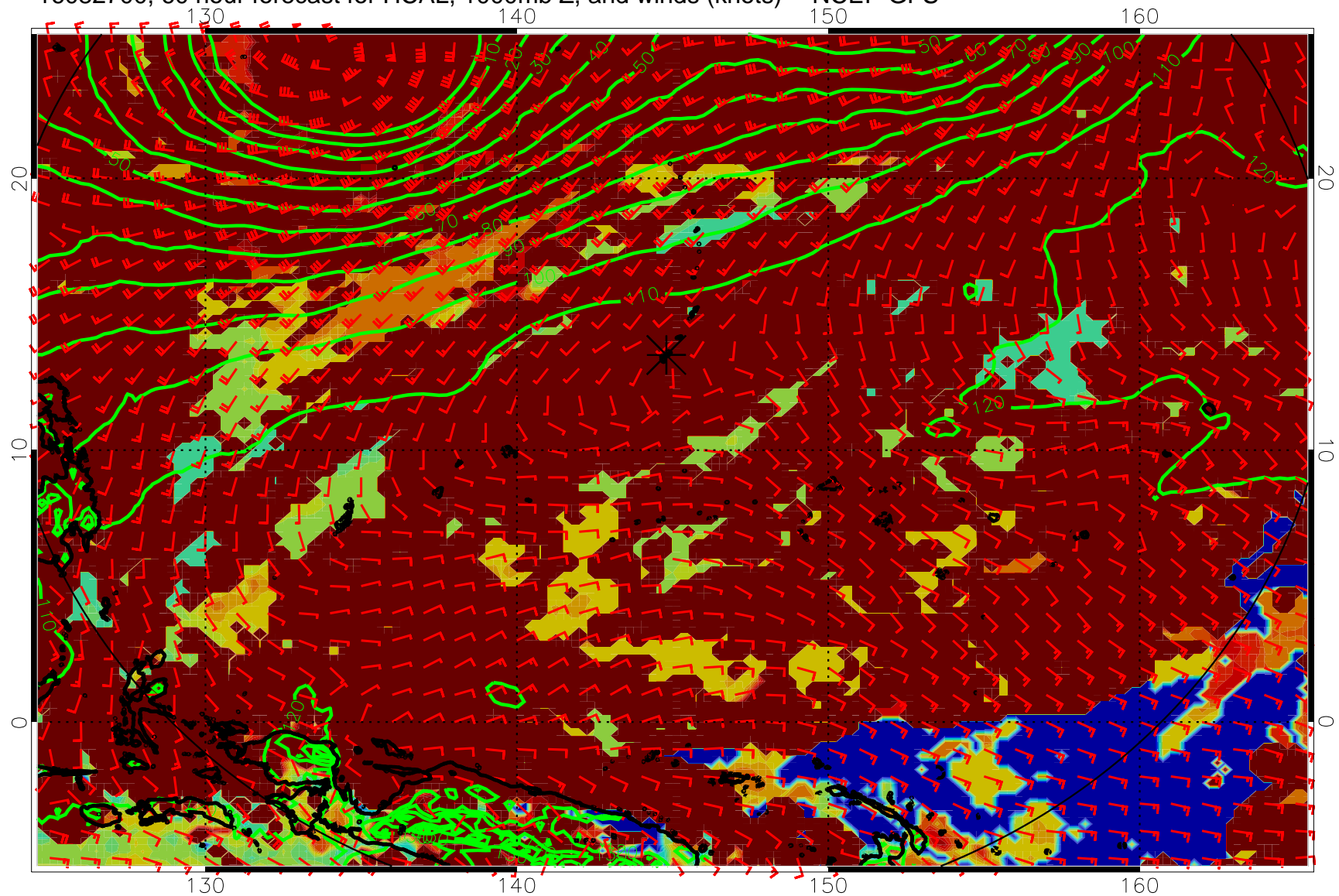
16082700, 60 hour forecast for HCAL, 1000mb Z, and winds (knots) -- NCEP GFS
