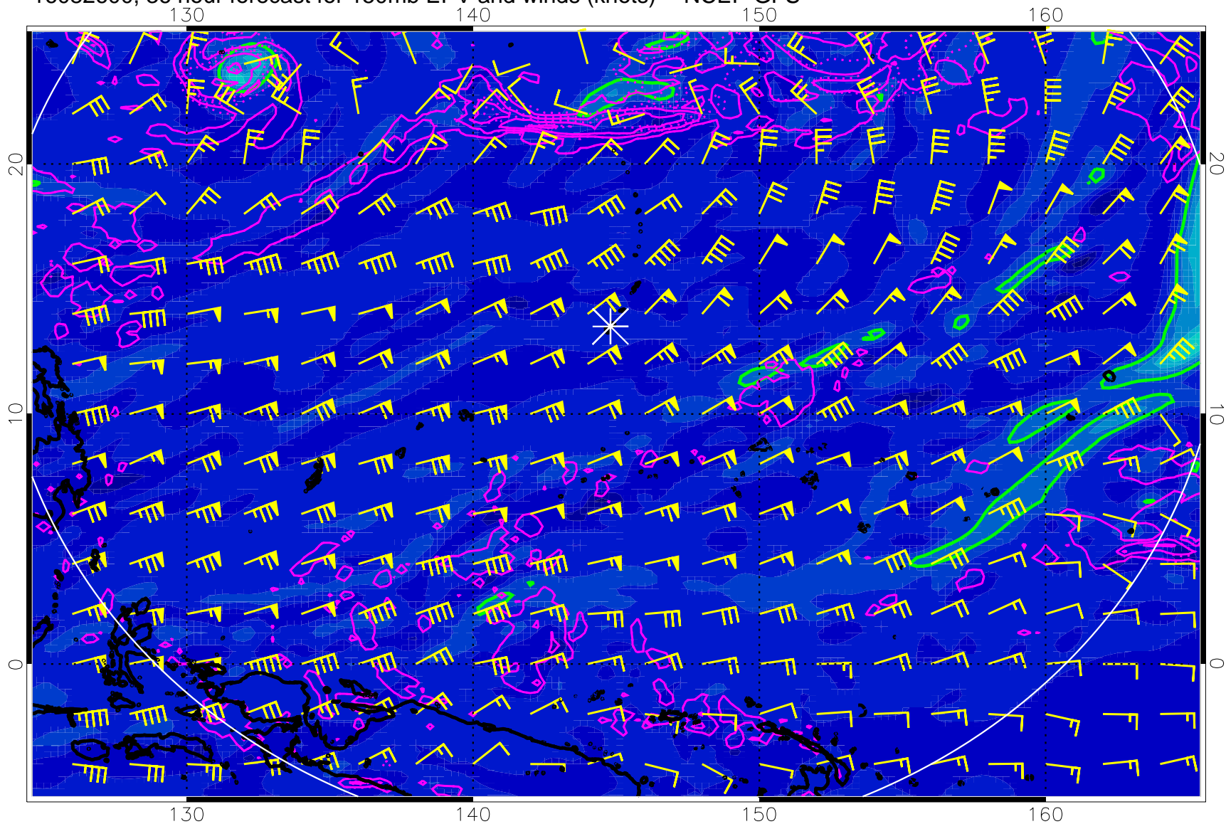
16082600, 36 hour forecast for 150mb EPV and winds (knots) -- NCEP GFS
