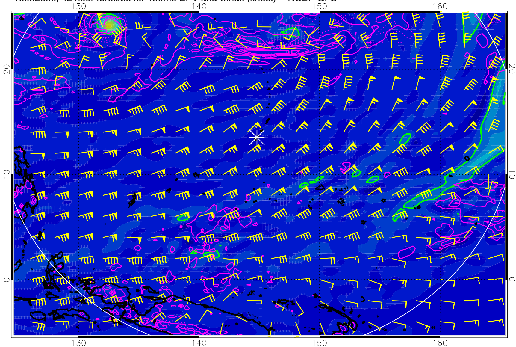
16082606, 42 hour forecast for 150mb EPV and winds (knots) -- NCEP GFS
