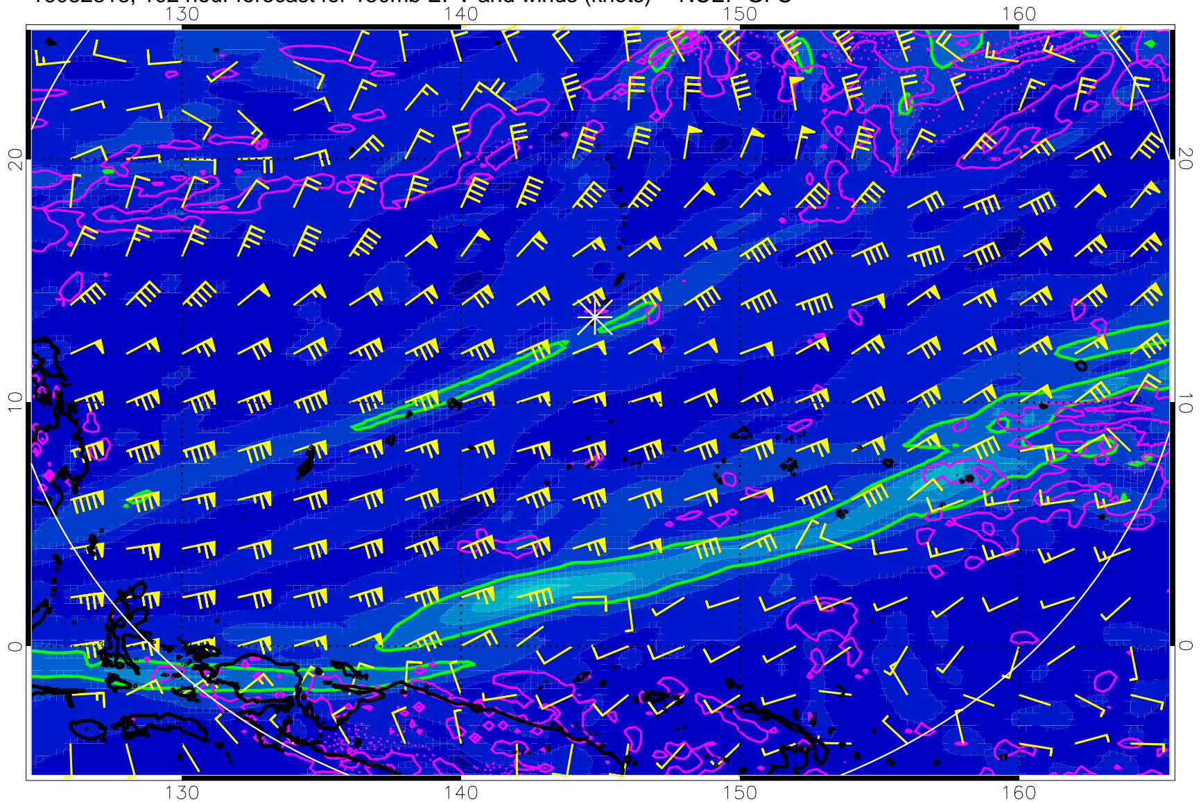
16082818, 102 hour forecast for 150mb EPV and winds (knots) -- NCEP GFS
