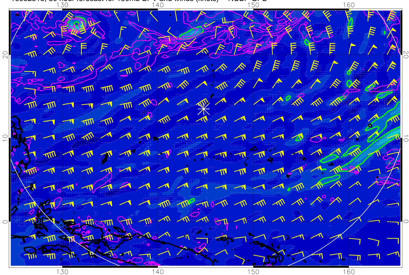
16082518, 30 hour forecast for 150mb EPV and winds (knots) -- NCEP GFS
