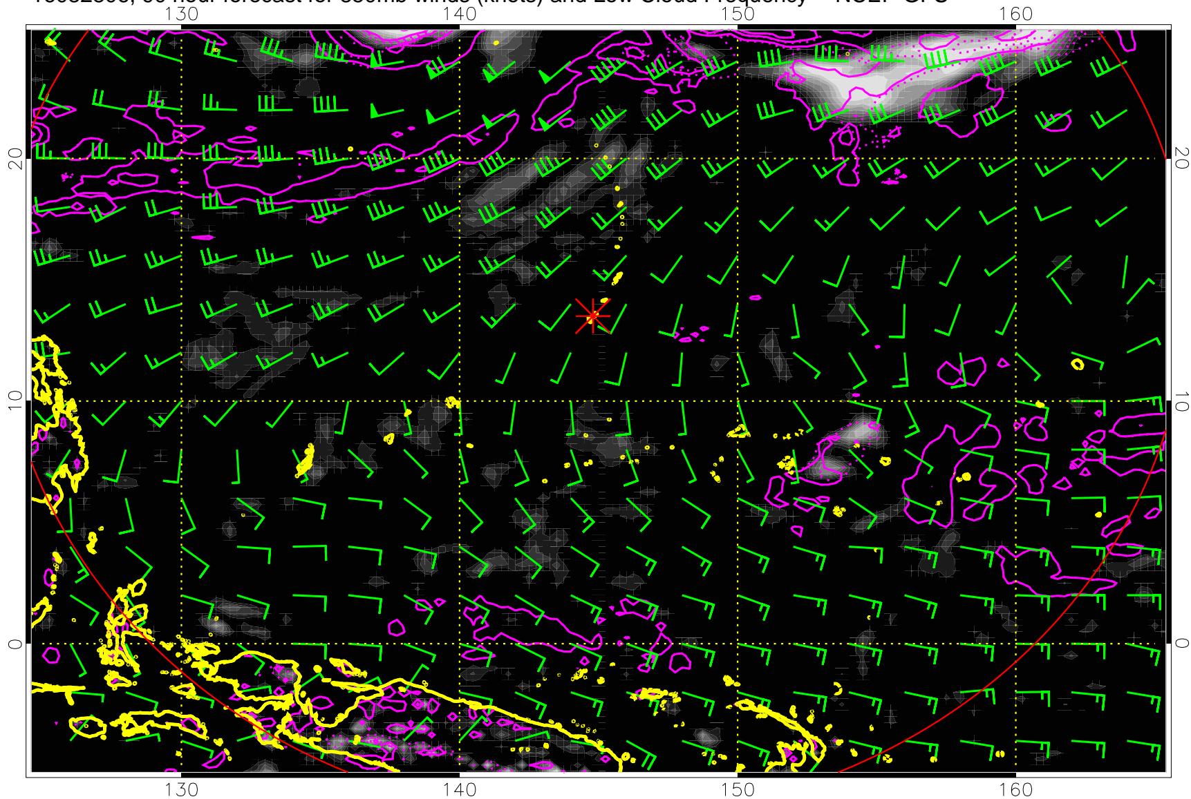
16082806, 90 hour forecast for 850mb winds (knots) and Low Cloud Frequency -- NCEP GFS
