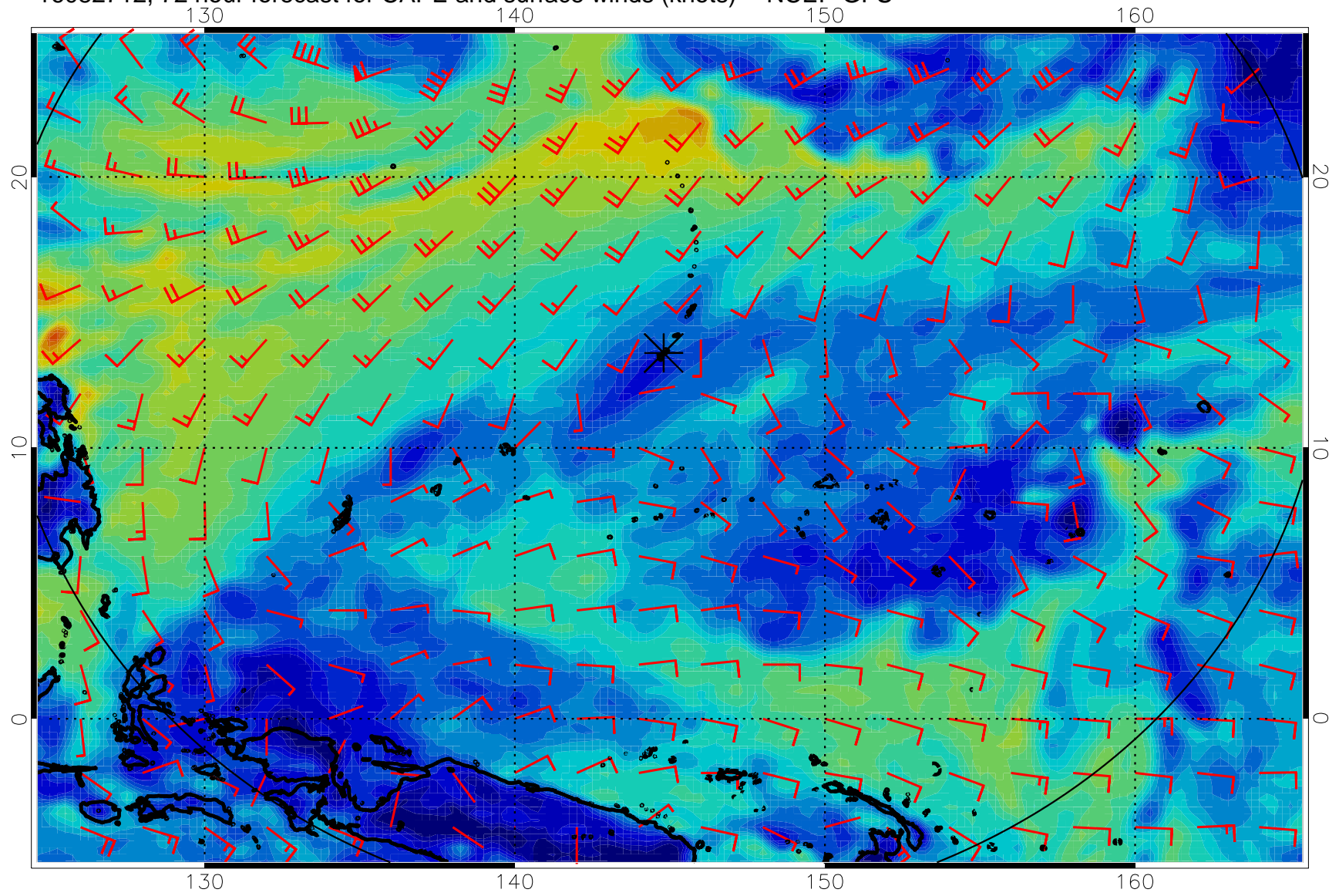
16082712, 72 hour forecast for CAPE and surface winds (knots) -- NCEP GFS
