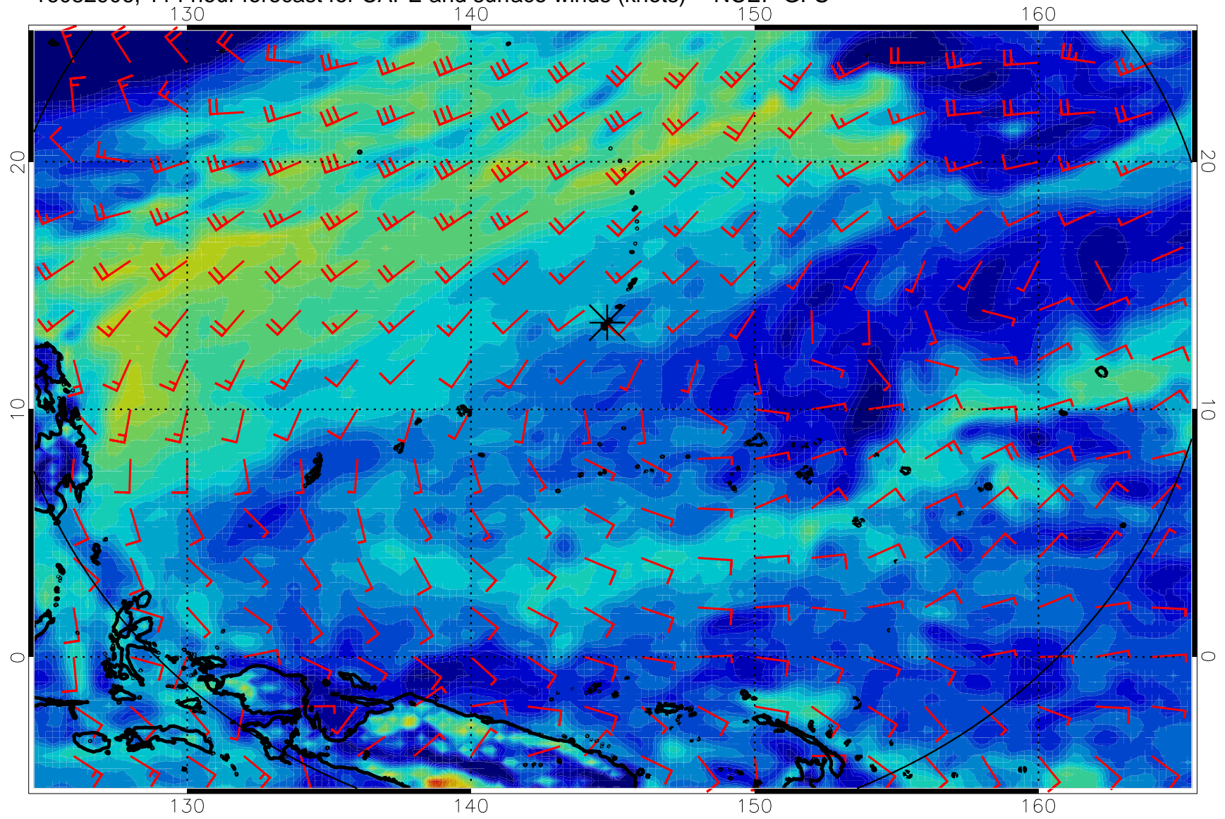
16082906, 114 hour forecast for CAPE and surface winds (knots) -- NCEP GFS
