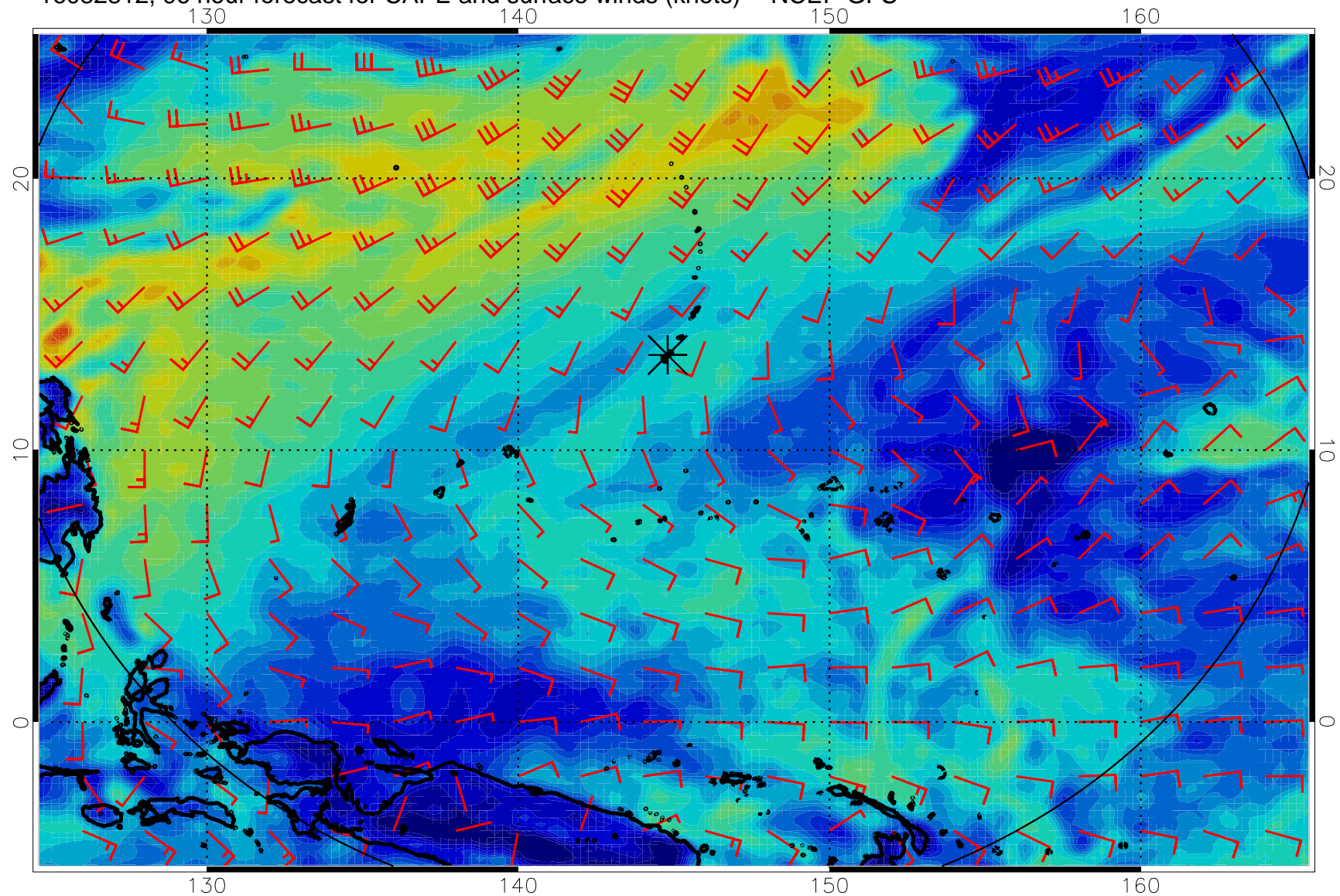
16082812, 96 hour forecast for CAPE and surface winds (knots) -- NCEP GFS
