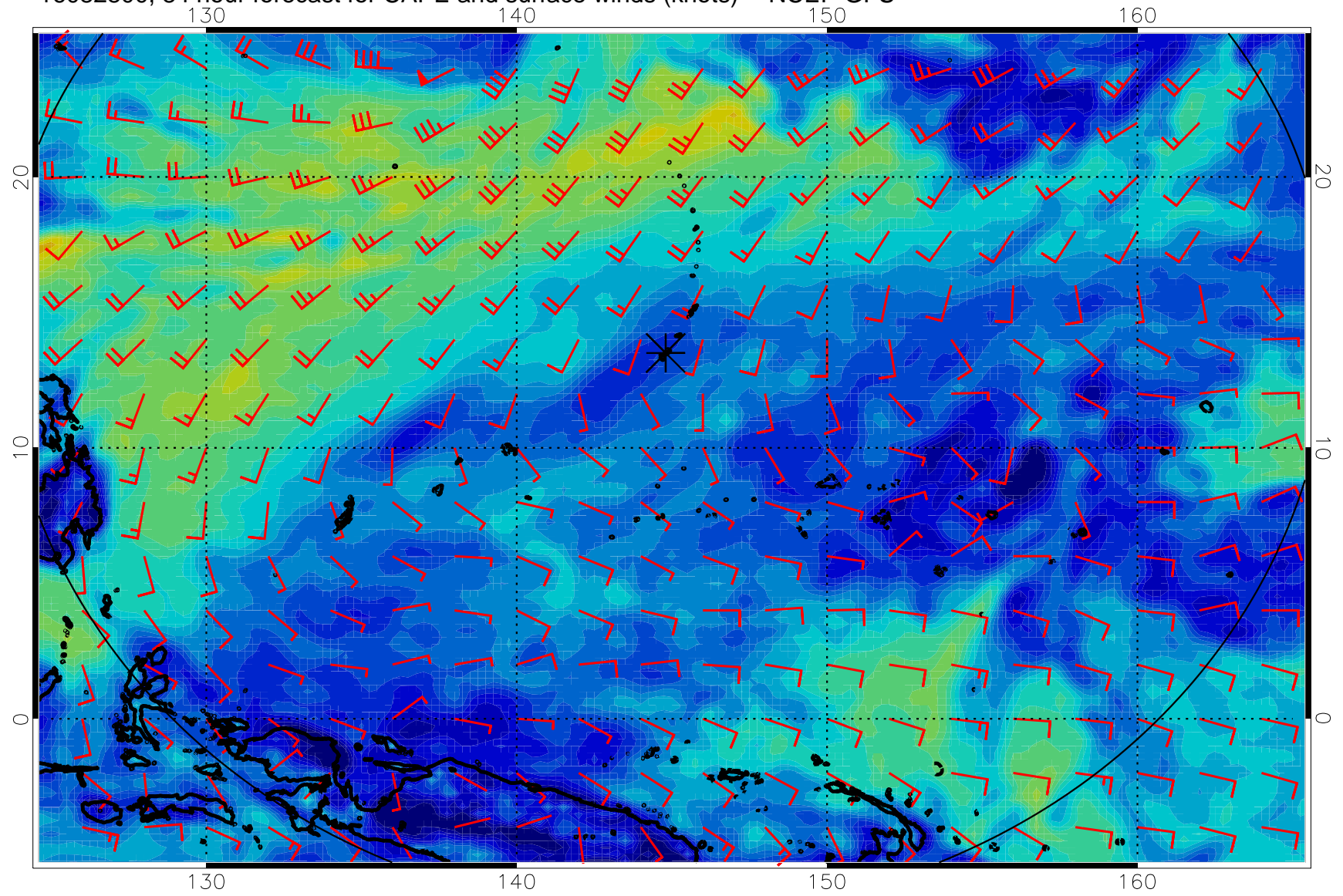
16082800, 84 hour forecast for CAPE and surface winds (knots) -- NCEP GFS
