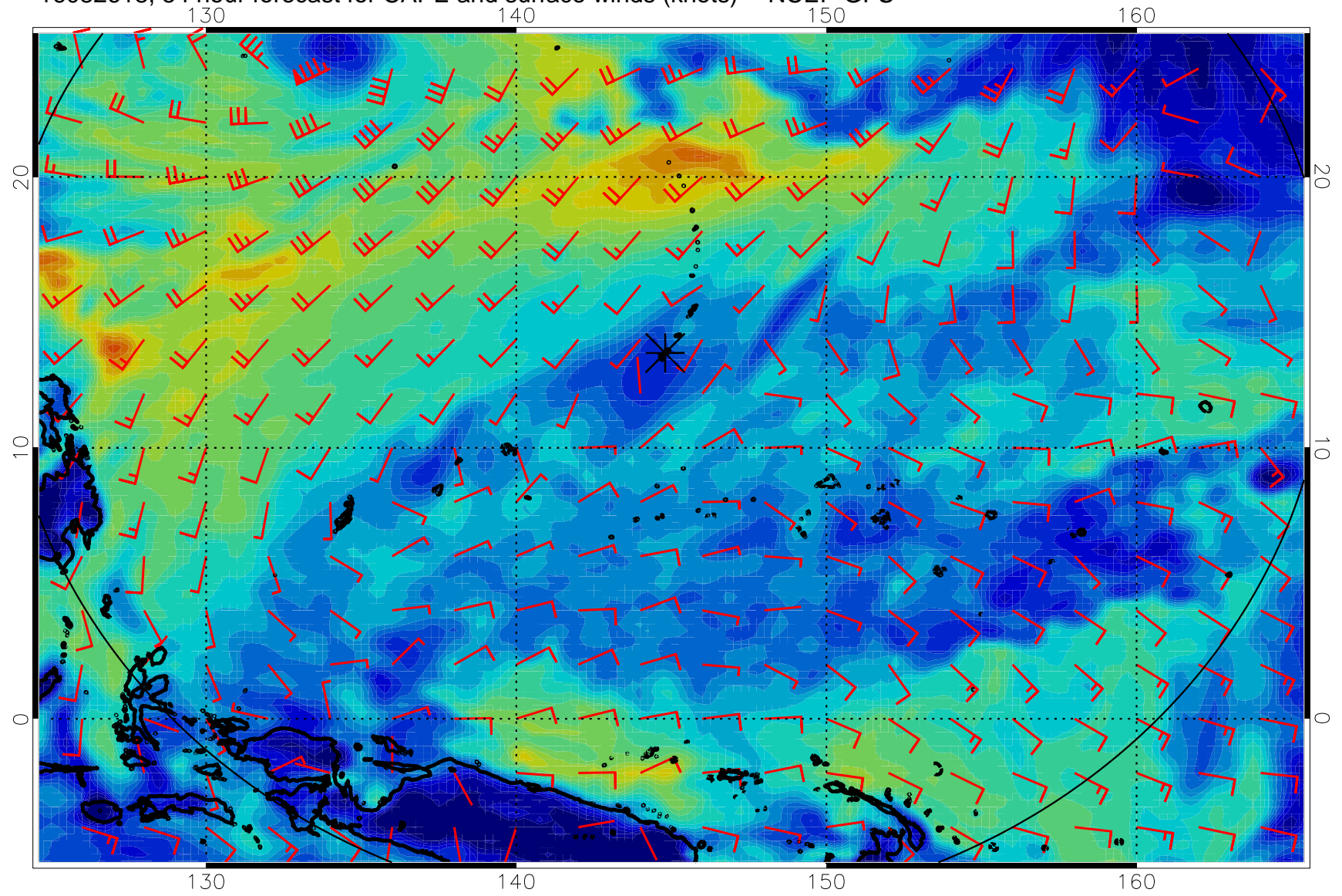
16082618, 54 hour forecast for CAPE and surface winds (knots) -- NCEP GFS
