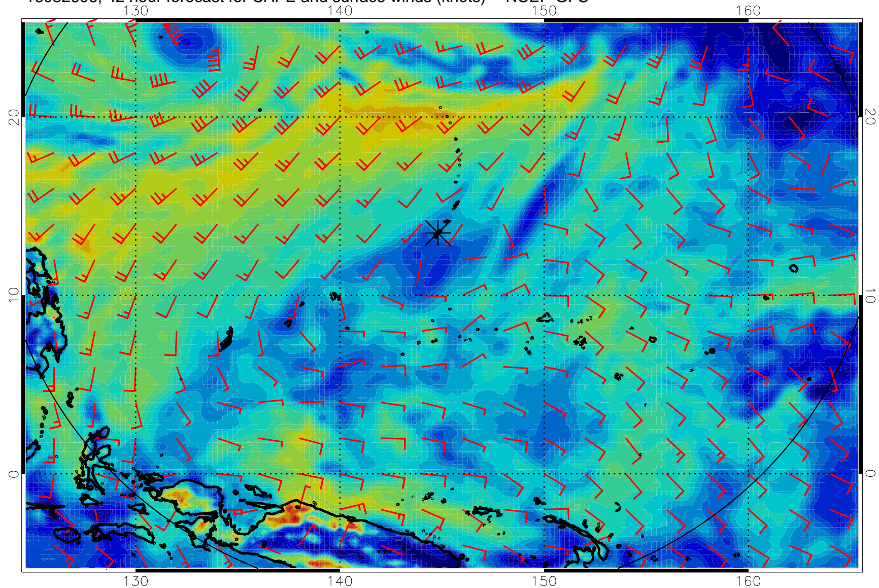
16082606, 42 hour forecast for CAPE and surface winds (knots) -- NCEP GFS
