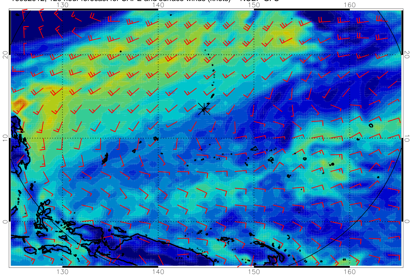
16082912, 120 hour forecast for CAPE and surface winds (knots) -- NCEP GFS
