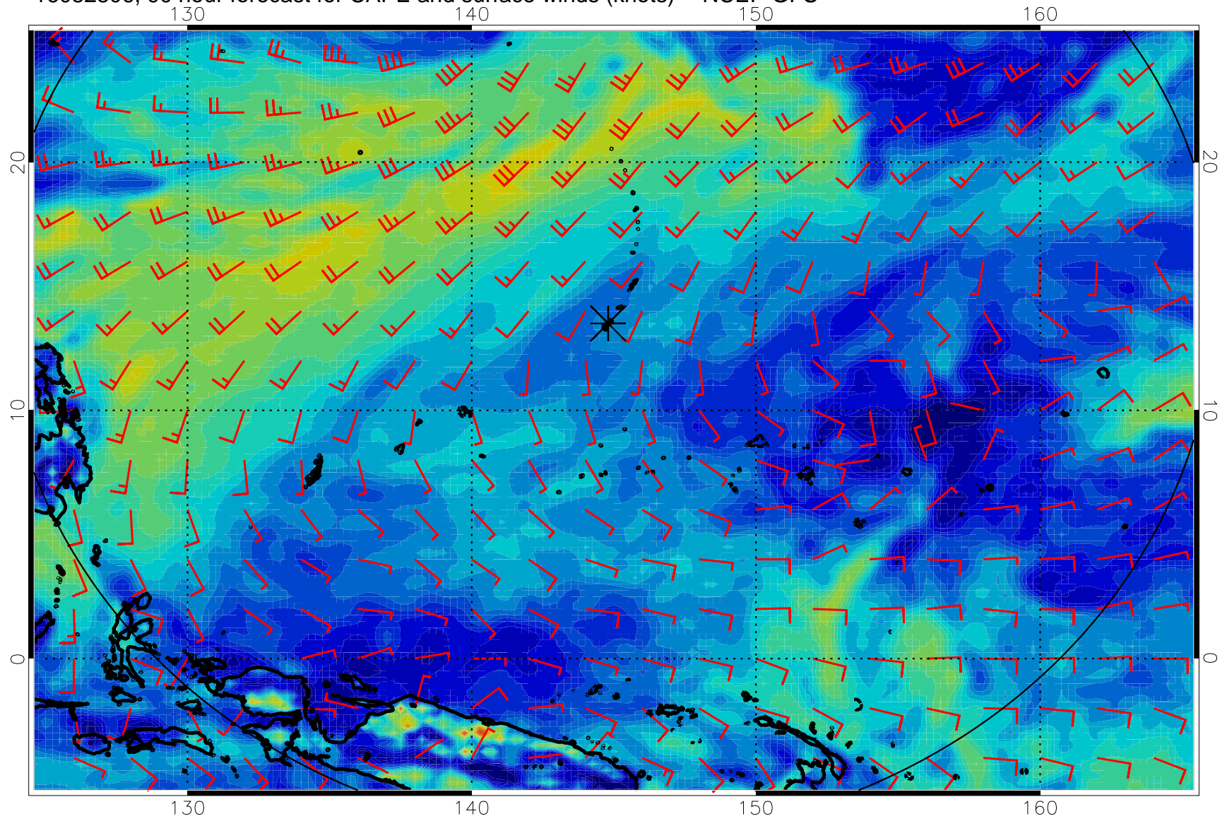
16082806, 90 hour forecast for CAPE and surface winds (knots) -- NCEP GFS
