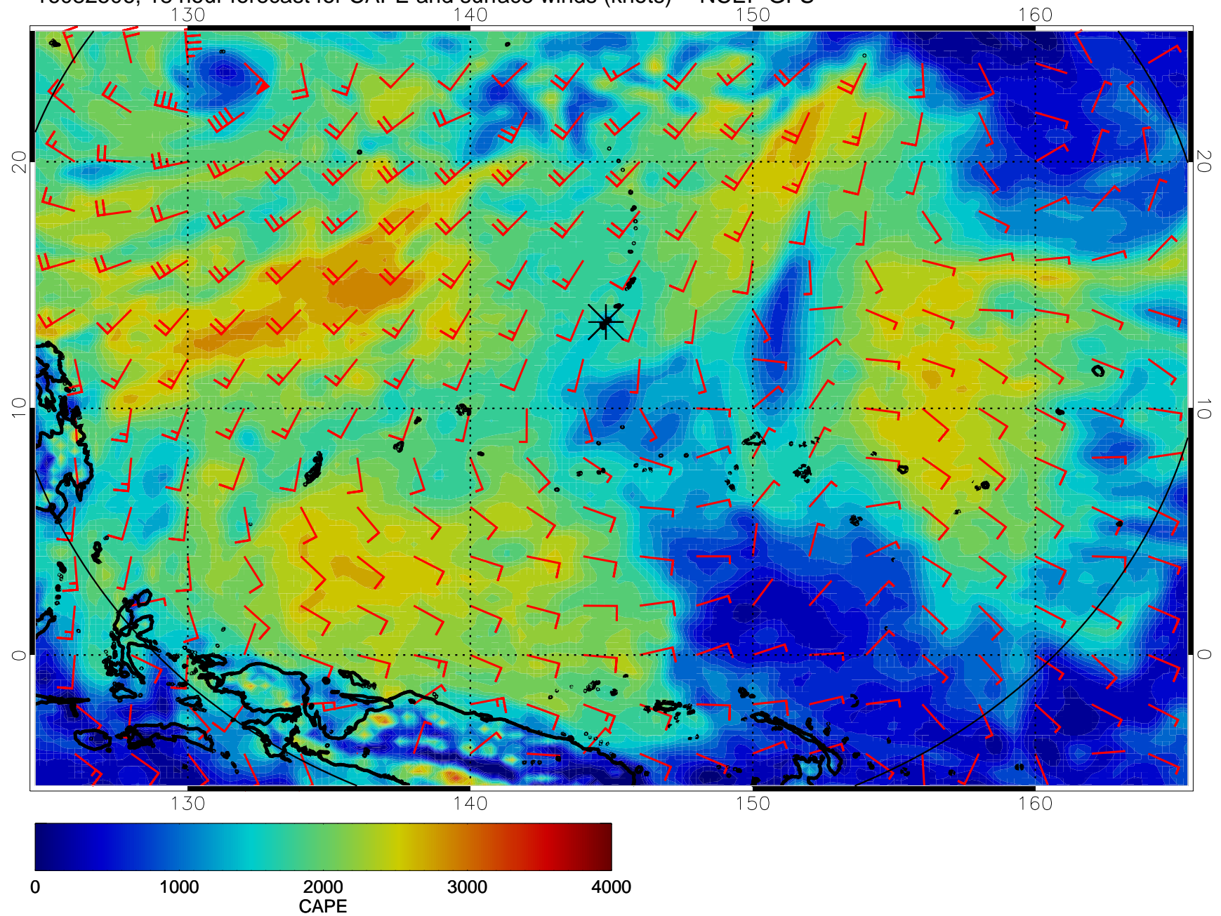
16082506, 18 hour forecast for CAPE and surface winds (knots) -- NCEP GFS
