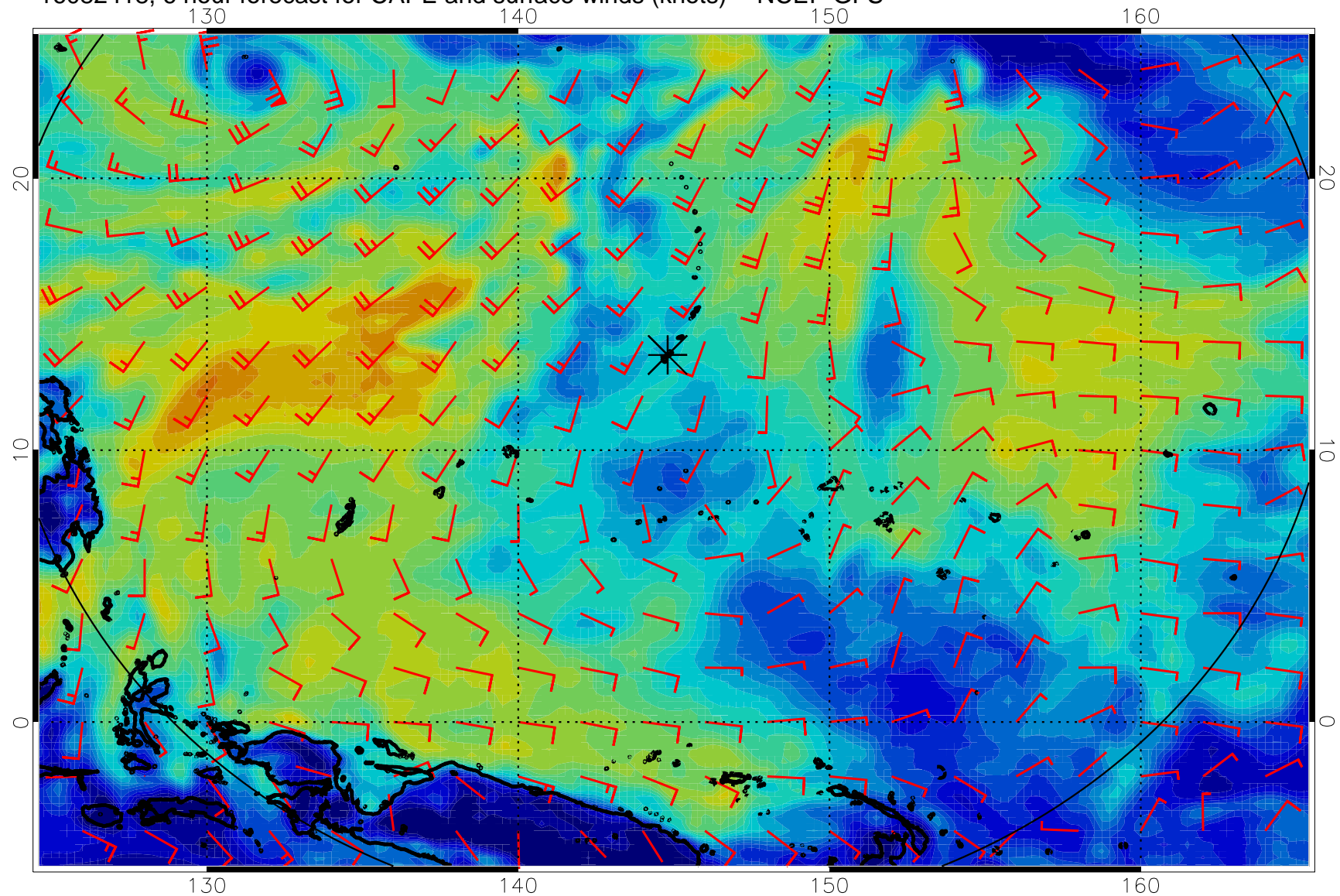
16082418, 6 hour forecast for CAPE and surface winds (knots) -- NCEP GFS
