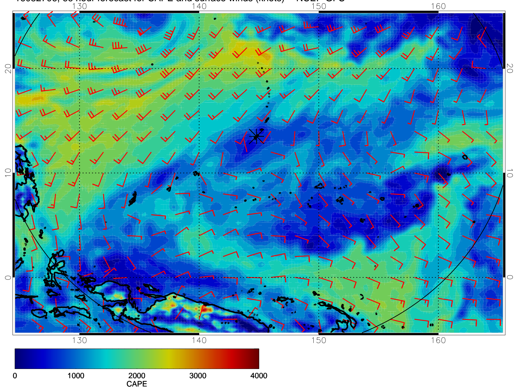
16082706, 66 hour forecast for CAPE and surface winds (knots) -- NCEP GFS
