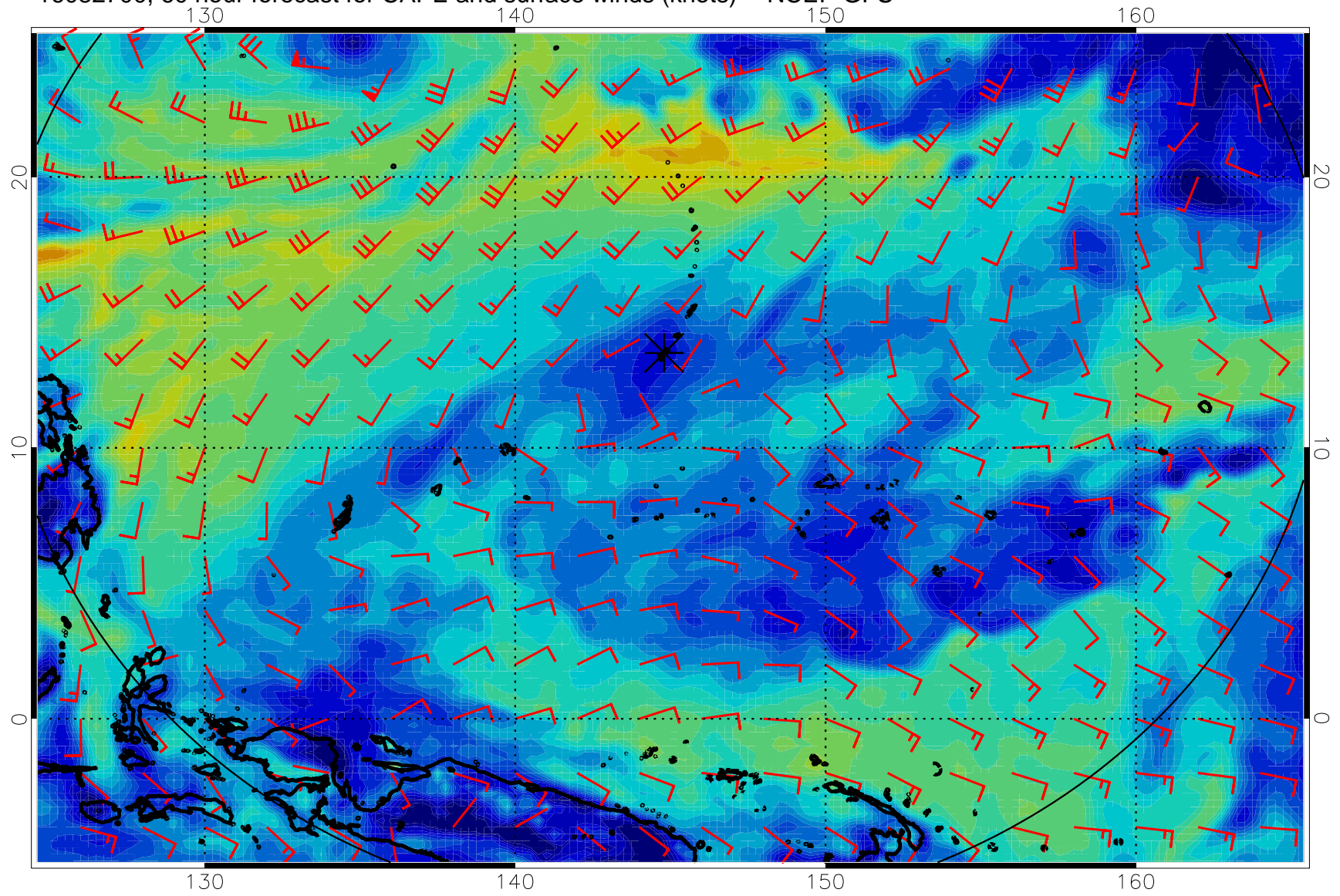
16082700, 60 hour forecast for CAPE and surface winds (knots) -- NCEP GFS
