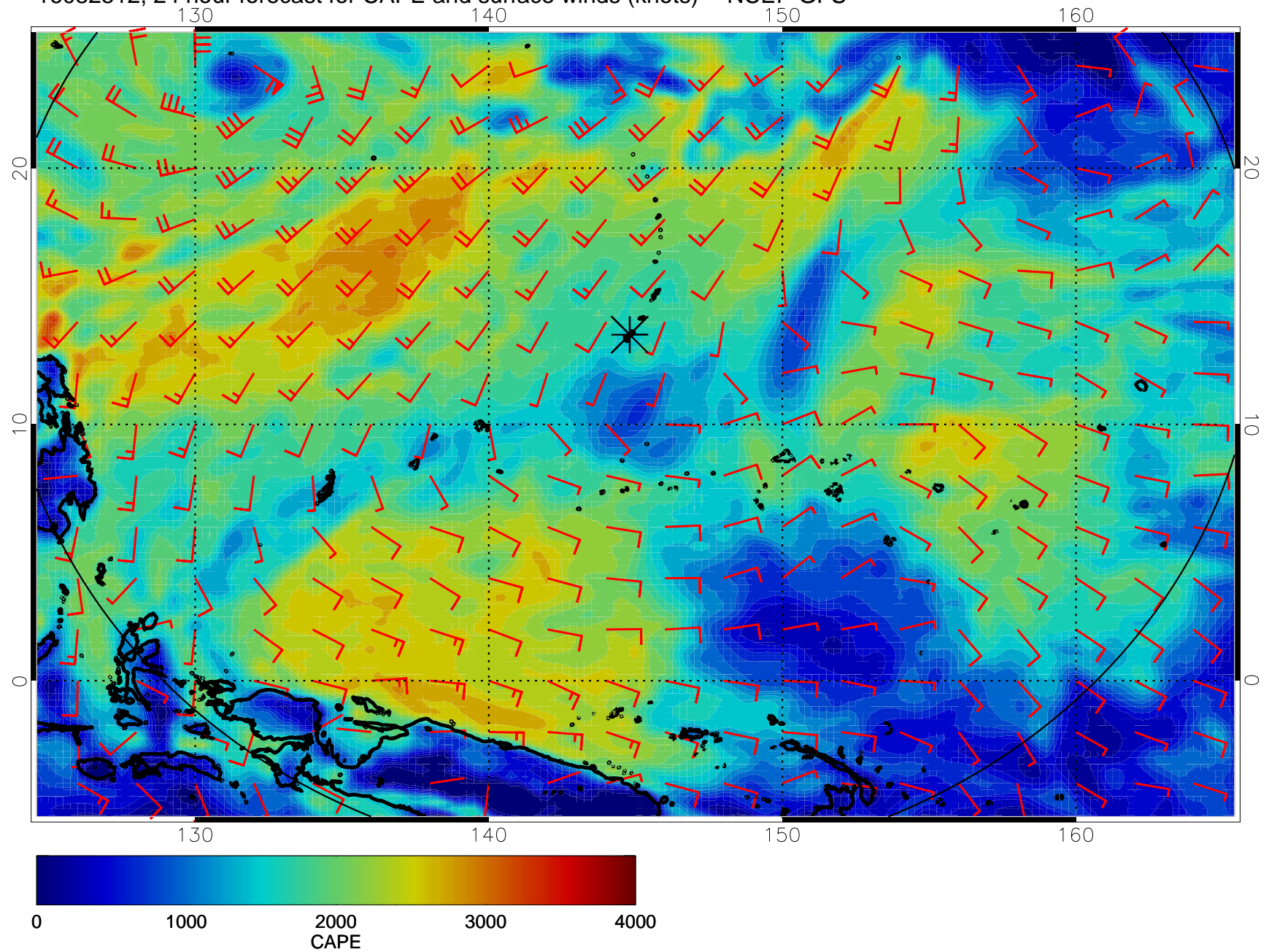
16082512, 24 hour forecast for CAPE and surface winds (knots) -- NCEP GFS
