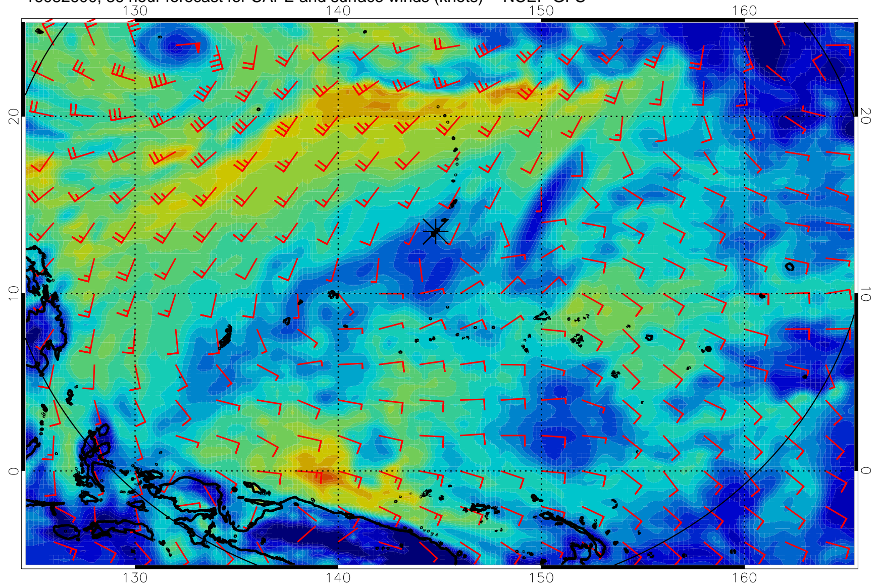
16082600, 36 hour forecast for CAPE and surface winds (knots) -- NCEP GFS
