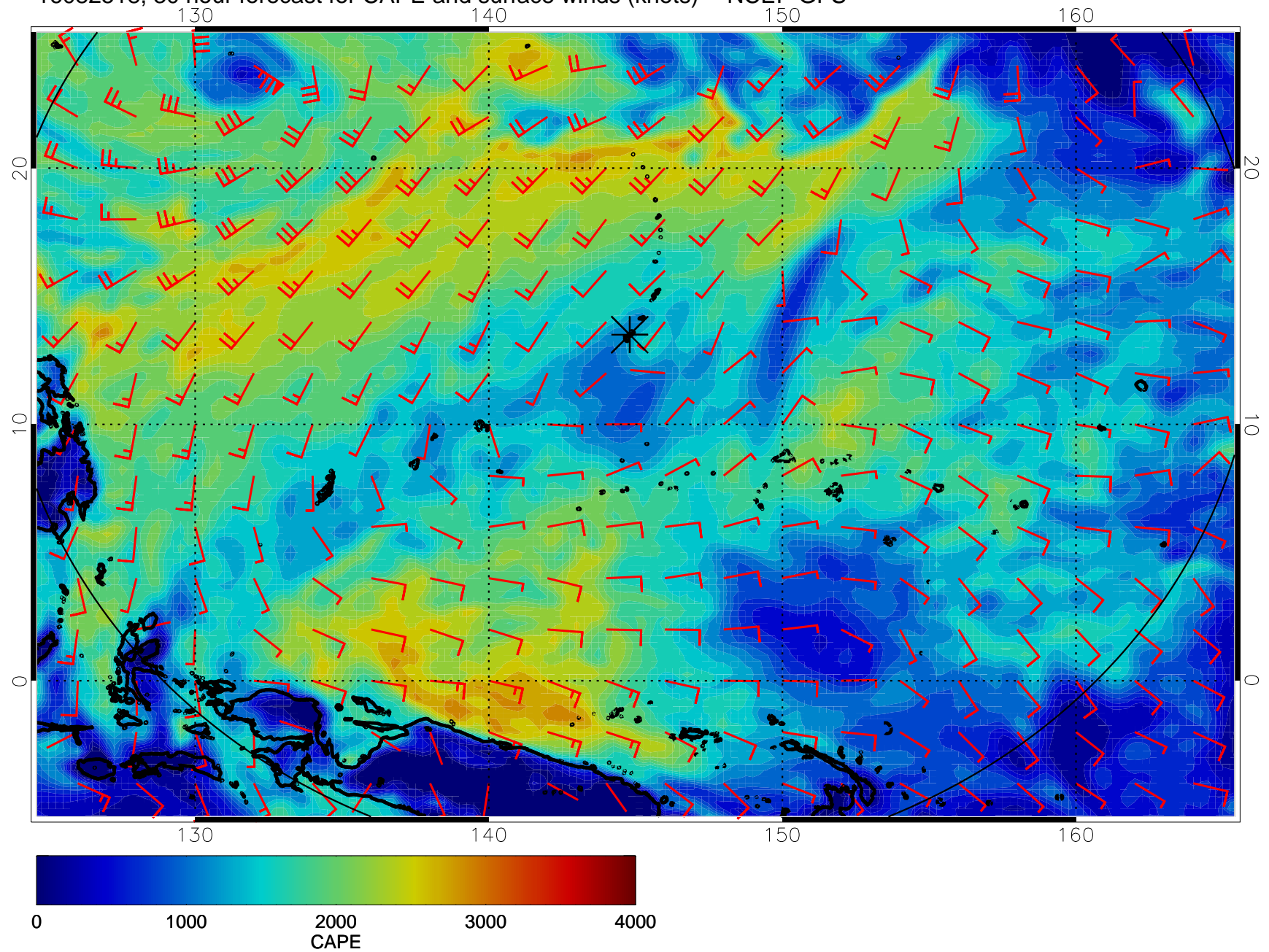
16082518, 30 hour forecast for CAPE and surface winds (knots) -- NCEP GFS
