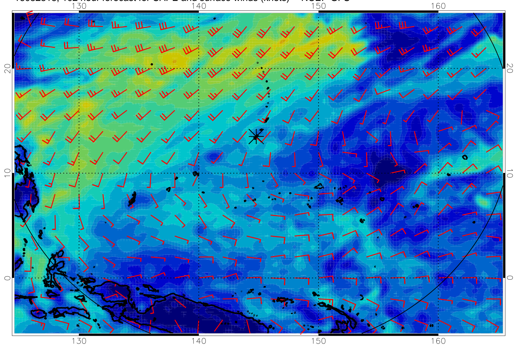
16082818, 102 hour forecast for CAPE and surface winds (knots) -- NCEP GFS
