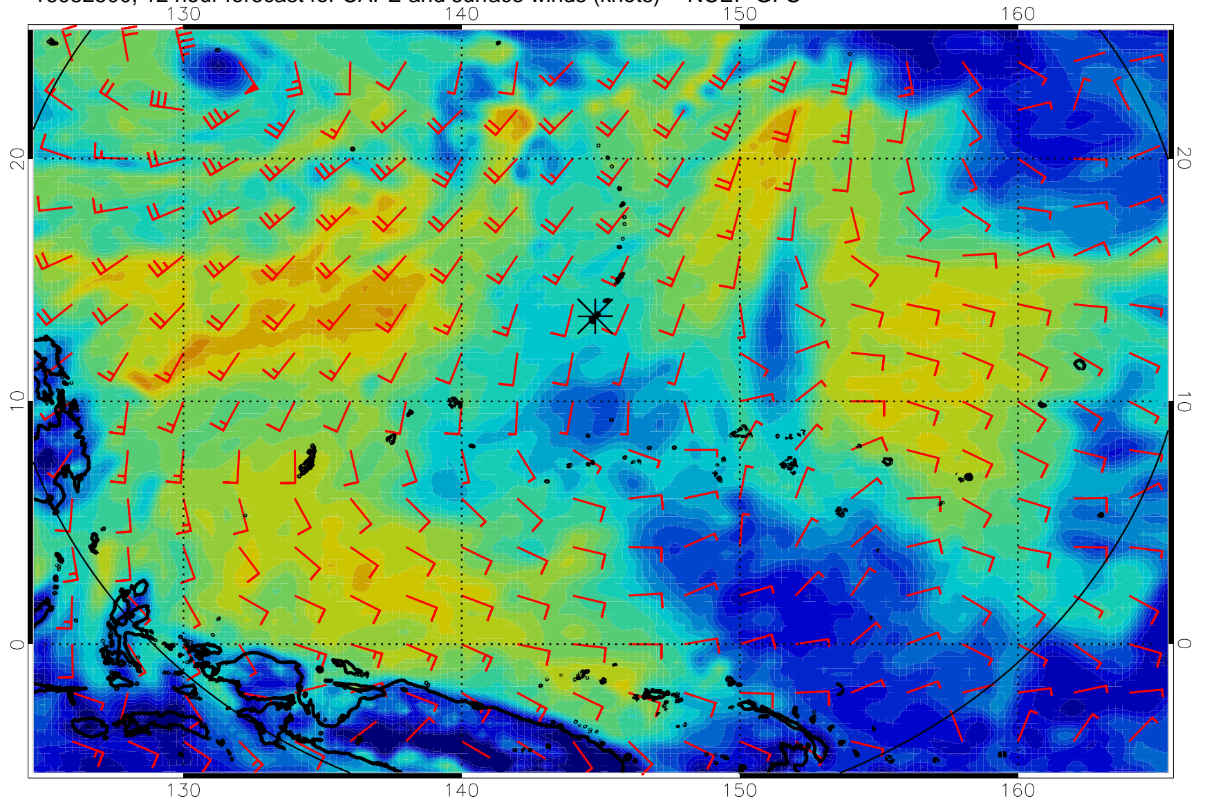
16082500, 12 hour forecast for CAPE and surface winds (knots) -- NCEP GFS
