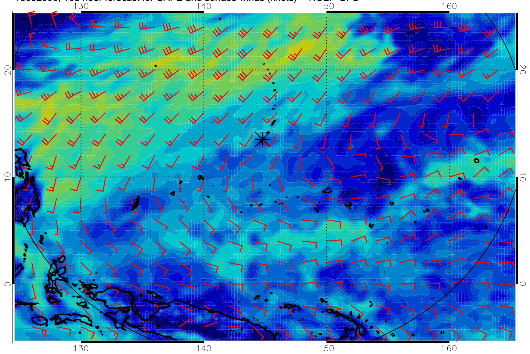
16082900, 108 hour forecast for CAPE and surface winds (knots) -- NCEP GFS
