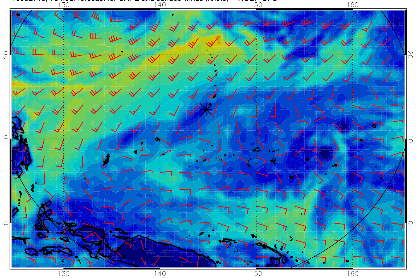
16082718, 78 hour forecast for CAPE and surface winds (knots) -- NCEP GFS
