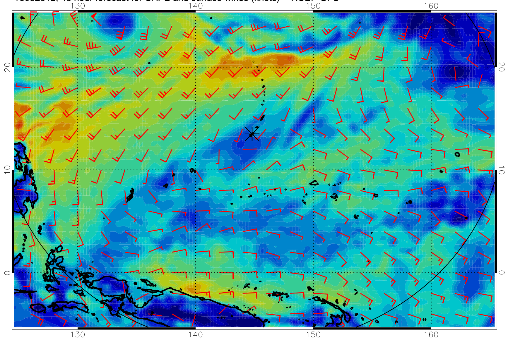
16082612, 48 hour forecast for CAPE and surface winds (knots) -- NCEP GFS
