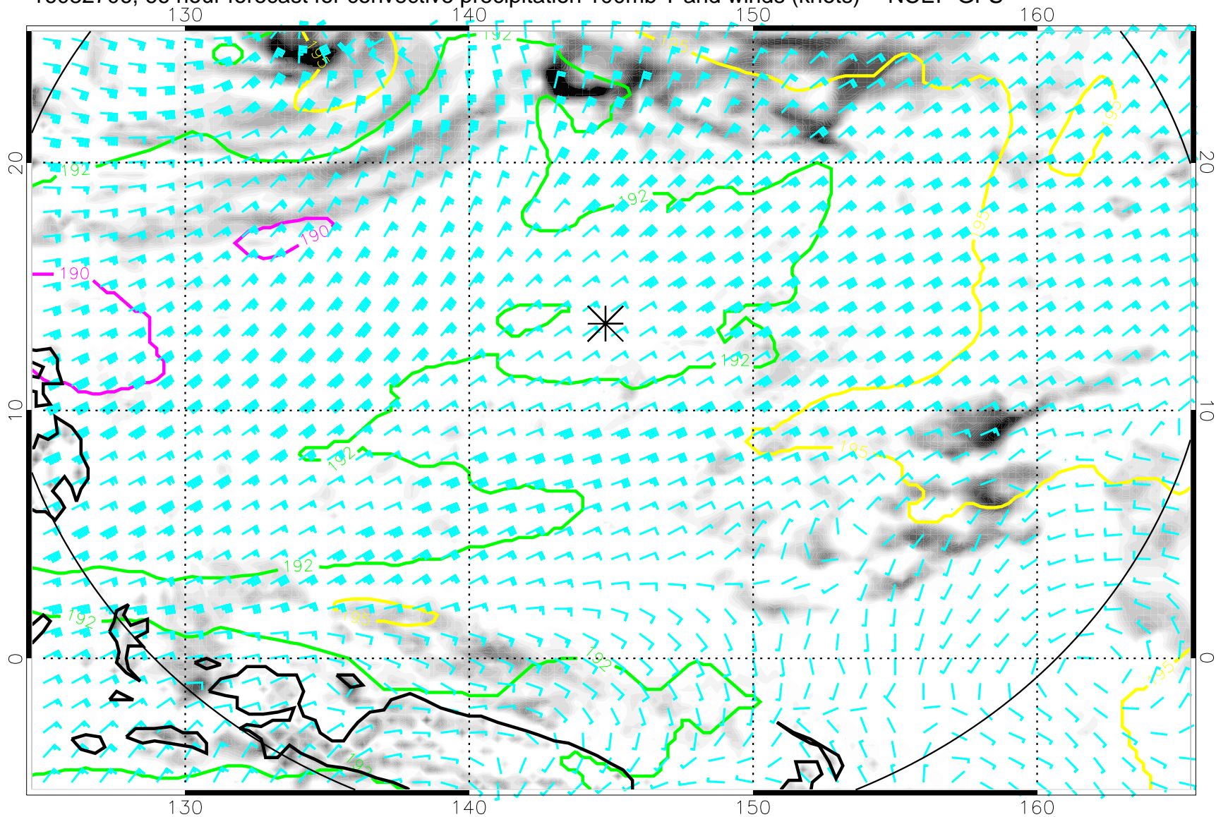
16082706, 66 hour forecast for convective precipitation 100mb T and winds (knots) -- NCEP GFS
