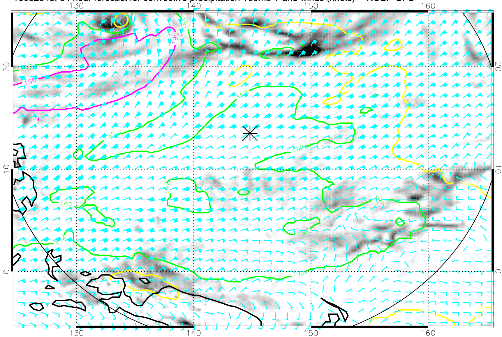
16082618, 54 hour forecast for convective precipitation 100mb T and winds (knots) -- NCEP GFS
