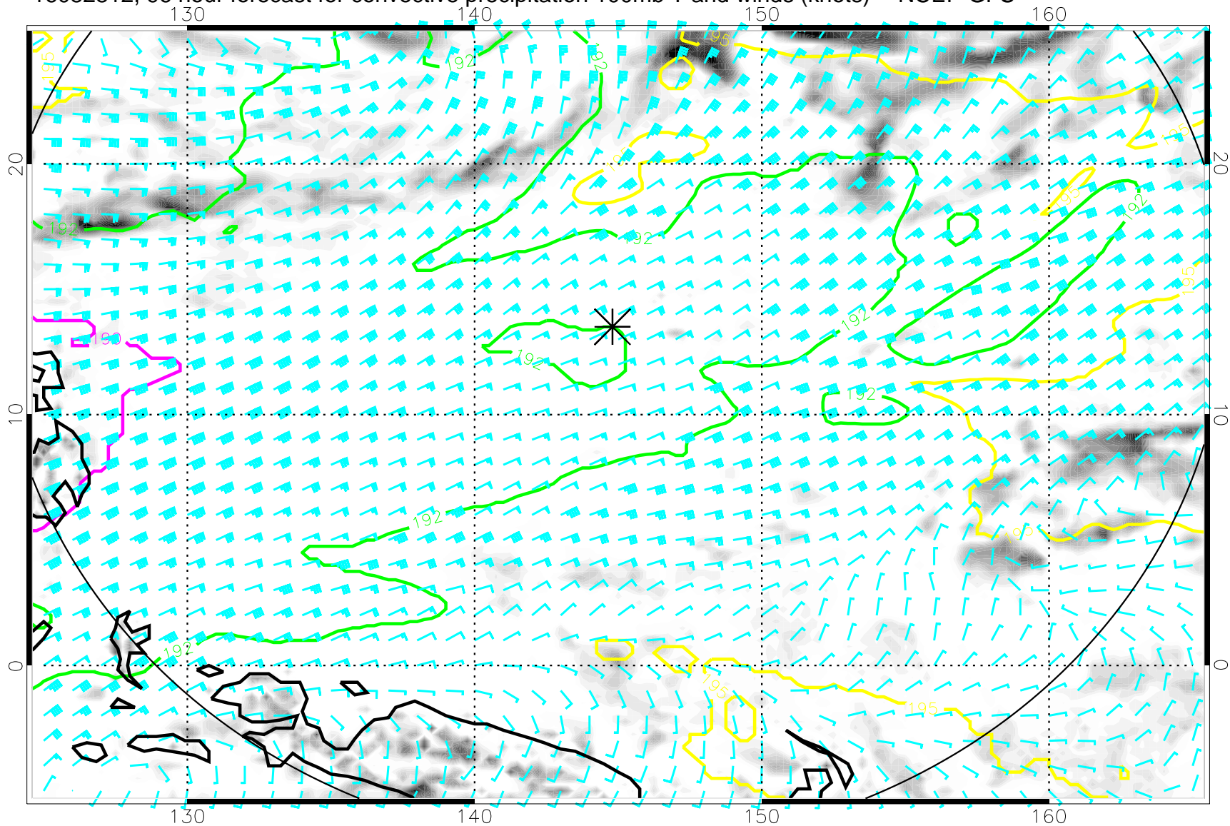
16082812, 96 hour forecast for convective precipitation 100mb T and winds (knots) -- NCEP GFS
