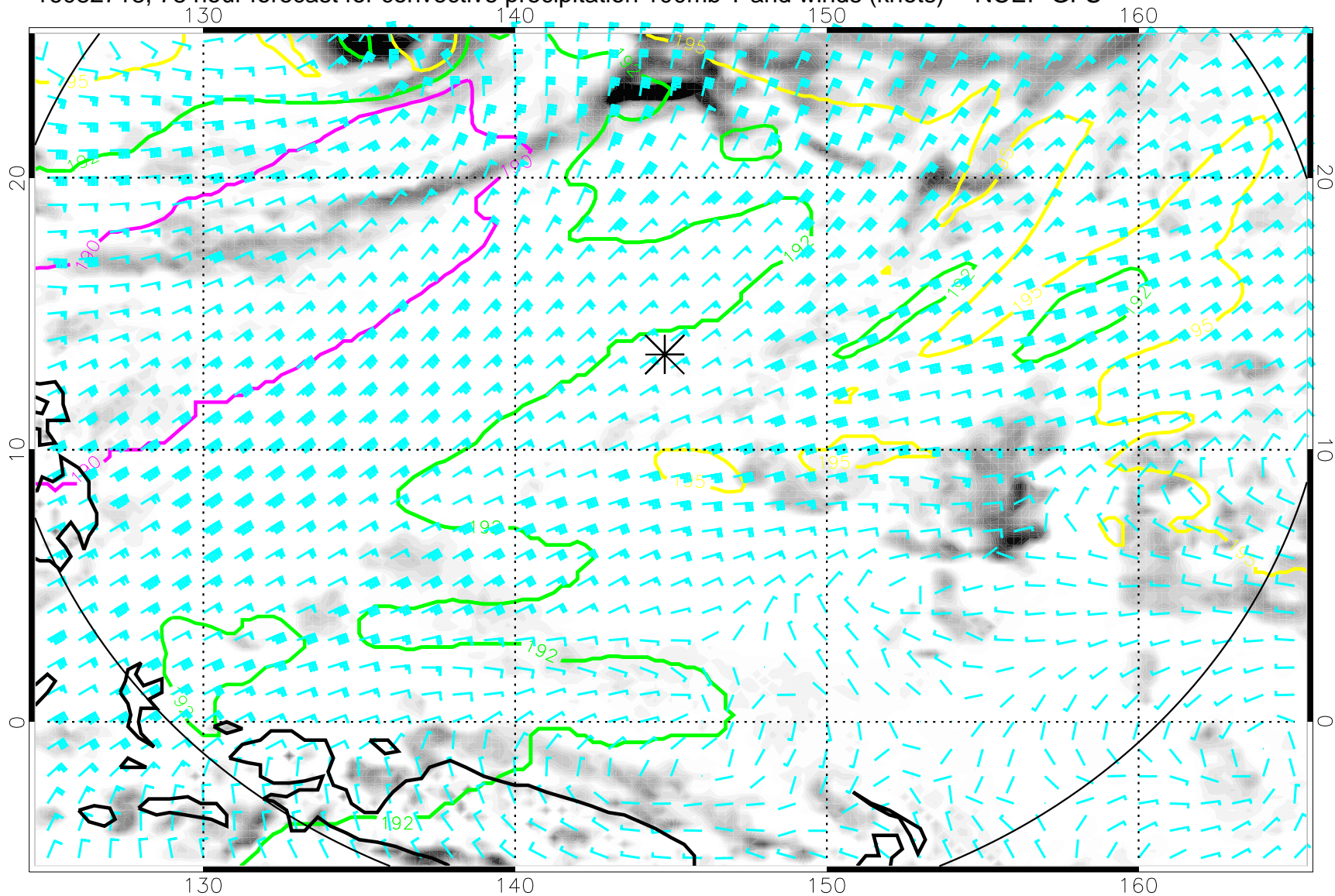
16082718, 78 hour forecast for convective precipitation 100mb T and winds (knots) -- NCEP GFS
