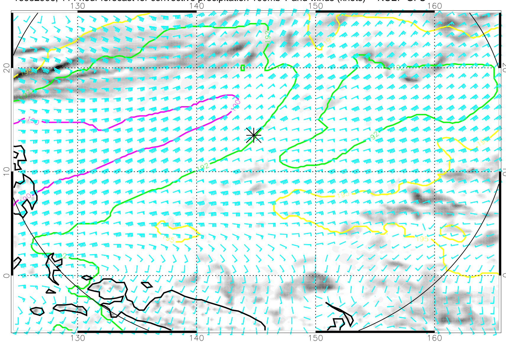
16082906, 114 hour forecast for convective precipitation 100mb T and winds (knots) -- NCEP GFS
