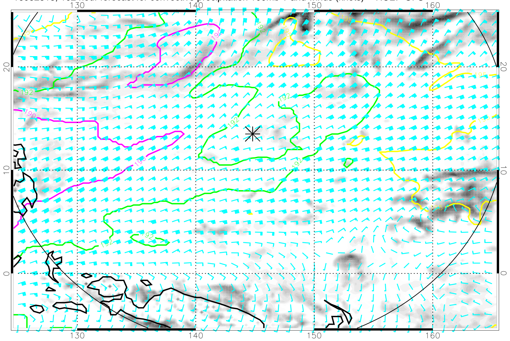
16082818, 102 hour forecast for convective precipitation 100mb T and winds (knots) -- NCEP GFS
