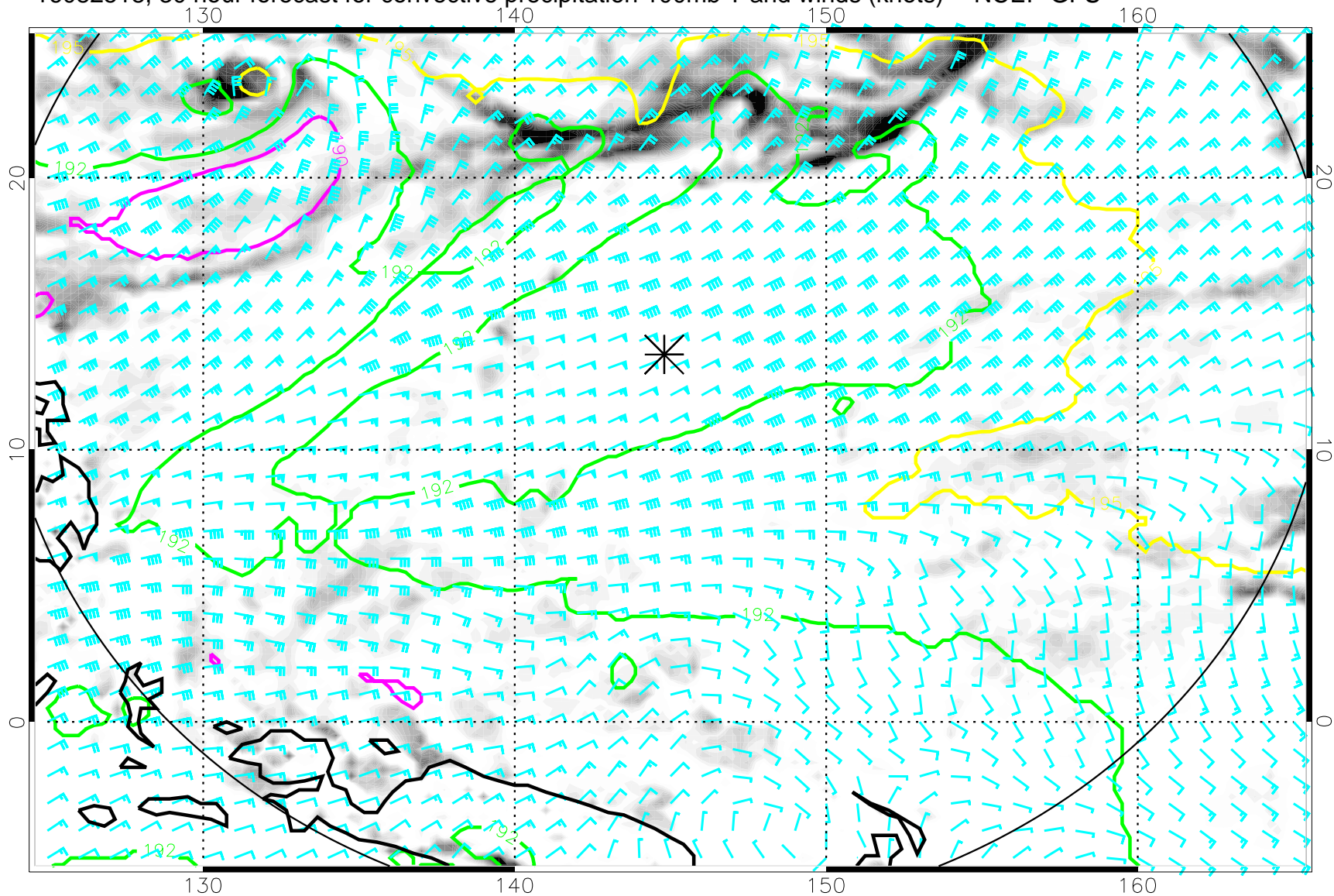
16082518, 30 hour forecast for convective precipitation 100mb T and winds (knots) -- NCEP GFS
