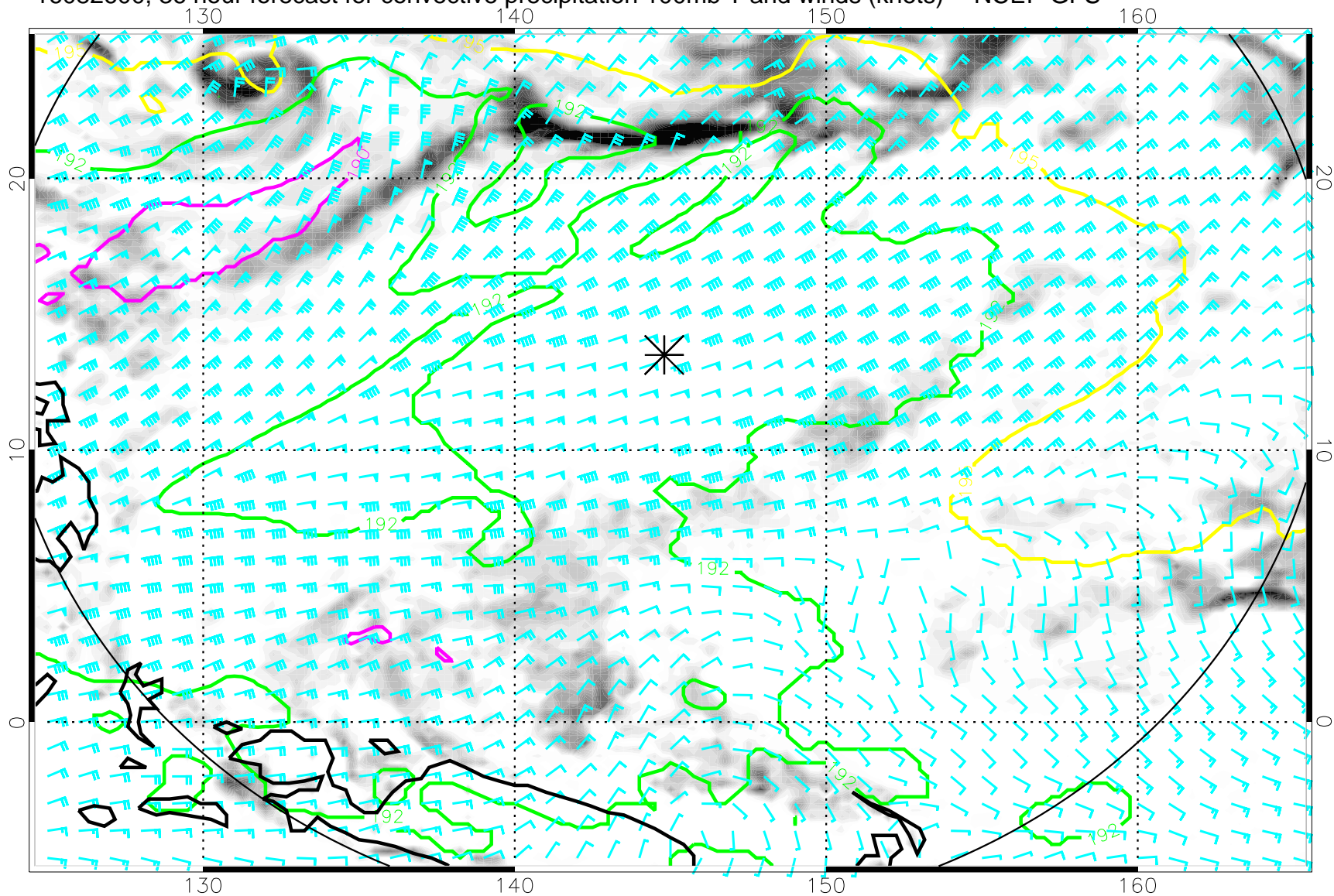
16082600, 36 hour forecast for convective precipitation 100mb T and winds (knots) -- NCEP GFS
