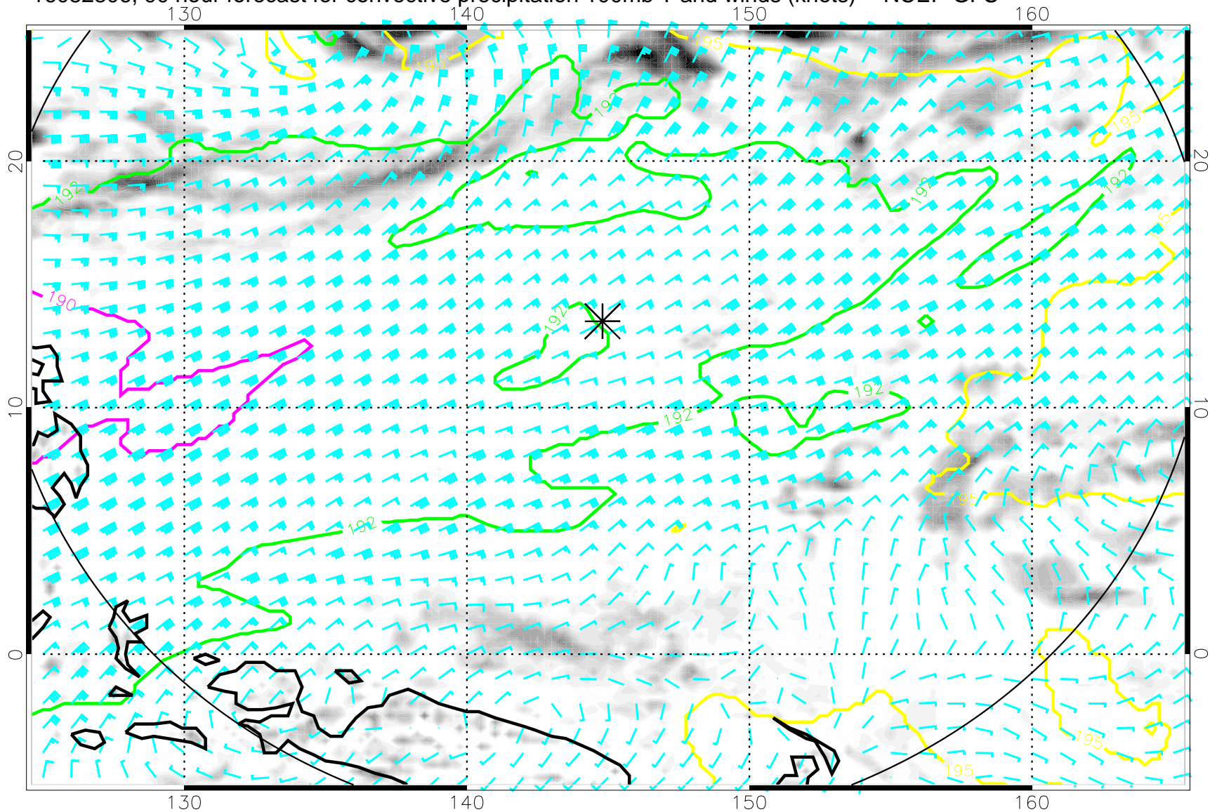
16082806, 90 hour forecast for convective precipitation 100mb T and winds (knots) -- NCEP GFS
