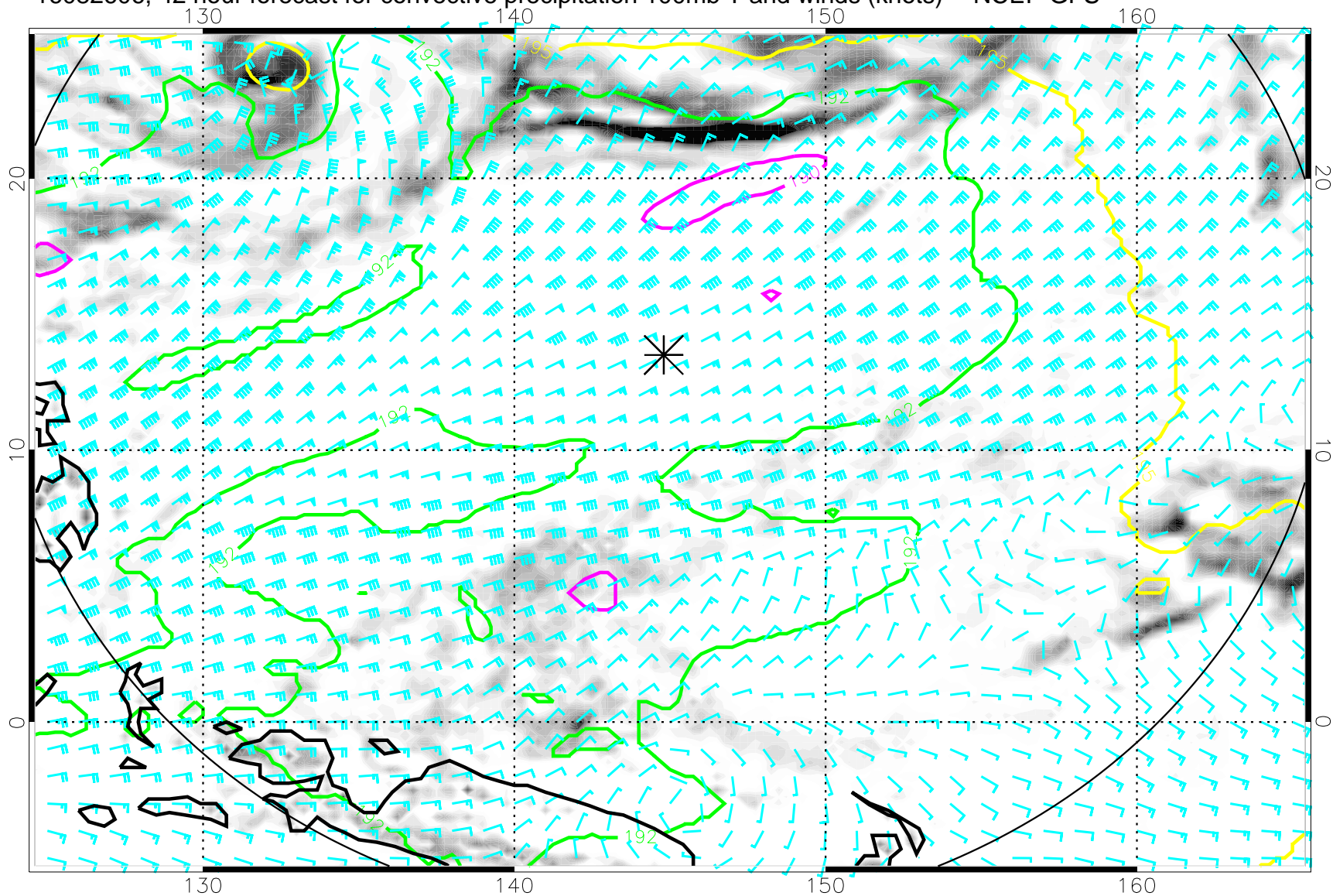
16082606, 42 hour forecast for convective precipitation 100mb T and winds (knots) -- NCEP GFS
