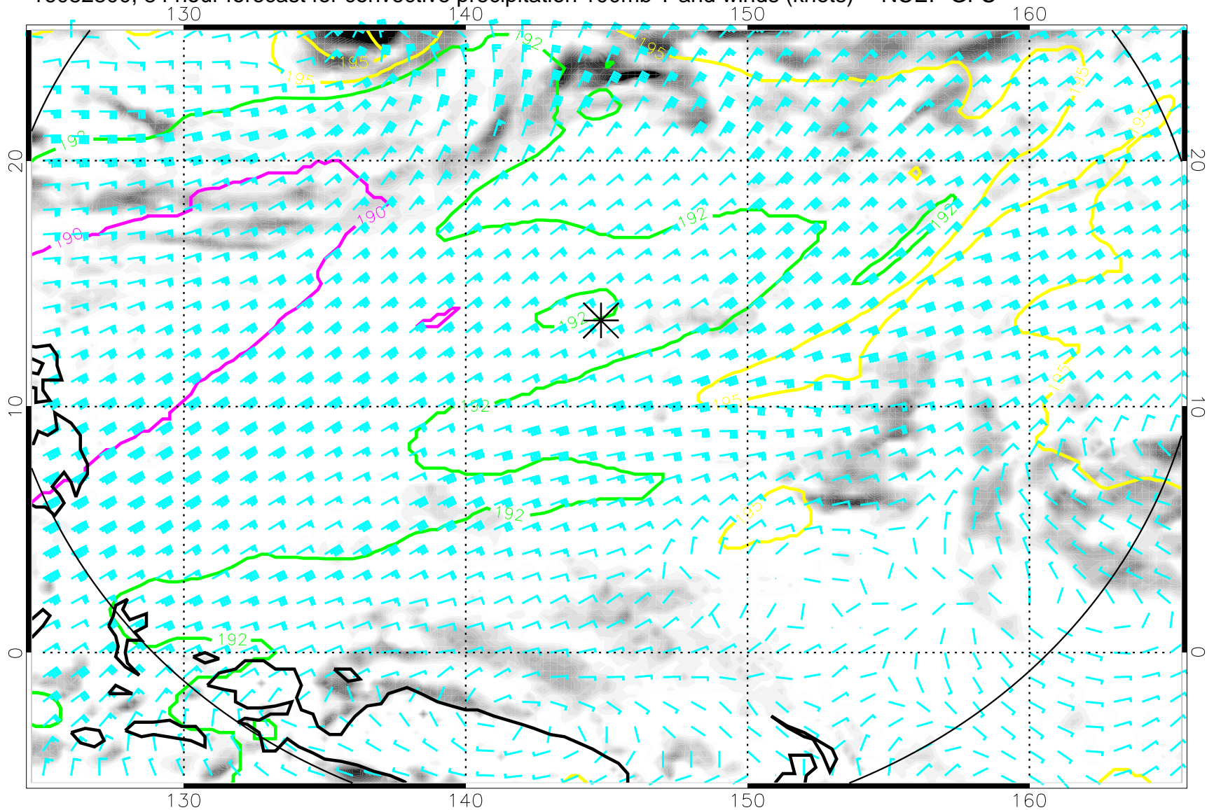
16082800, 84 hour forecast for convective precipitation 100mb T and winds (knots) -- NCEP GFS
