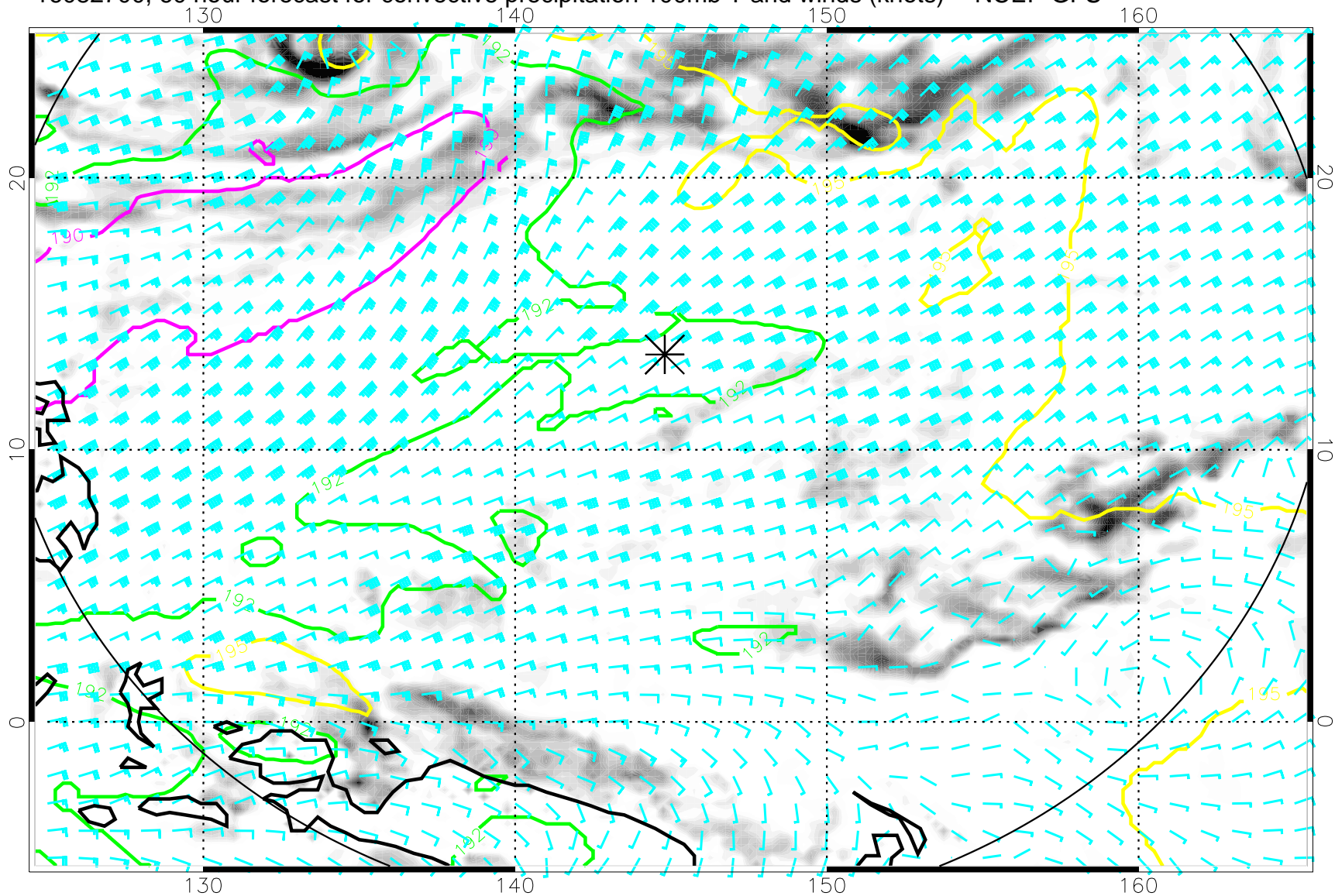
16082700, 60 hour forecast for convective precipitation 100mb T and winds (knots) -- NCEP GFS
