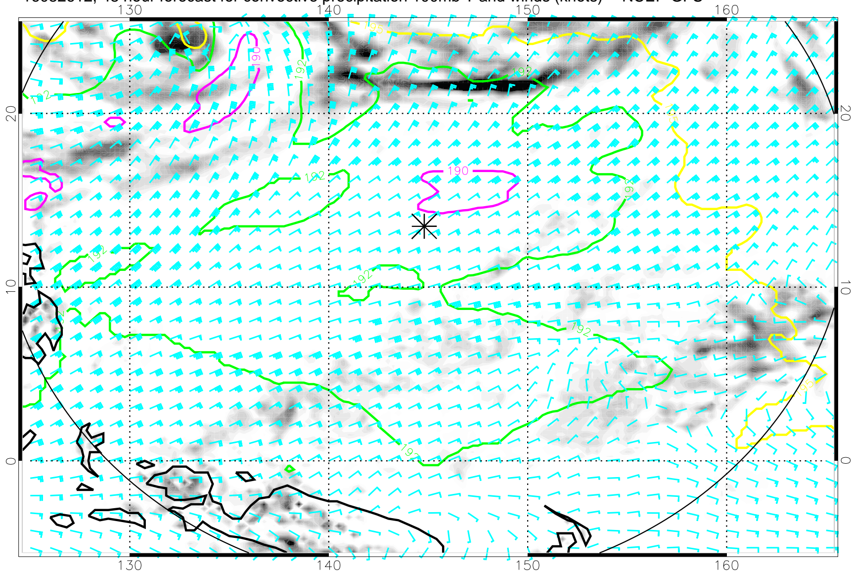
16082612, 48 hour forecast for convective precipitation 100mb T and winds (knots) -- NCEP GFS
