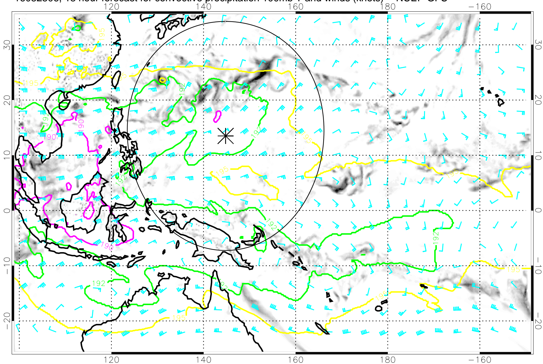
16082506, 18 hour forecast for convective precipitation 100mb T and winds (knots) -- NCEP GFS
