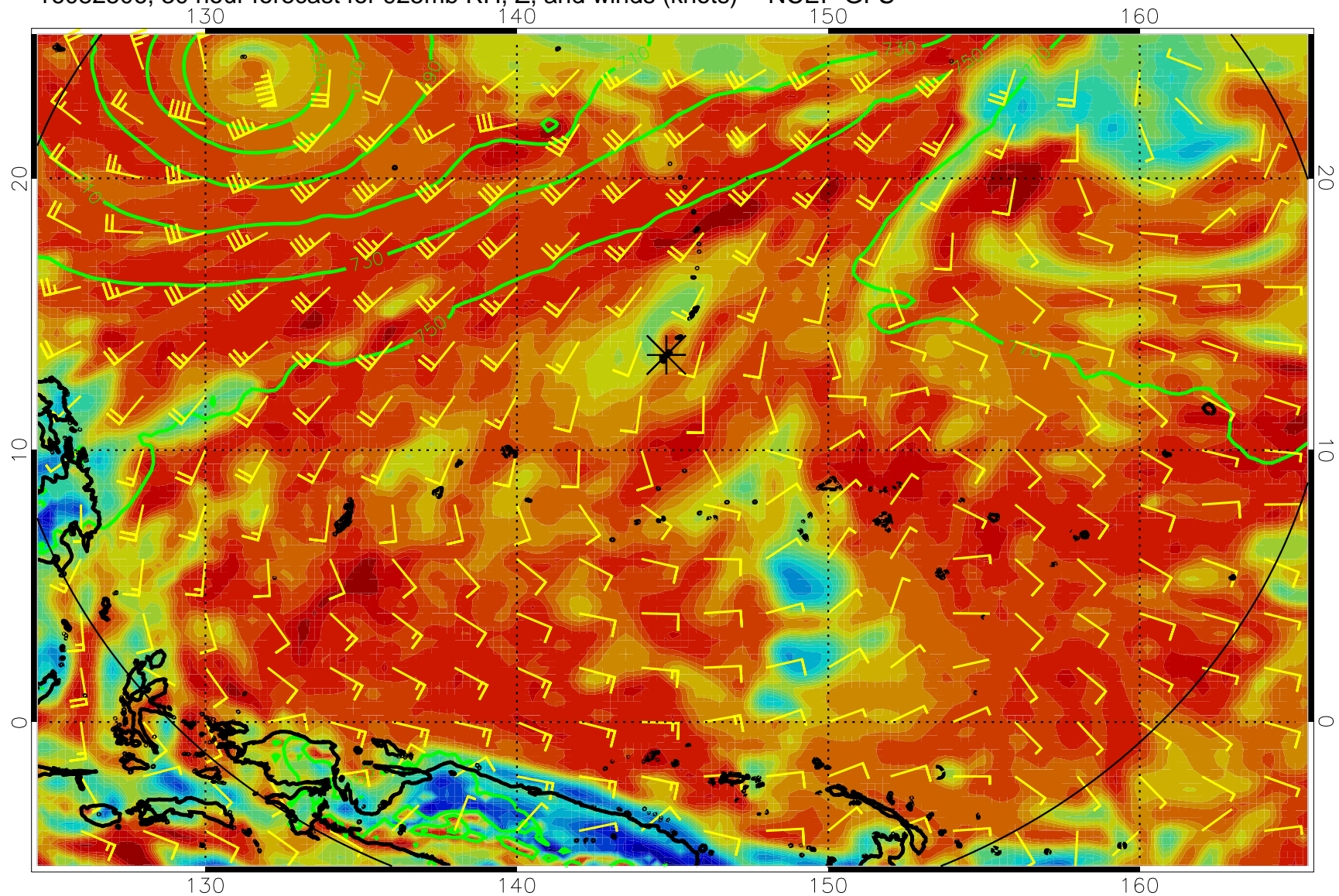
16082506, 30 hour forecast for 925mb RH, Z, and winds (knots) -- NCEP GFS
