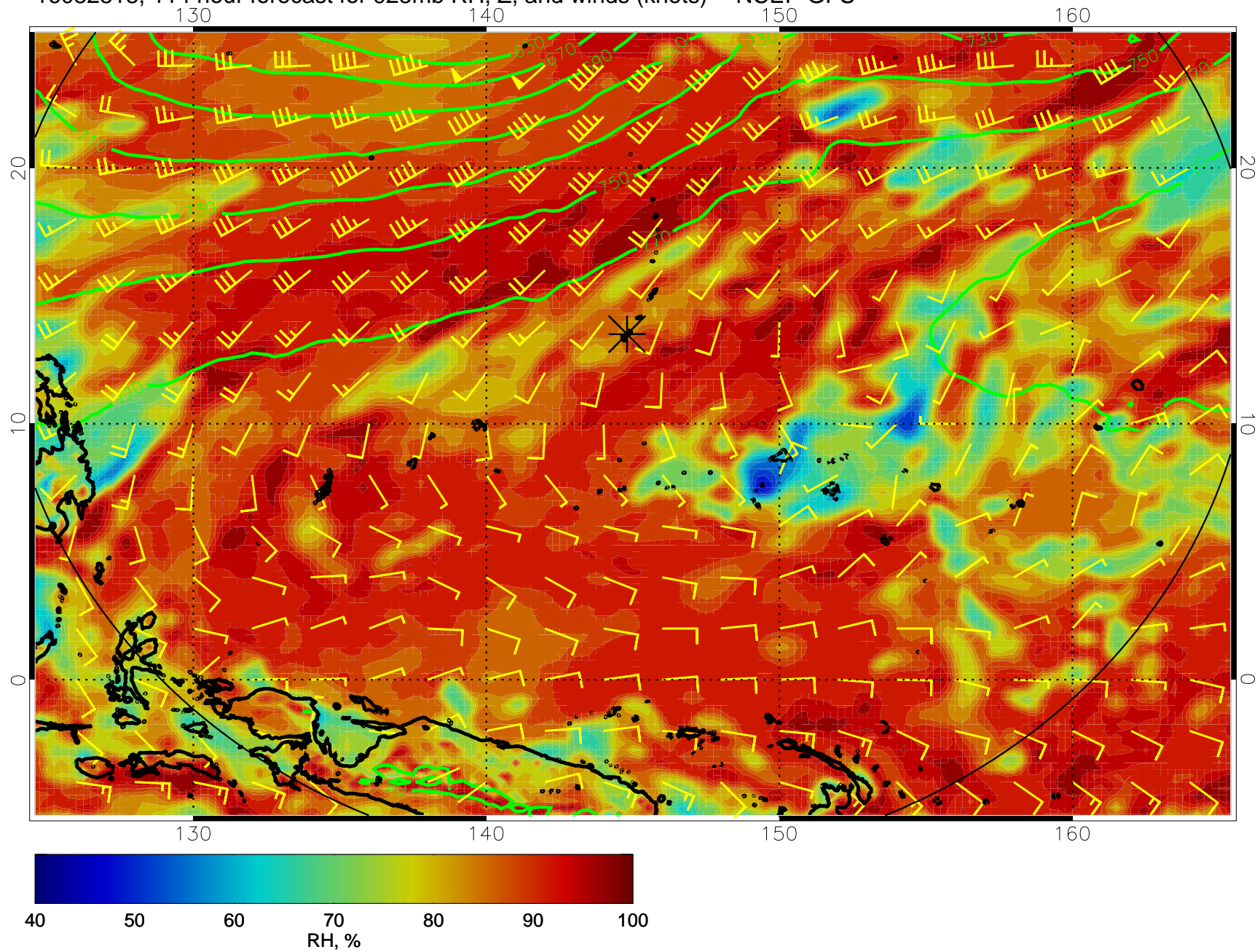
16082818, 114 hour forecast for 925mb RH, Z, and winds (knots) -- NCEP GFS
