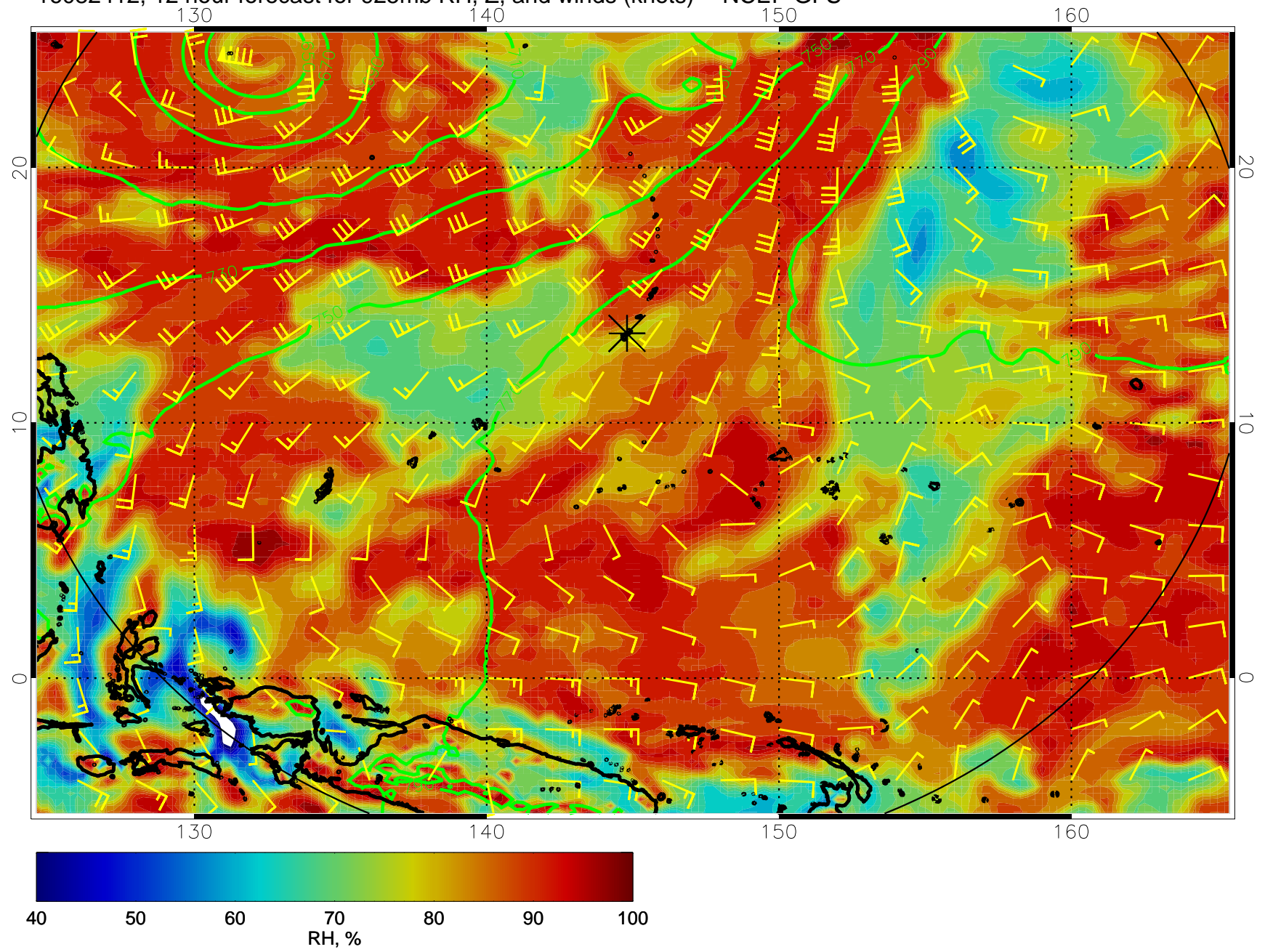
16082412, 12 hour forecast for 925mb RH, Z, and winds (knots) -- NCEP GFS
