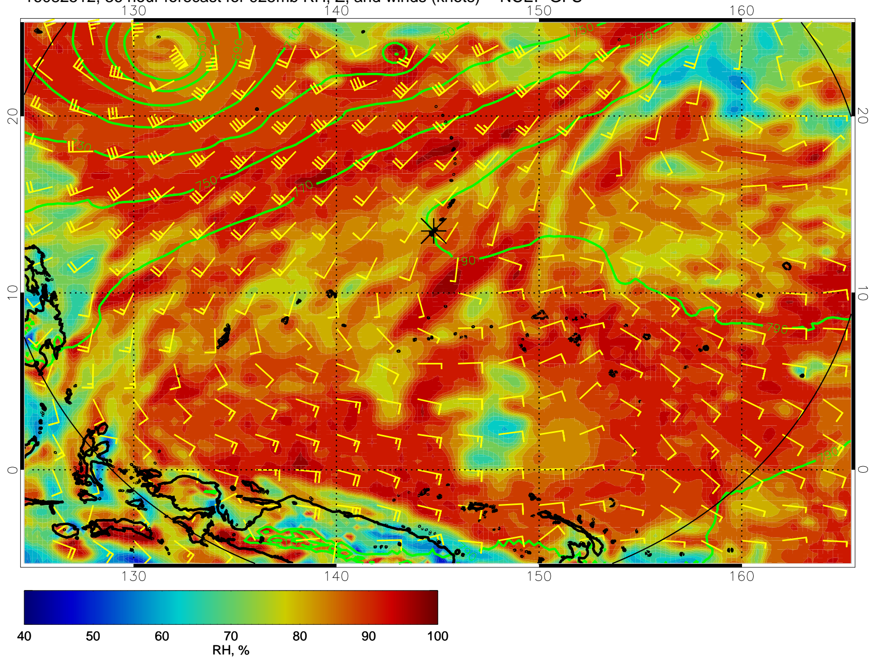
16082512, 36 hour forecast for 925mb RH, Z, and winds (knots) -- NCEP GFS
