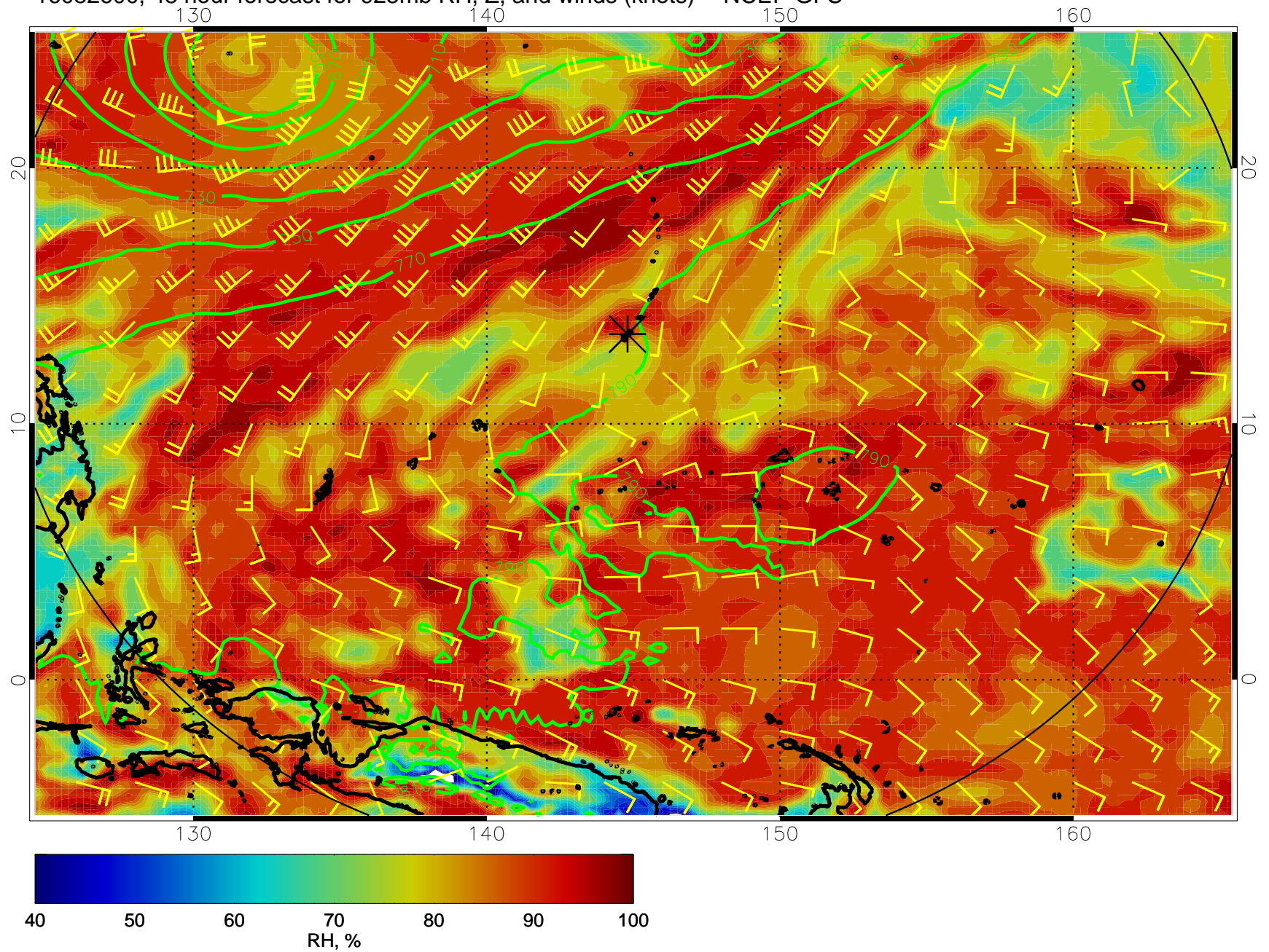
16082600, 48 hour forecast for 925mb RH, Z, and winds (knots) -- NCEP GFS
