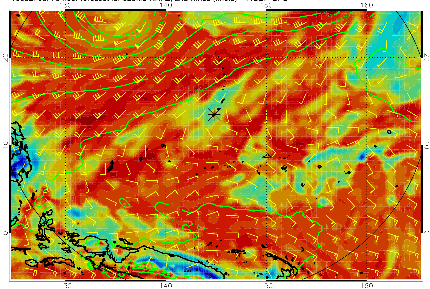
16082706, 78 hour forecast for 925mb RH, Z, and winds (knots) -- NCEP GFS
