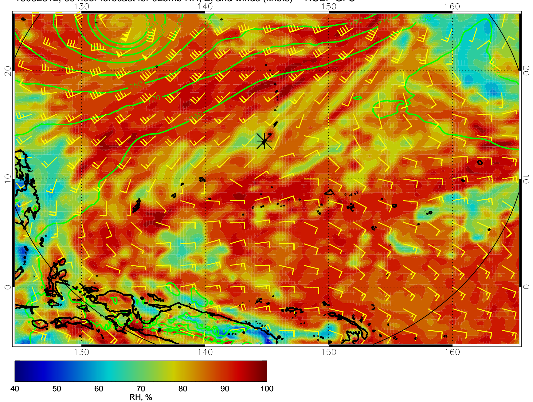
16082612, 60 hour forecast for 925mb RH, Z, and winds (knots) -- NCEP GFS
