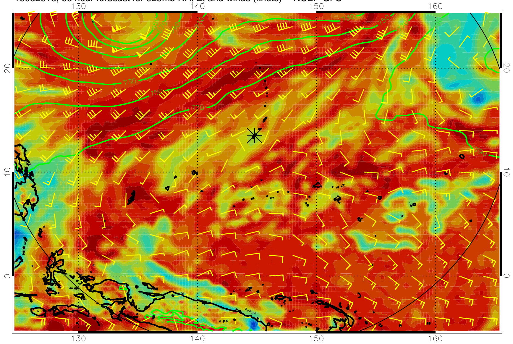
16082618, 66 hour forecast for 925mb RH, Z, and winds (knots) -- NCEP GFS
