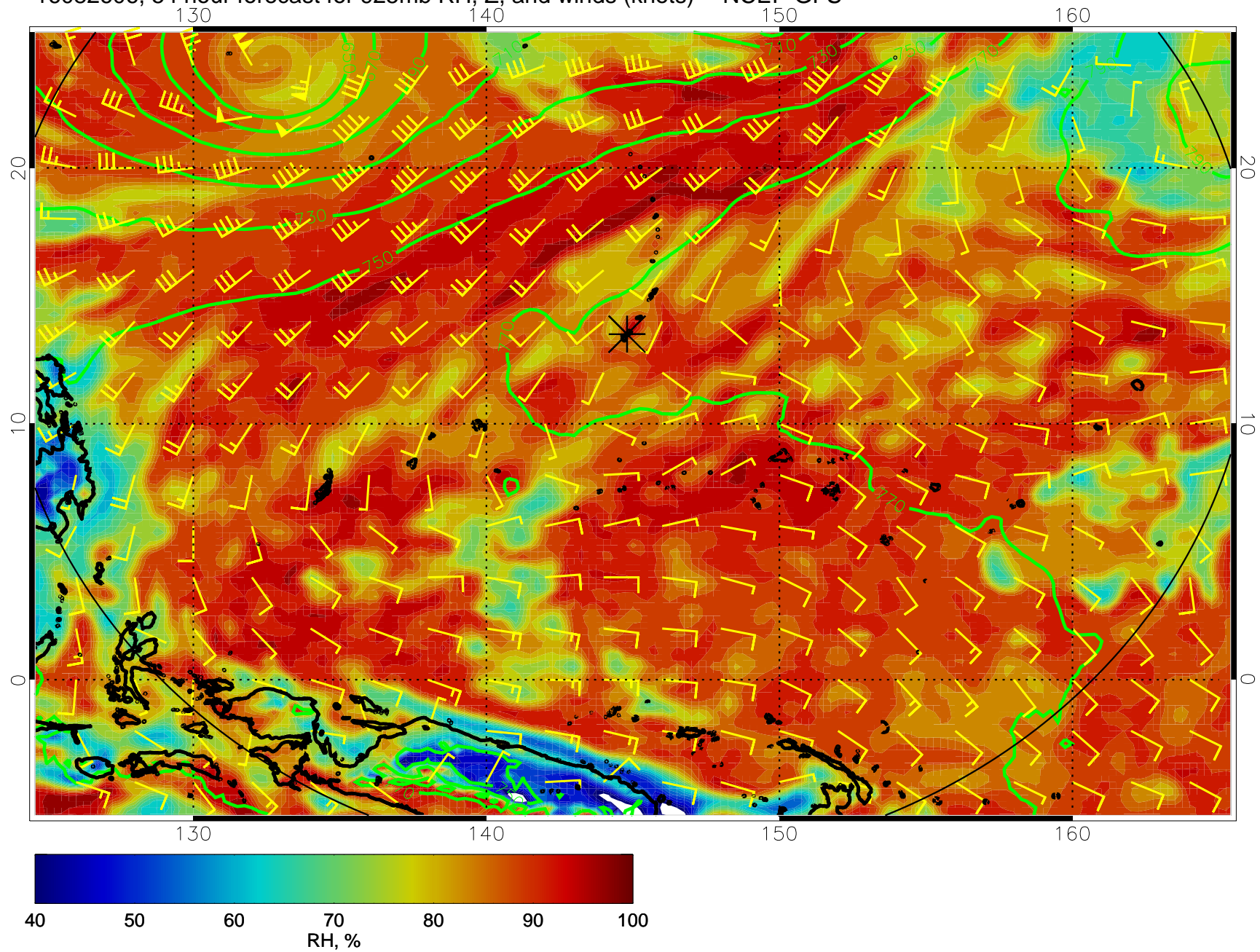
16082606, 54 hour forecast for 925mb RH, Z, and winds (knots) -- NCEP GFS
