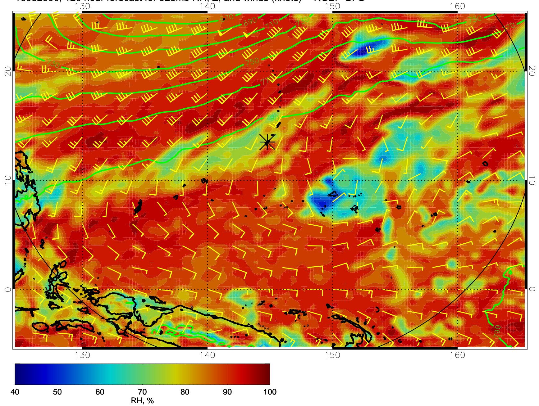
16082900, 120 hour forecast for 925mb RH, Z, and winds (knots) -- NCEP GFS
