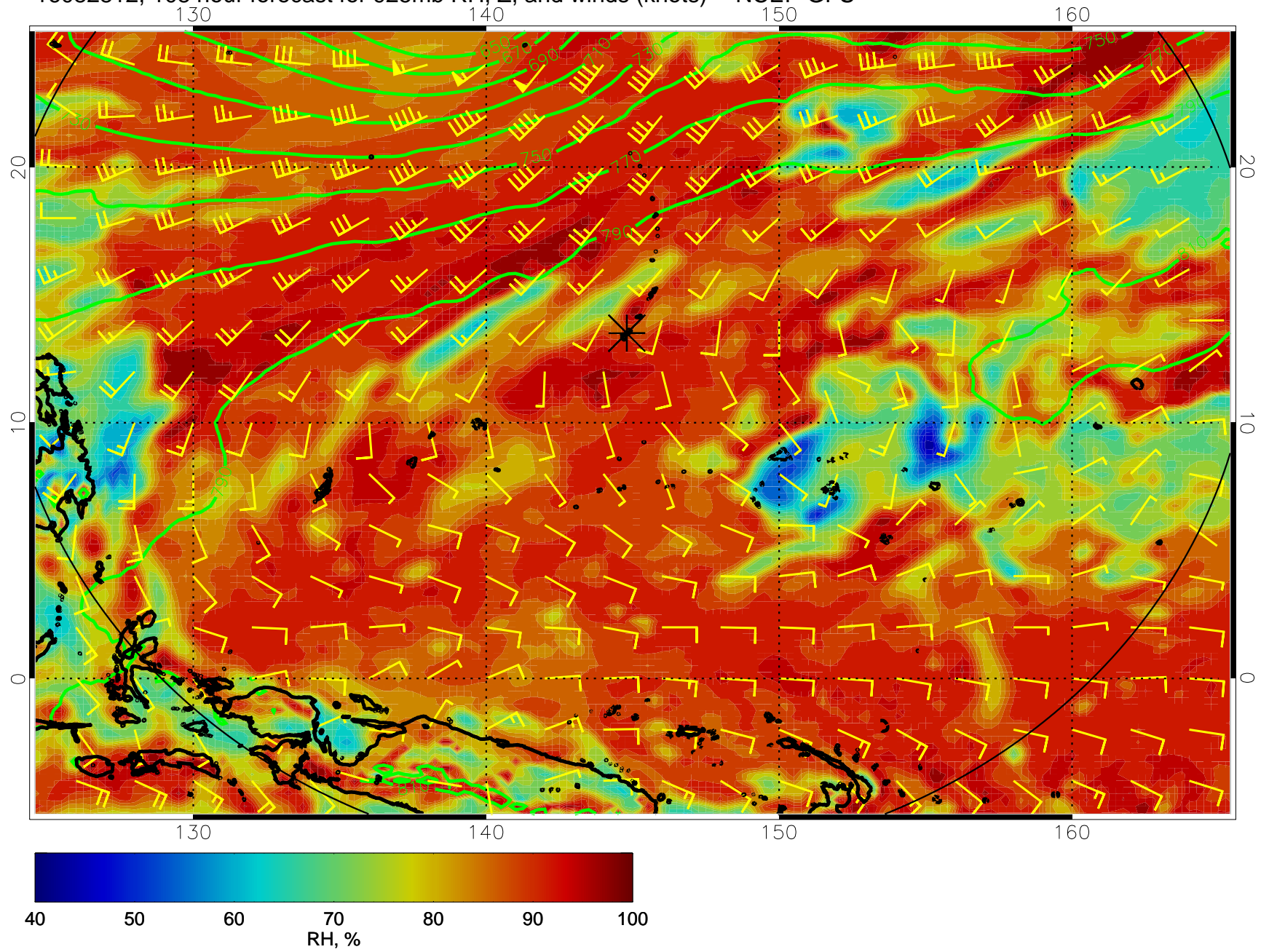
16082812, 108 hour forecast for 925mb RH, Z, and winds (knots) -- NCEP GFS
