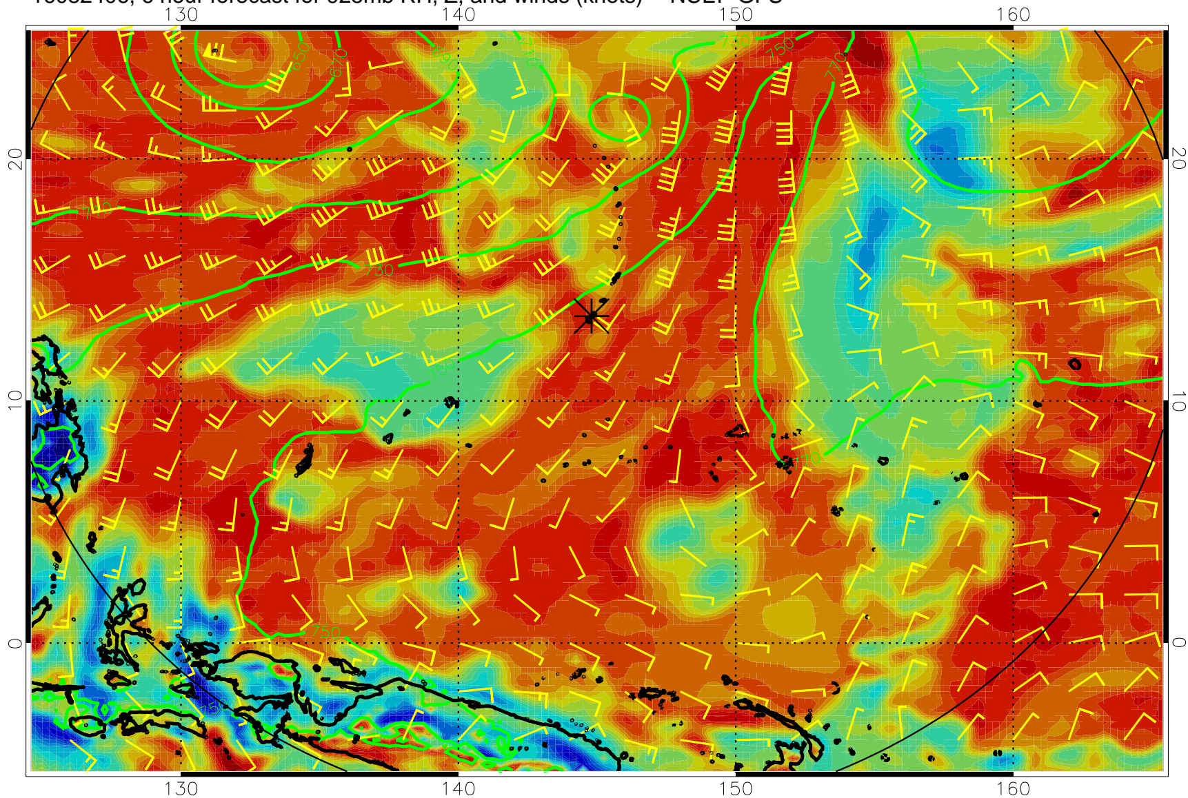
16082406, 6 hour forecast for 925mb RH, Z, and winds (knots) -- NCEP GFS
