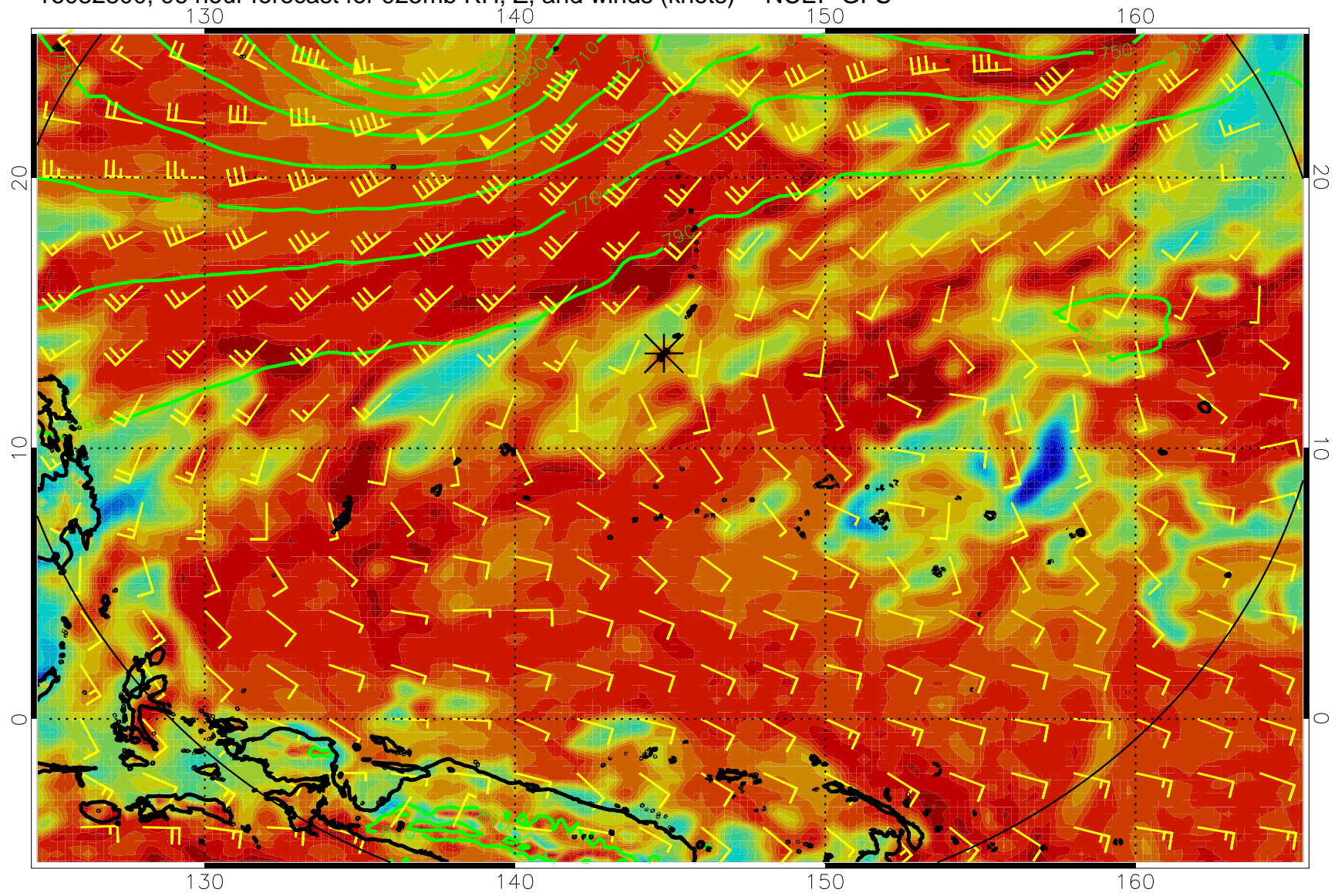
16082800, 96 hour forecast for 925mb RH, Z, and winds (knots) -- NCEP GFS
