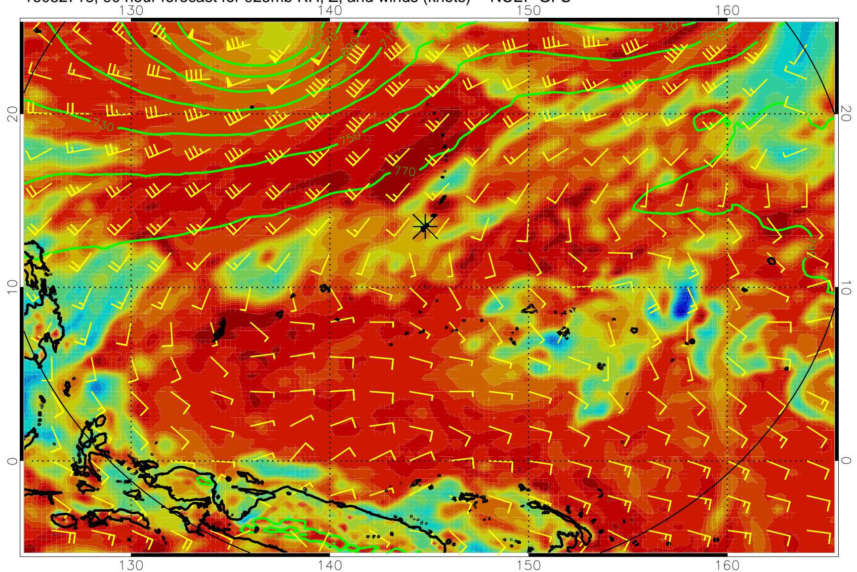
16082718, 90 hour forecast for 925mb RH, Z, and winds (knots) -- NCEP GFS
