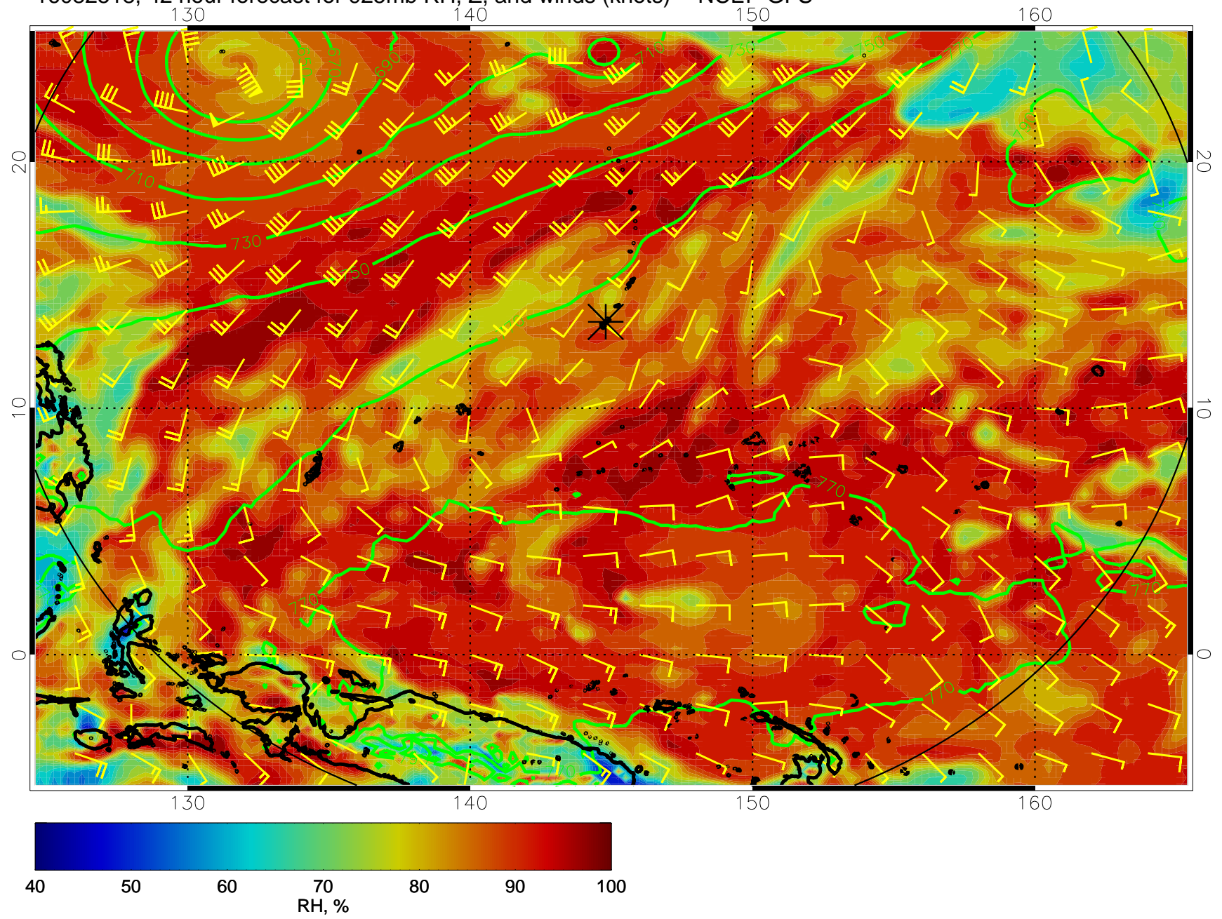
16082518, 42 hour forecast for 925mb RH, Z, and winds (knots) -- NCEP GFS
