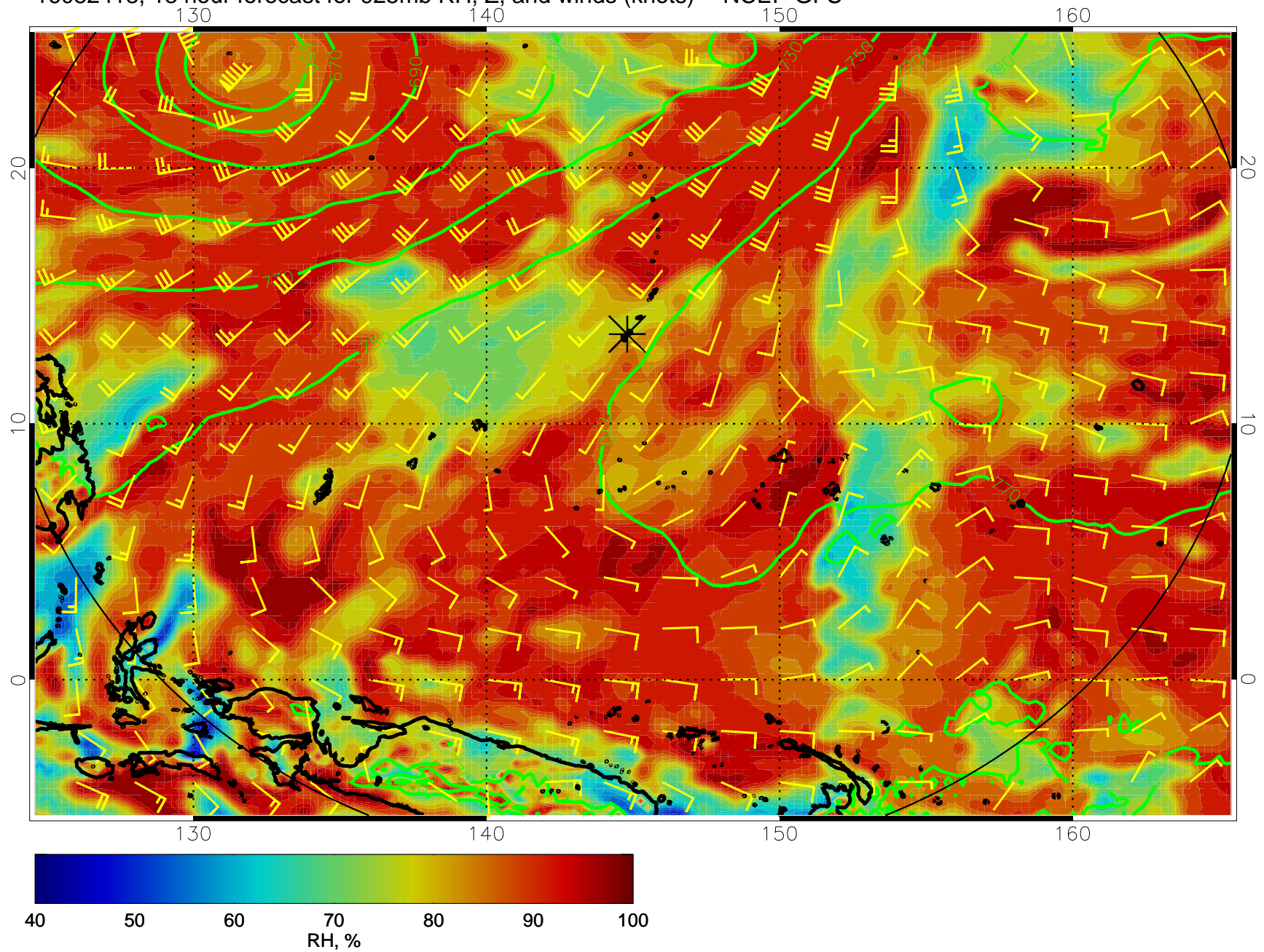
16082418, 18 hour forecast for 925mb RH, Z, and winds (knots) -- NCEP GFS
