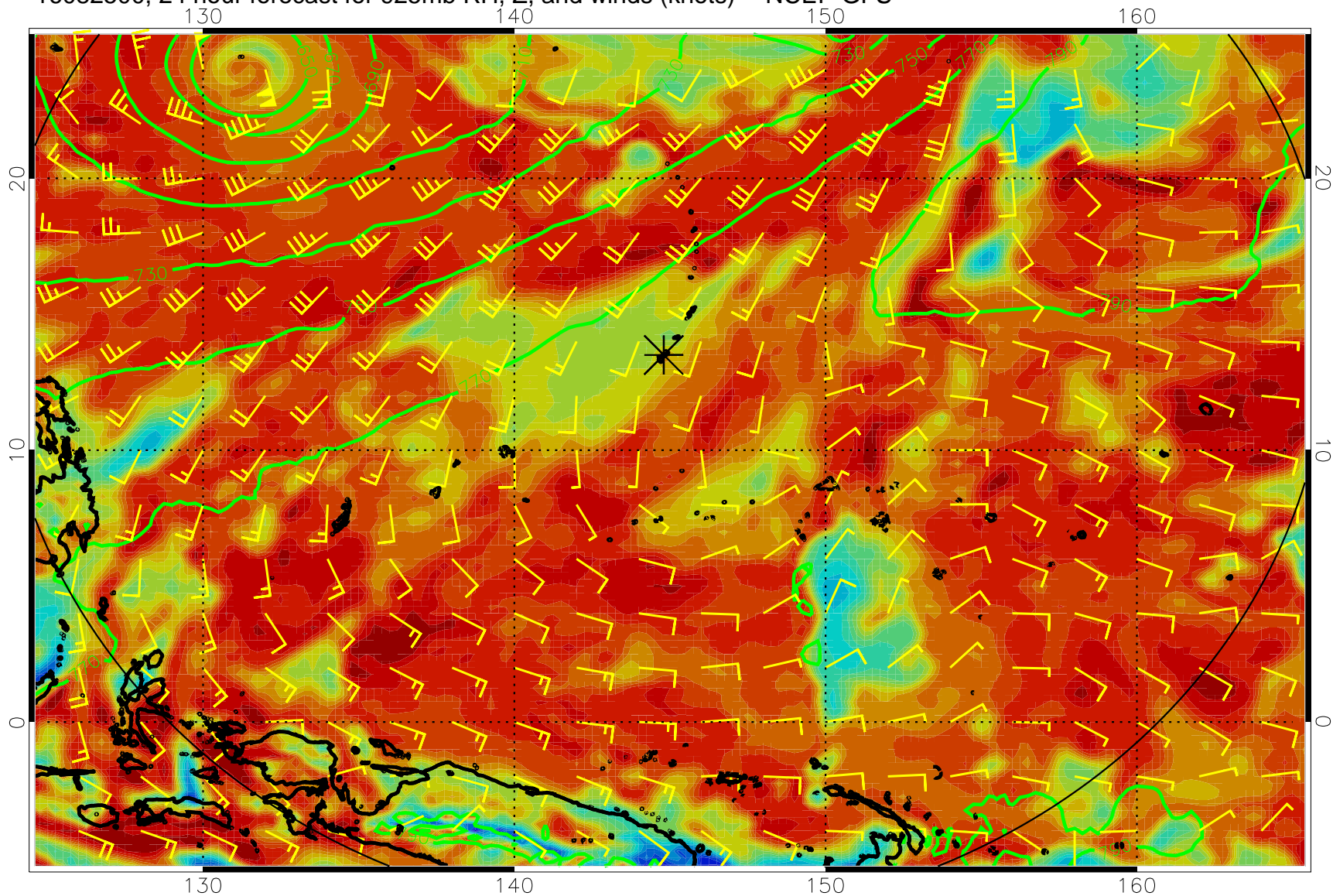
16082500, 24 hour forecast for 925mb RH, Z, and winds (knots) -- NCEP GFS
