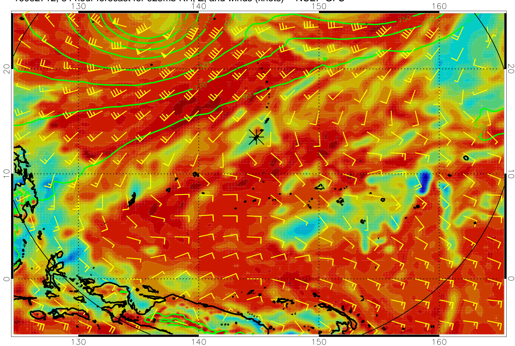
16082712, 84 hour forecast for 925mb RH, Z, and winds (knots) -- NCEP GFS
