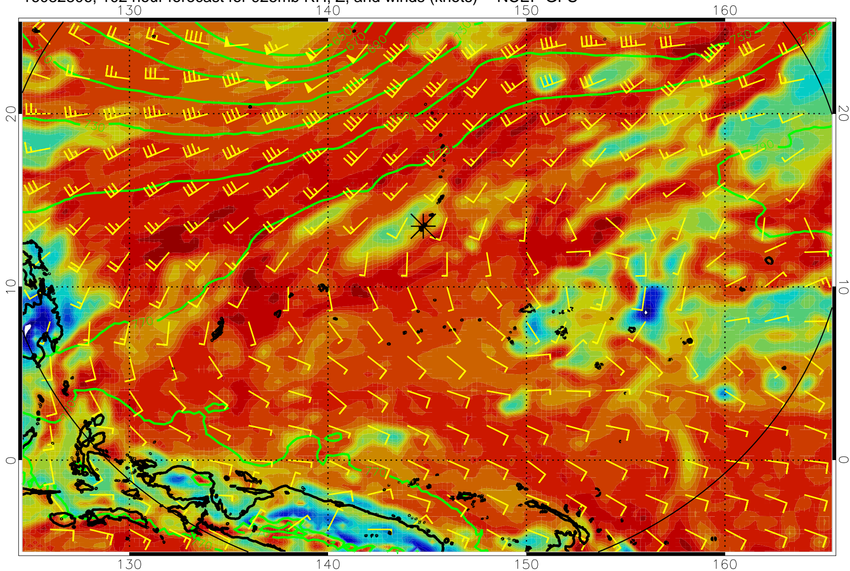
16082806, 102 hour forecast for 925mb RH, Z, and winds (knots) -- NCEP GFS
