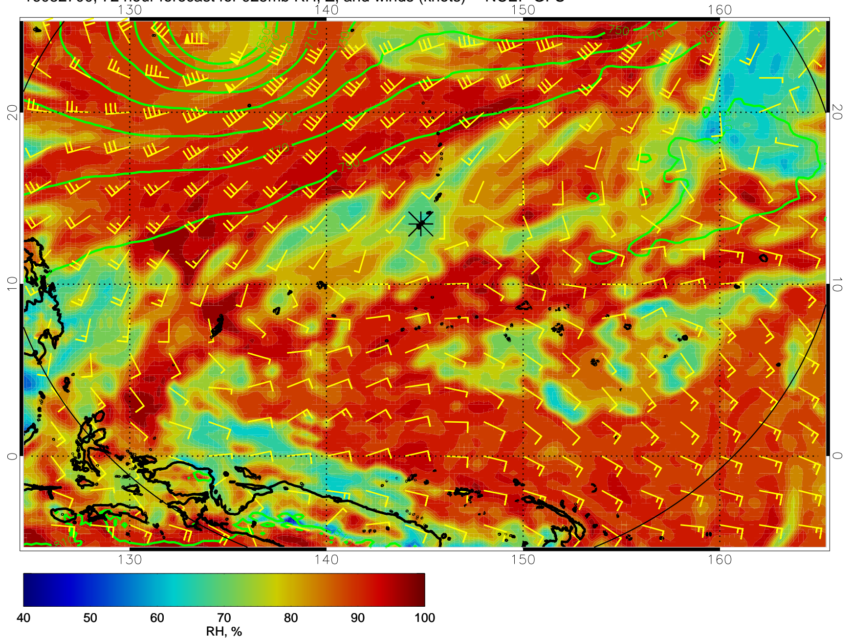
16082700, 72 hour forecast for 925mb RH, Z, and winds (knots) -- NCEP GFS
