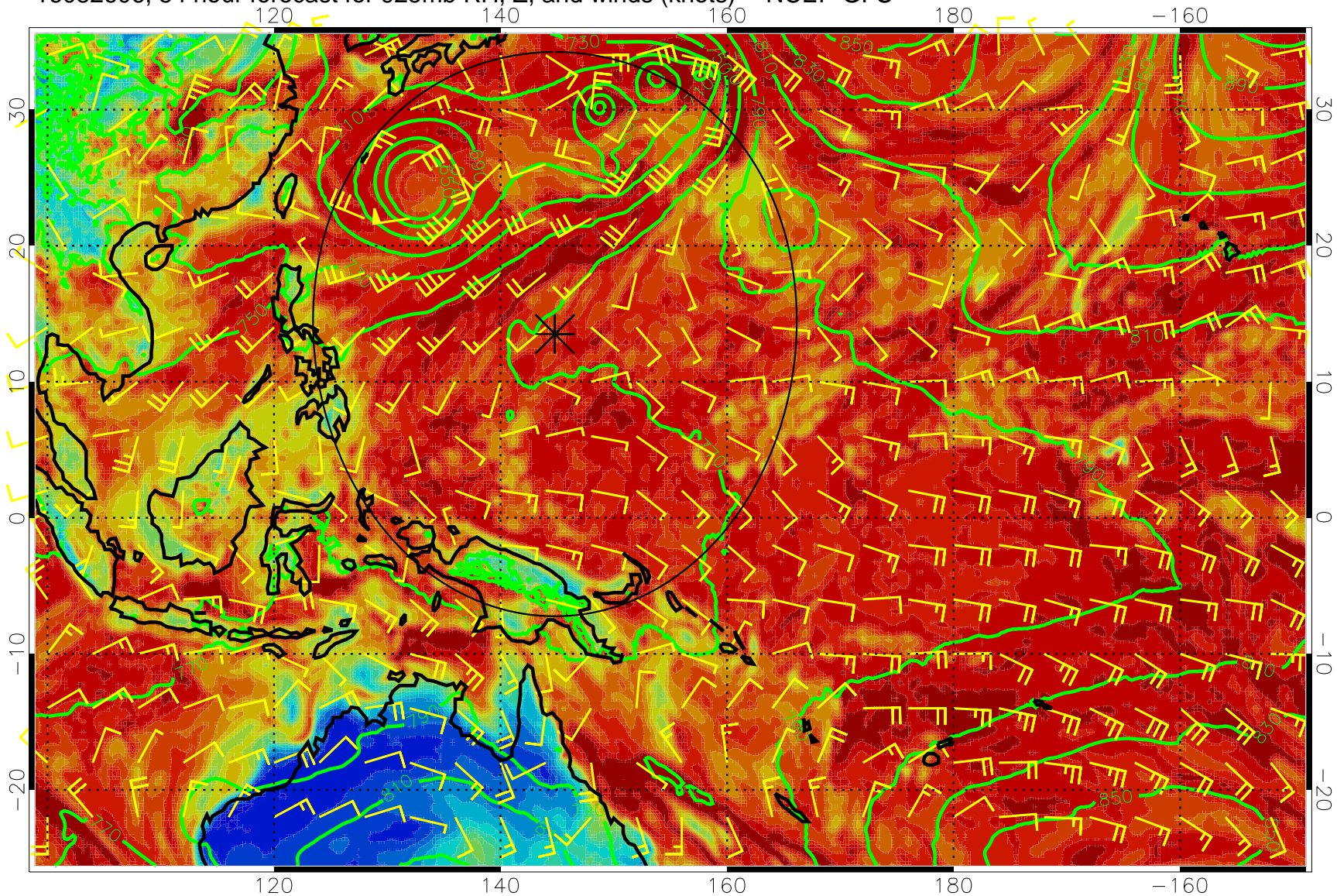
16082606, 54 hour forecast for 925mb RH, Z, and winds (knots) -- NCEP GFS
