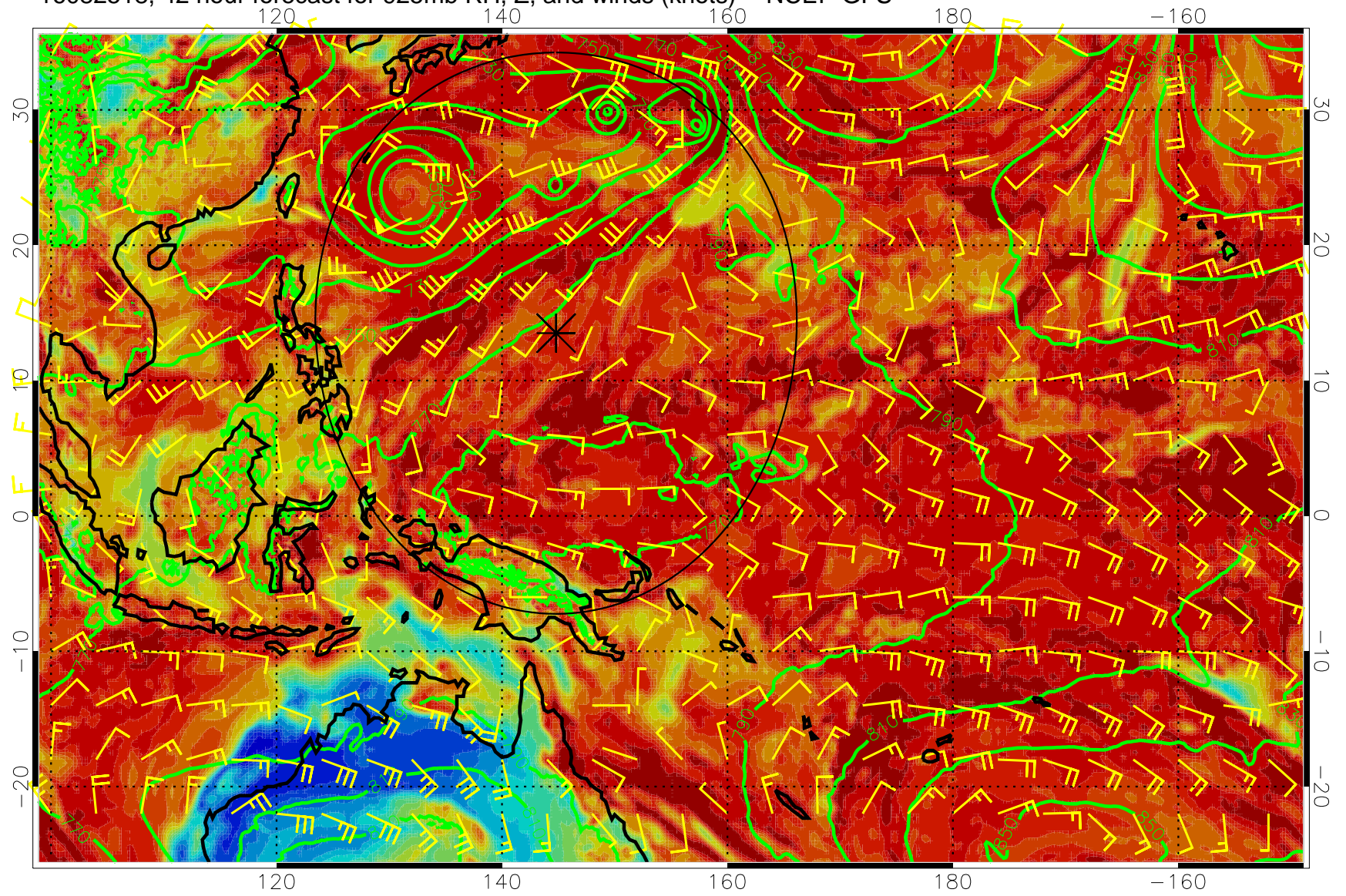
16082518, 42 hour forecast for 925mb RH, Z, and winds (knots) -- NCEP GFS
