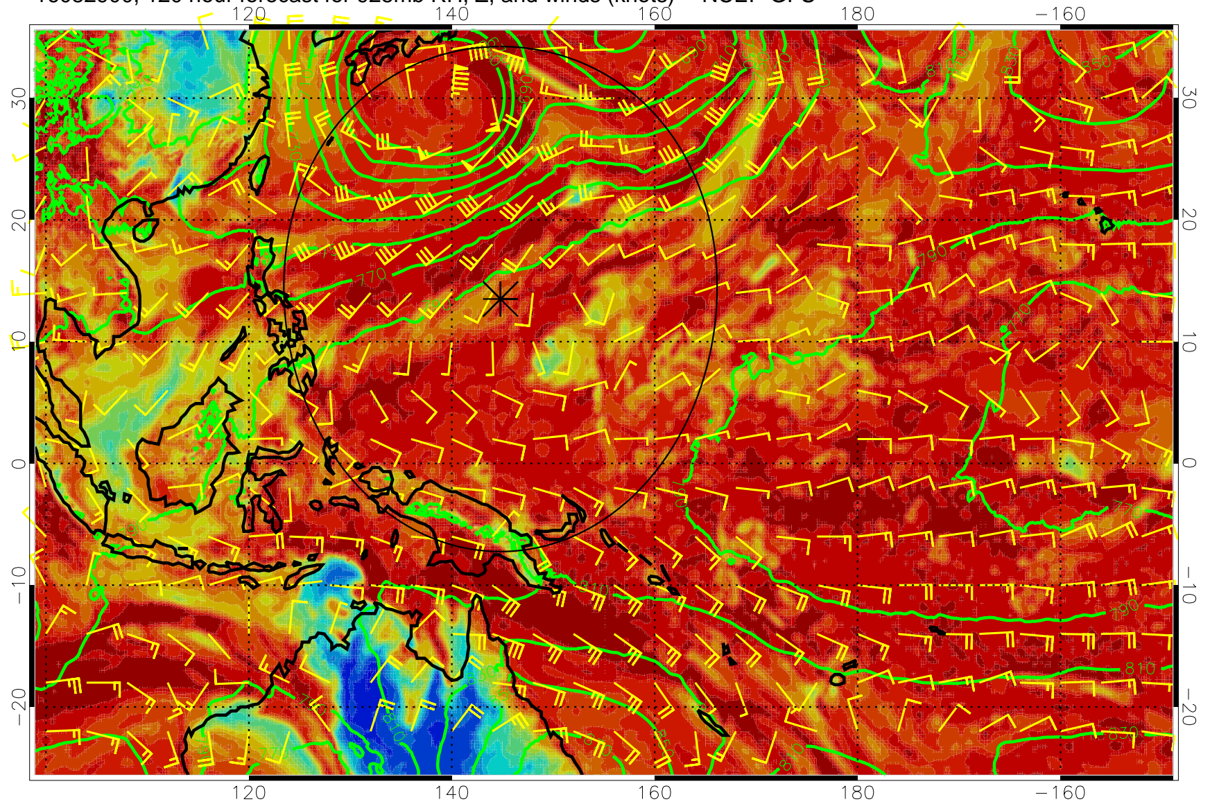
16082900, 120 hour forecast for 925mb RH, Z, and winds (knots) -- NCEP GFS
