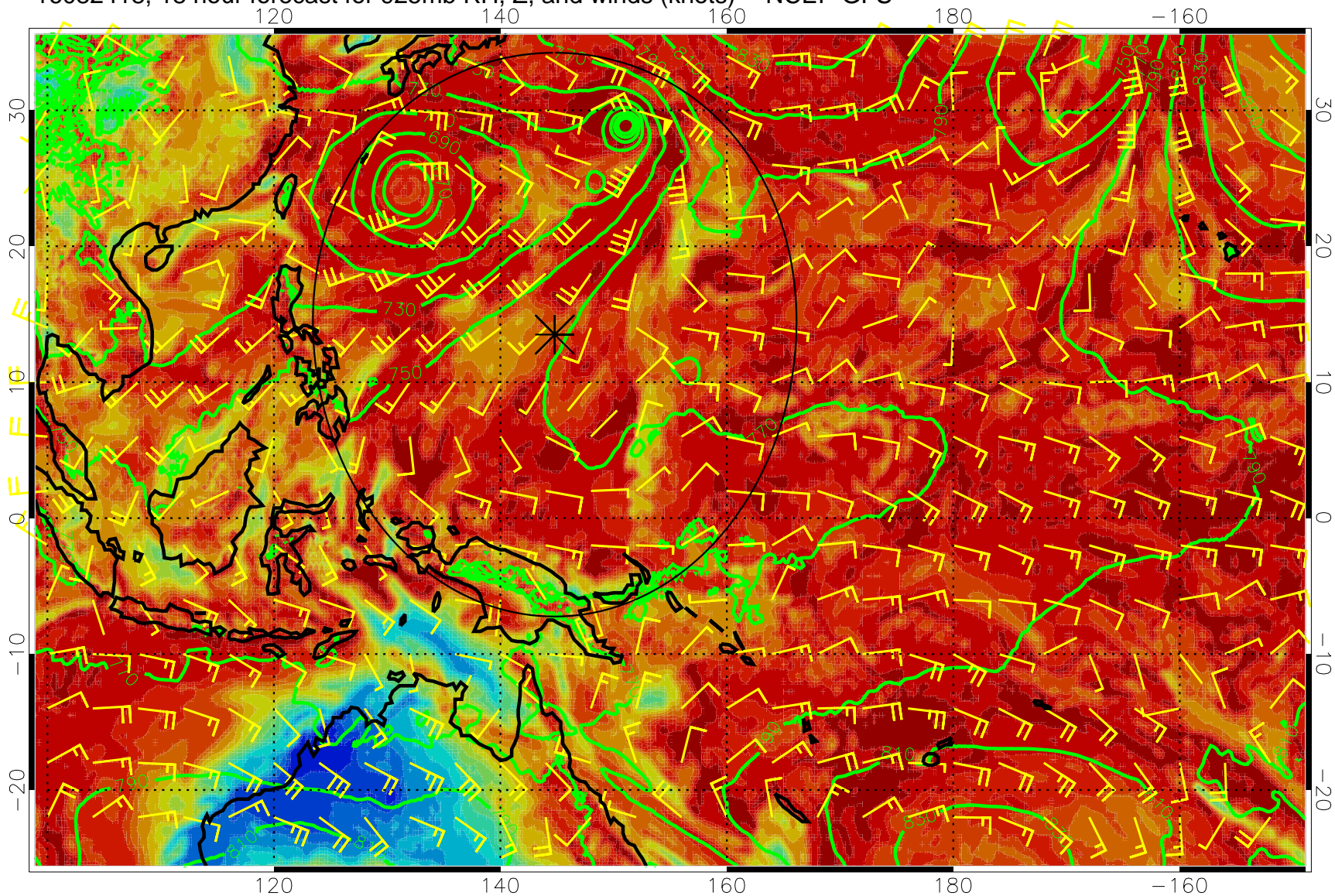
16082418, 18 hour forecast for 925mb RH, Z, and winds (knots) -- NCEP GFS
