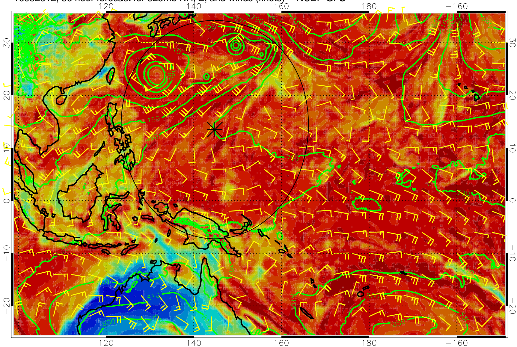
16082512, 36 hour forecast for 925mb RH, Z, and winds (knots) -- NCEP GFS
