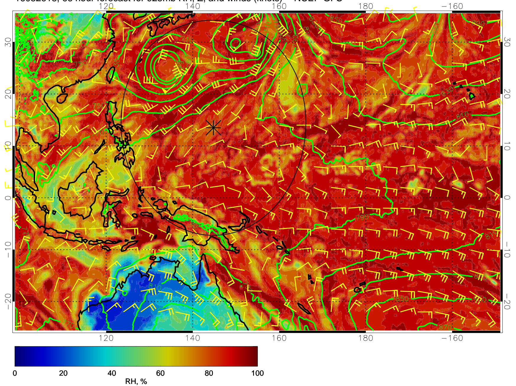
16082618, 66 hour forecast for 925mb RH, Z, and winds (knots) -- NCEP GFS
