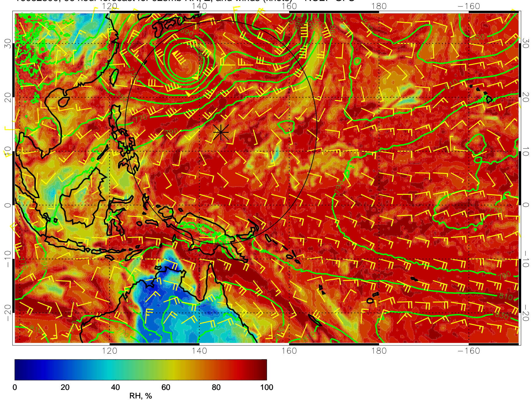
16082800, 96 hour forecast for 925mb RH, Z, and winds (knots) -- NCEP GFS
