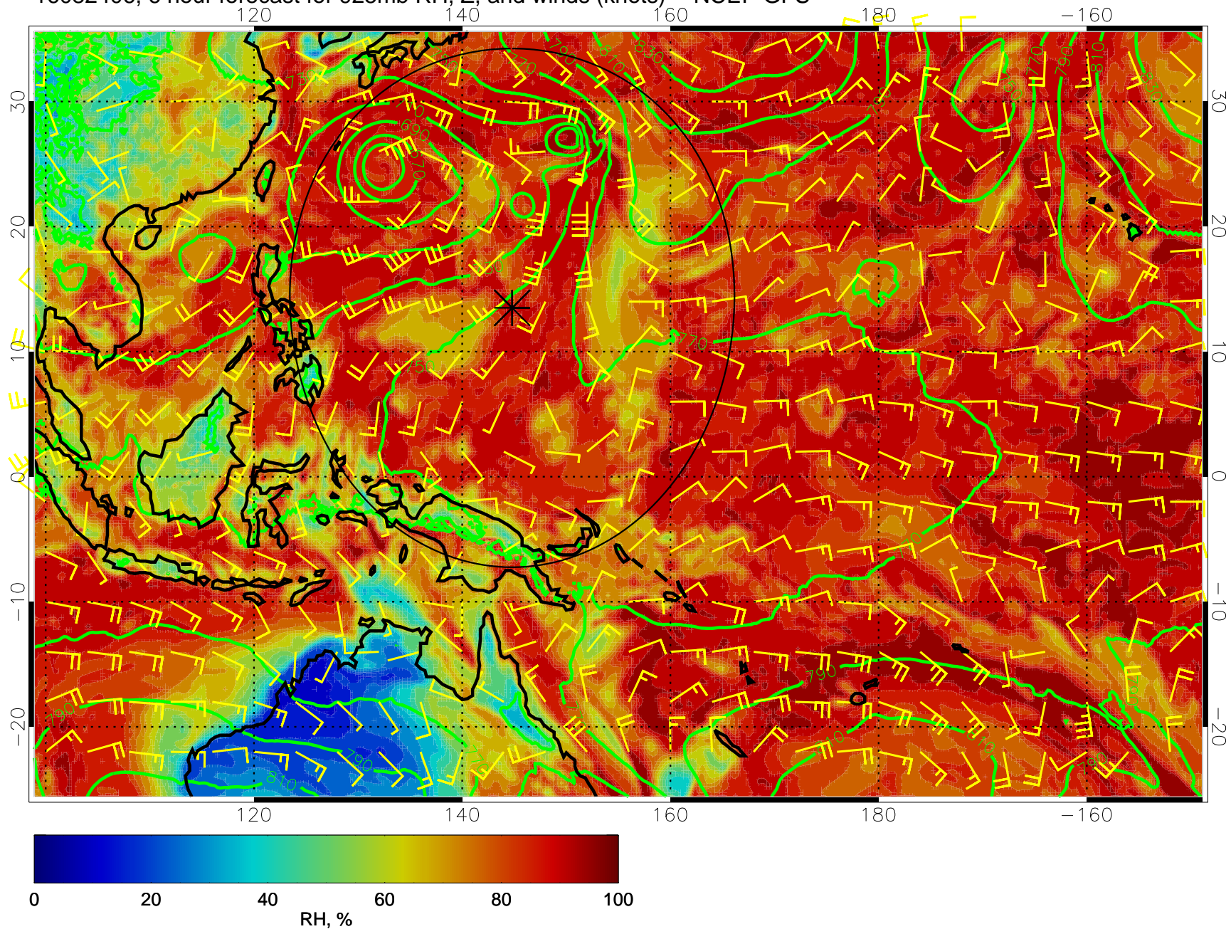
16082406, 6 hour forecast for 925mb RH, Z, and winds (knots) -- NCEP GFS
