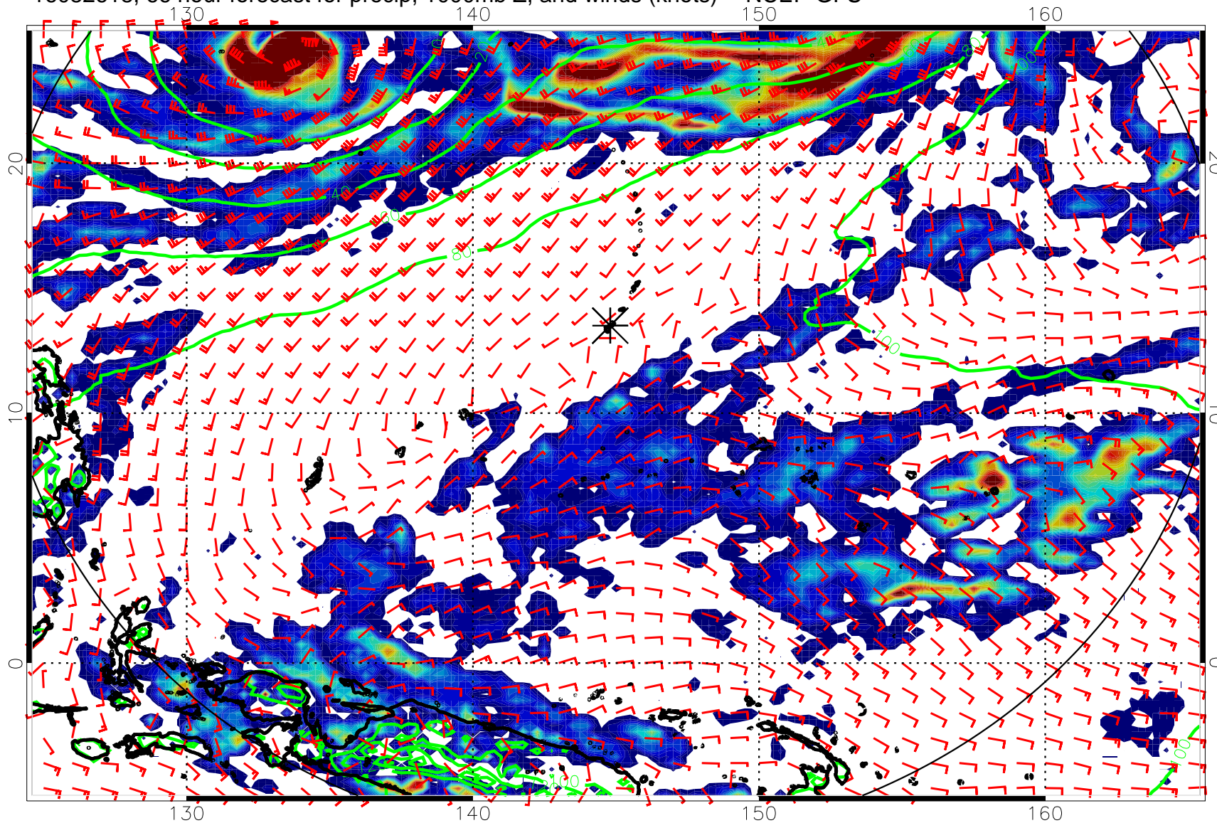
16082618, 66 hour forecast for precip, 1000mb Z, and winds (knots) -- NCEP GFS
