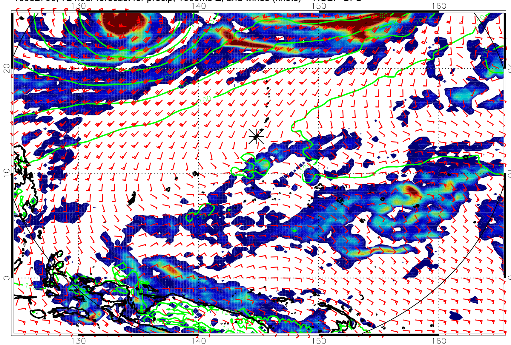
16082700, 72 hour forecast for precip, 1000mb Z, and winds (knots) -- NCEP GFS
