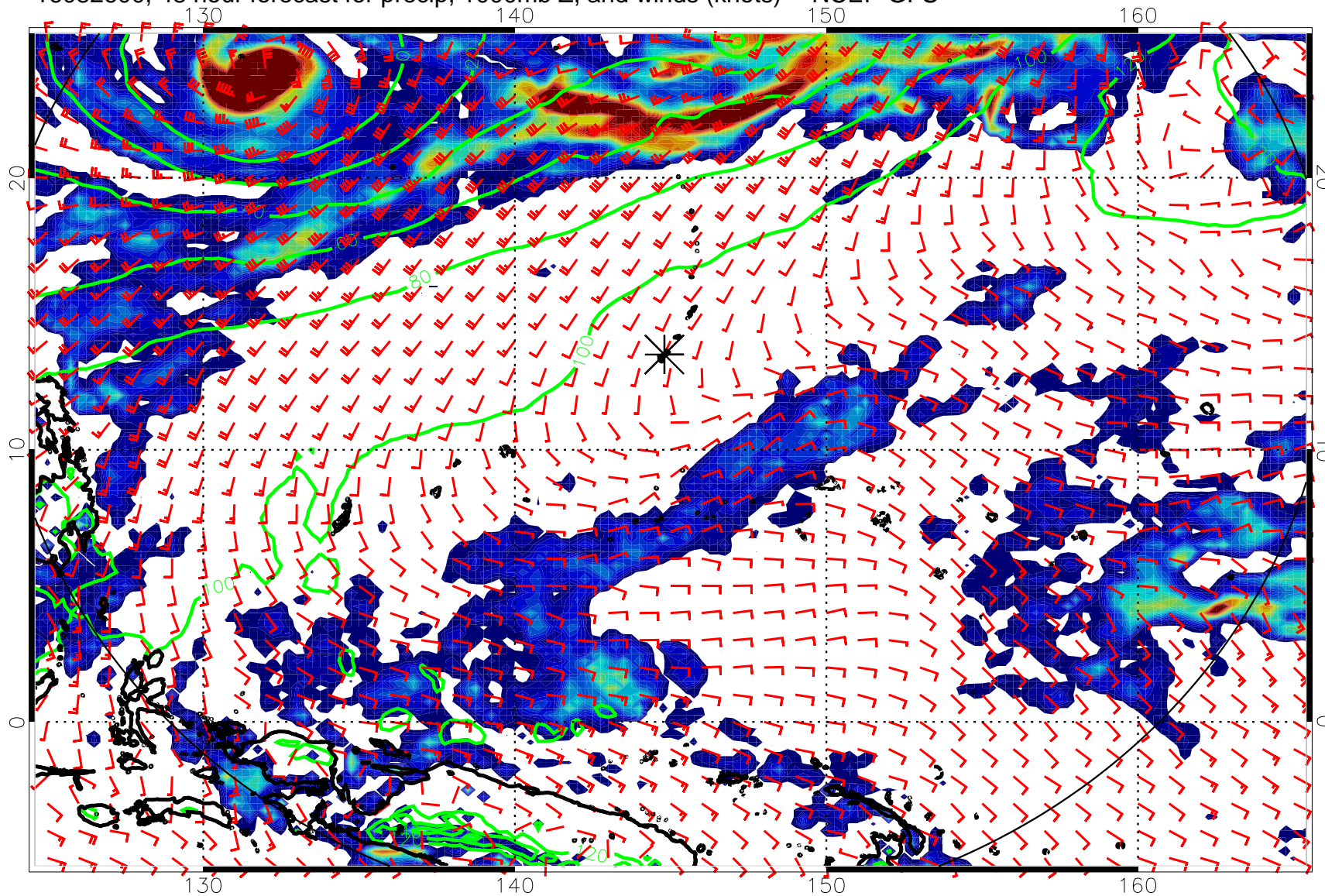
16082600, 48 hour forecast for precip, 1000mb Z, and winds (knots) -- NCEP GFS
