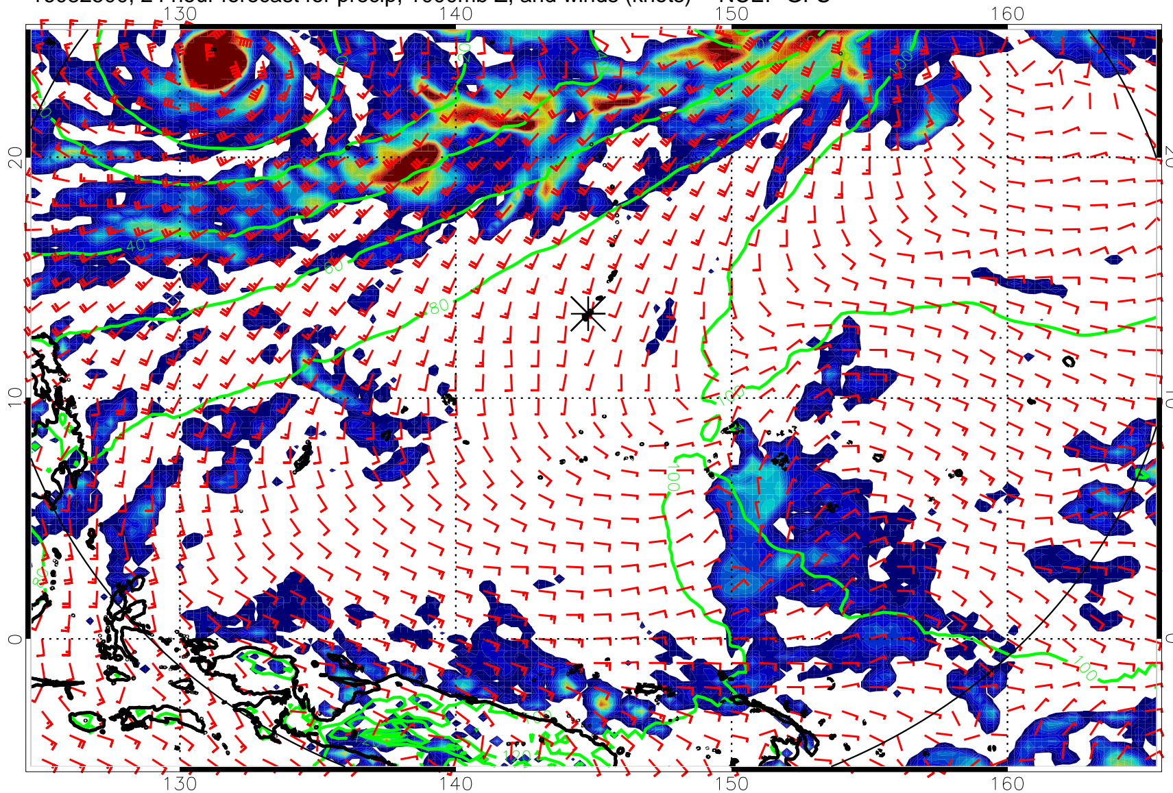
16082500, 24 hour forecast for precip, 1000mb Z, and winds (knots) -- NCEP GFS
