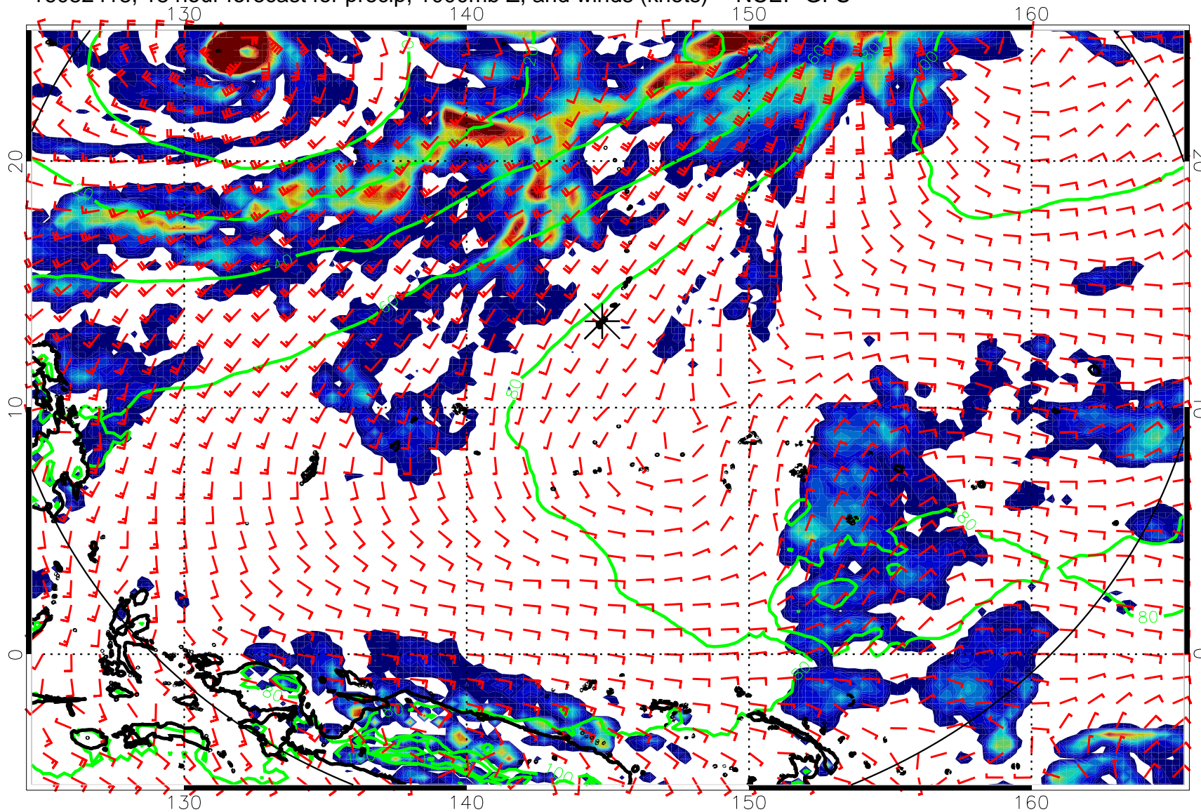
16082418, 18 hour forecast for precip, 1000mb Z, and winds (knots) -- NCEP GFS
