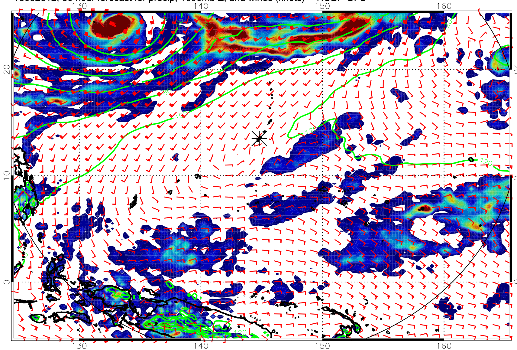
16082612, 60 hour forecast for precip, 1000mb Z, and winds (knots) -- NCEP GFS
