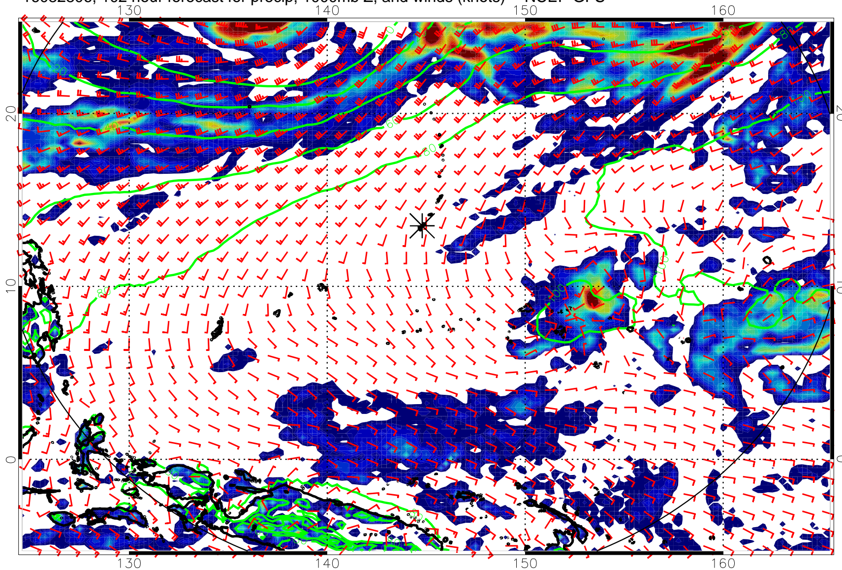
16082806, 102 hour forecast for precip, 1000mb Z, and winds (knots) -- NCEP GFS
