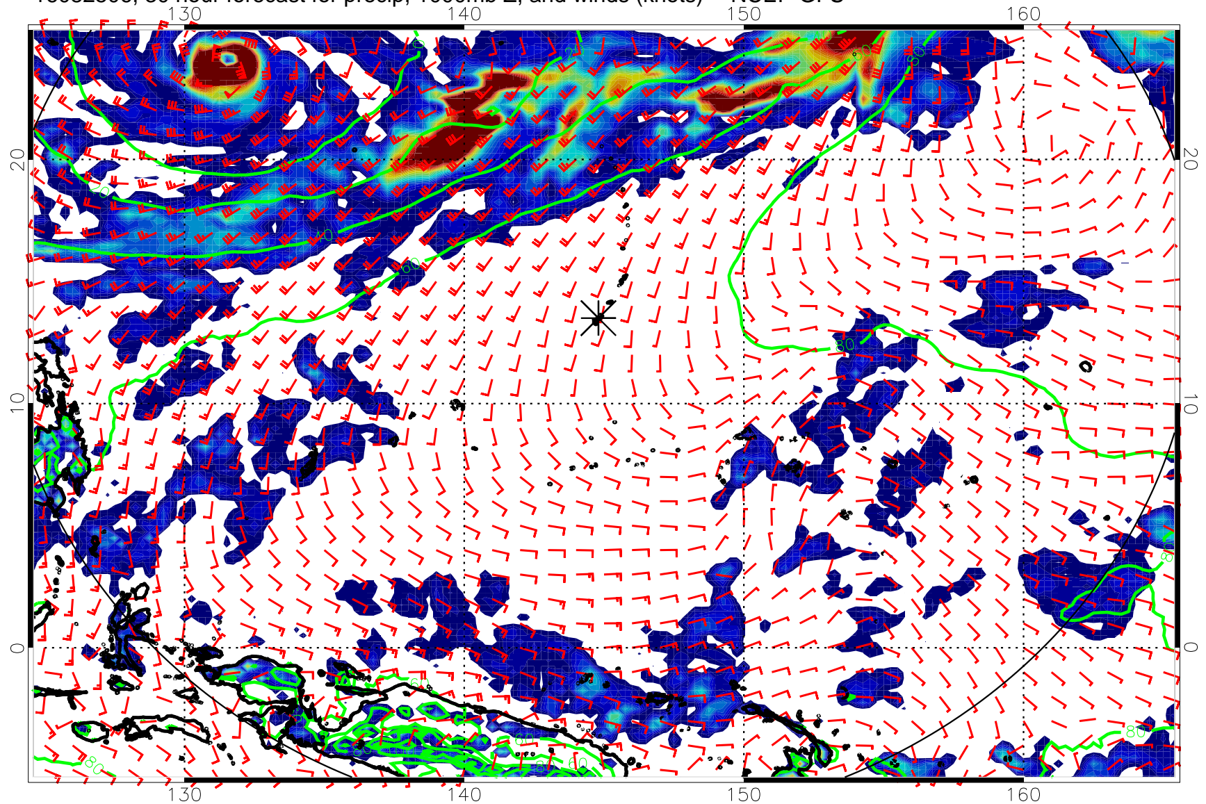
16082506, 30 hour forecast for precip, 1000mb Z, and winds (knots) -- NCEP GFS
