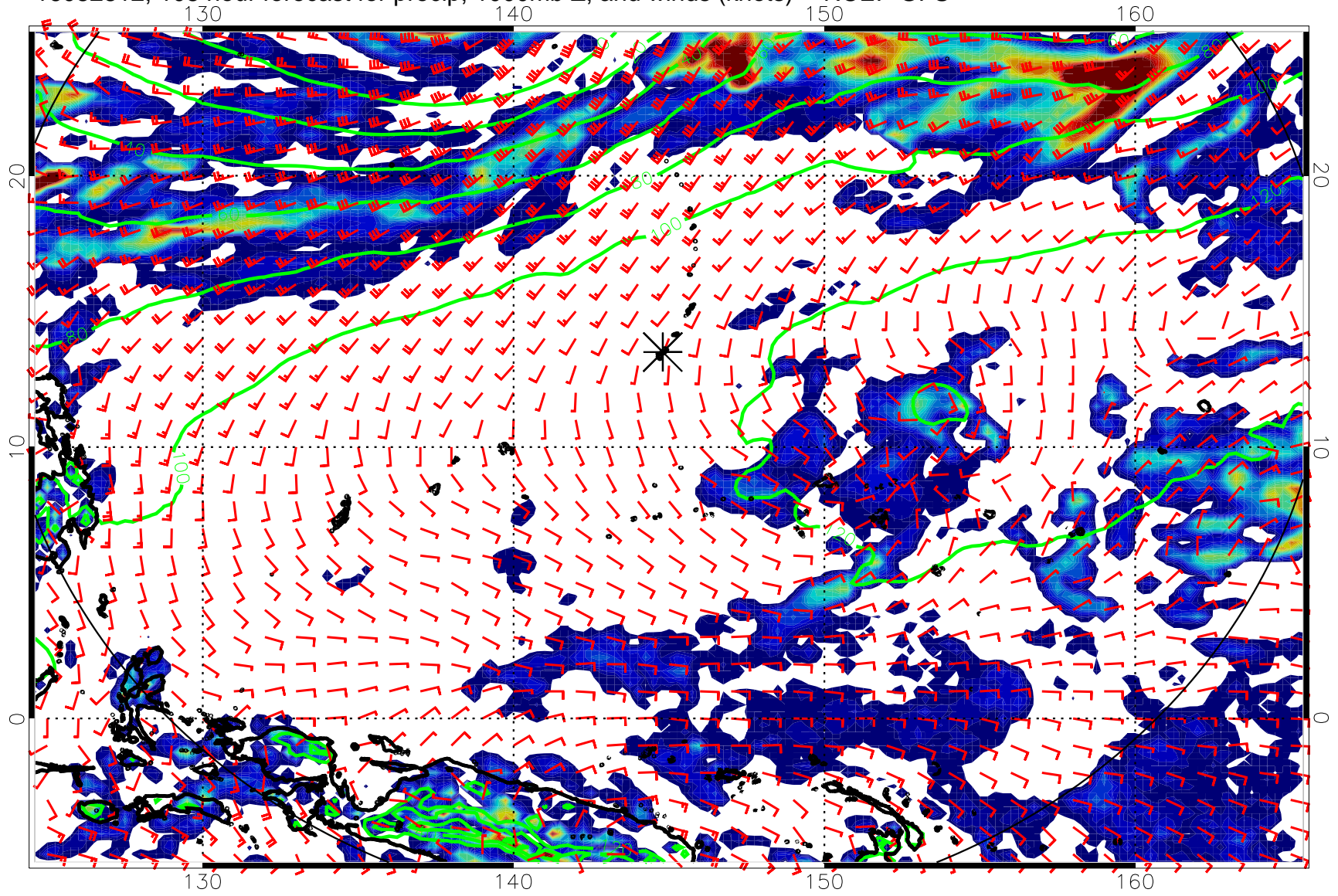
16082812, 108 hour forecast for precip, 1000mb Z, and winds (knots) -- NCEP GFS
