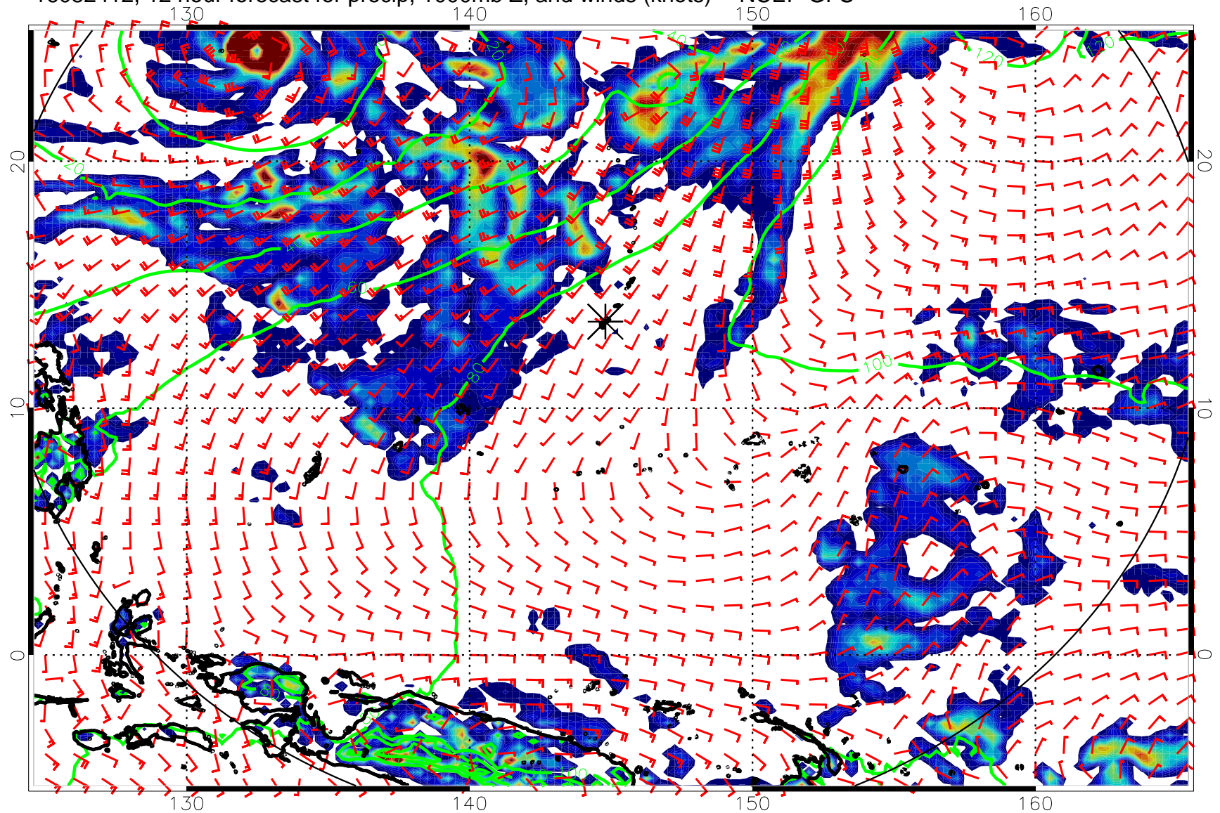
16082412, 12 hour forecast for precip, 1000mb Z, and winds (knots) -- NCEP GFS
