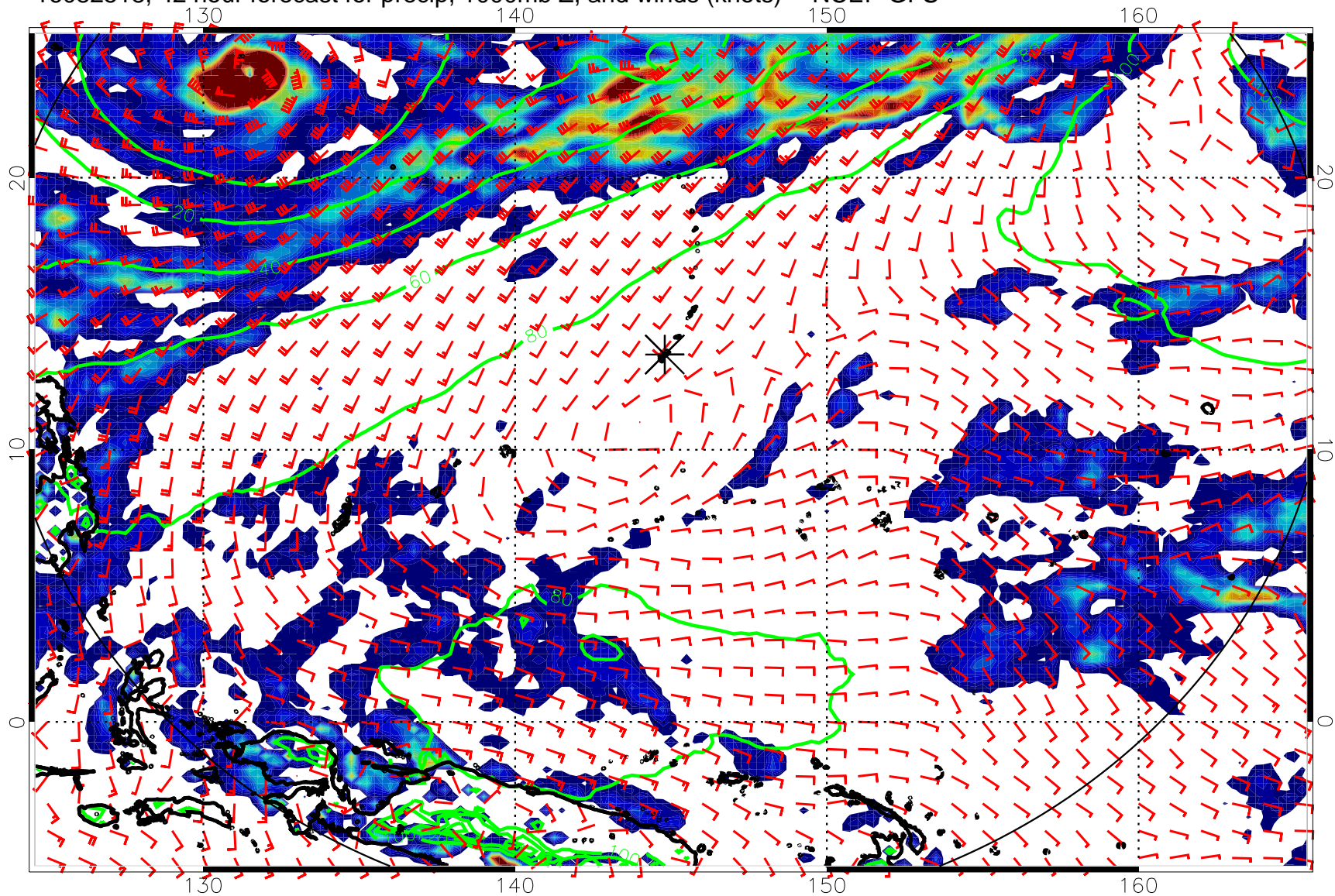
16082518, 42 hour forecast for precip, 1000mb Z, and winds (knots) -- NCEP GFS
