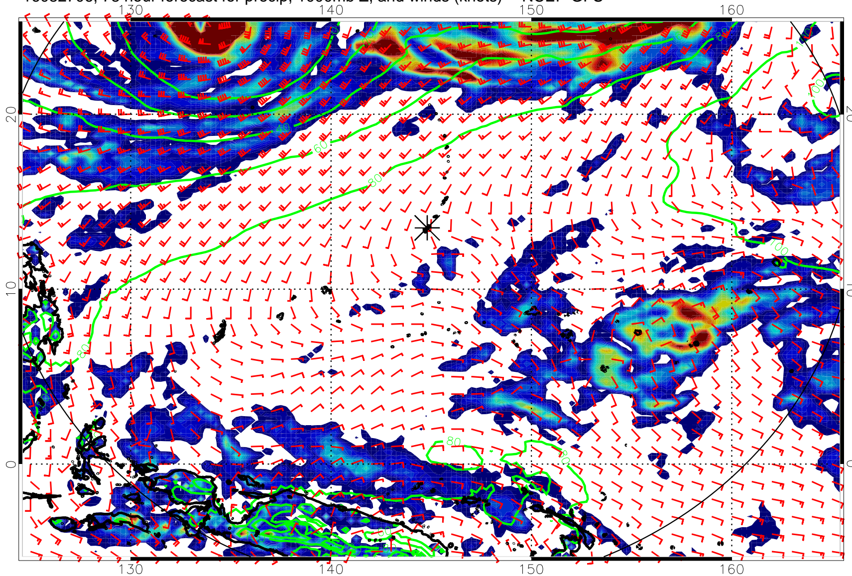
16082706, 78 hour forecast for precip, 1000mb Z, and winds (knots) -- NCEP GFS
