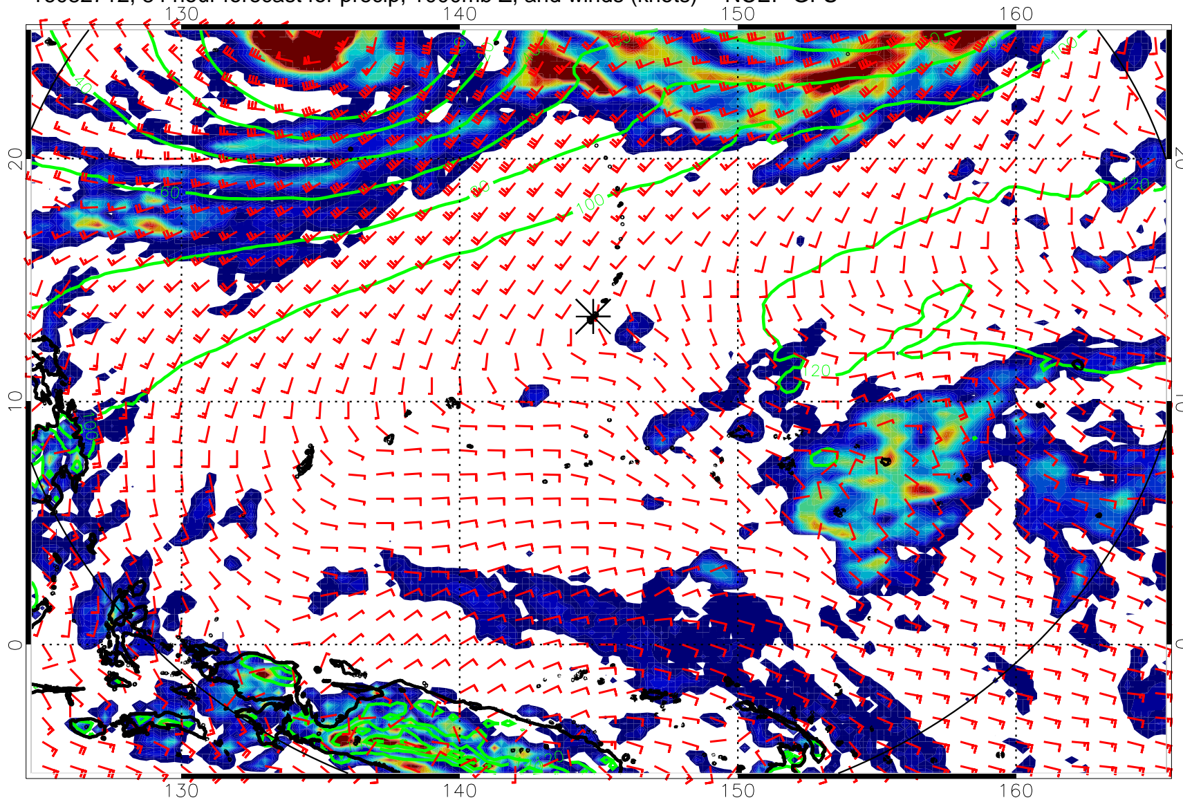
16082712, 84 hour forecast for precip, 1000mb Z, and winds (knots) -- NCEP GFS
