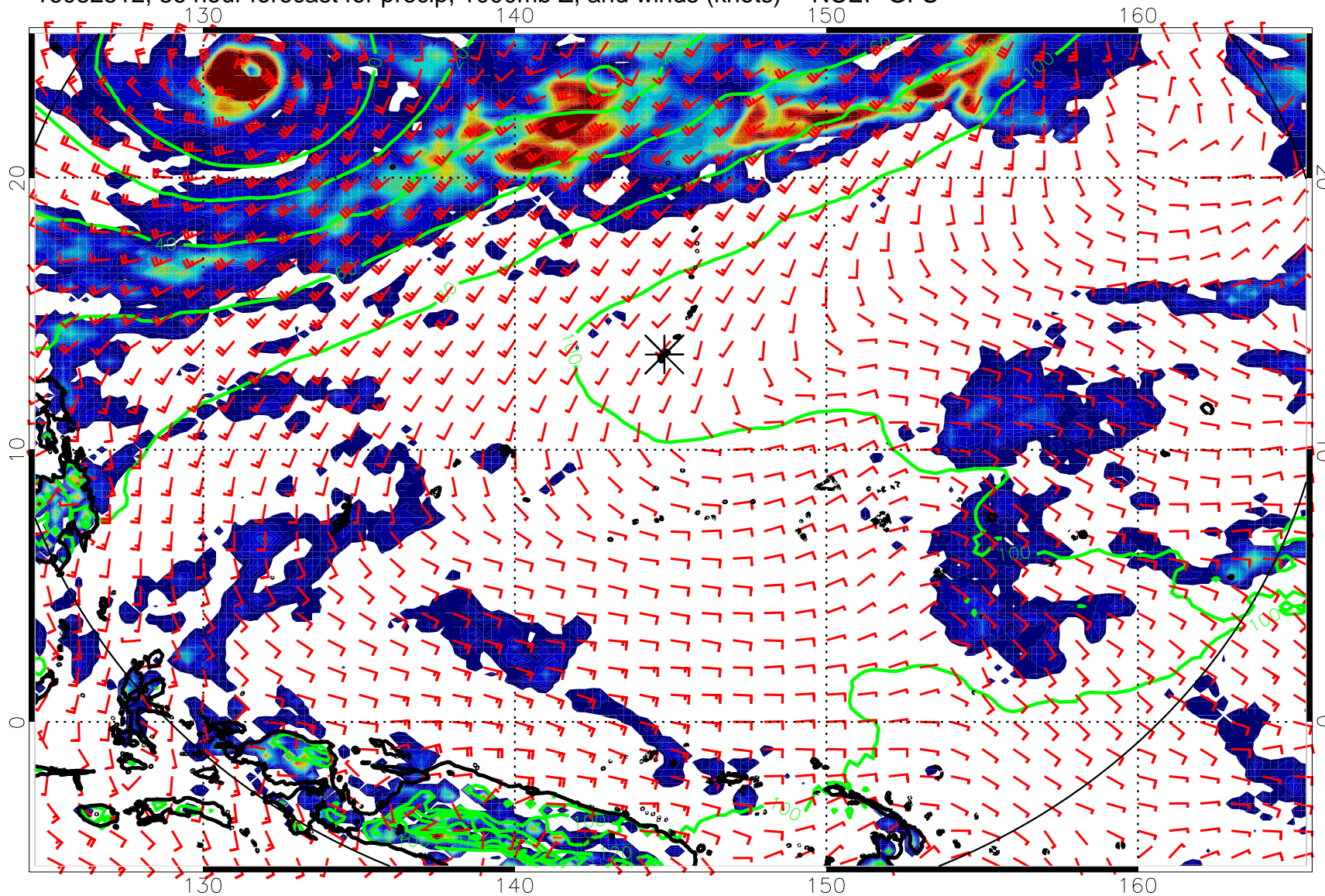
16082512, 36 hour forecast for precip, 1000mb Z, and winds (knots) -- NCEP GFS
