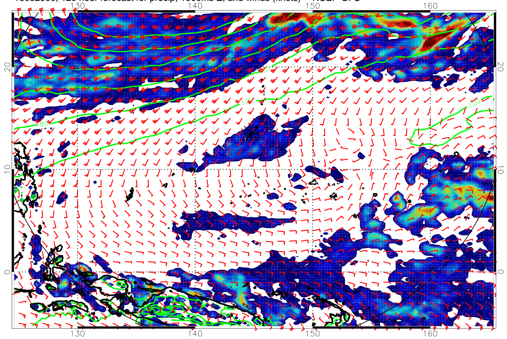
16082900, 120 hour forecast for precip, 1000mb Z, and winds (knots) -- NCEP GFS
