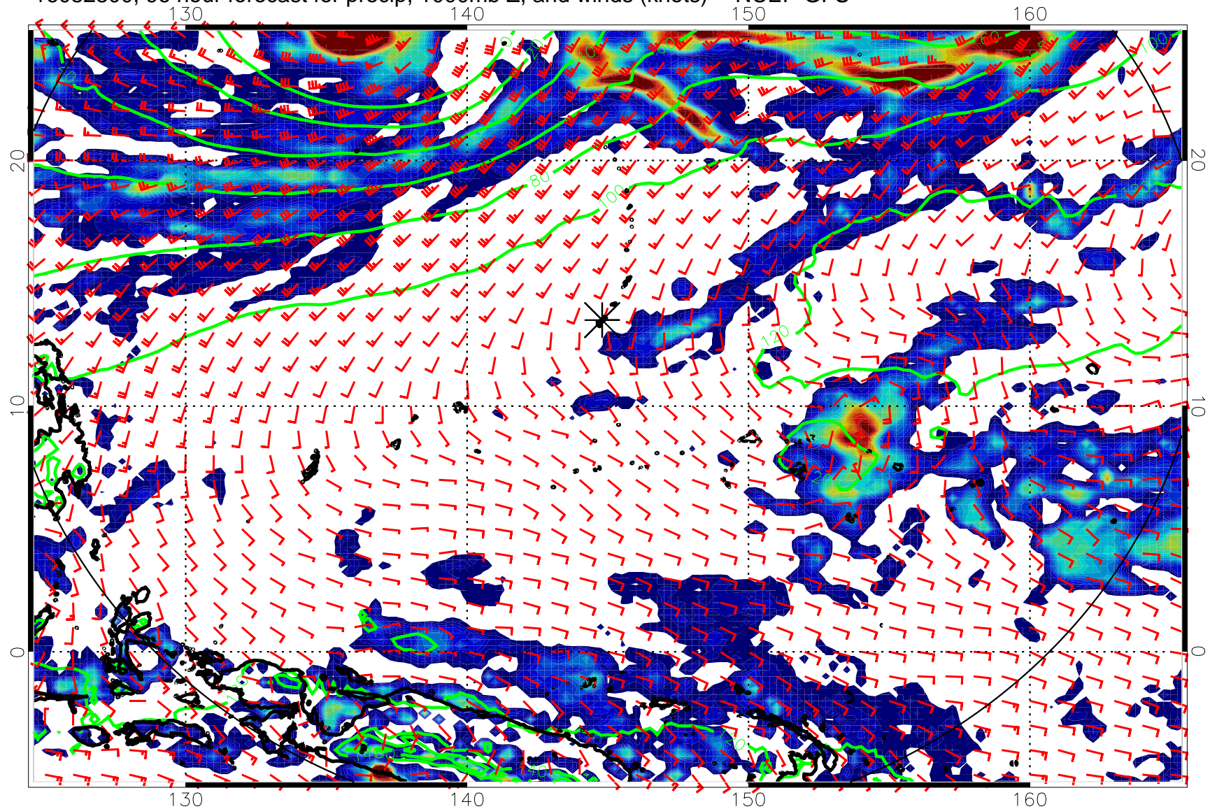
16082800, 96 hour forecast for precip, 1000mb Z, and winds (knots) -- NCEP GFS
