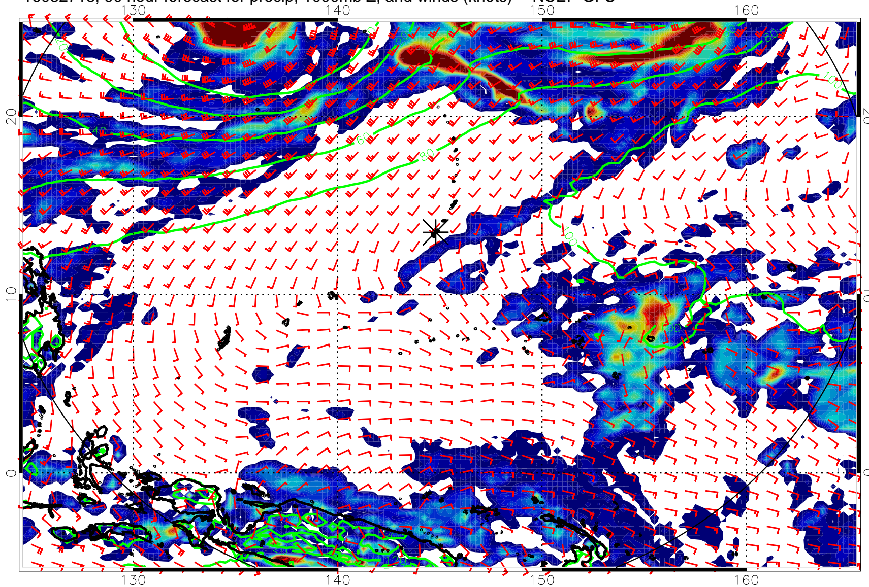
16082718, 90 hour forecast for precip, 1000mb Z, and winds (knots) -- NCEP GFS
