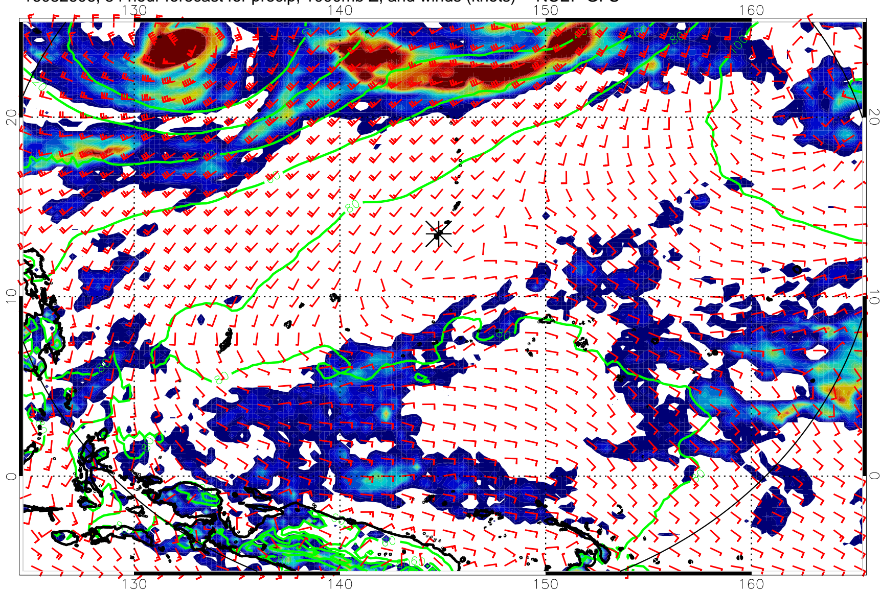
16082606, 54 hour forecast for precip, 1000mb Z, and winds (knots) -- NCEP GFS
