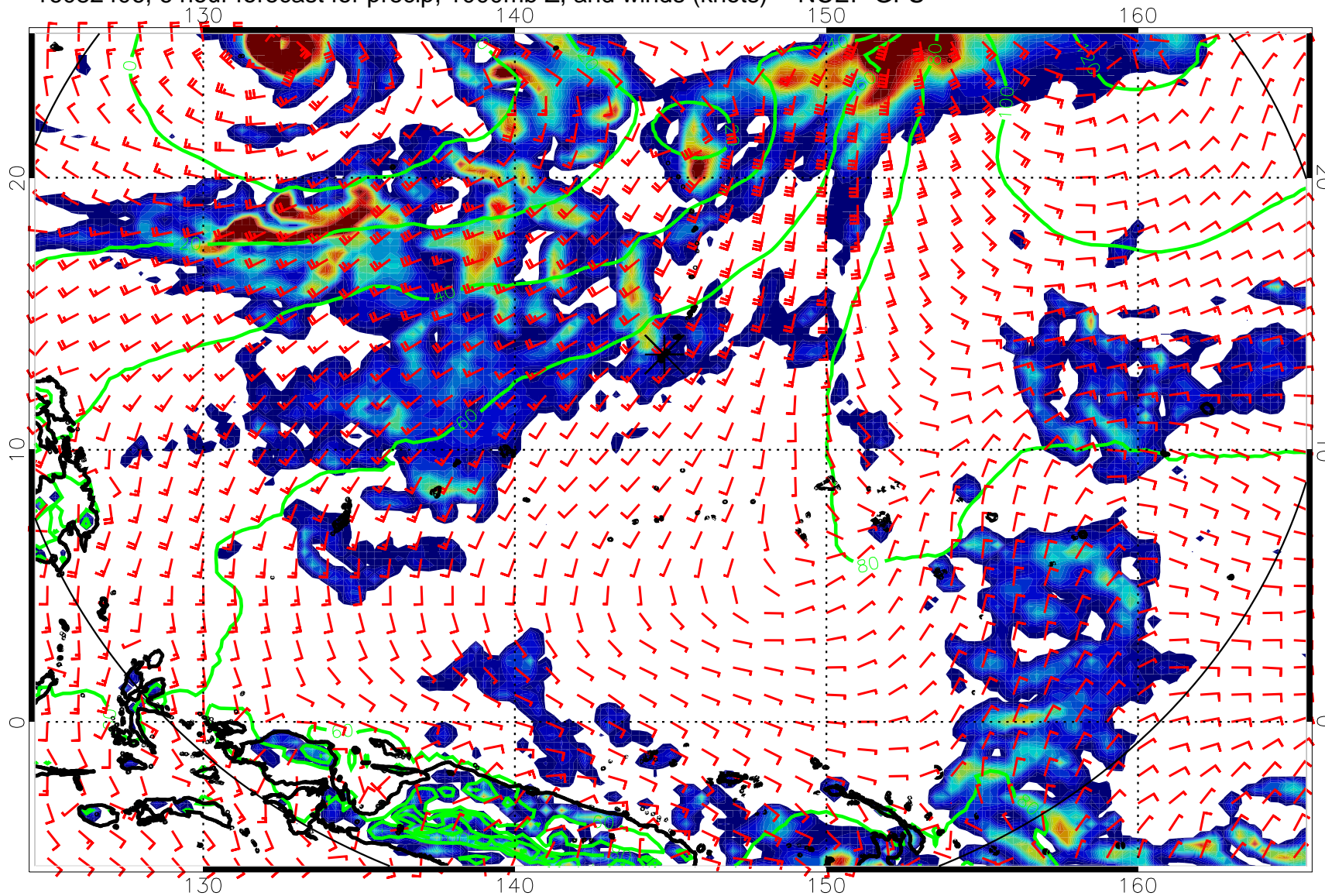
16082406, 6 hour forecast for precip, 1000mb Z, and winds (knots) -- NCEP GFS
