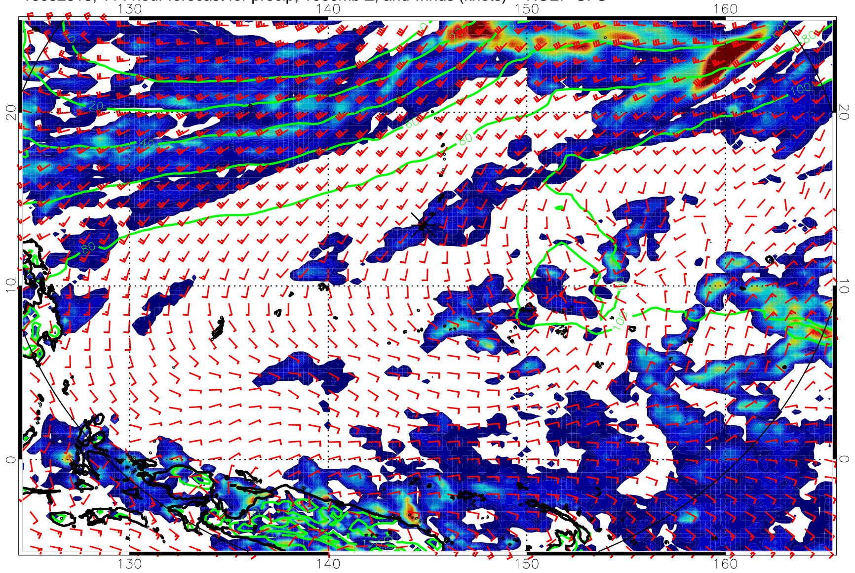
16082818, 114 hour forecast for precip, 1000mb Z, and winds (knots) -- NCEP GFS
