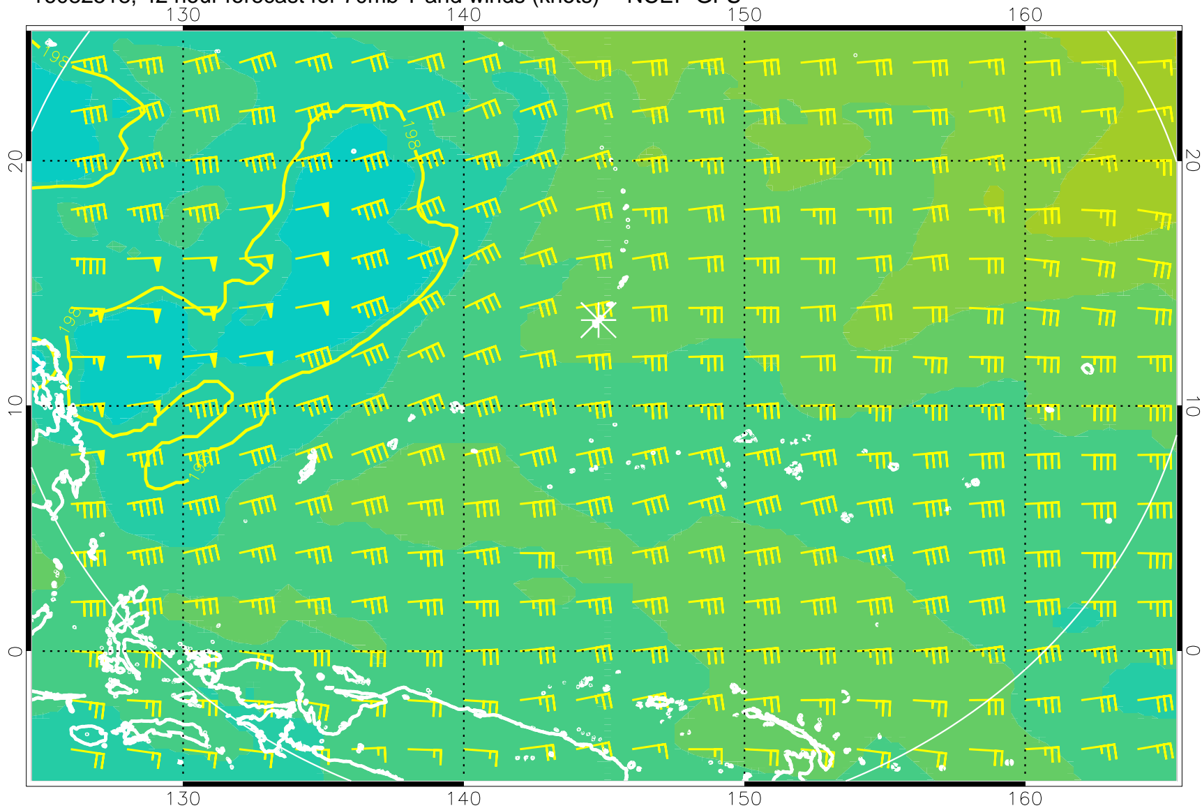
16082518, 42 hour forecast for 70mb T and winds (knots) -- NCEP GFS
