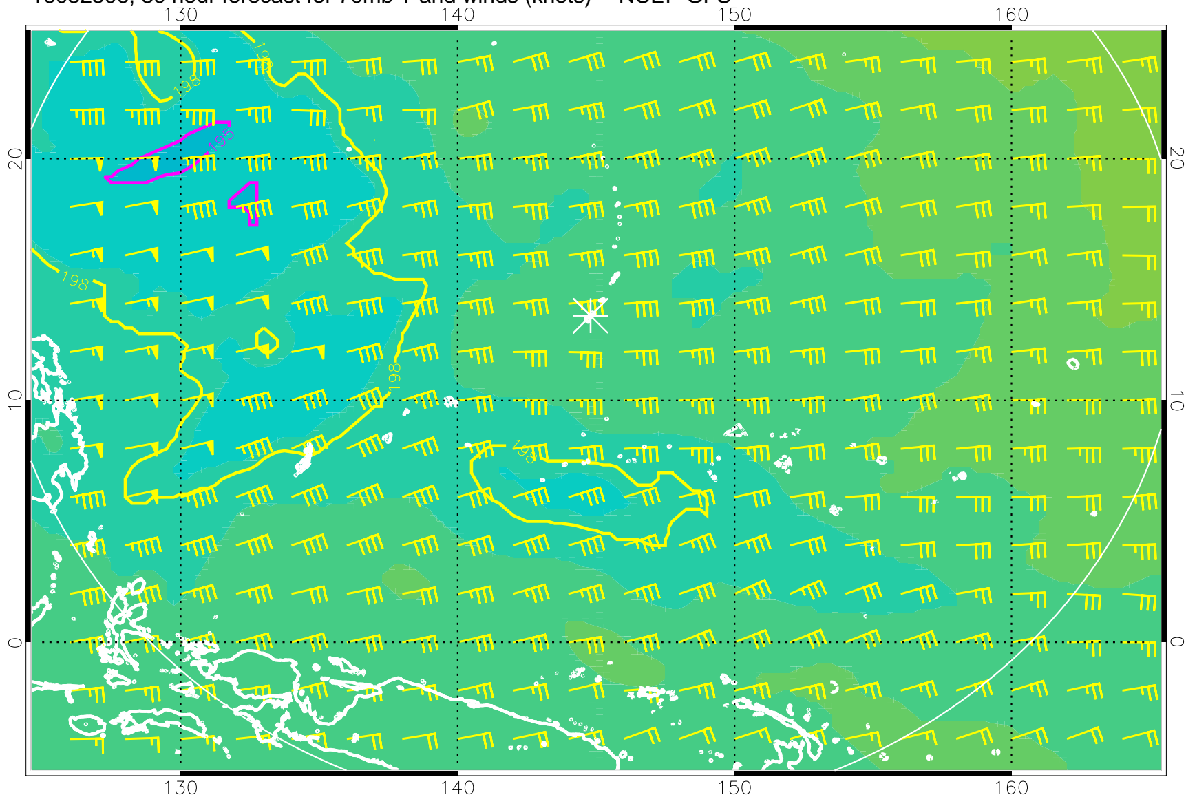
16082506, 30 hour forecast for 70mb T and winds (knots) -- NCEP GFS
