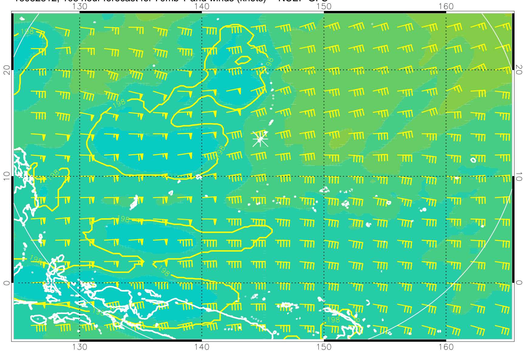
16082812, 108 hour forecast for 70mb T and winds (knots) -- NCEP GFS
