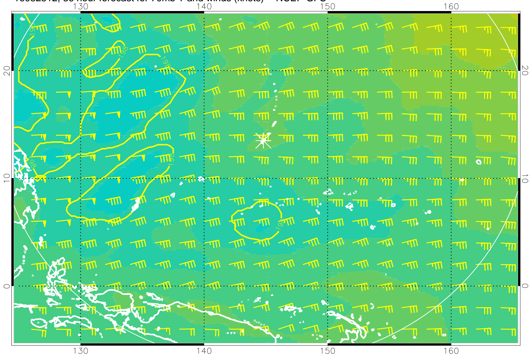
16082512, 36 hour forecast for 70mb T and winds (knots) -- NCEP GFS
