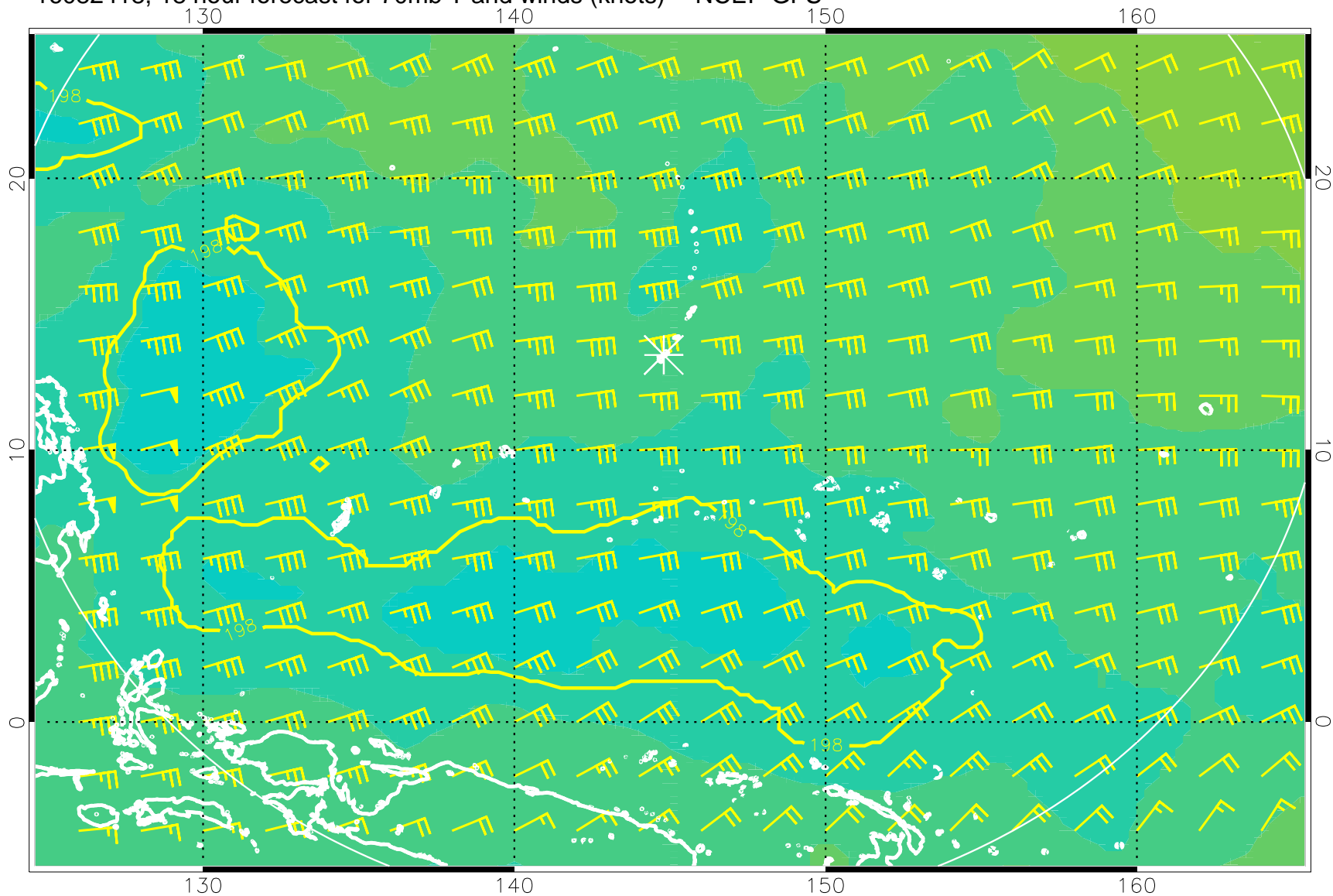
16082418, 18 hour forecast for 70mb T and winds (knots) -- NCEP GFS
