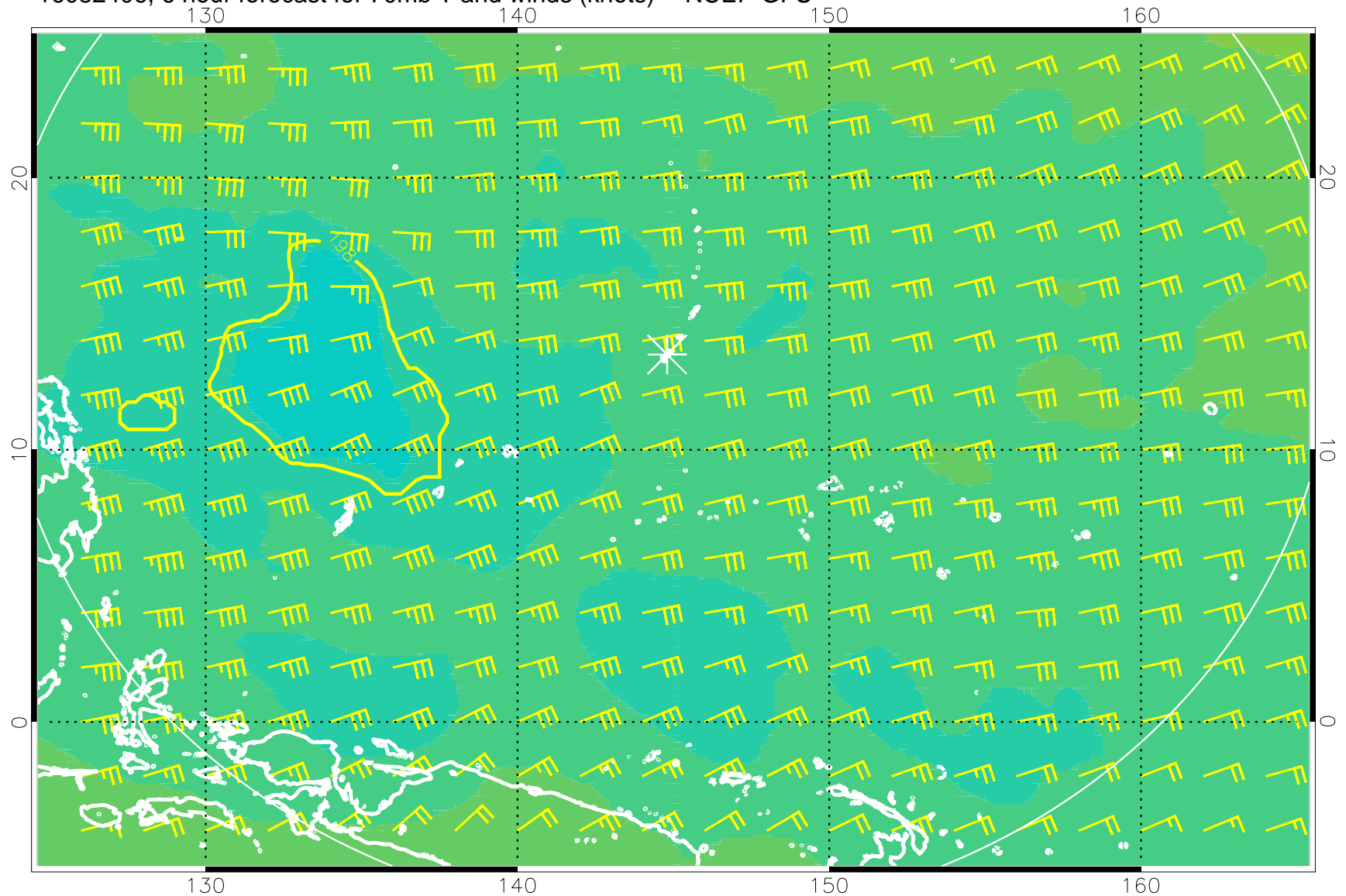
16082406, 6 hour forecast for 70mb T and winds (knots) -- NCEP GFS
