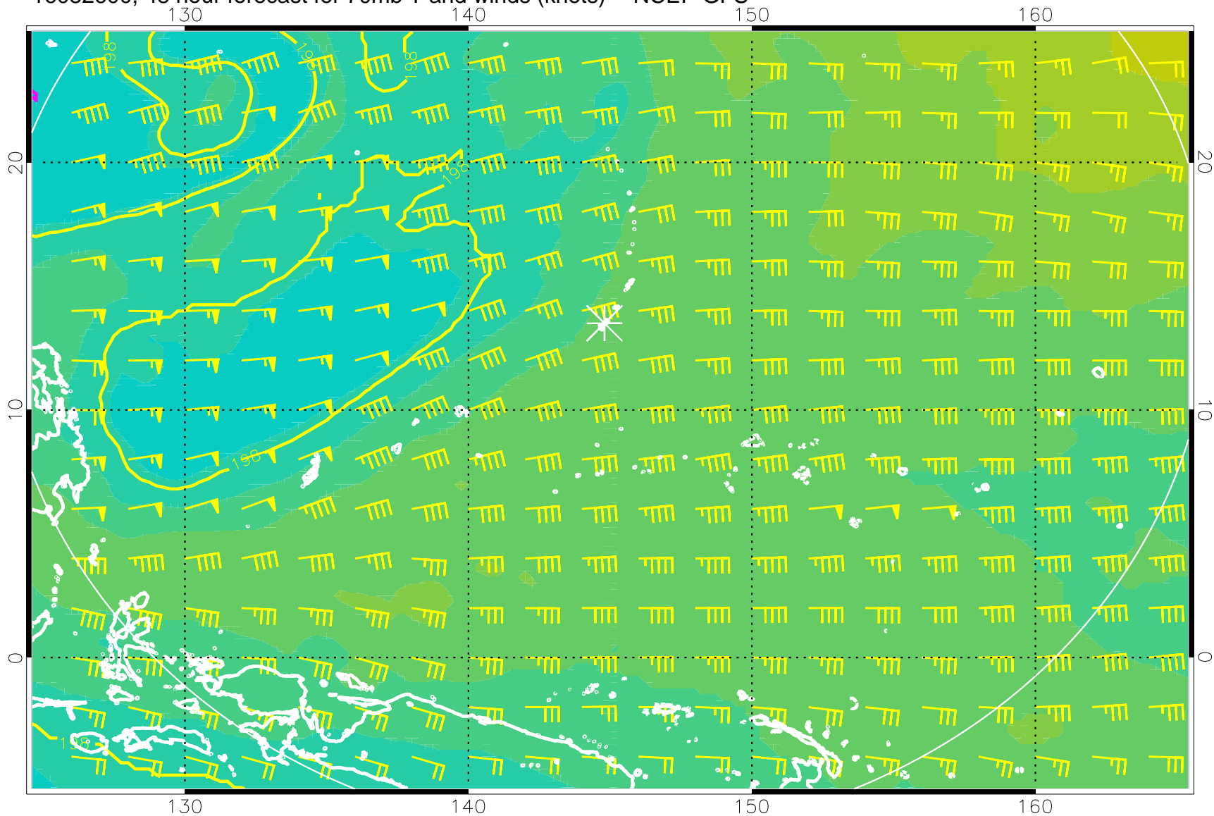
16082600, 48 hour forecast for 70mb T and winds (knots) -- NCEP GFS
