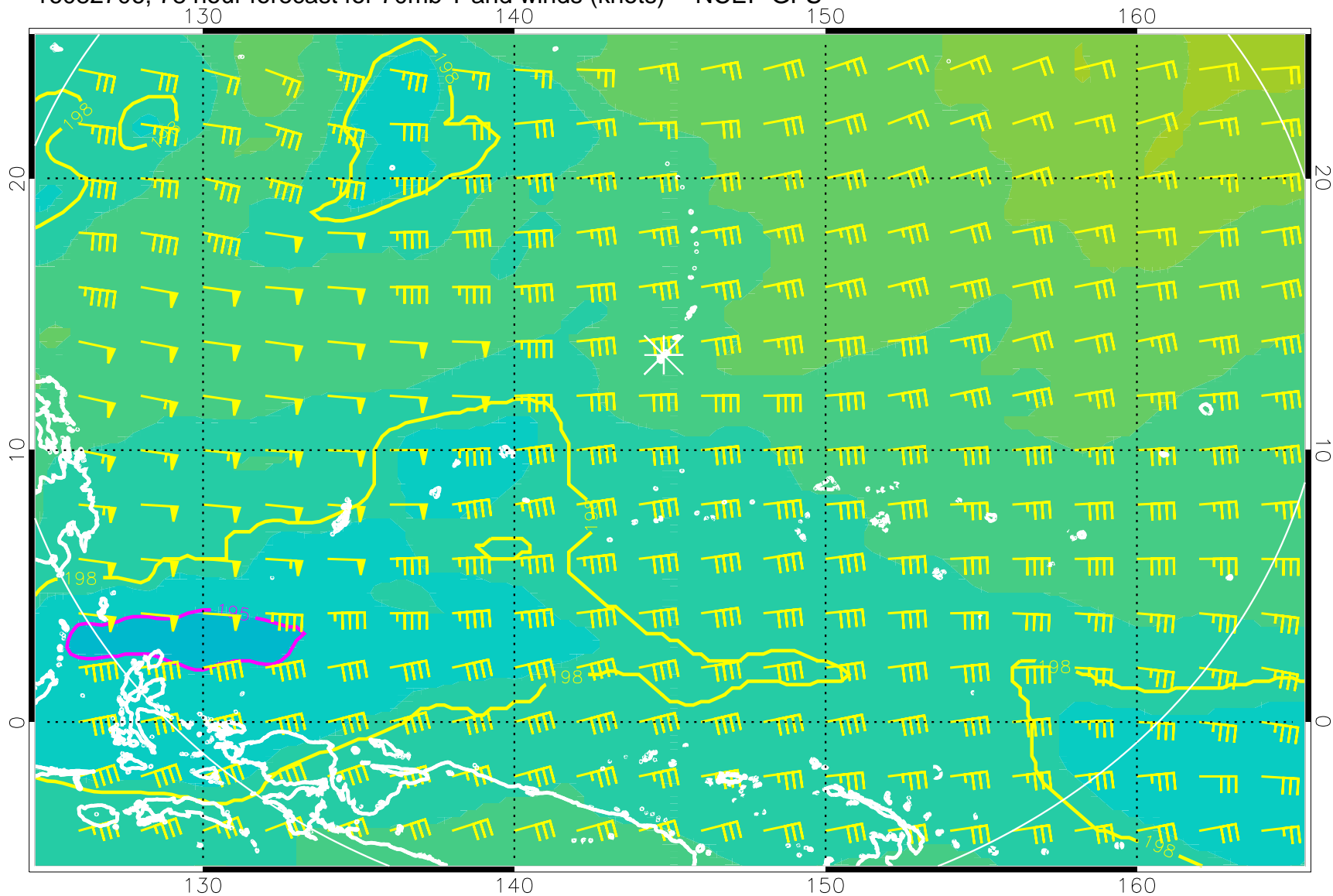
16082706, 78 hour forecast for 70mb T and winds (knots) -- NCEP GFS
