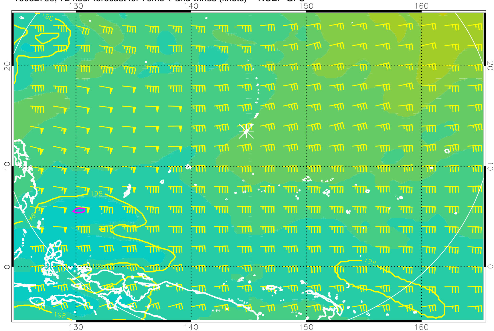
16082700, 72 hour forecast for 70mb T and winds (knots) -- NCEP GFS
