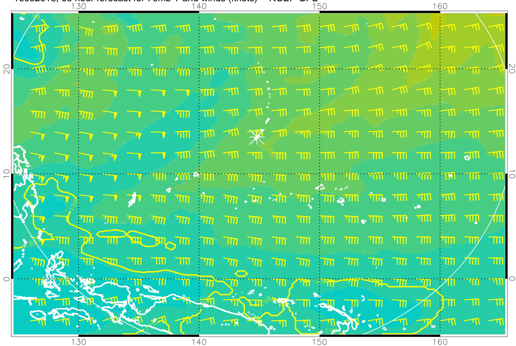
16082618, 66 hour forecast for 70mb T and winds (knots) -- NCEP GFS
