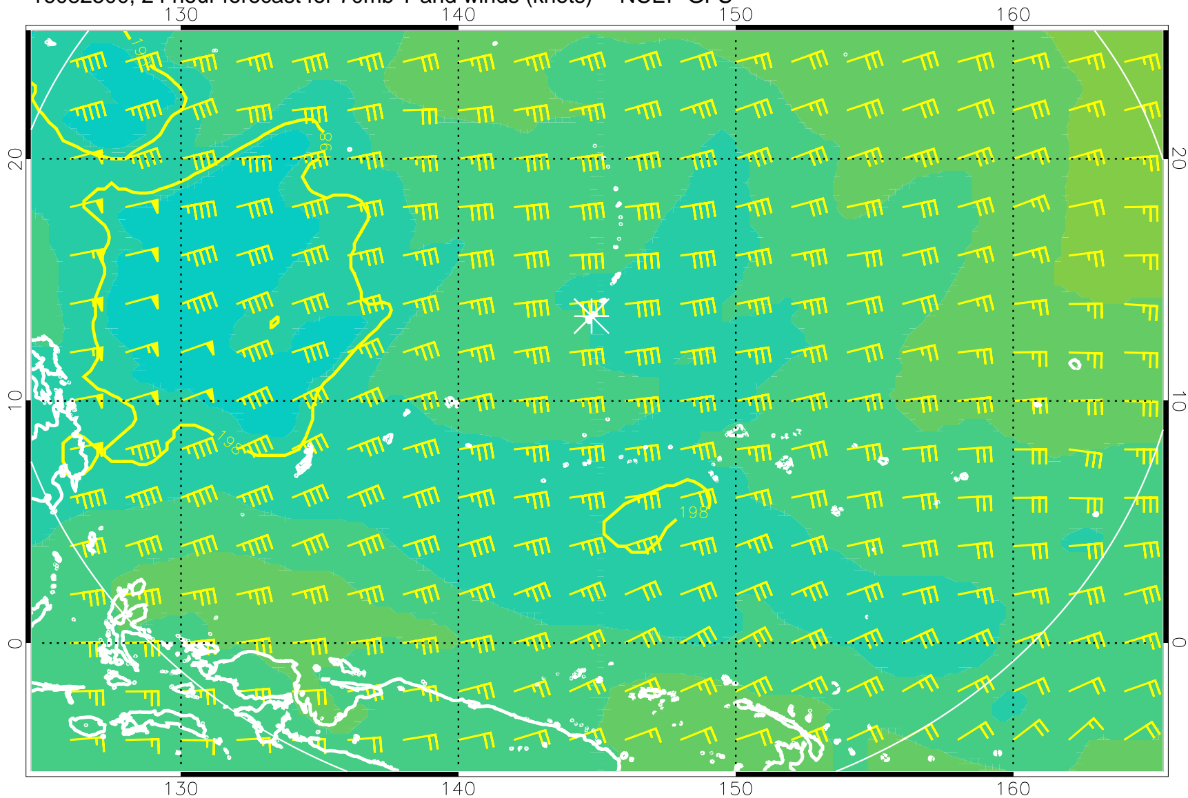
16082500, 24 hour forecast for 70mb T and winds (knots) -- NCEP GFS
