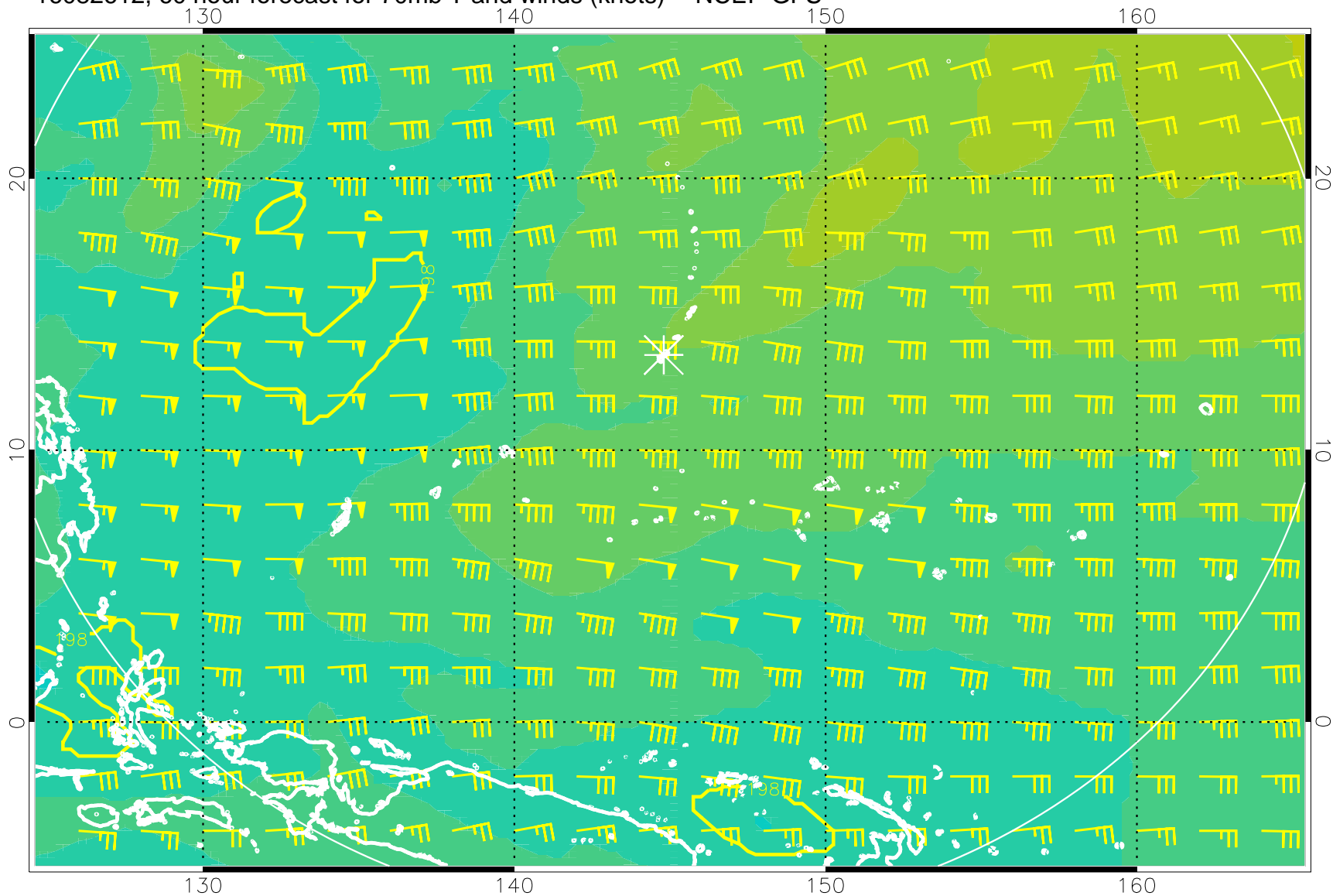
16082612, 60 hour forecast for 70mb T and winds (knots) -- NCEP GFS
