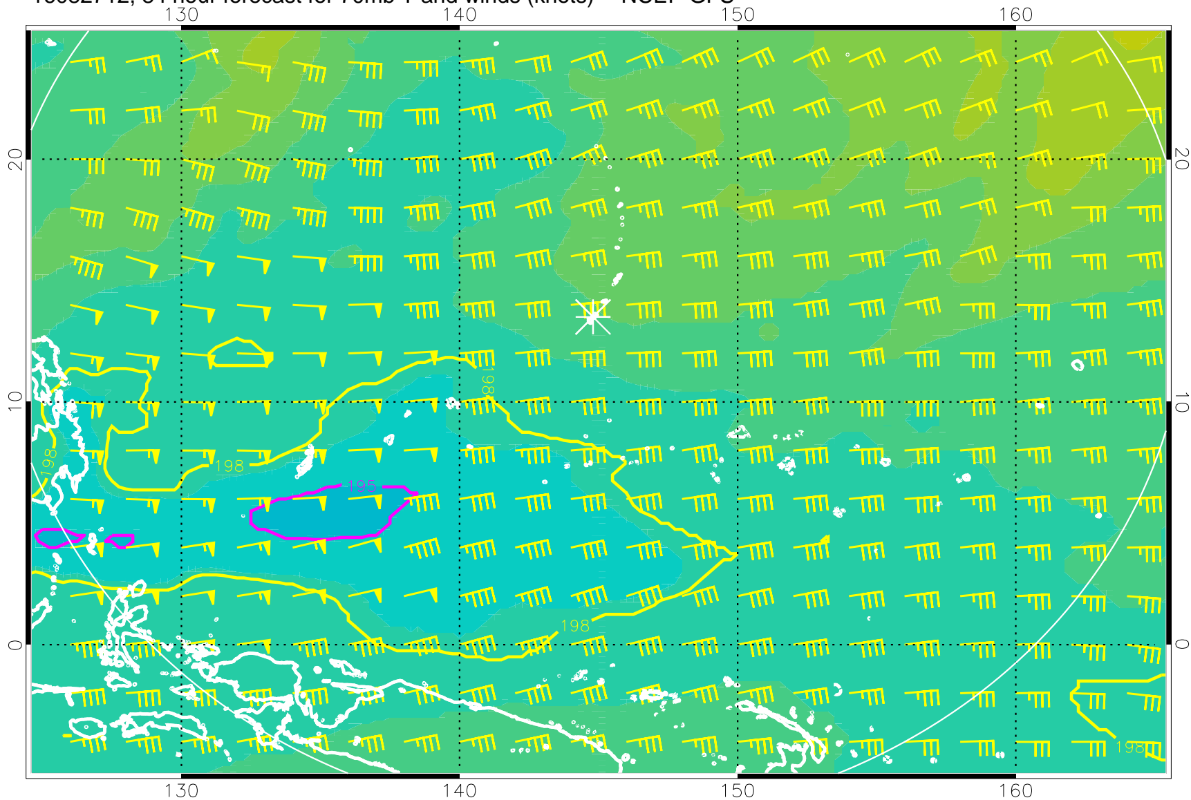
16082712, 84 hour forecast for 70mb T and winds (knots) -- NCEP GFS
