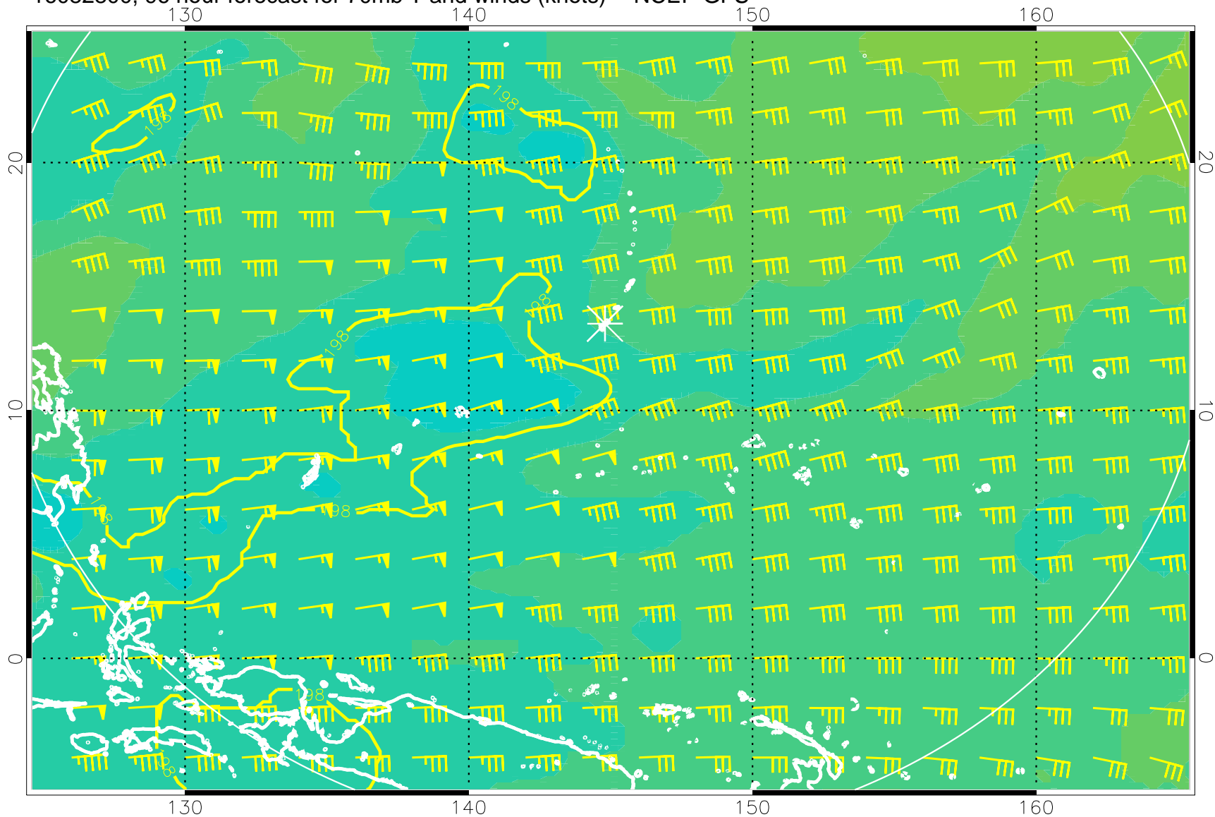
16082800, 96 hour forecast for 70mb T and winds (knots) -- NCEP GFS
