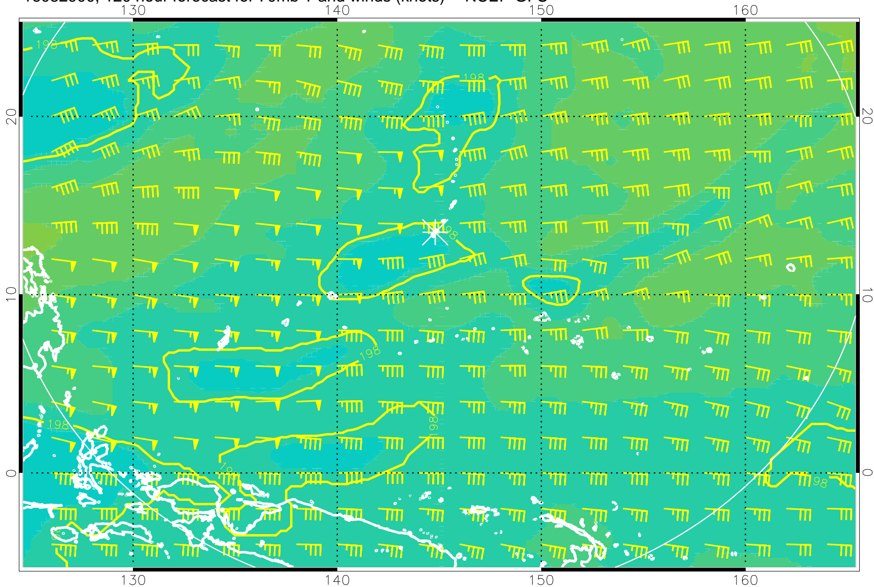
16082900, 120 hour forecast for 70mb T and winds (knots) -- NCEP GFS
