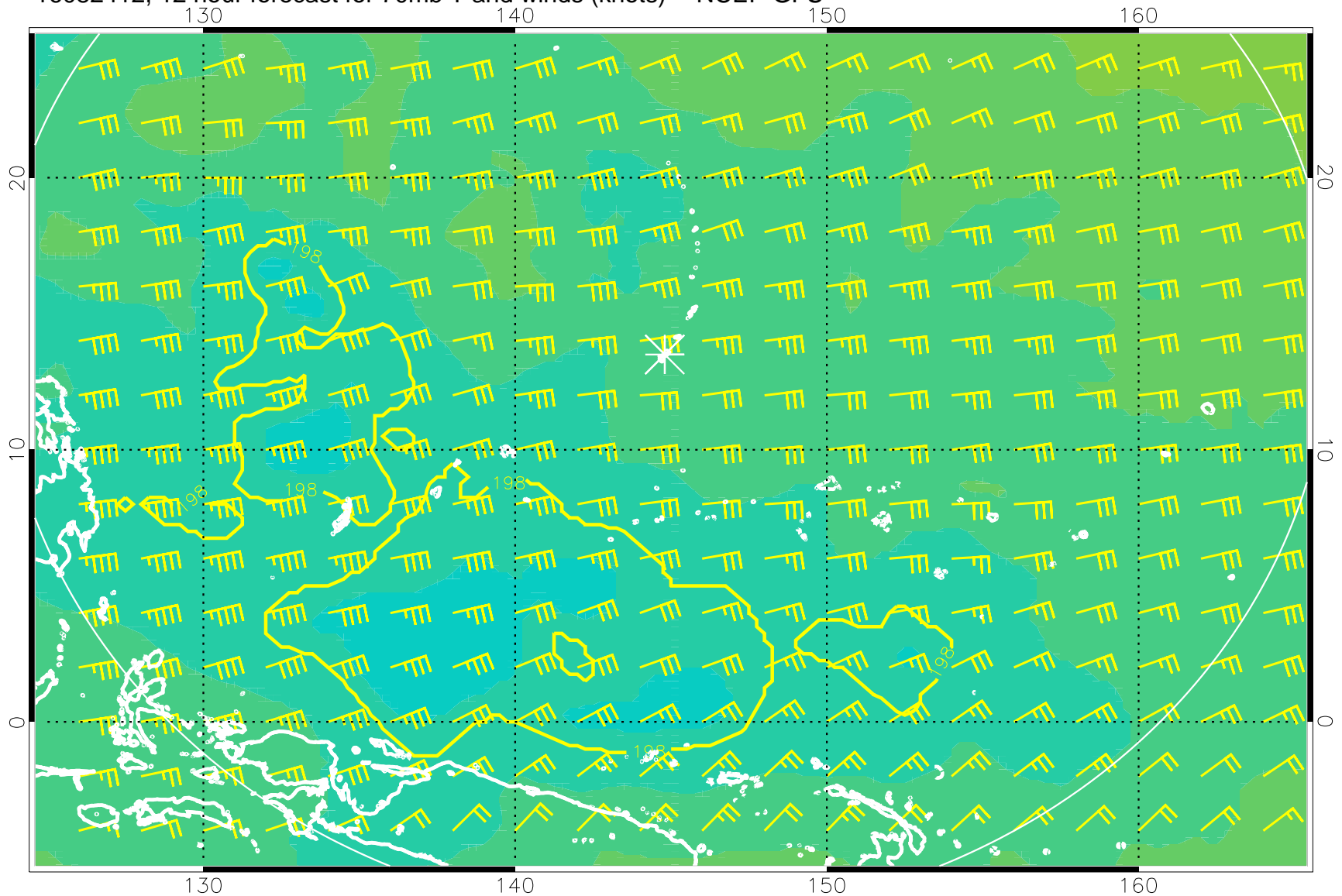
16082412, 12 hour forecast for 70mb T and winds (knots) -- NCEP GFS
