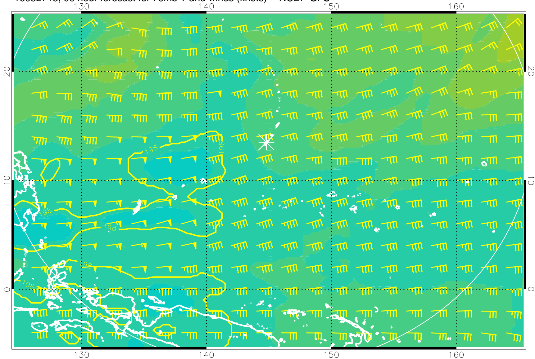
16082718, 90 hour forecast for 70mb T and winds (knots) -- NCEP GFS
