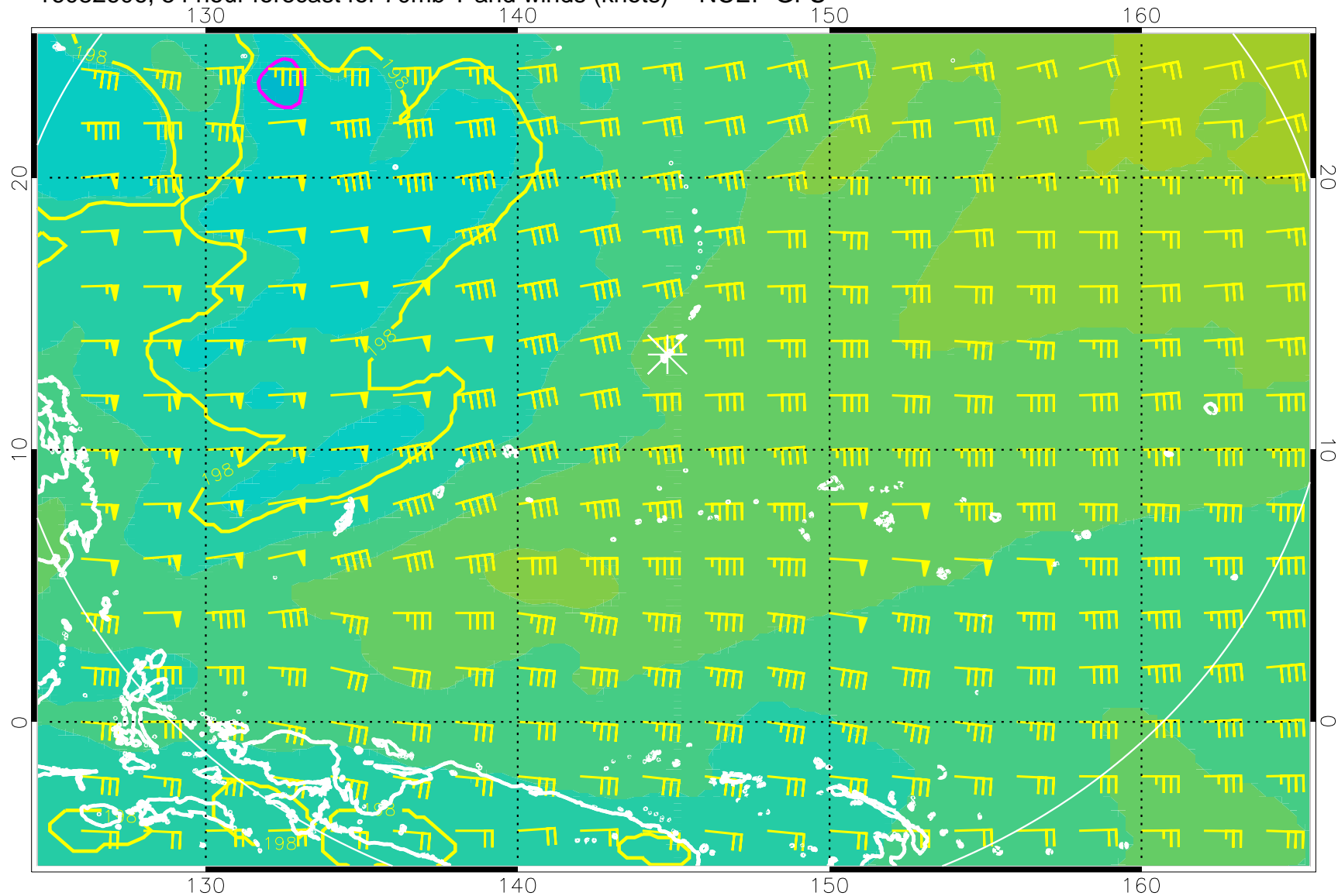
16082606, 54 hour forecast for 70mb T and winds (knots) -- NCEP GFS
