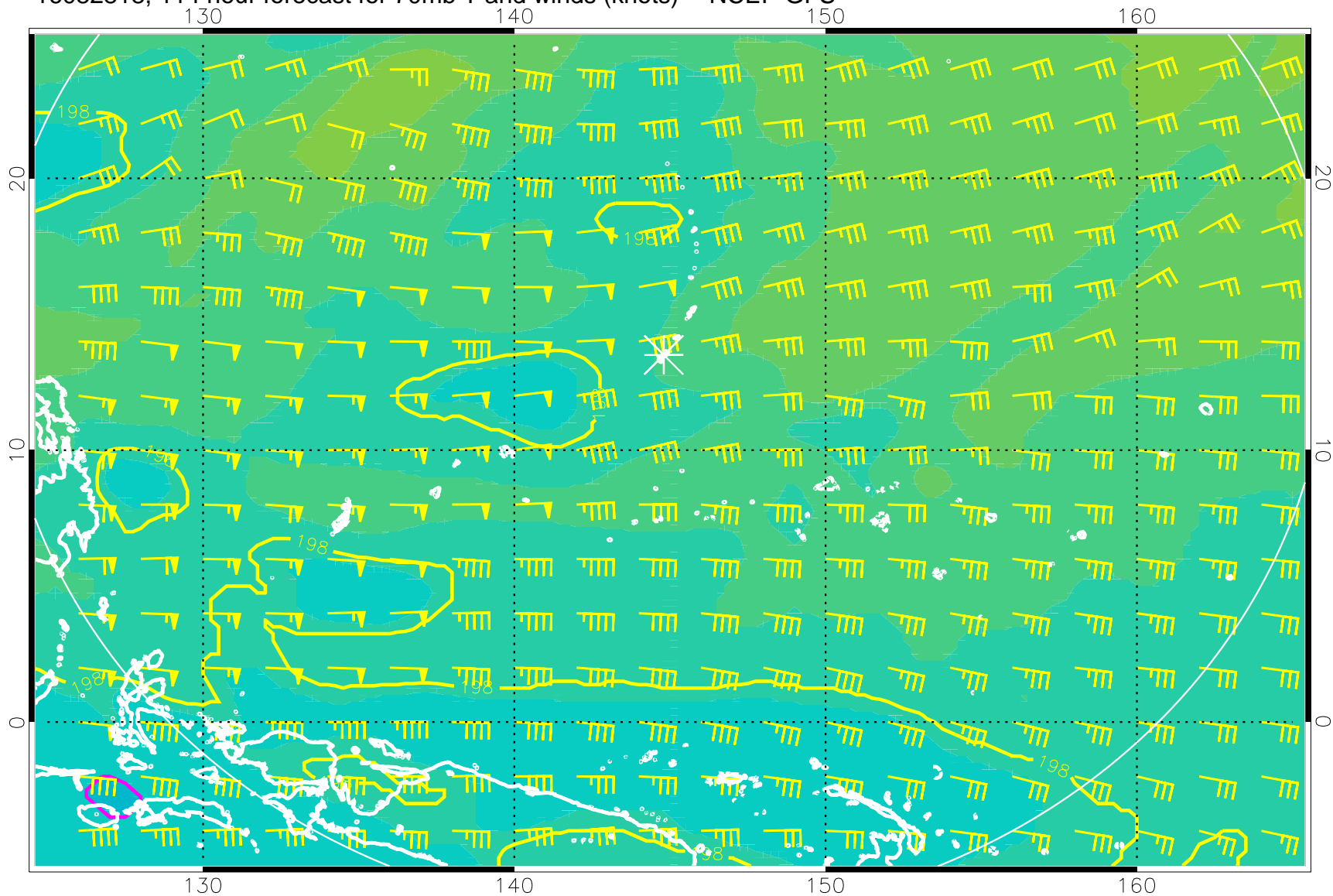
16082818, 114 hour forecast for 70mb T and winds (knots) -- NCEP GFS
