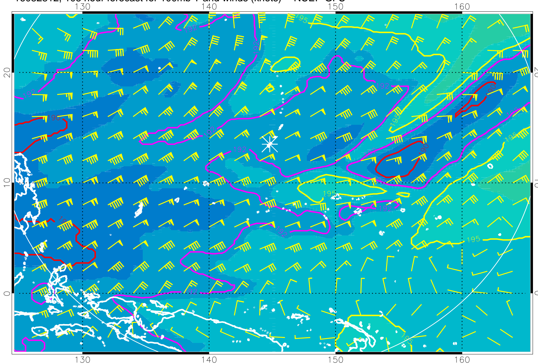
16082812, 108 hour forecast for 100mb T and winds (knots) -- NCEP GFS
