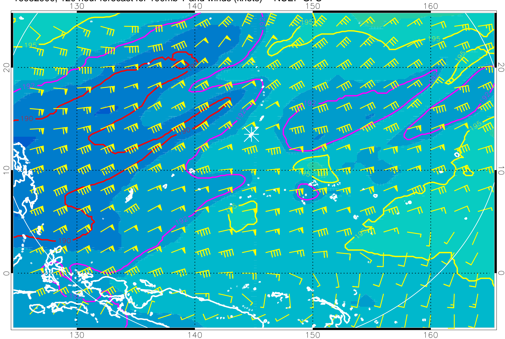
16082900, 120 hour forecast for 100mb T and winds (knots) -- NCEP GFS
