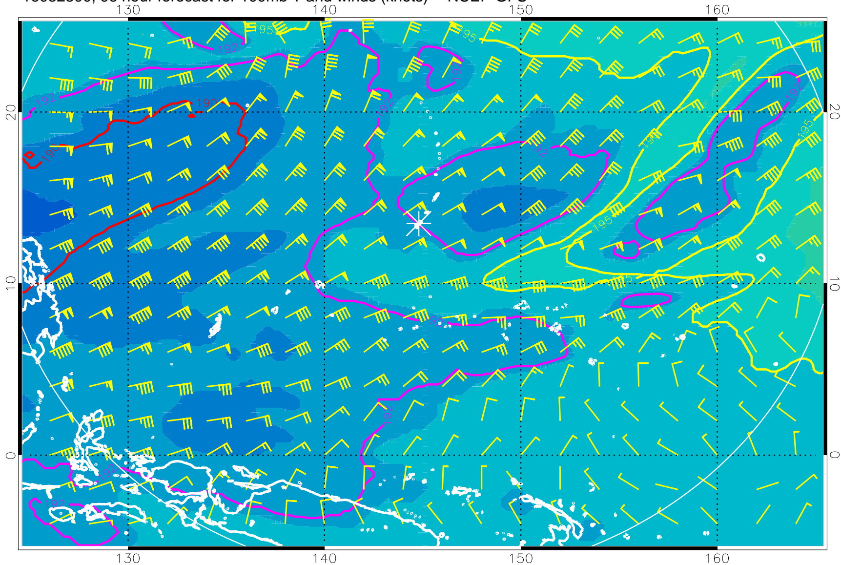
16082800, 96 hour forecast for 100mb T and winds (knots) -- NCEP GFS
