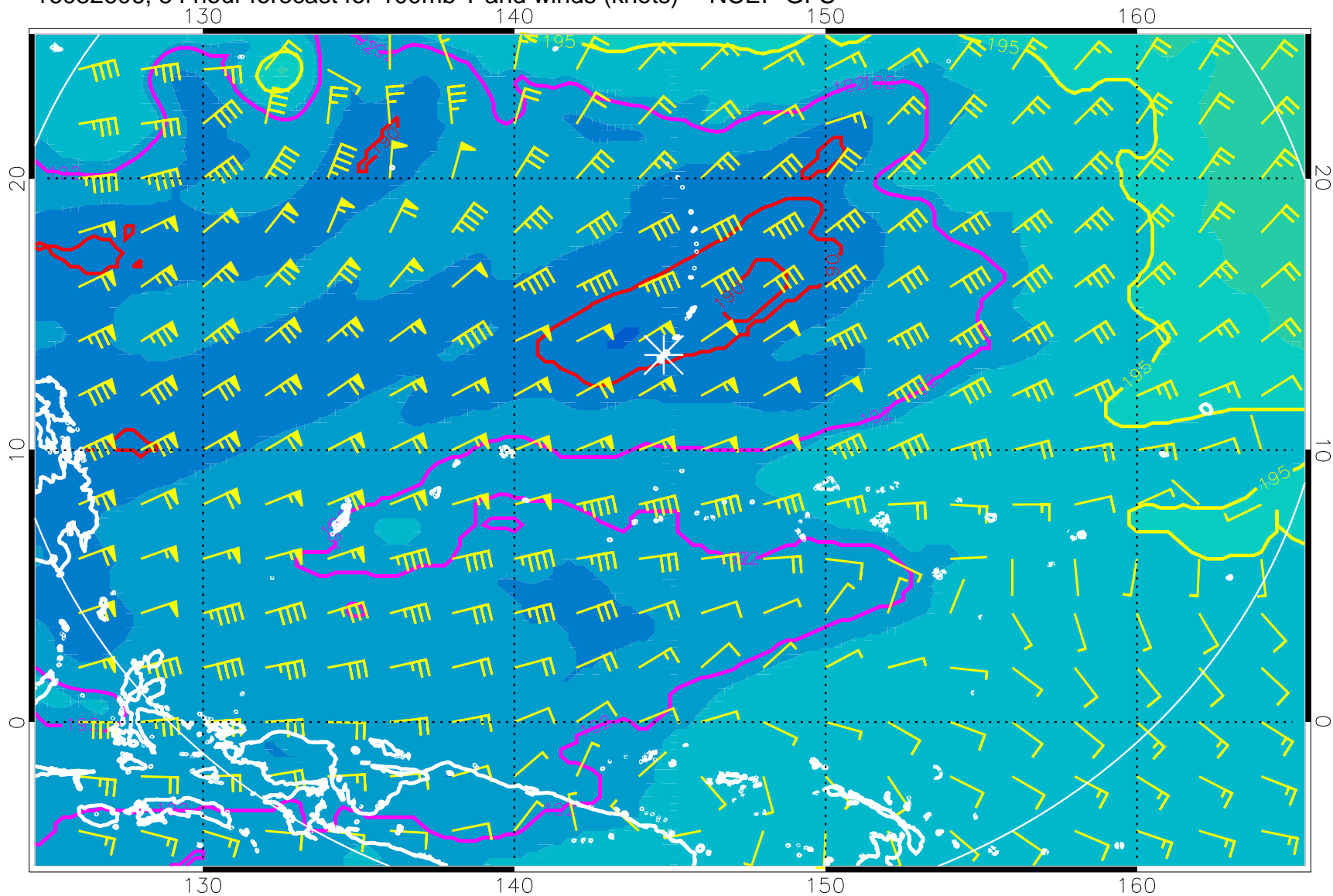
16082606, 54 hour forecast for 100mb T and winds (knots) -- NCEP GFS
