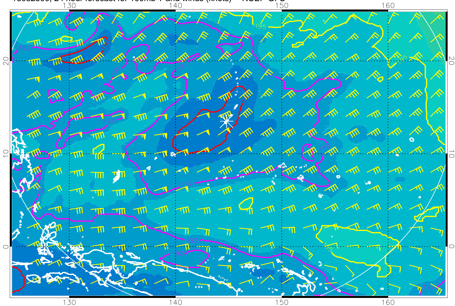
16082500, 24 hour forecast for 100mb T and winds (knots) -- NCEP GFS
