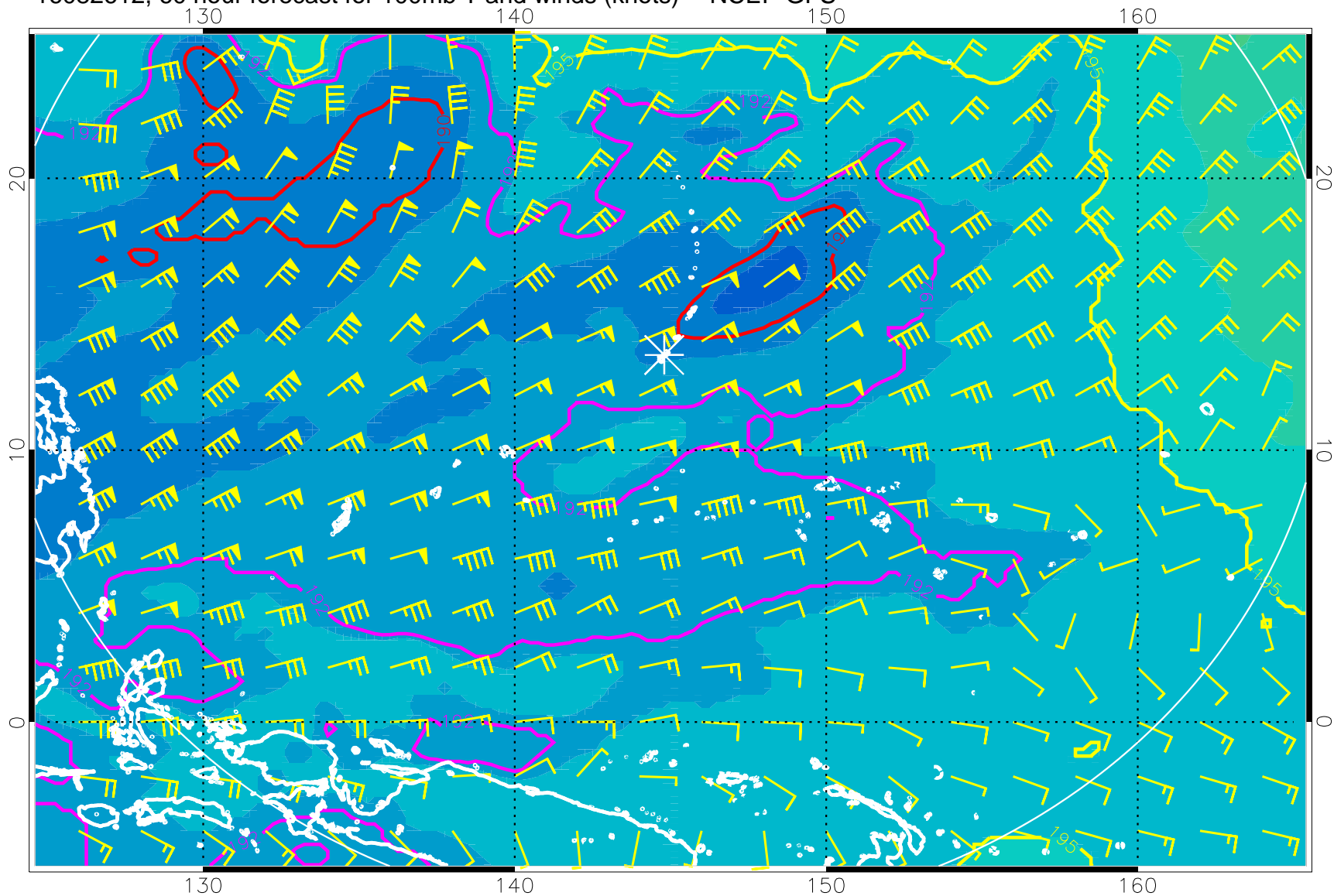
16082612, 60 hour forecast for 100mb T and winds (knots) -- NCEP GFS
