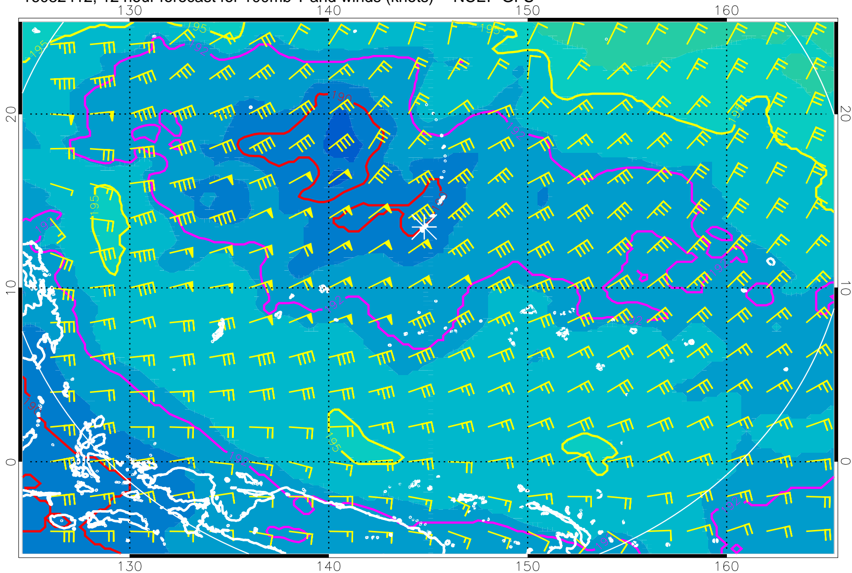
16082412, 12 hour forecast for 100mb T and winds (knots) -- NCEP GFS
