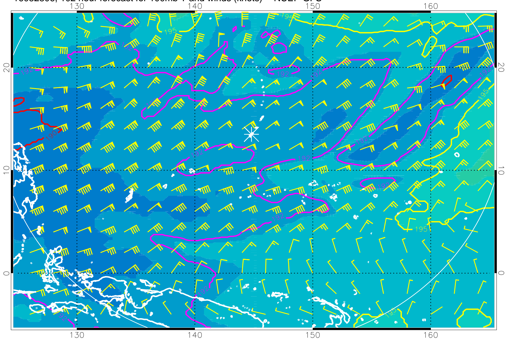
16082806, 102 hour forecast for 100mb T and winds (knots) -- NCEP GFS
