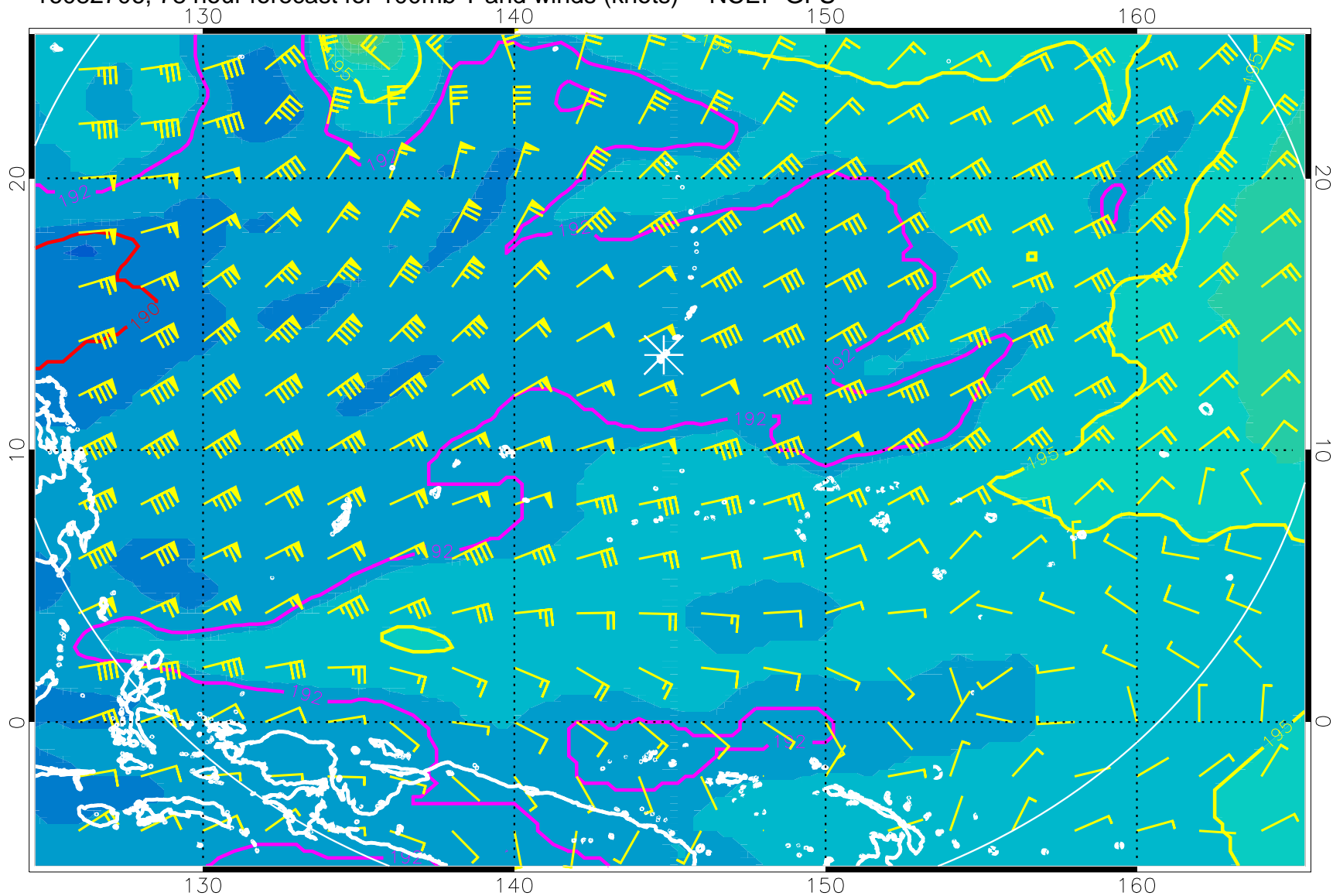
16082706, 78 hour forecast for 100mb T and winds (knots) -- NCEP GFS
