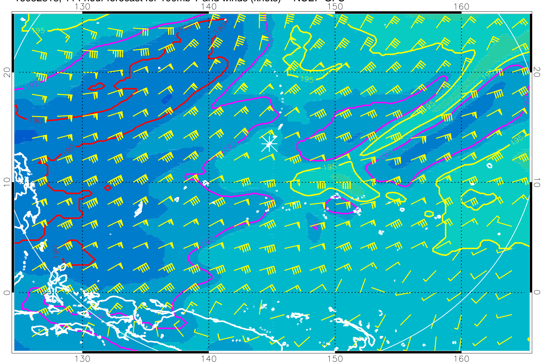
16082818, 114 hour forecast for 100mb T and winds (knots) -- NCEP GFS
