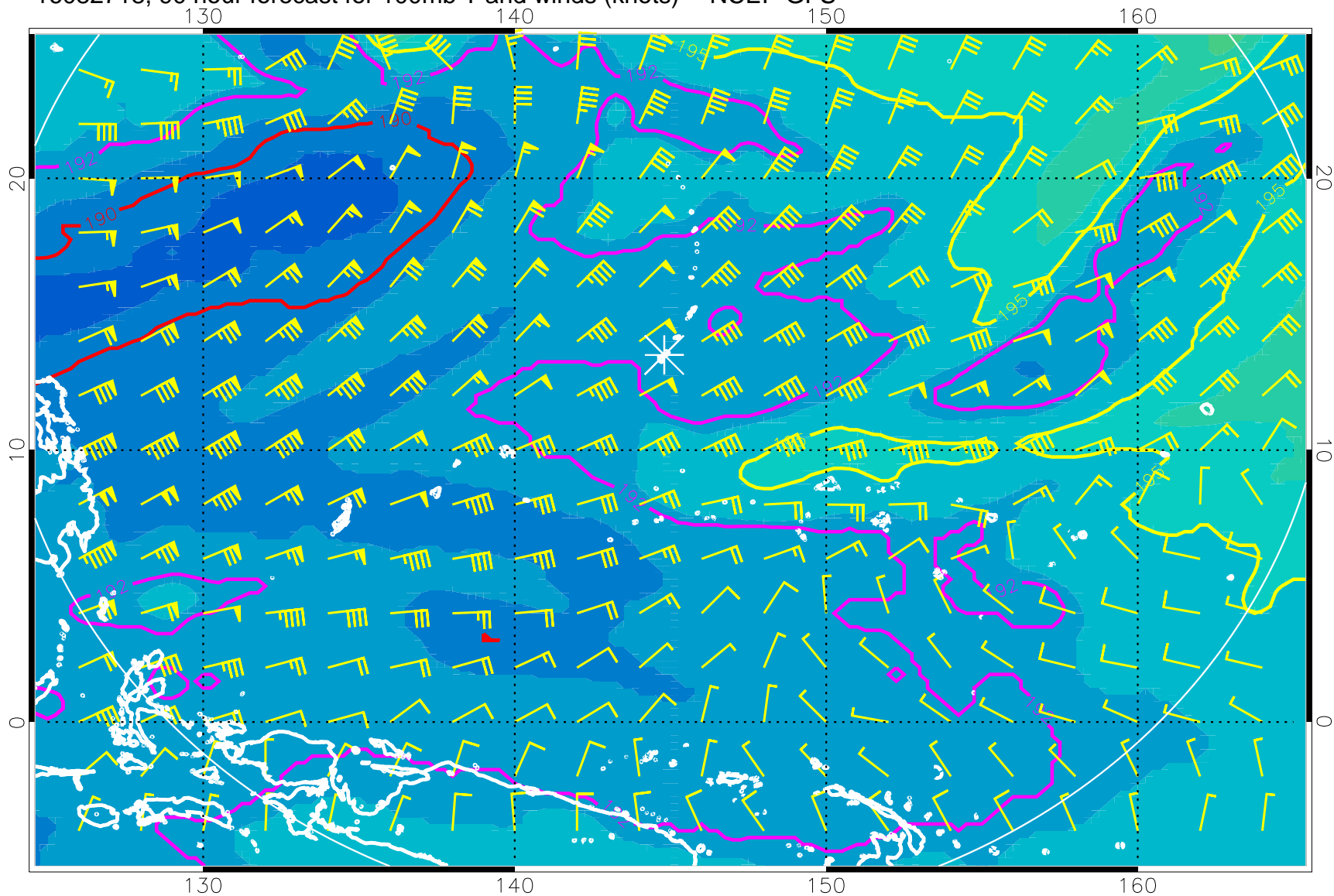
16082718, 90 hour forecast for 100mb T and winds (knots) -- NCEP GFS
