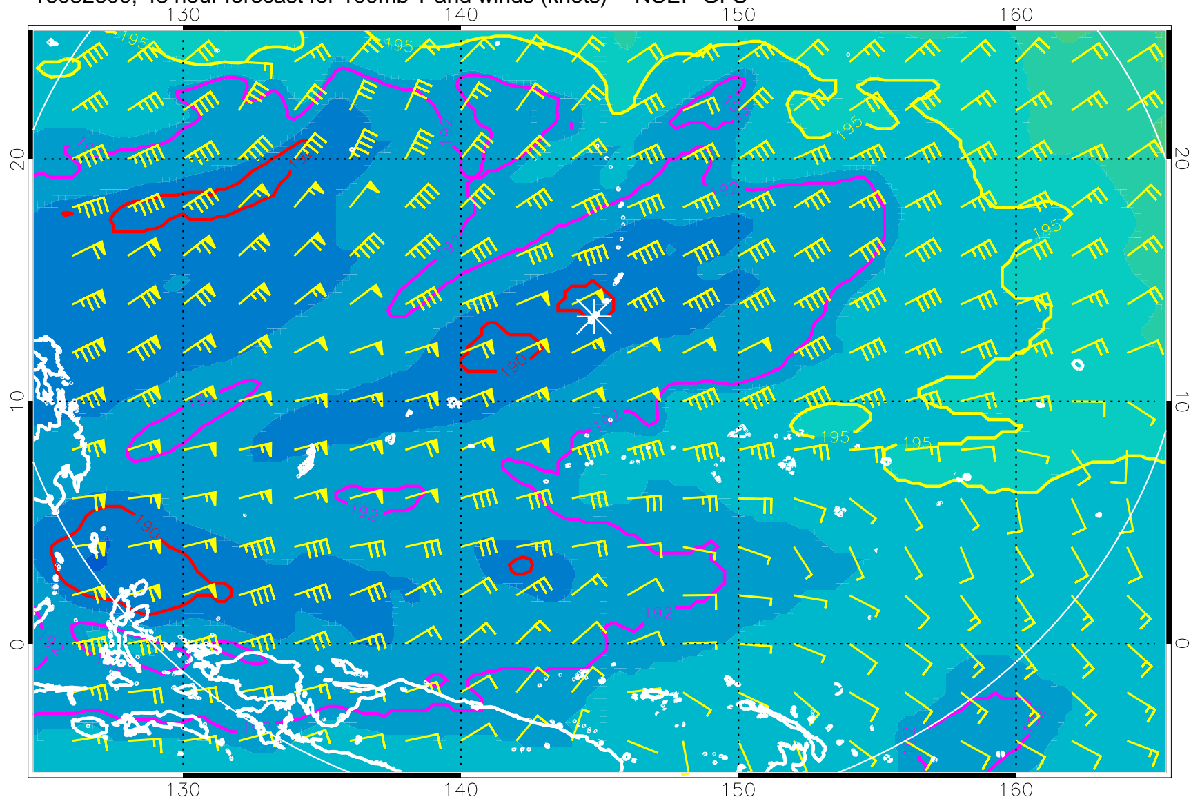
16082600, 48 hour forecast for 100mb T and winds (knots) -- NCEP GFS
