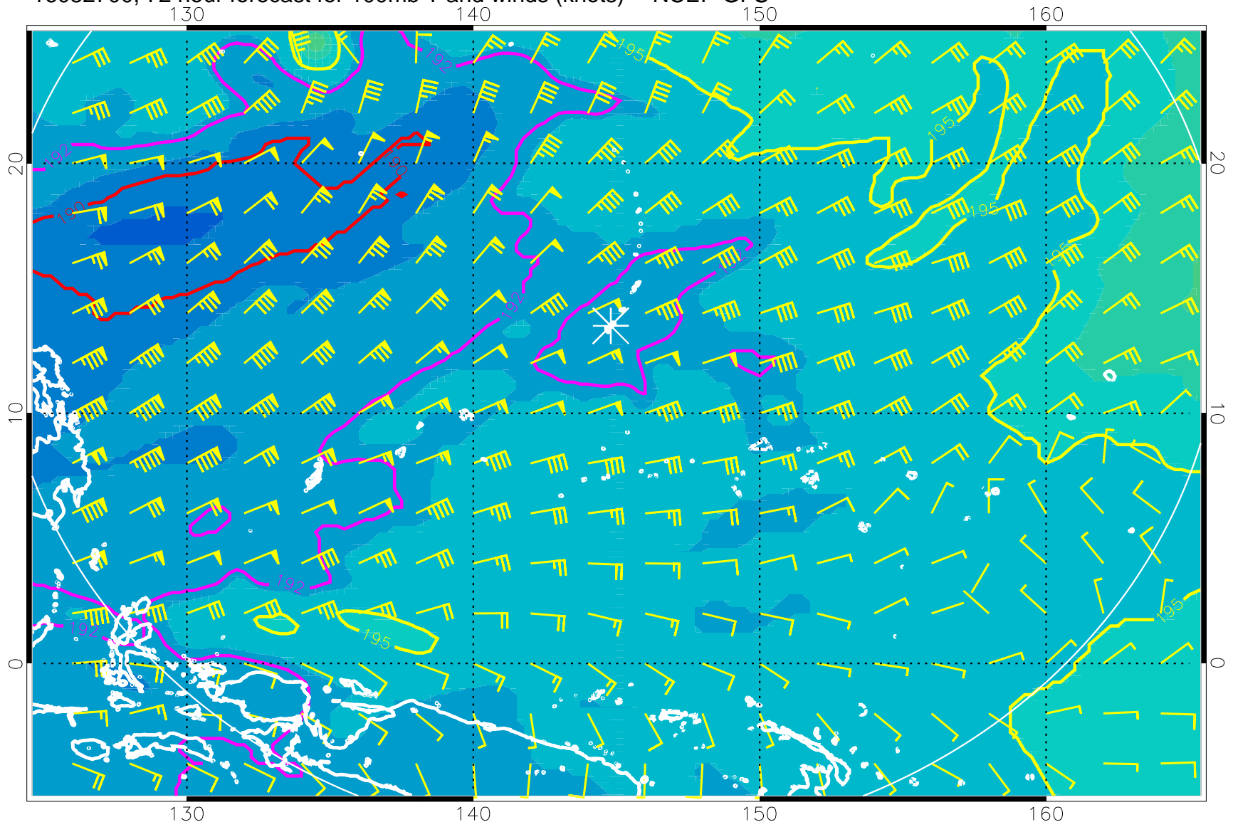
16082700, 72 hour forecast for 100mb T and winds (knots) -- NCEP GFS
