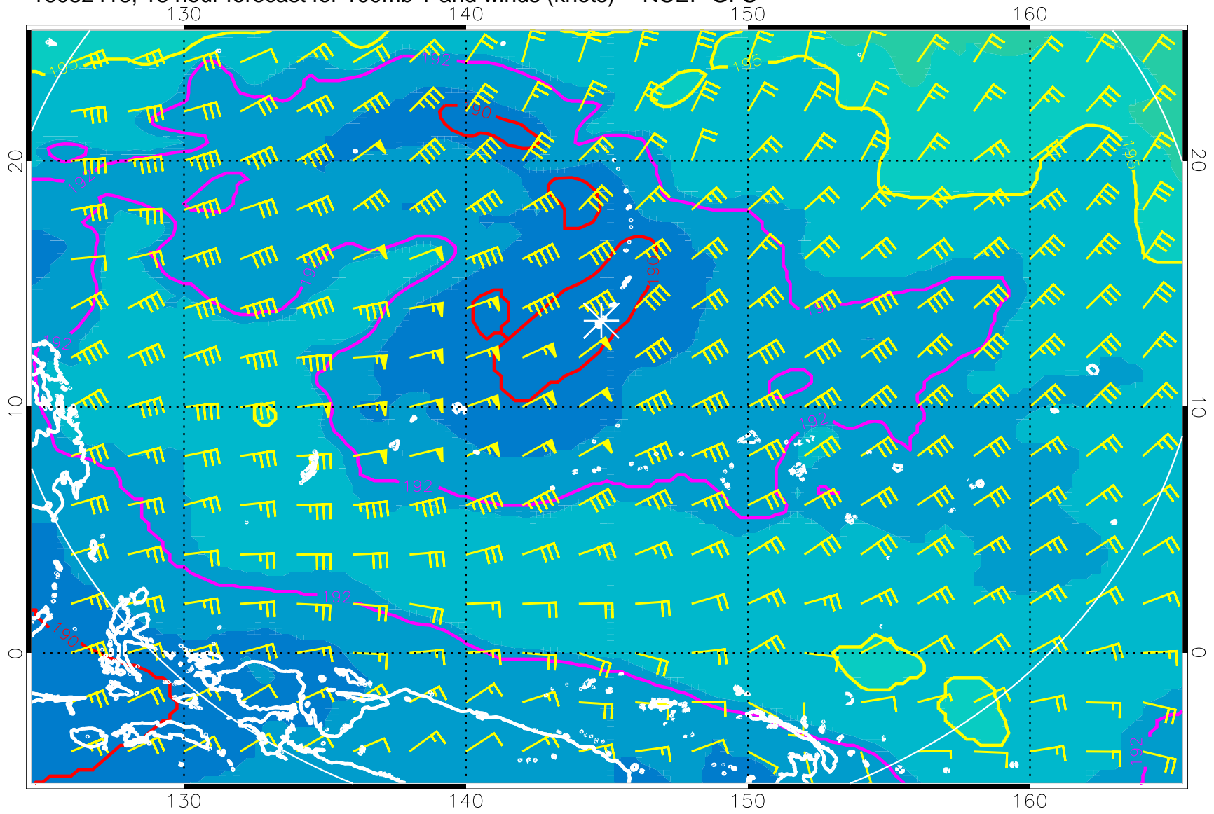
16082418, 18 hour forecast for 100mb T and winds (knots) -- NCEP GFS
