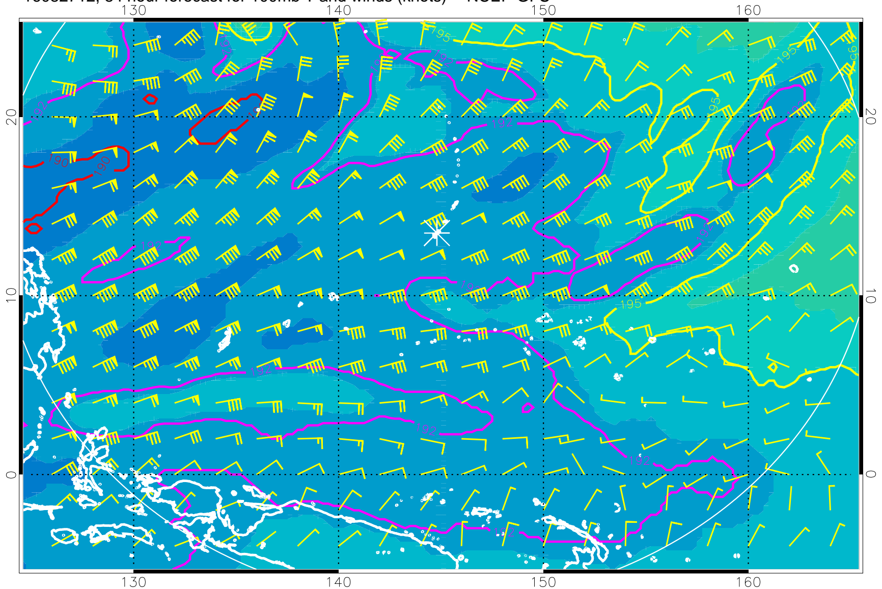
16082712, 84 hour forecast for 100mb T and winds (knots) -- NCEP GFS
