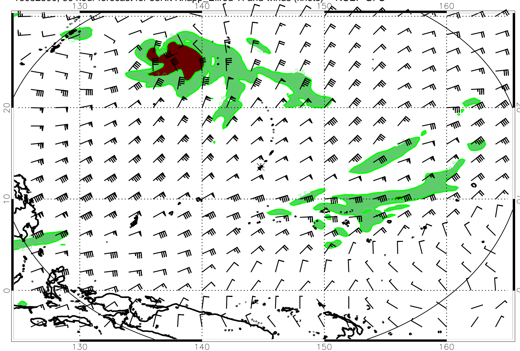
16082800, 96 hour forecast for 53Kft Knapp_Ellrod TI and winds (knots) -- NCEP GFS
