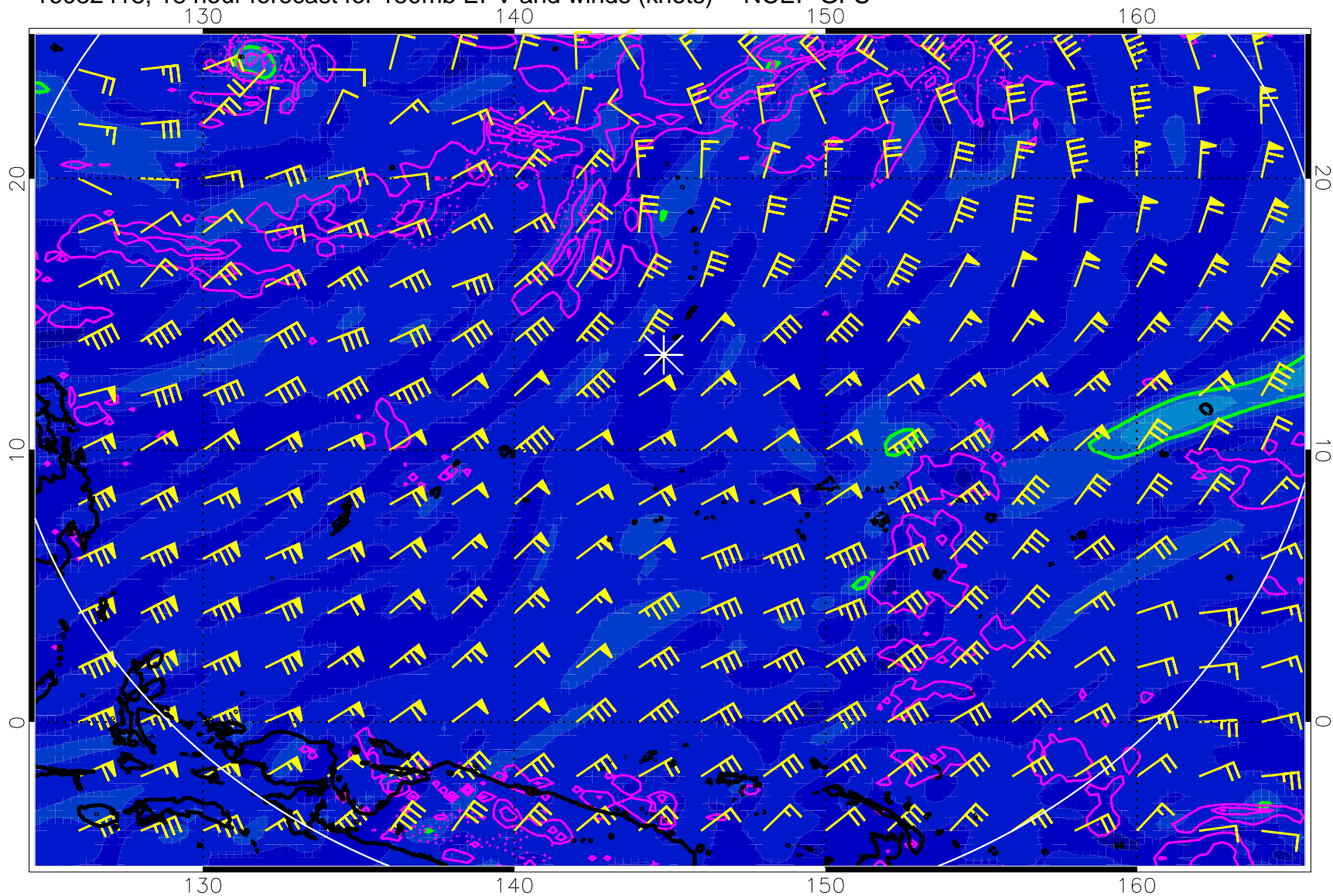
16082418, 18 hour forecast for 150mb EPV and winds (knots) -- NCEP GFS
