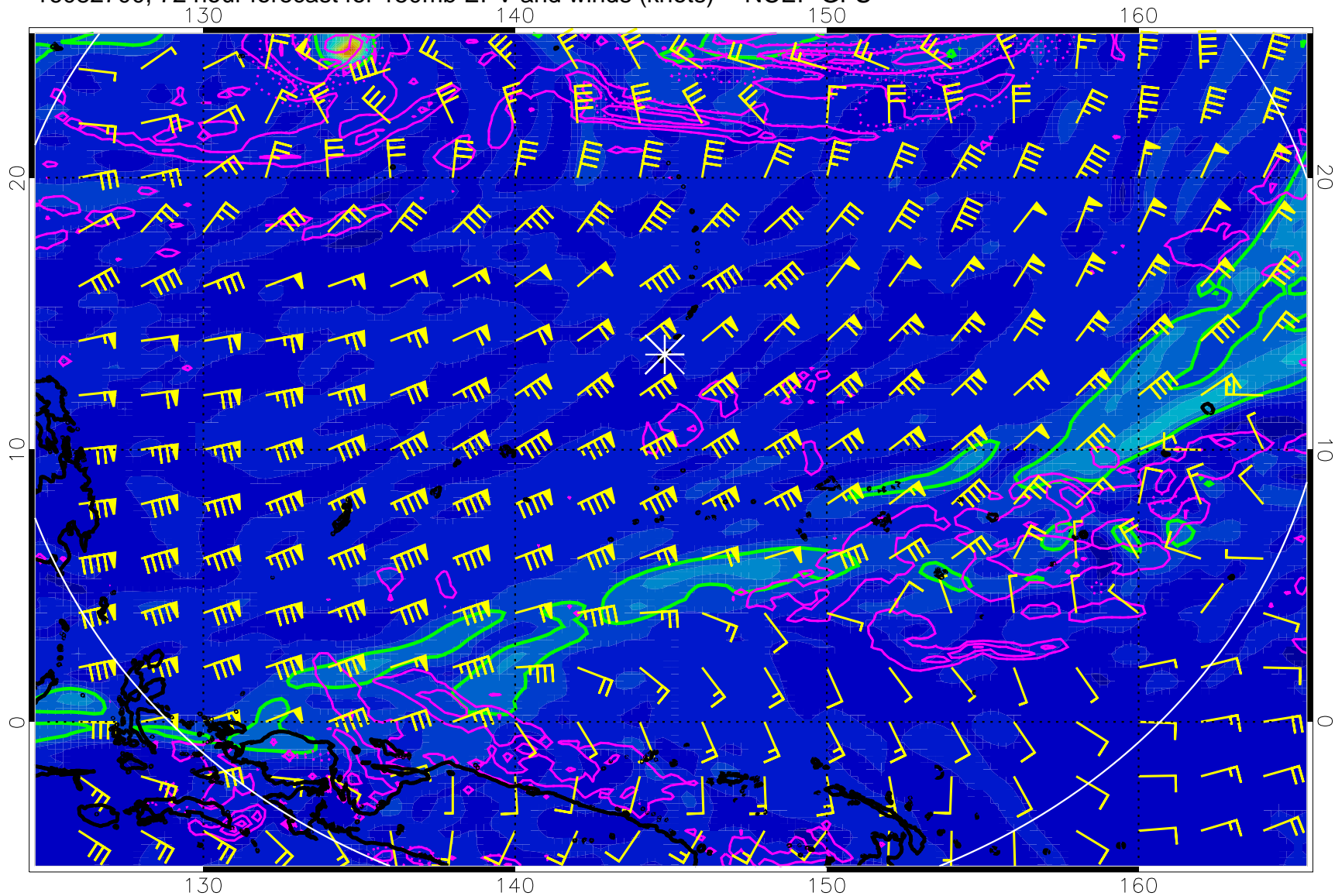
16082700, 72 hour forecast for 150mb EPV and winds (knots) -- NCEP GFS
