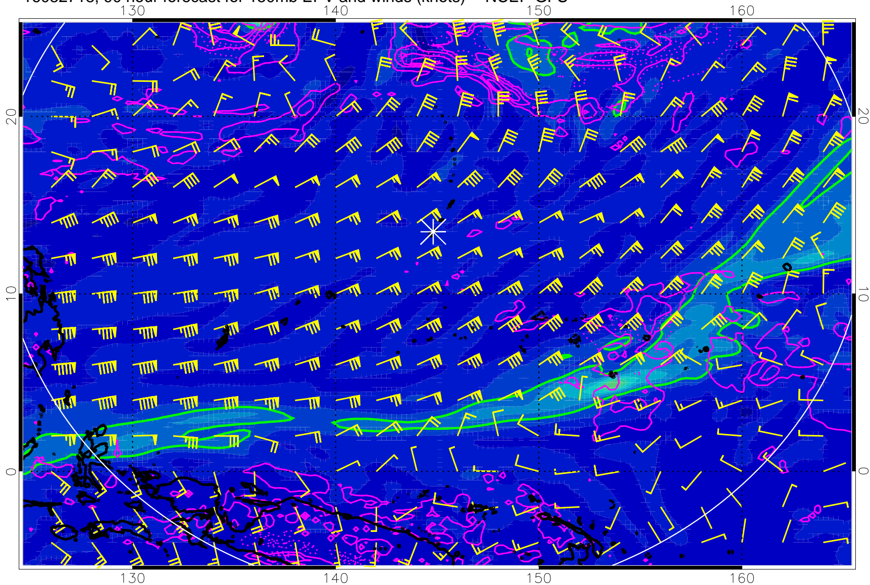
16082718, 90 hour forecast for 150mb EPV and winds (knots) -- NCEP GFS
