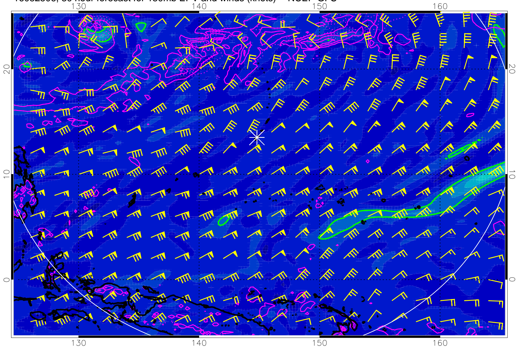
16082506, 30 hour forecast for 150mb EPV and winds (knots) -- NCEP GFS
