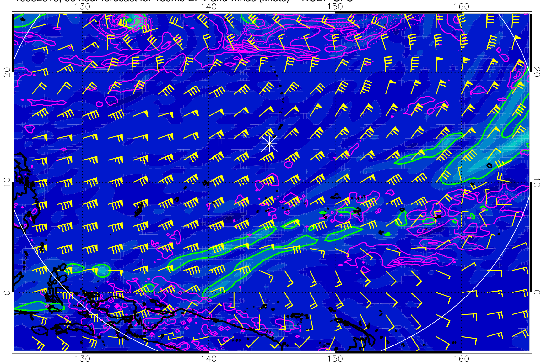
16082618, 66 hour forecast for 150mb EPV and winds (knots) -- NCEP GFS
