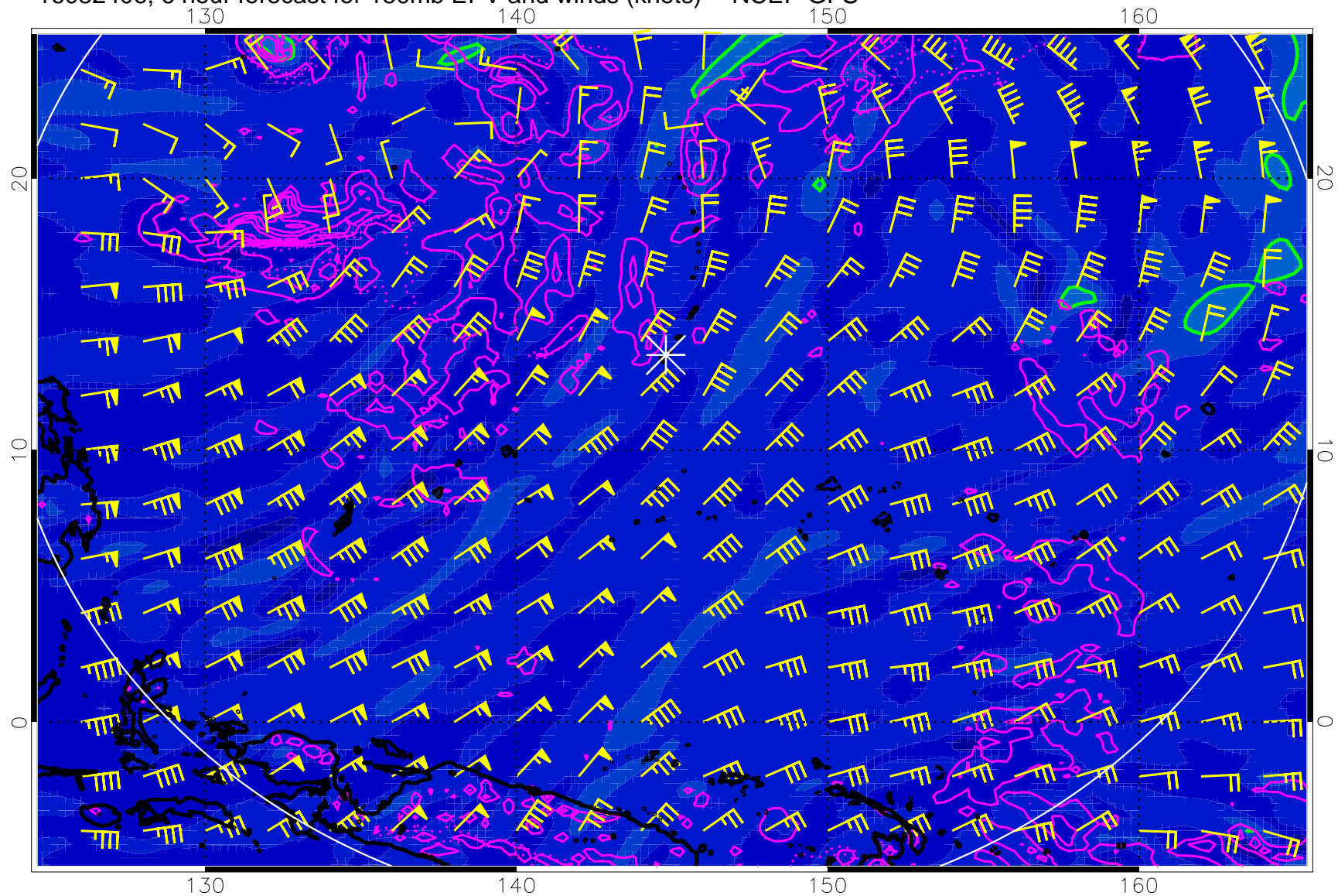
16082406, 6 hour forecast for 150mb EPV and winds (knots) -- NCEP GFS
