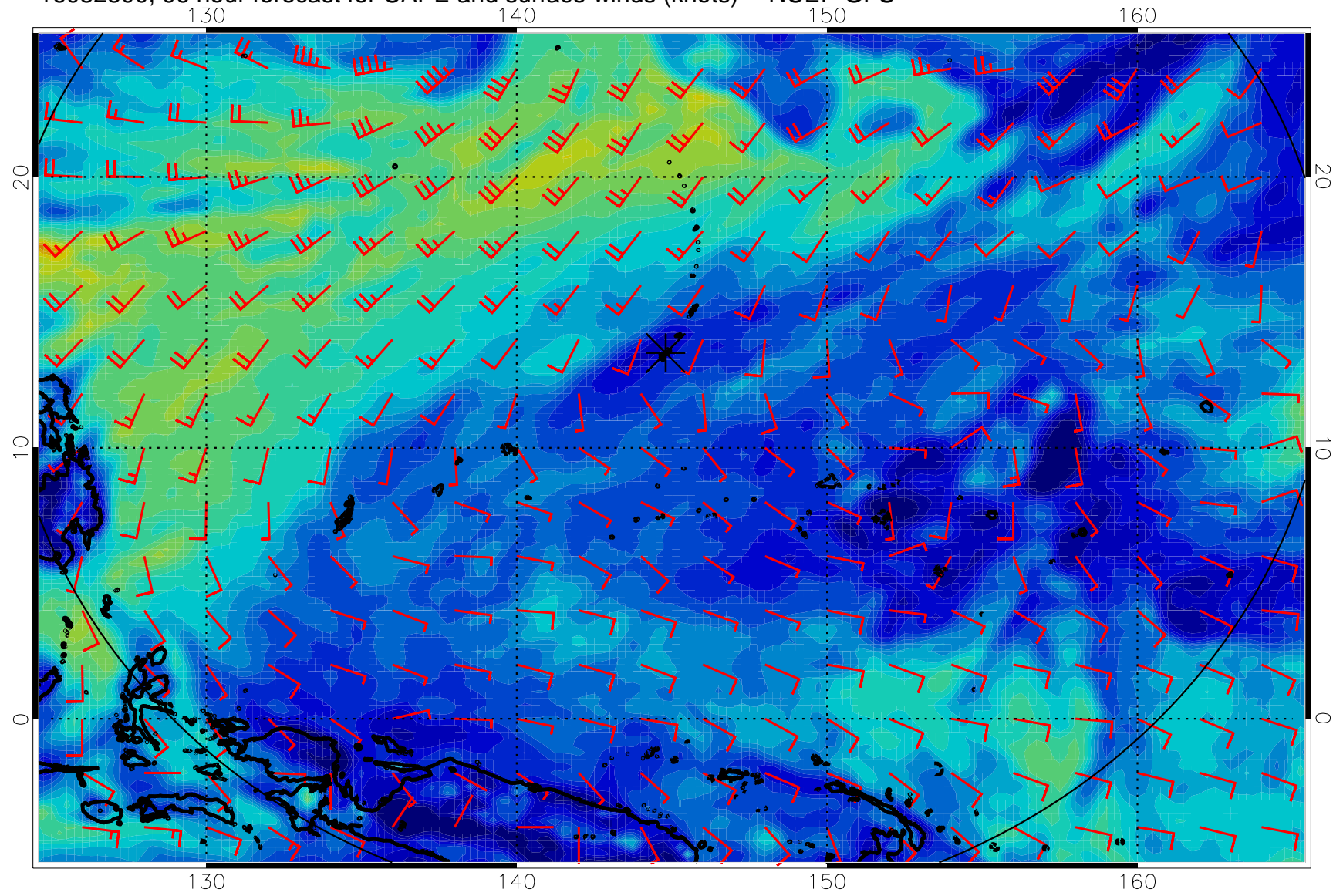
16082800, 96 hour forecast for CAPE and surface winds (knots) -- NCEP GFS
