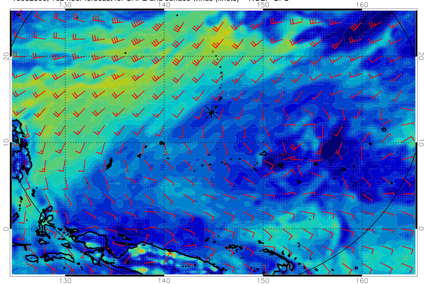
16082806, 102 hour forecast for CAPE and surface winds (knots) -- NCEP GFS
