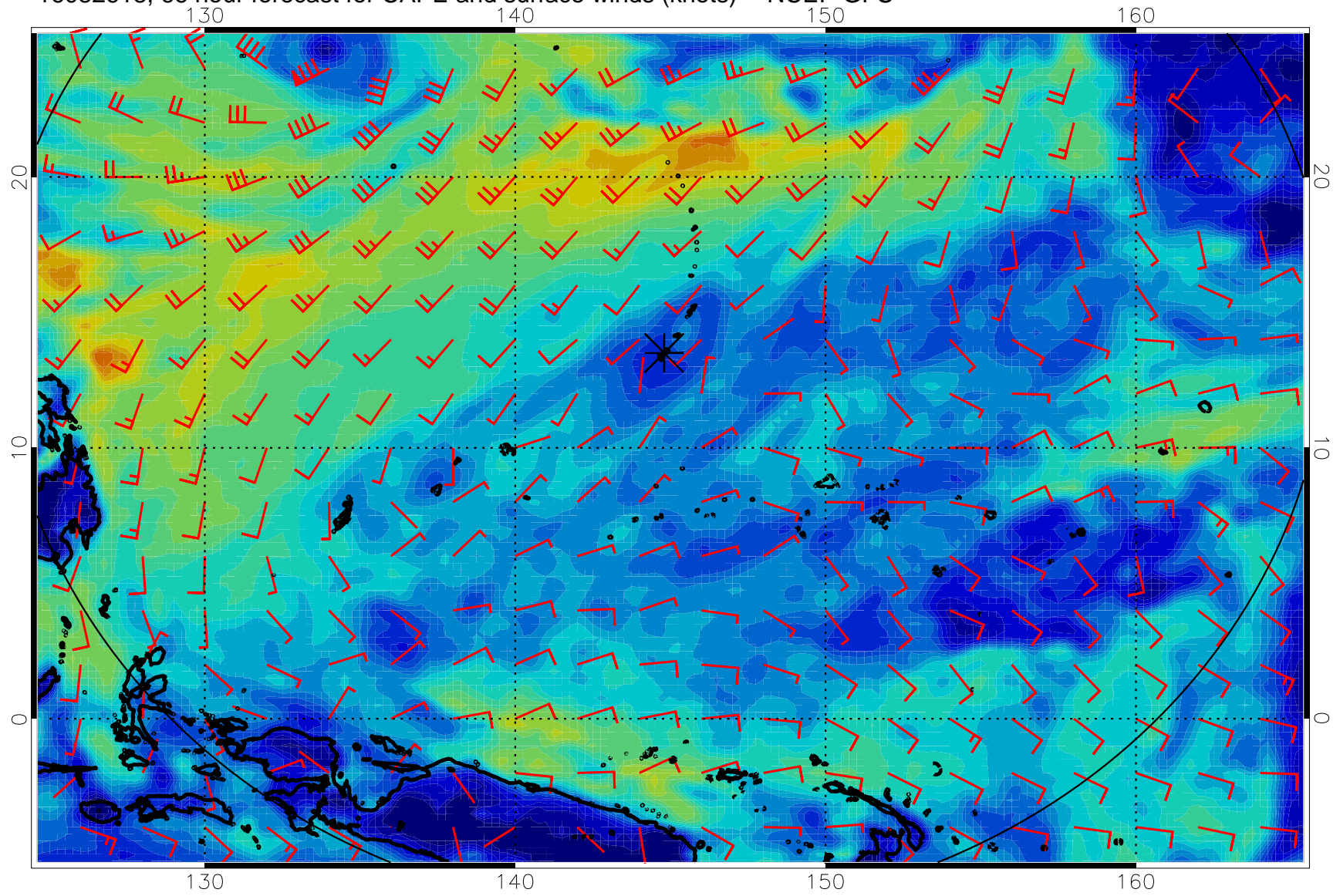
16082618, 66 hour forecast for CAPE and surface winds (knots) -- NCEP GFS
