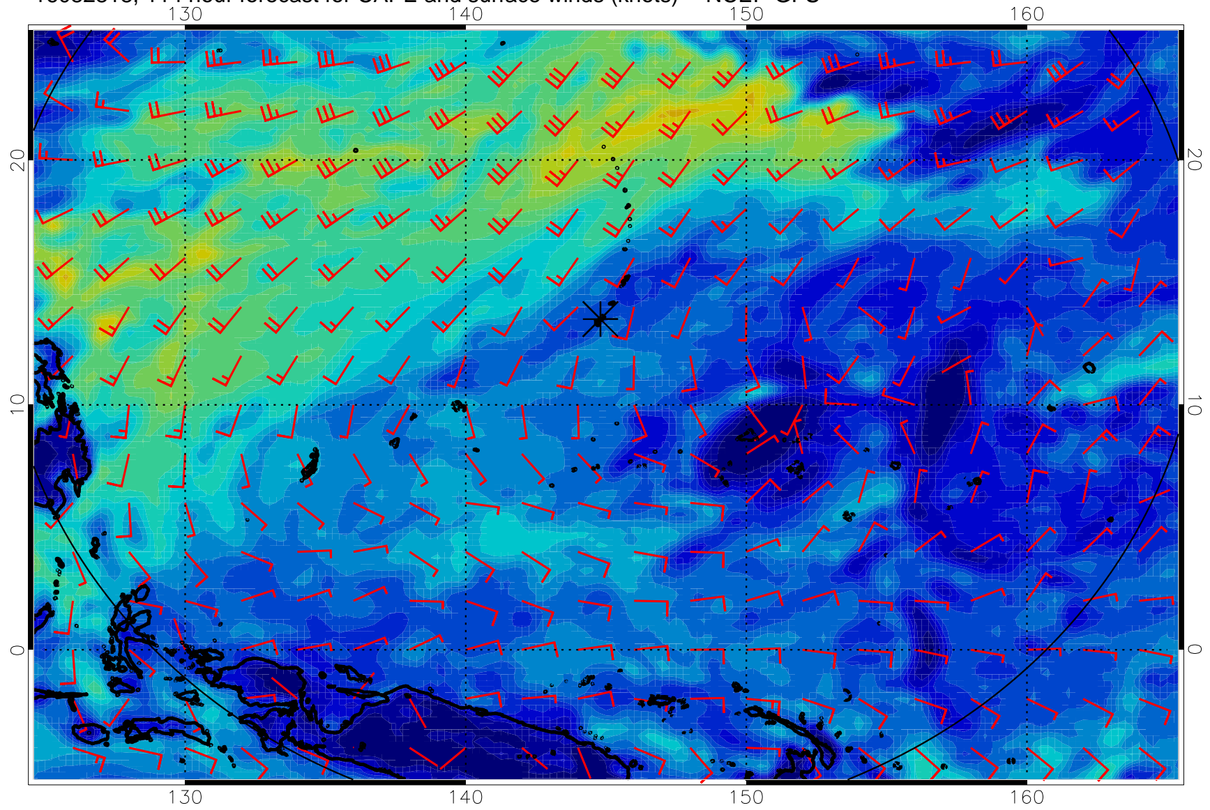
16082818, 114 hour forecast for CAPE and surface winds (knots) -- NCEP GFS
