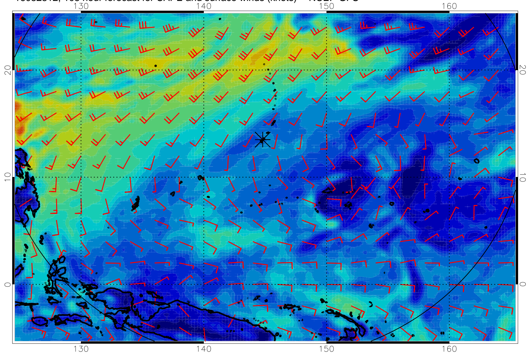
16082812, 108 hour forecast for CAPE and surface winds (knots) -- NCEP GFS
