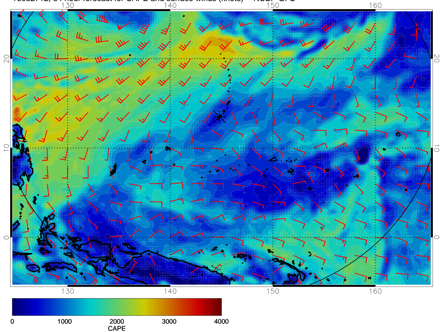
16082712, 84 hour forecast for CAPE and surface winds (knots) -- NCEP GFS
