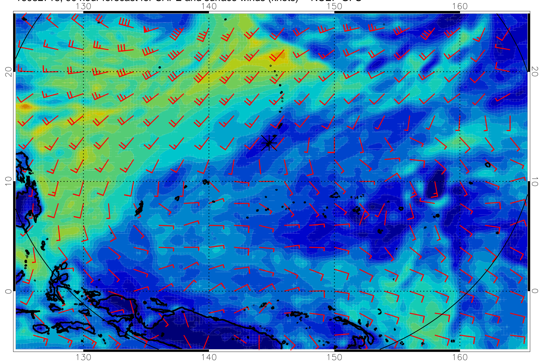
16082718, 90 hour forecast for CAPE and surface winds (knots) -- NCEP GFS
