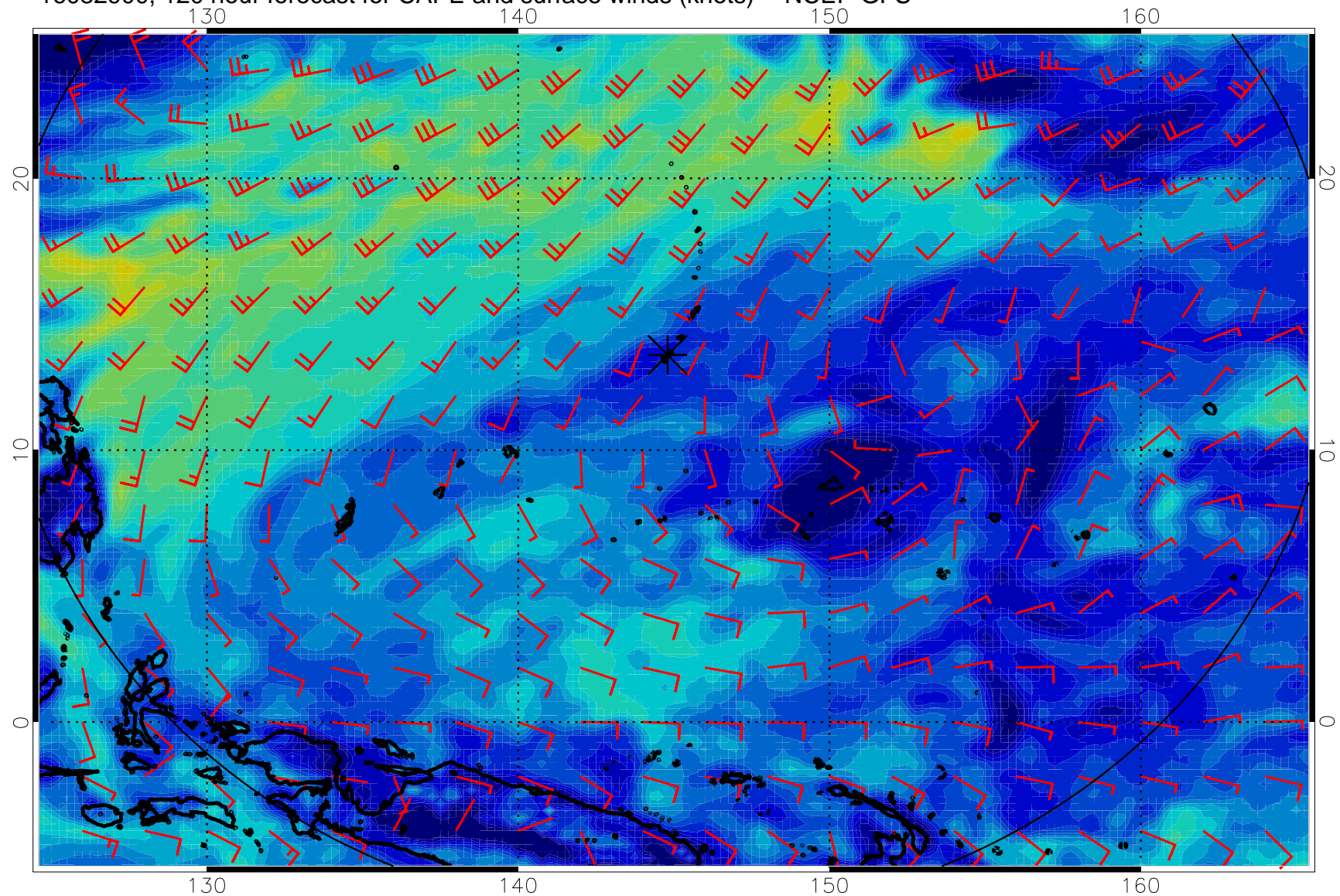
16082900, 120 hour forecast for CAPE and surface winds (knots) -- NCEP GFS
