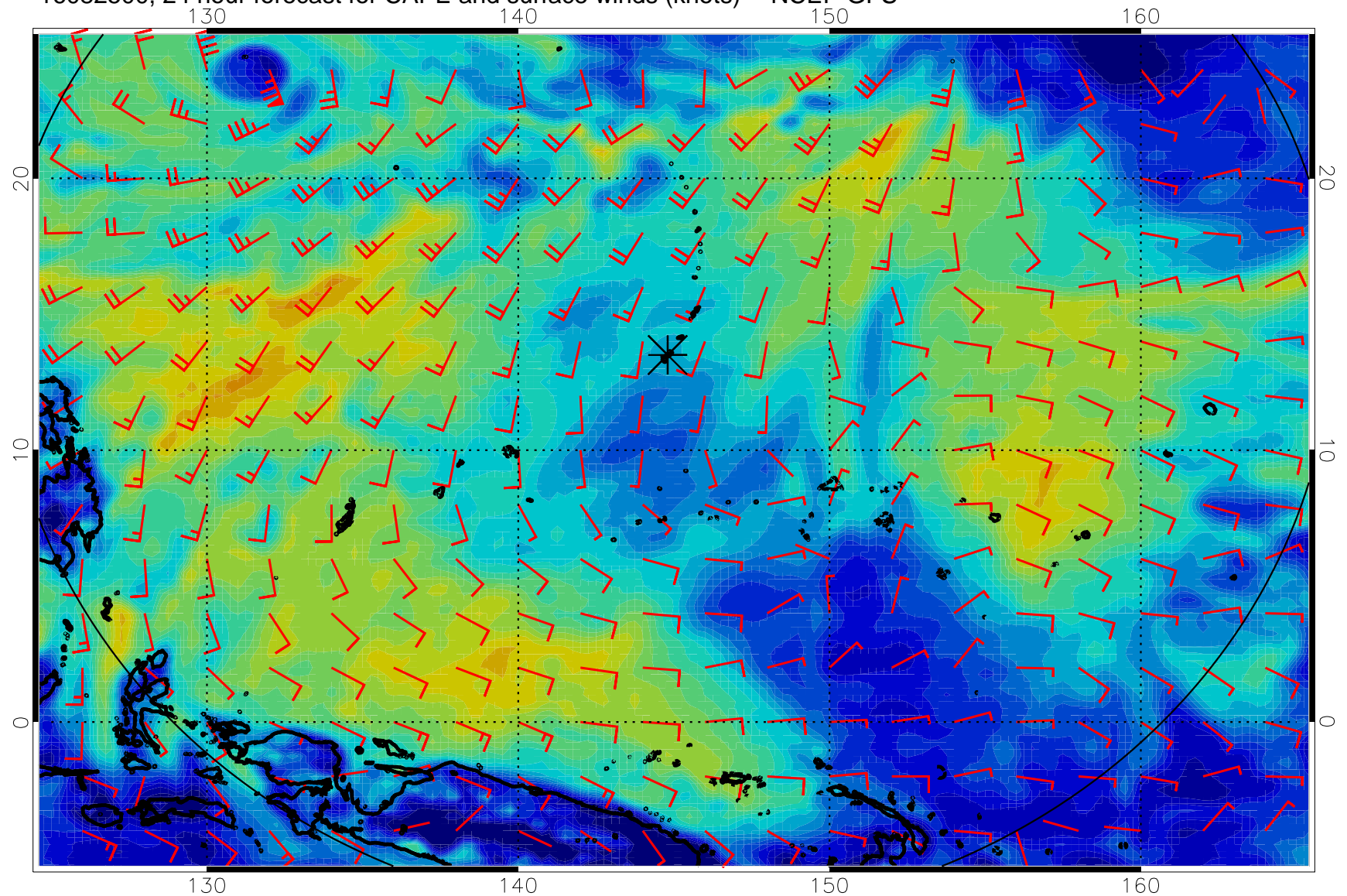
16082500, 24 hour forecast for CAPE and surface winds (knots) -- NCEP GFS
