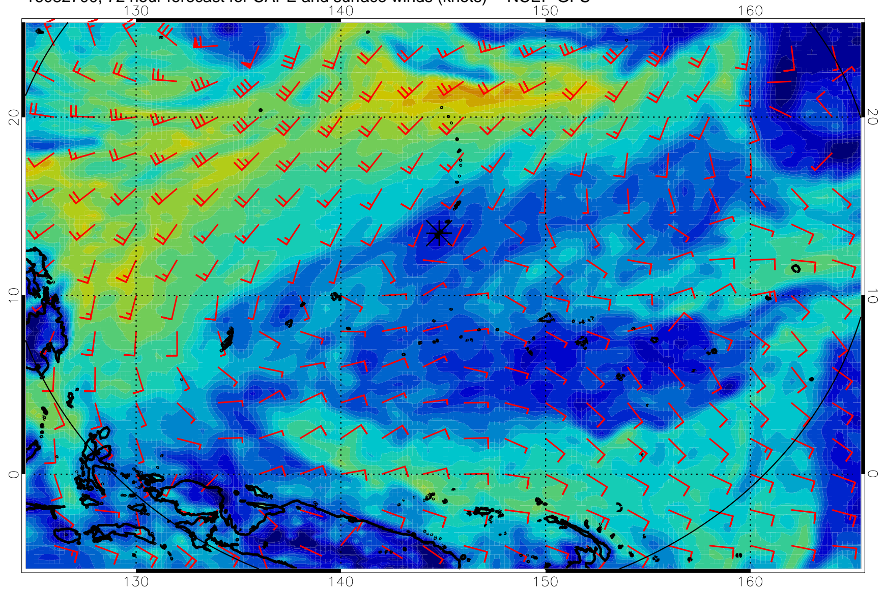
16082700, 72 hour forecast for CAPE and surface winds (knots) -- NCEP GFS
