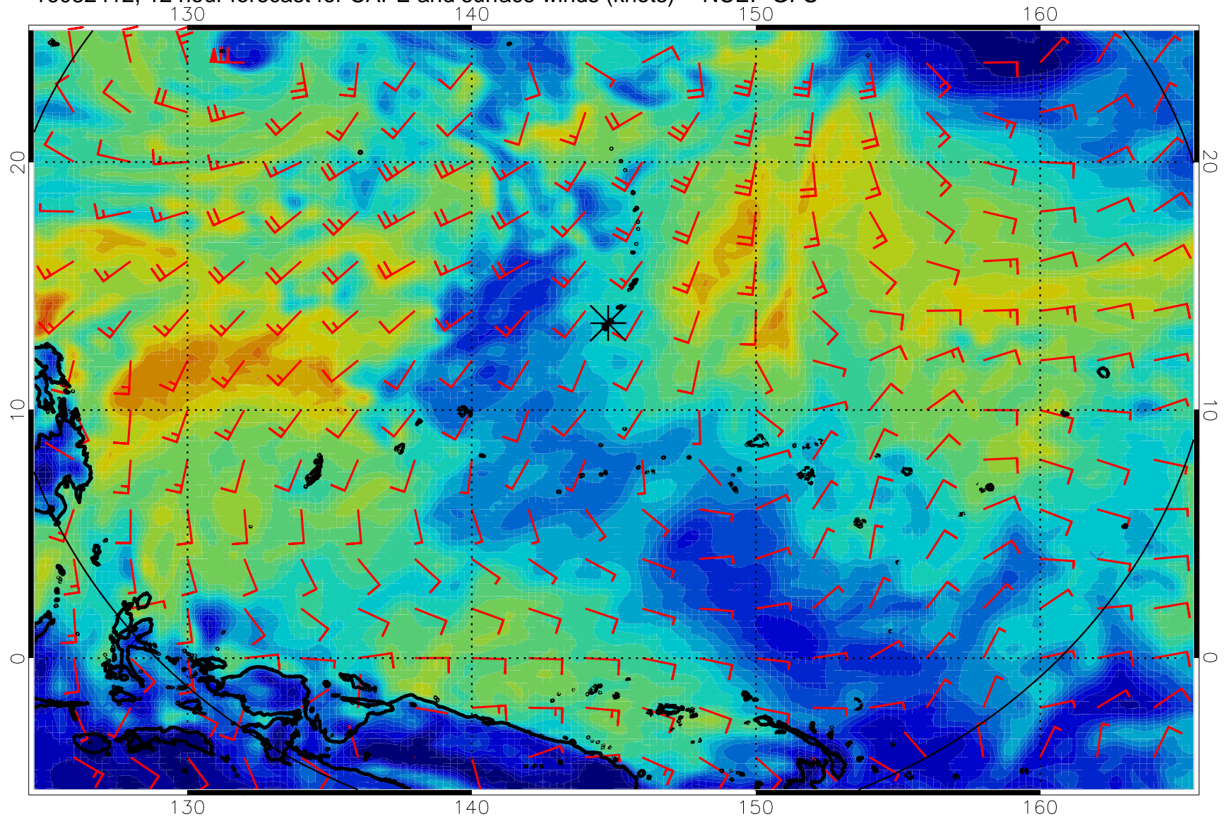
16082412, 12 hour forecast for CAPE and surface winds (knots) -- NCEP GFS
