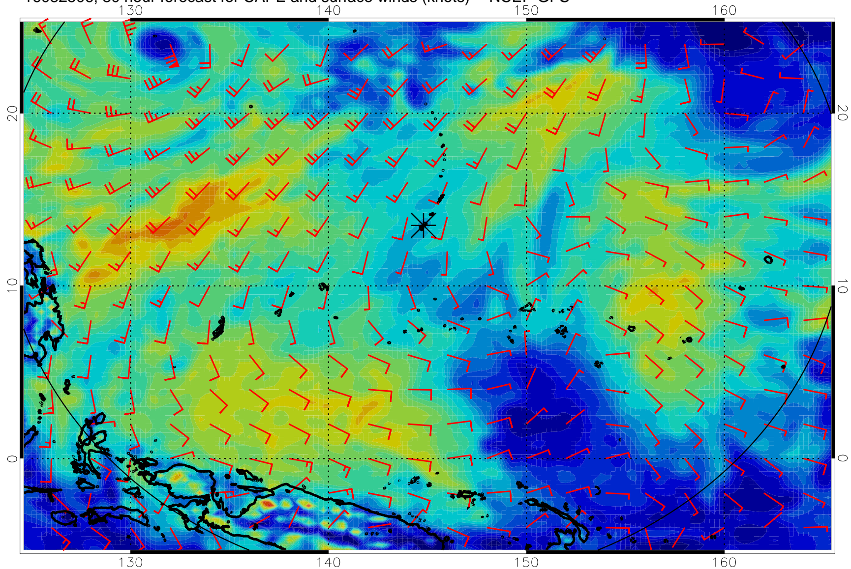
16082506, 30 hour forecast for CAPE and surface winds (knots) -- NCEP GFS
