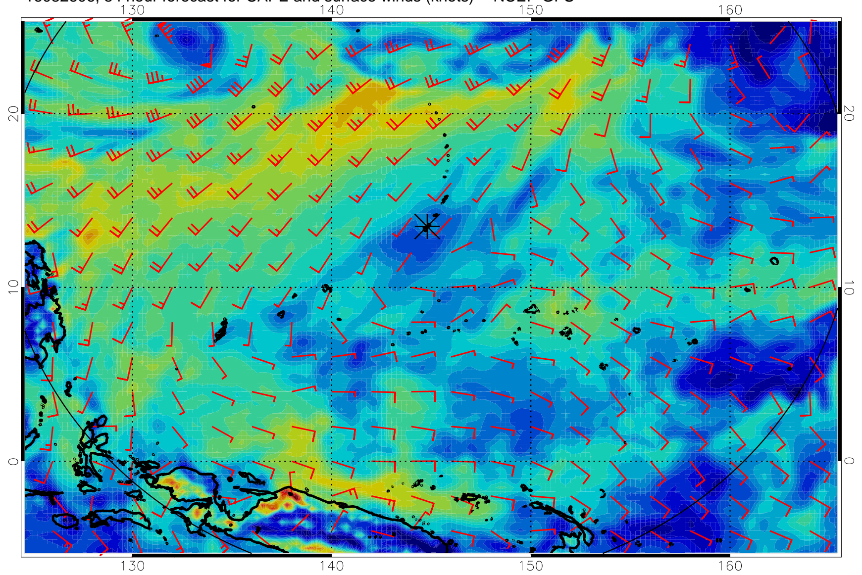
16082606, 54 hour forecast for CAPE and surface winds (knots) -- NCEP GFS
