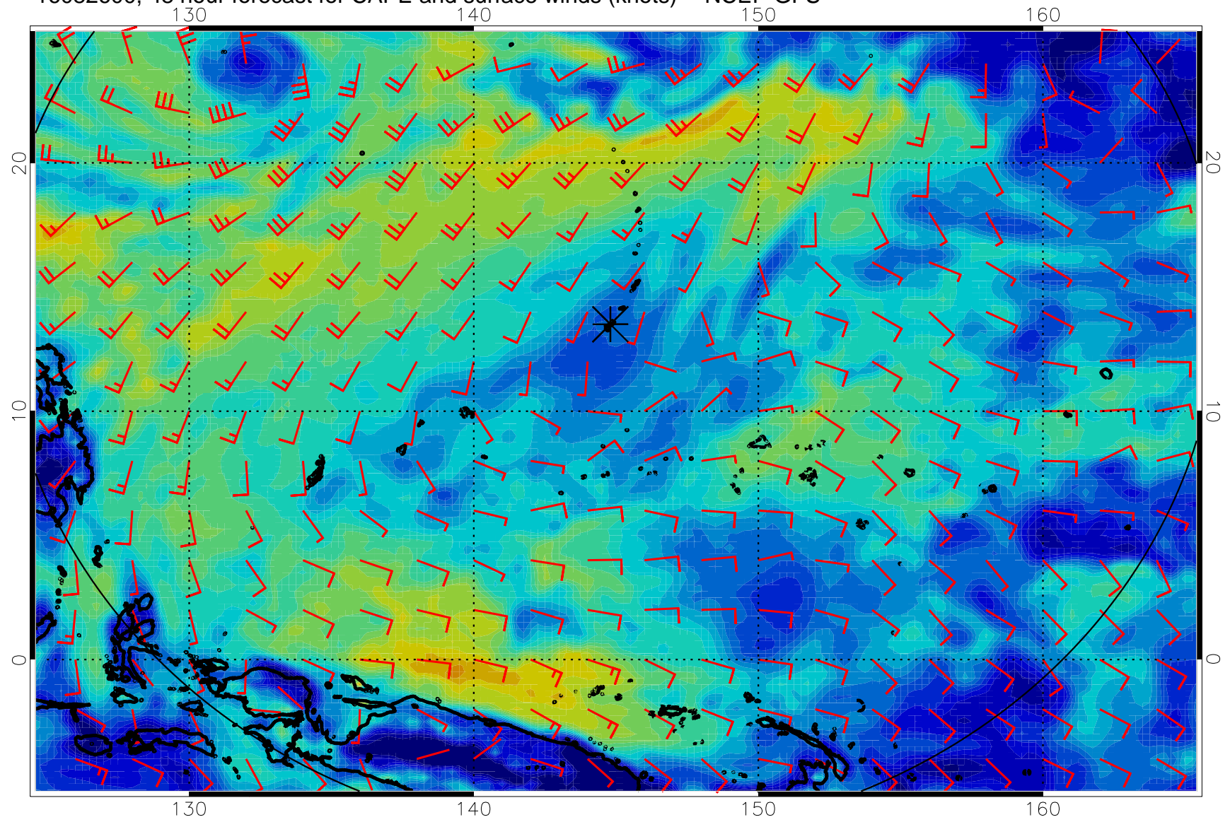
16082600, 48 hour forecast for CAPE and surface winds (knots) -- NCEP GFS
