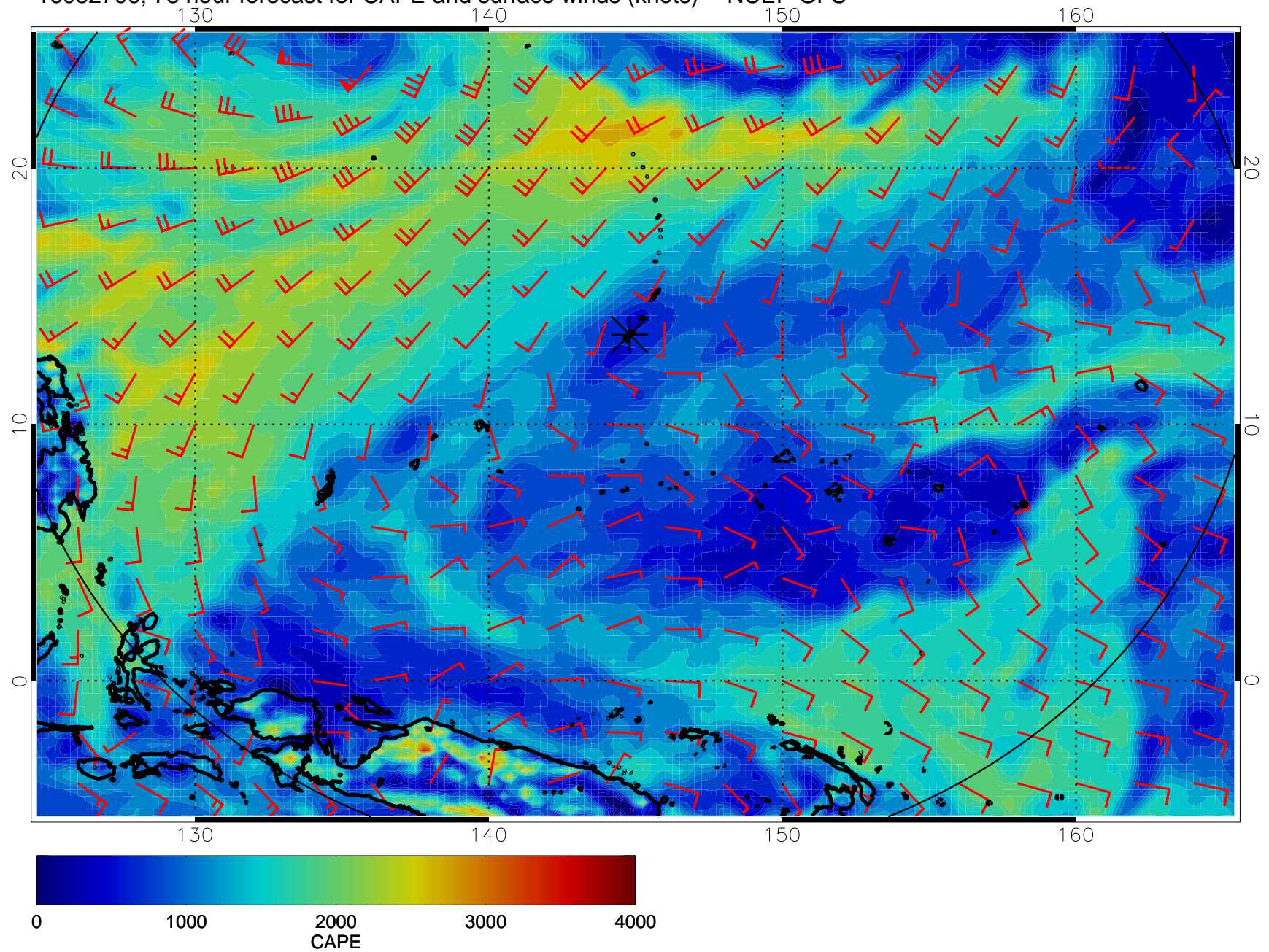
16082706, 78 hour forecast for CAPE and surface winds (knots) -- NCEP GFS
