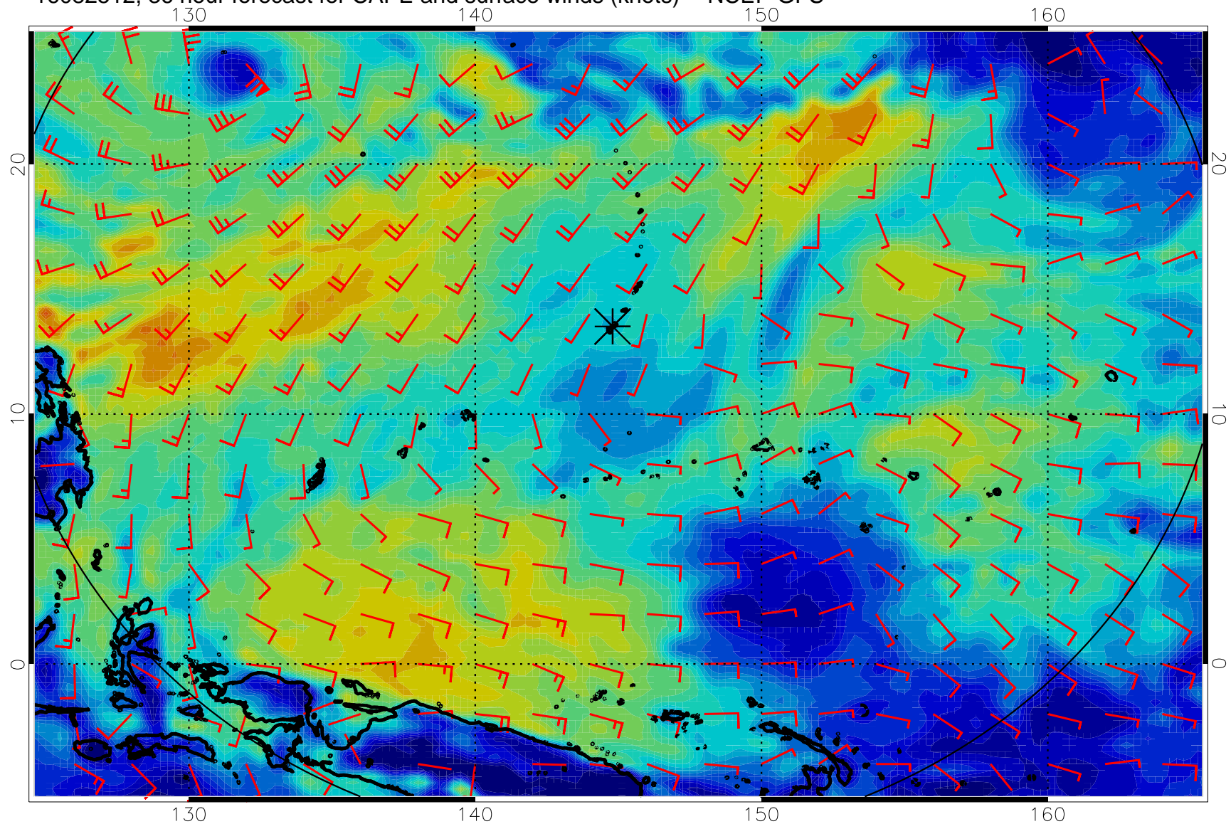
16082512, 36 hour forecast for CAPE and surface winds (knots) -- NCEP GFS
