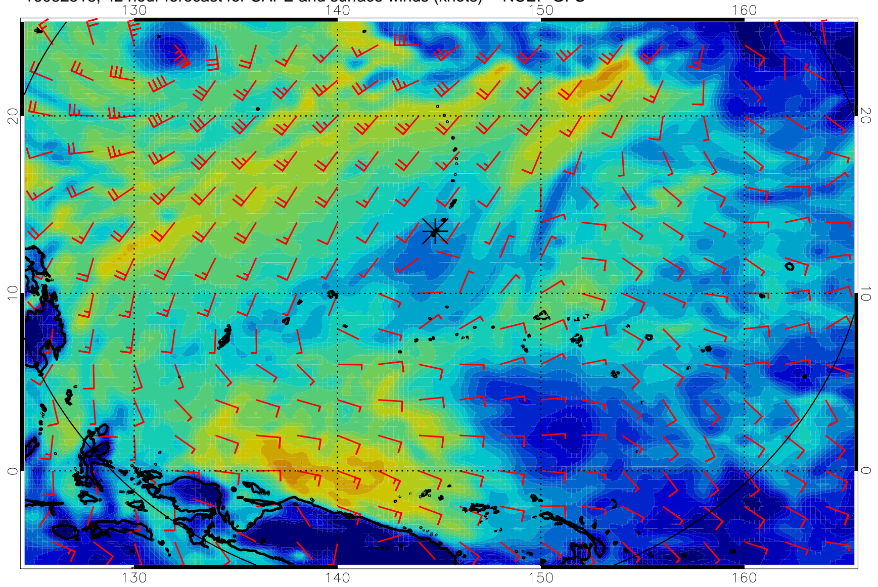
16082518, 42 hour forecast for CAPE and surface winds (knots) -- NCEP GFS
