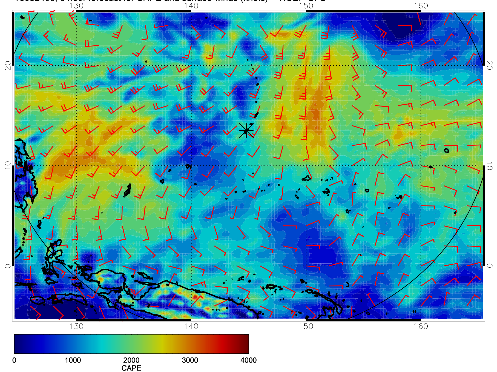
16082406, 6 hour forecast for CAPE and surface winds (knots) -- NCEP GFS
