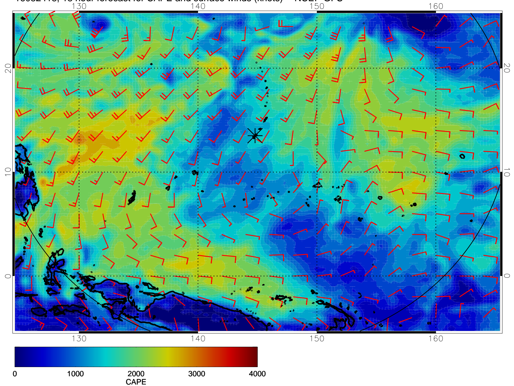
16082418, 18 hour forecast for CAPE and surface winds (knots) -- NCEP GFS
