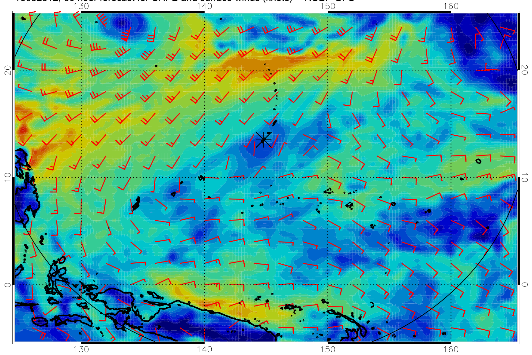
16082612, 60 hour forecast for CAPE and surface winds (knots) -- NCEP GFS
