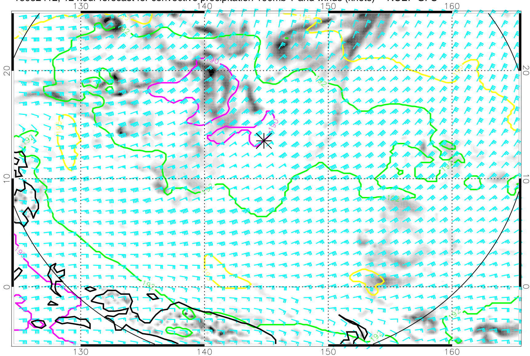
16082412, 12 hour forecast for convective precipitation 100mb T and winds (knots) -- NCEP GFS
