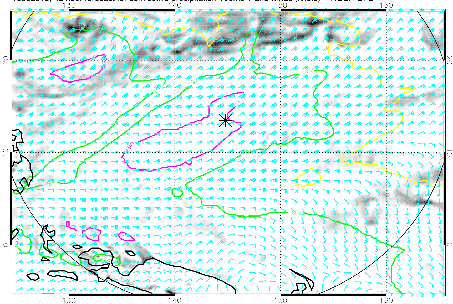
16082518, 42 hour forecast for convective precipitation 100mb T and winds (knots) -- NCEP GFS
