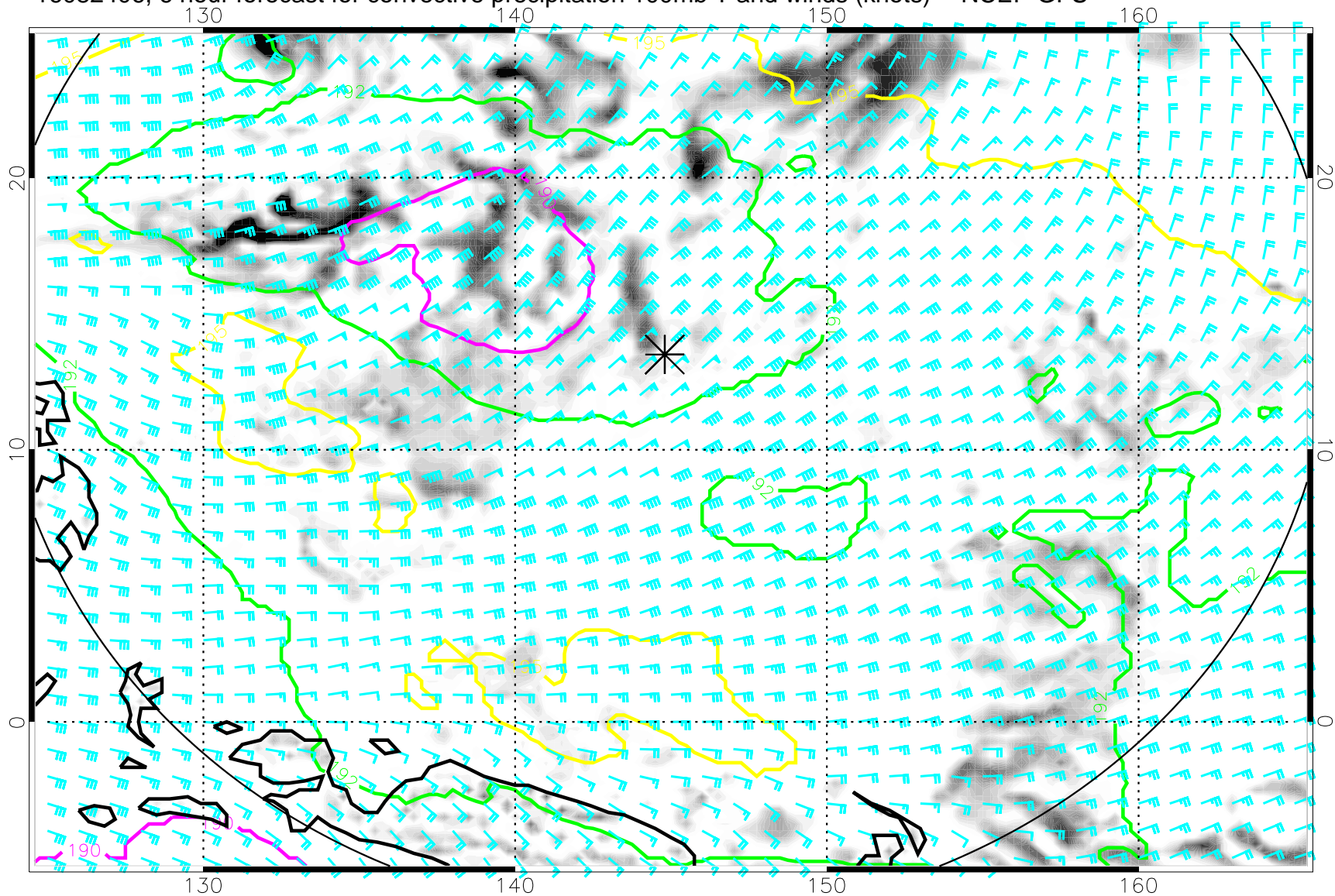
16082406, 6 hour forecast for convective precipitation 100mb T and winds (knots) -- NCEP GFS
