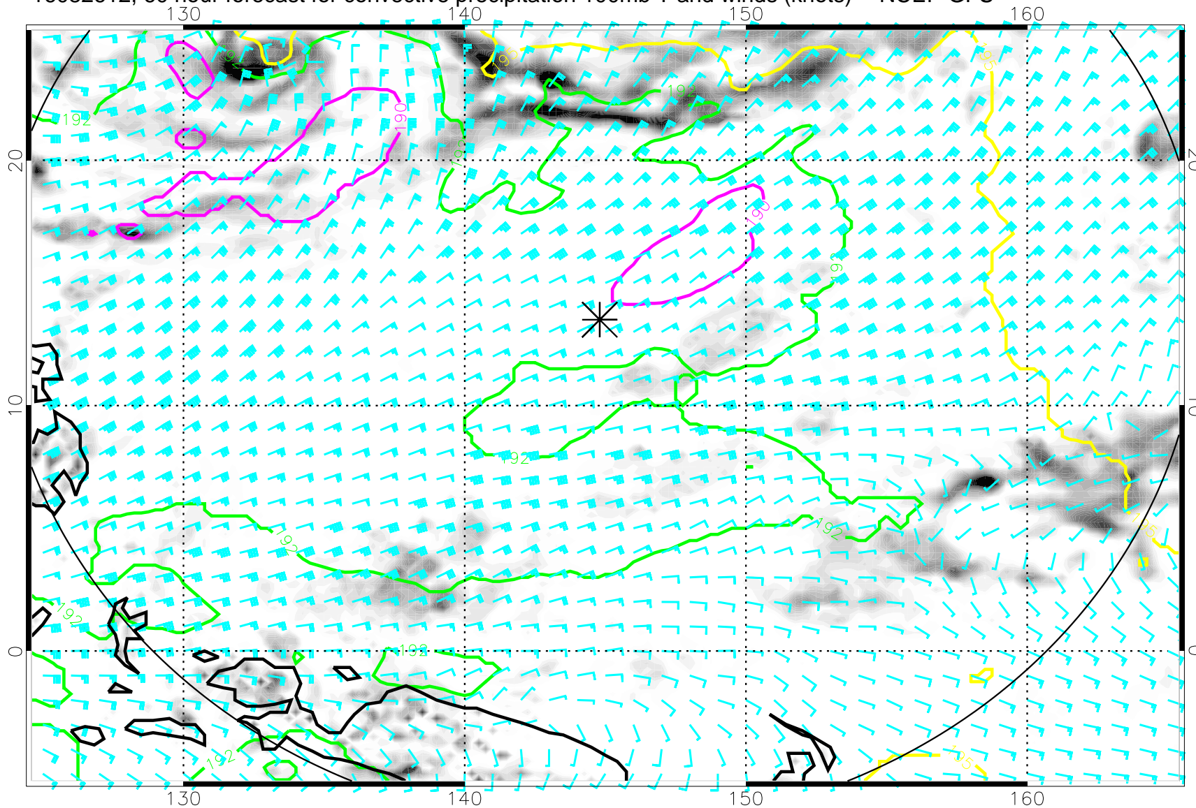
16082612, 60 hour forecast for convective precipitation 100mb T and winds (knots) -- NCEP GFS
