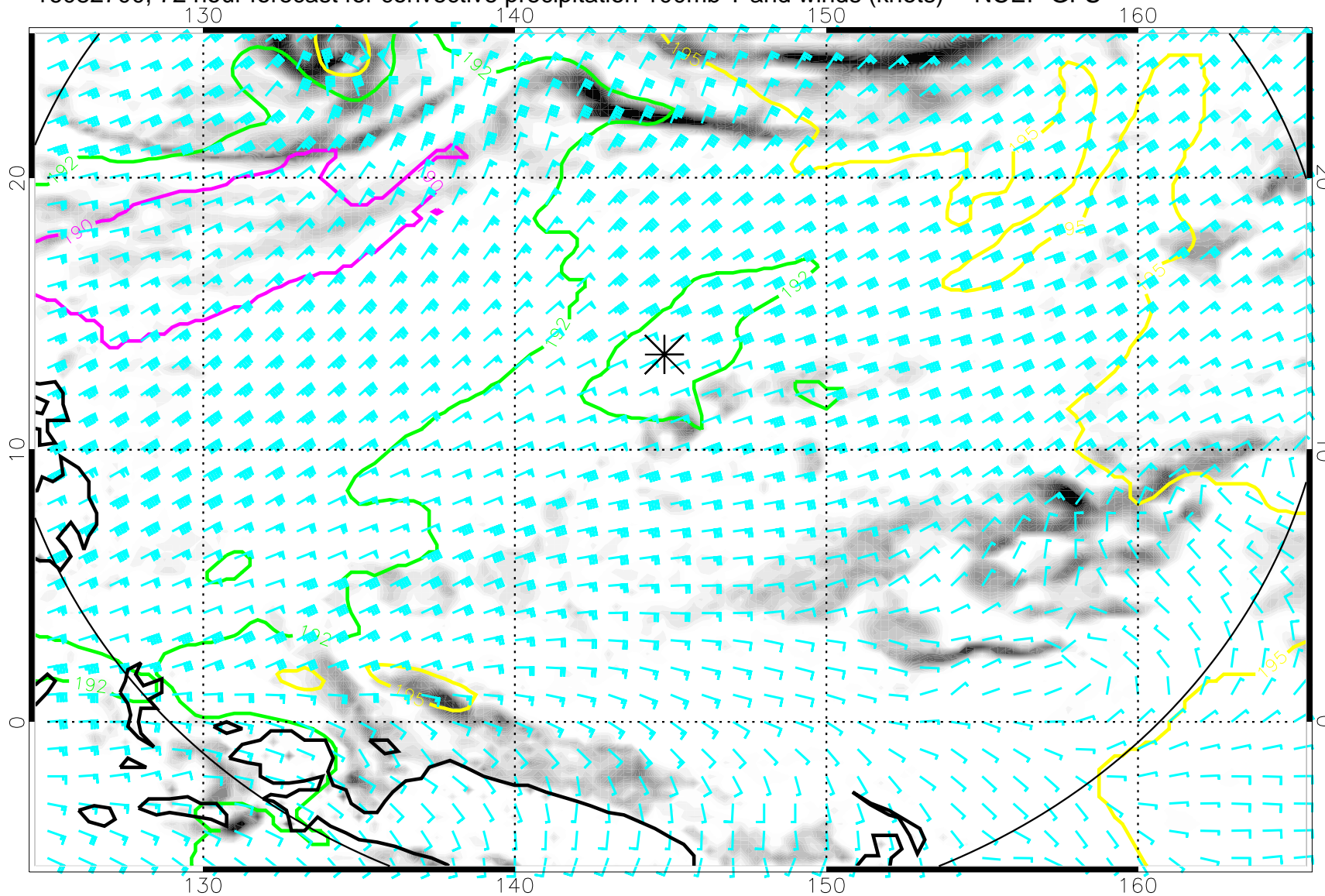
16082700, 72 hour forecast for convective precipitation 100mb T and winds (knots) -- NCEP GFS
