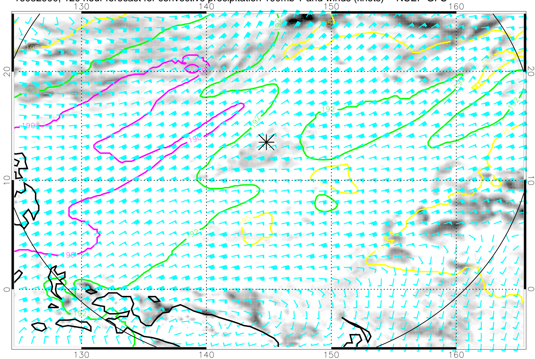
16082900, 120 hour forecast for convective precipitation 100mb T and winds (knots) -- NCEP GFS
