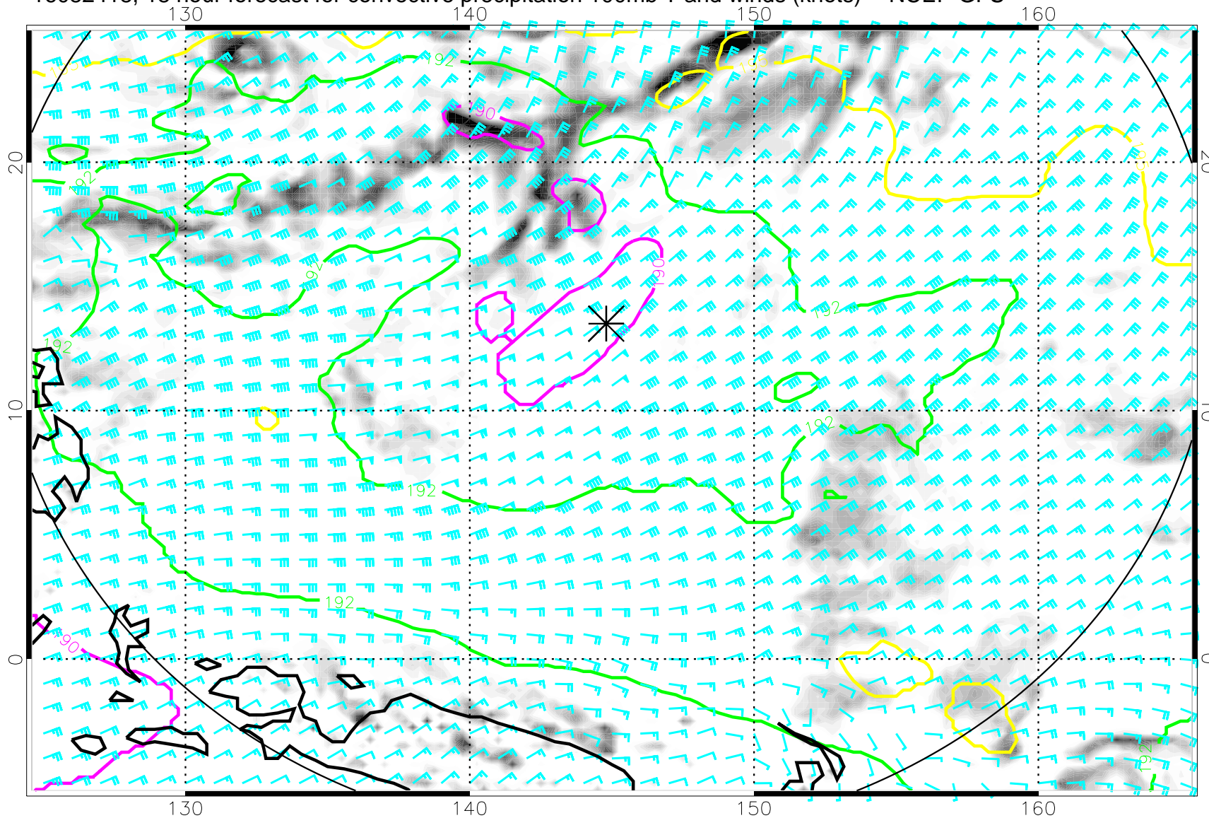
16082418, 18 hour forecast for convective precipitation 100mb T and winds (knots) -- NCEP GFS
