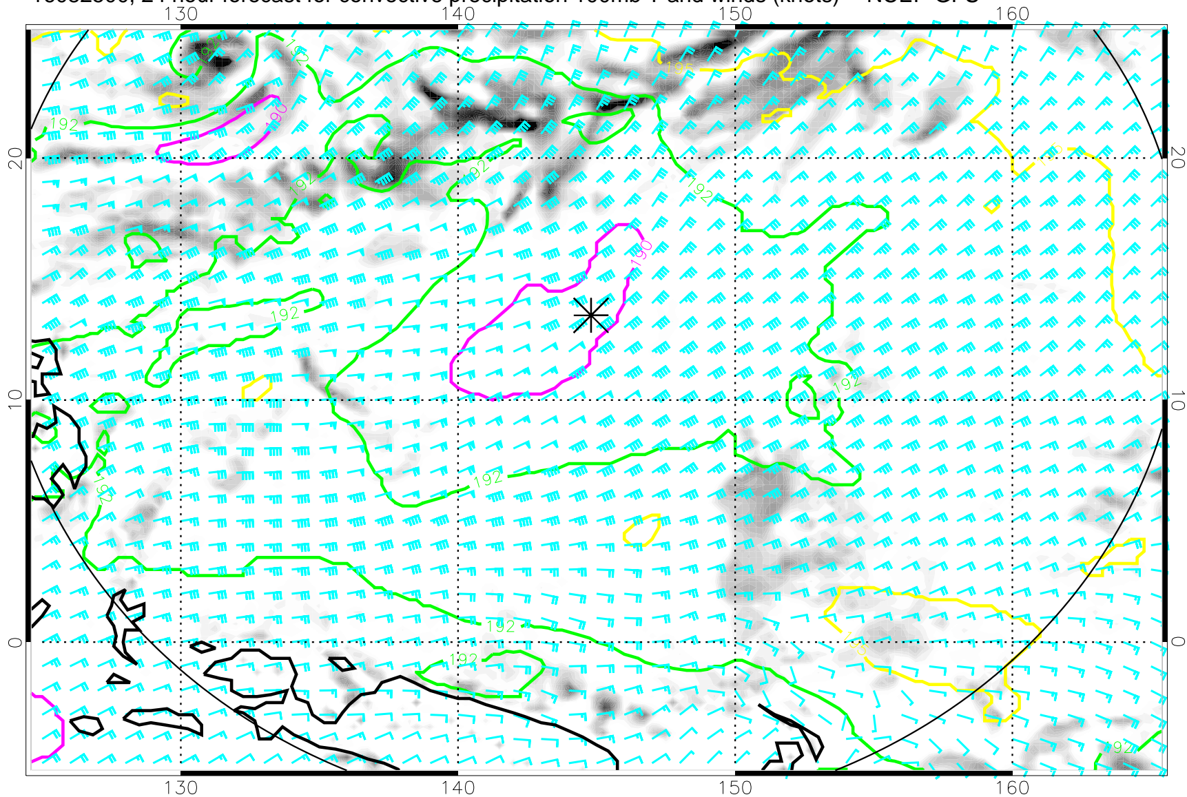
16082500, 24 hour forecast for convective precipitation 100mb T and winds (knots) -- NCEP GFS
