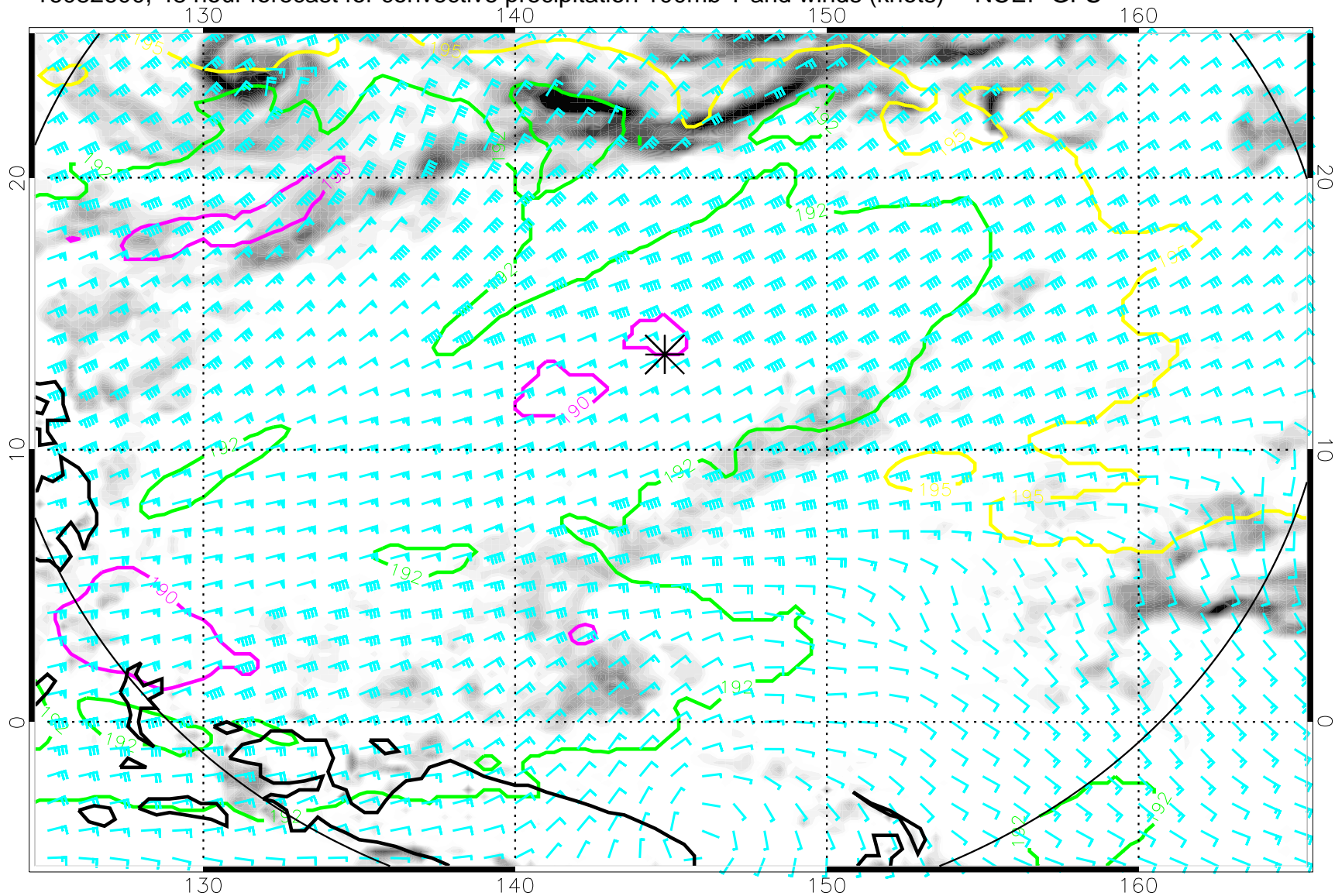
16082600, 48 hour forecast for convective precipitation 100mb T and winds (knots) -- NCEP GFS
