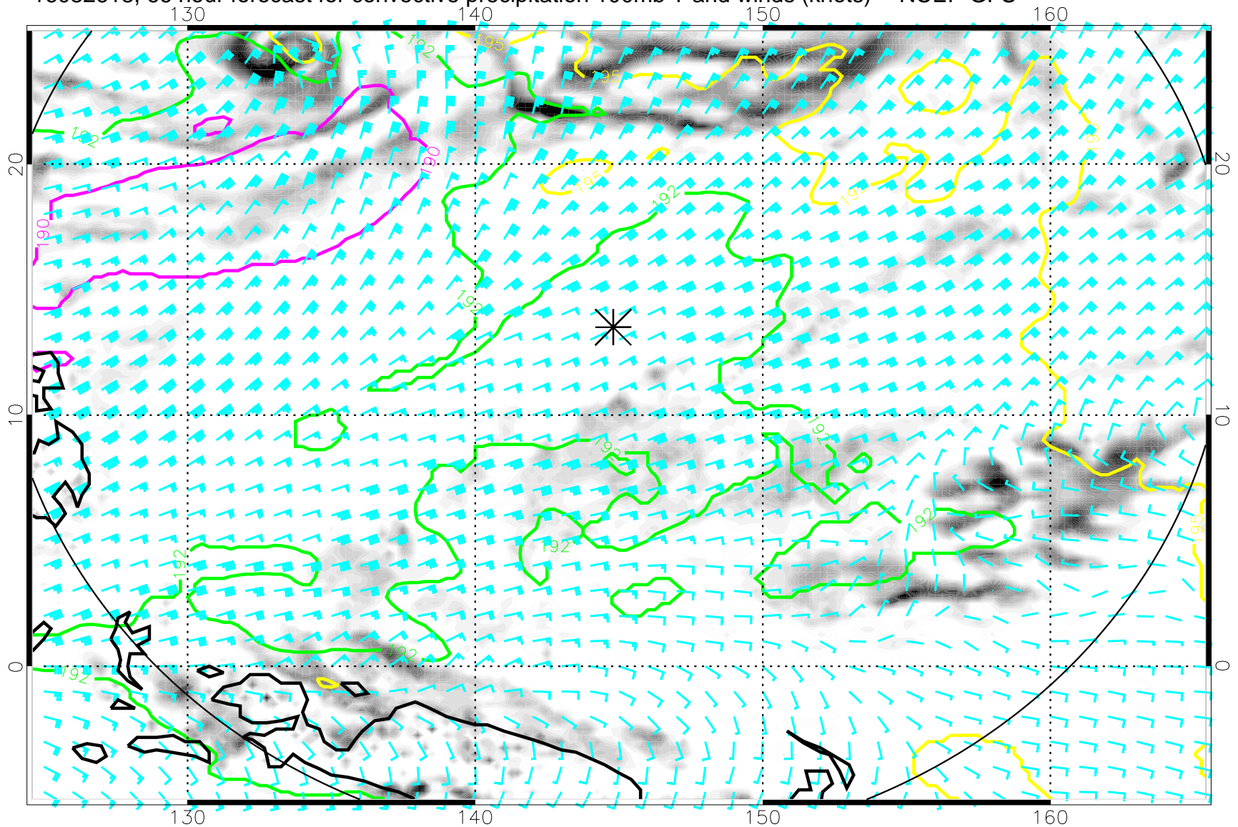
16082618, 66 hour forecast for convective precipitation 100mb T and winds (knots) -- NCEP GFS
