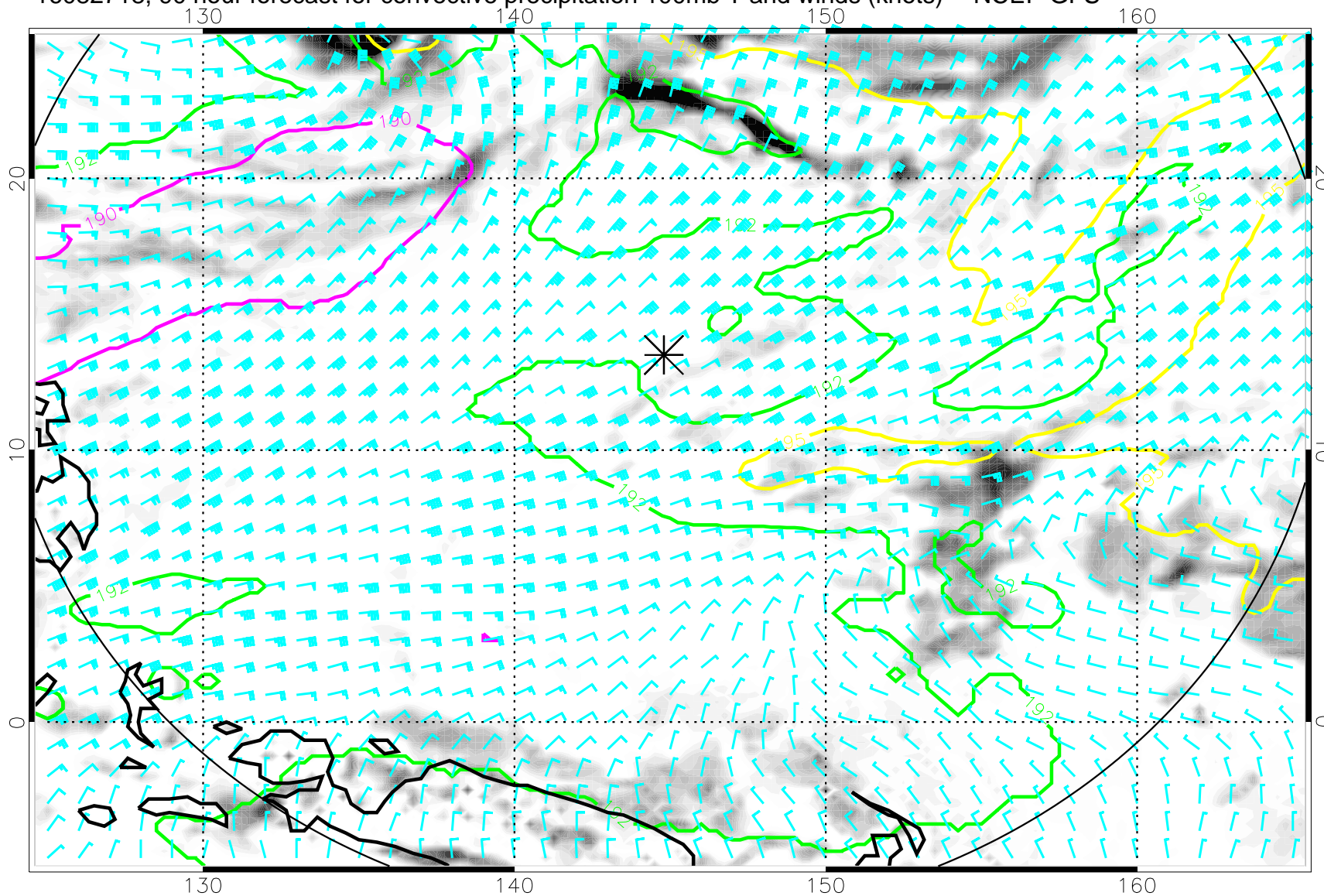
16082718, 90 hour forecast for convective precipitation 100mb T and winds (knots) -- NCEP GFS
