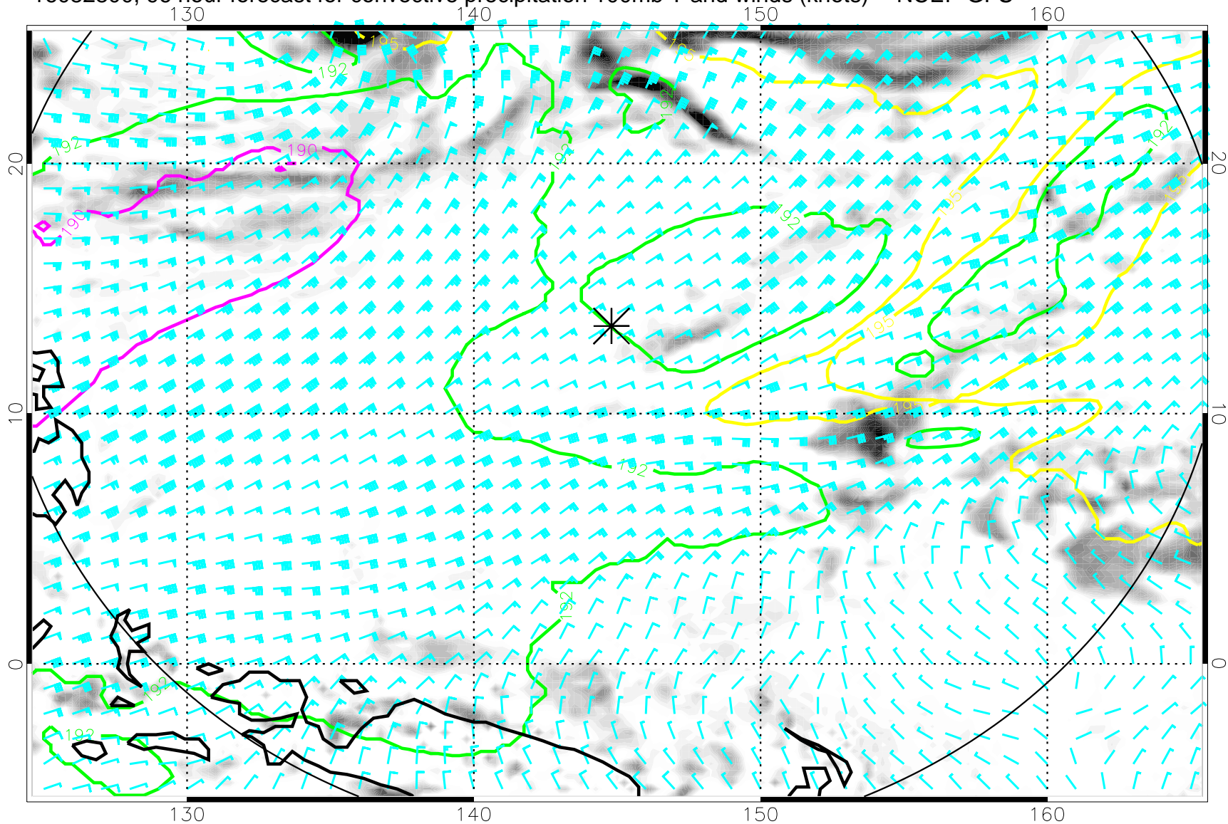
16082800, 96 hour forecast for convective precipitation 100mb T and winds (knots) -- NCEP GFS
