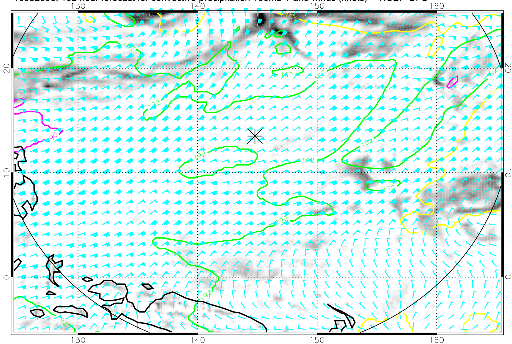
16082806, 102 hour forecast for convective precipitation 100mb T and winds (knots) -- NCEP GFS
