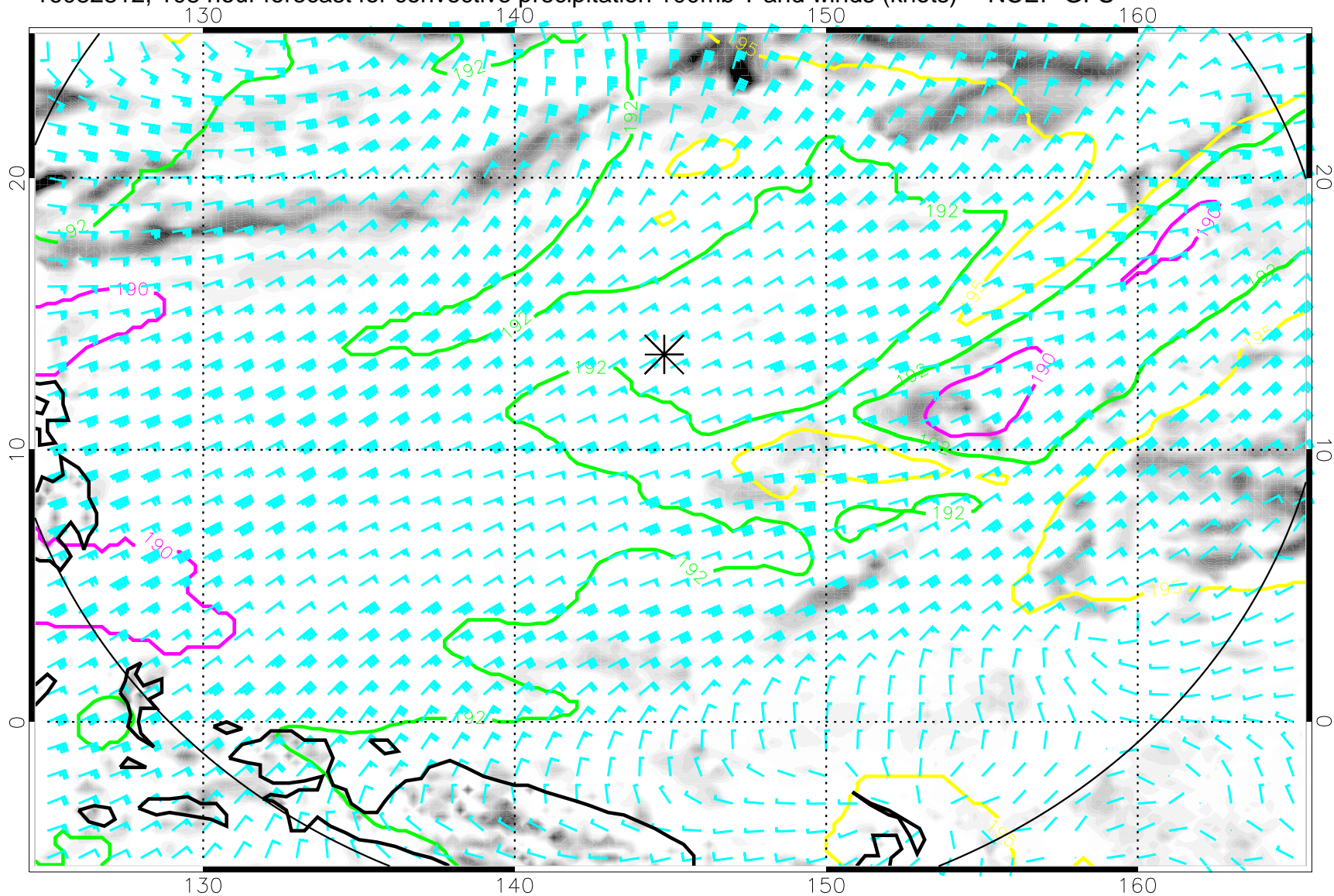
16082812, 108 hour forecast for convective precipitation 100mb T and winds (knots) -- NCEP GFS
