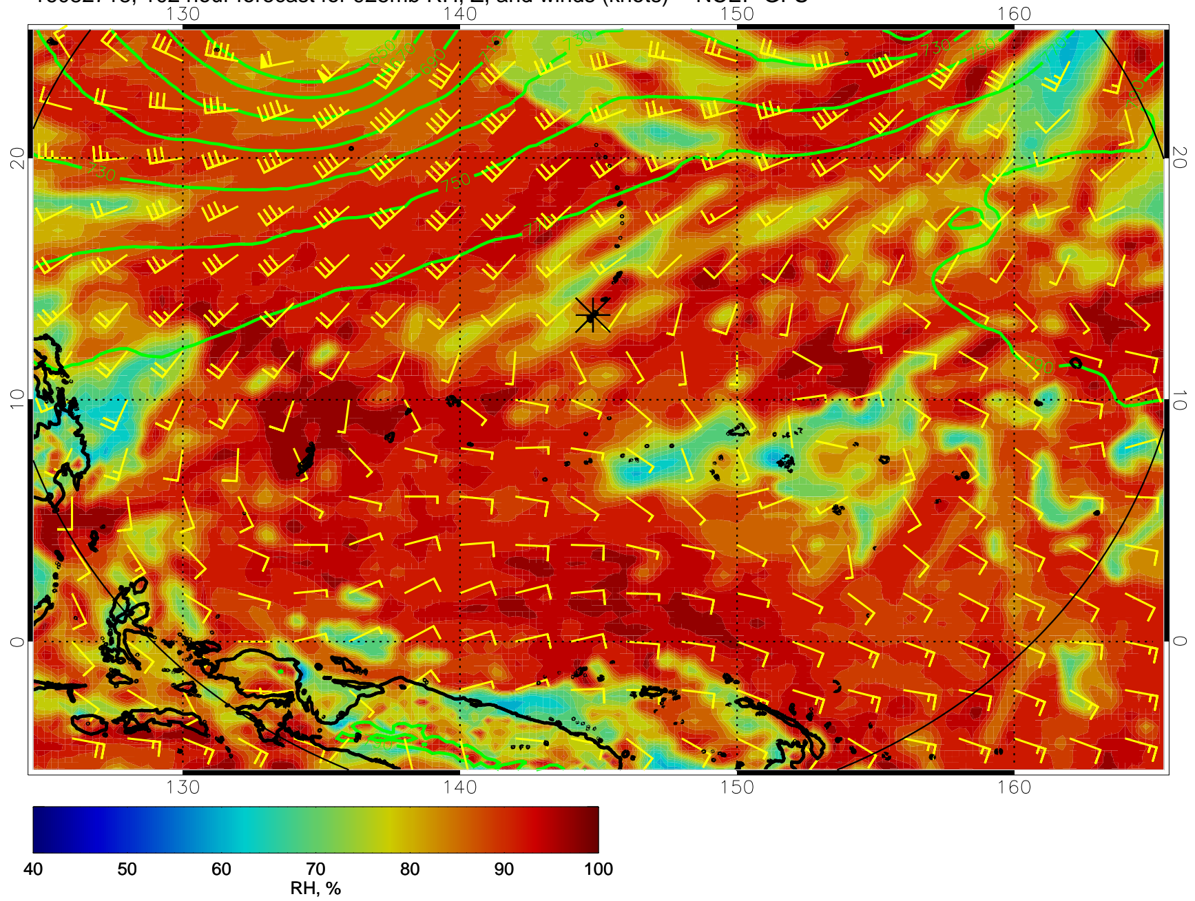
16082718, 102 hour forecast for 925mb RH, Z, and winds (knots) -- NCEP GFS
