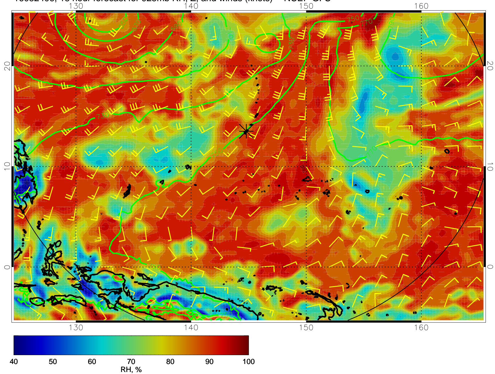
16082406, 18 hour forecast for 925mb RH, Z, and winds (knots) -- NCEP GFS
