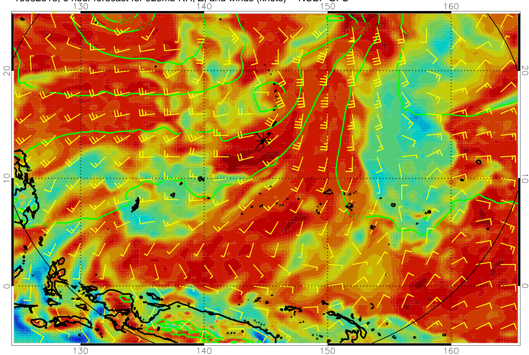
16082318, 6 hour forecast for 925mb RH, Z, and winds (knots) -- NCEP GFS
