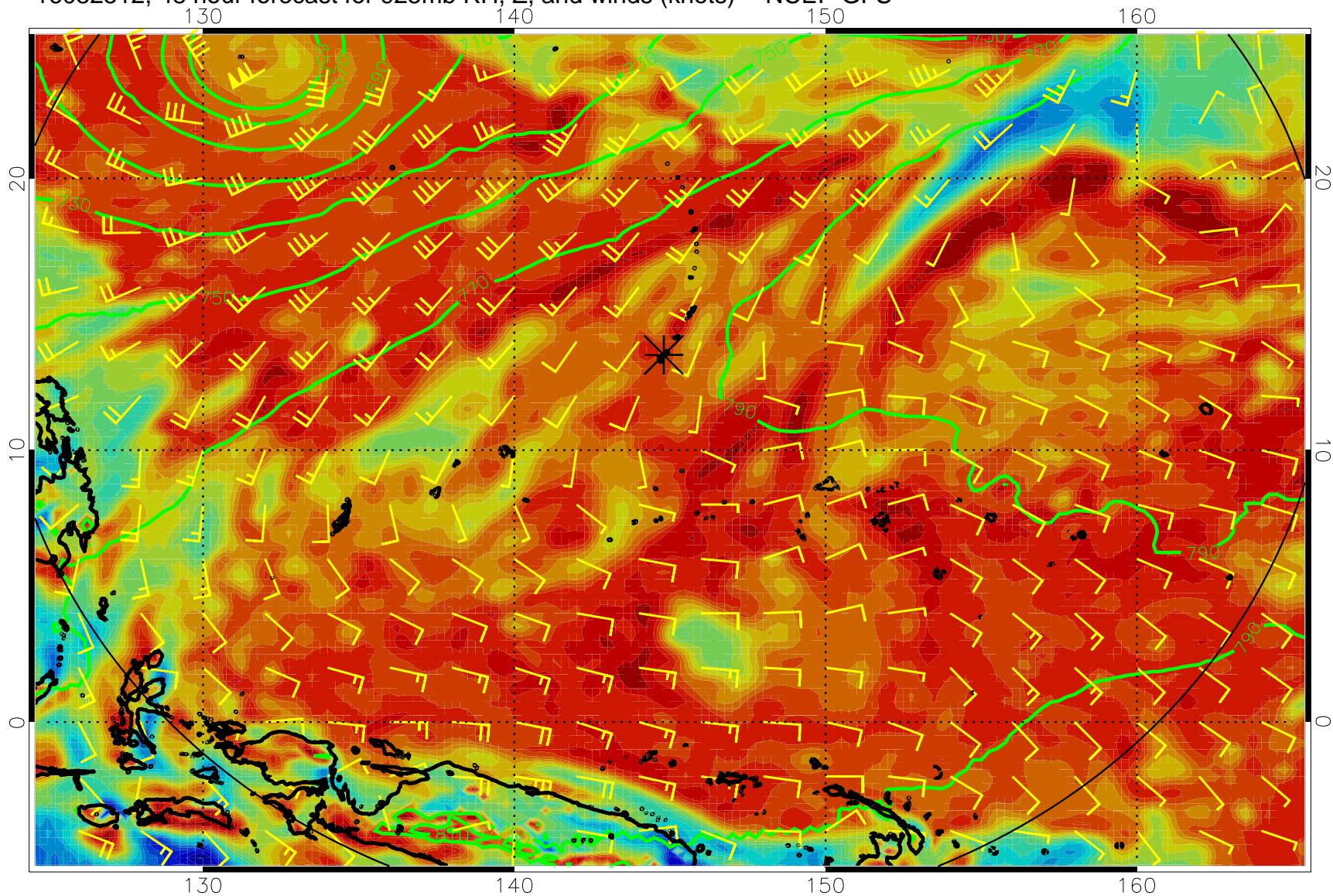
16082512, 48 hour forecast for 925mb RH, Z, and winds (knots) -- NCEP GFS
