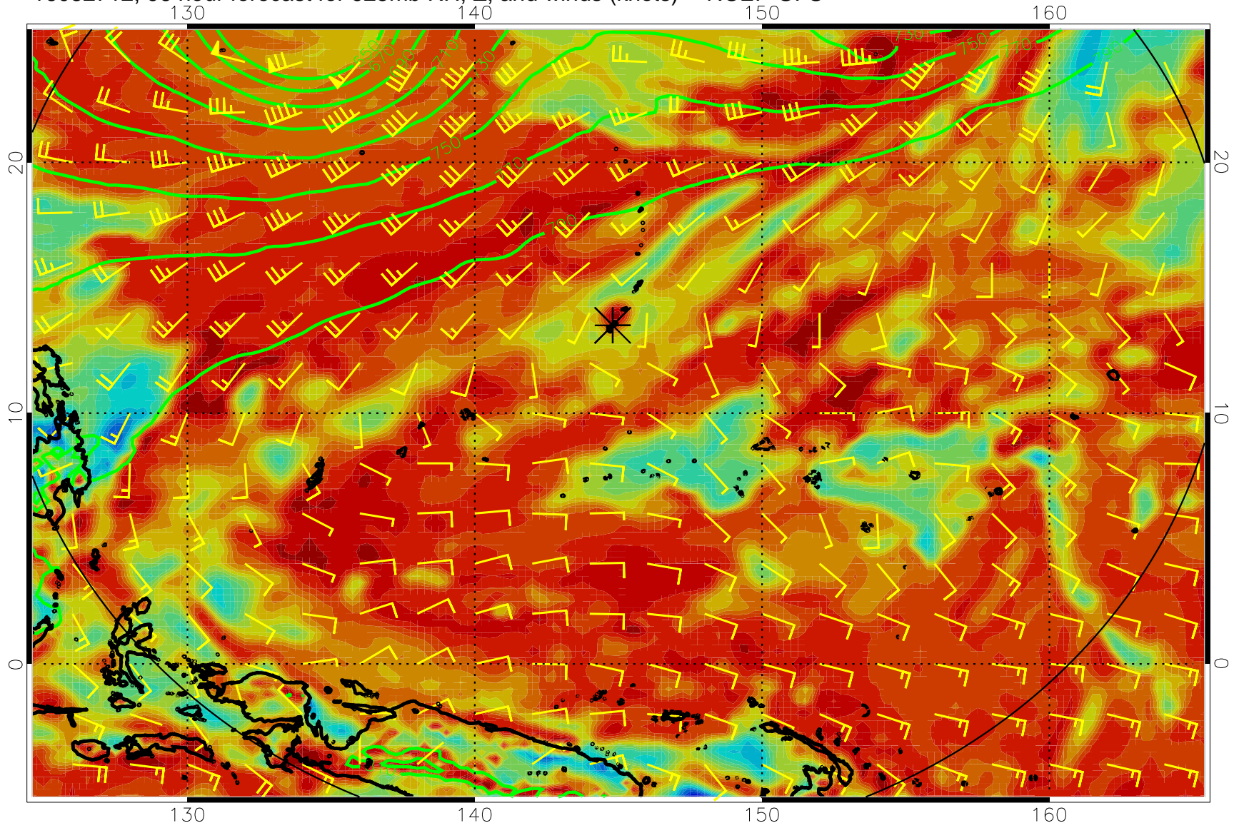
16082712, 96 hour forecast for 925mb RH, Z, and winds (knots) -- NCEP GFS
