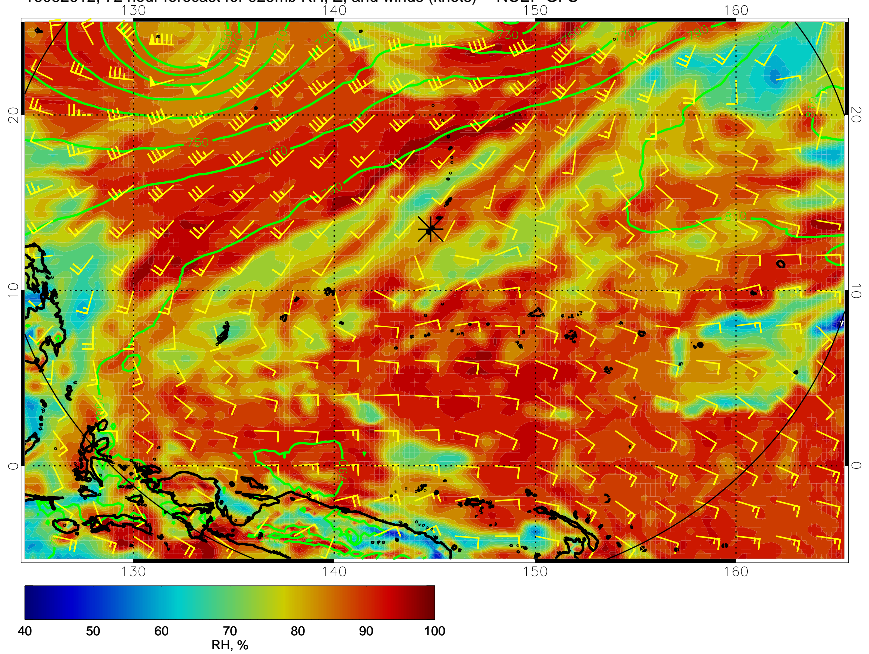
16082612, 72 hour forecast for 925mb RH, Z, and winds (knots) -- NCEP GFS
