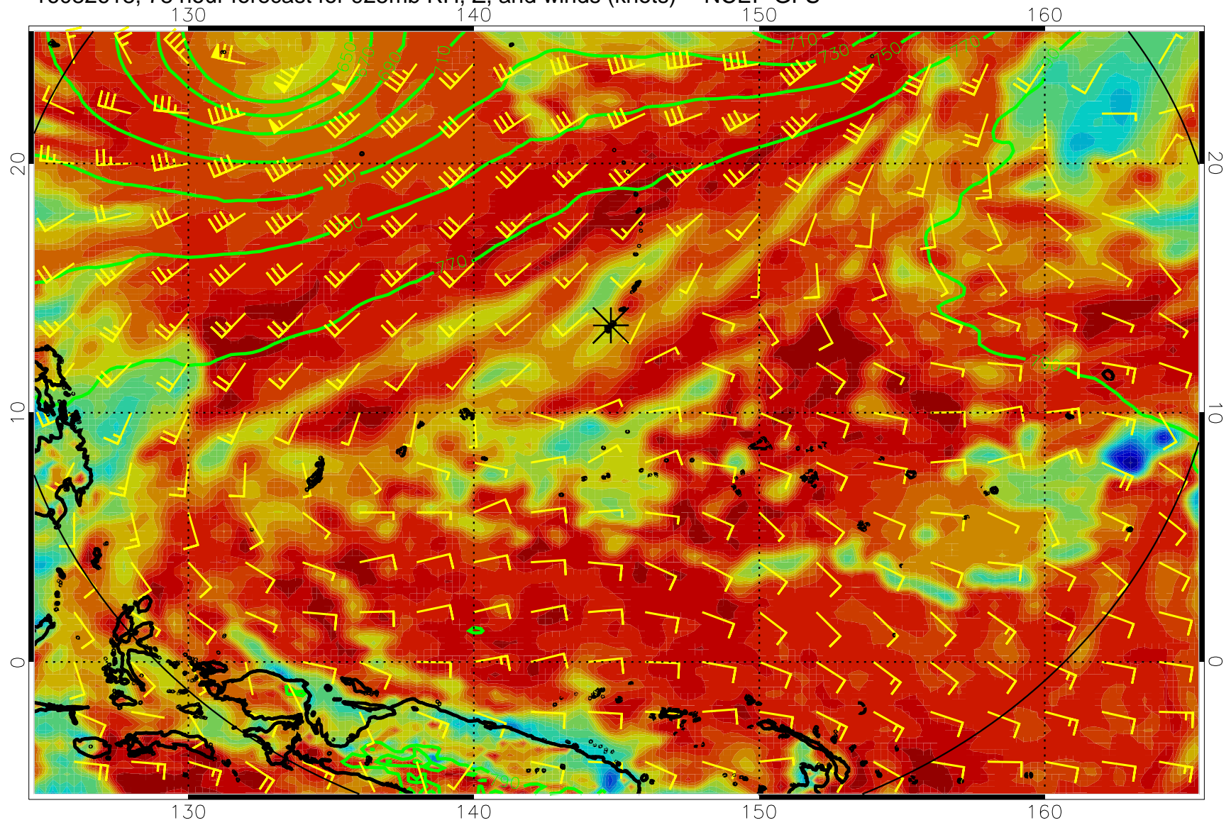
16082618, 78 hour forecast for 925mb RH, Z, and winds (knots) -- NCEP GFS
