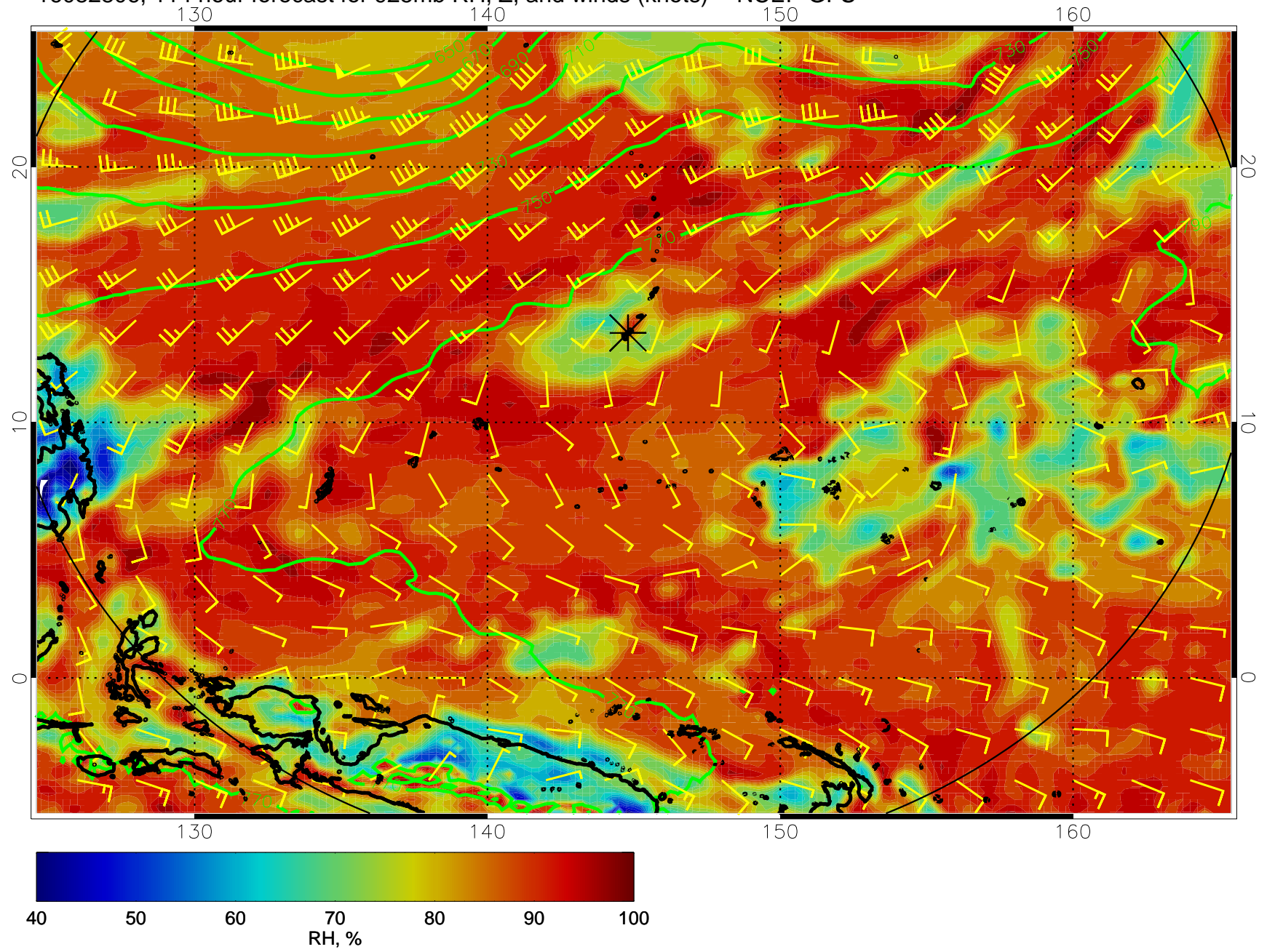
16082806, 114 hour forecast for 925mb RH, Z, and winds (knots) -- NCEP GFS
