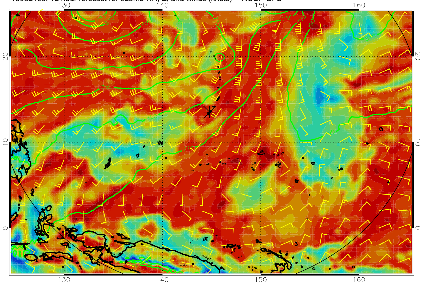
16082400, 12 hour forecast for 925mb RH, Z, and winds (knots) -- NCEP GFS
