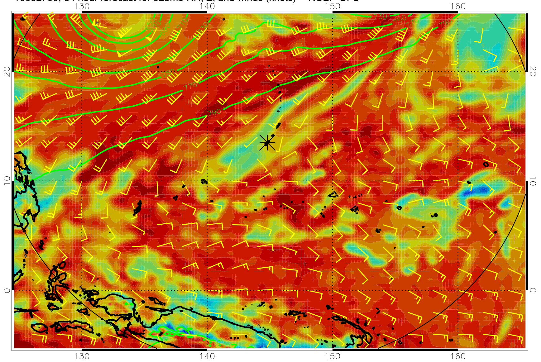
16082700, 84 hour forecast for 925mb RH, Z, and winds (knots) -- NCEP GFS
