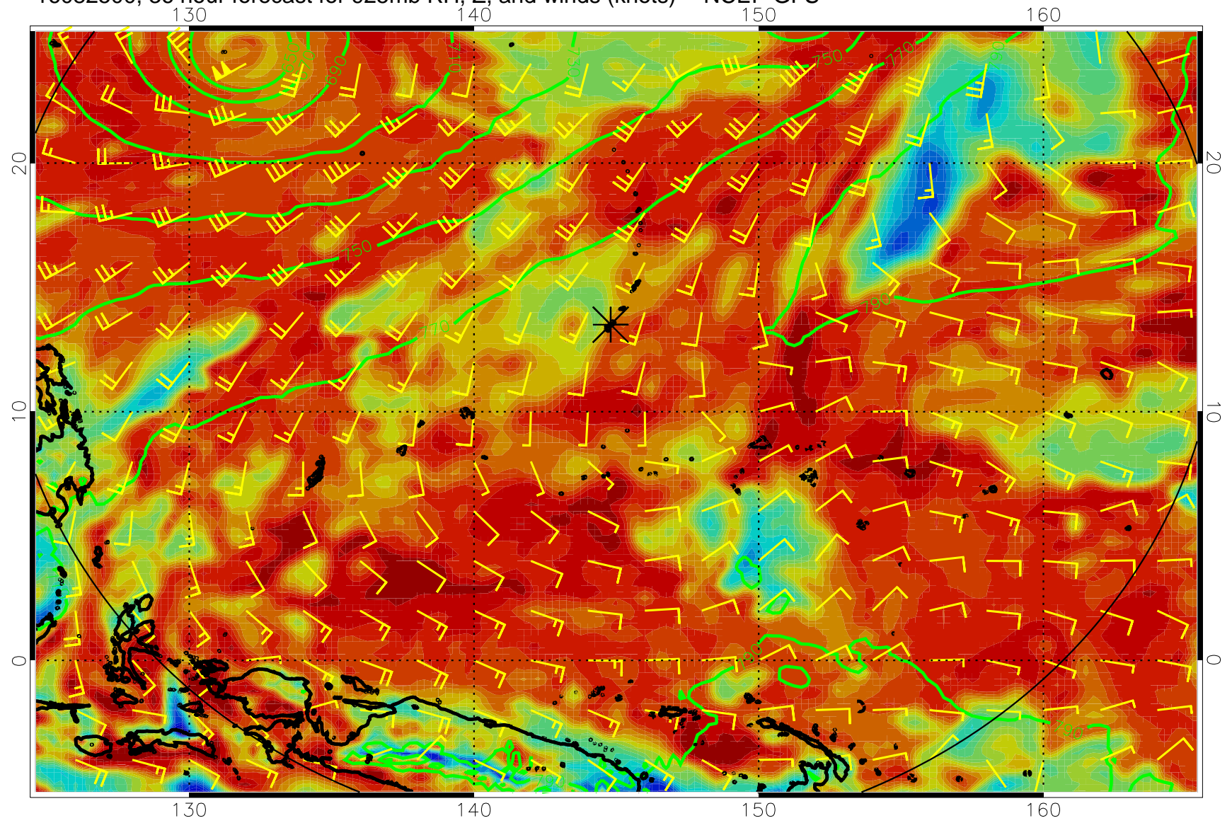
16082500, 36 hour forecast for 925mb RH, Z, and winds (knots) -- NCEP GFS
