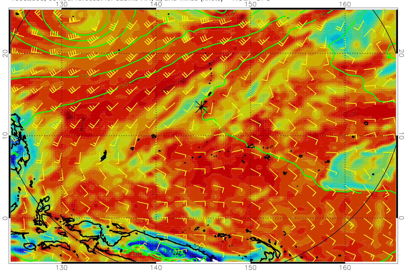
16082606, 66 hour forecast for 925mb RH, Z, and winds (knots) -- NCEP GFS
