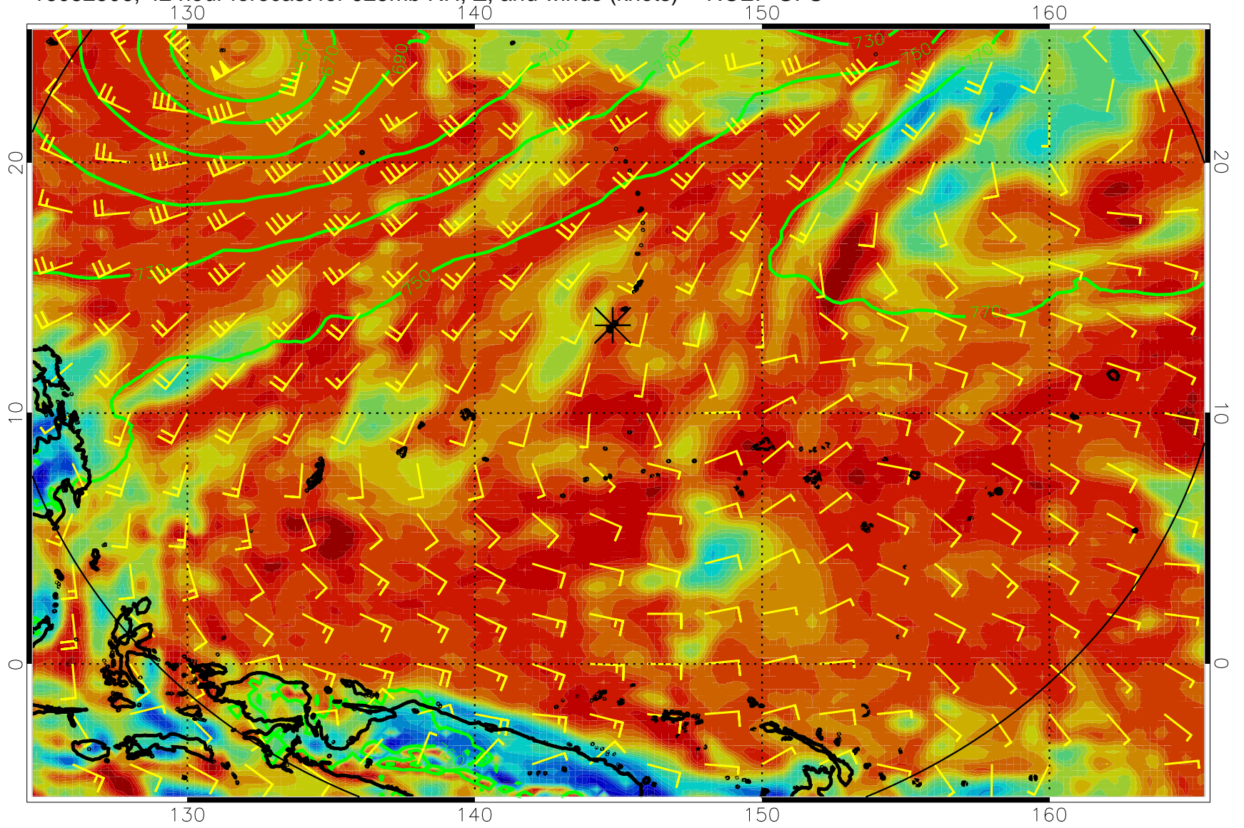
16082506, 42 hour forecast for 925mb RH, Z, and winds (knots) -- NCEP GFS
