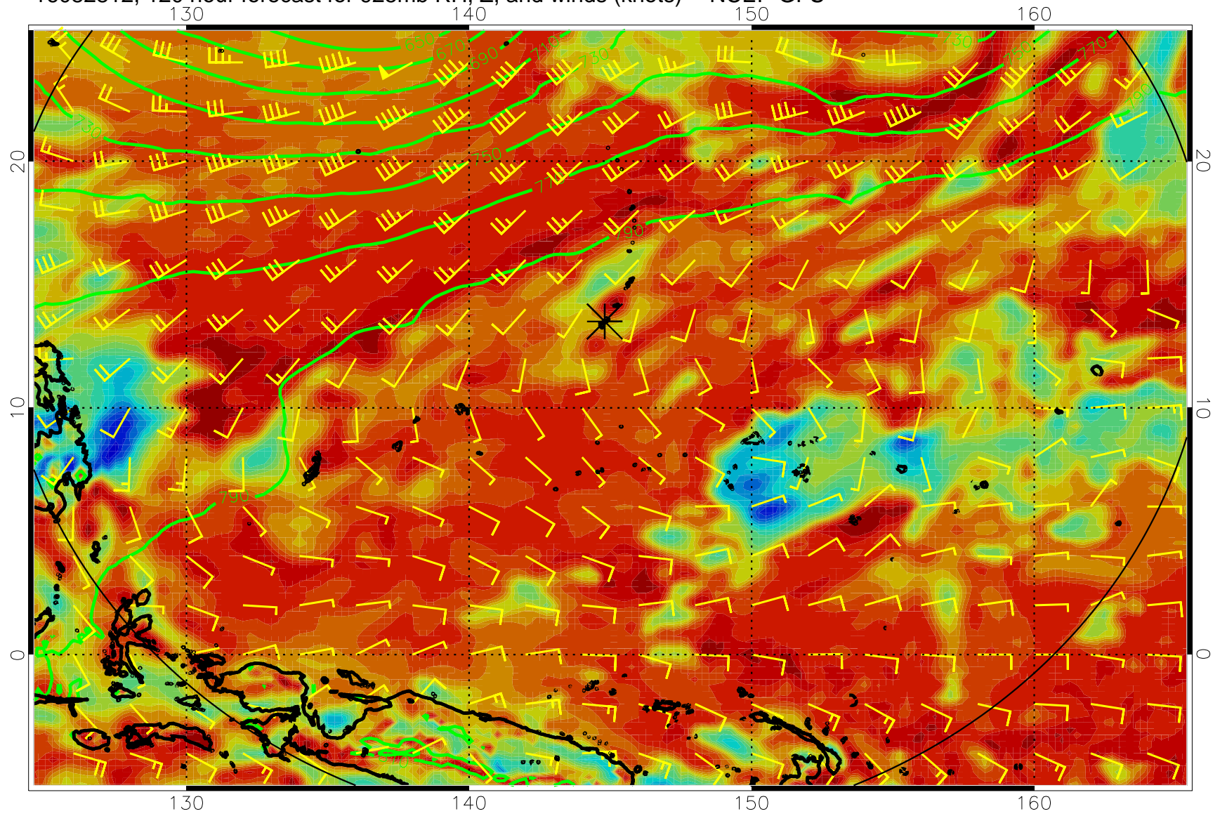
16082812, 120 hour forecast for 925mb RH, Z, and winds (knots) -- NCEP GFS
