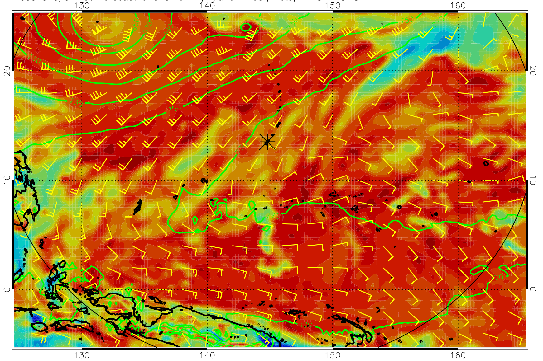
16082518, 54 hour forecast for 925mb RH, Z, and winds (knots) -- NCEP GFS
