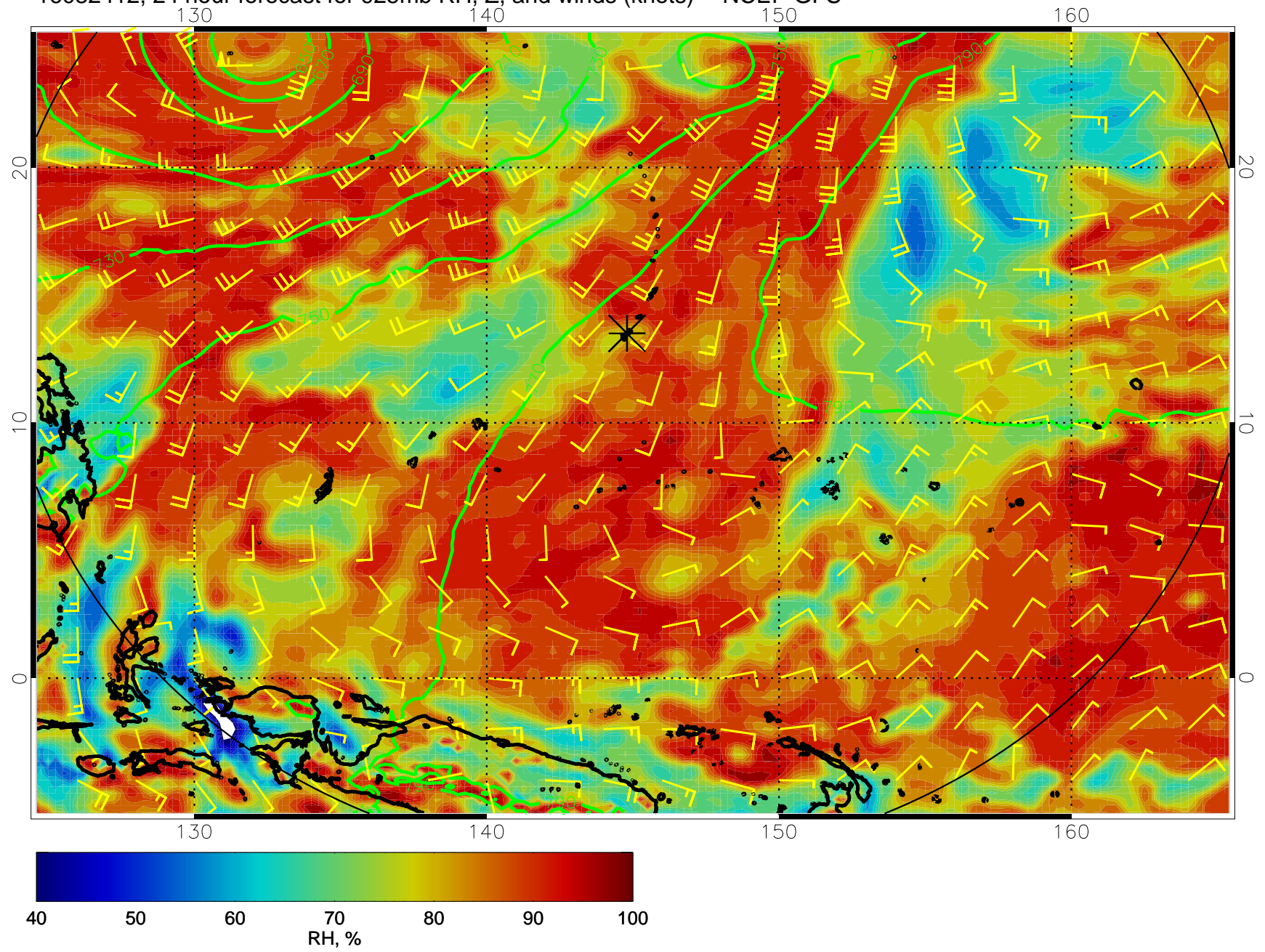
16082412, 24 hour forecast for 925mb RH, Z, and winds (knots) -- NCEP GFS
