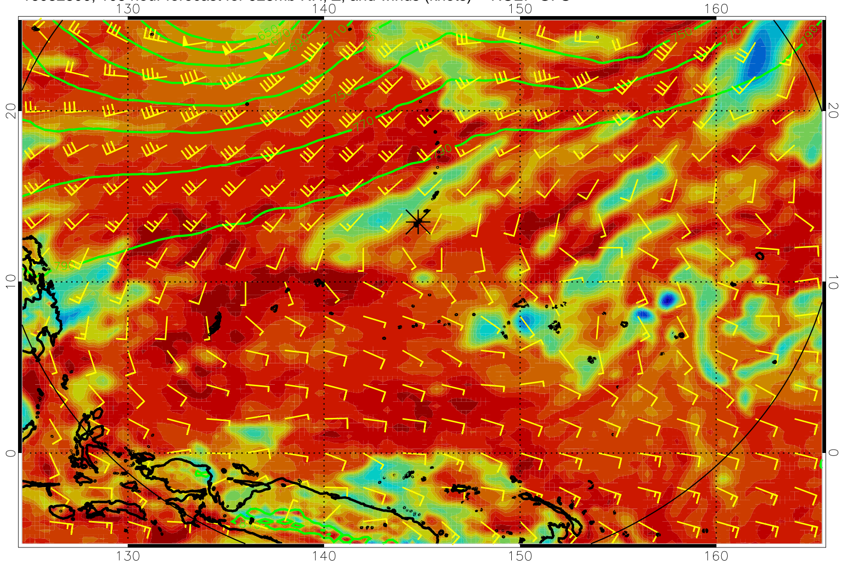
16082800, 108 hour forecast for 925mb RH, Z, and winds (knots) -- NCEP GFS
