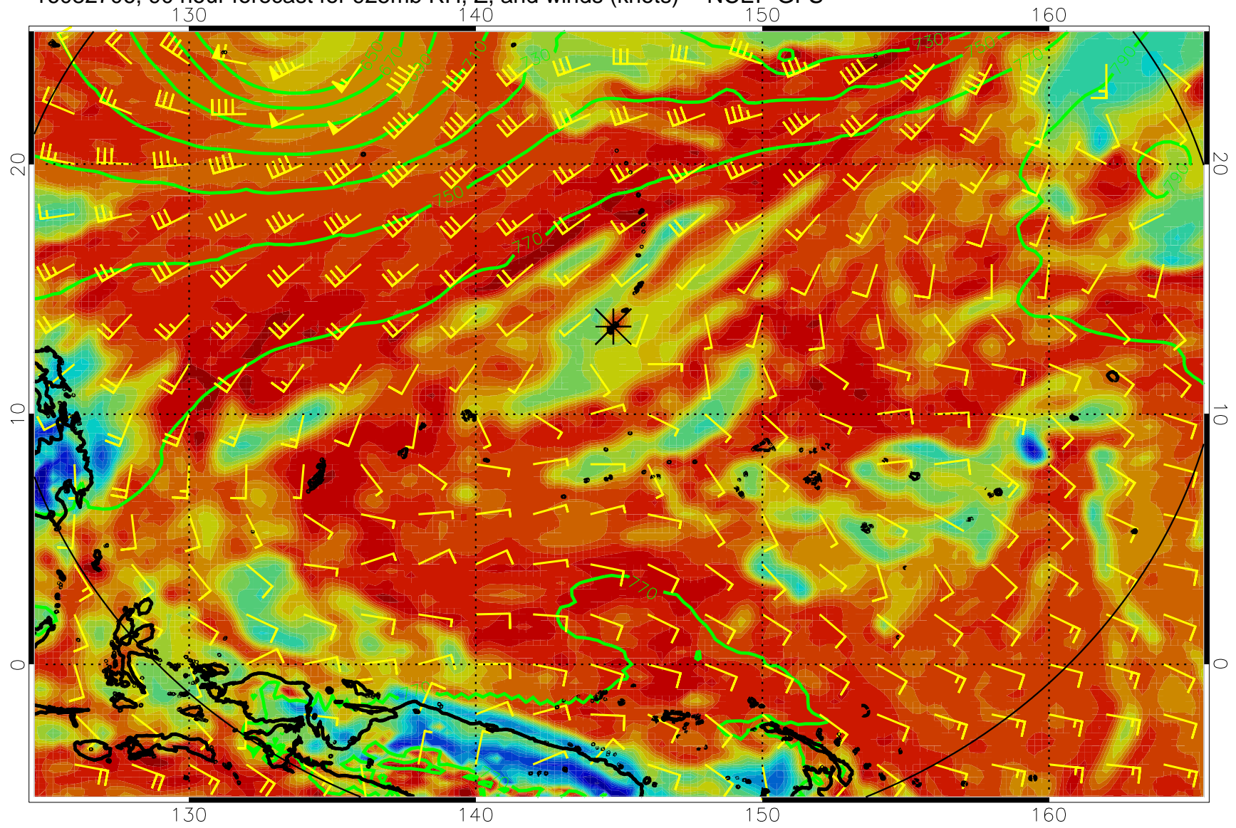
16082706, 90 hour forecast for 925mb RH, Z, and winds (knots) -- NCEP GFS
