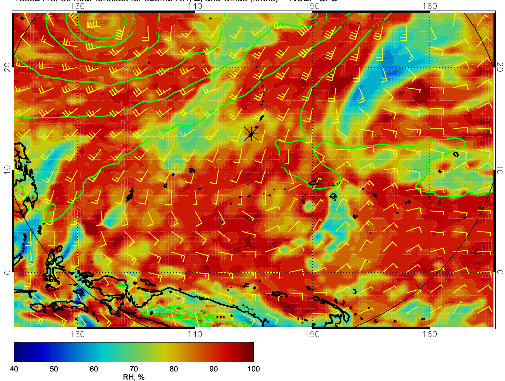
16082418, 30 hour forecast for 925mb RH, Z, and winds (knots) -- NCEP GFS
