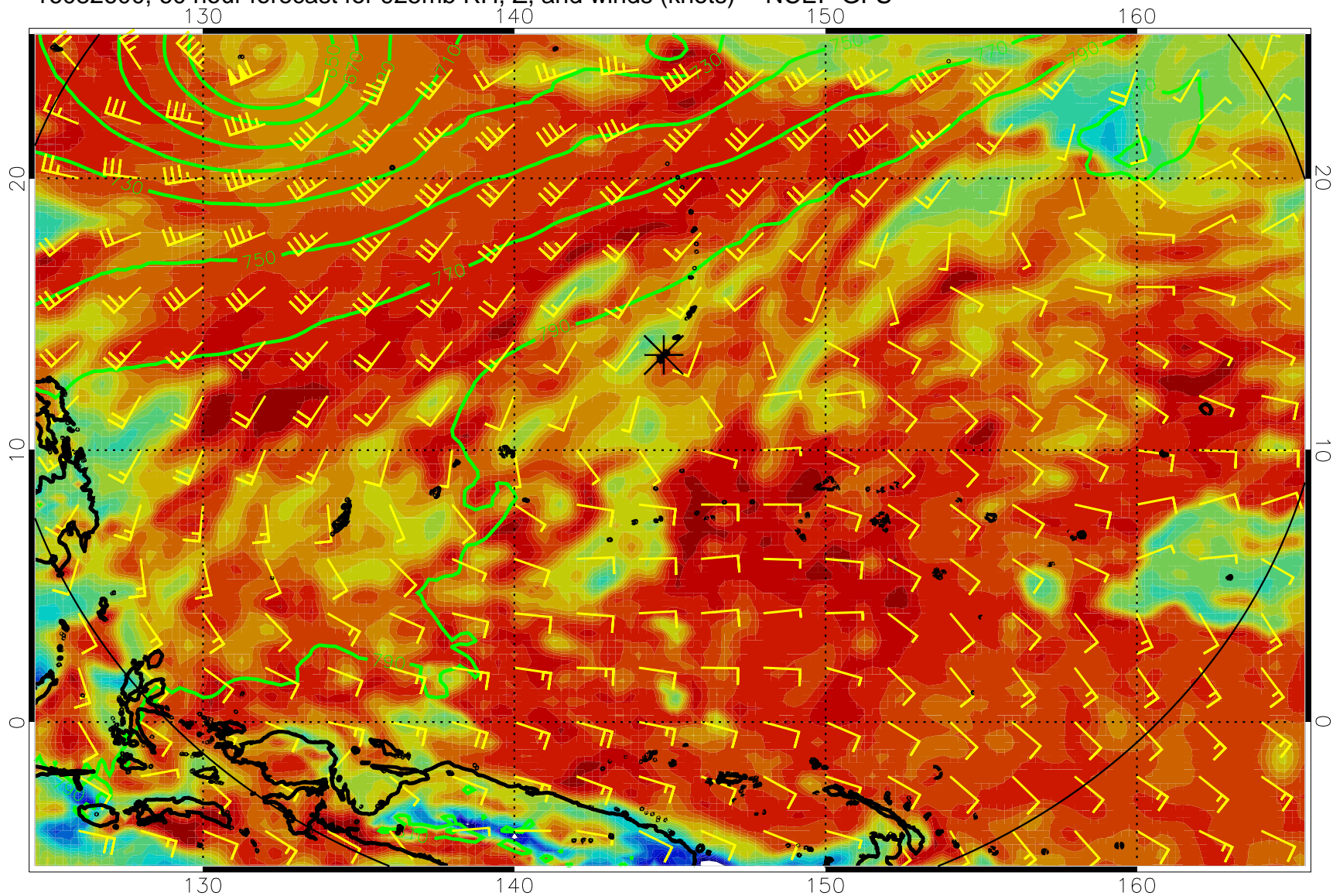
16082600, 60 hour forecast for 925mb RH, Z, and winds (knots) -- NCEP GFS
