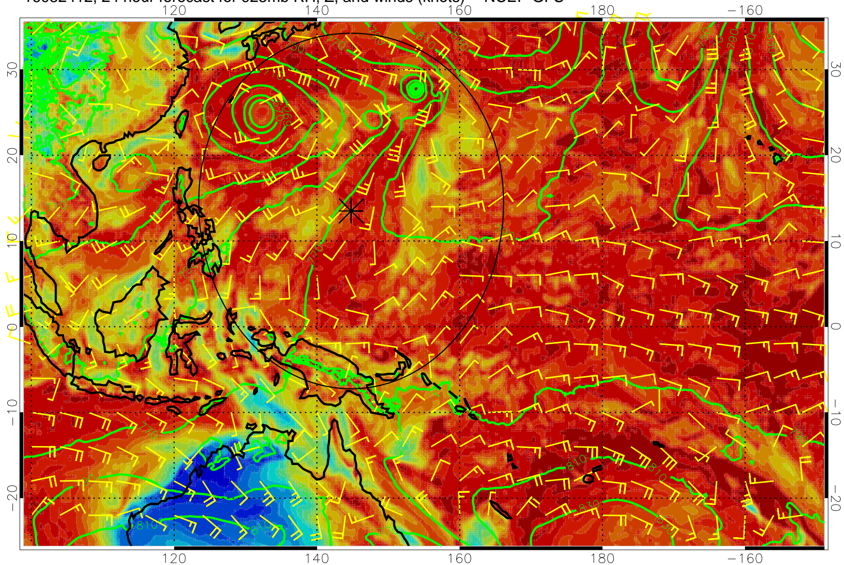
16082412, 24 hour forecast for 925mb RH, Z, and winds (knots) -- NCEP GFS
