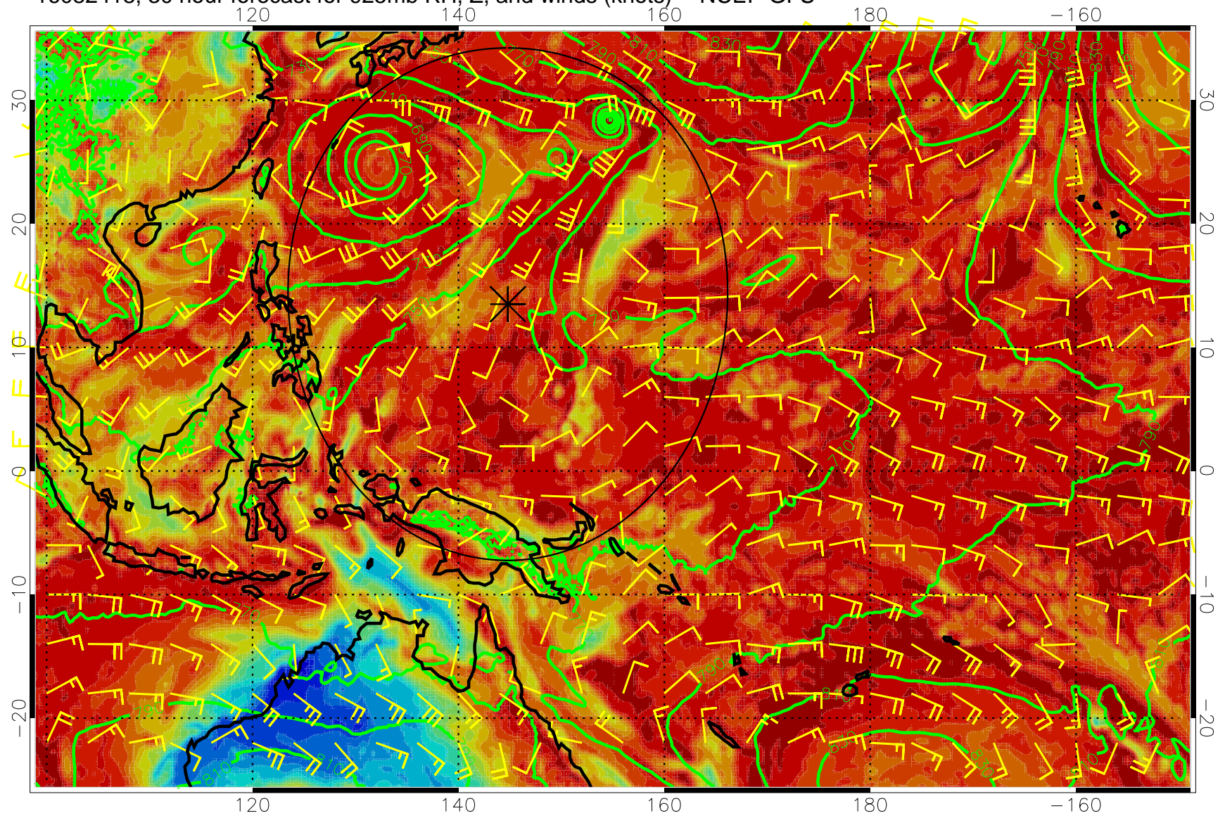
16082418, 30 hour forecast for 925mb RH, Z, and winds (knots) -- NCEP GFS
