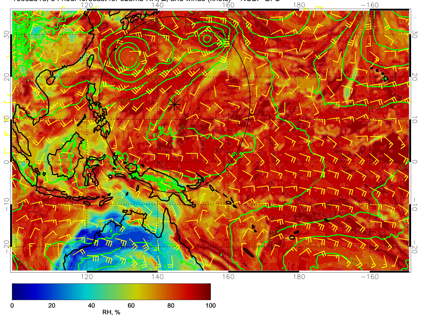
16082518, 54 hour forecast for 925mb RH, Z, and winds (knots) -- NCEP GFS
