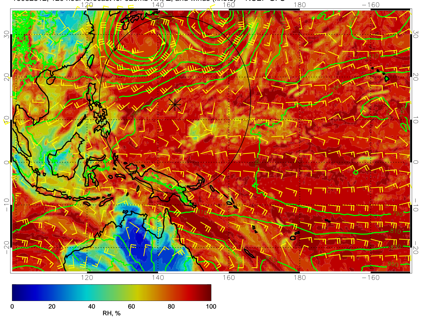
16082812, 120 hour forecast for 925mb RH, Z, and winds (knots) -- NCEP GFS
