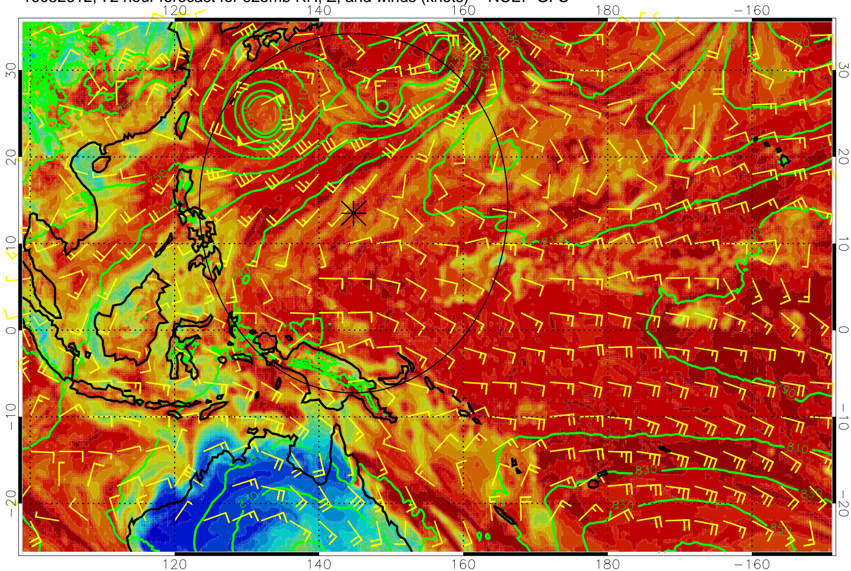
16082612, 72 hour forecast for 925mb RH, Z, and winds (knots) -- NCEP GFS
