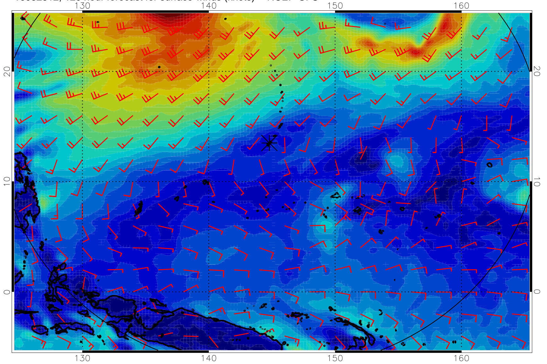
16082812, 120 hour forecast for surface winds (knots) -- NCEP GFS
