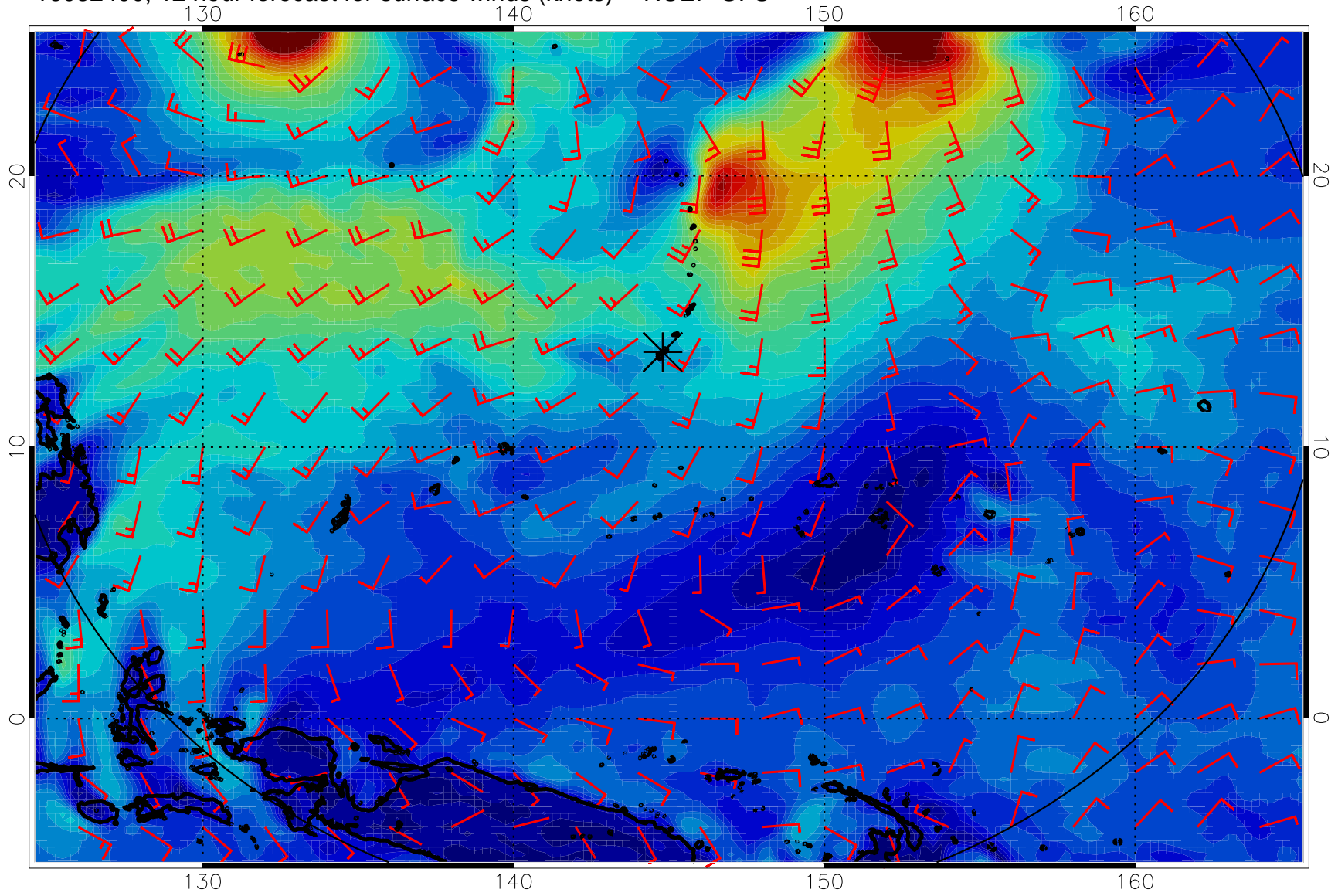
16082400, 12 hour forecast for surface winds (knots) -- NCEP GFS
