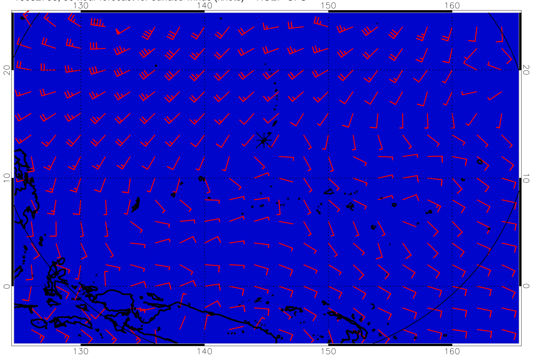
16082706, 90 hour forecast for surface winds (knots) -- NCEP GFS
