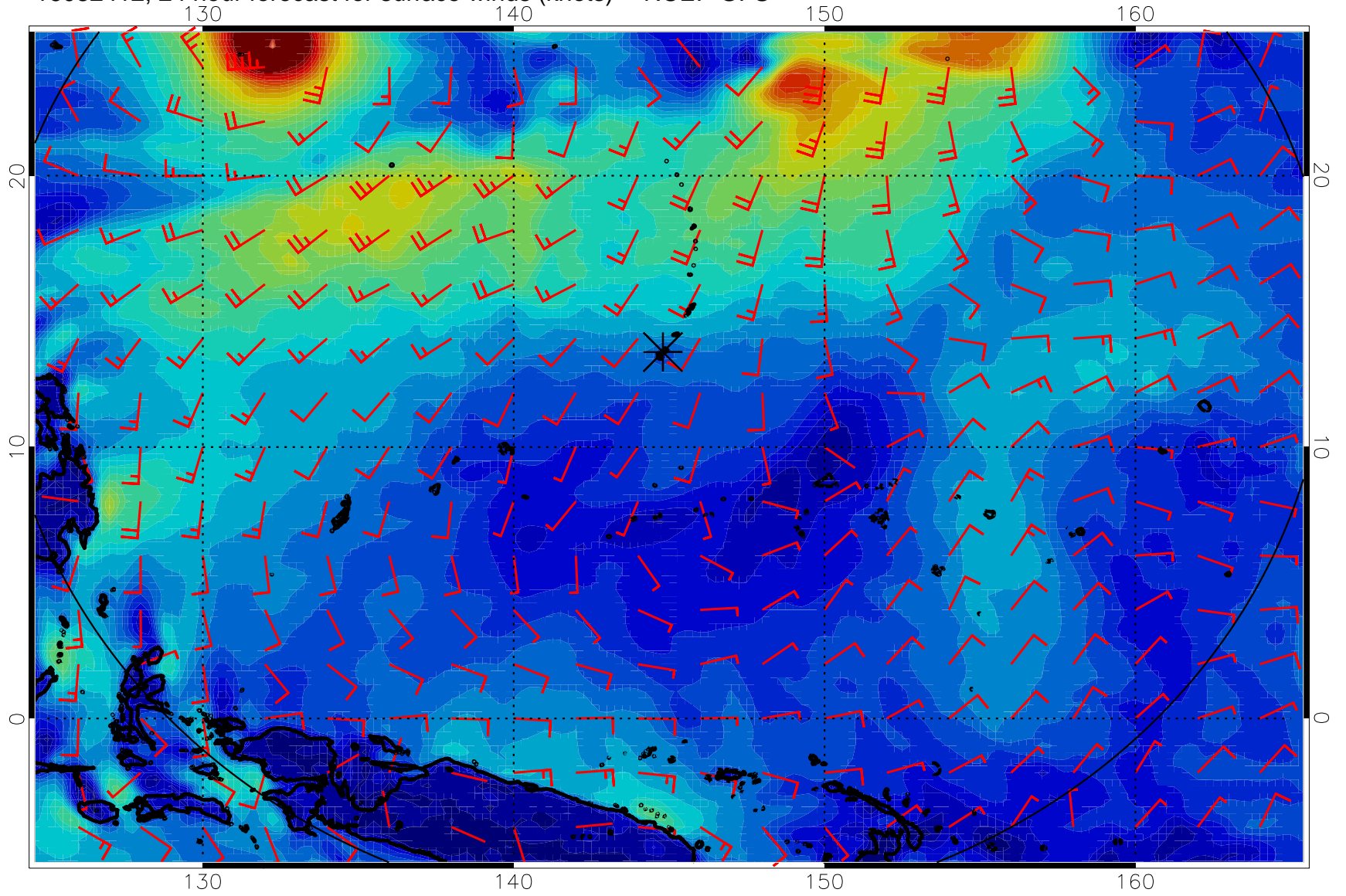
16082412, 24 hour forecast for surface winds (knots) -- NCEP GFS
