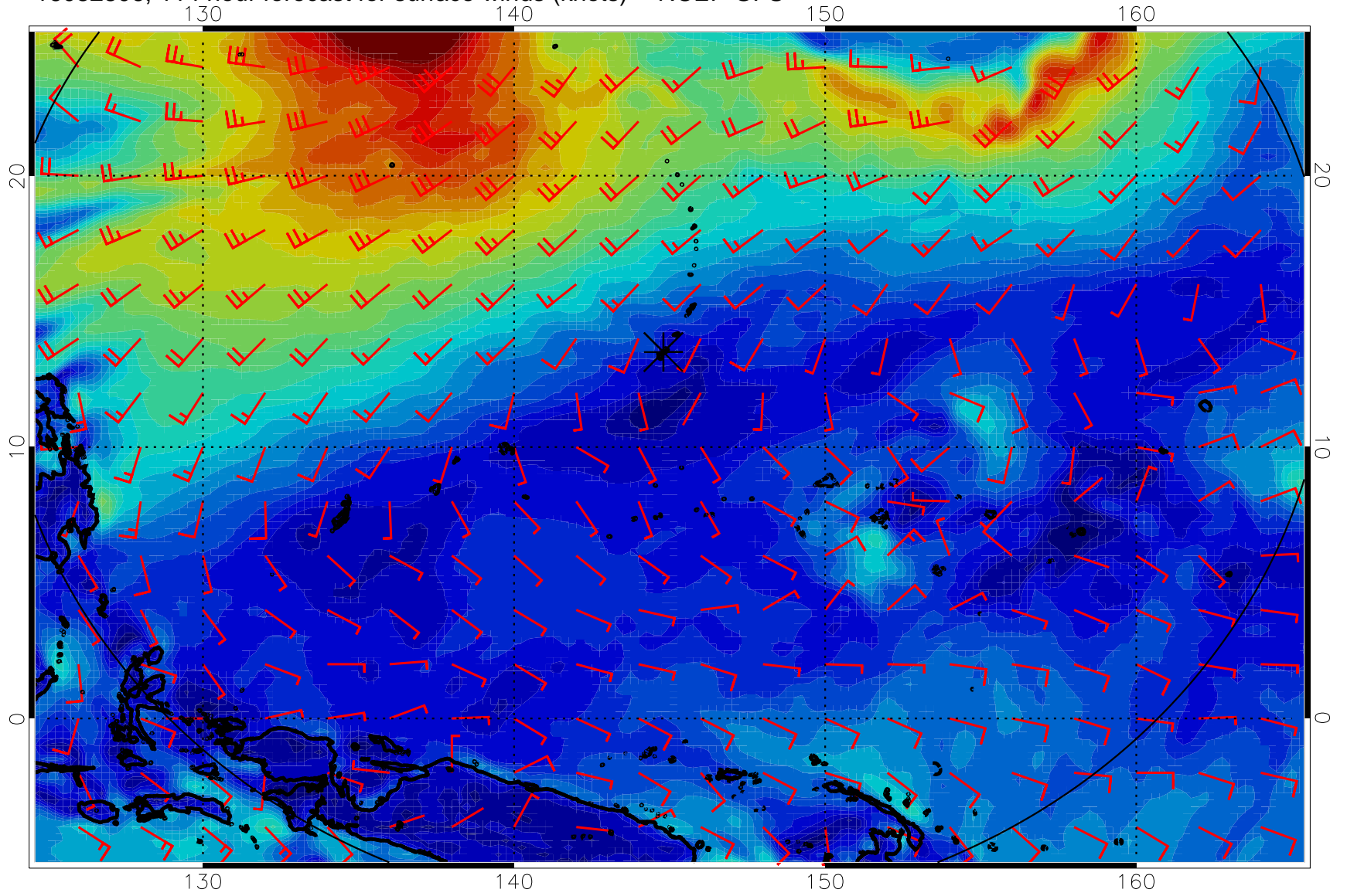
16082806, 114 hour forecast for surface winds (knots) -- NCEP GFS
