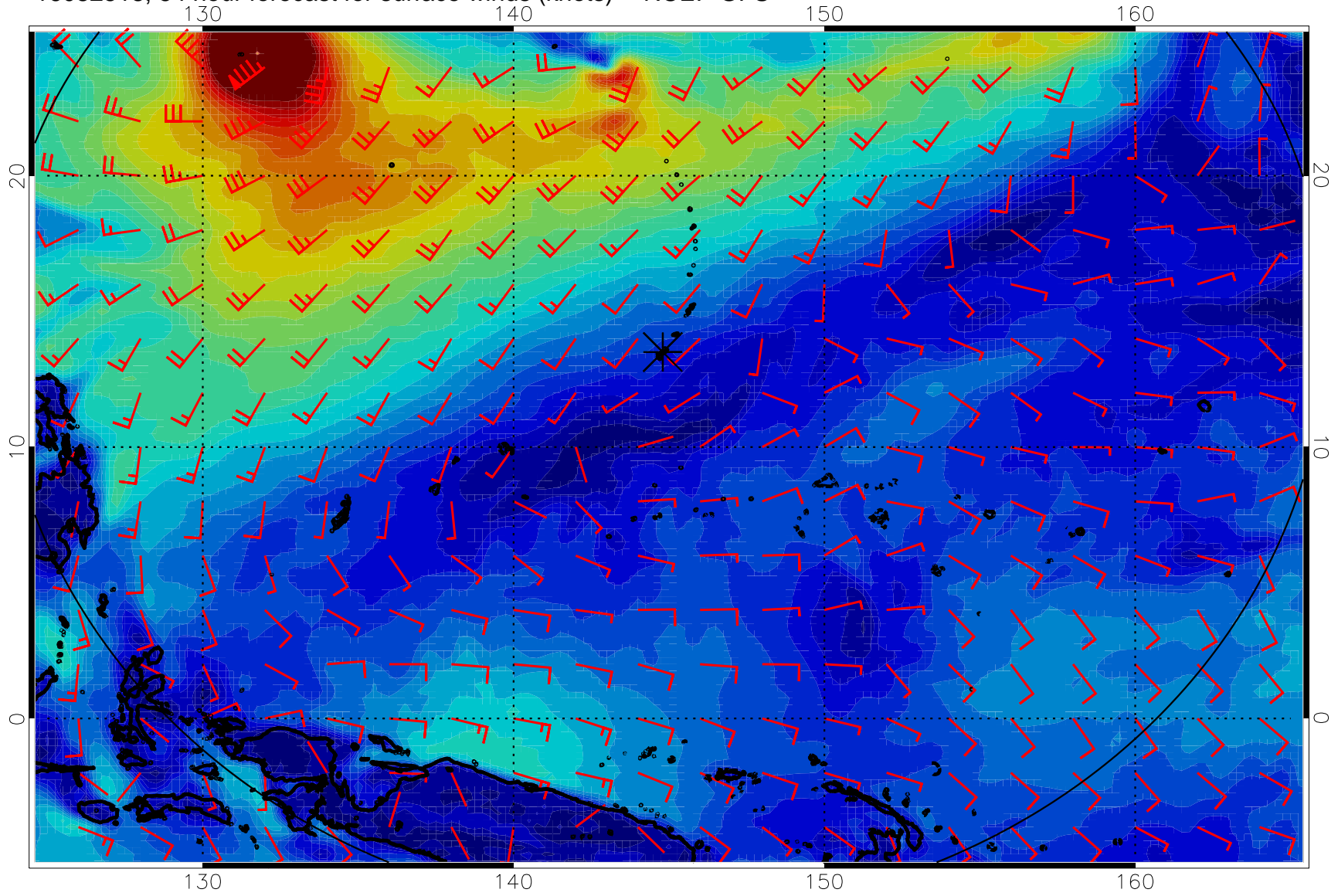
16082518, 54 hour forecast for surface winds (knots) -- NCEP GFS
