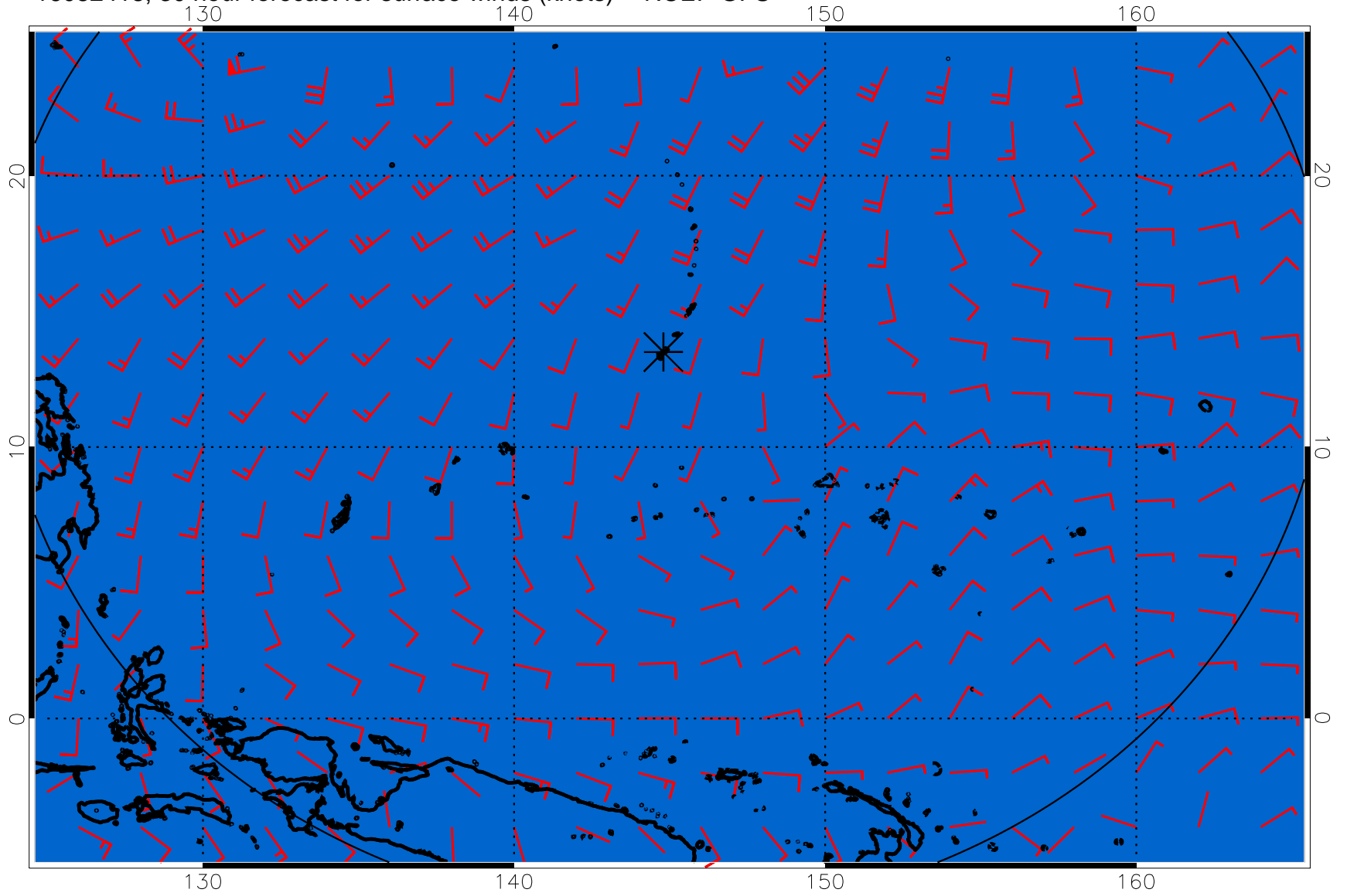
16082418, 30 hour forecast for surface winds (knots) -- NCEP GFS
