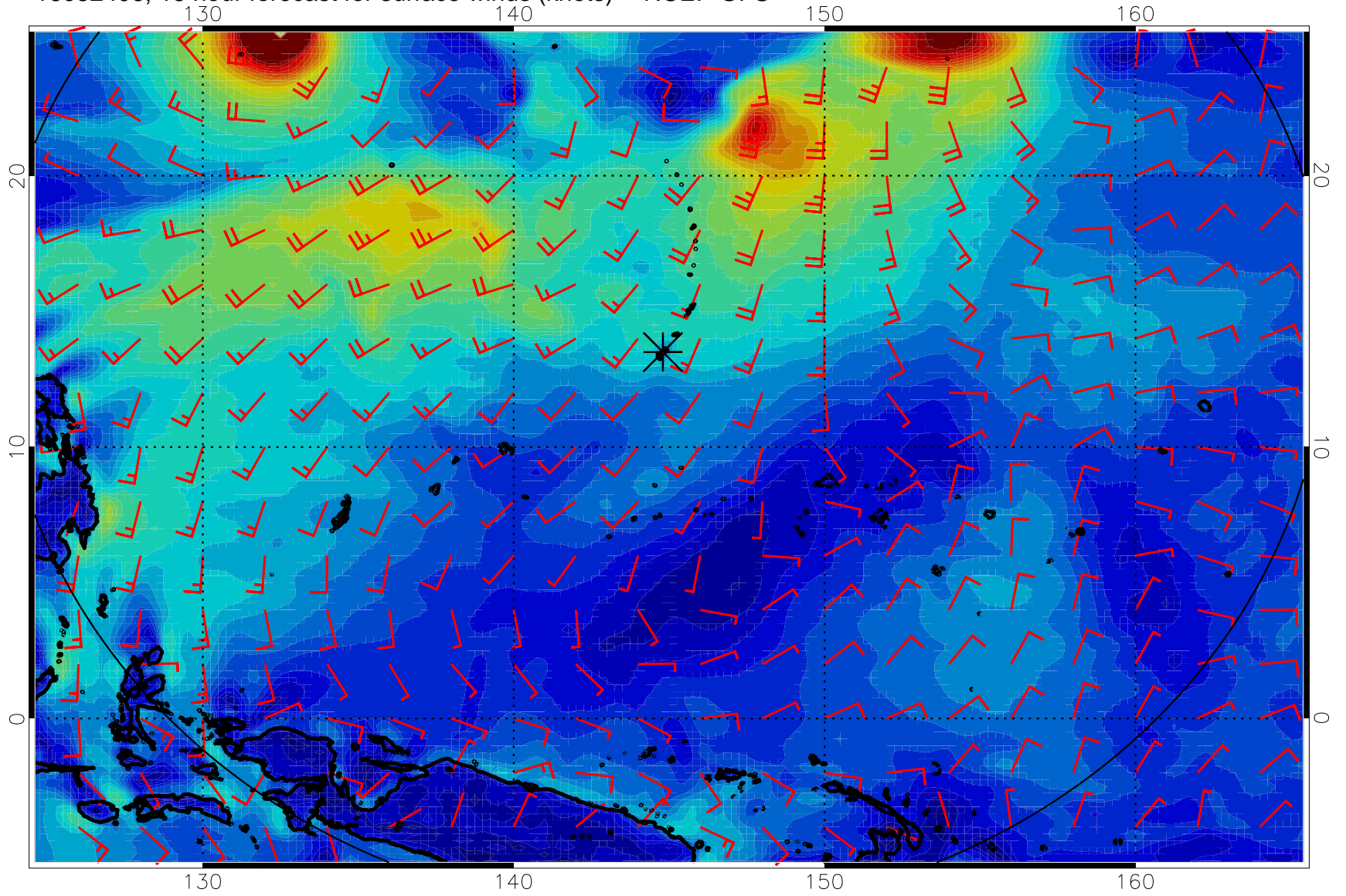
16082406, 18 hour forecast for surface winds (knots) -- NCEP GFS
