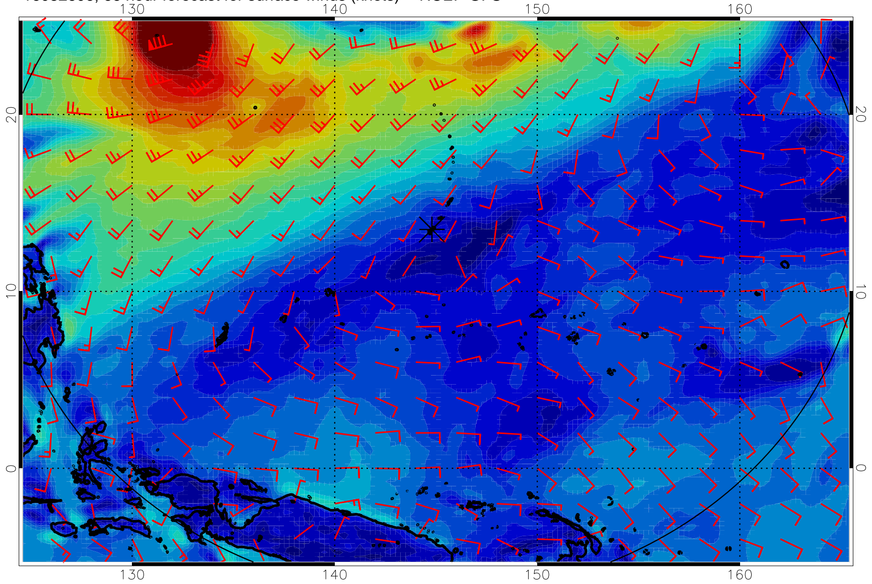
16082606, 66 hour forecast for surface winds (knots) -- NCEP GFS
