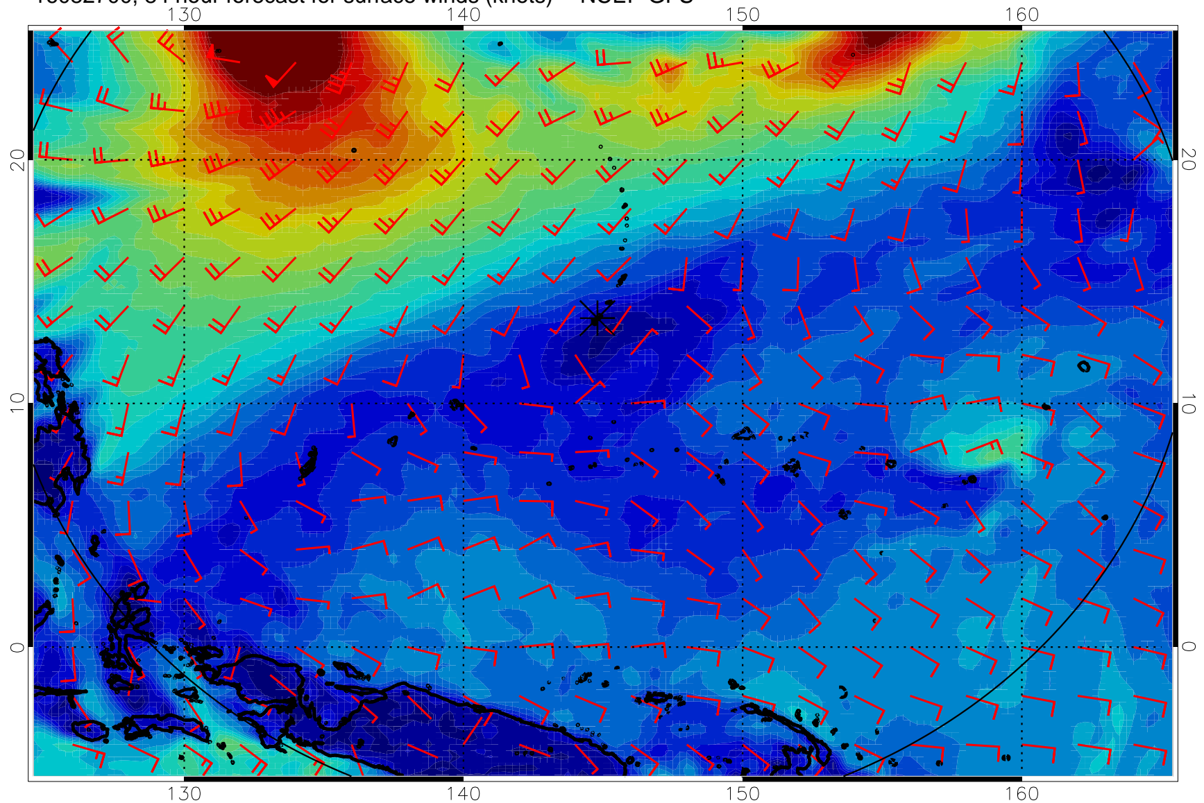
16082700, 84 hour forecast for surface winds (knots) -- NCEP GFS
