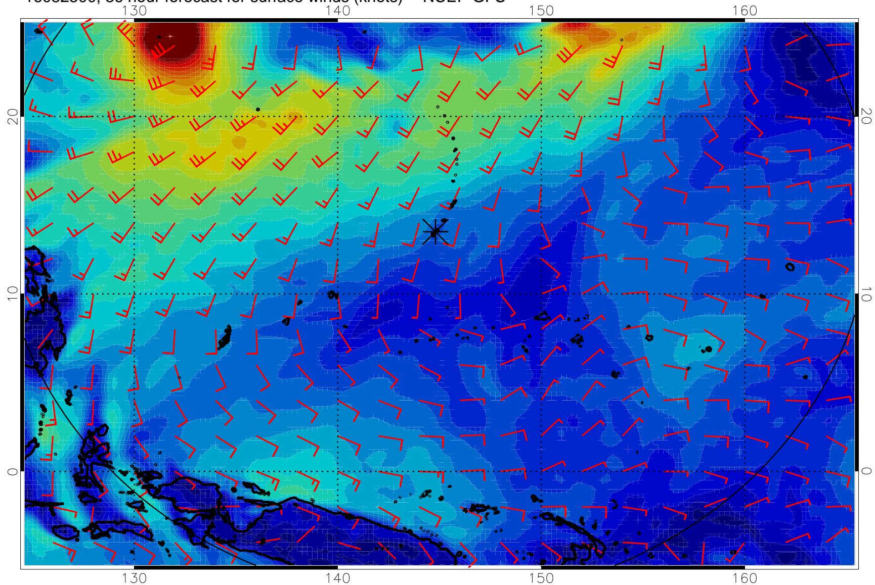
16082500, 36 hour forecast for surface winds (knots) -- NCEP GFS
