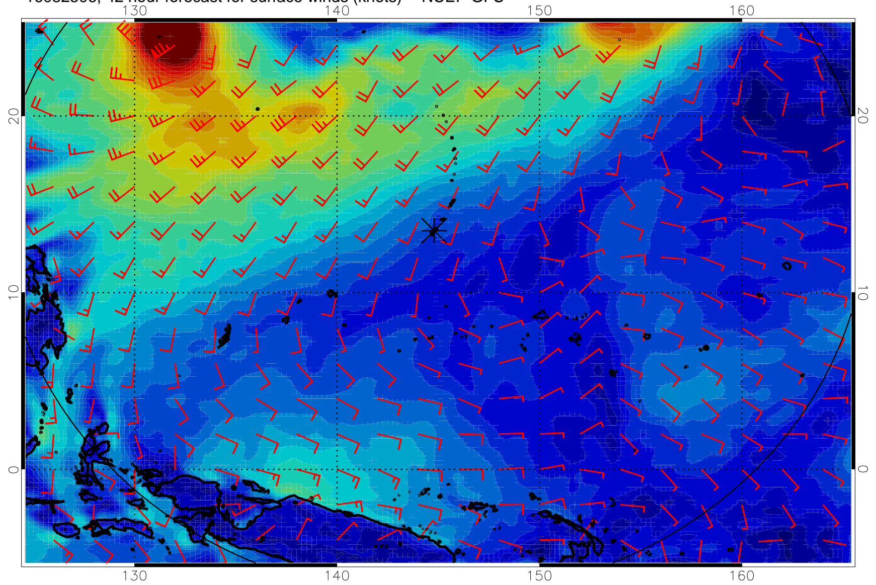
16082506, 42 hour forecast for surface winds (knots) -- NCEP GFS
