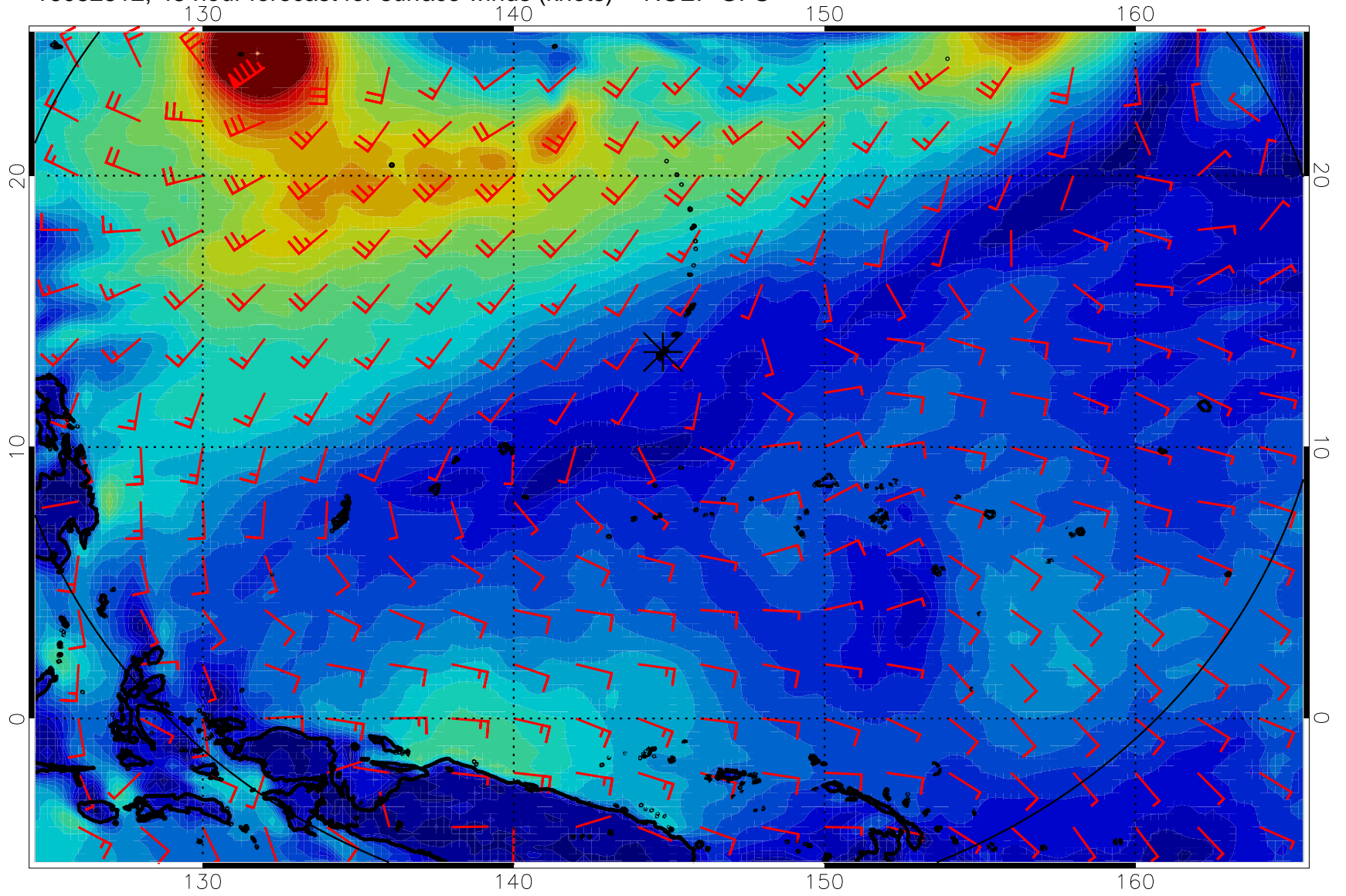
16082512, 48 hour forecast for surface winds (knots) -- NCEP GFS
