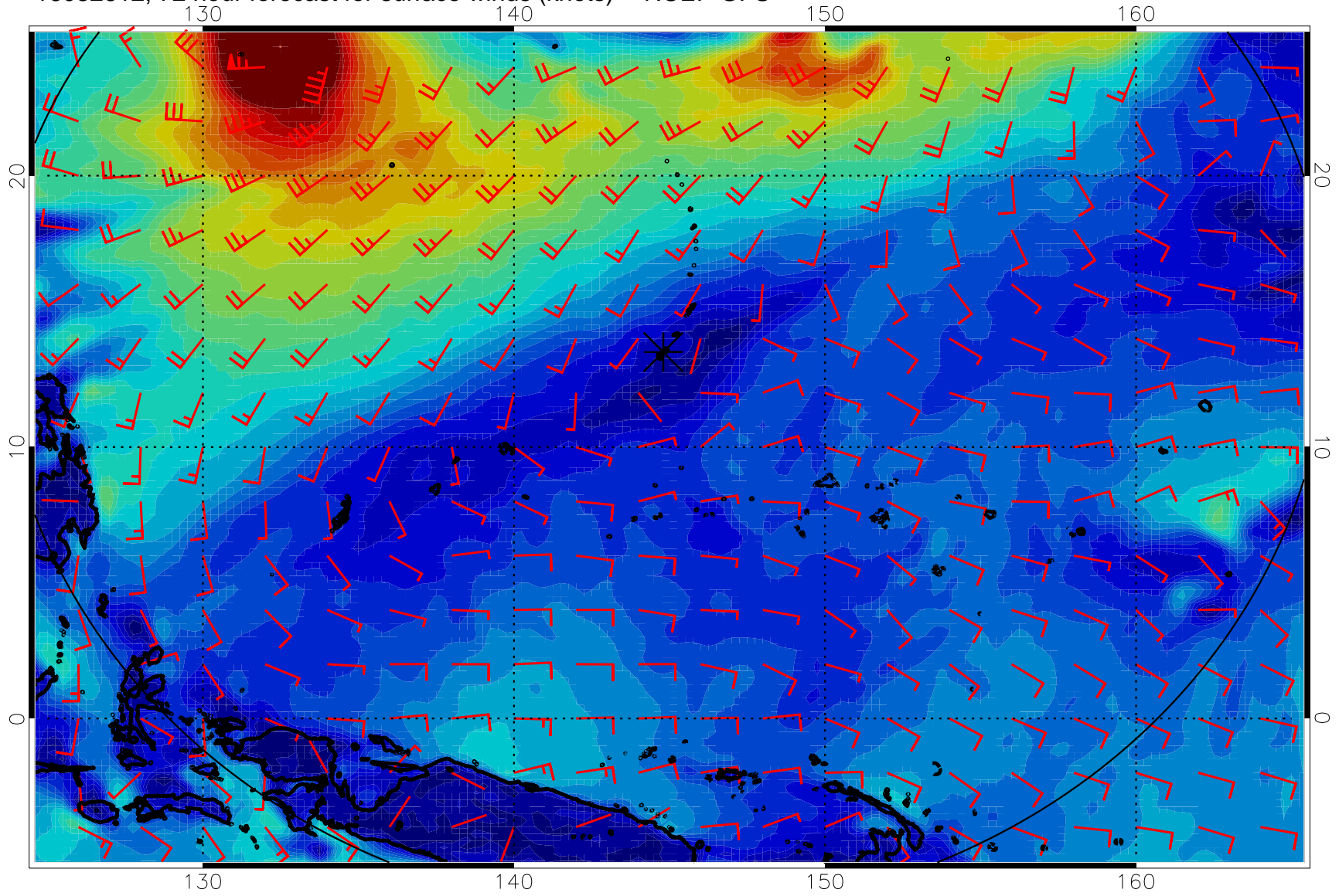
16082612, 72 hour forecast for surface winds (knots) -- NCEP GFS
