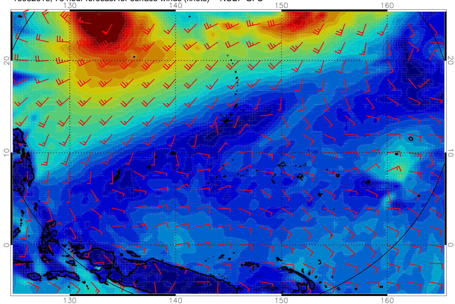
16082618, 78 hour forecast for surface winds (knots) -- NCEP GFS
