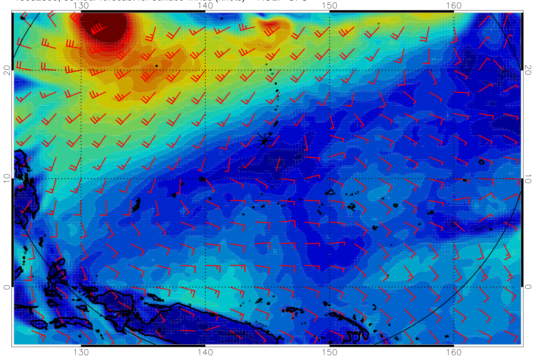
16082600, 60 hour forecast for surface winds (knots) -- NCEP GFS
