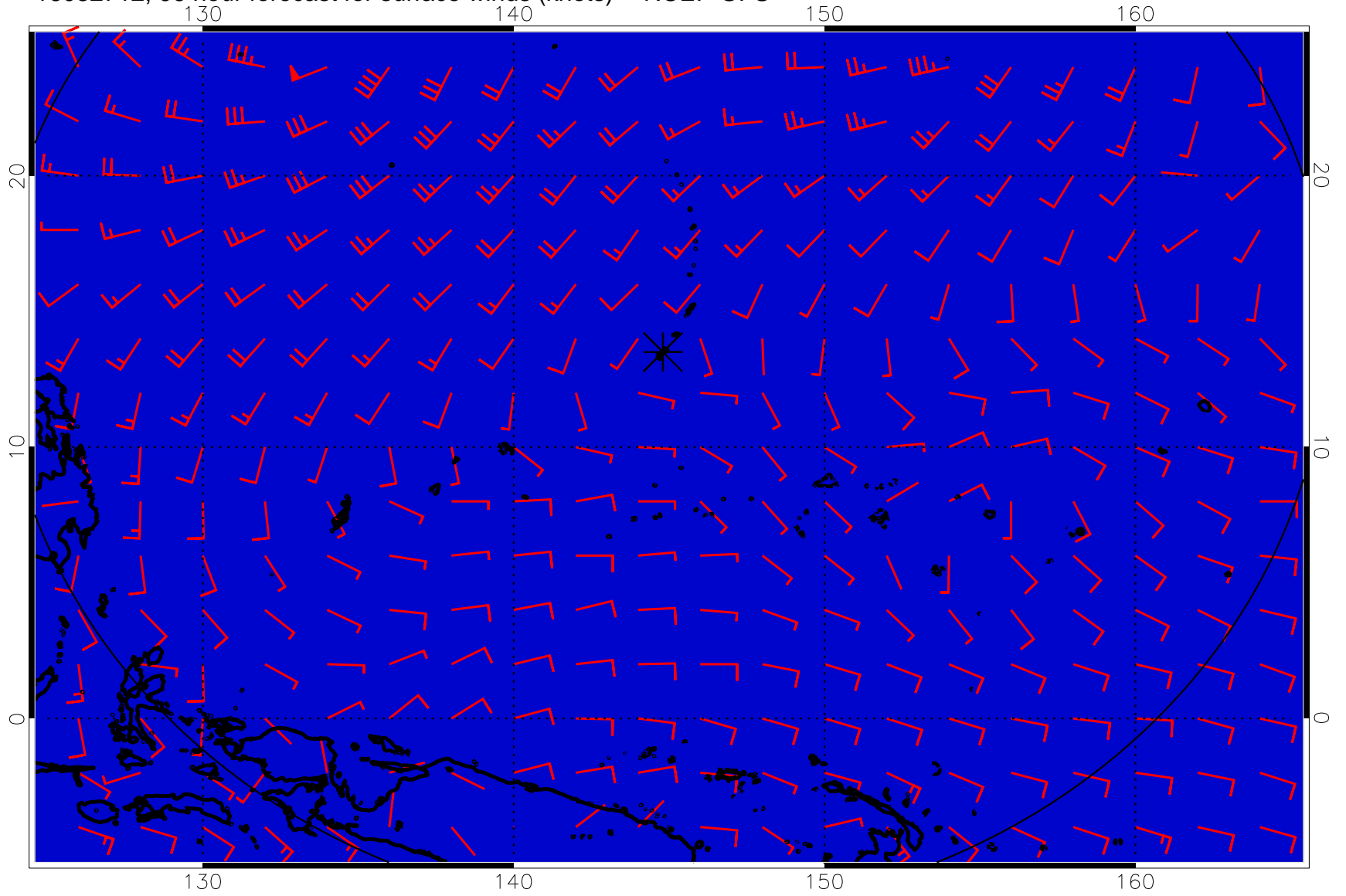
16082712, 96 hour forecast for surface winds (knots) -- NCEP GFS
