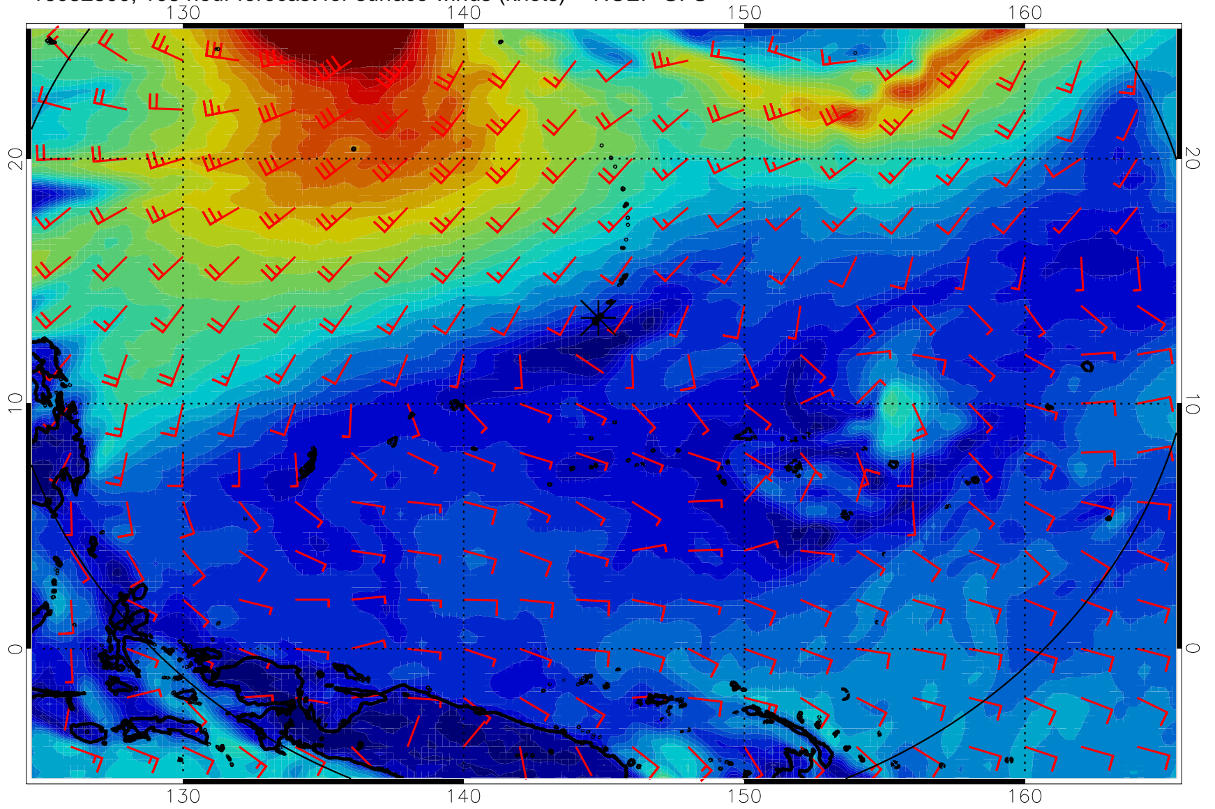
16082800, 108 hour forecast for surface winds (knots) -- NCEP GFS
