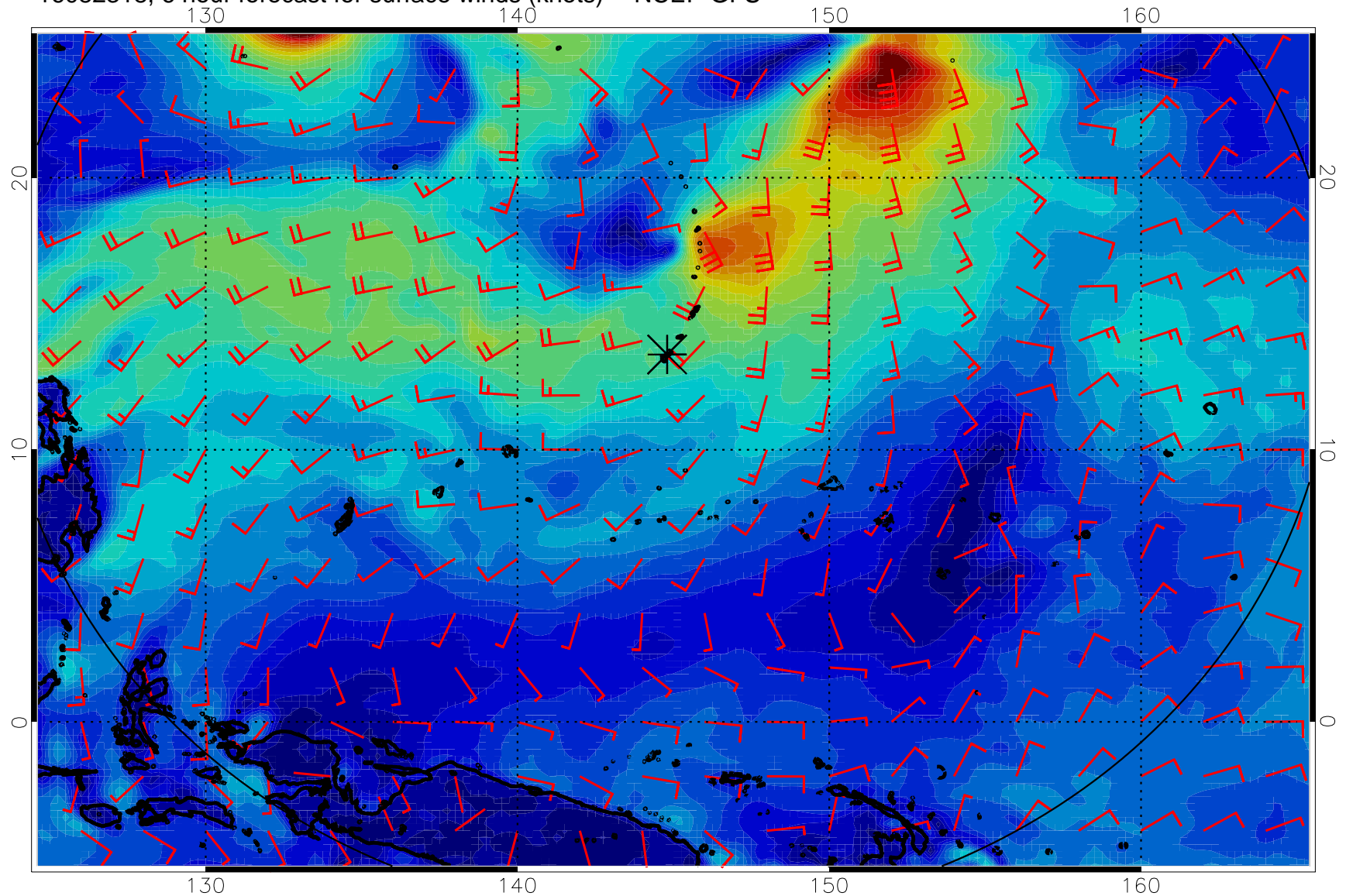
16082318, 6 hour forecast for surface winds (knots) -- NCEP GFS
