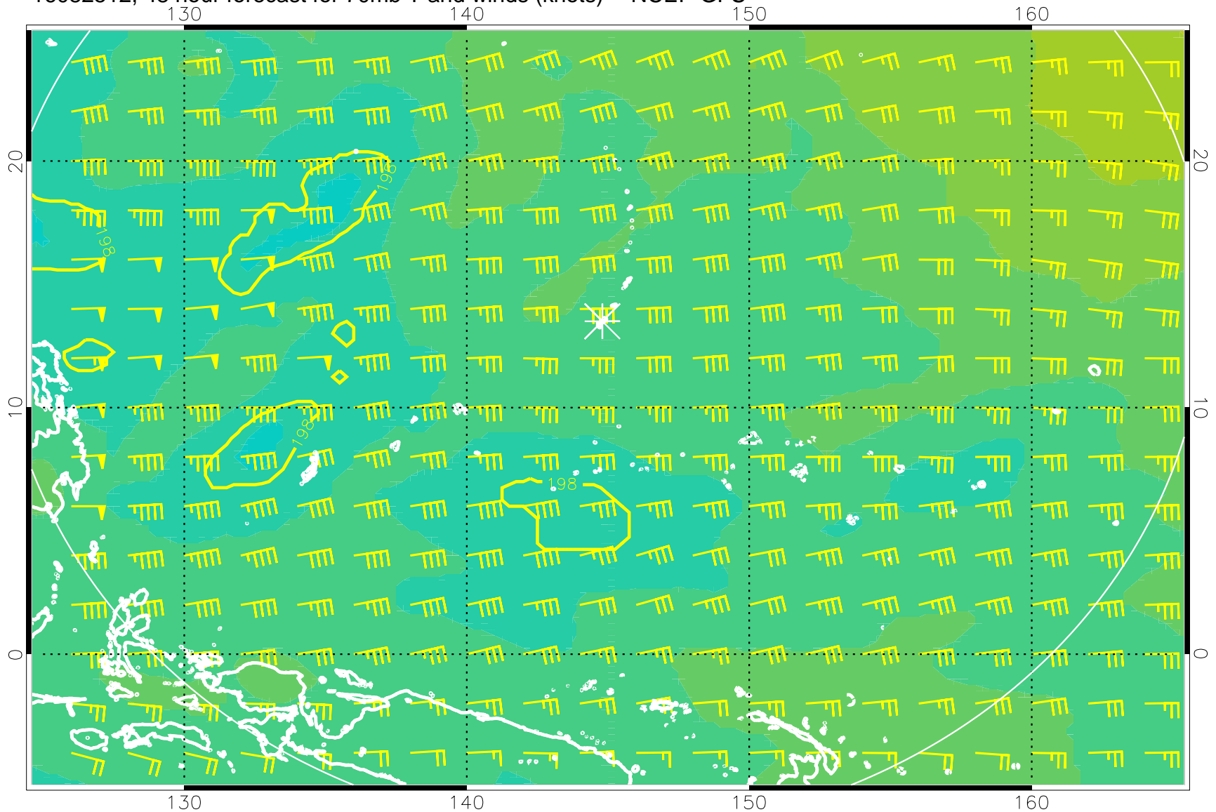
16082512, 48 hour forecast for 70mb T and winds (knots) -- NCEP GFS
