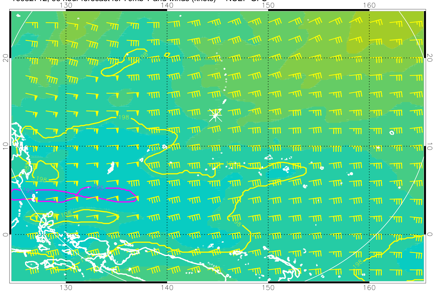
16082712, 96 hour forecast for 70mb T and winds (knots) -- NCEP GFS
