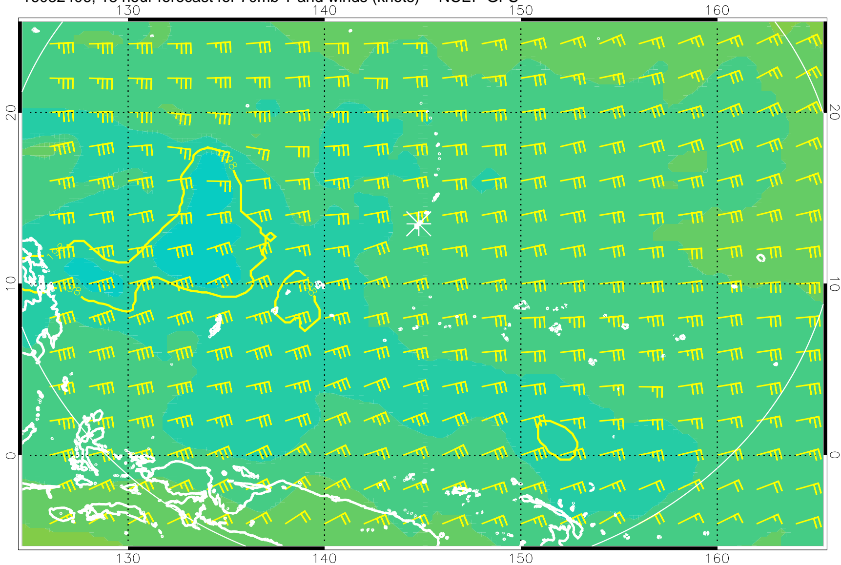
16082406, 18 hour forecast for 70mb T and winds (knots) -- NCEP GFS
