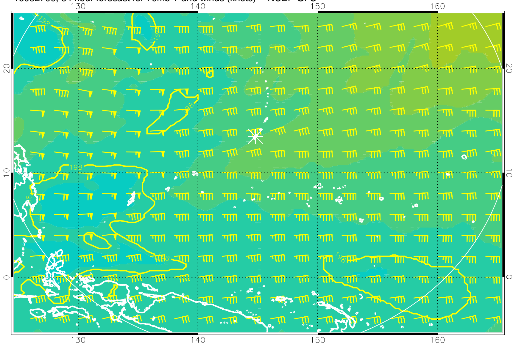
16082700, 84 hour forecast for 70mb T and winds (knots) -- NCEP GFS
