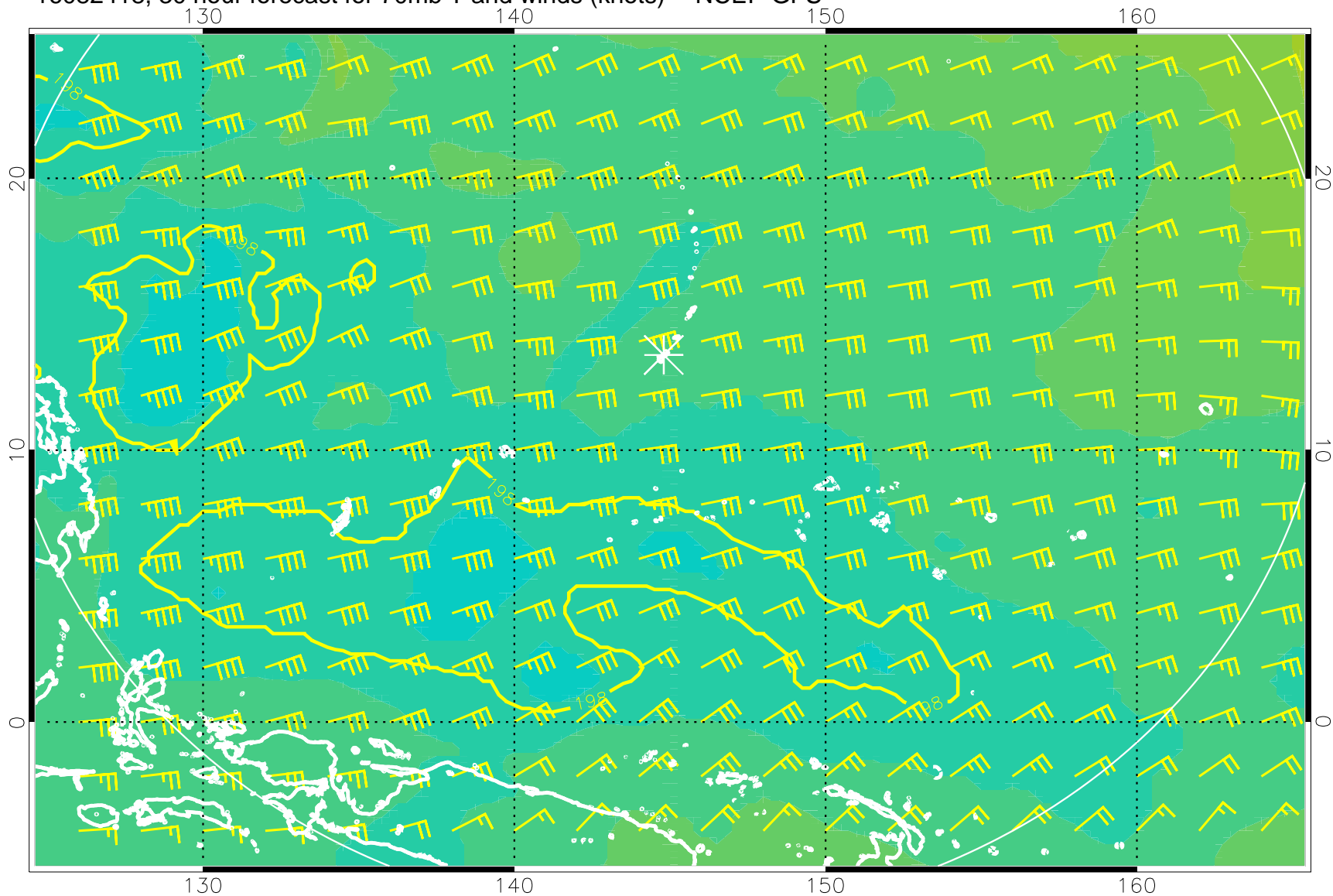
16082418, 30 hour forecast for 70mb T and winds (knots) -- NCEP GFS
