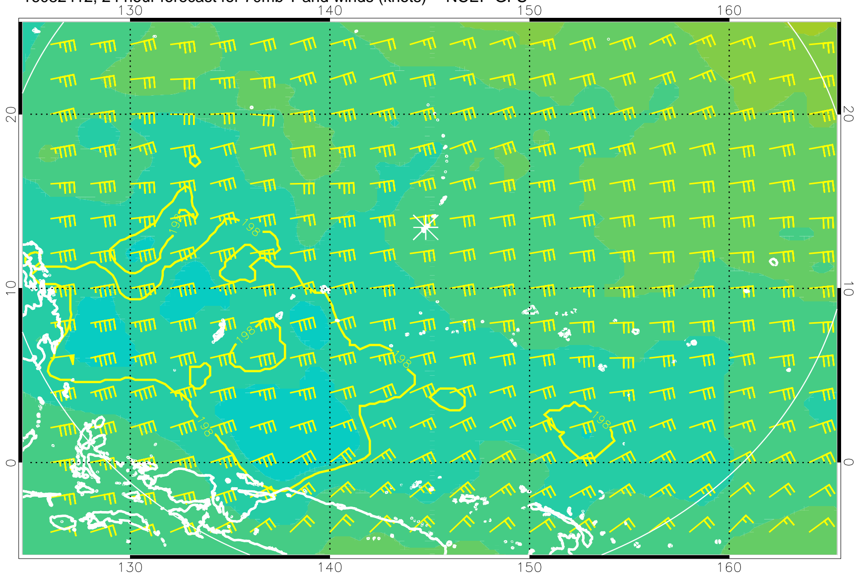
16082412, 24 hour forecast for 70mb T and winds (knots) -- NCEP GFS
