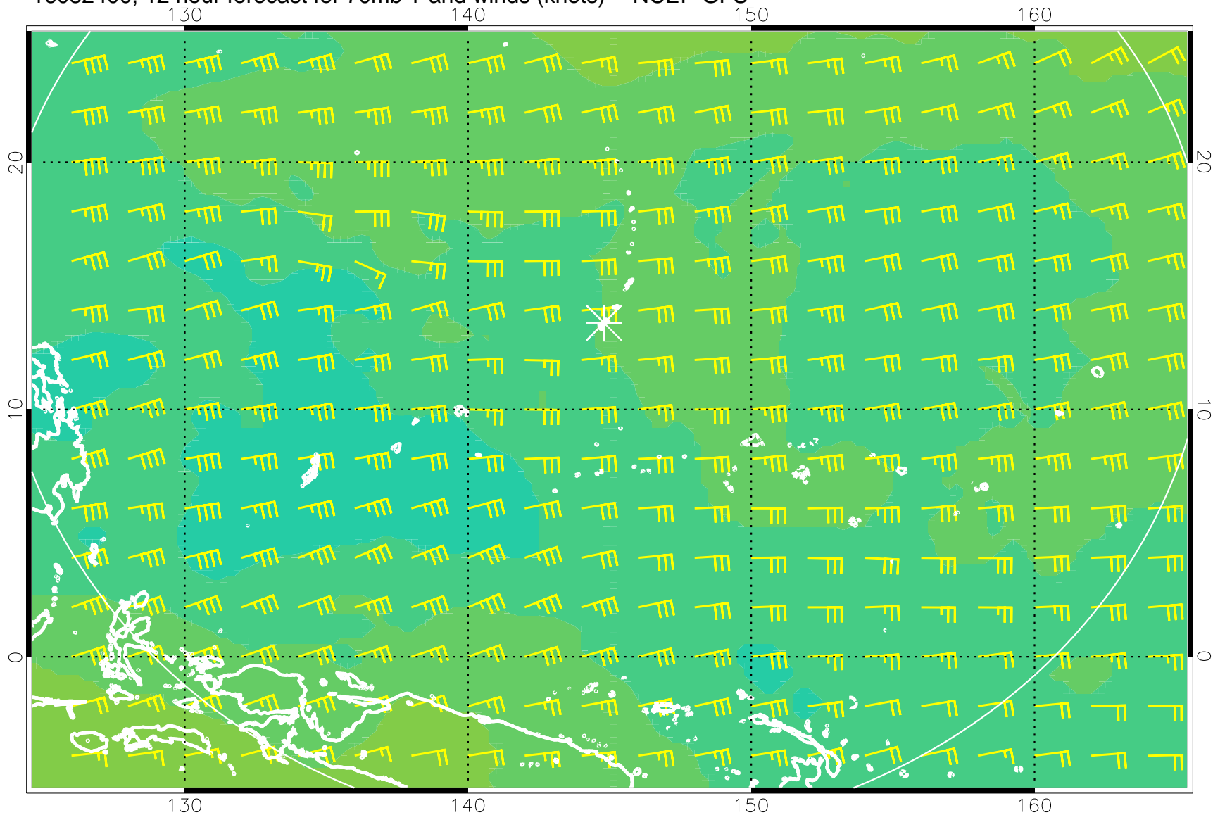
16082400, 12 hour forecast for 70mb T and winds (knots) -- NCEP GFS
