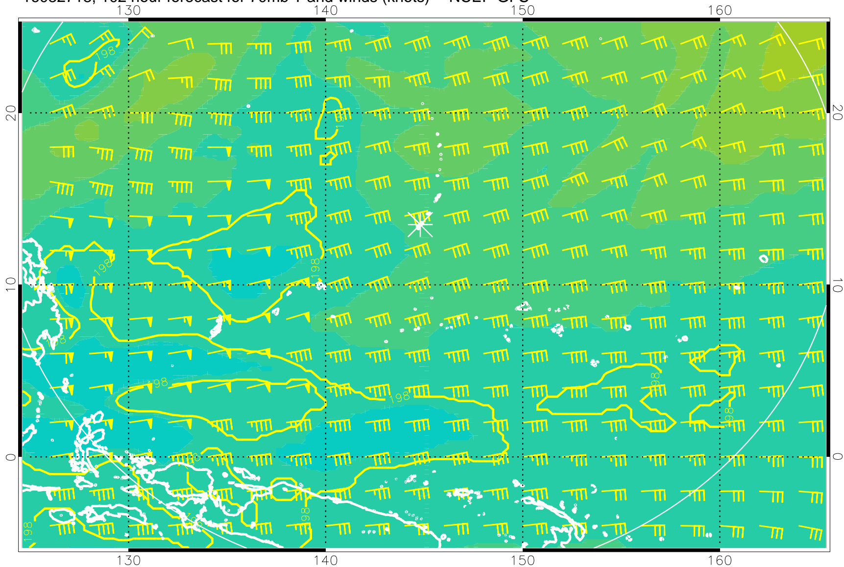
16082718, 102 hour forecast for 70mb T and winds (knots) -- NCEP GFS
