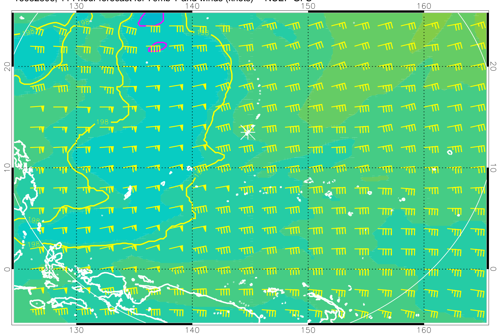
16082806, 114 hour forecast for 70mb T and winds (knots) -- NCEP GFS
