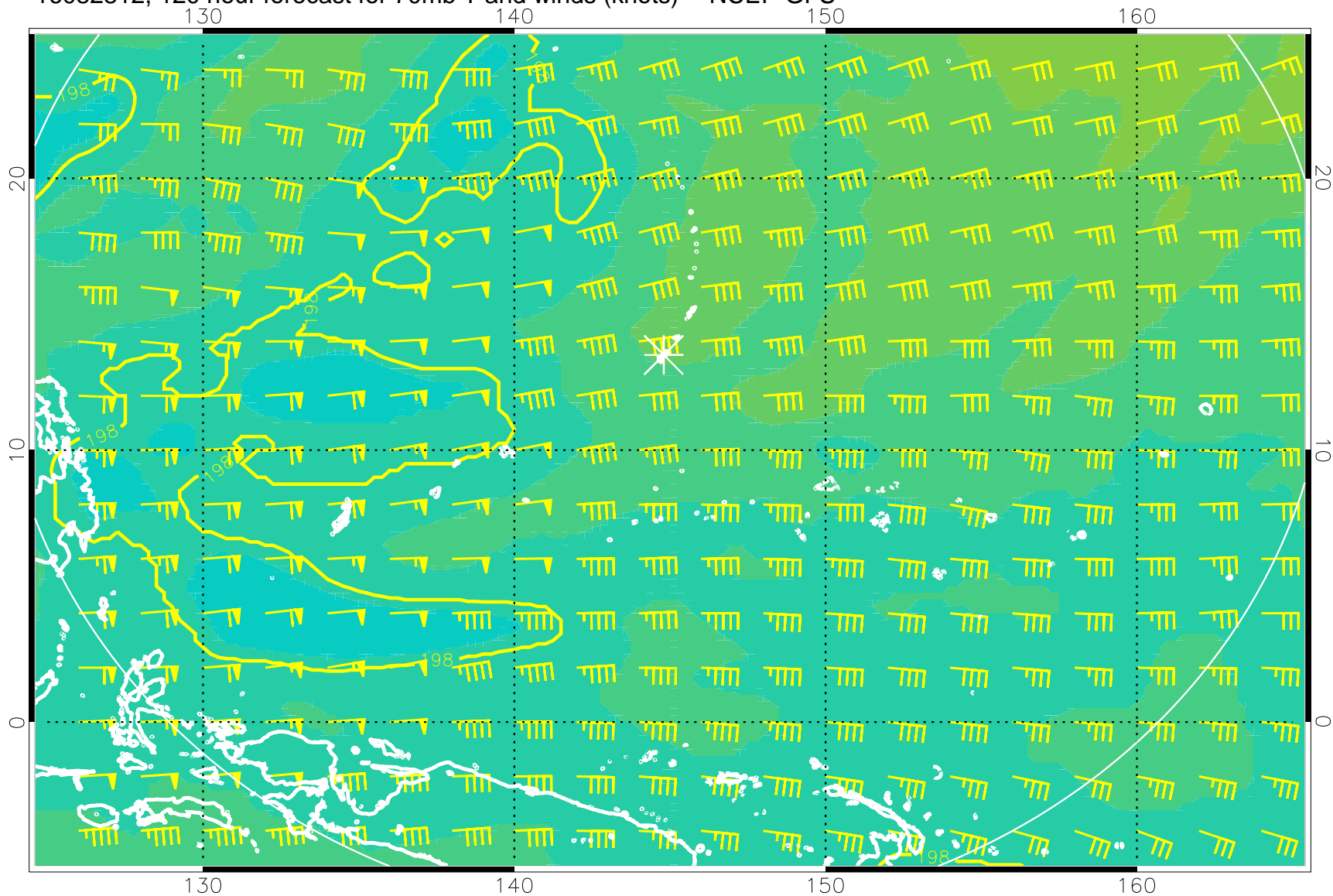
16082812, 120 hour forecast for 70mb T and winds (knots) -- NCEP GFS
