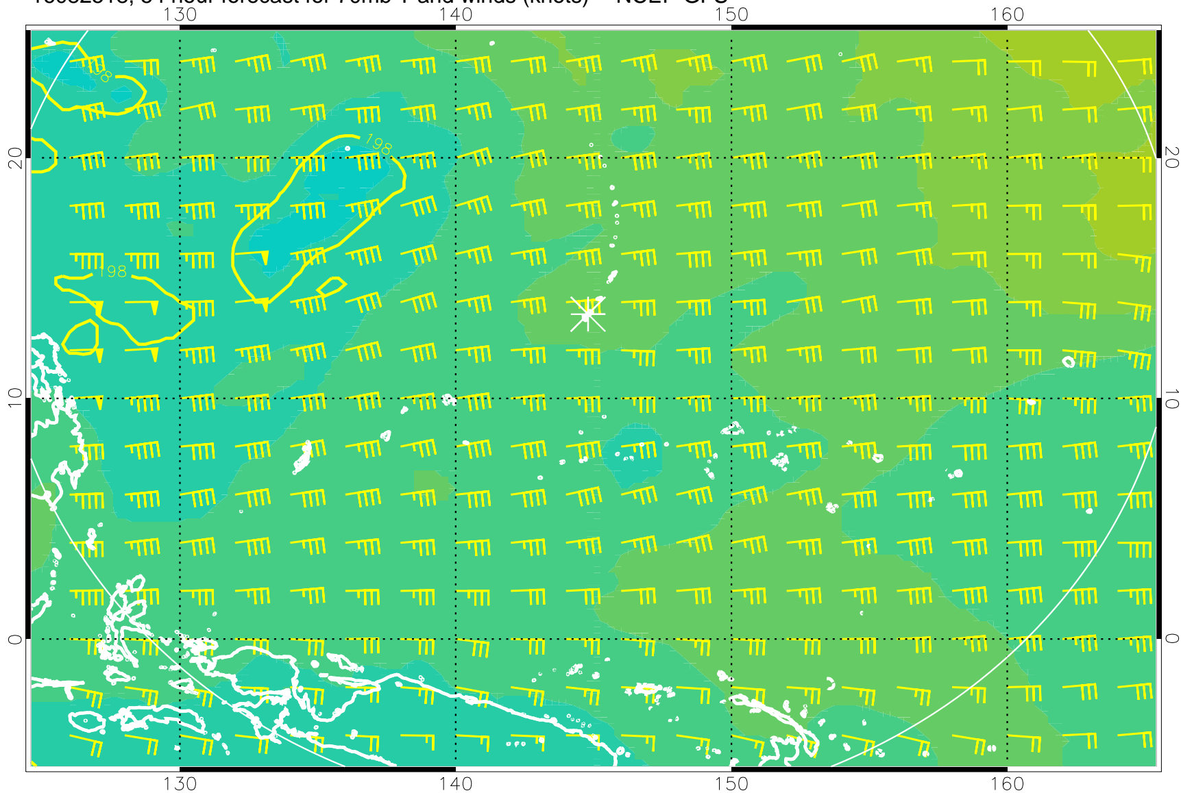
16082518, 54 hour forecast for 70mb T and winds (knots) -- NCEP GFS
