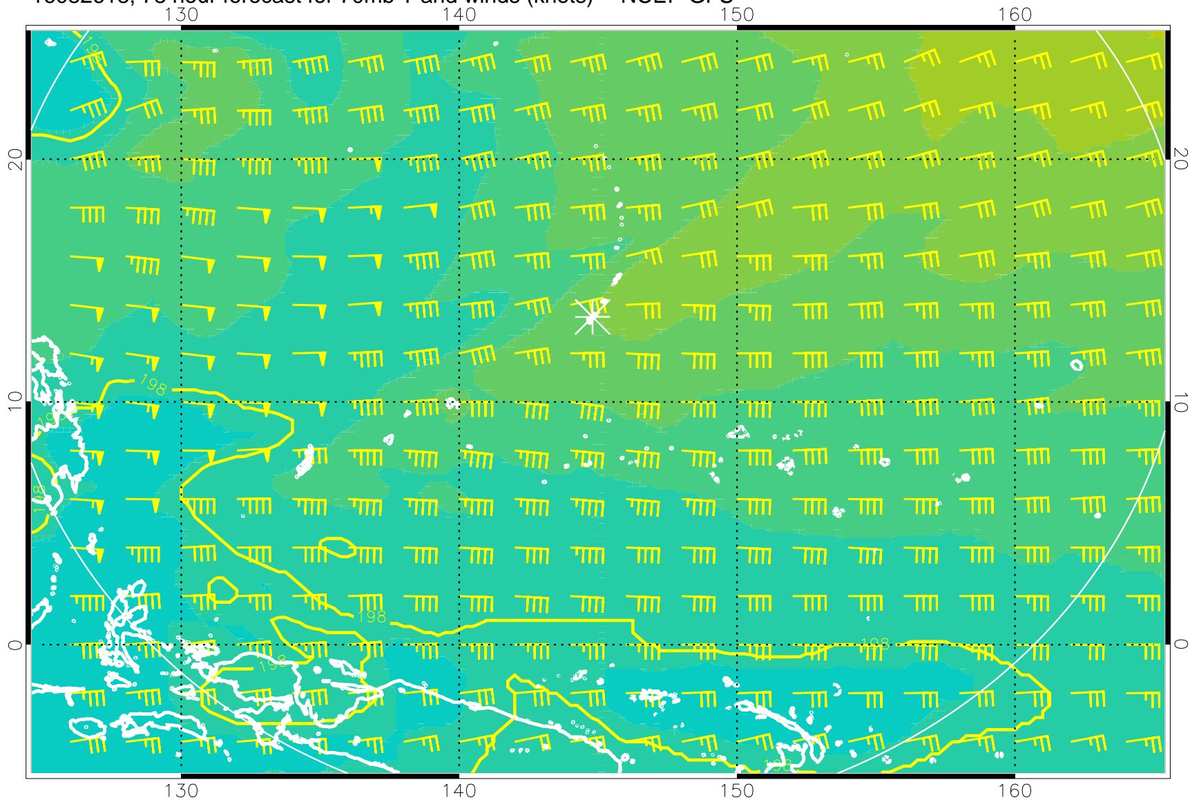
16082618, 78 hour forecast for 70mb T and winds (knots) -- NCEP GFS
