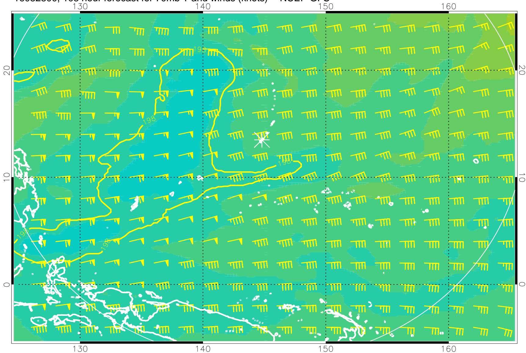
16082800, 108 hour forecast for 70mb T and winds (knots) -- NCEP GFS
