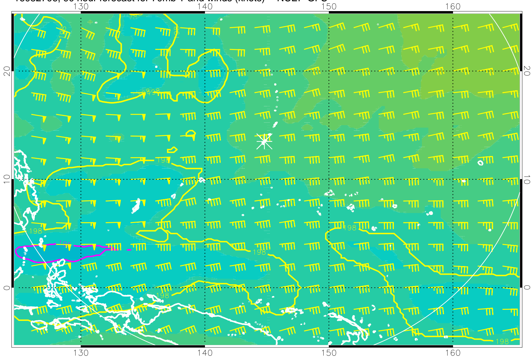
16082706, 90 hour forecast for 70mb T and winds (knots) -- NCEP GFS
