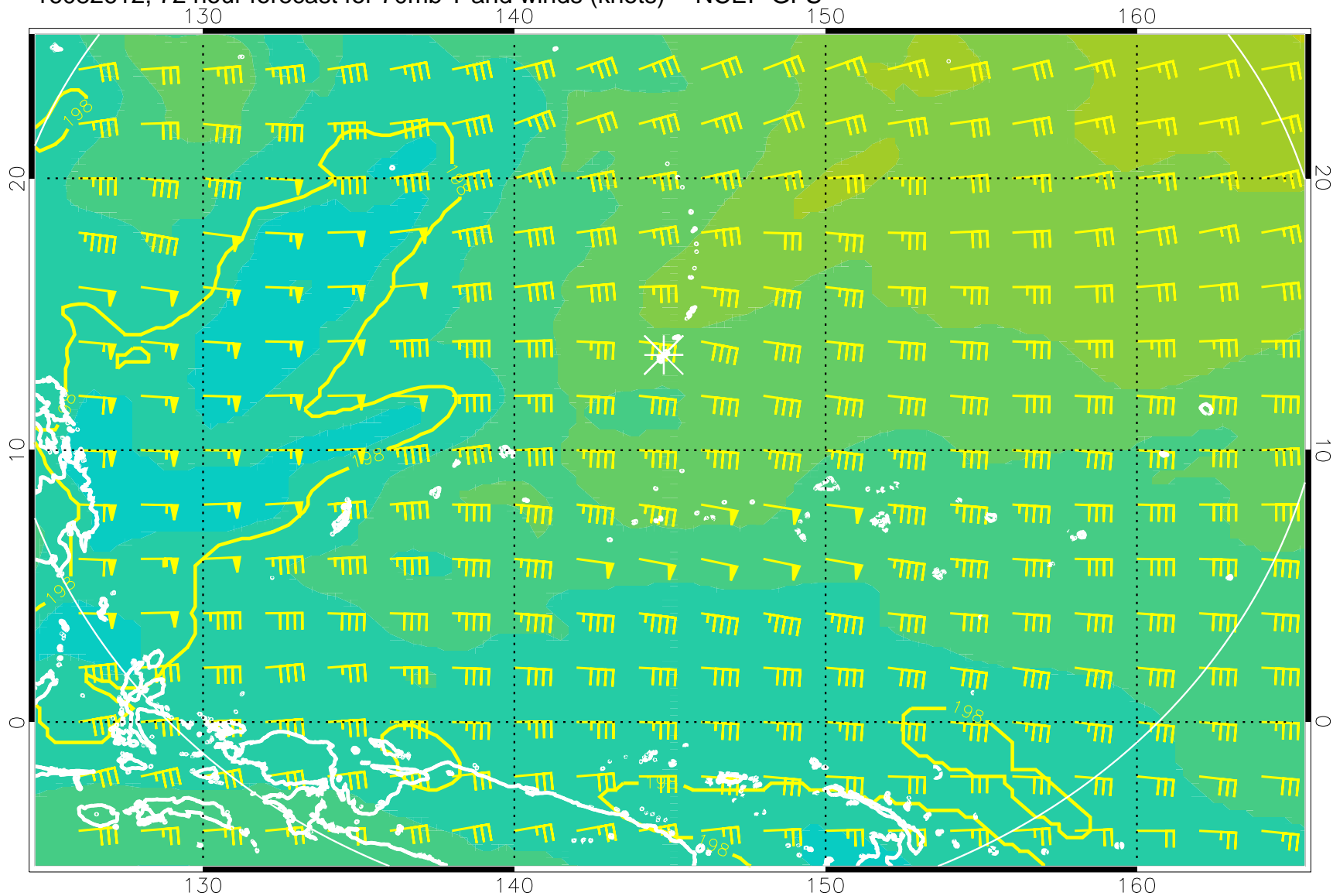
16082612, 72 hour forecast for 70mb T and winds (knots) -- NCEP GFS
