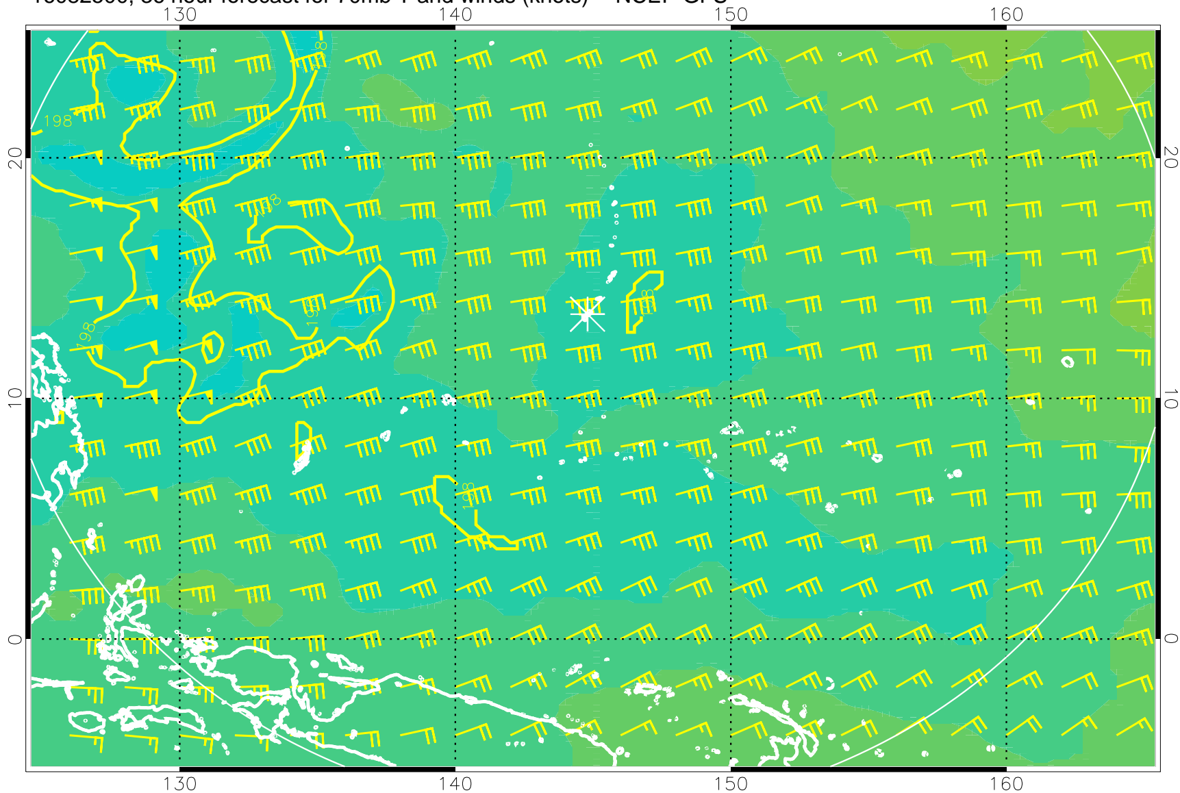
16082500, 36 hour forecast for 70mb T and winds (knots) -- NCEP GFS
