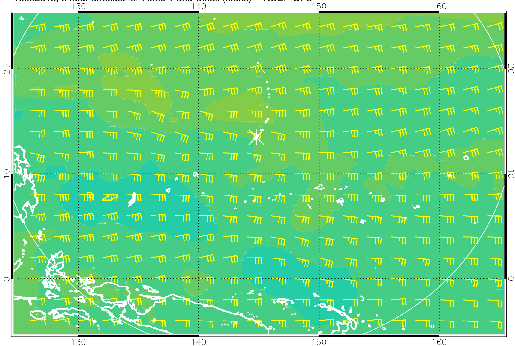
16082318, 6 hour forecast for 70mb T and winds (knots) -- NCEP GFS
