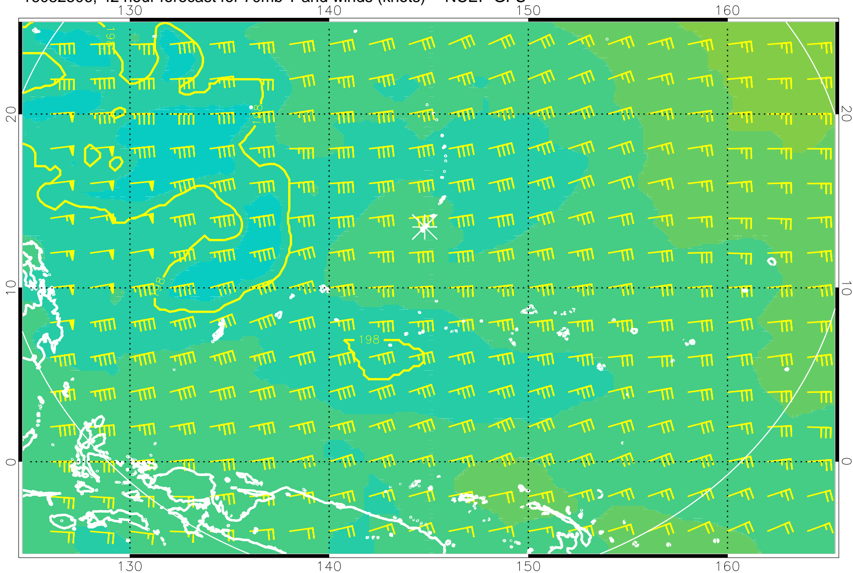
16082506, 42 hour forecast for 70mb T and winds (knots) -- NCEP GFS
