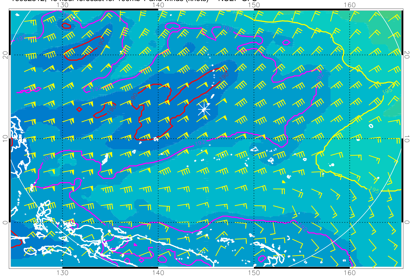
16082512, 48 hour forecast for 100mb T and winds (knots) -- NCEP GFS
