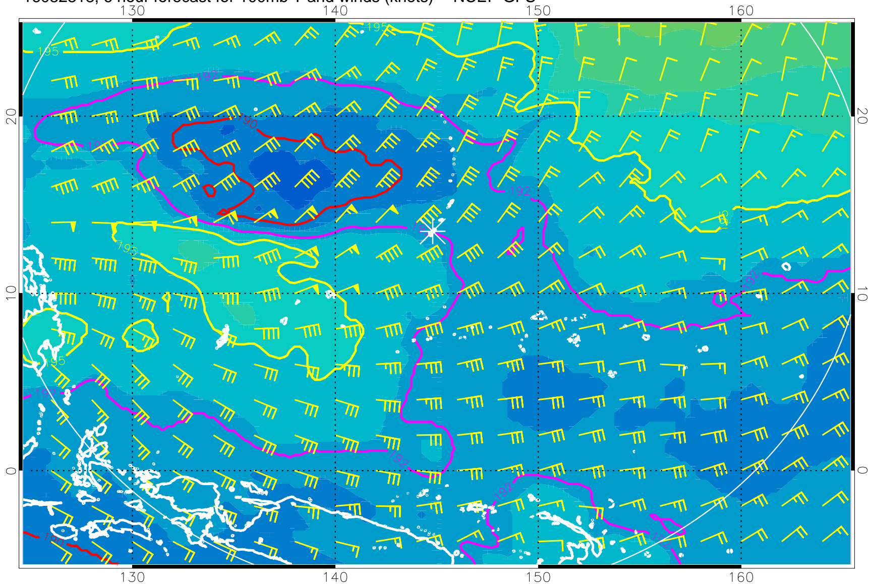
16082318, 6 hour forecast for 100mb T and winds (knots) -- NCEP GFS
