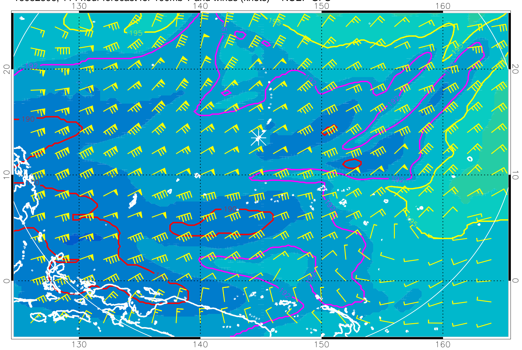
16082806, 114 hour forecast for 100mb T and winds (knots) -- NCEP GFS
