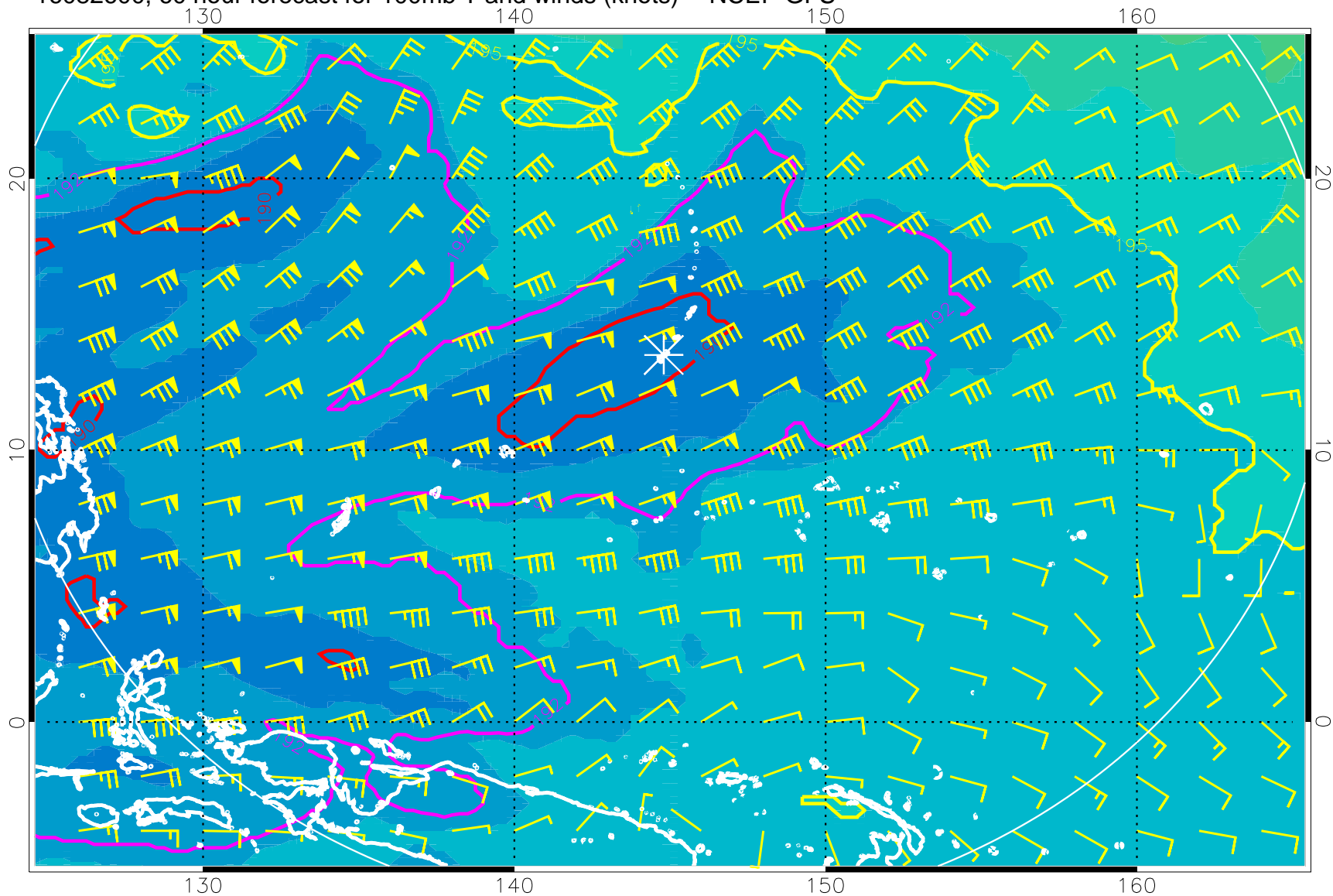
16082600, 60 hour forecast for 100mb T and winds (knots) -- NCEP GFS
