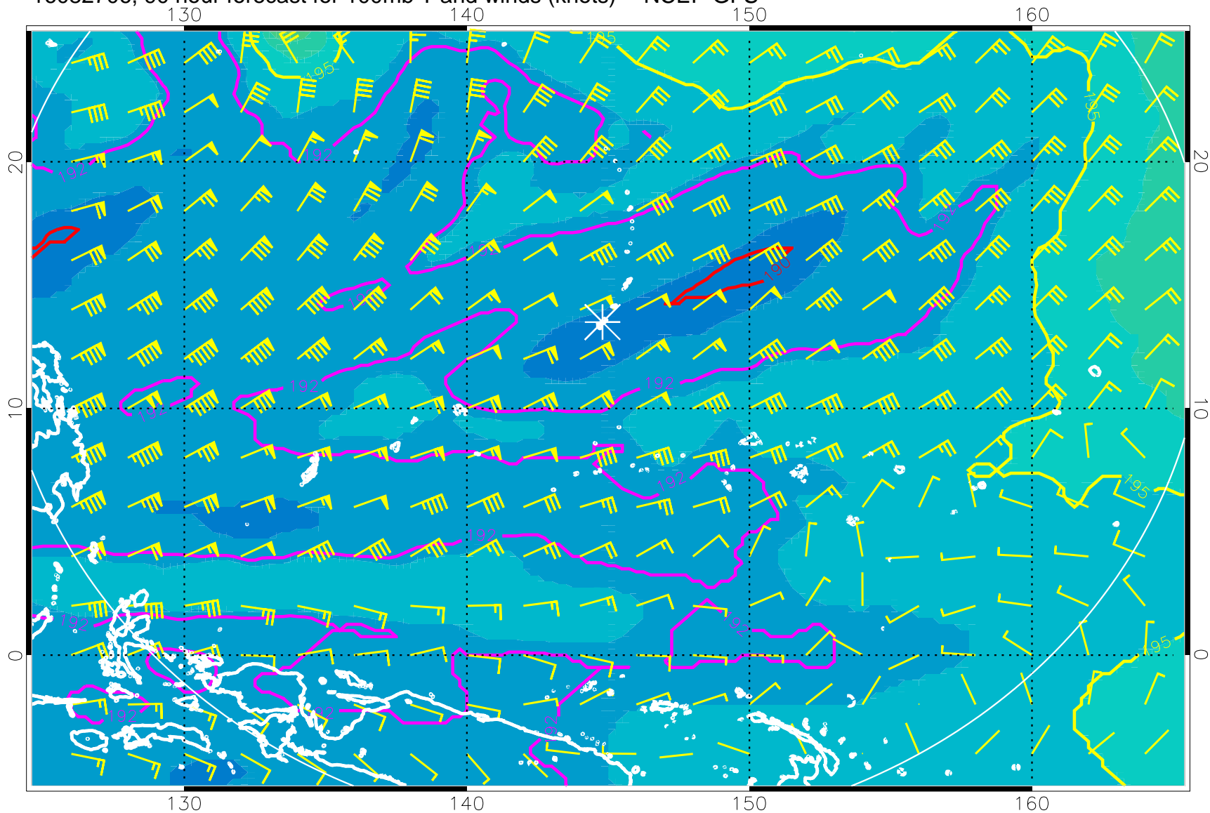
16082706, 90 hour forecast for 100mb T and winds (knots) -- NCEP GFS
