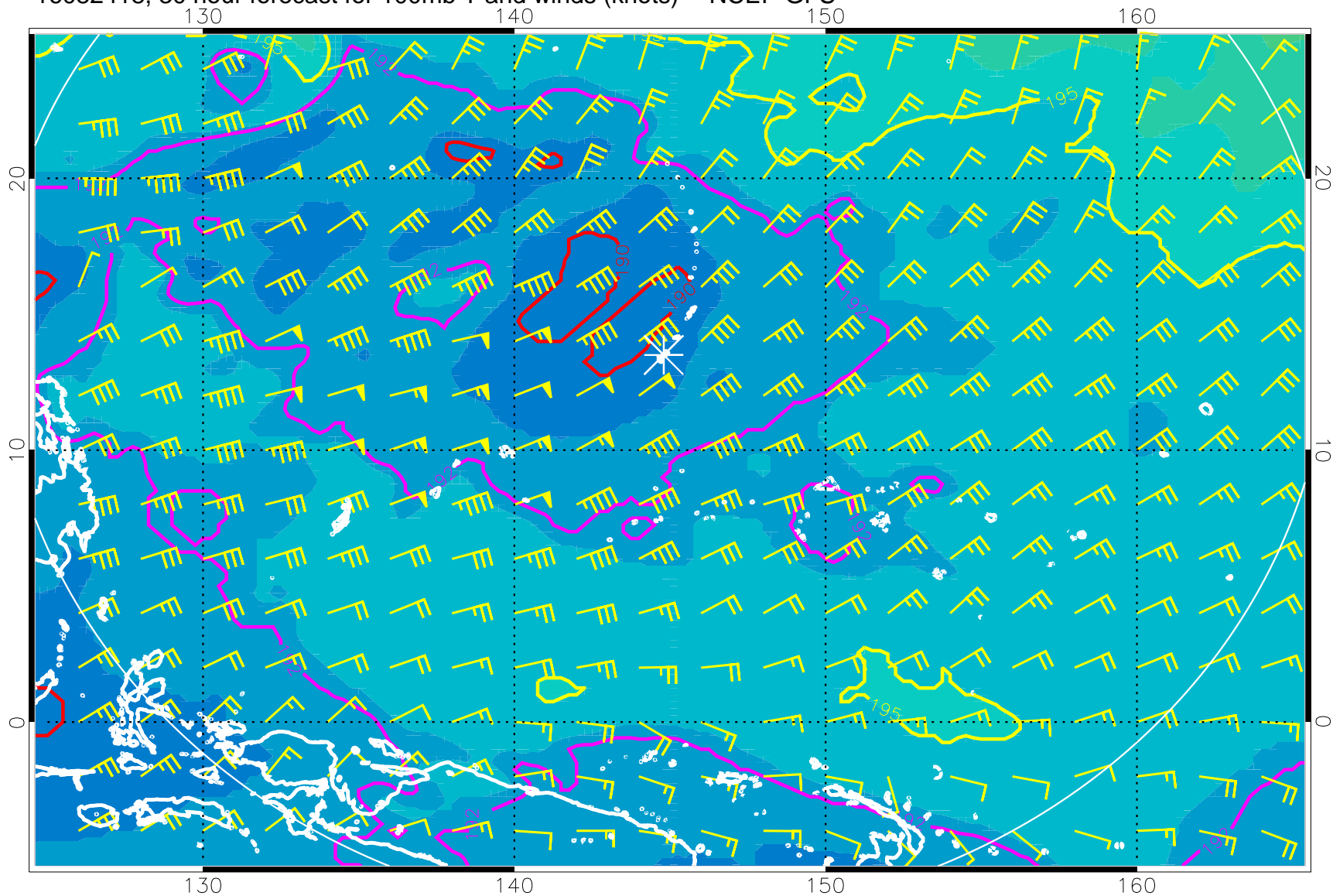
16082418, 30 hour forecast for 100mb T and winds (knots) -- NCEP GFS
