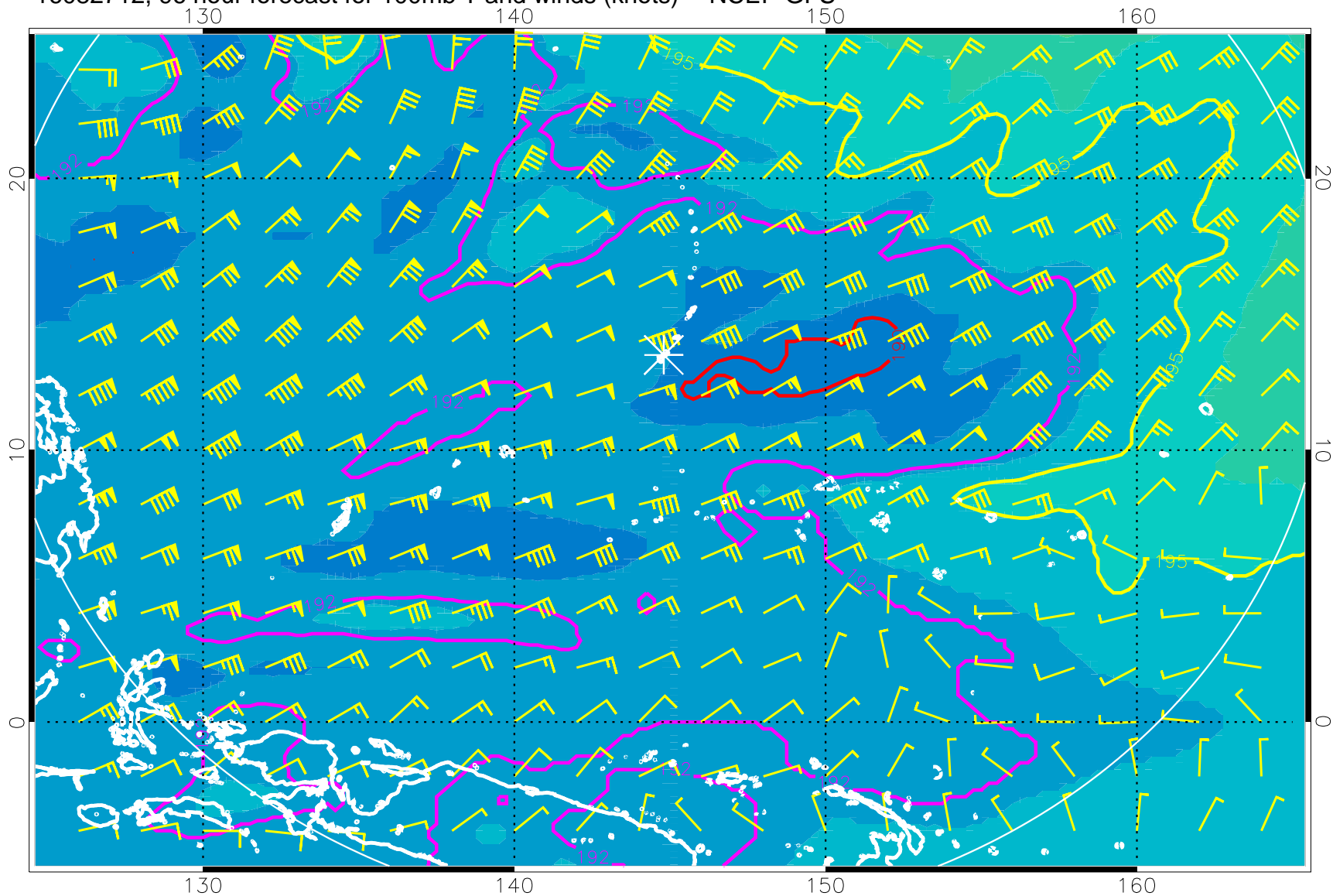
16082712, 96 hour forecast for 100mb T and winds (knots) -- NCEP GFS
