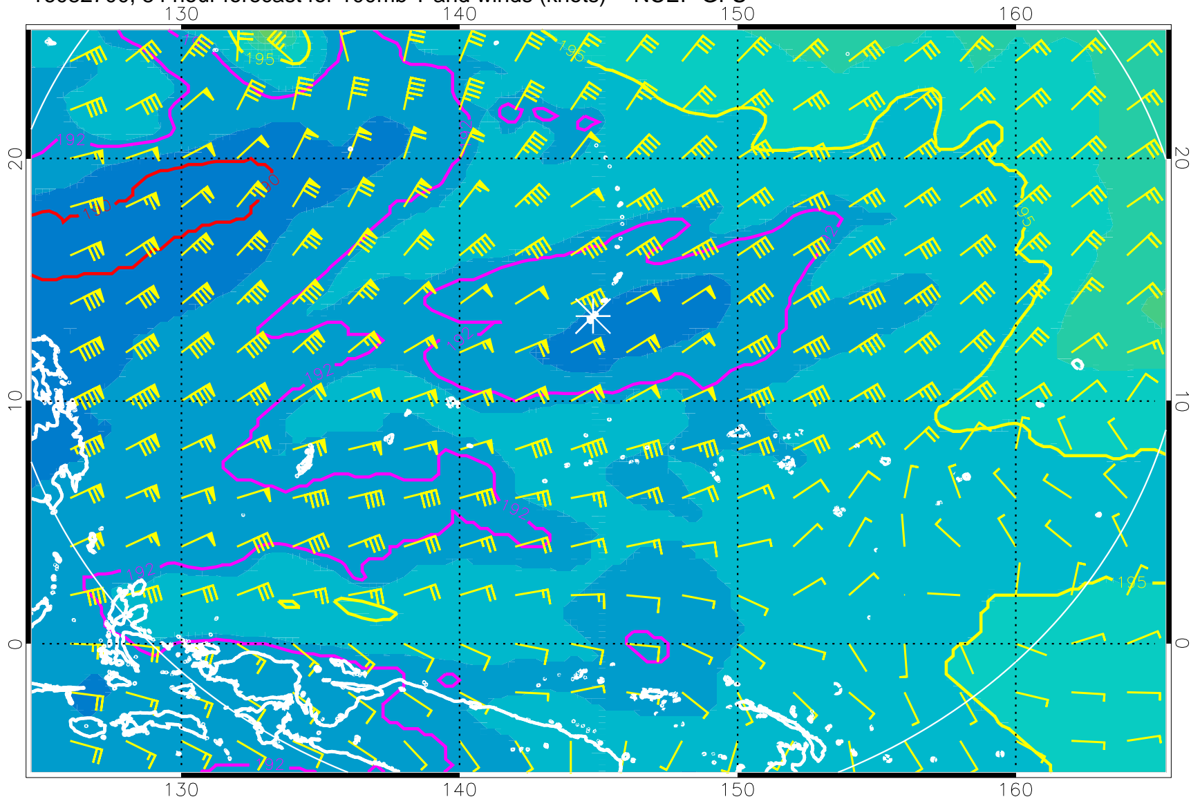
16082700, 84 hour forecast for 100mb T and winds (knots) -- NCEP GFS
