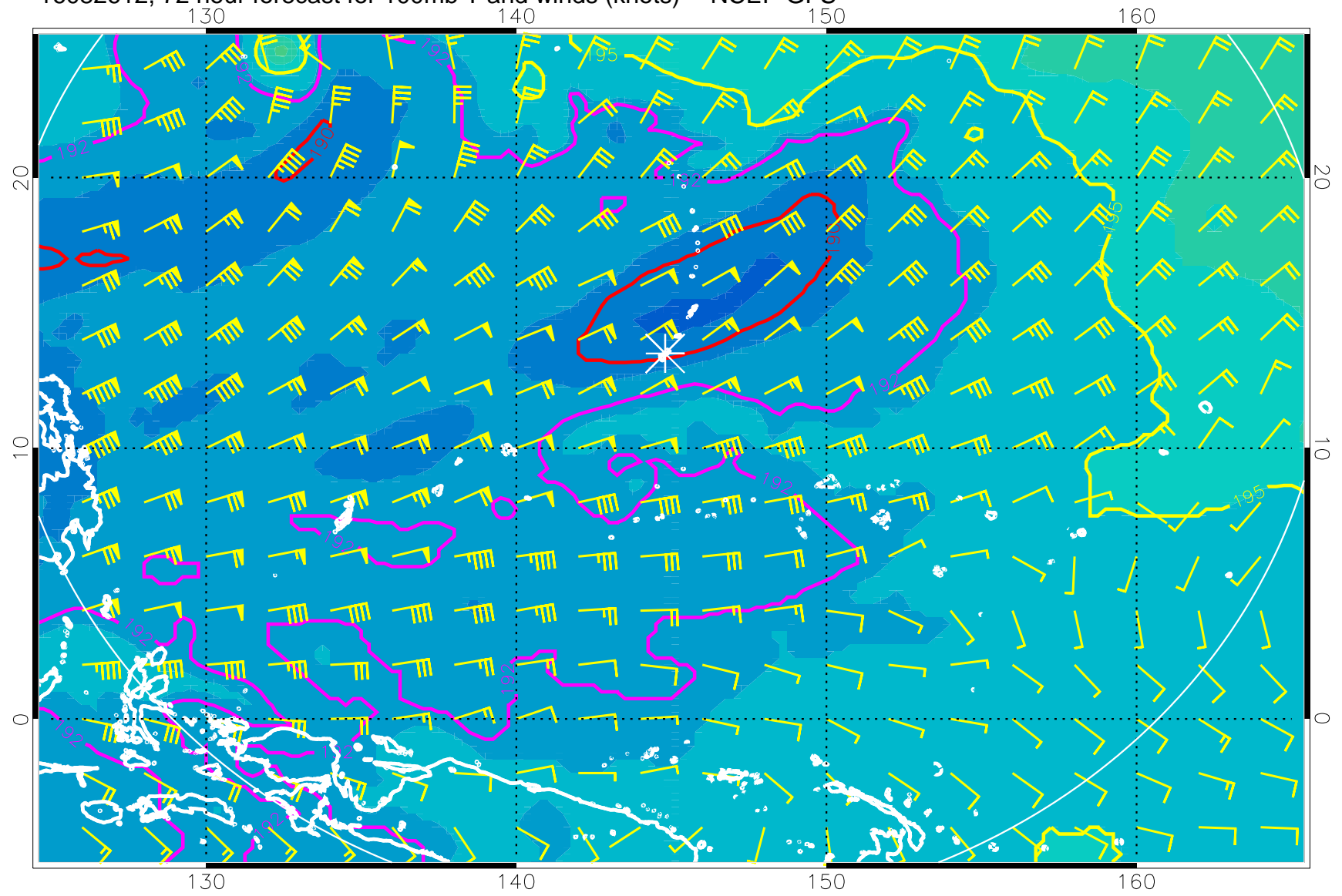
16082612, 72 hour forecast for 100mb T and winds (knots) -- NCEP GFS
