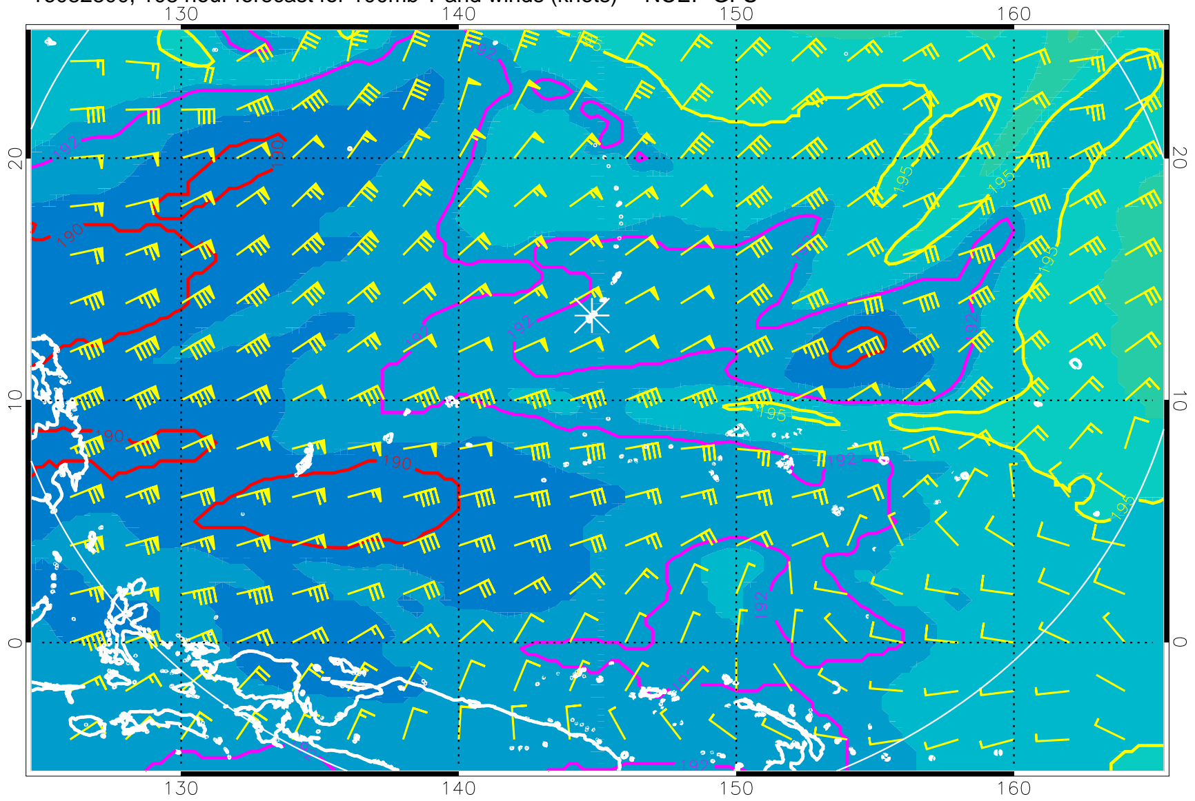
16082800, 108 hour forecast for 100mb T and winds (knots) -- NCEP GFS
