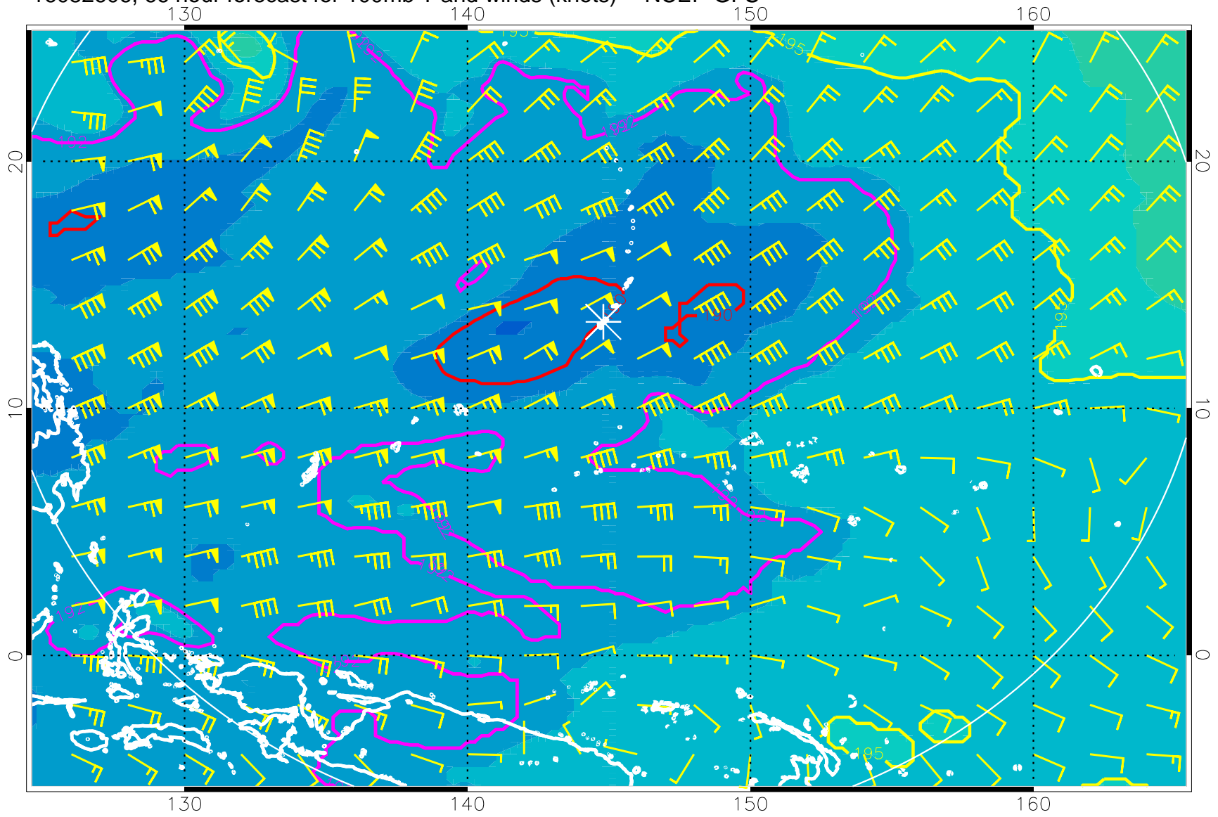
16082606, 66 hour forecast for 100mb T and winds (knots) -- NCEP GFS
