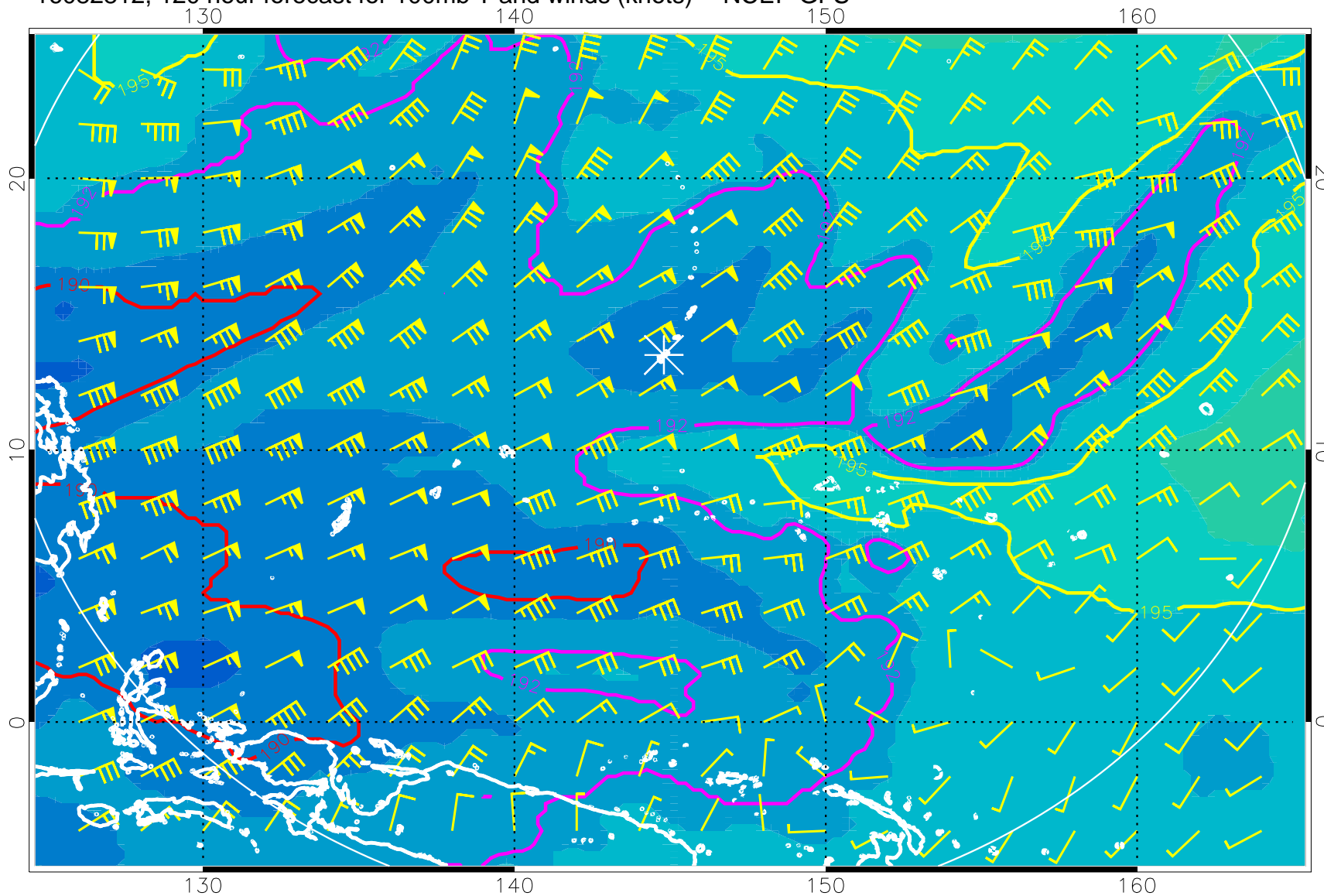
16082812, 120 hour forecast for 100mb T and winds (knots) -- NCEP GFS
