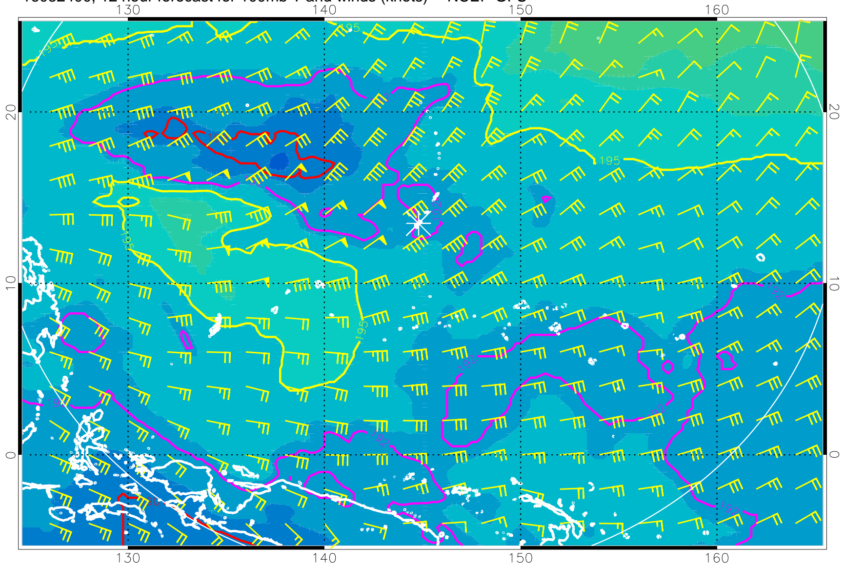
16082400, 12 hour forecast for 100mb T and winds (knots) -- NCEP GFS
