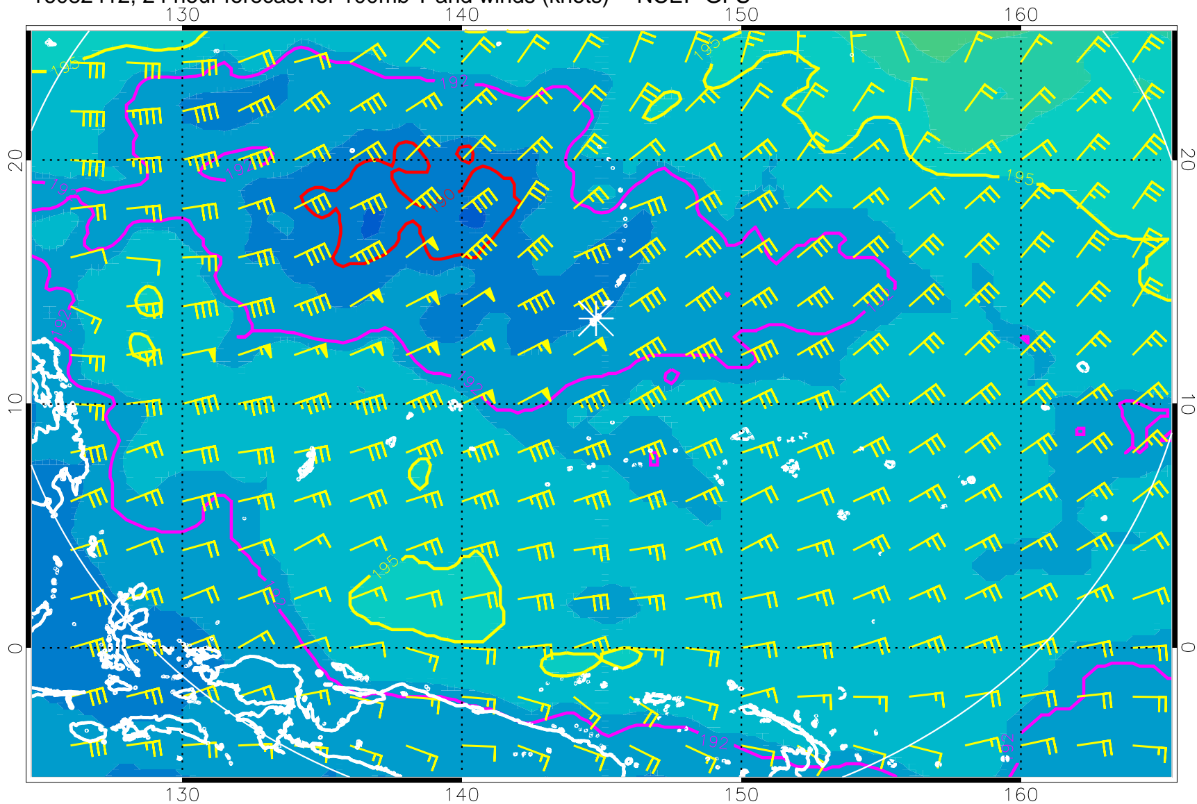
16082412, 24 hour forecast for 100mb T and winds (knots) -- NCEP GFS
