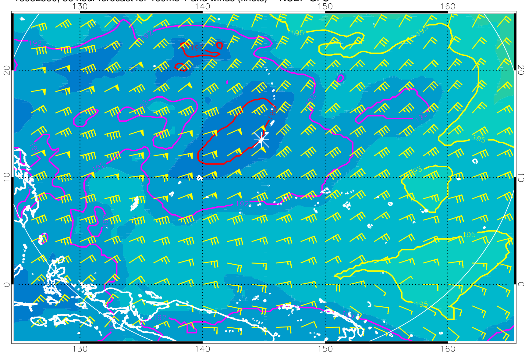
16082500, 36 hour forecast for 100mb T and winds (knots) -- NCEP GFS
