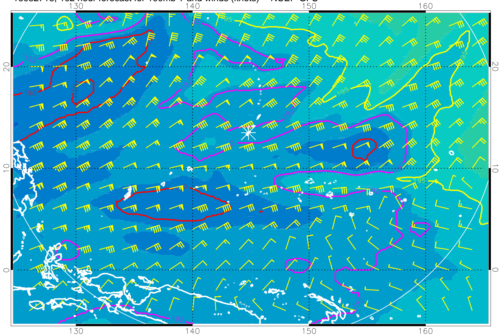
16082718, 102 hour forecast for 100mb T and winds (knots) -- NCEP GFS
