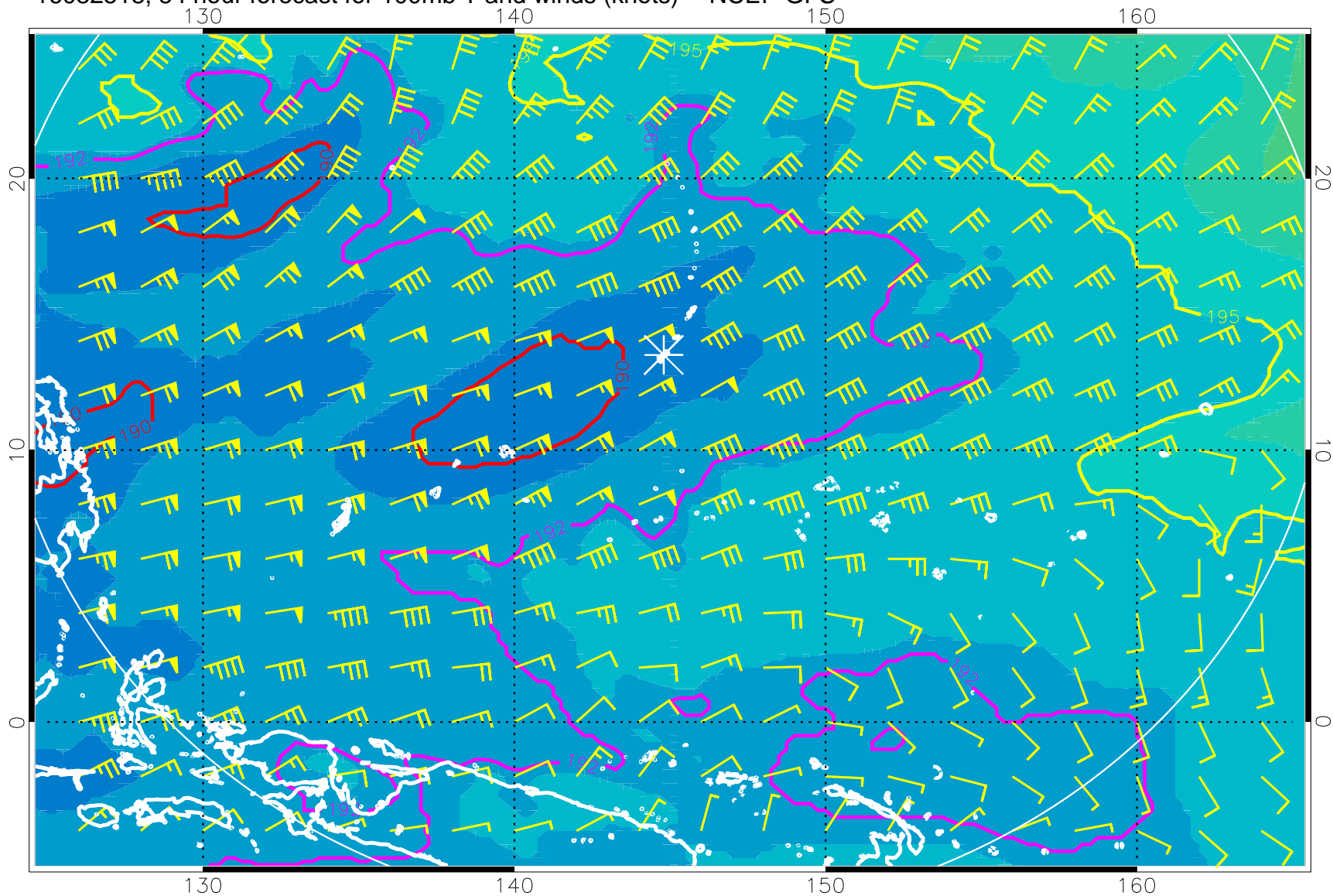
16082518, 54 hour forecast for 100mb T and winds (knots) -- NCEP GFS
