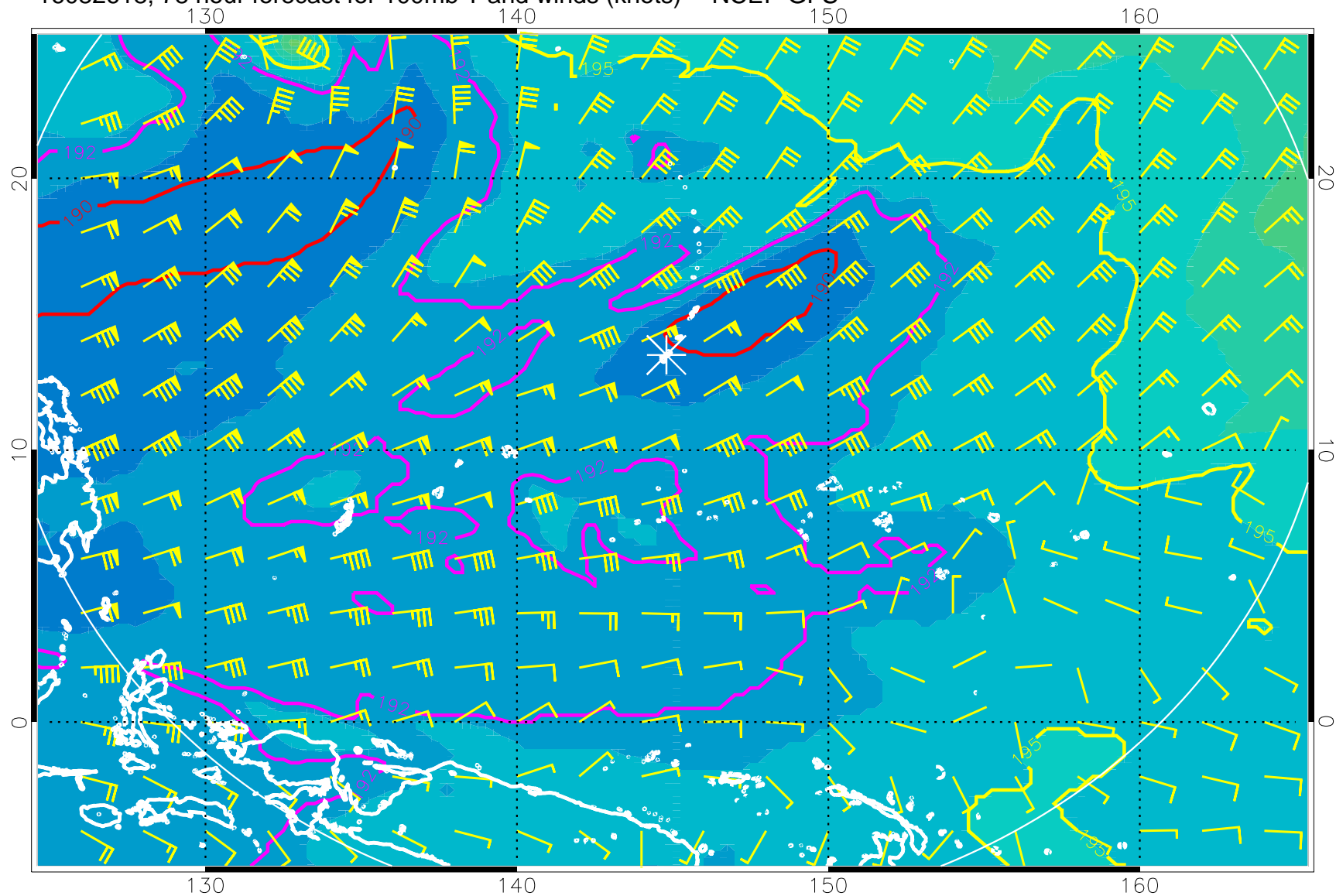
16082618, 78 hour forecast for 100mb T and winds (knots) -- NCEP GFS
