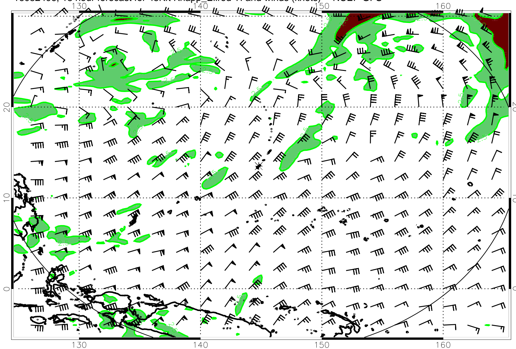
16082406, 18 hour forecast for 45Kft Knapp_Ellrod TI and winds (knots) -- NCEP GFS
