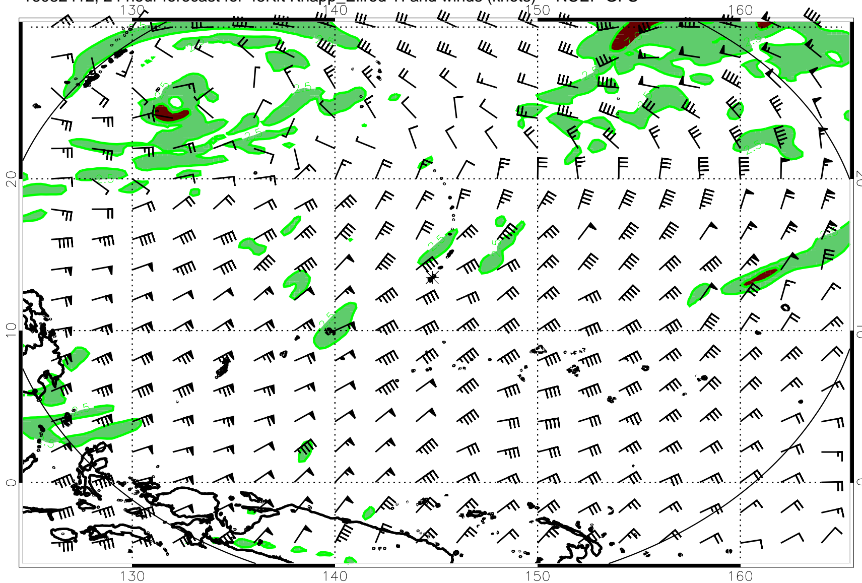
16082412, 24 hour forecast for 45Kft Knapp_Ellrod TI and winds (knots) -- NCEP GFS
