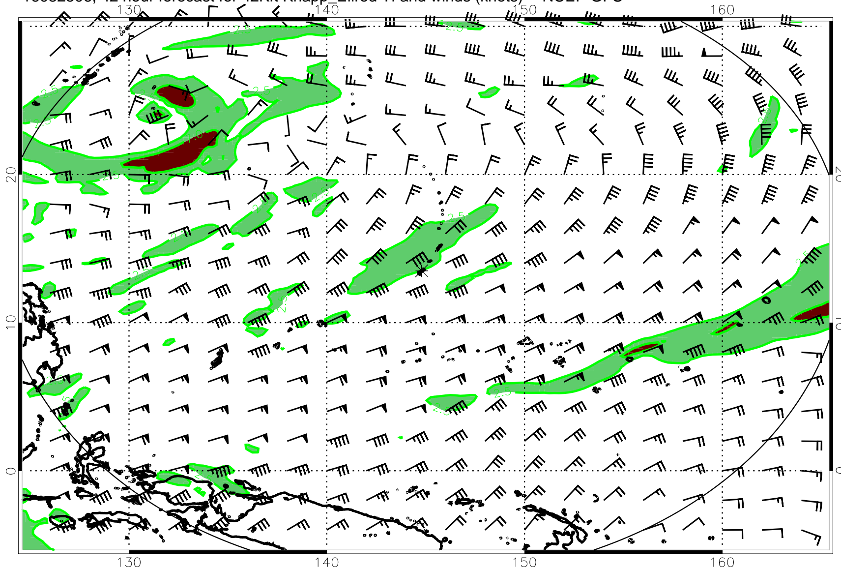
16082506, 42 hour forecast for 42Kft Knapp_Ellrod TI and winds (knots) -- NCEP GFS
