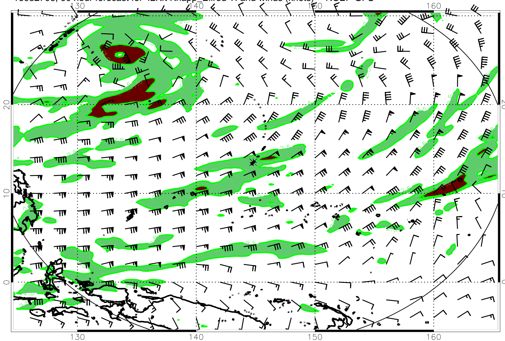
16082706, 90 hour forecast for 42Kft Knapp_Ellrod TI and winds (knots) -- NCEP GFS
